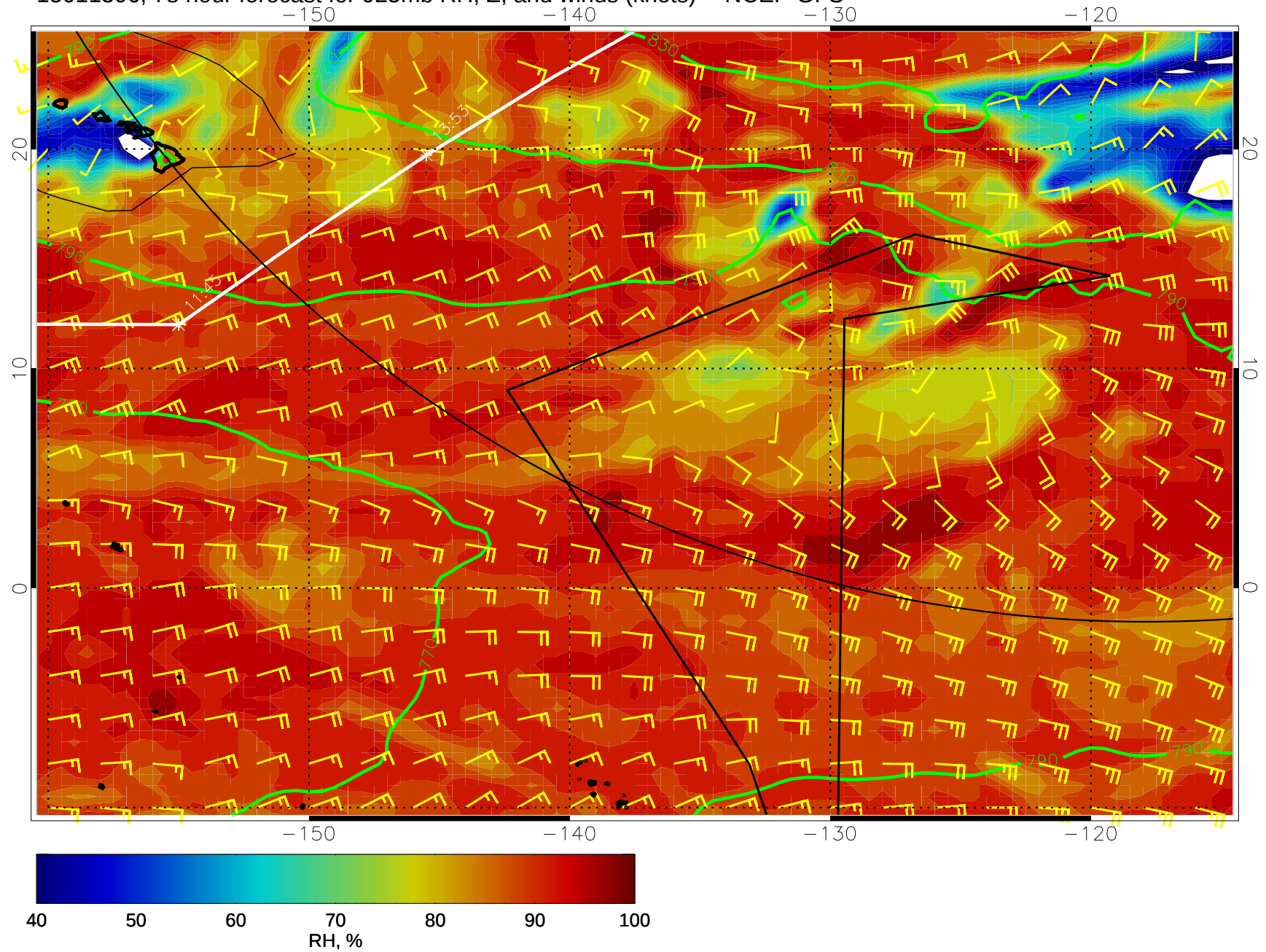
15011306, 78 hour forecast for 925mb RH, Z, and winds (knots) -- NCEP GFS
