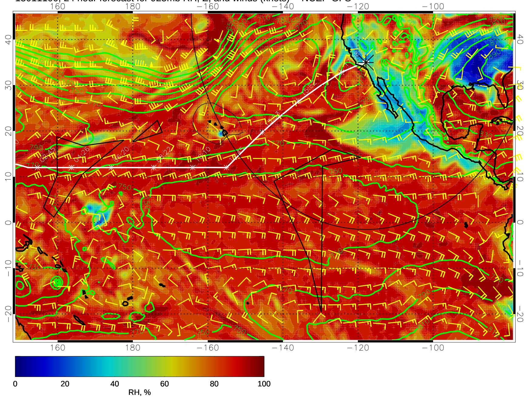
15011100, 24 hour forecast for 925mb RH, Z, and winds (knots) -- NCEP GFS
