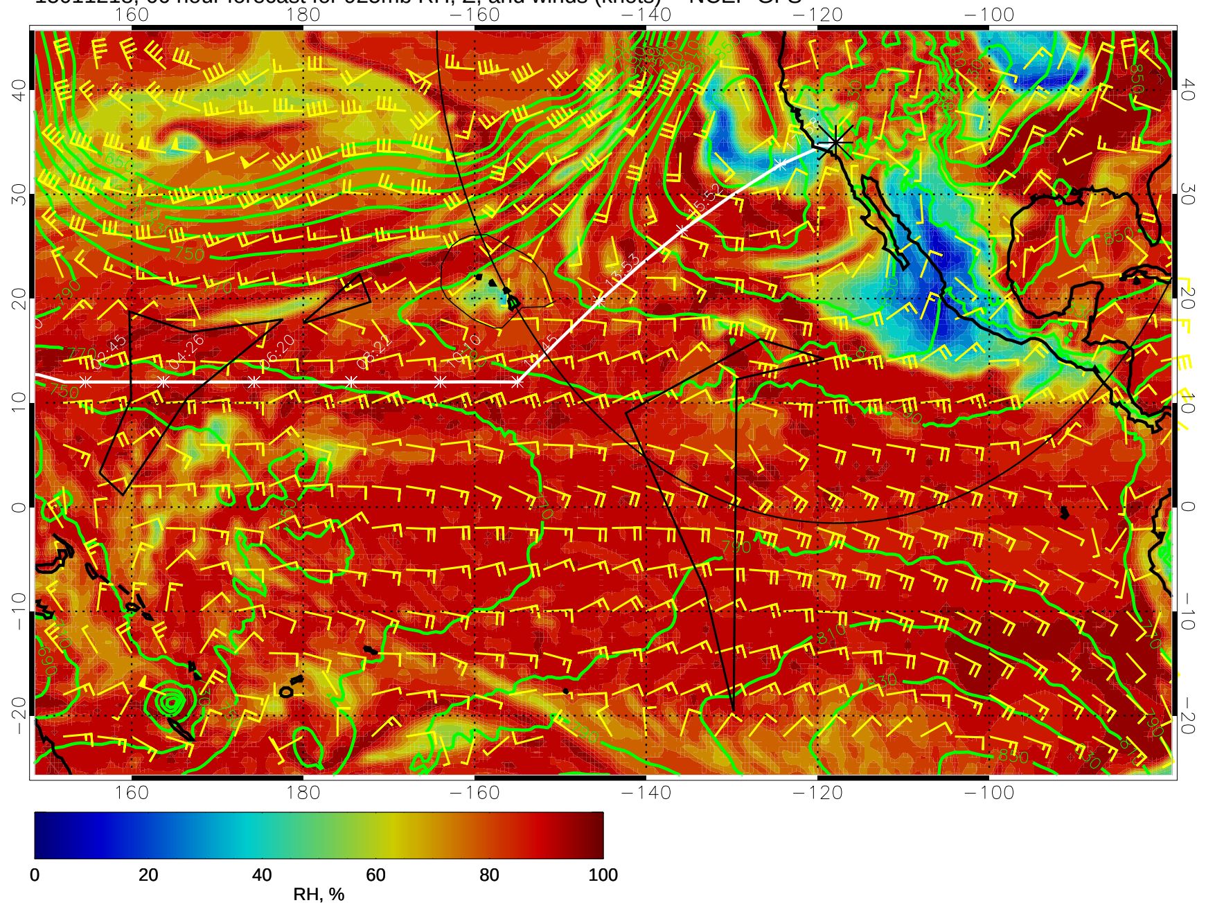
15011218, 66 hour forecast for 925mb RH, Z, and winds (knots) -- NCEP GFS
