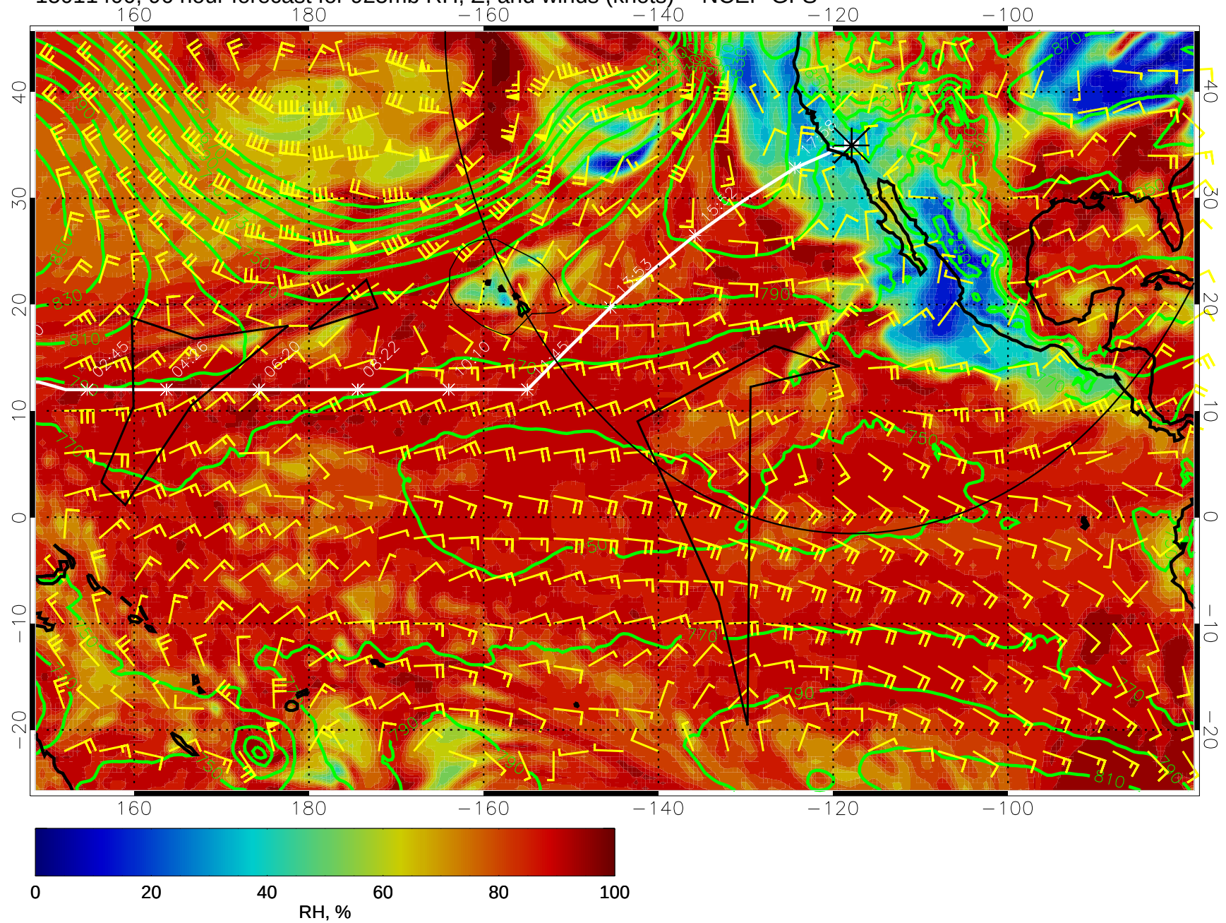
15011400, 96 hour forecast for 925mb RH, Z, and winds (knots) -- NCEP GFS
