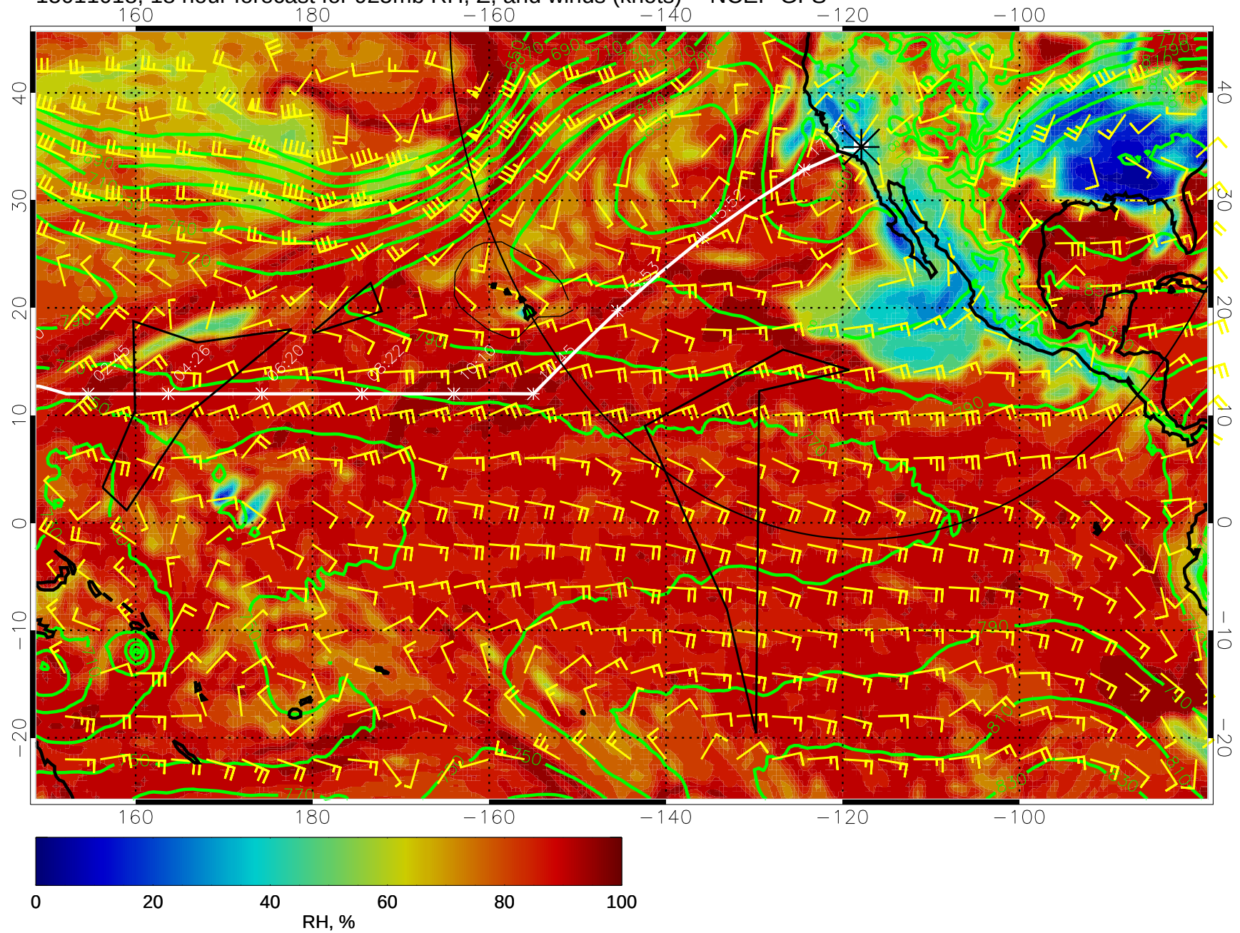
15011018, 18 hour forecast for 925mb RH, Z, and winds (knots) -- NCEP GFS
