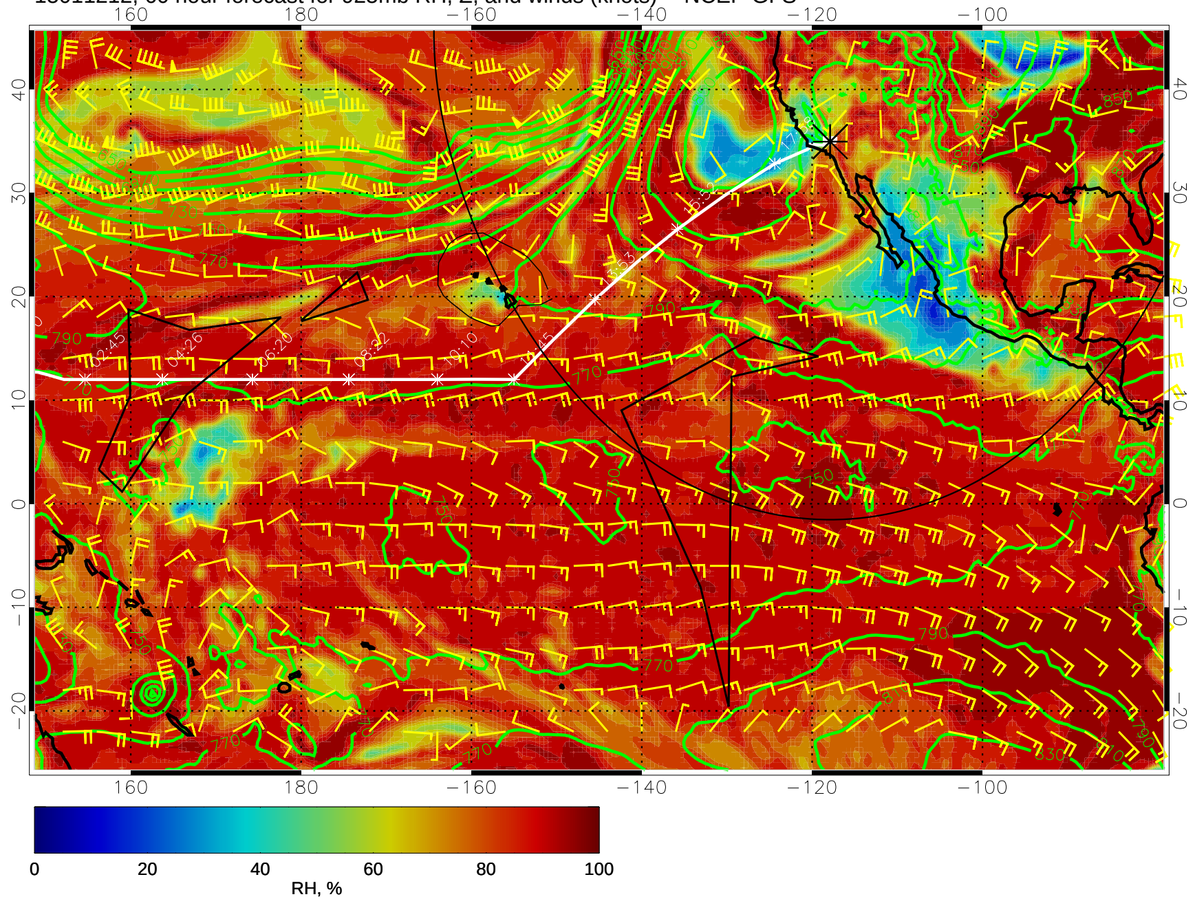
15011212, 60 hour forecast for 925mb RH, Z, and winds (knots) -- NCEP GFS
