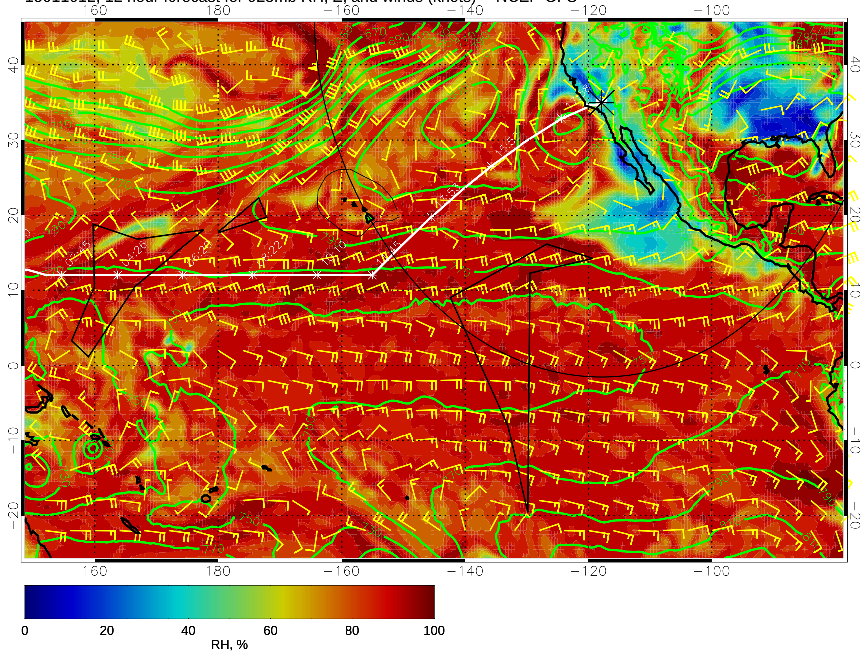
15011012, 12 hour forecast for 925mb RH, Z, and winds (knots) -- NCEP GFS
