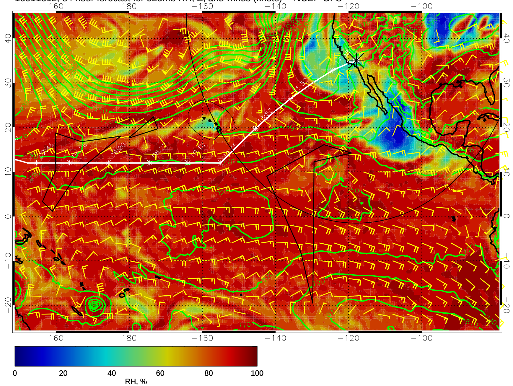
15011312, 84 hour forecast for 925mb RH, Z, and winds (knots) -- NCEP GFS
