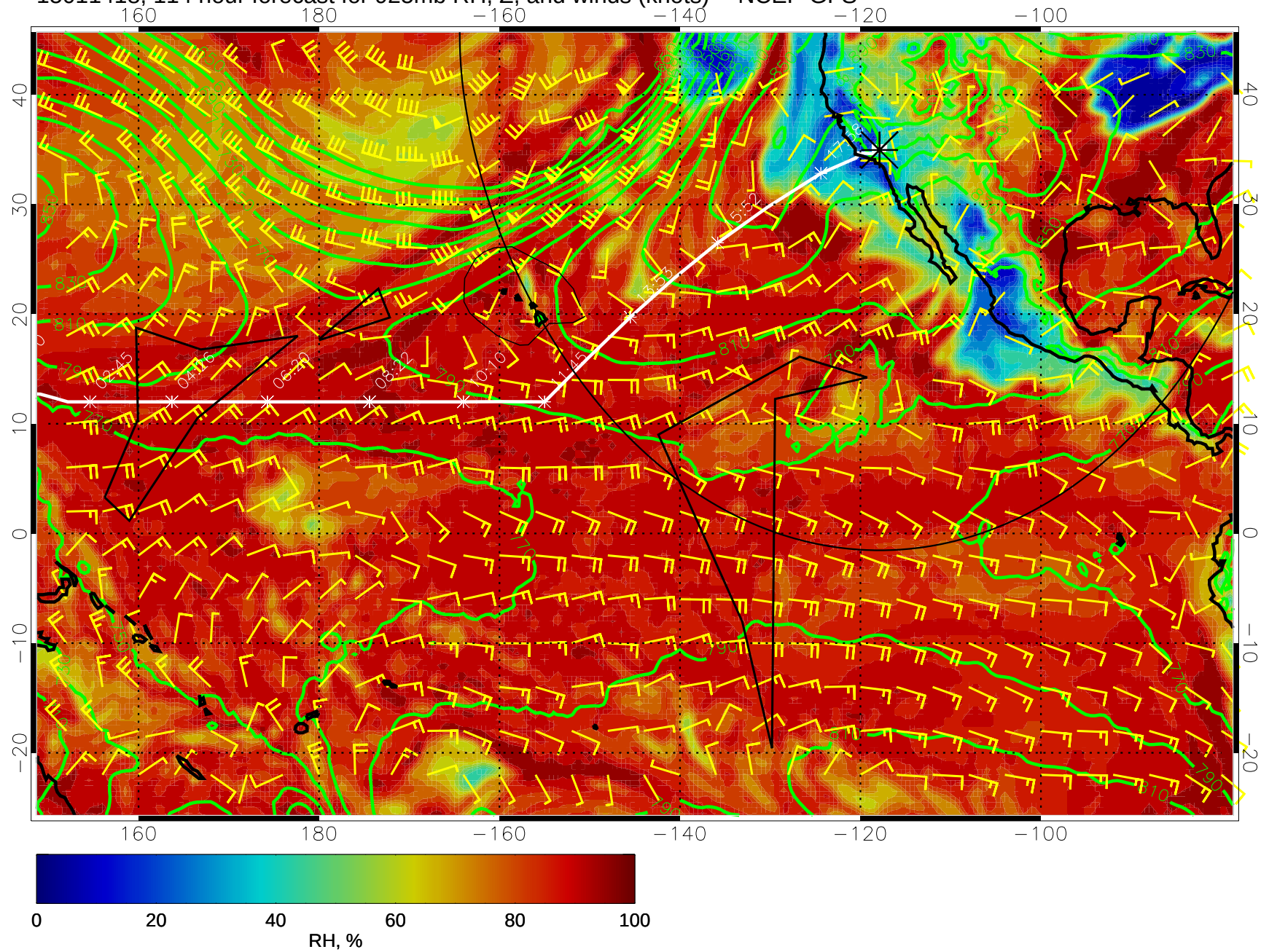
15011418, 114 hour forecast for 925mb RH, Z, and winds (knots) -- NCEP GFS
