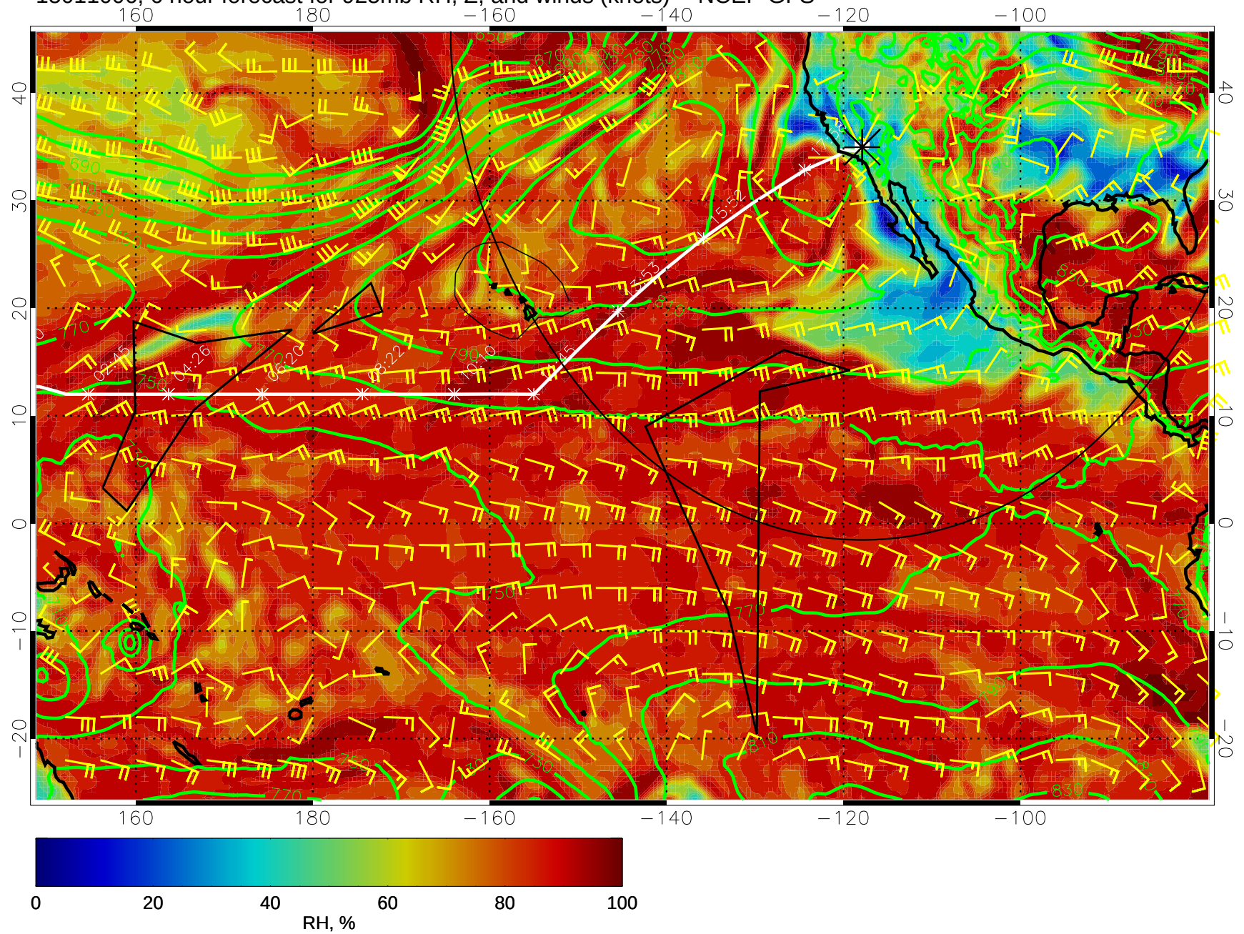
15011006, 6 hour forecast for 925mb RH, Z, and winds (knots) -- NCEP GFS
