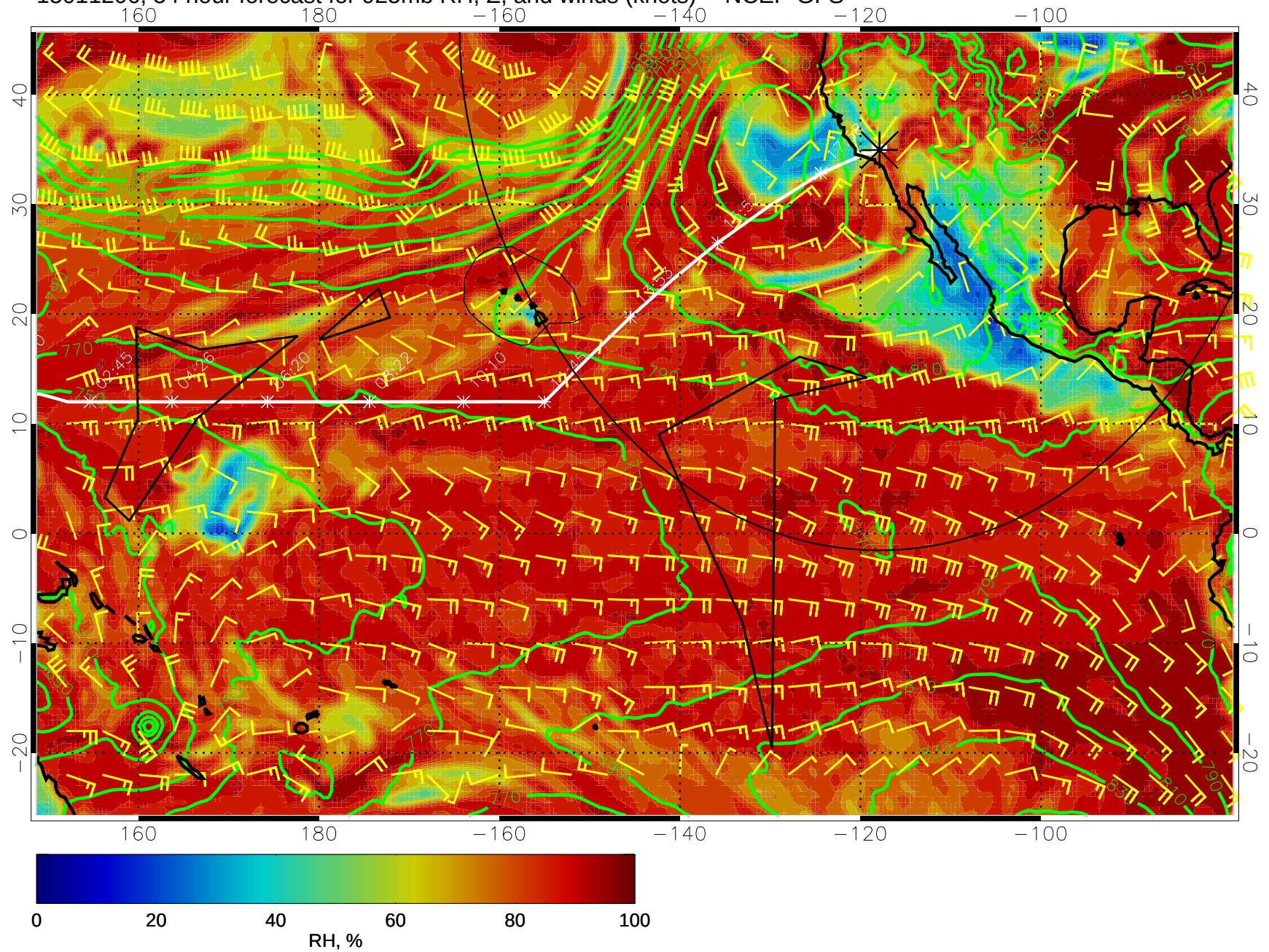
15011206, 54 hour forecast for 925mb RH, Z, and winds (knots) -- NCEP GFS
