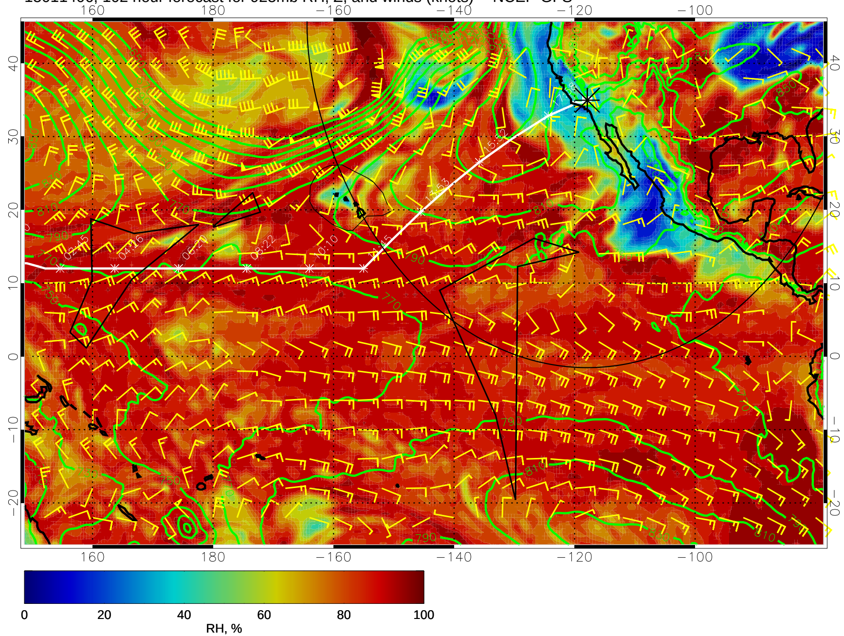
15011406, 102 hour forecast for 925mb RH, Z, and winds (knots) -- NCEP GFS
