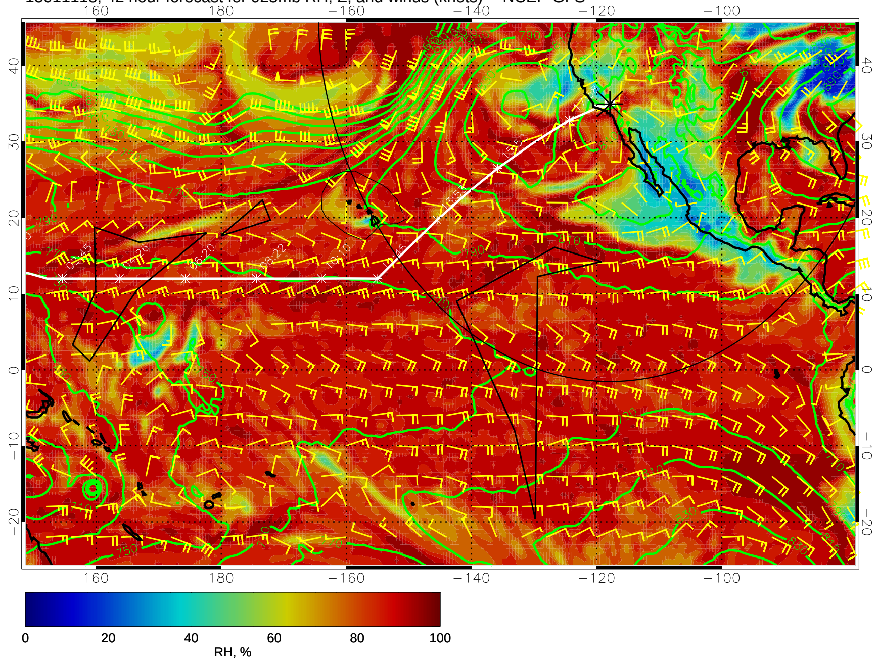
15011118, 42 hour forecast for 925mb RH, Z, and winds (knots) -- NCEP GFS
