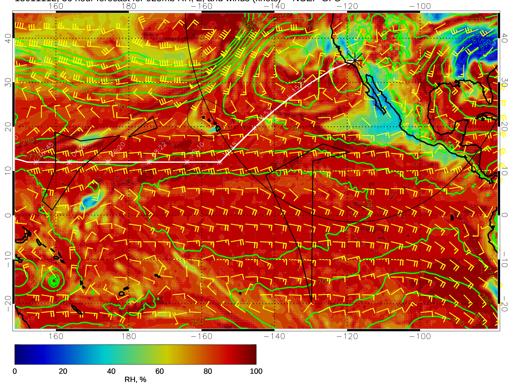
15011112, 36 hour forecast for 925mb RH, Z, and winds (knots) -- NCEP GFS
