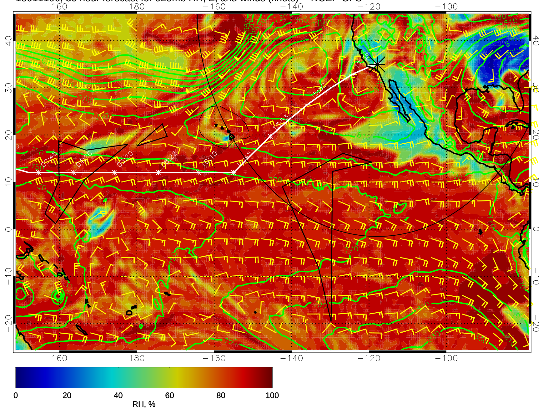
15011106, 30 hour forecast for 925mb RH, Z, and winds (knots) -- NCEP GFS
