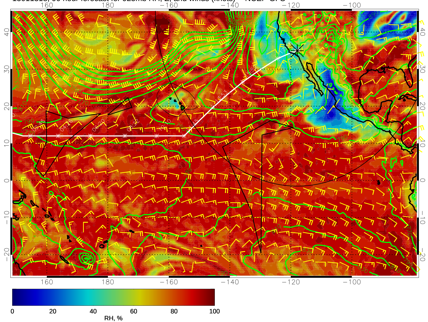
15011318, 90 hour forecast for 925mb RH, Z, and winds (knots) -- NCEP GFS
