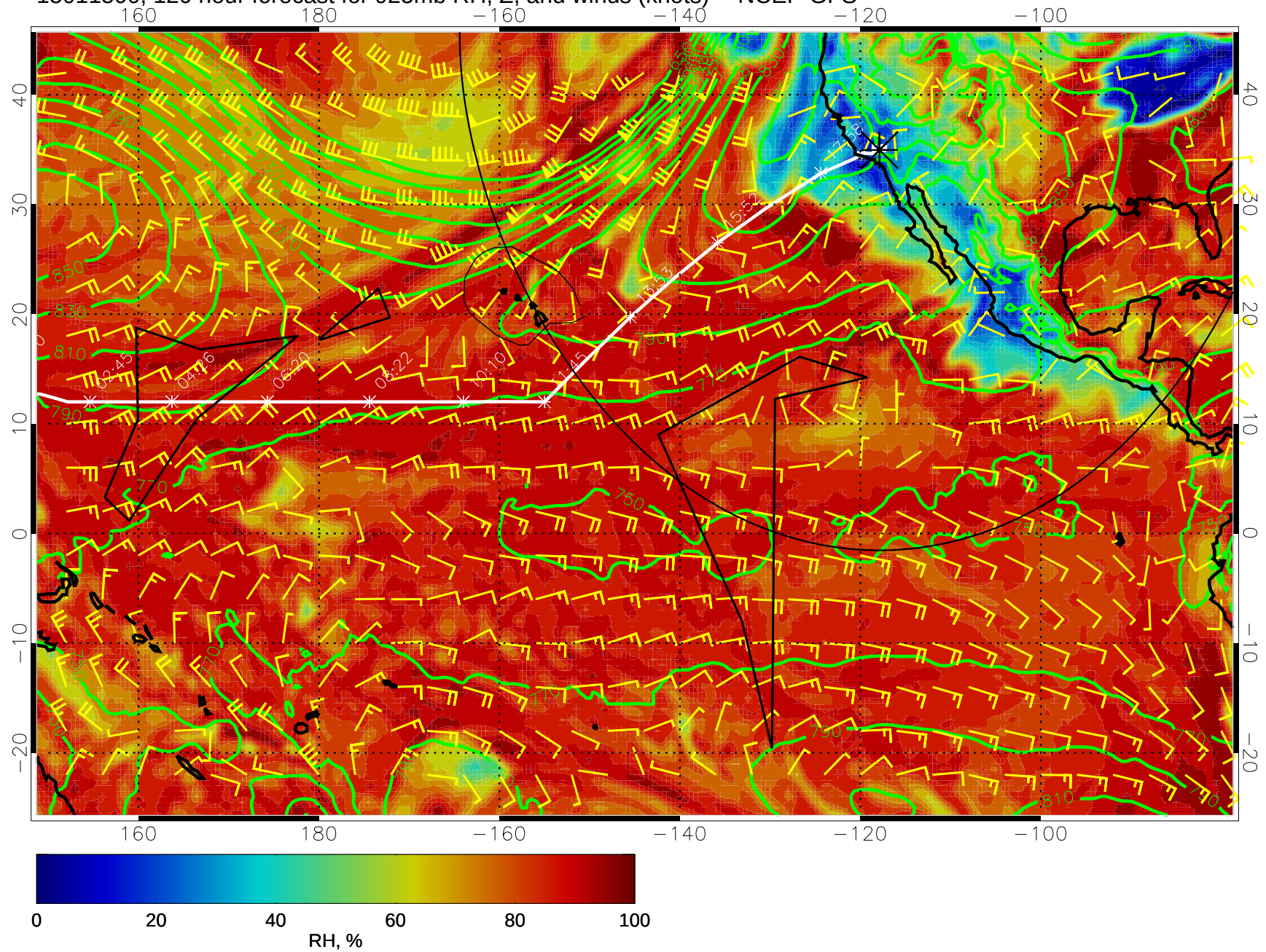
15011500, 120 hour forecast for 925mb RH, Z, and winds (knots) -- NCEP GFS
