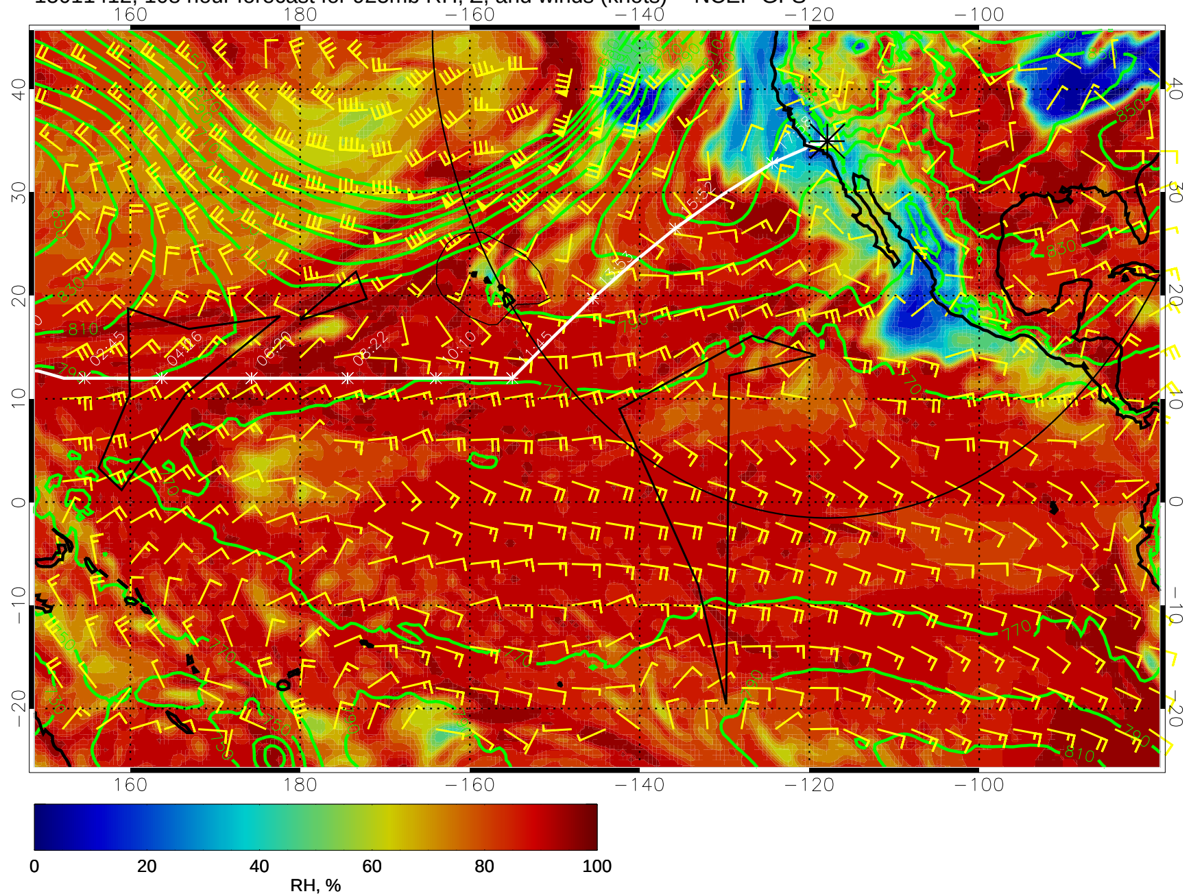
15011412, 108 hour forecast for 925mb RH, Z, and winds (knots) -- NCEP GFS
