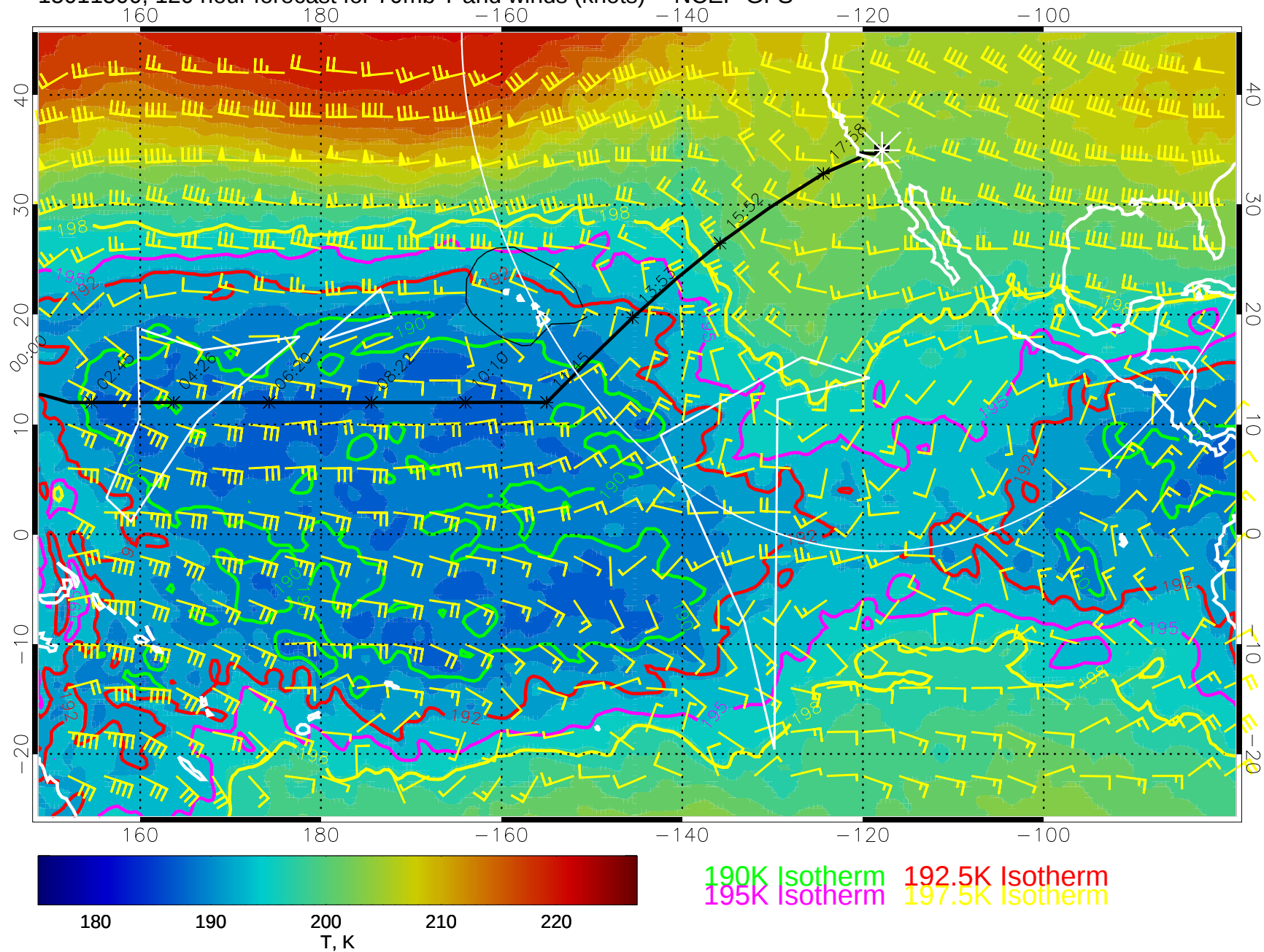
15011500, 120 hour forecast for 70mb T and winds (knots) -- NCEP GFS
