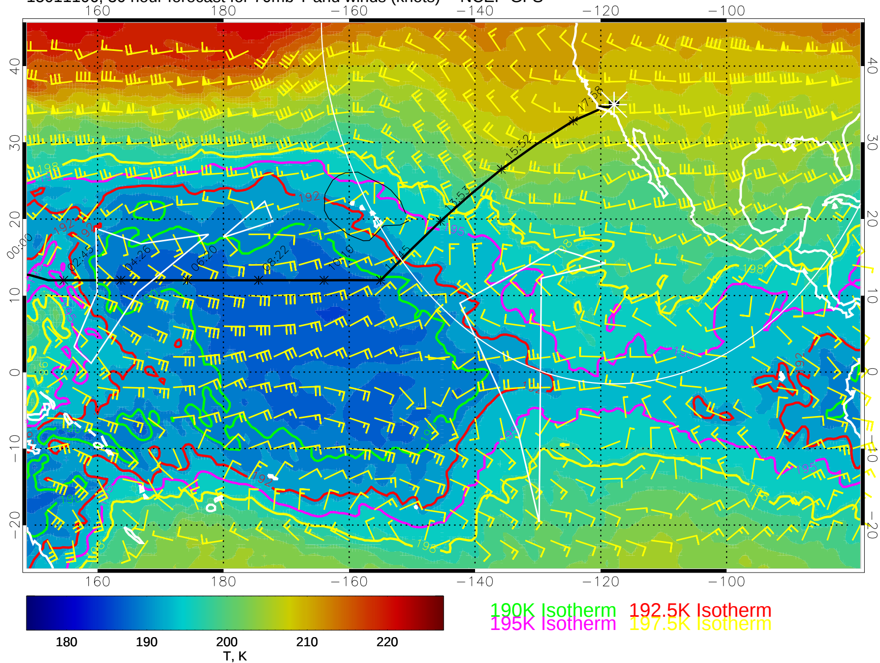
15011106, 30 hour forecast for 70mb T and winds (knots) -- NCEP GFS
