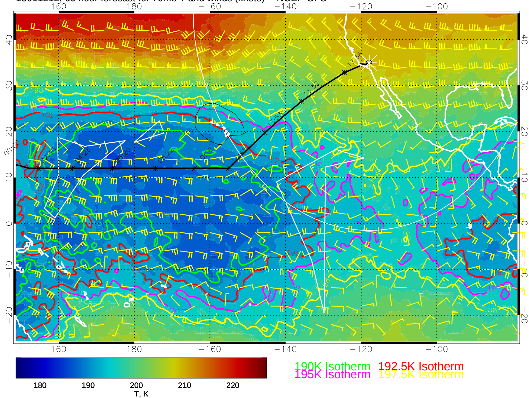
15011212, 60 hour forecast for 70mb T and winds (knots) -- NCEP GFS
