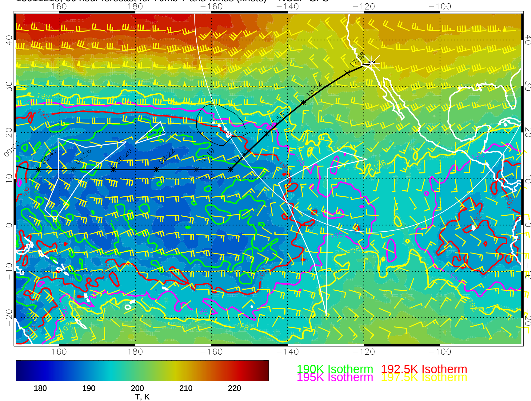
15011218, 66 hour forecast for 70mb T and winds (knots) -- NCEP GFS
