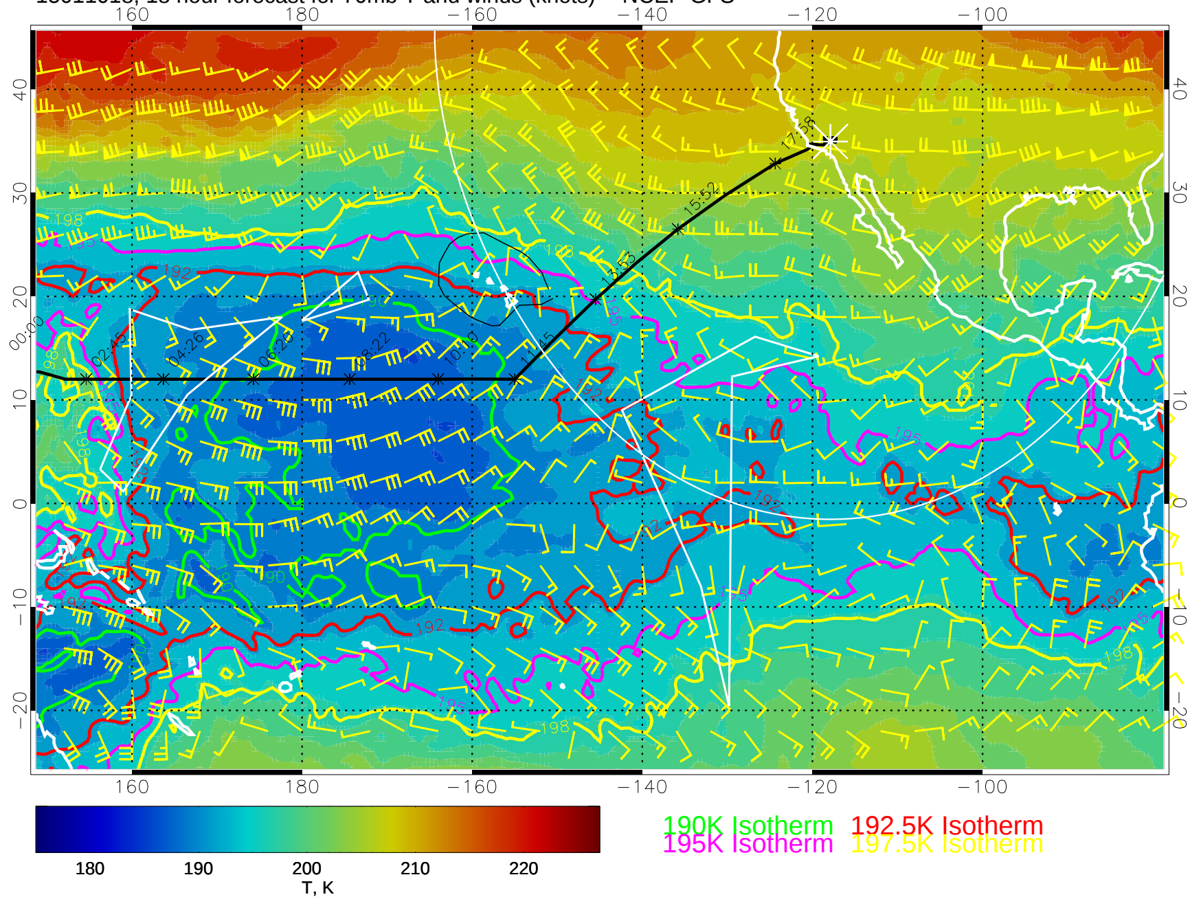
15011018, 18 hour forecast for 70mb T and winds (knots) -- NCEP GFS
