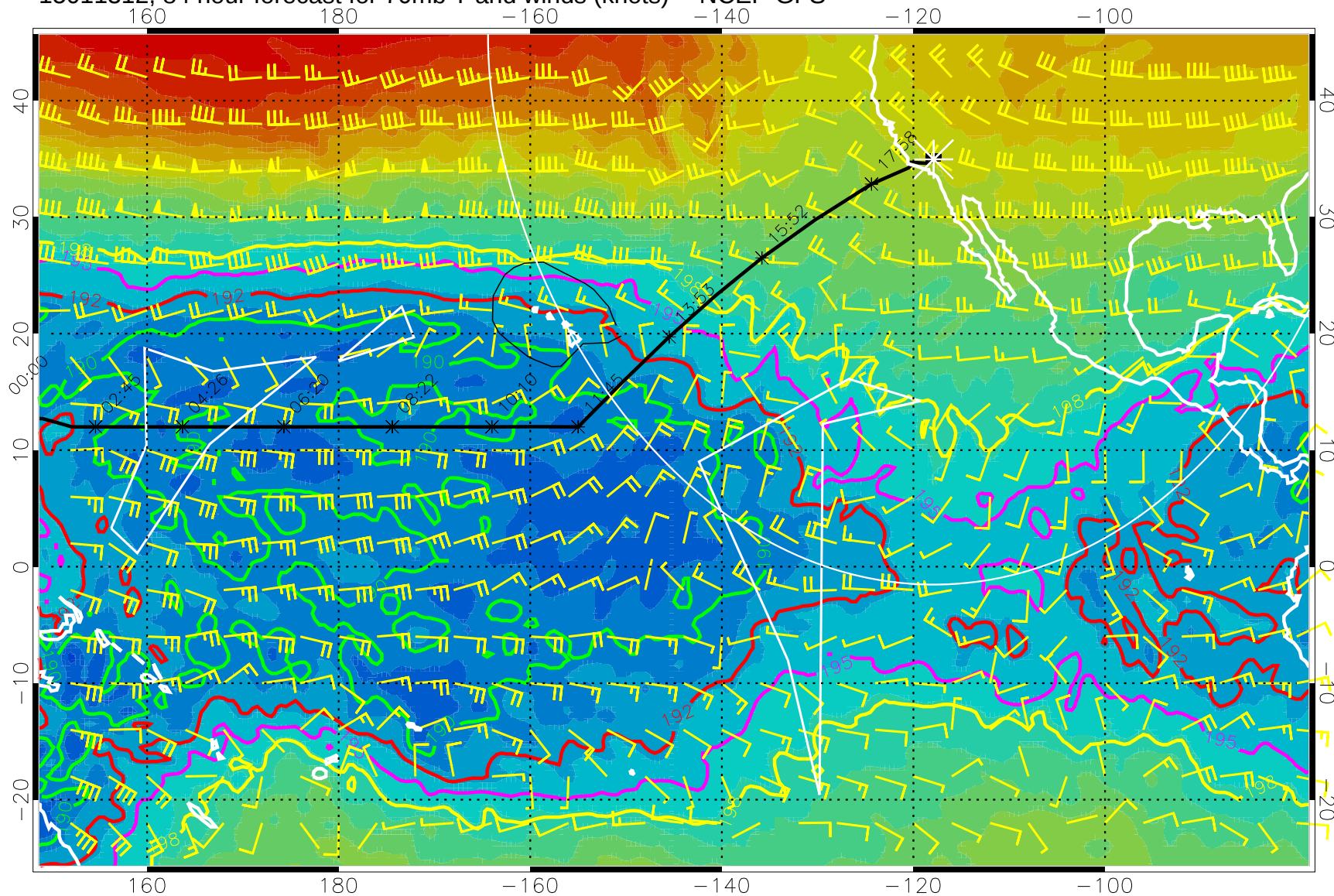
15011312, 84 hour forecast for 70mb T and winds (knots) -- NCEP GFS
