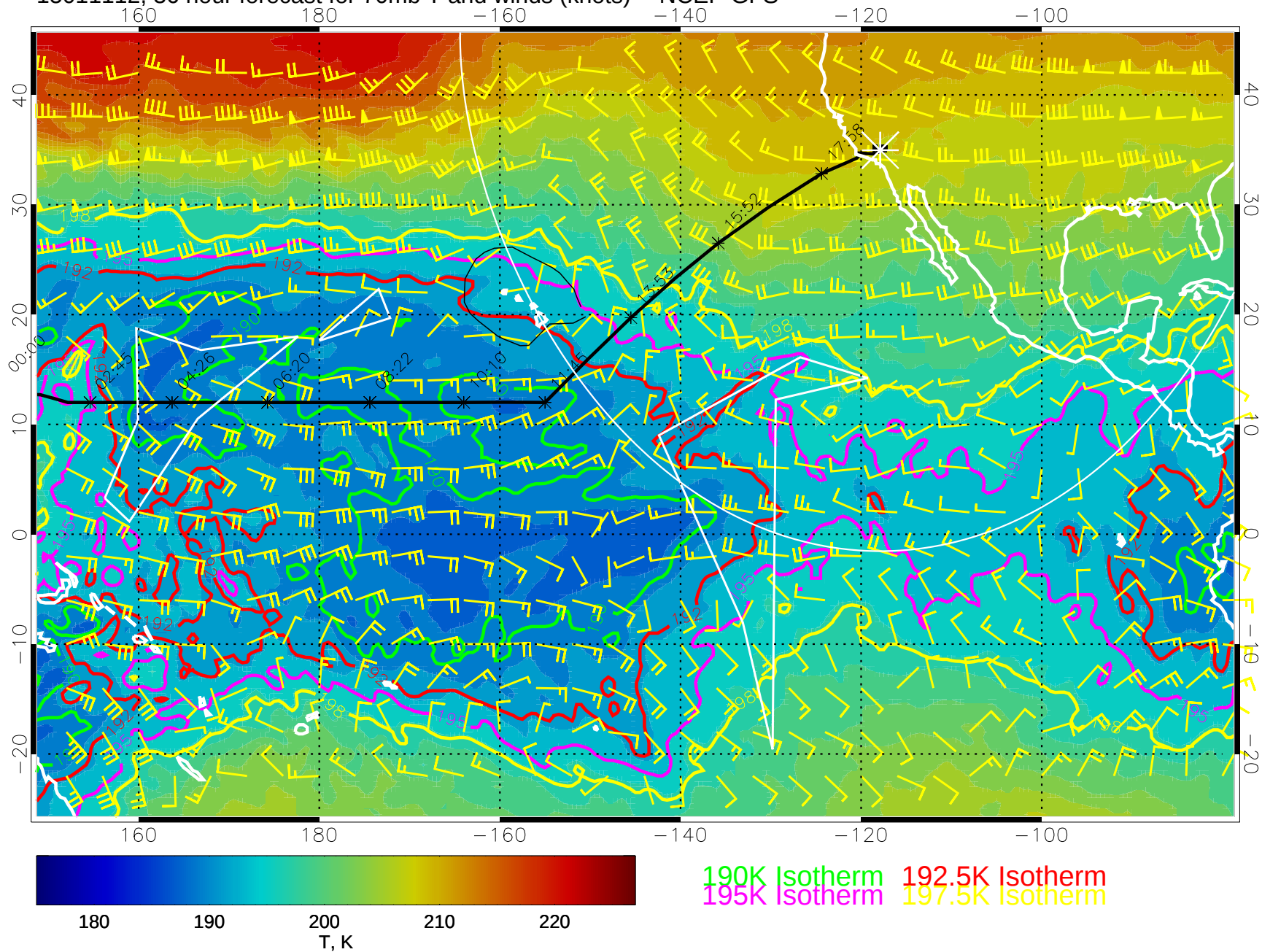
15011112, 36 hour forecast for 70mb T and winds (knots) -- NCEP GFS
