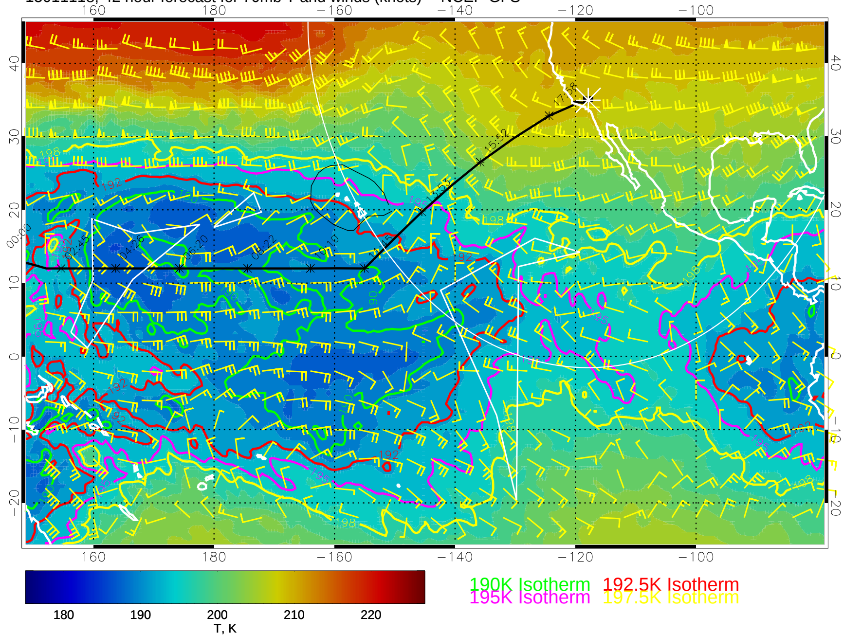
15011118, 42 hour forecast for 70mb T and winds (knots) -- NCEP GFS
