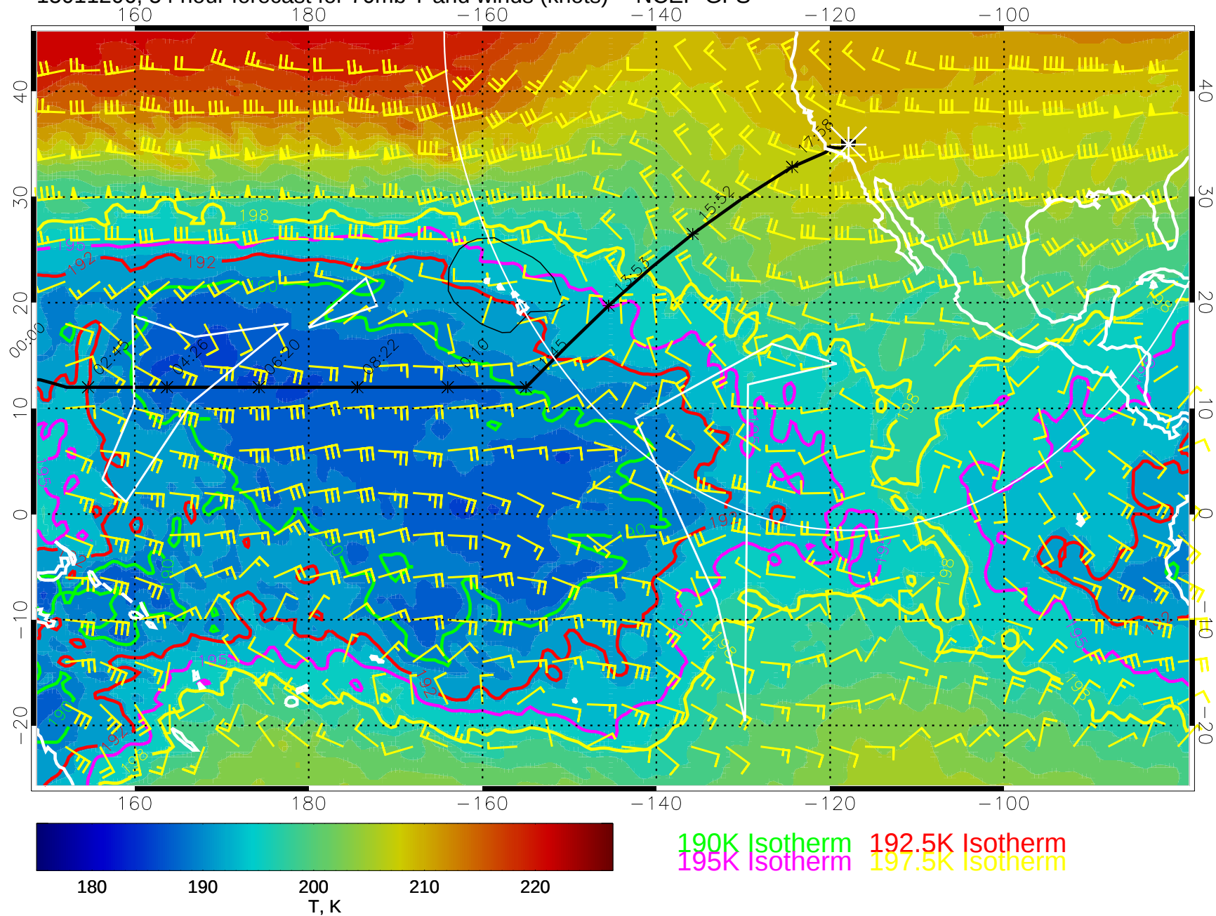
15011206, 54 hour forecast for 70mb T and winds (knots) -- NCEP GFS
