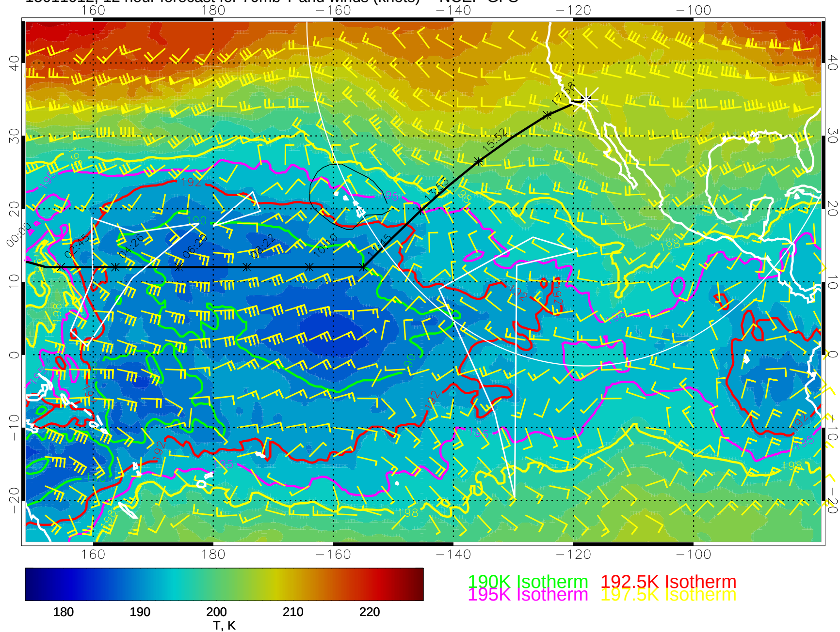
15011012, 12 hour forecast for 70mb T and winds (knots) -- NCEP GFS
