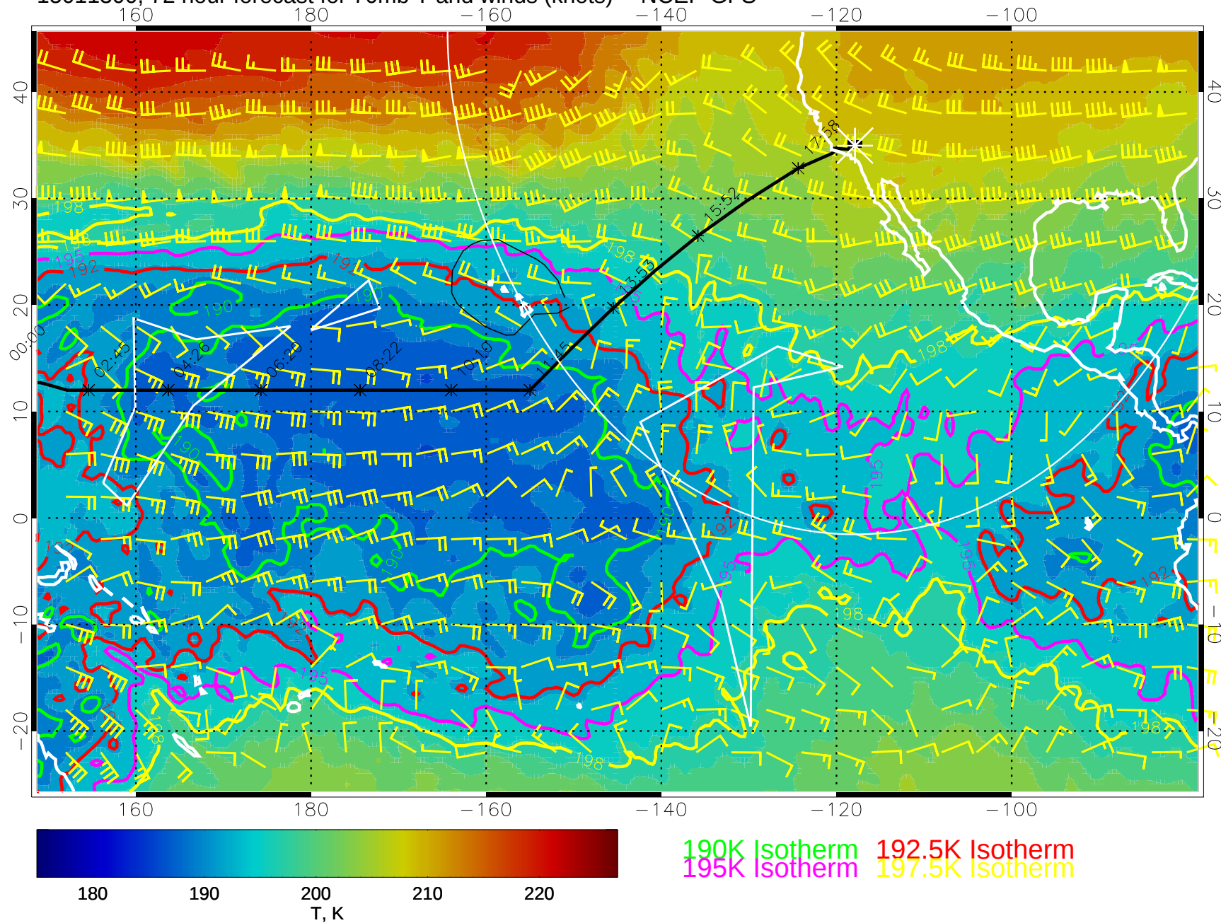
15011300, 72 hour forecast for 70mb T and winds (knots) -- NCEP GFS
