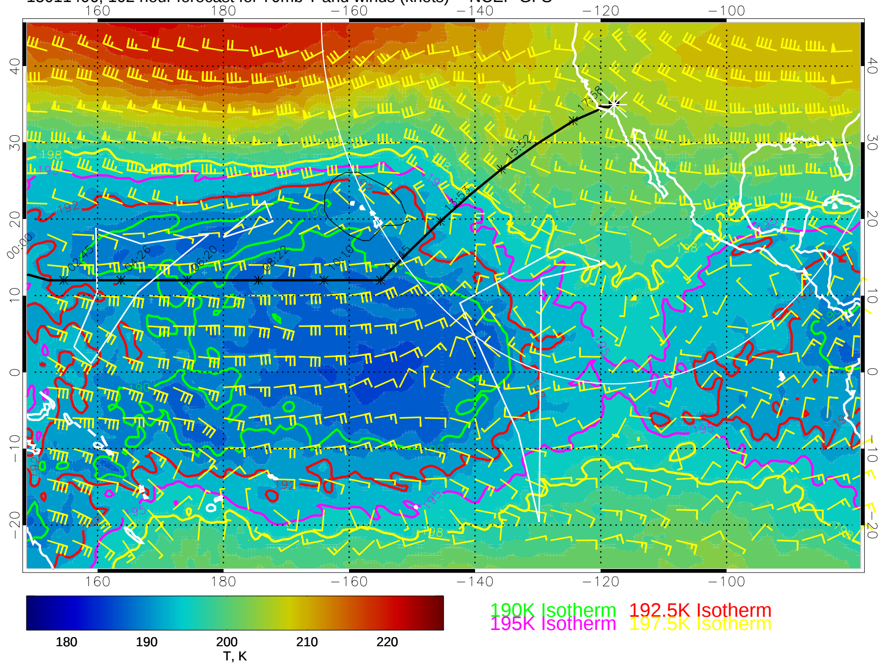
15011406, 102 hour forecast for 70mb T and winds (knots) -- NCEP GFS
