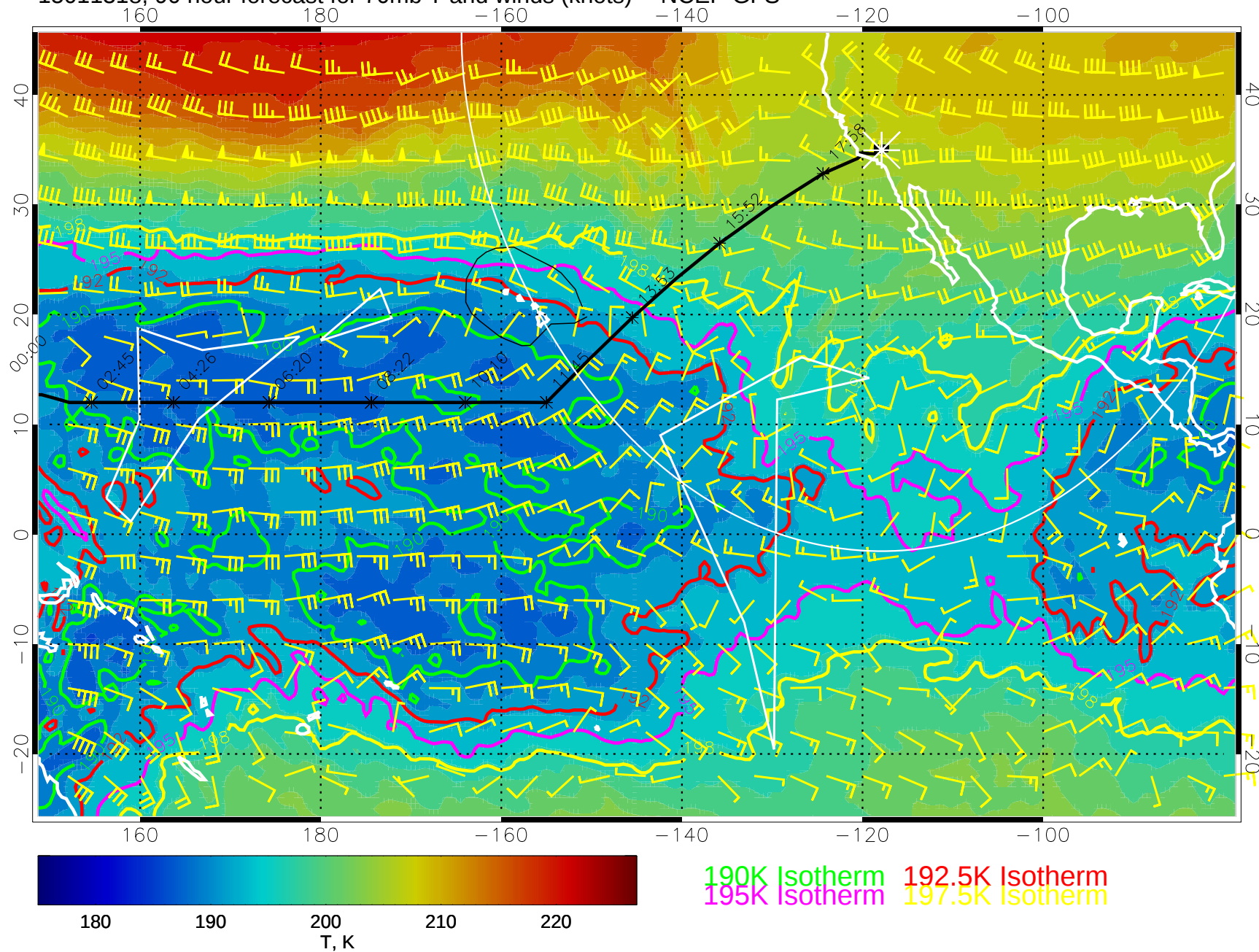
15011318, 90 hour forecast for 70mb T and winds (knots) -- NCEP GFS
