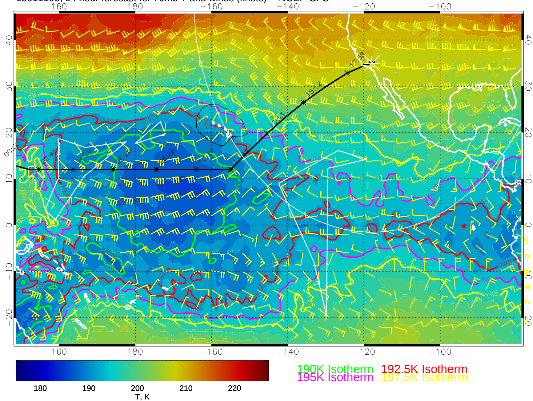
15011100, 24 hour forecast for 70mb T and winds (knots) -- NCEP GFS
