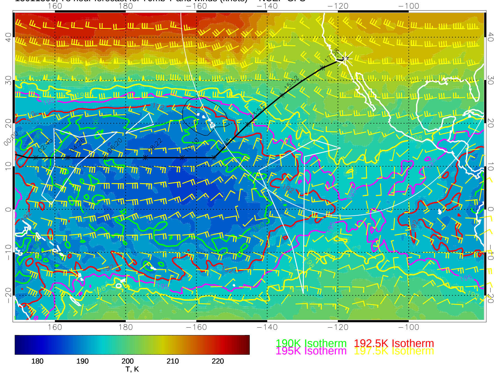
15011306, 78 hour forecast for 70mb T and winds (knots) -- NCEP GFS
