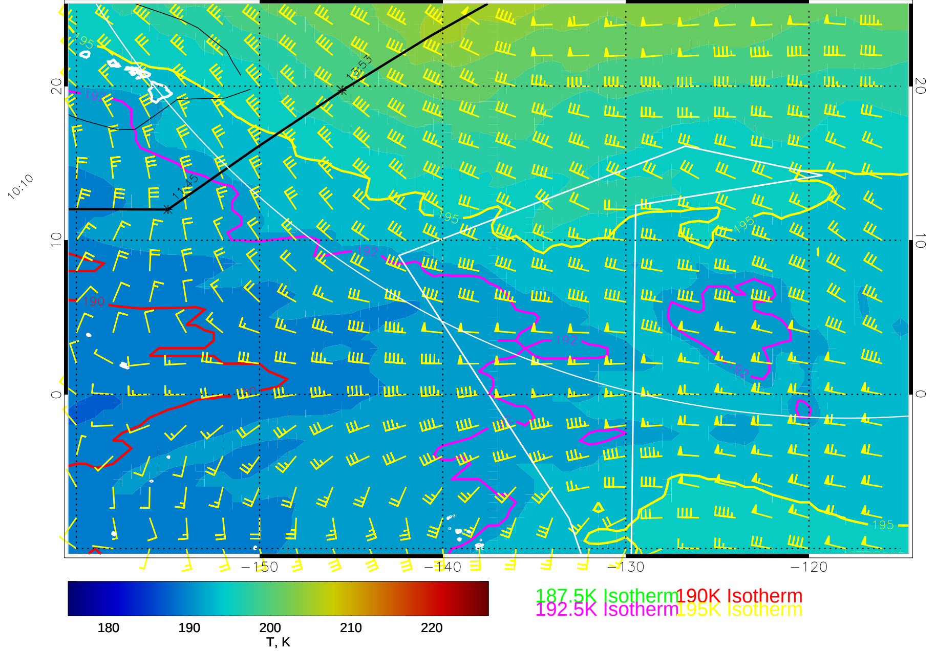
15011106, 30 hour forecast for 100mb T and winds (knots) -- NCEP GFS
