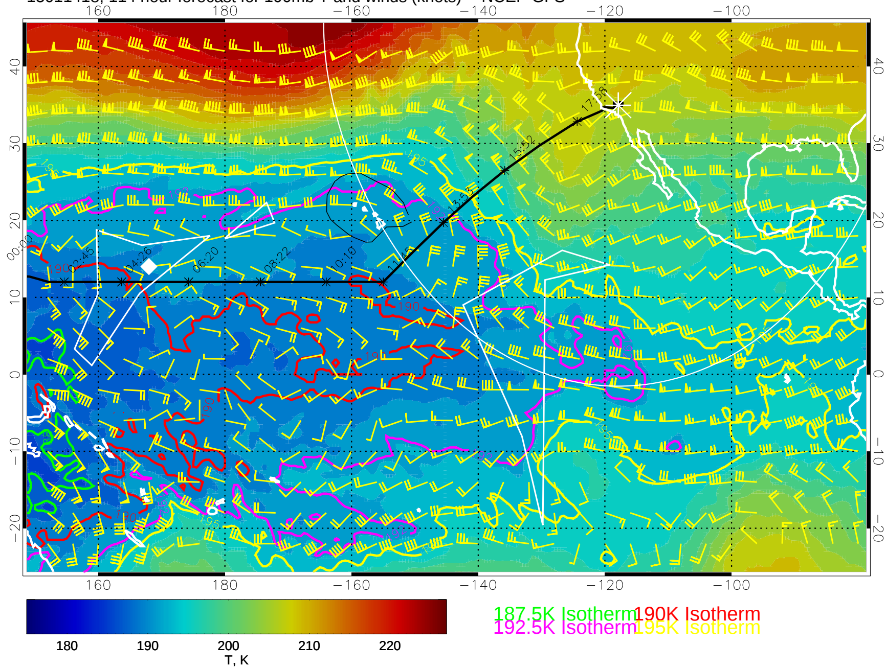
15011418, 114 hour forecast for 100mb T and winds (knots) -- NCEP GFS
