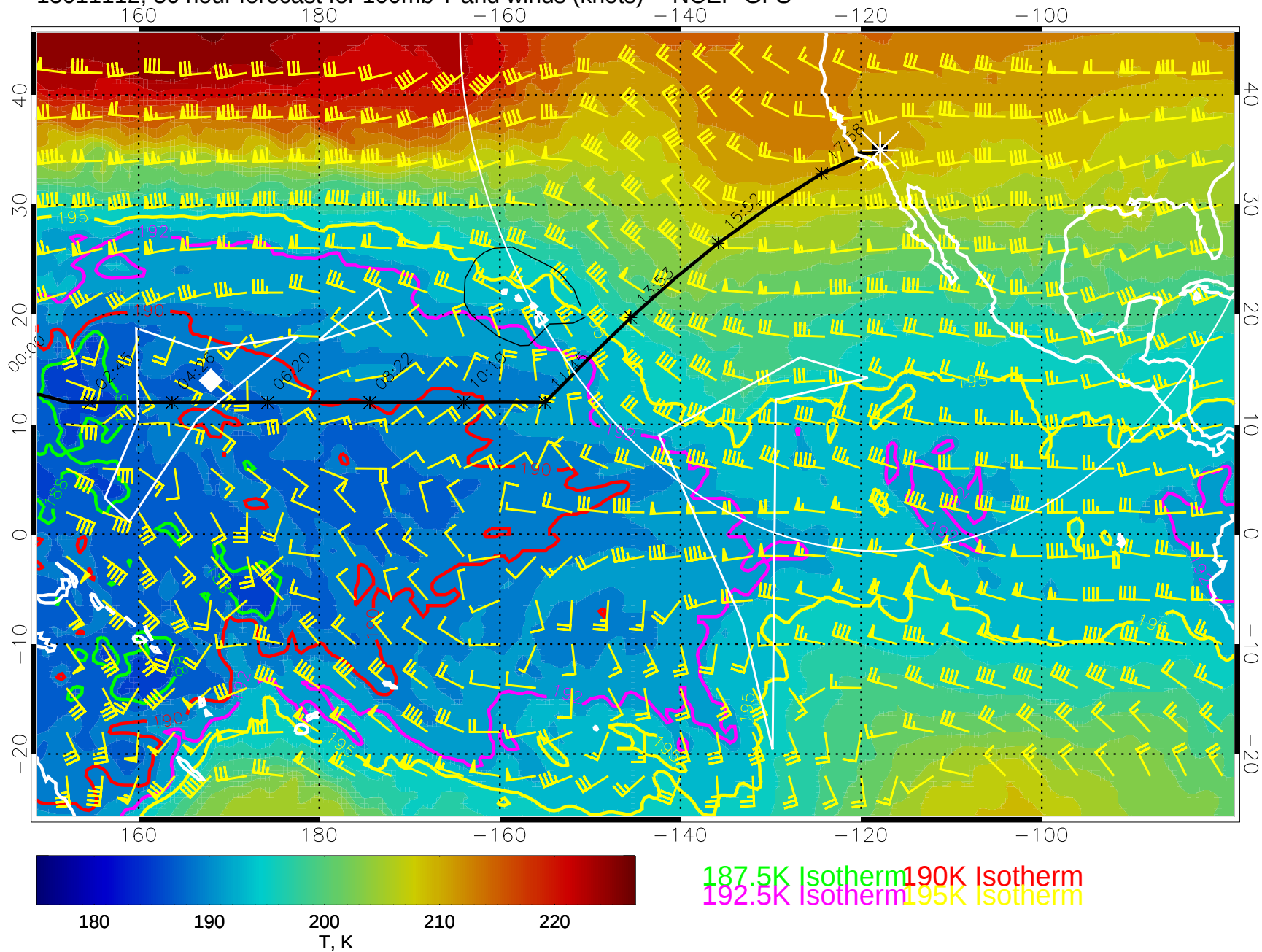
15011112, 36 hour forecast for 100mb T and winds (knots) -- NCEP GFS
