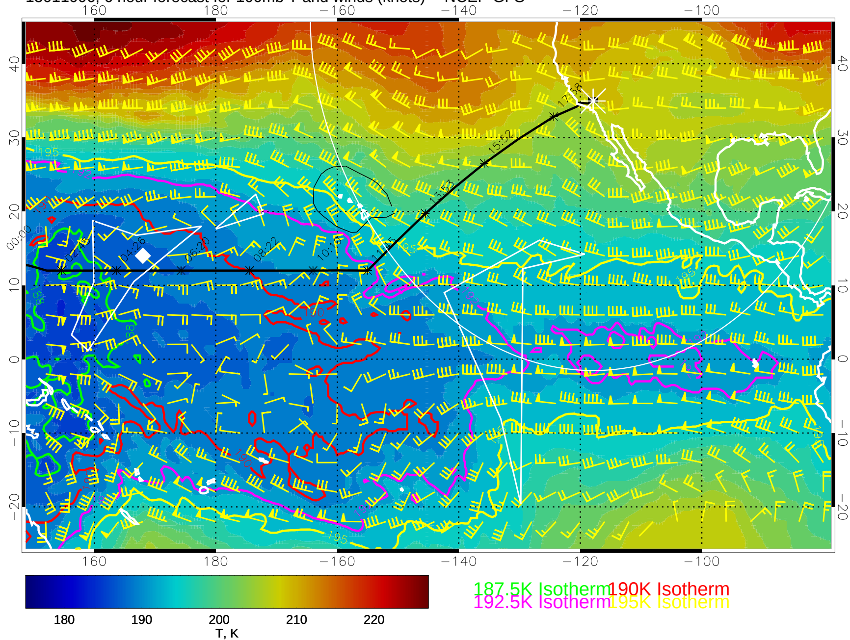
15011006, 6 hour forecast for 100mb T and winds (knots) -- NCEP GFS
