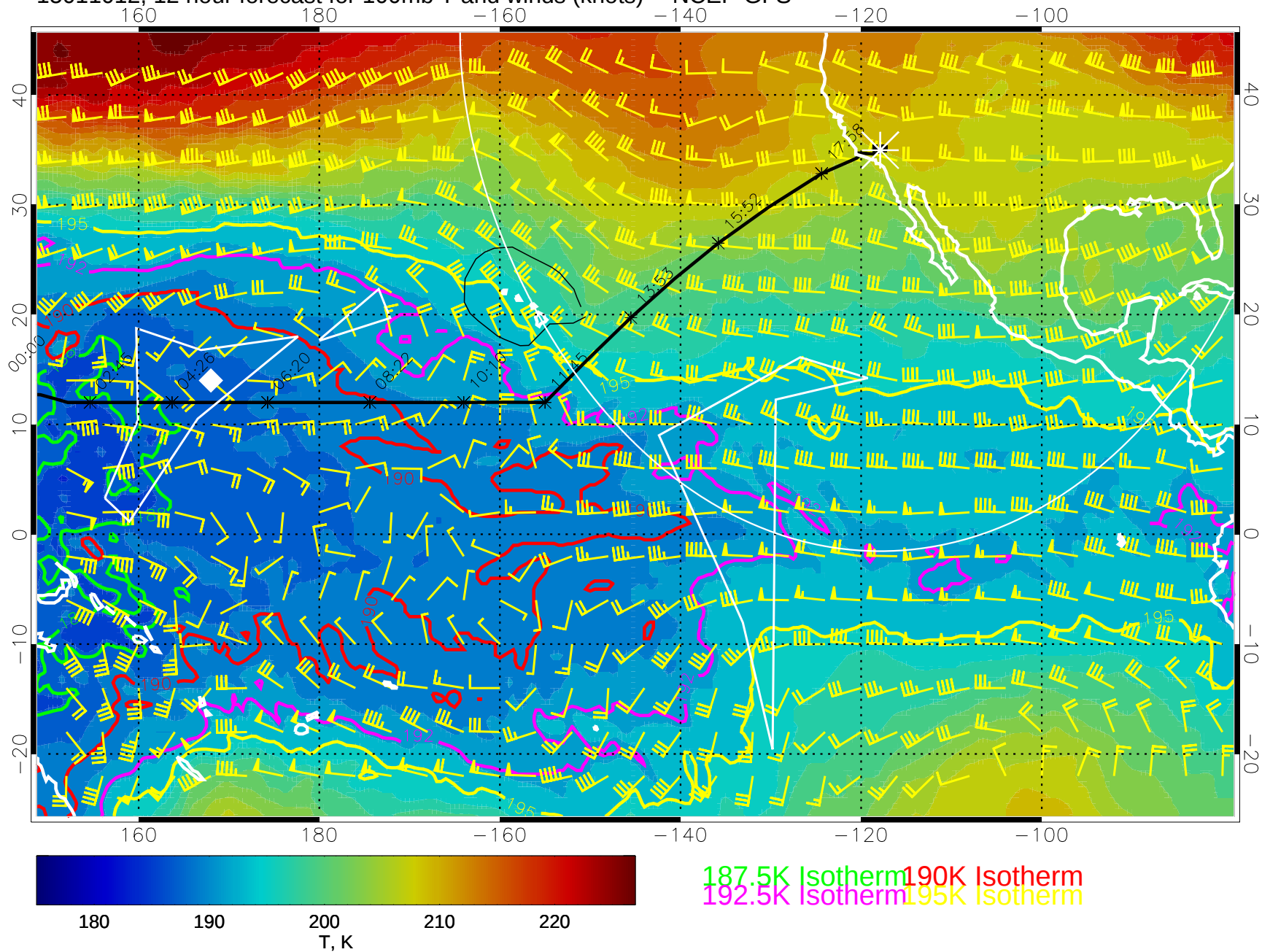
15011012, 12 hour forecast for 100mb T and winds (knots) -- NCEP GFS
