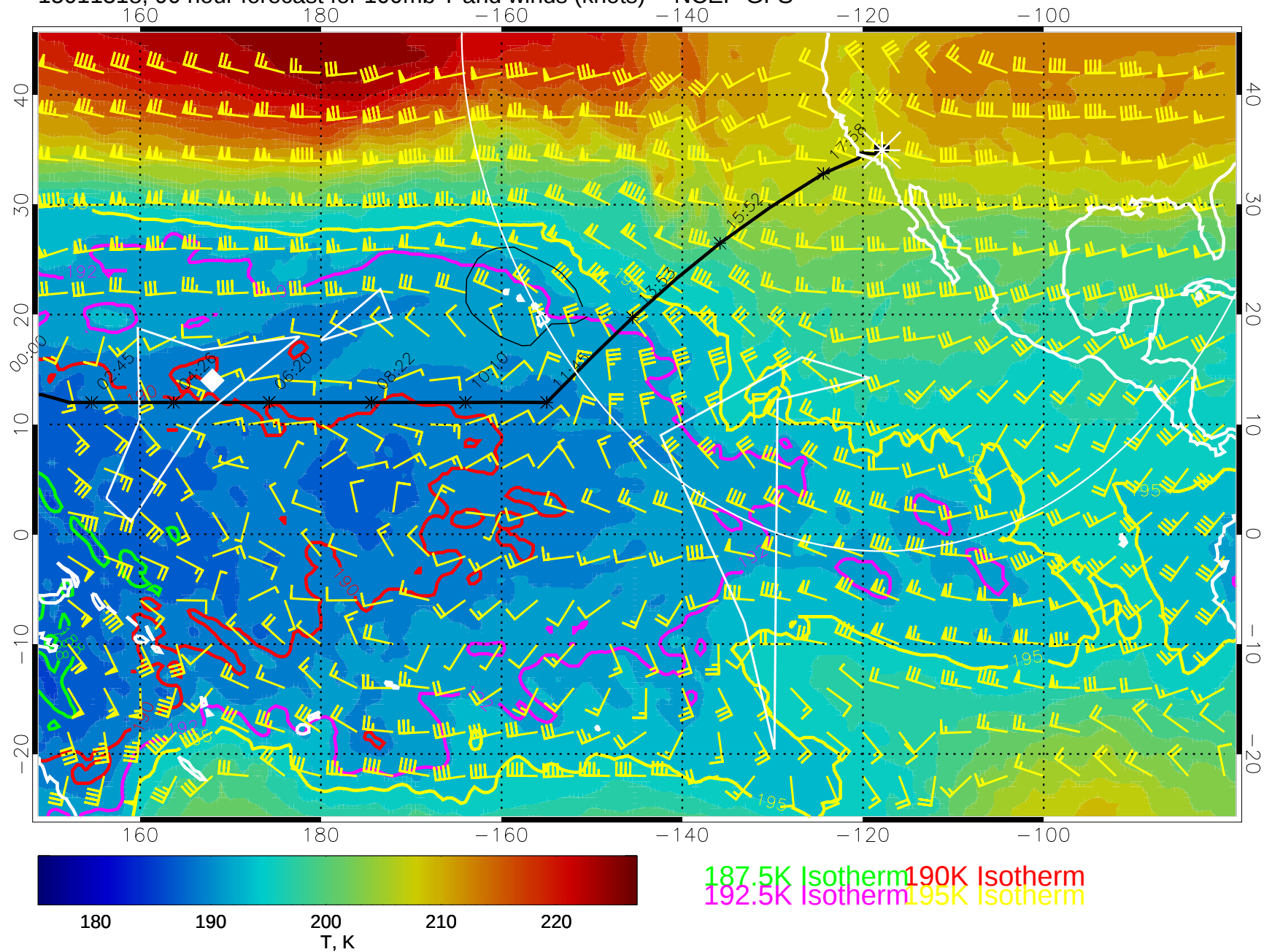
15011318, 90 hour forecast for 100mb T and winds (knots) -- NCEP GFS
