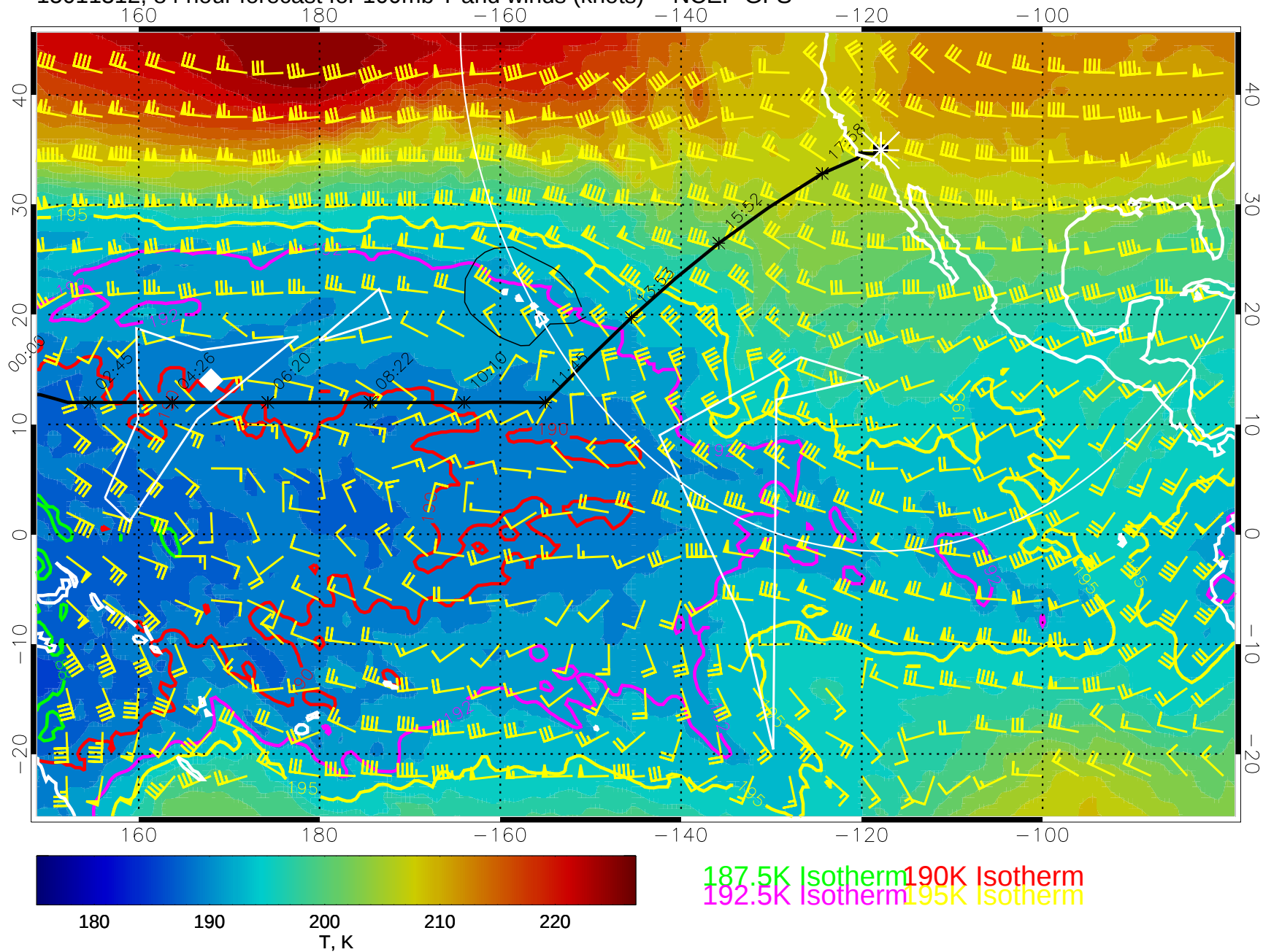
15011312, 84 hour forecast for 100mb T and winds (knots) -- NCEP GFS
