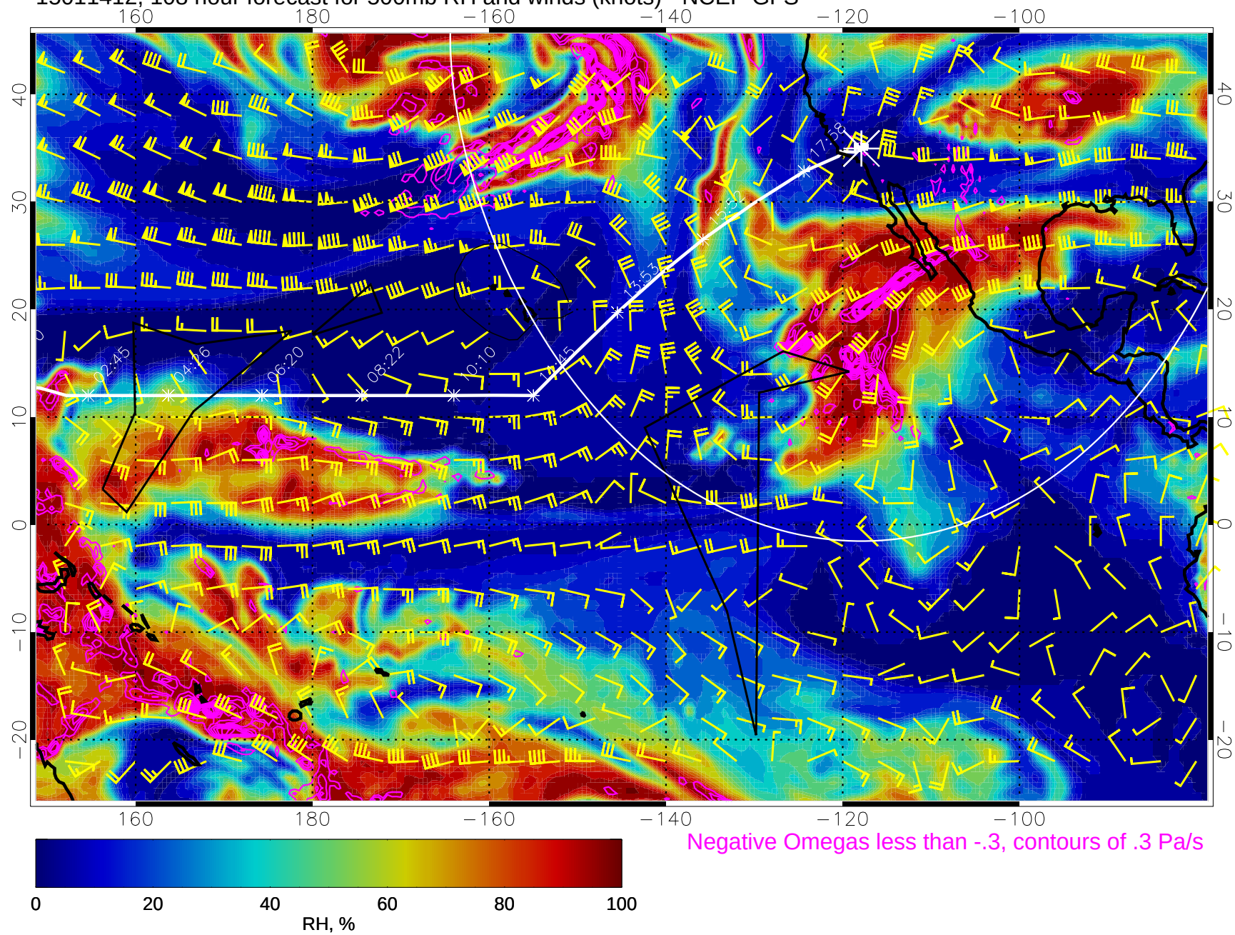
15011412, 108 hour forecast for 500mb RH and winds (knots) - NCEP GFS
