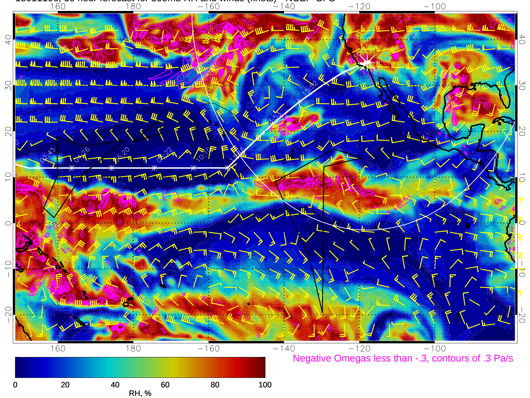
15011106, 30 hour forecast for 500mb RH and winds (knots) - NCEP GFS
