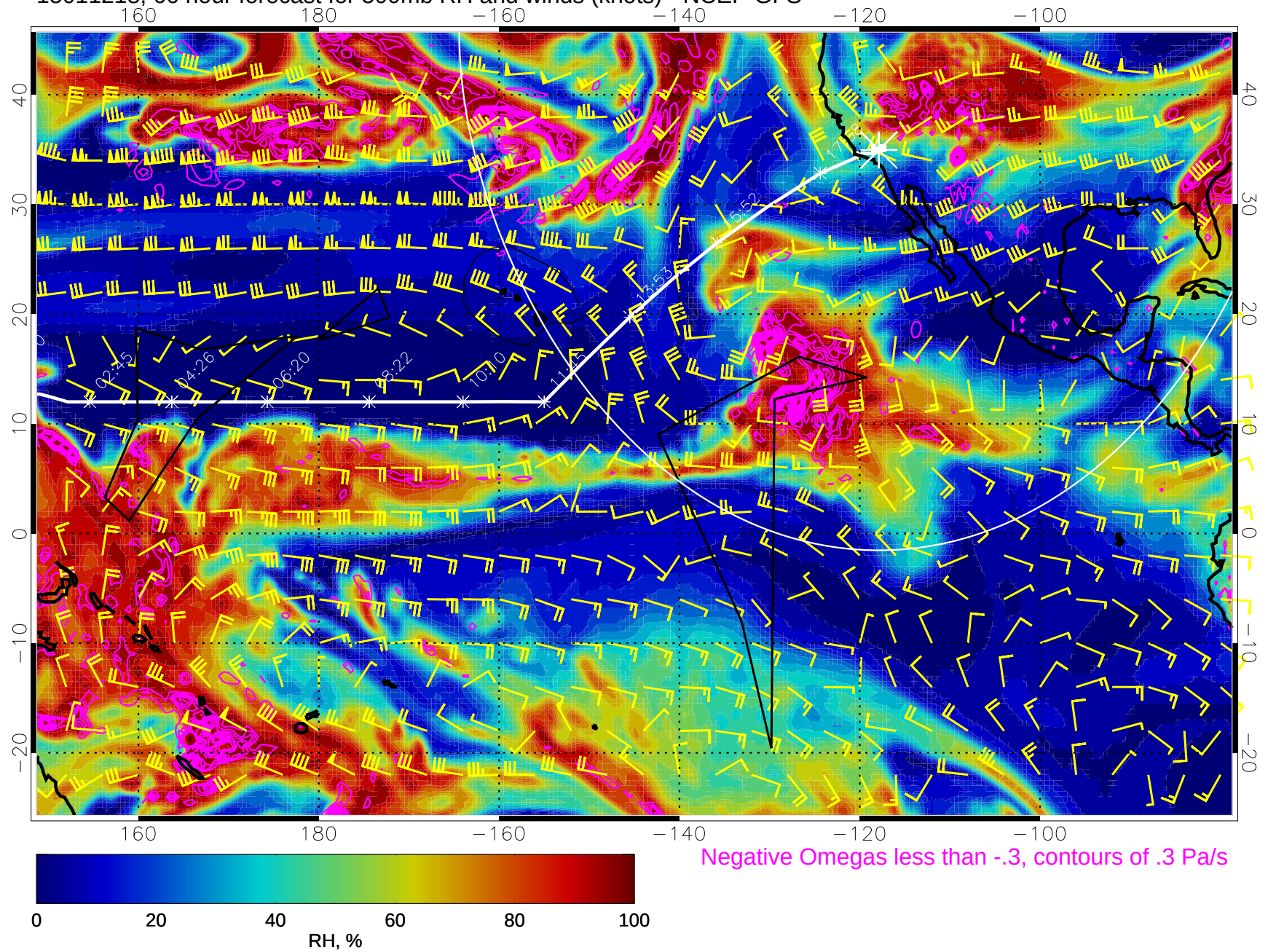
15011218, 66 hour forecast for 500mb RH and winds (knots) - NCEP GFS
