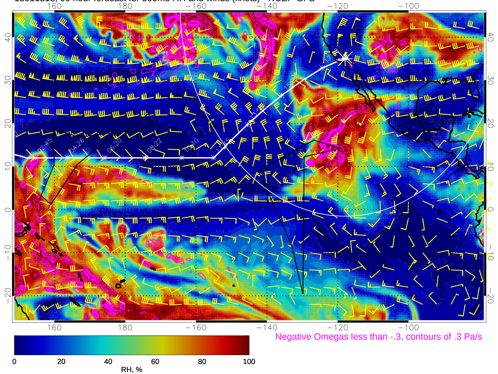
15011318, 90 hour forecast for 500mb RH and winds (knots) - NCEP GFS
