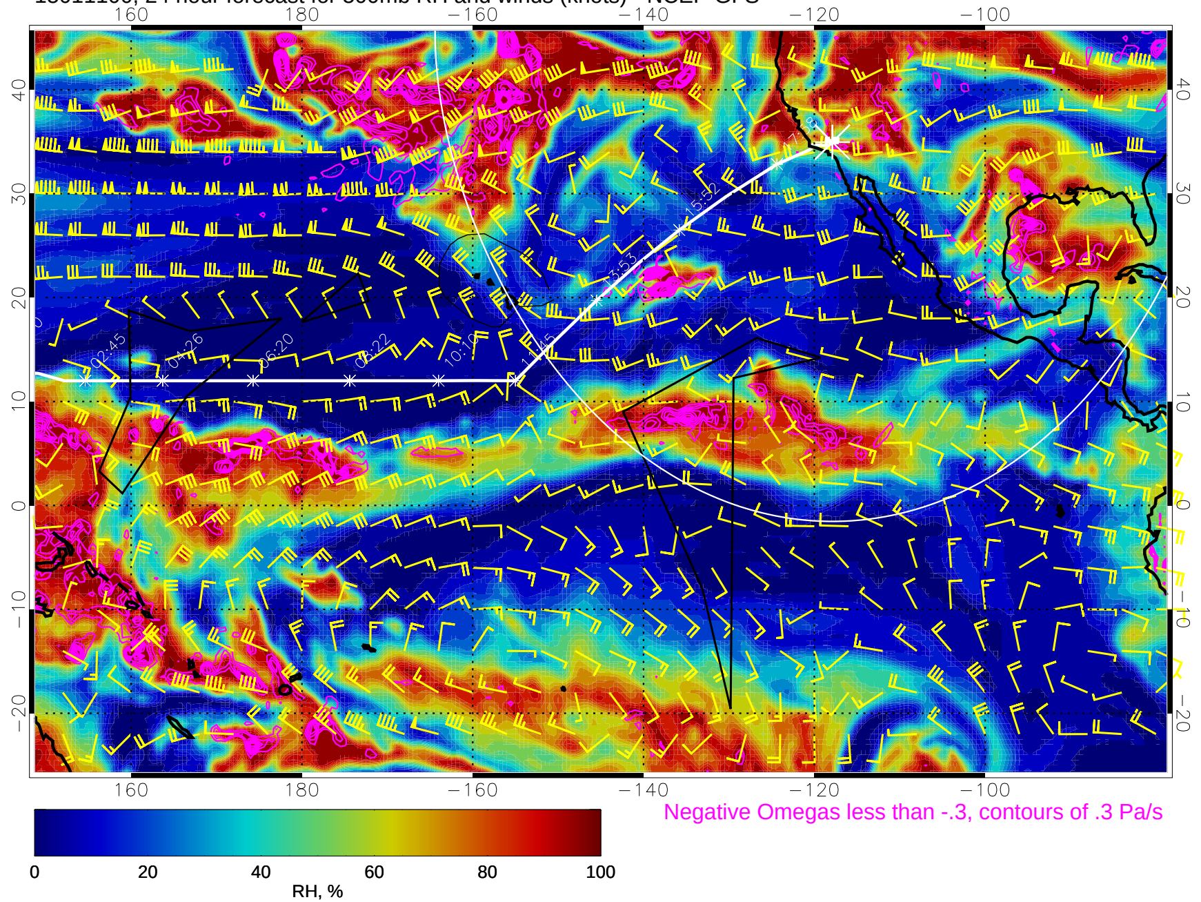
15011100, 24 hour forecast for 500mb RH and winds (knots) - NCEP GFS
