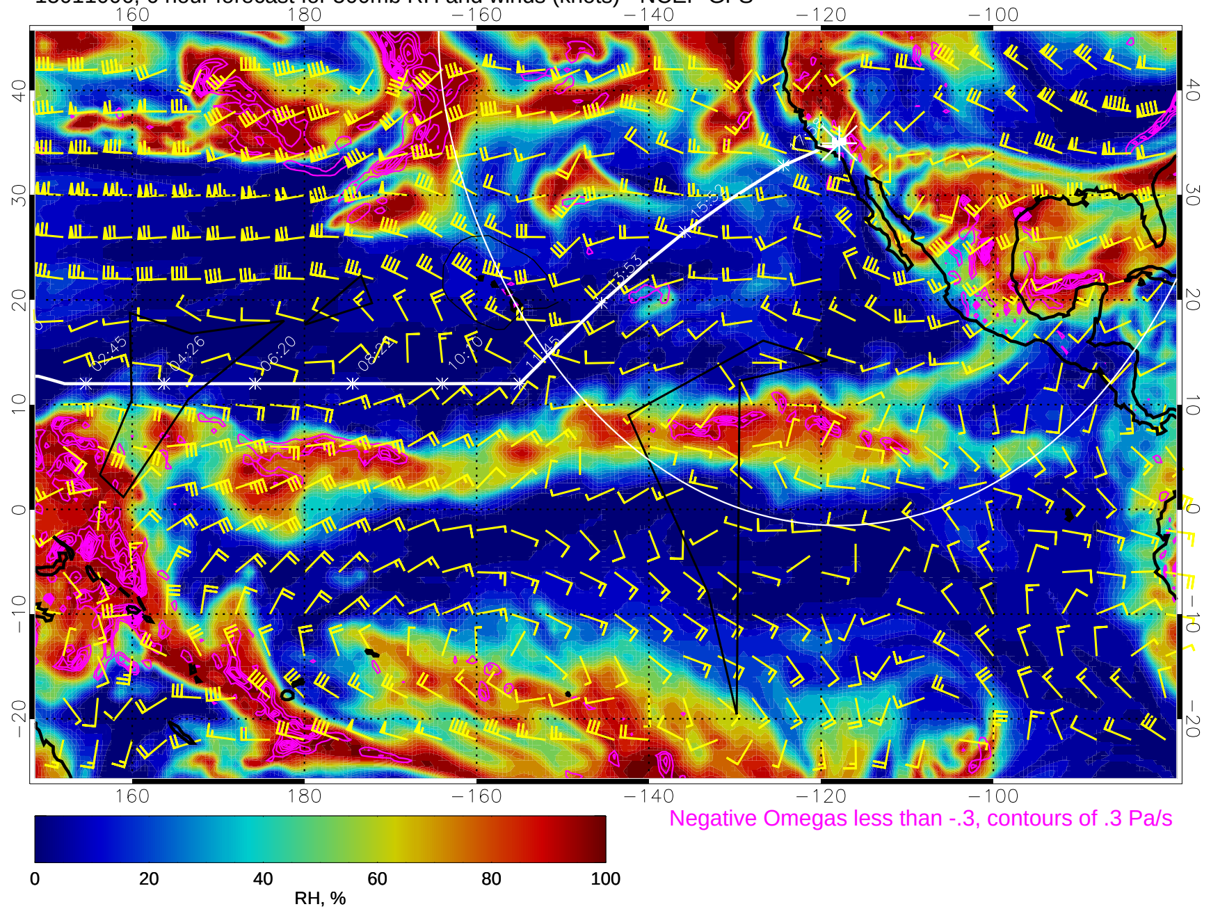
15011006, 6 hour forecast for 500mb RH and winds (knots) - NCEP GFS
