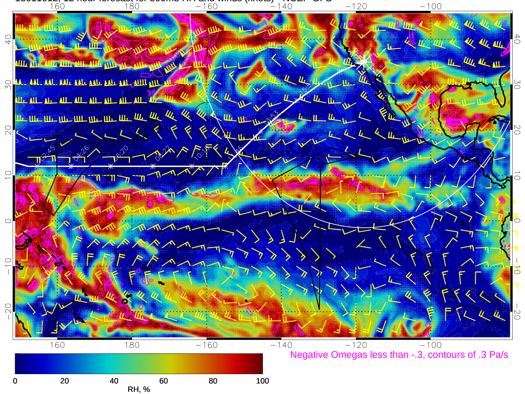
15011012, 12 hour forecast for 500mb RH and winds (knots) - NCEP GFS
