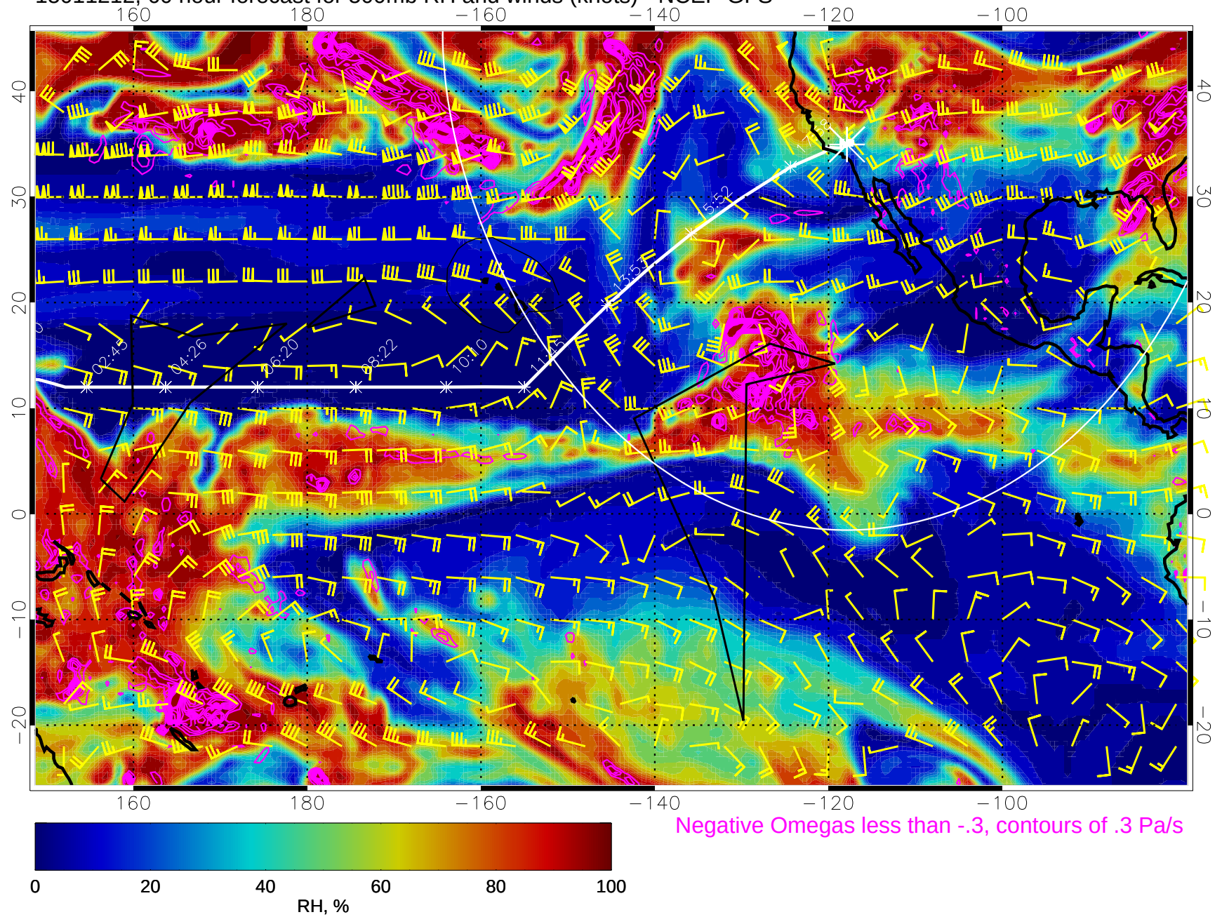
15011212, 60 hour forecast for 500mb RH and winds (knots) - NCEP GFS
