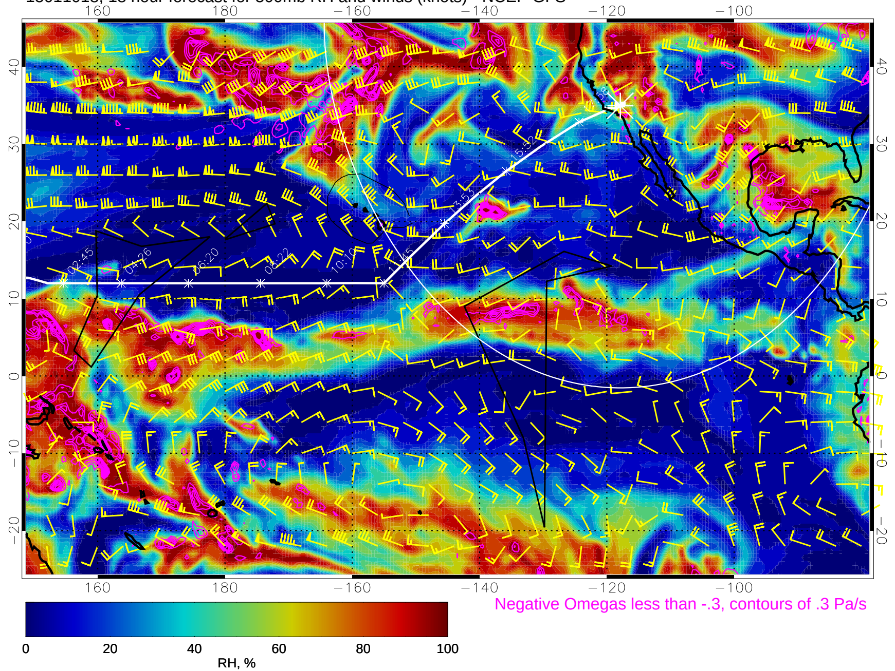
15011018, 18 hour forecast for 500mb RH and winds (knots) - NCEP GFS
