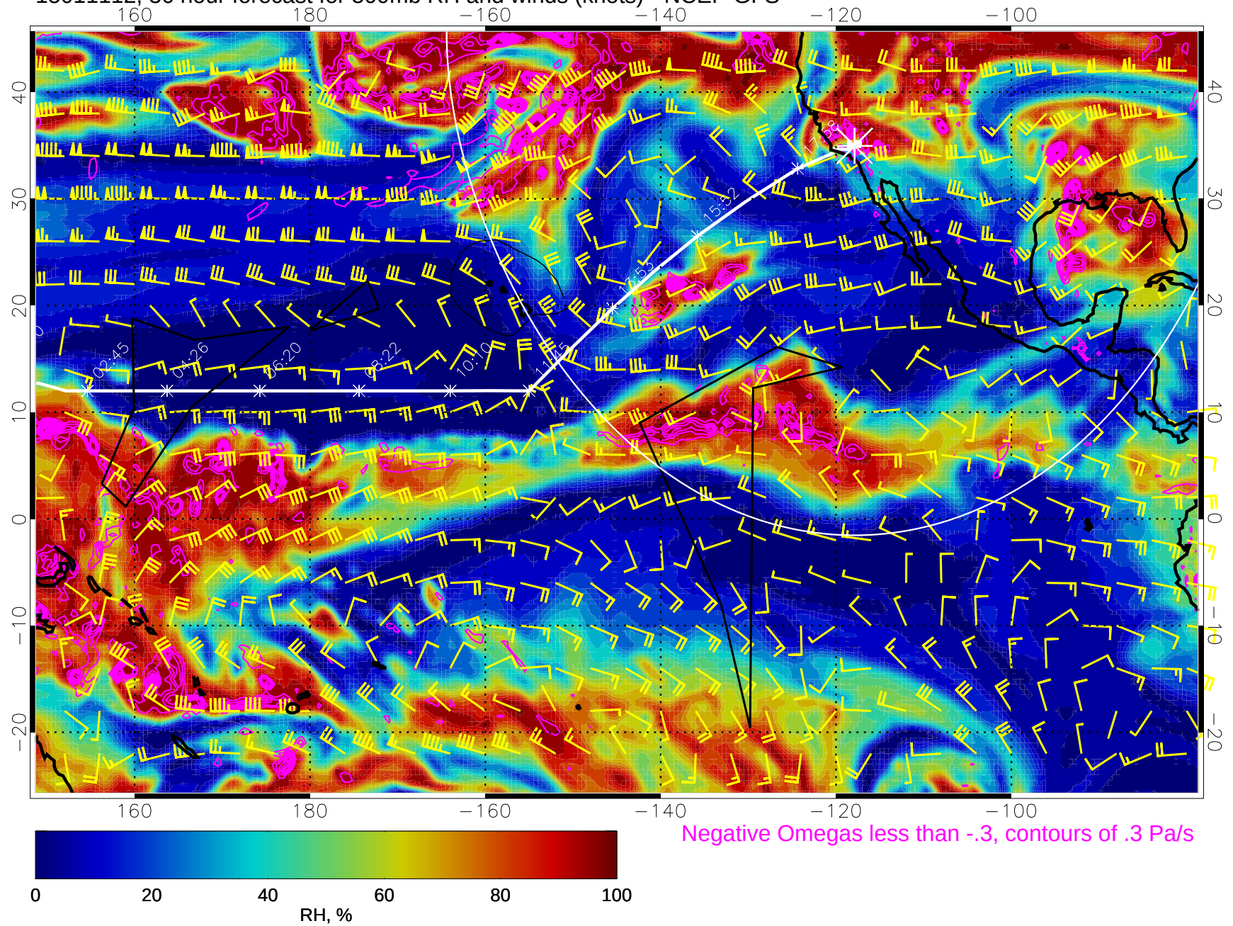
15011112, 36 hour forecast for 500mb RH and winds (knots) - NCEP GFS
