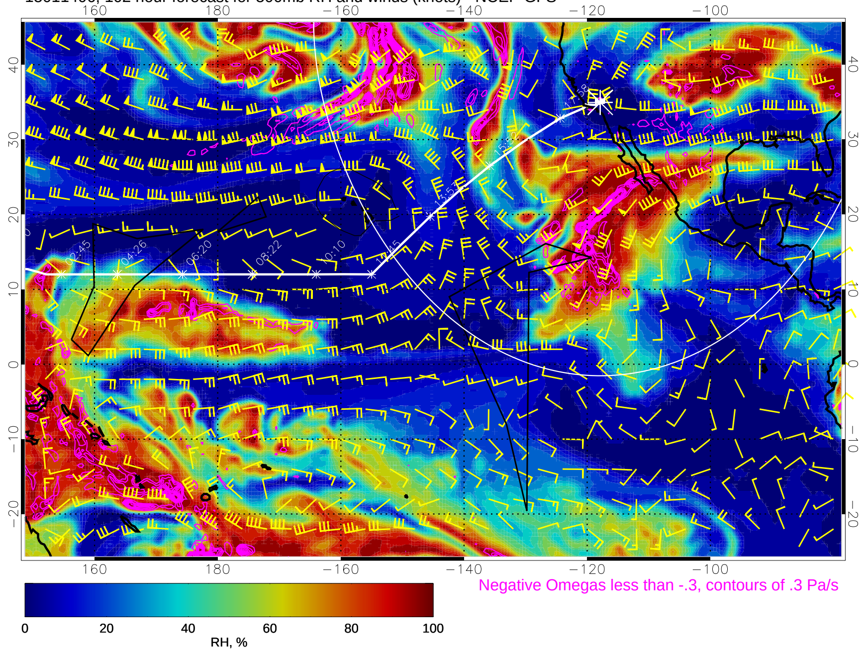
15011406, 102 hour forecast for 500mb RH and winds (knots) - NCEP GFS
