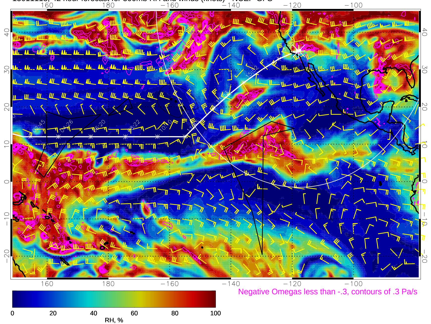
15011118, 42 hour forecast for 500mb RH and winds (knots) - NCEP GFS
