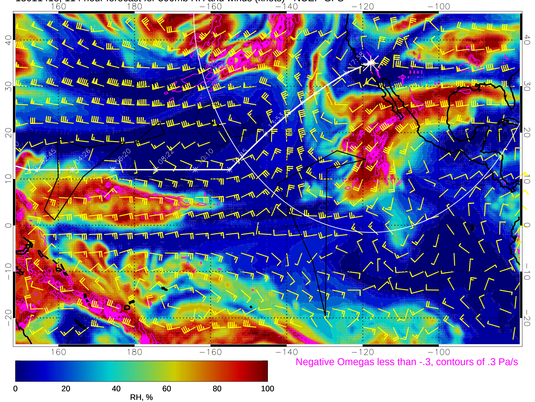
15011418, 114 hour forecast for 500mb RH and winds (knots) - NCEP GFS
