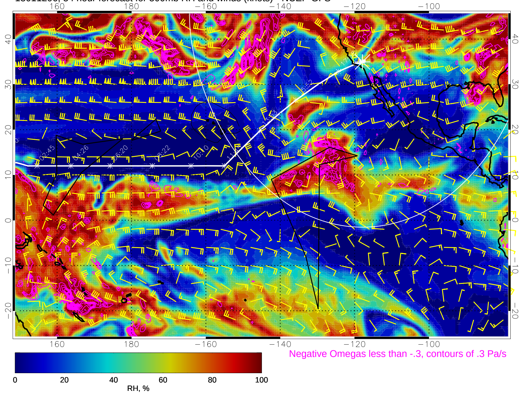
15011206, 54 hour forecast for 500mb RH and winds (knots) - NCEP GFS
