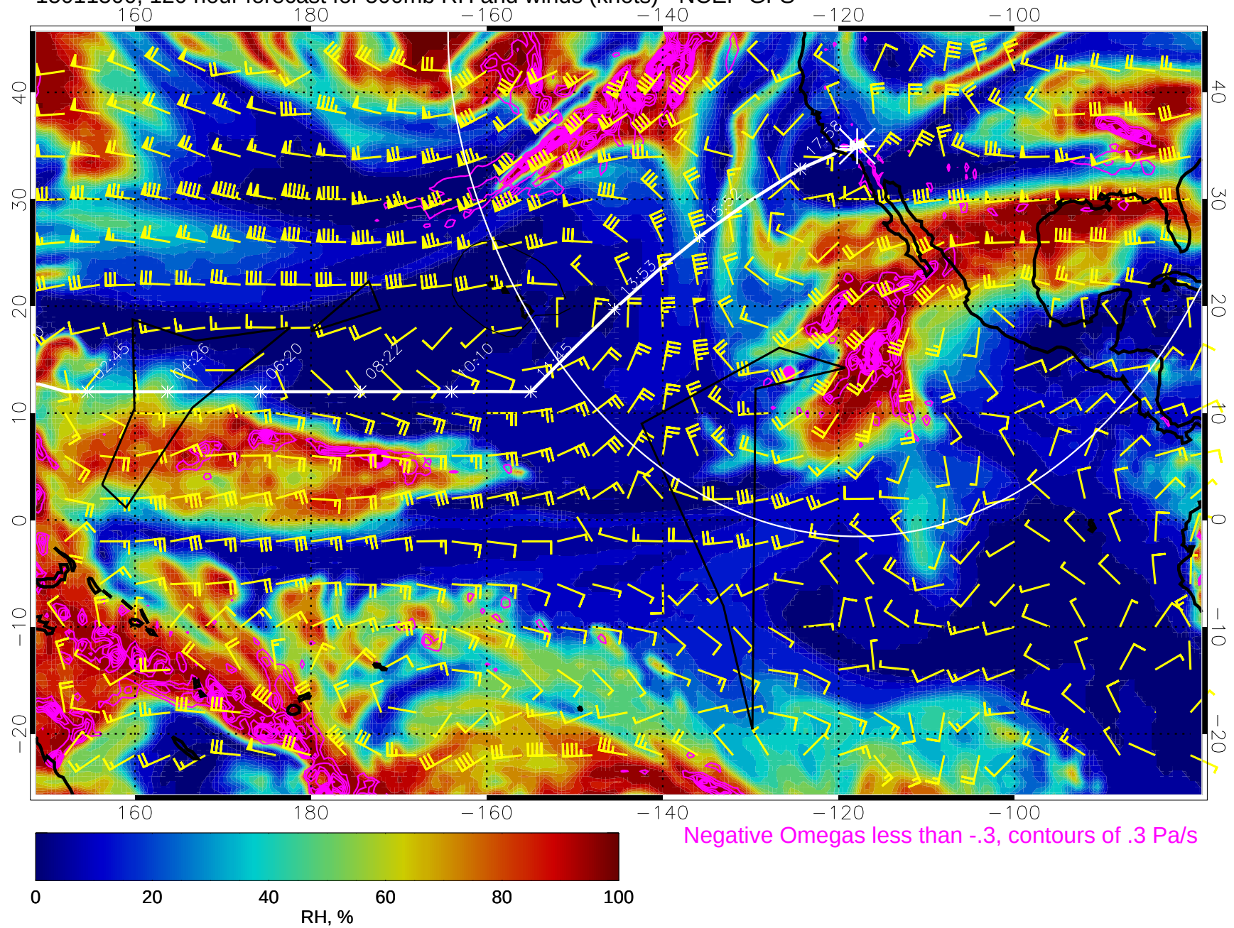
15011500, 120 hour forecast for 500mb RH and winds (knots) - NCEP GFS
