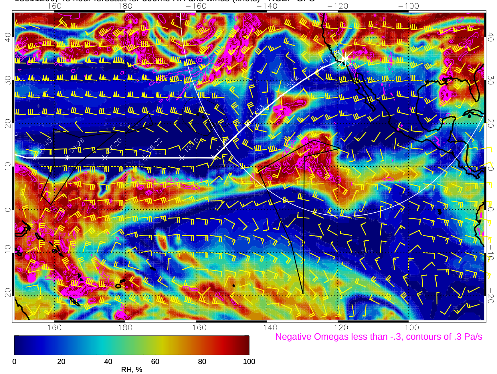
15011200, 48 hour forecast for 500mb RH and winds (knots) - NCEP GFS
