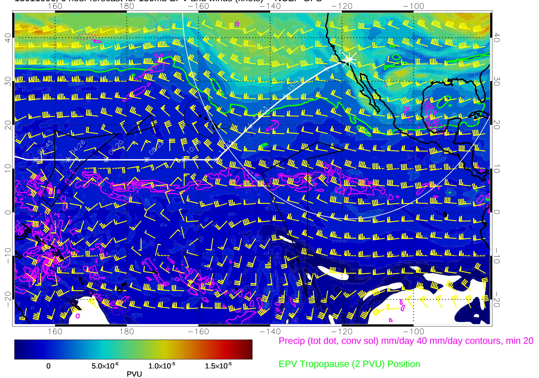
15011006, 6 hour forecast for 150mb EPV and winds (knots) -- NCEP GFS
