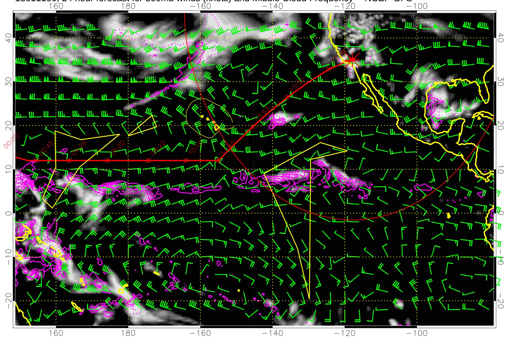
15011100, 24 hour forecast for 500mb winds (knots) and Middle Cloud Frequency -- NCEP GFS
