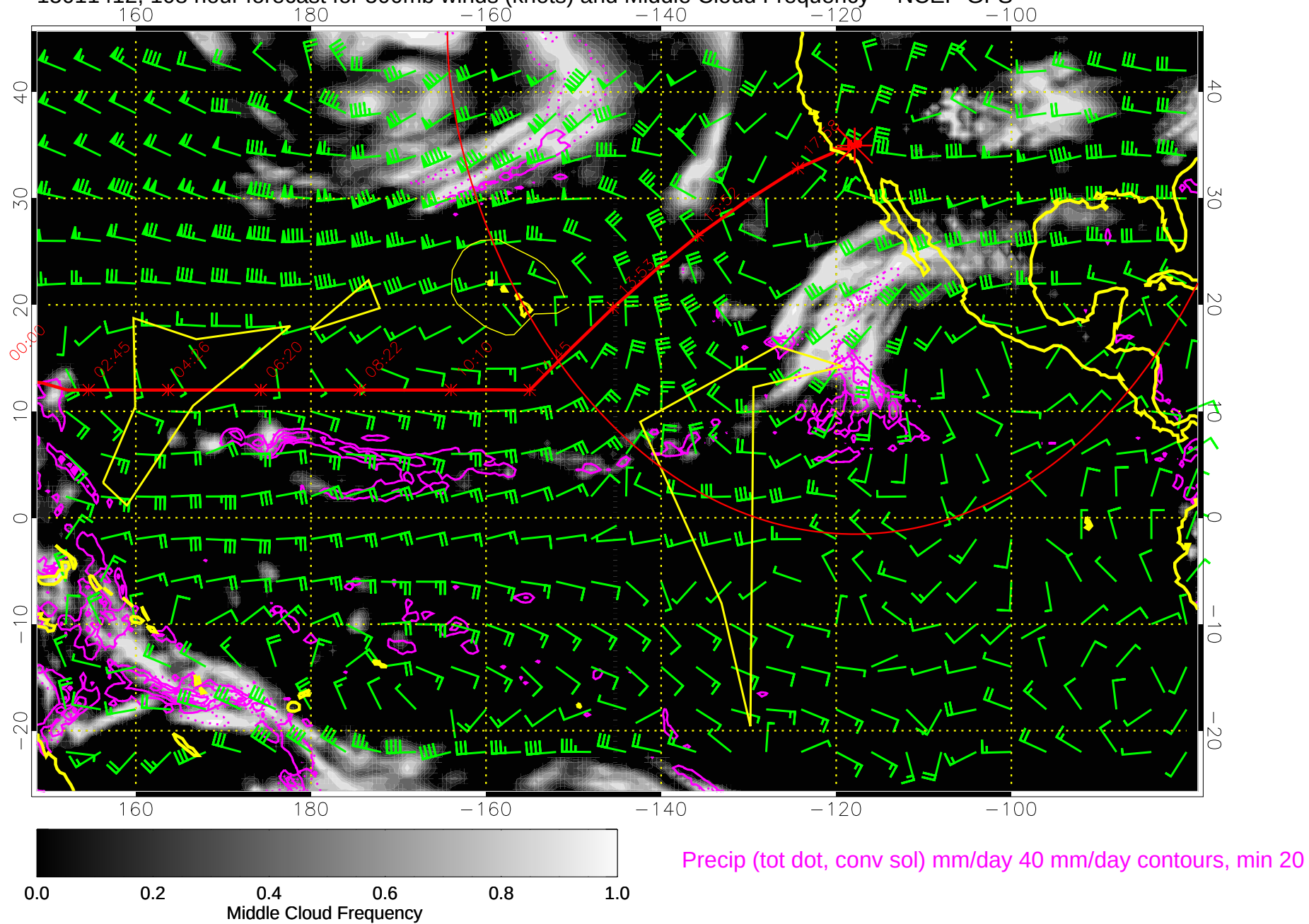
15011412, 108 hour forecast for 500mb winds (knots) and Middle Cloud Frequency -- NCEP GFS
