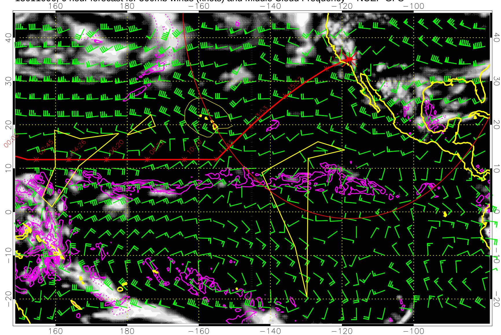
15011006, 6 hour forecast for 500mb winds (knots) and Middle Cloud Frequency -- NCEP GFS
