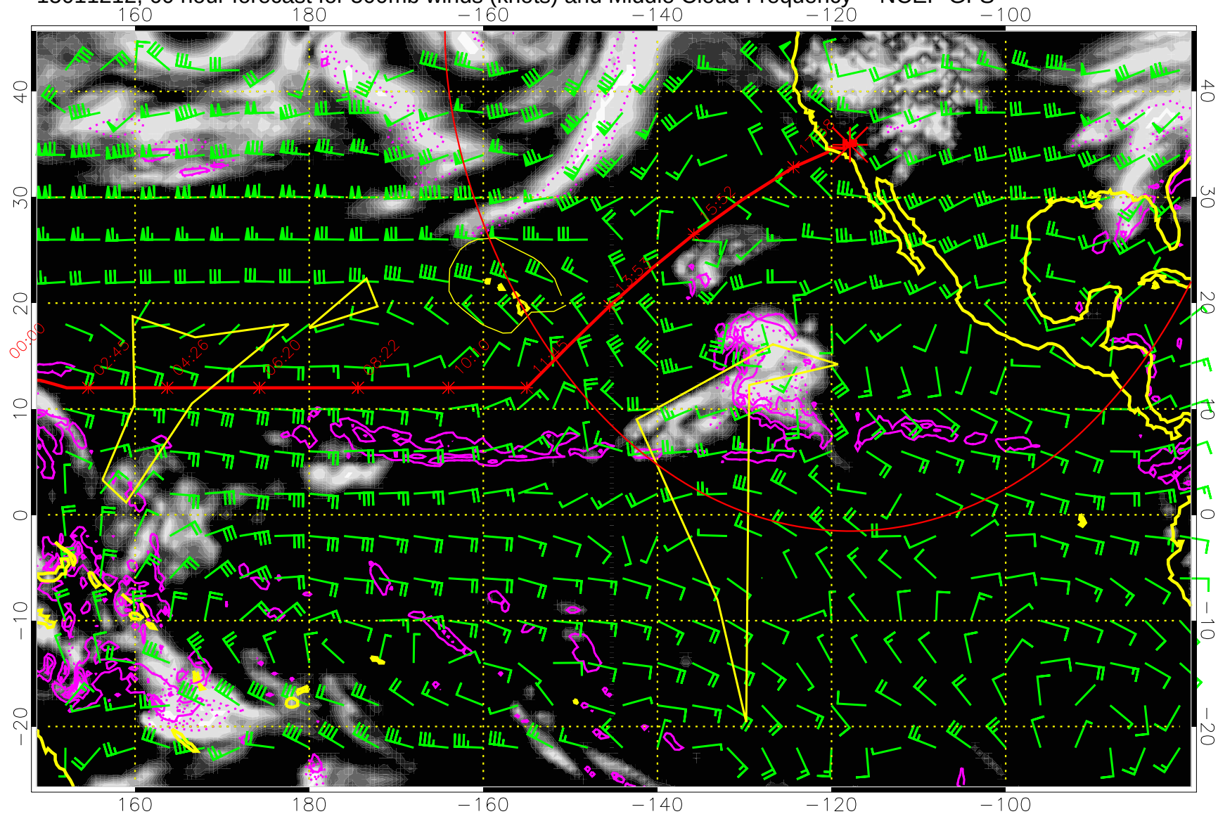
15011212, 60 hour forecast for 500mb winds (knots) and Middle Cloud Frequency -- NCEP GFS
