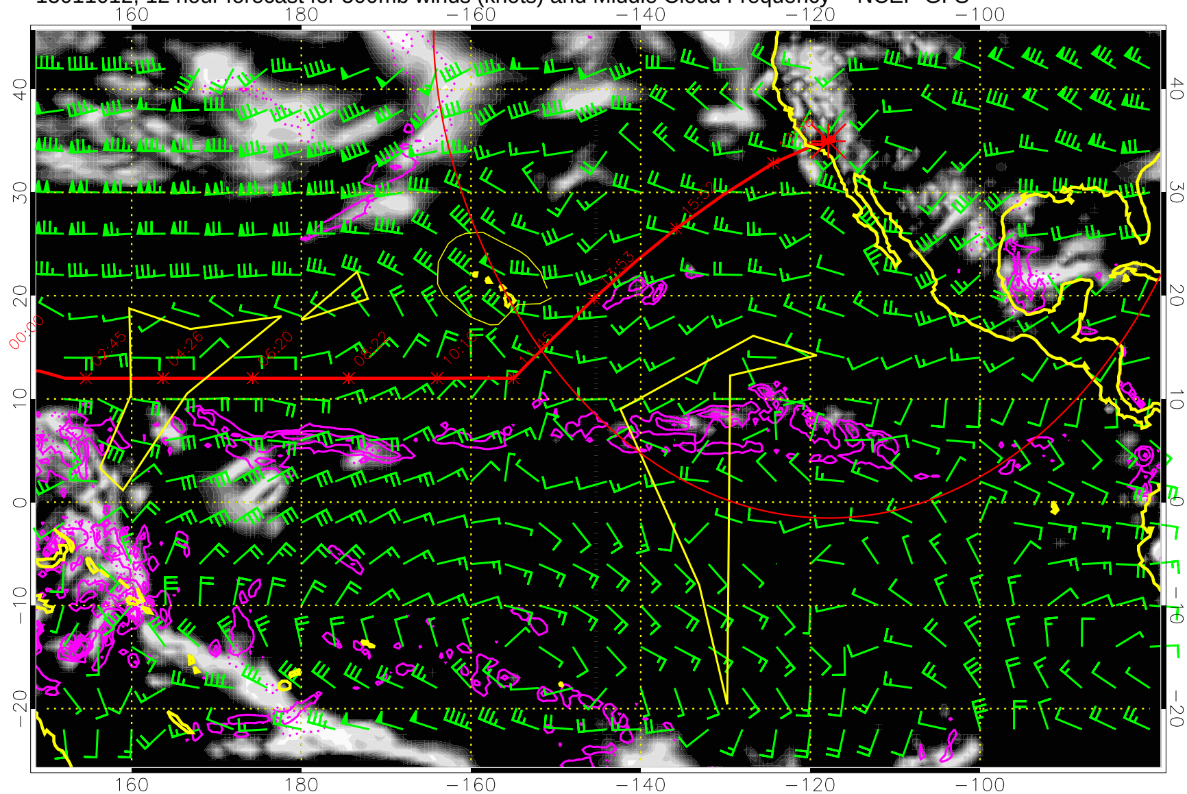
15011012, 12 hour forecast for 500mb winds (knots) and Middle Cloud Frequency -- NCEP GFS
