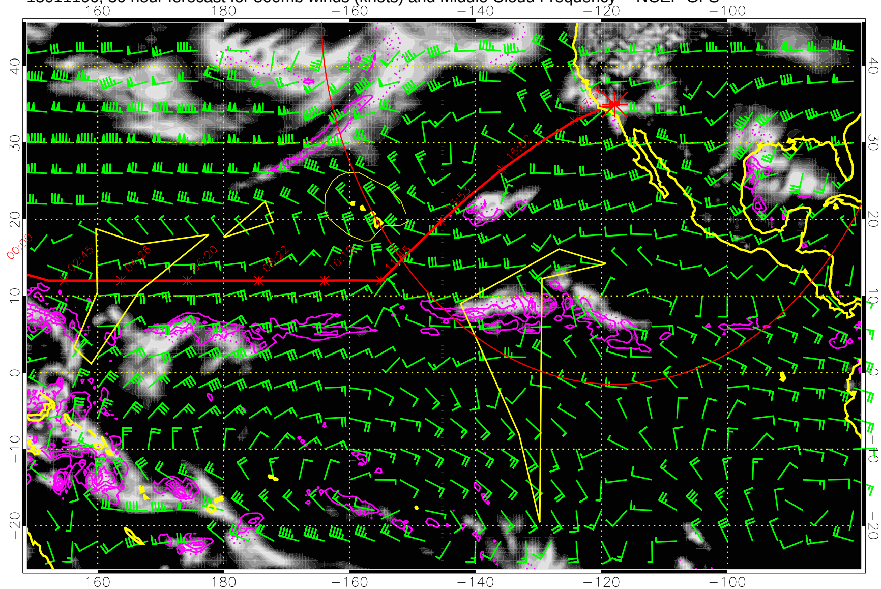
15011106, 30 hour forecast for 500mb winds (knots) and Middle Cloud Frequency -- NCEP GFS
