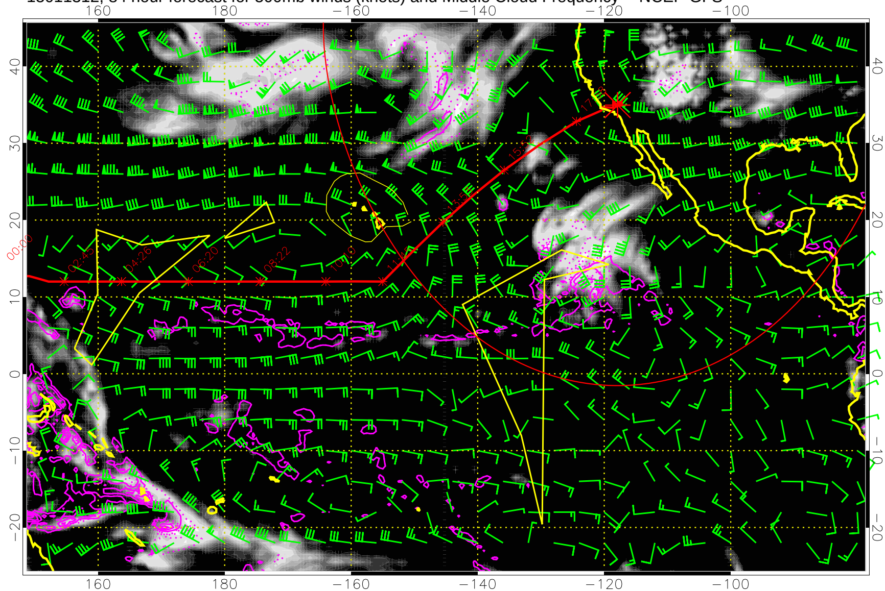
15011312, 84 hour forecast for 500mb winds (knots) and Middle Cloud Frequency -- NCEP GFS
