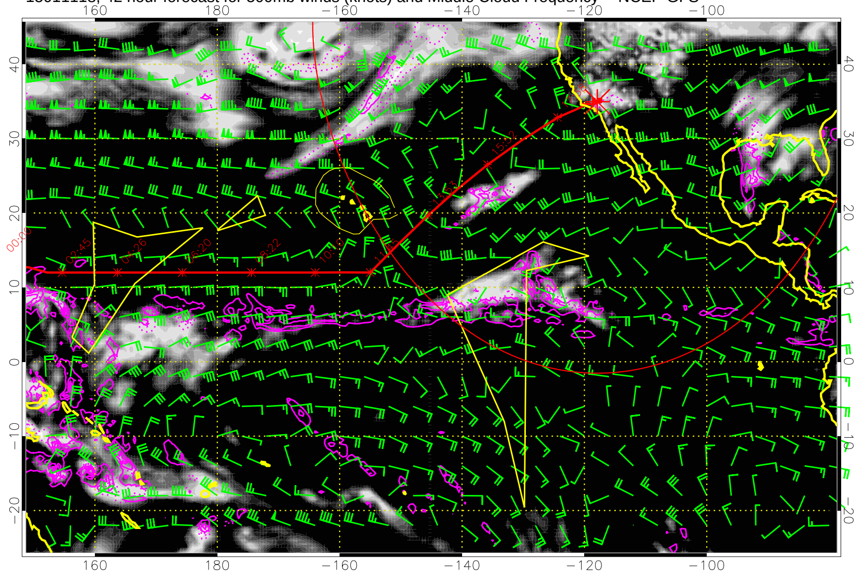
15011118, 42 hour forecast for 500mb winds (knots) and Middle Cloud Frequency -- NCEP GFS
