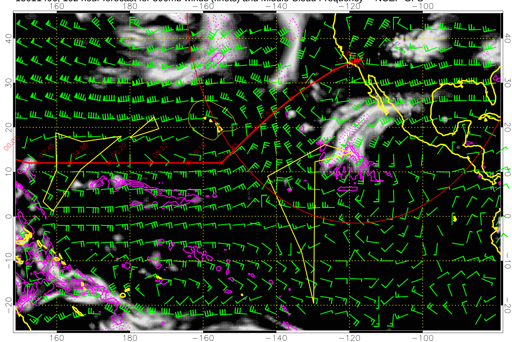
15011406, 102 hour forecast for 500mb winds (knots) and Middle Cloud Frequency -- NCEP GFS
