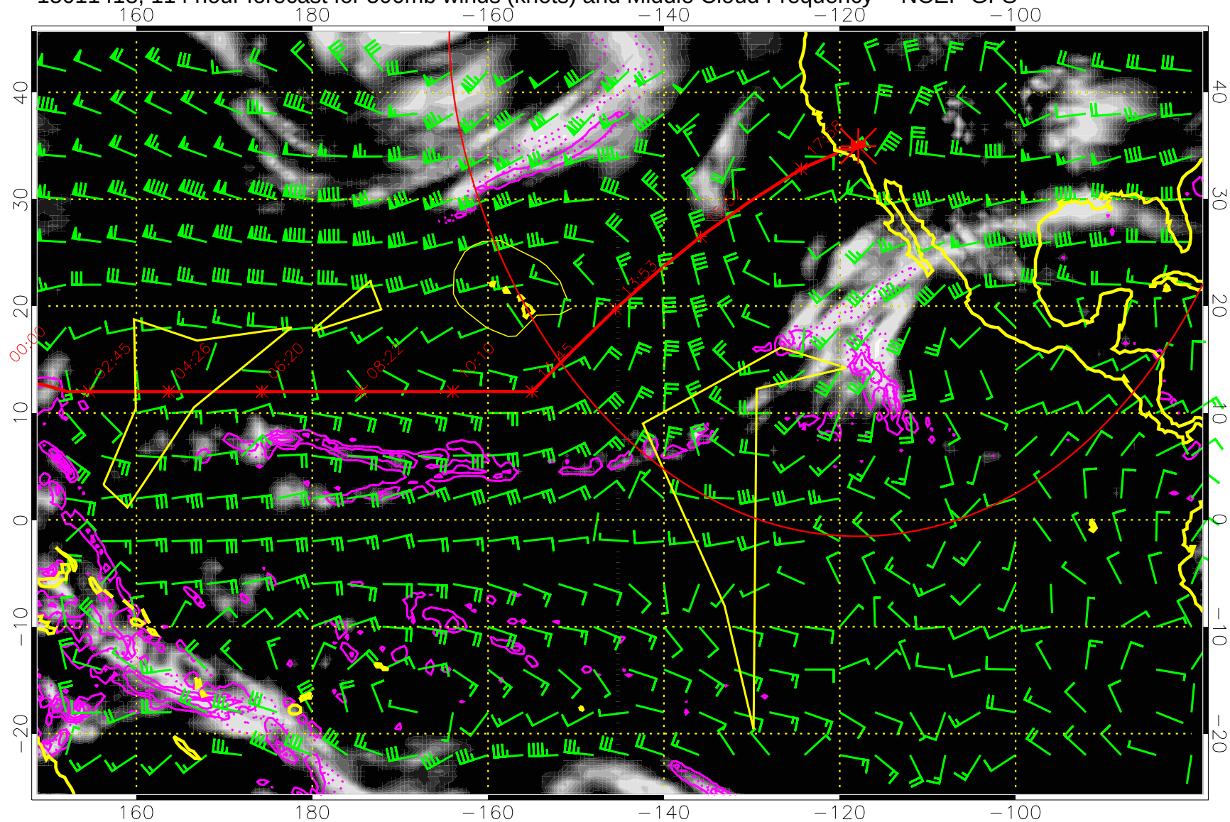
15011418, 114 hour forecast for 500mb winds (knots) and Middle Cloud Frequency -- NCEP GFS
