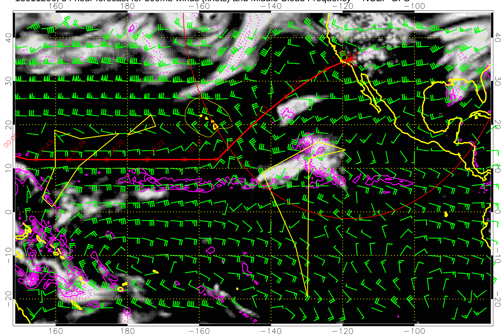
15011206, 54 hour forecast for 500mb winds (knots) and Middle Cloud Frequency -- NCEP GFS
