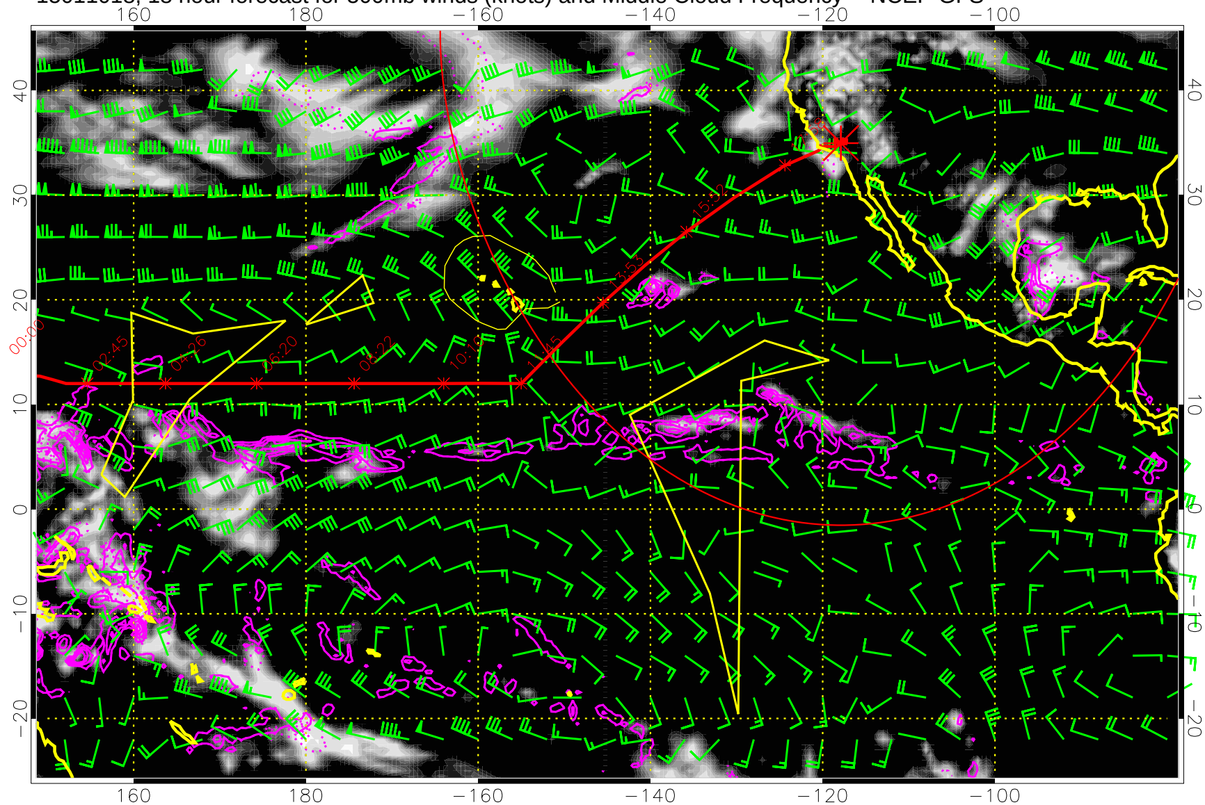
15011018, 18 hour forecast for 500mb winds (knots) and Middle Cloud Frequency -- NCEP GFS
