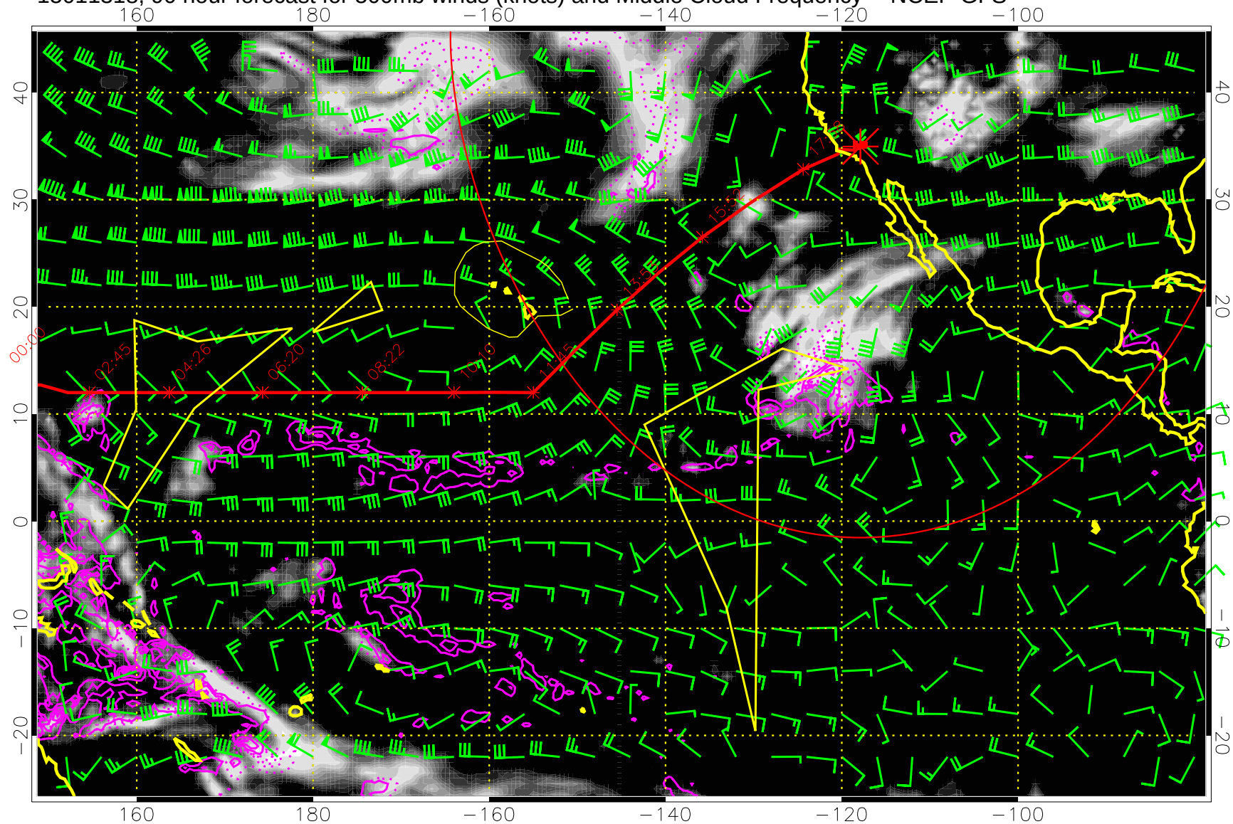
15011318, 90 hour forecast for 500mb winds (knots) and Middle Cloud Frequency -- NCEP GFS
