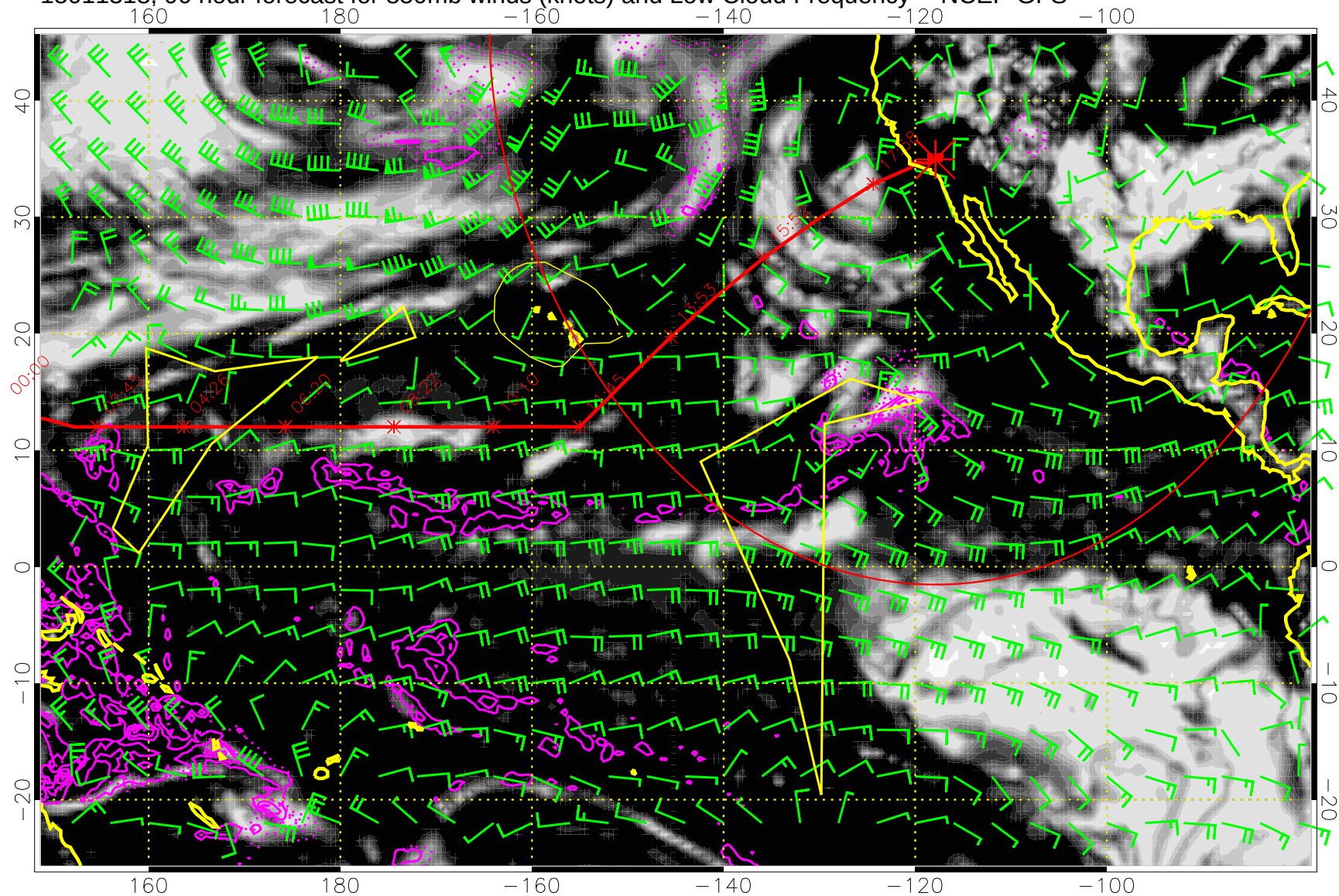
15011318, 90 hour forecast for 850mb winds (knots) and Low Cloud Frequency -- NCEP GFS
