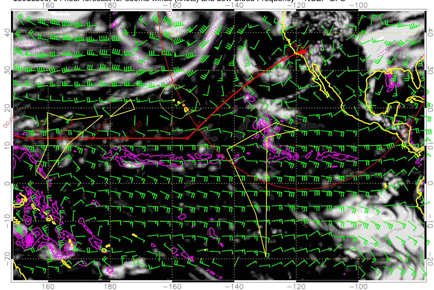
15011206, 54 hour forecast for 850mb winds (knots) and Low Cloud Frequency -- NCEP GFS
