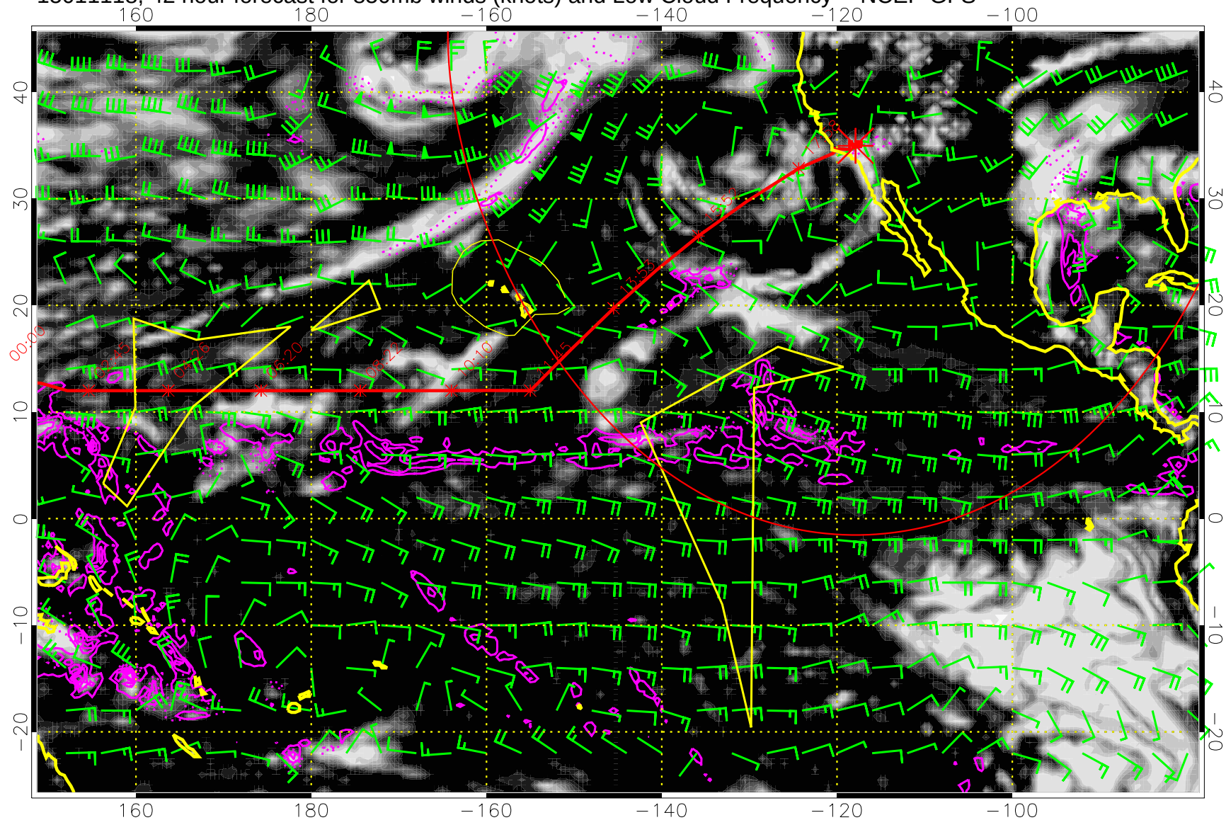
15011118, 42 hour forecast for 850mb winds (knots) and Low Cloud Frequency -- NCEP GFS
