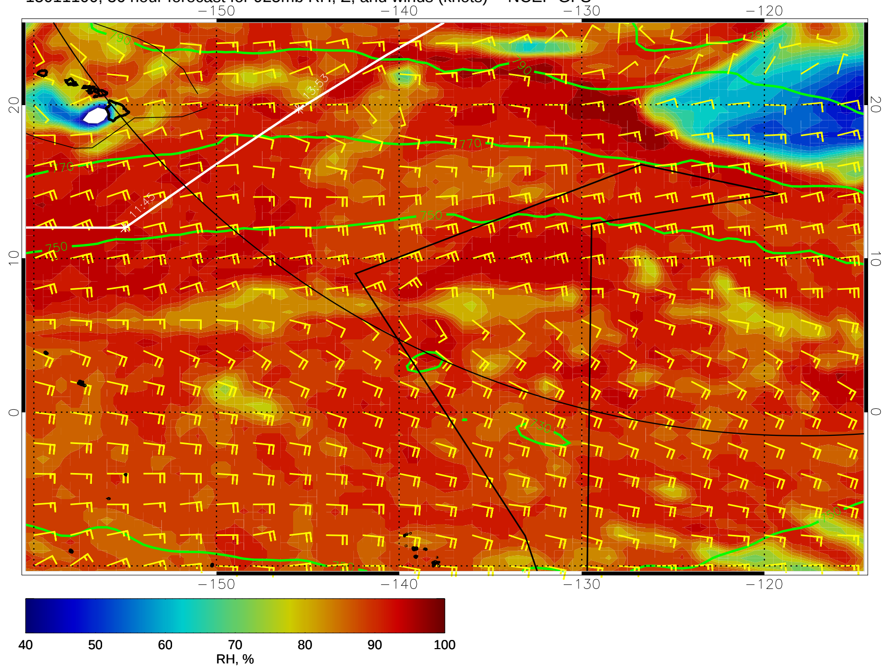
15011100, 36 hour forecast for 925mb RH, Z, and winds (knots) -- NCEP GFS
