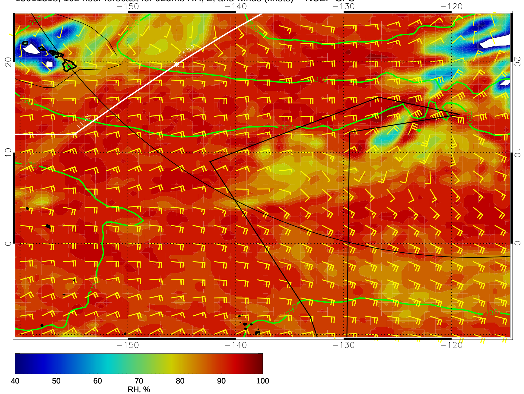
15011318, 102 hour forecast for 925mb RH, Z, and winds (knots) -- NCEP GFS
