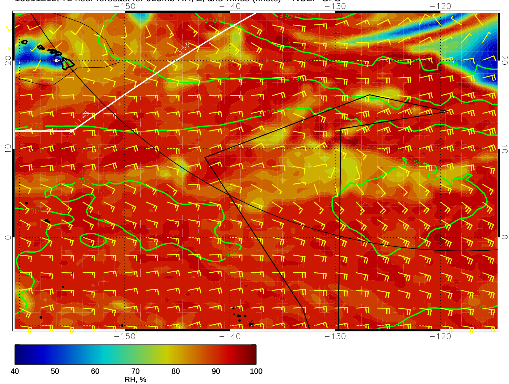
15011212, 72 hour forecast for 925mb RH, Z, and winds (knots) -- NCEP GFS
