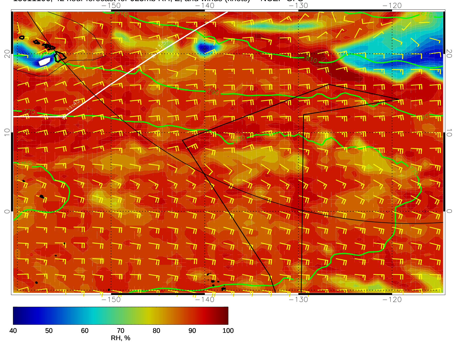
15011106, 42 hour forecast for 925mb RH, Z, and winds (knots) -- NCEP GFS
