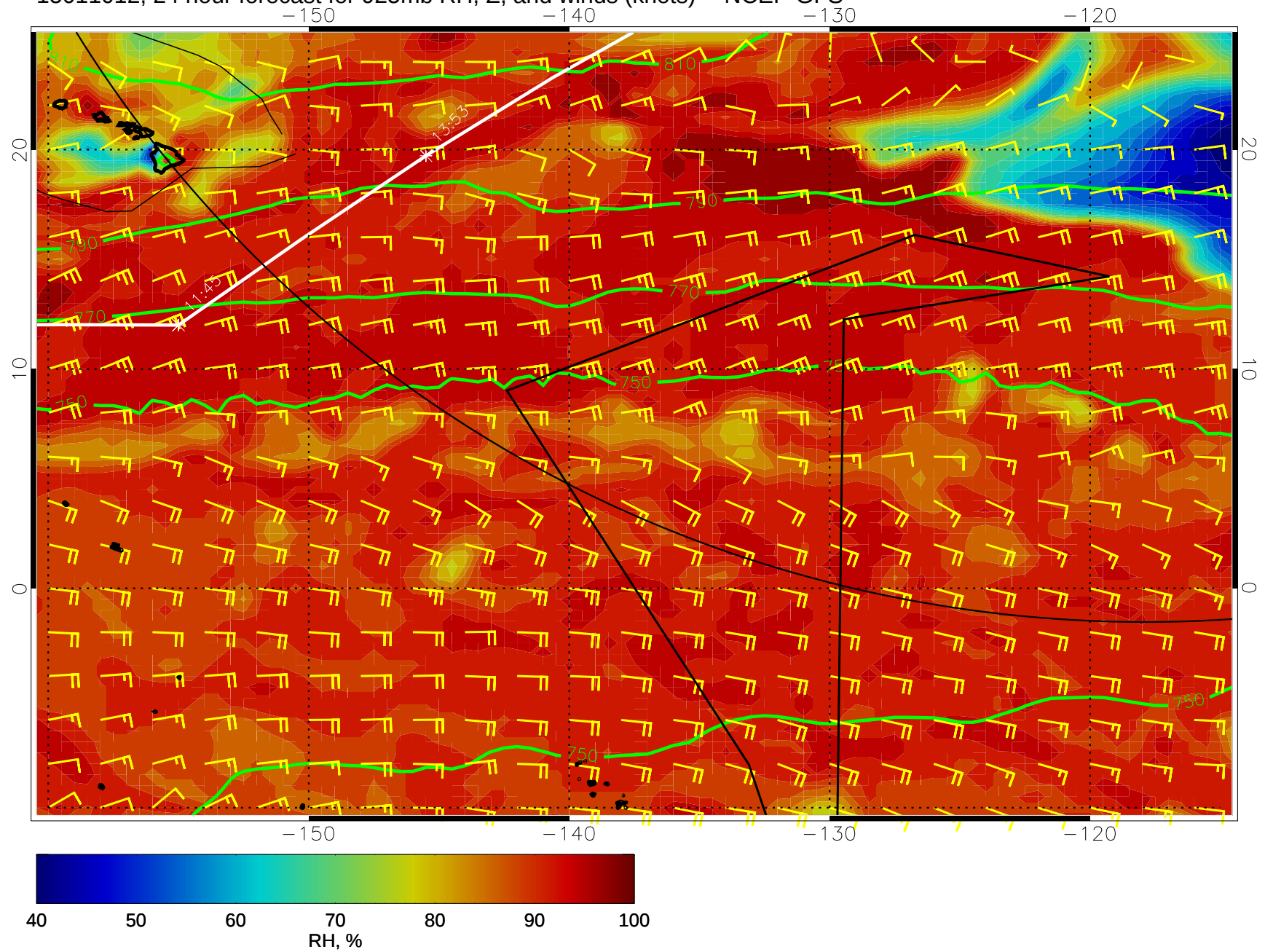
15011012, 24 hour forecast for 925mb RH, Z, and winds (knots) -- NCEP GFS
