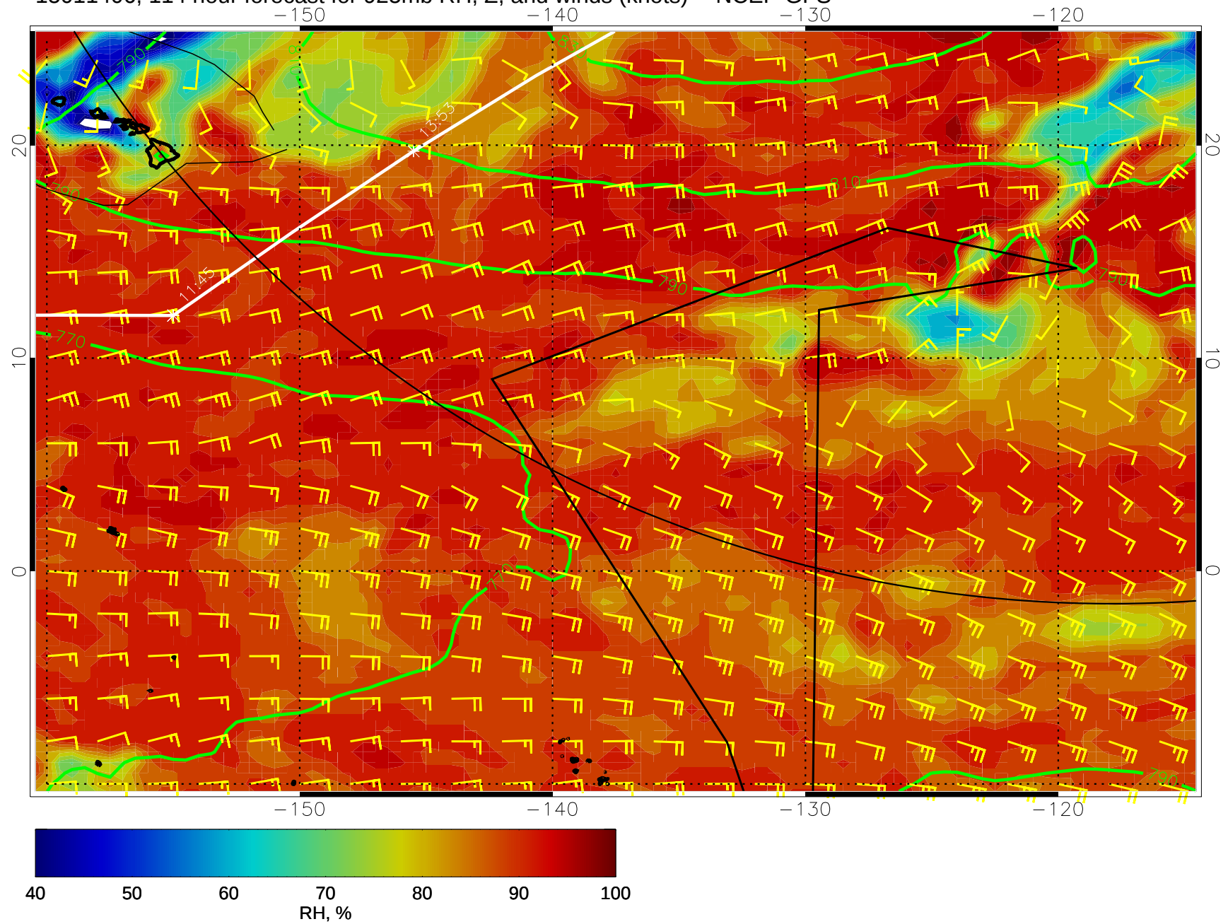
15011406, 114 hour forecast for 925mb RH, Z, and winds (knots) -- NCEP GFS
