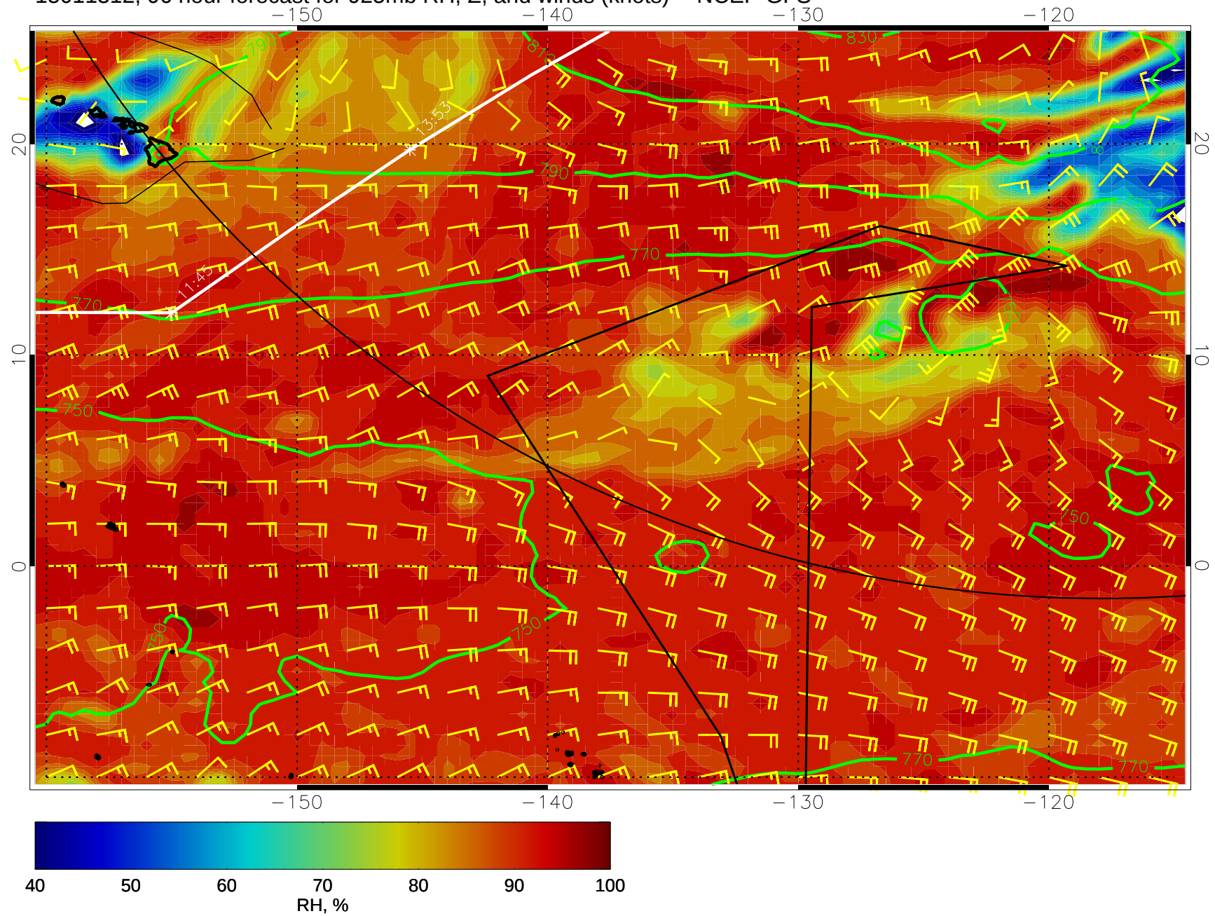
15011312, 96 hour forecast for 925mb RH, Z, and winds (knots) -- NCEP GFS
