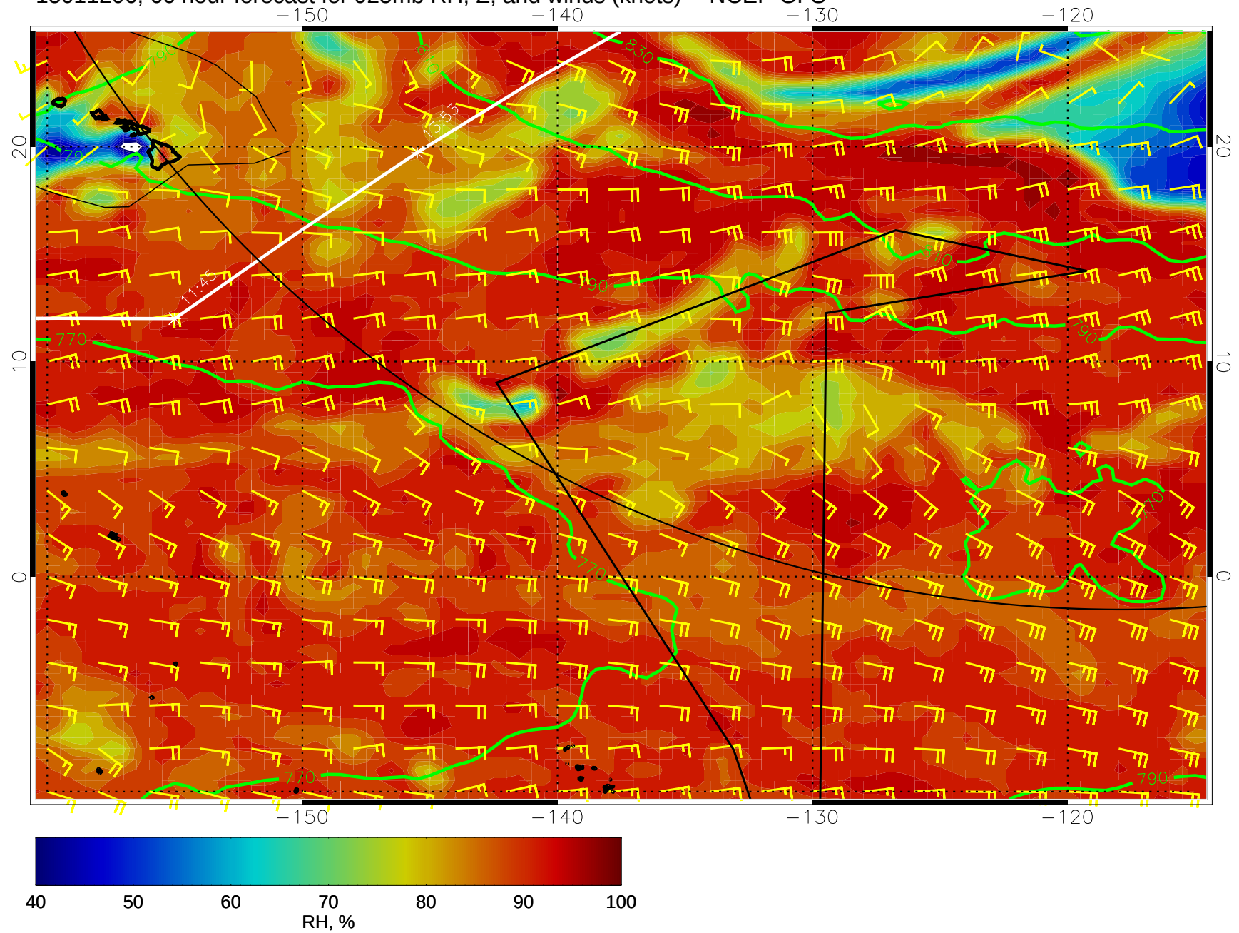
15011206, 66 hour forecast for 925mb RH, Z, and winds (knots) -- NCEP GFS
