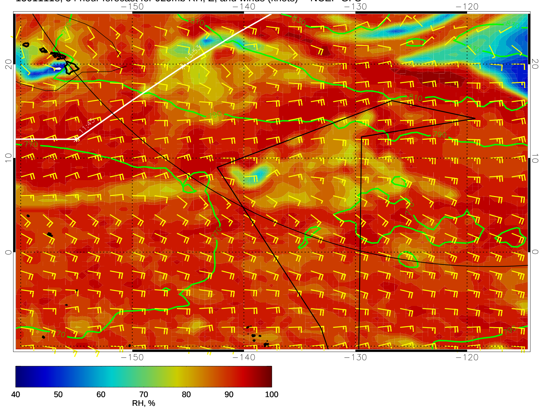
15011118, 54 hour forecast for 925mb RH, Z, and winds (knots) -- NCEP GFS
