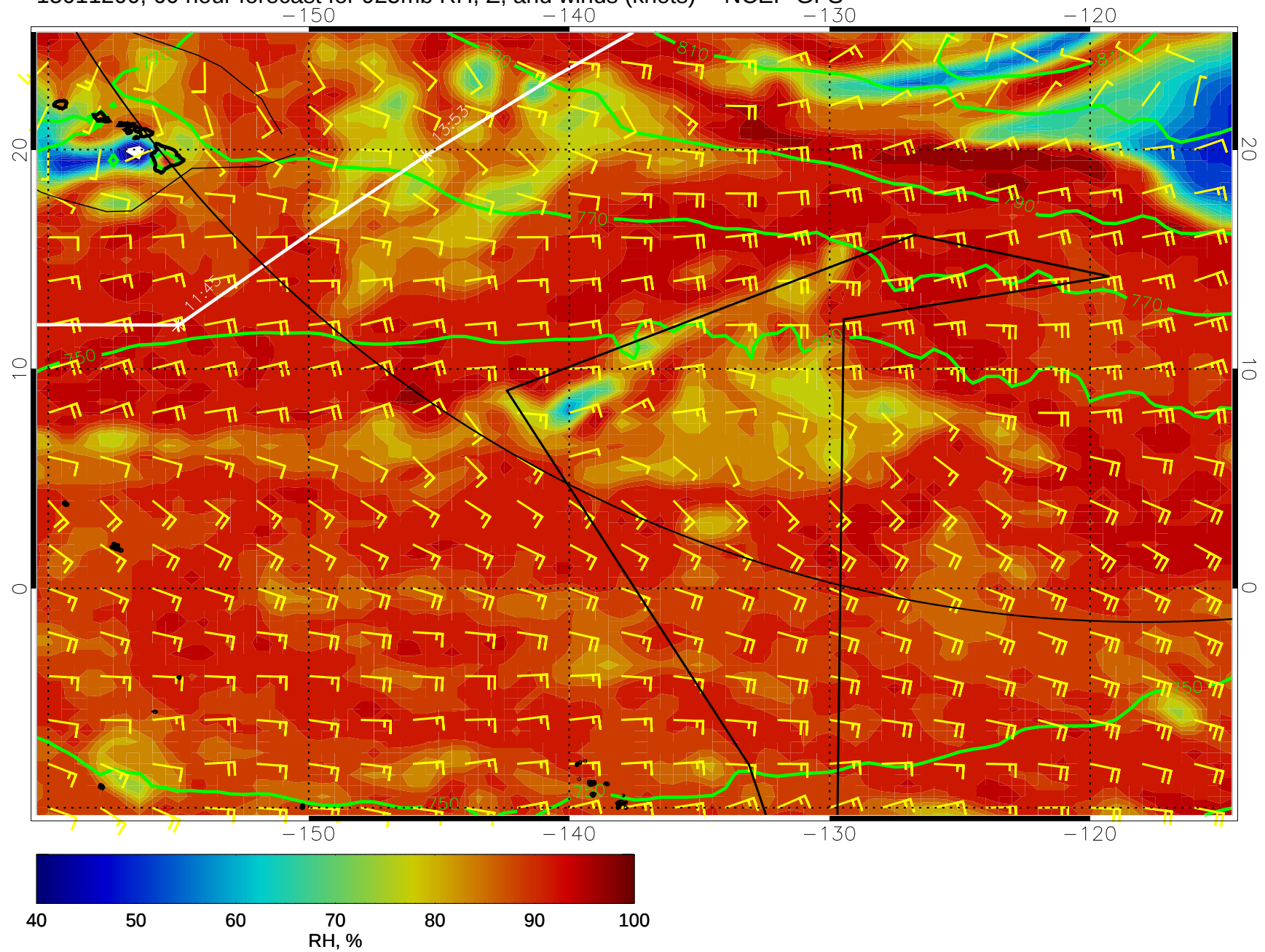
15011200, 60 hour forecast for 925mb RH, Z, and winds (knots) -- NCEP GFS
