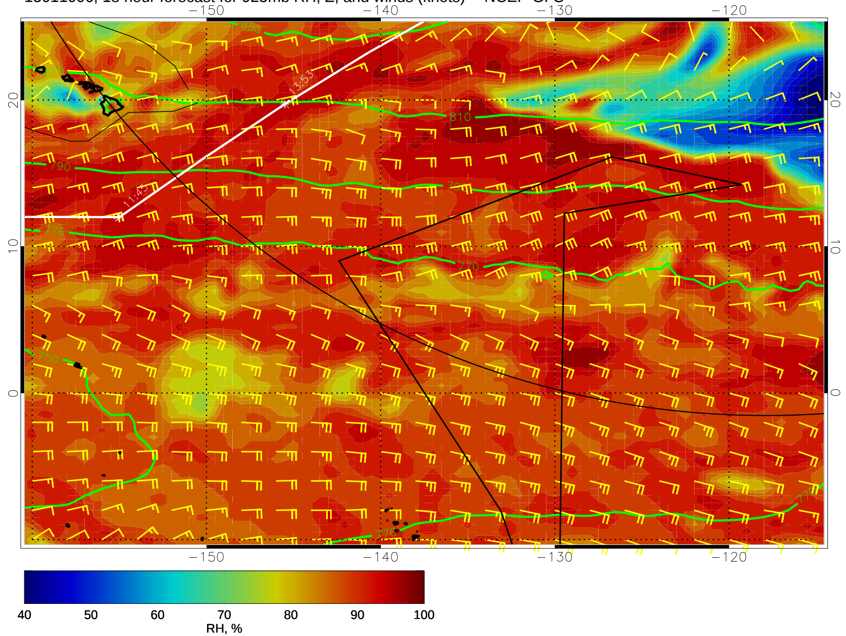
15011006, 18 hour forecast for 925mb RH, Z, and winds (knots) -- NCEP GFS
