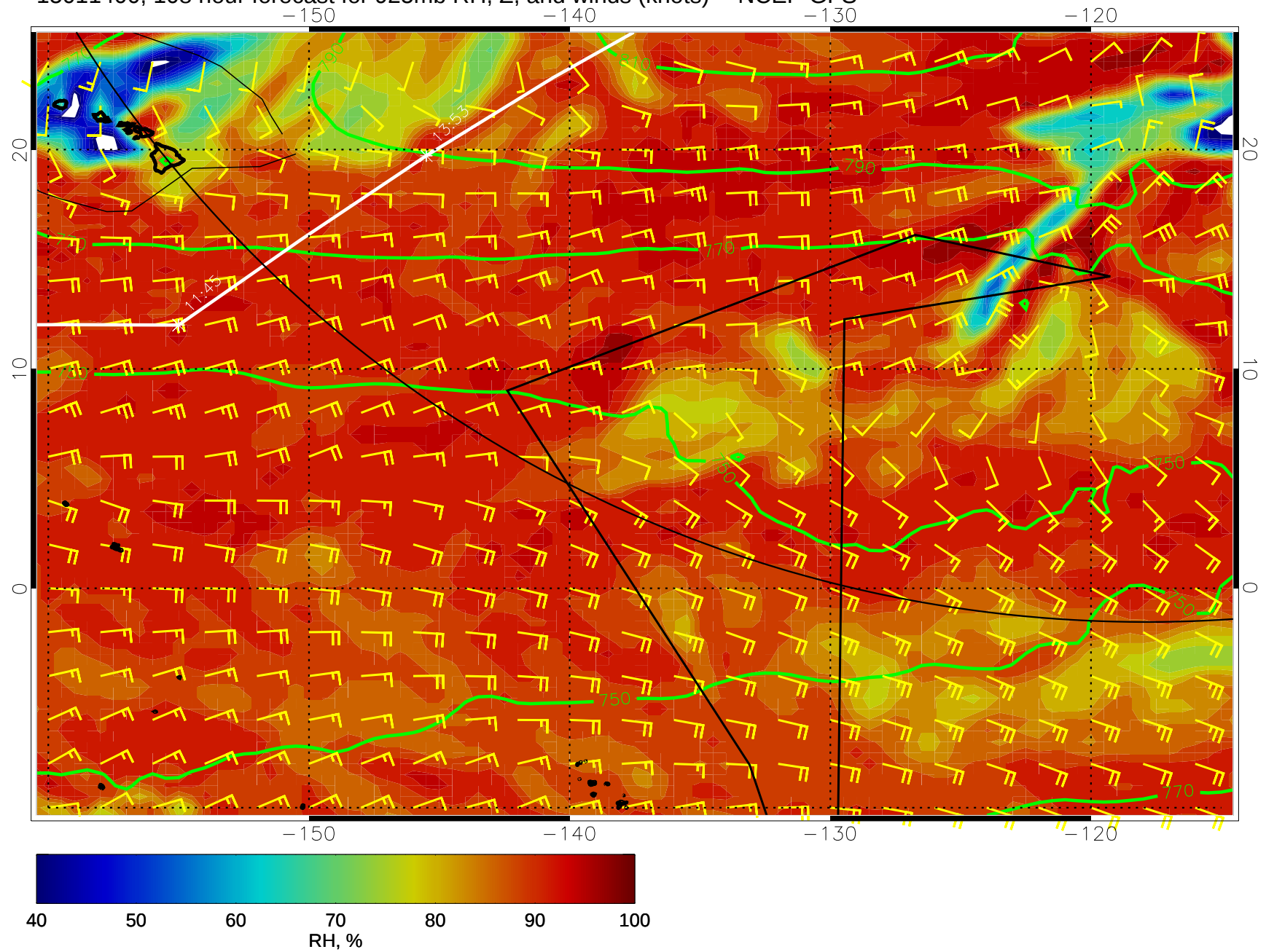
15011400, 108 hour forecast for 925mb RH, Z, and winds (knots) -- NCEP GFS
