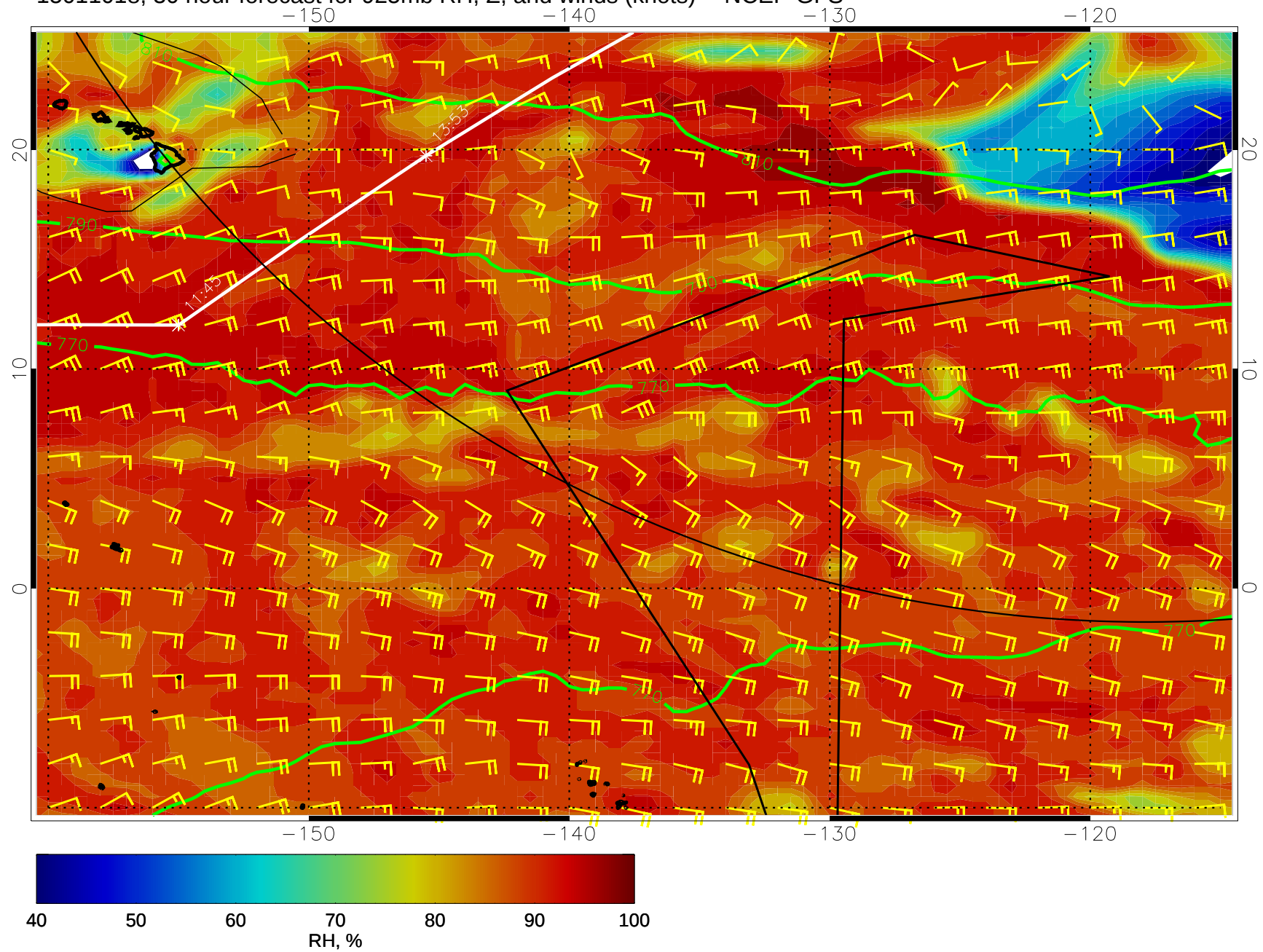
15011018, 30 hour forecast for 925mb RH, Z, and winds (knots) -- NCEP GFS
