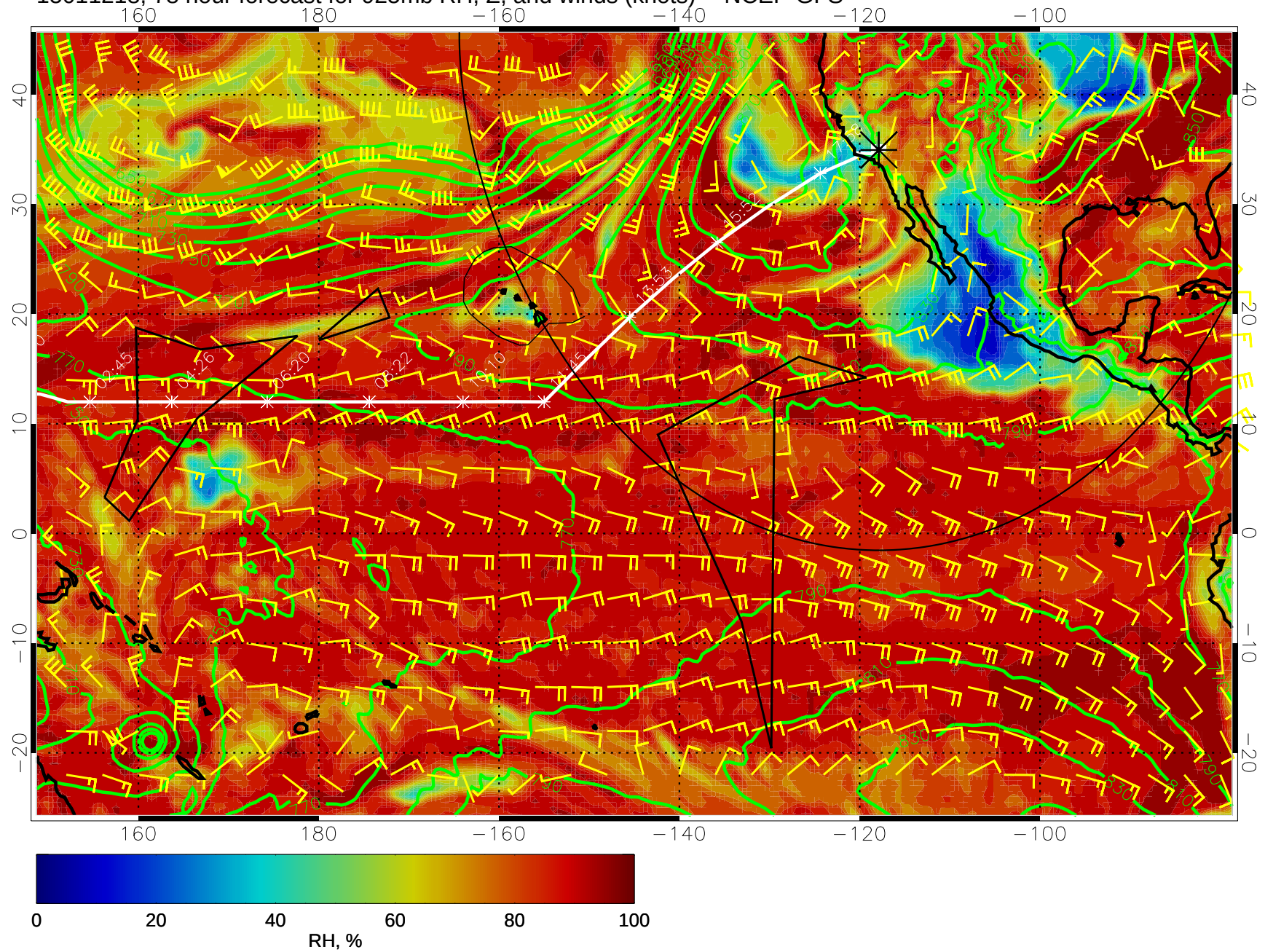
15011218, 78 hour forecast for 925mb RH, Z, and winds (knots) -- NCEP GFS
