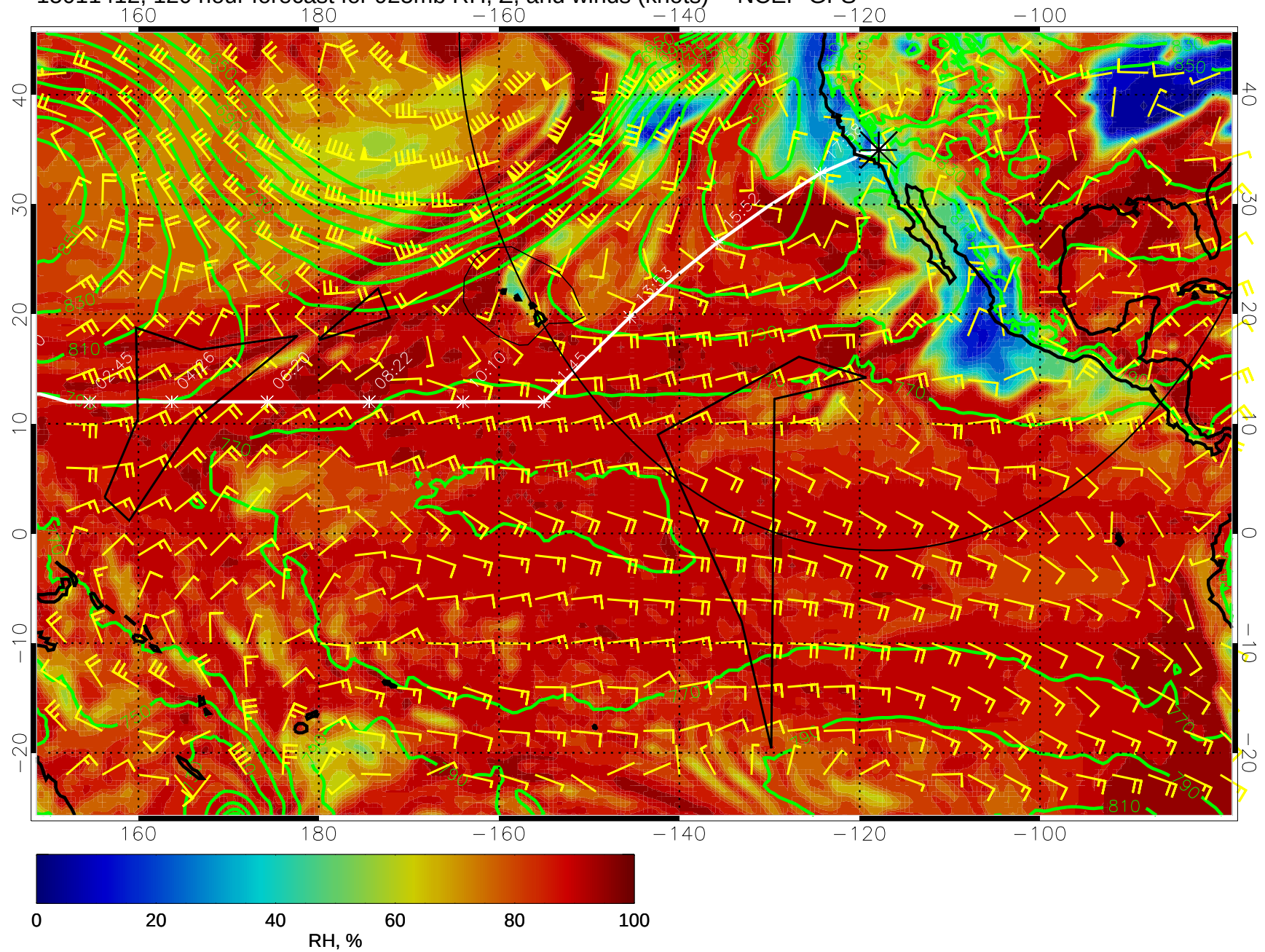
15011412, 120 hour forecast for 925mb RH, Z, and winds (knots) -- NCEP GFS
