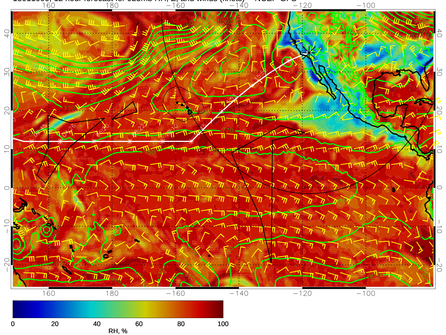
15011000, 12 hour forecast for 925mb RH, Z, and winds (knots) -- NCEP GFS
