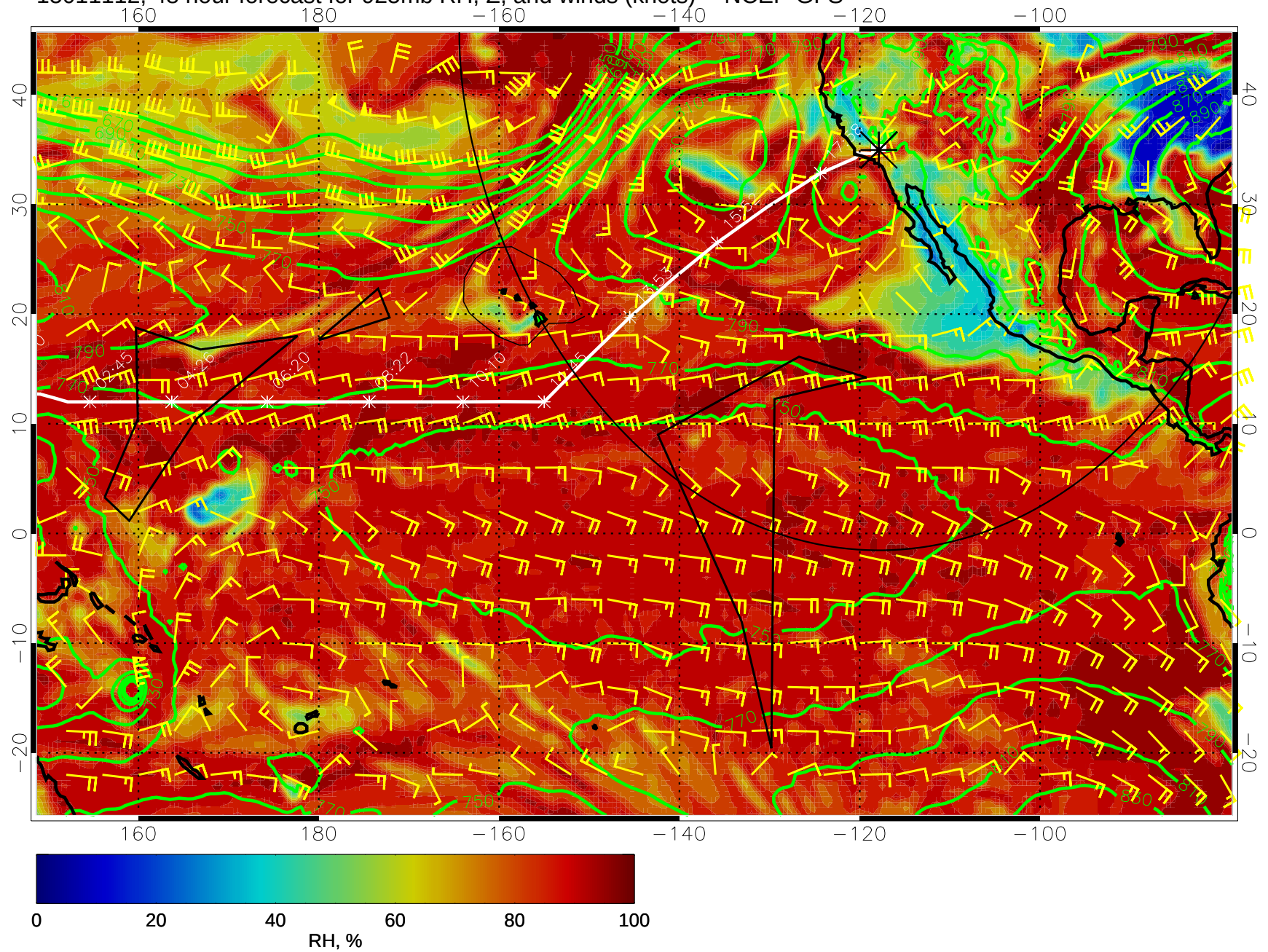
15011112, 48 hour forecast for 925mb RH, Z, and winds (knots) -- NCEP GFS
