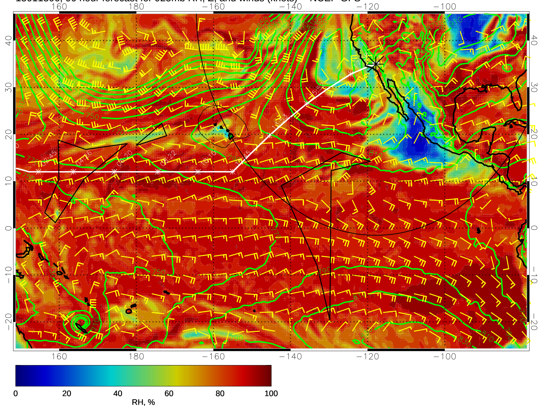
15011306, 90 hour forecast for 925mb RH, Z, and winds (knots) -- NCEP GFS
