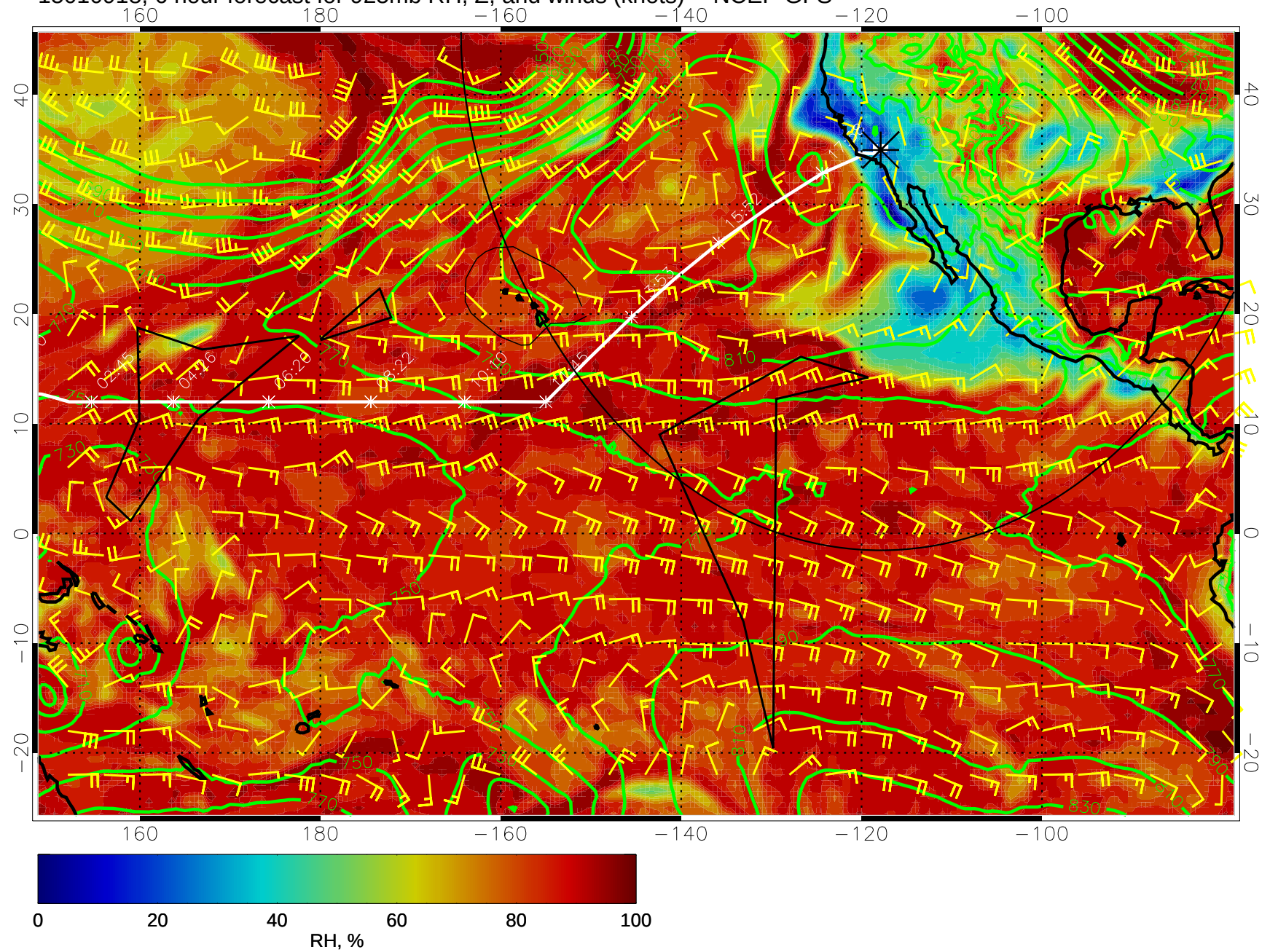
15010918, 6 hour forecast for 925mb RH, Z, and winds (knots) -- NCEP GFS
