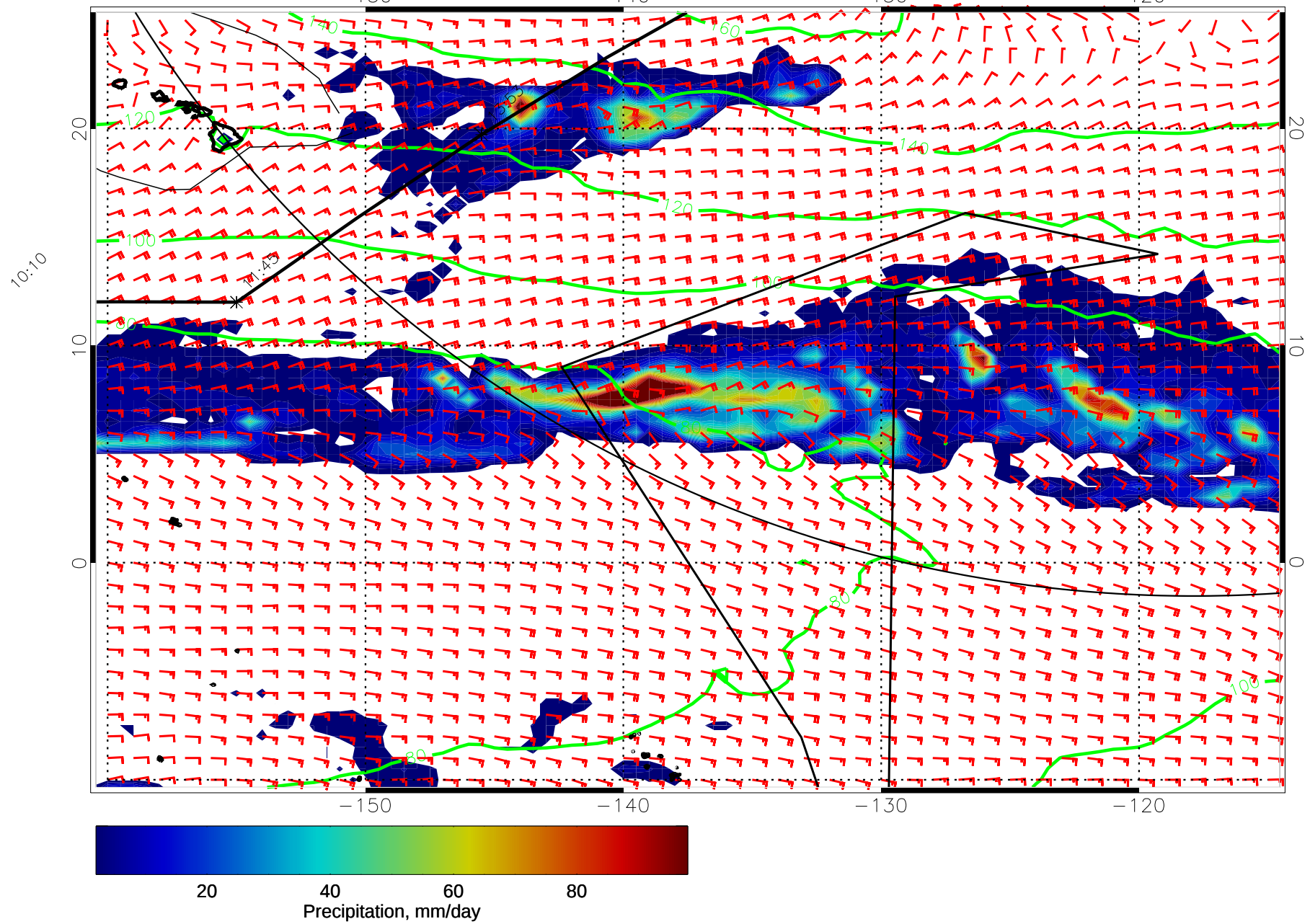
15011106, 42 hour forecast for precip, 1000mb Z, and winds (knots) -- NCEP GFS
