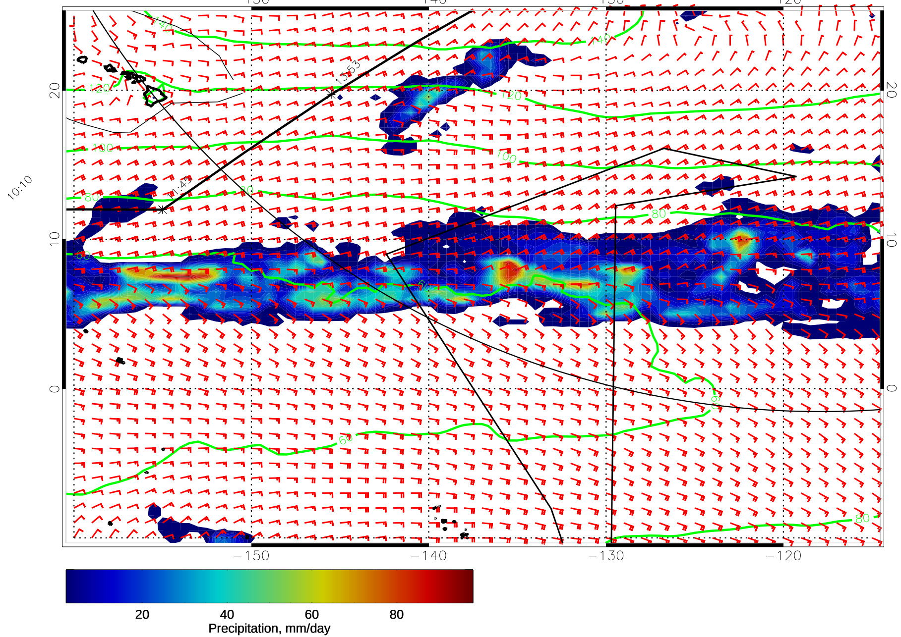
15011000, 12 hour forecast for precip, 1000mb Z, and winds (knots) -- NCEP GFS
