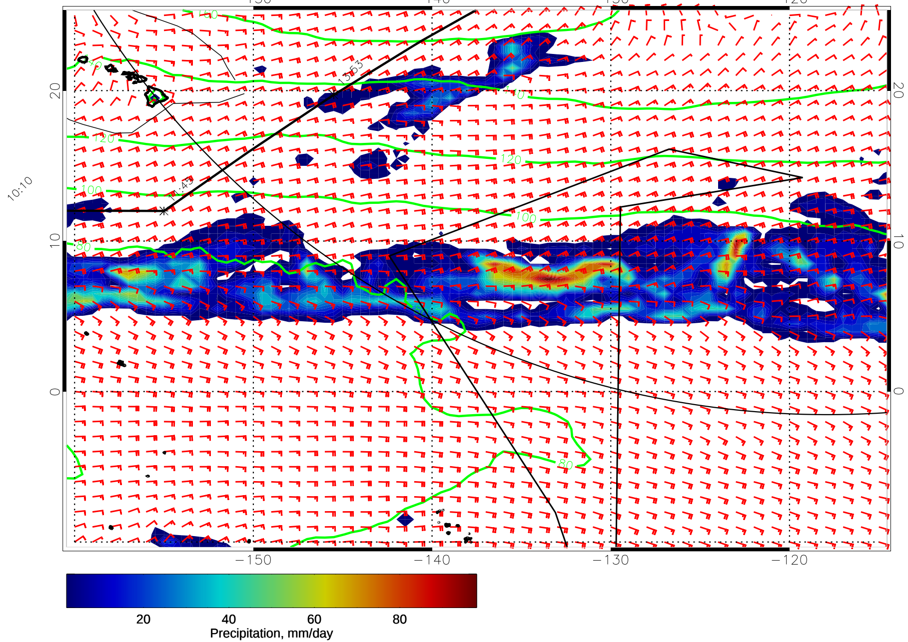
15011006, 18 hour forecast for precip, 1000mb Z, and winds (knots) -- NCEP GFS
