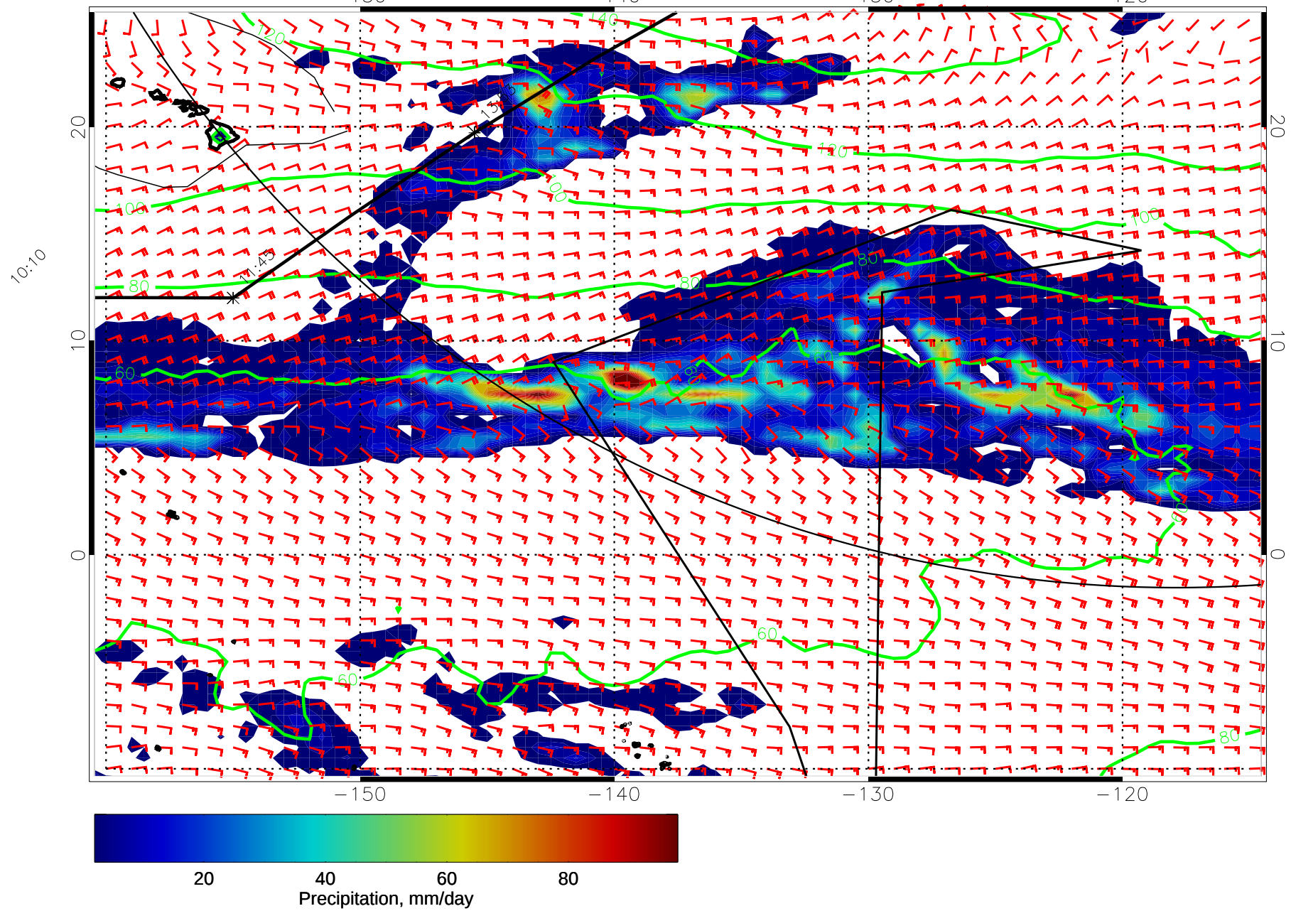
15011112, 48 hour forecast for precip, 1000mb Z, and winds (knots) -- NCEP GFS
