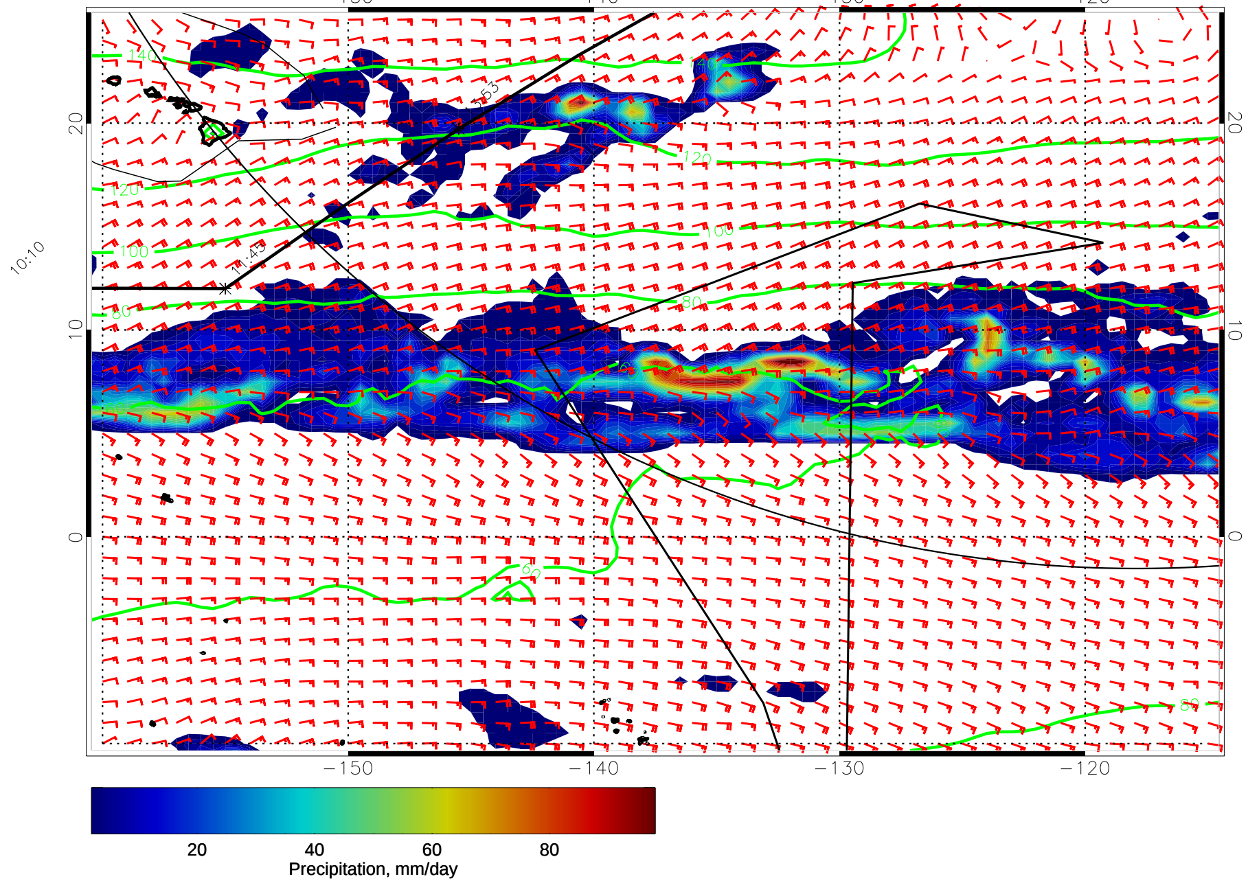
15011012, 24 hour forecast for precip, 1000mb Z, and winds (knots) -- NCEP GFS
