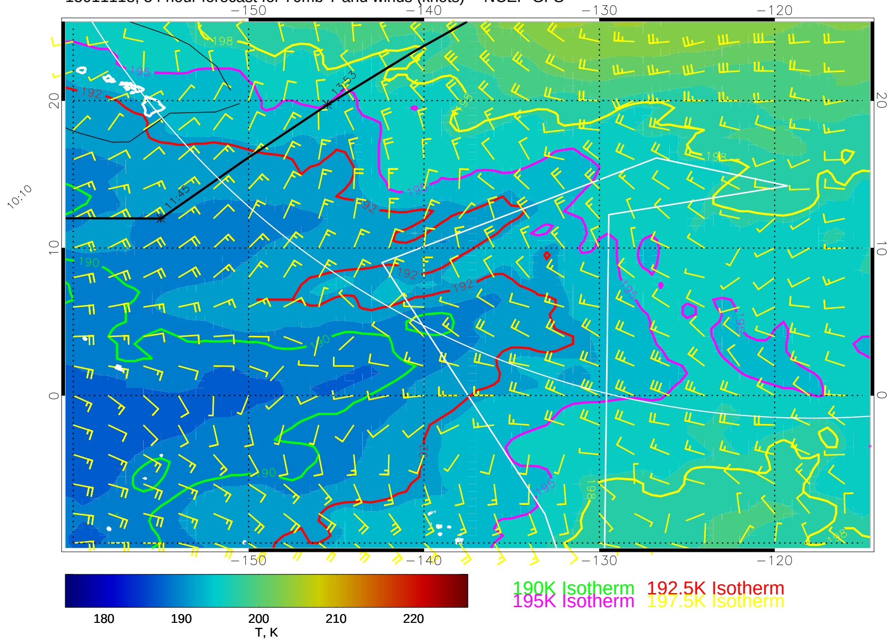
15011118, 54 hour forecast for 70mb T and winds (knots) -- NCEP GFS
