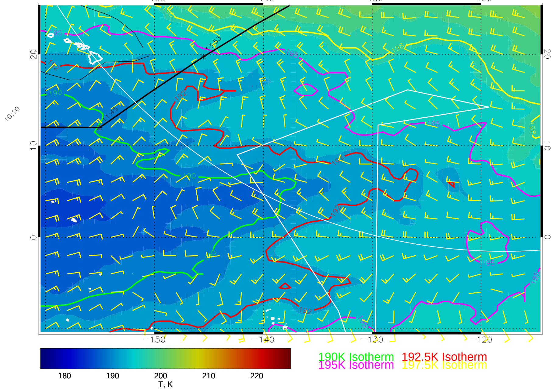
15011012, 24 hour forecast for 70mb T and winds (knots) -- NCEP GFS
