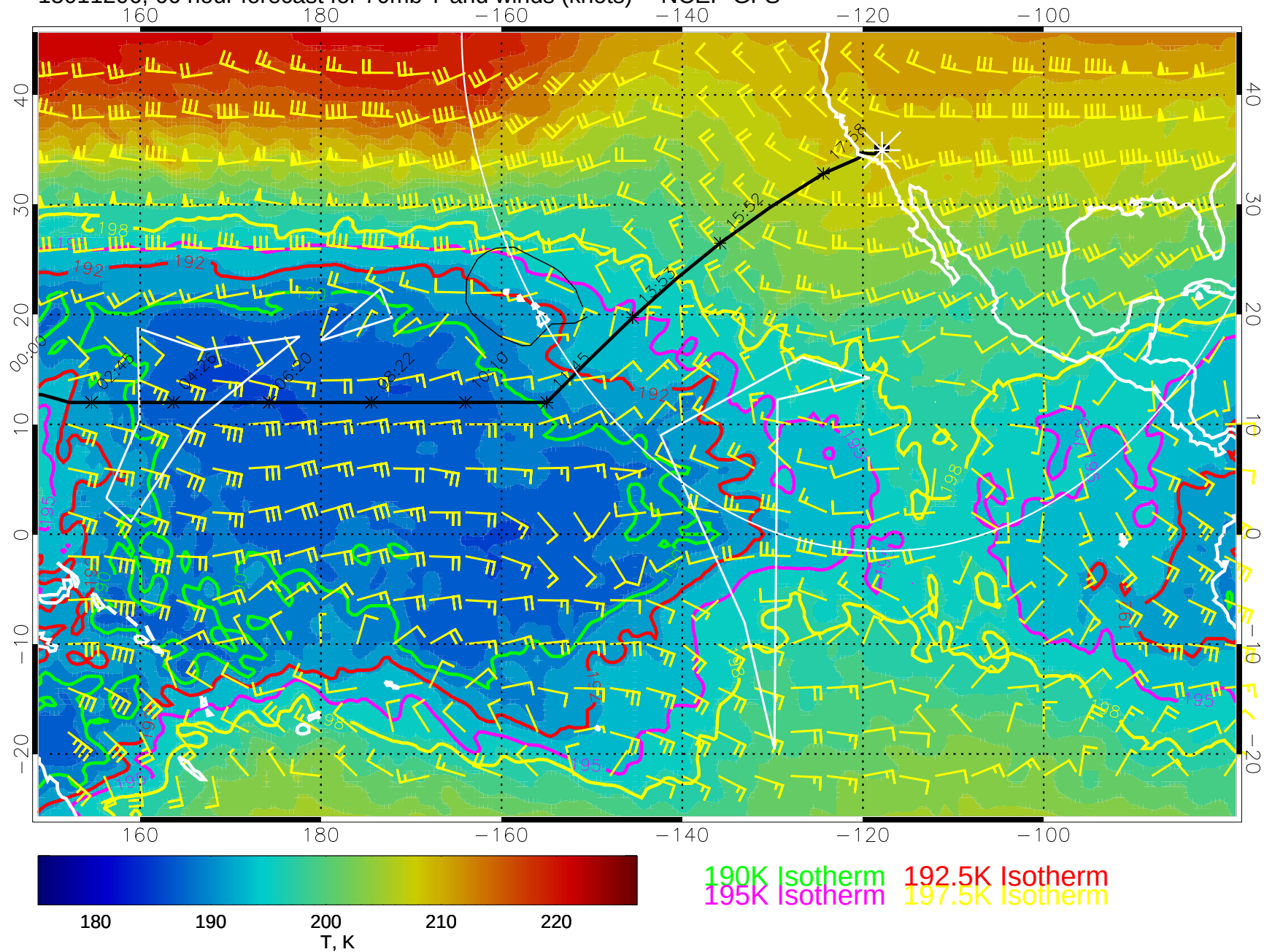
15011206, 66 hour forecast for 70mb T and winds (knots) -- NCEP GFS
