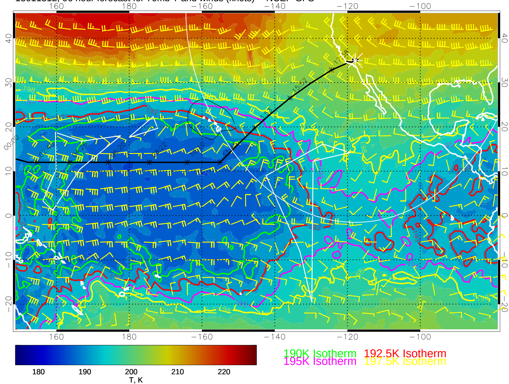
15011312, 96 hour forecast for 70mb T and winds (knots) -- NCEP GFS
