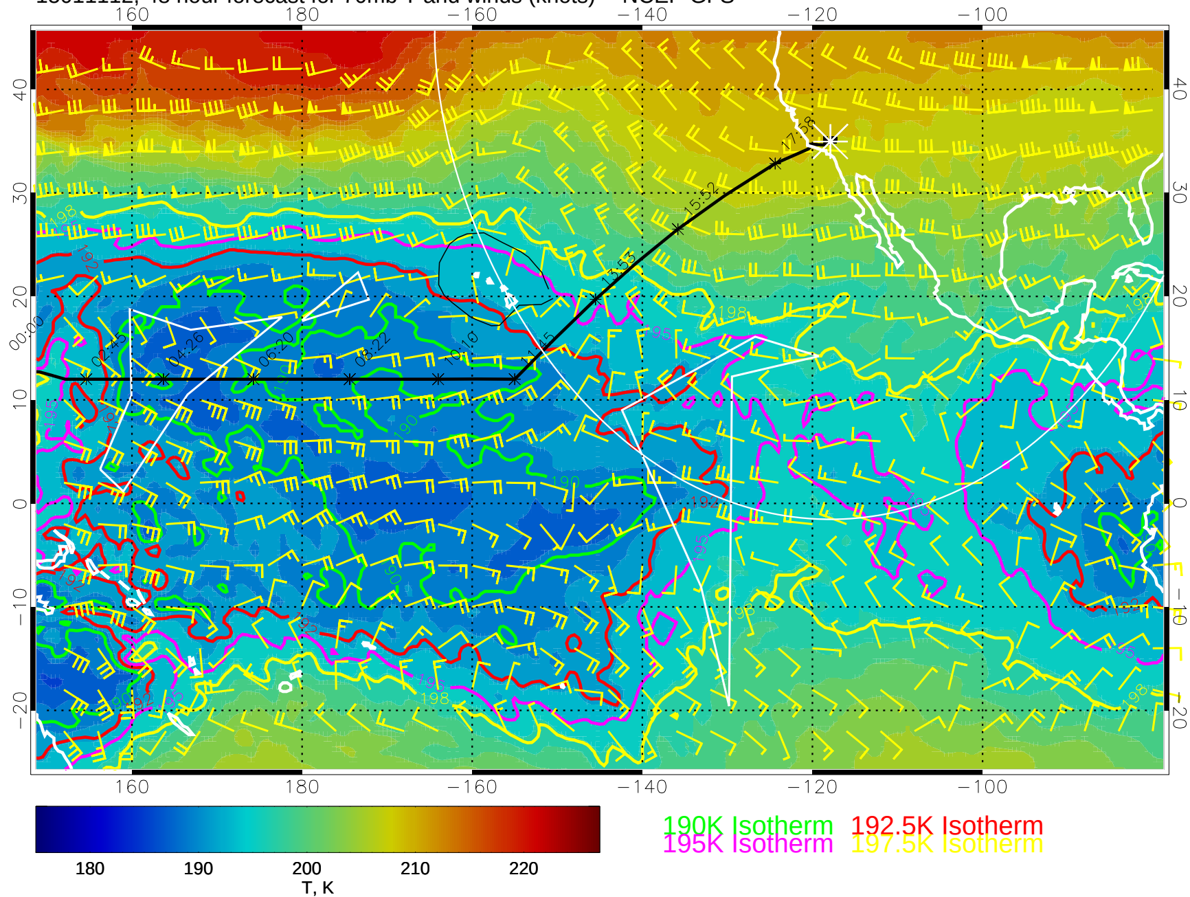
15011112, 48 hour forecast for 70mb T and winds (knots) -- NCEP GFS
