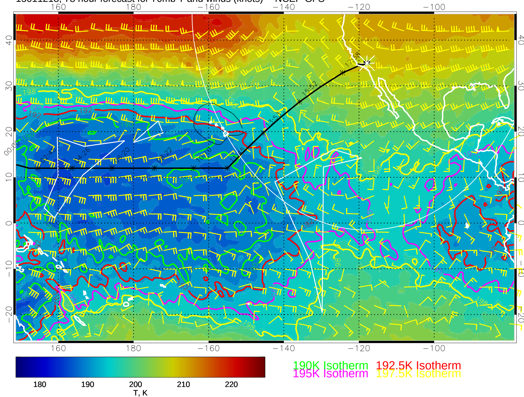
15011218, 78 hour forecast for 70mb T and winds (knots) -- NCEP GFS
