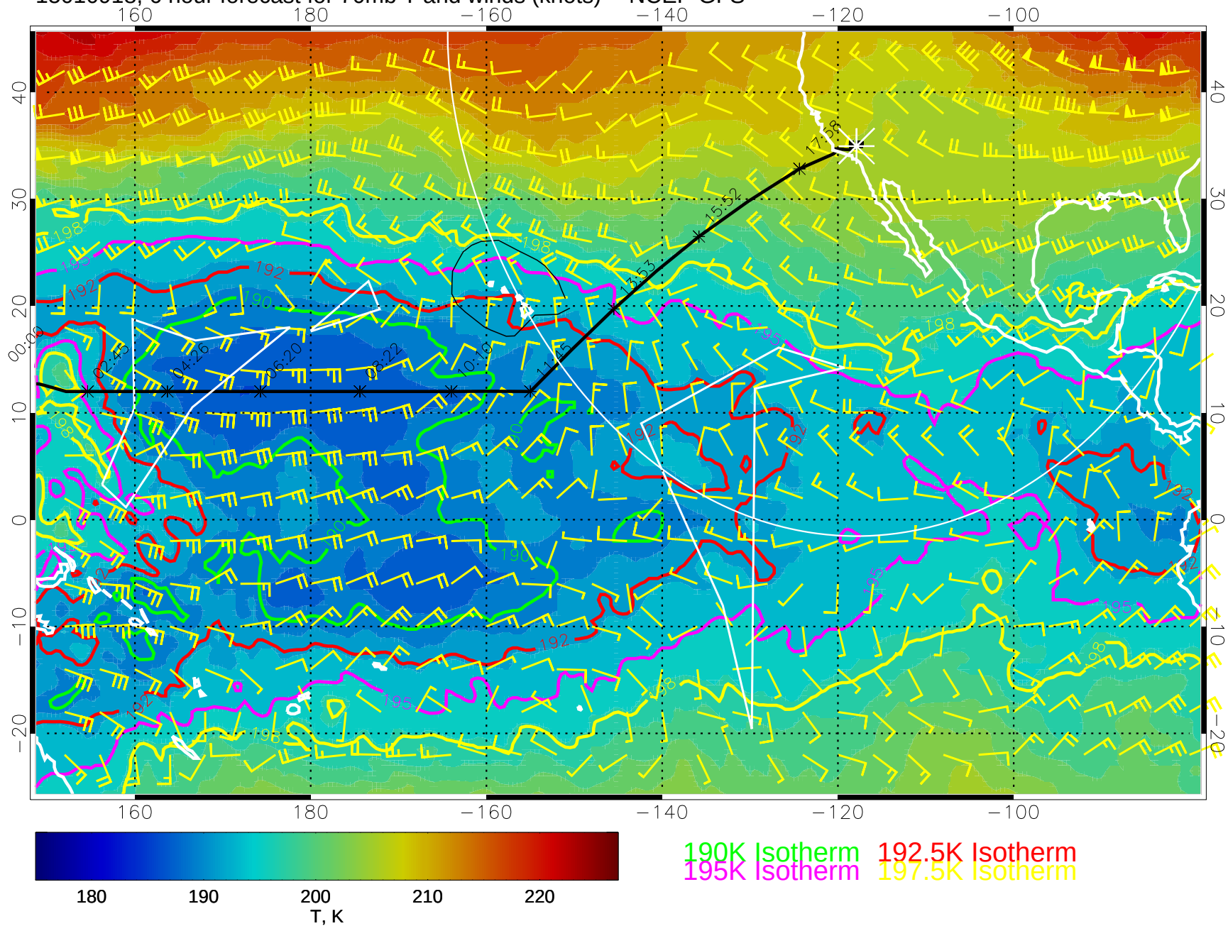
15010918, 6 hour forecast for 70mb T and winds (knots) -- NCEP GFS
