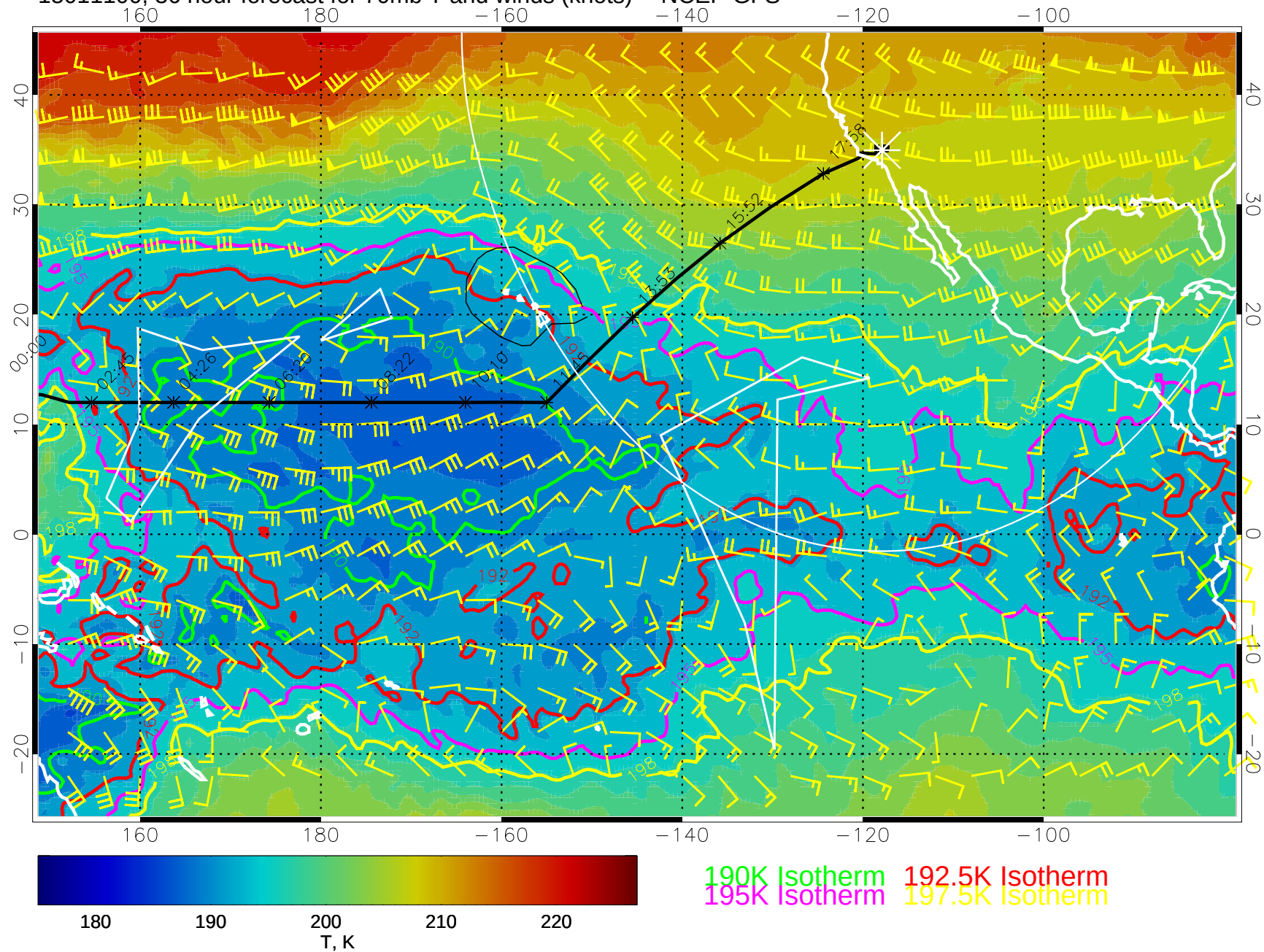
15011100, 36 hour forecast for 70mb T and winds (knots) -- NCEP GFS
