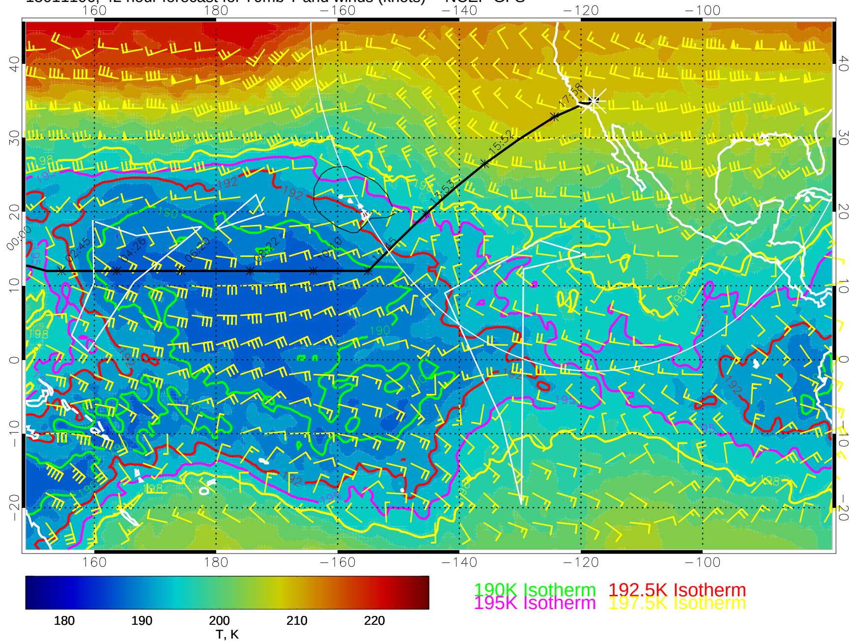
15011106, 42 hour forecast for 70mb T and winds (knots) -- NCEP GFS
