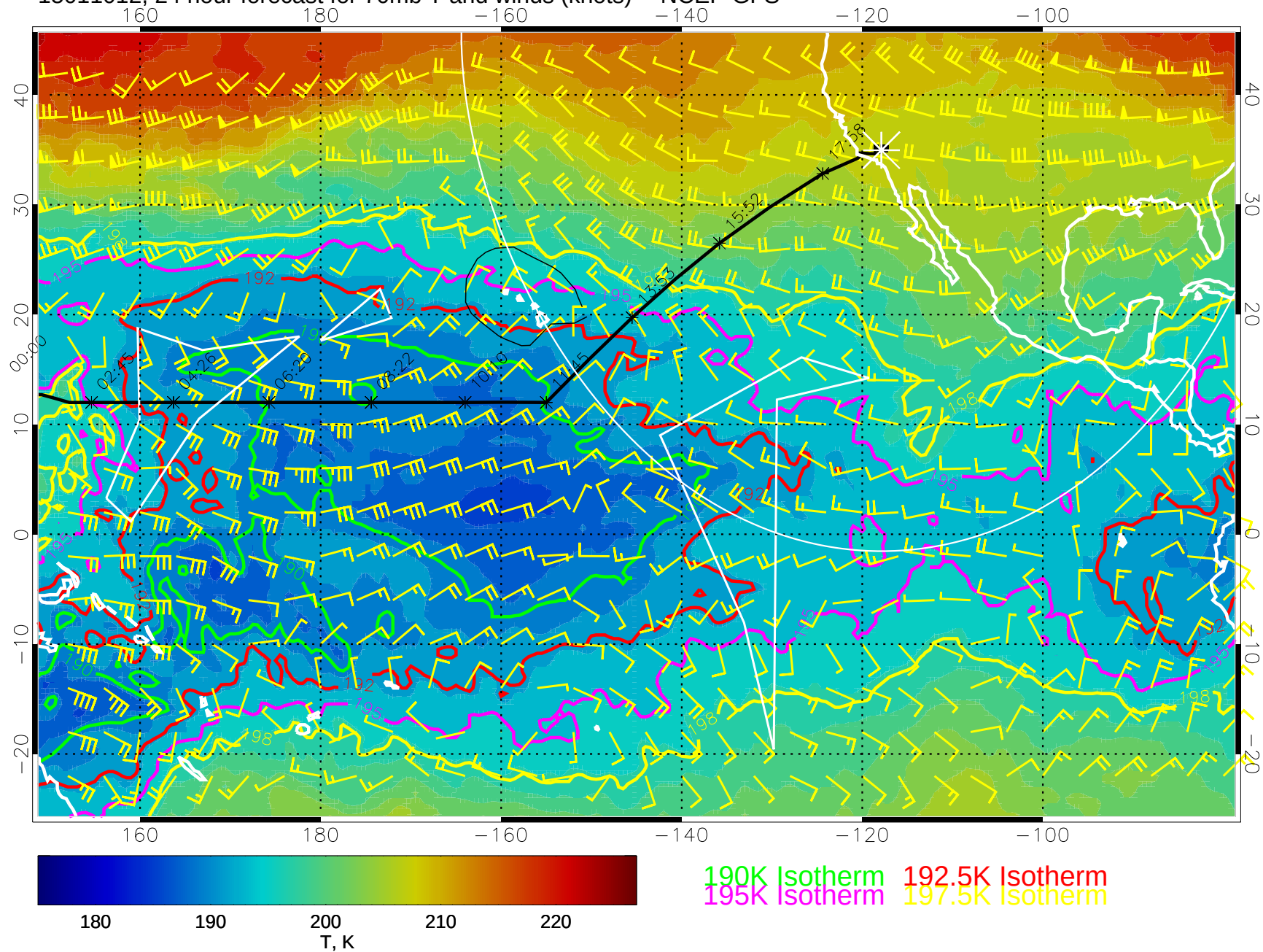
15011012, 24 hour forecast for 70mb T and winds (knots) -- NCEP GFS
