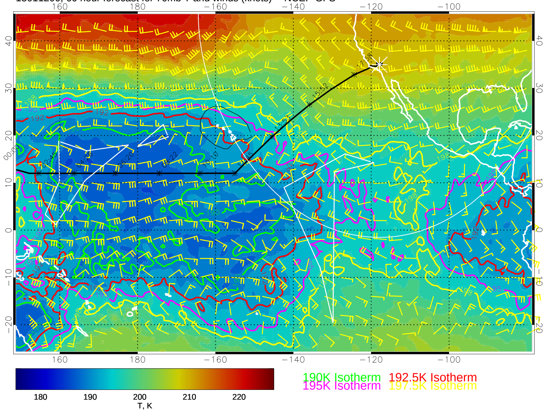
15011200, 60 hour forecast for 70mb T and winds (knots) -- NCEP GFS
