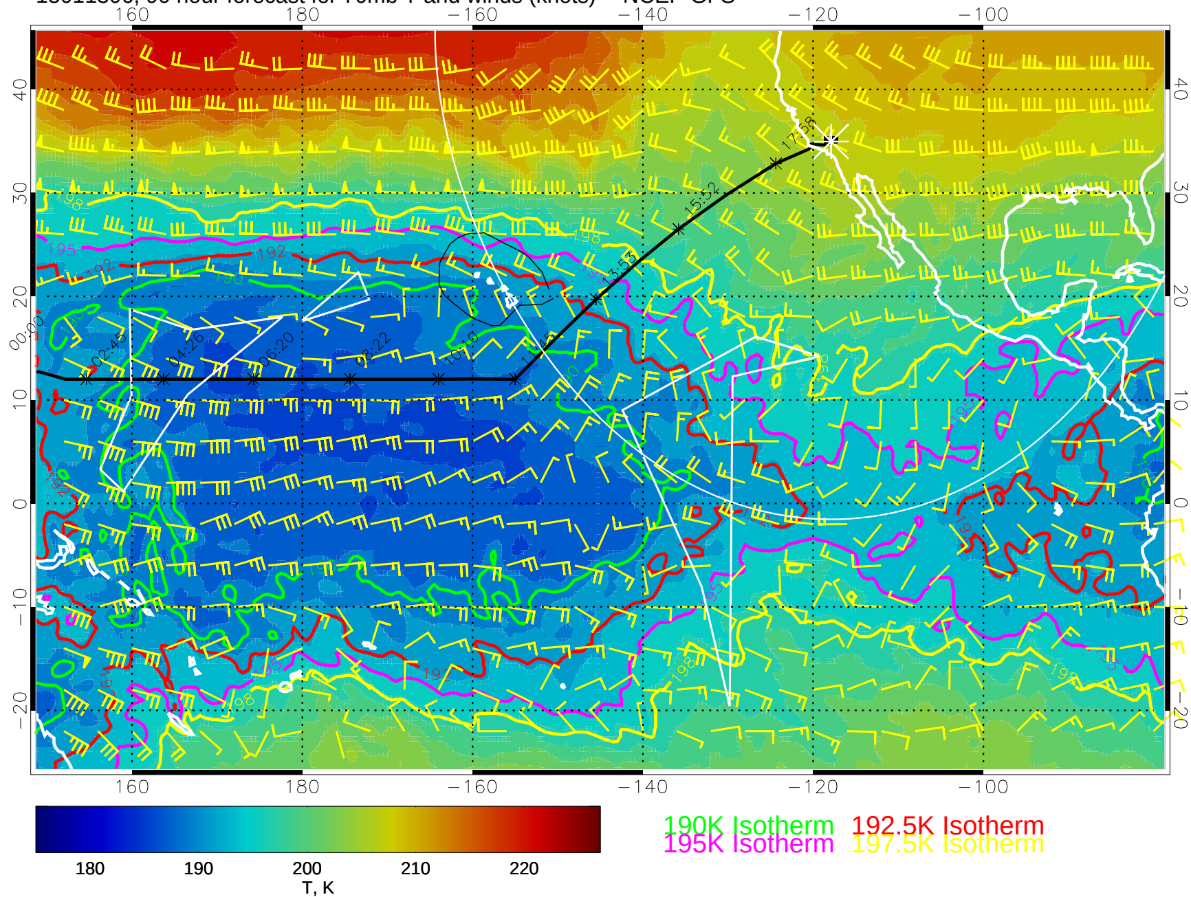
15011306, 90 hour forecast for 70mb T and winds (knots) -- NCEP GFS
