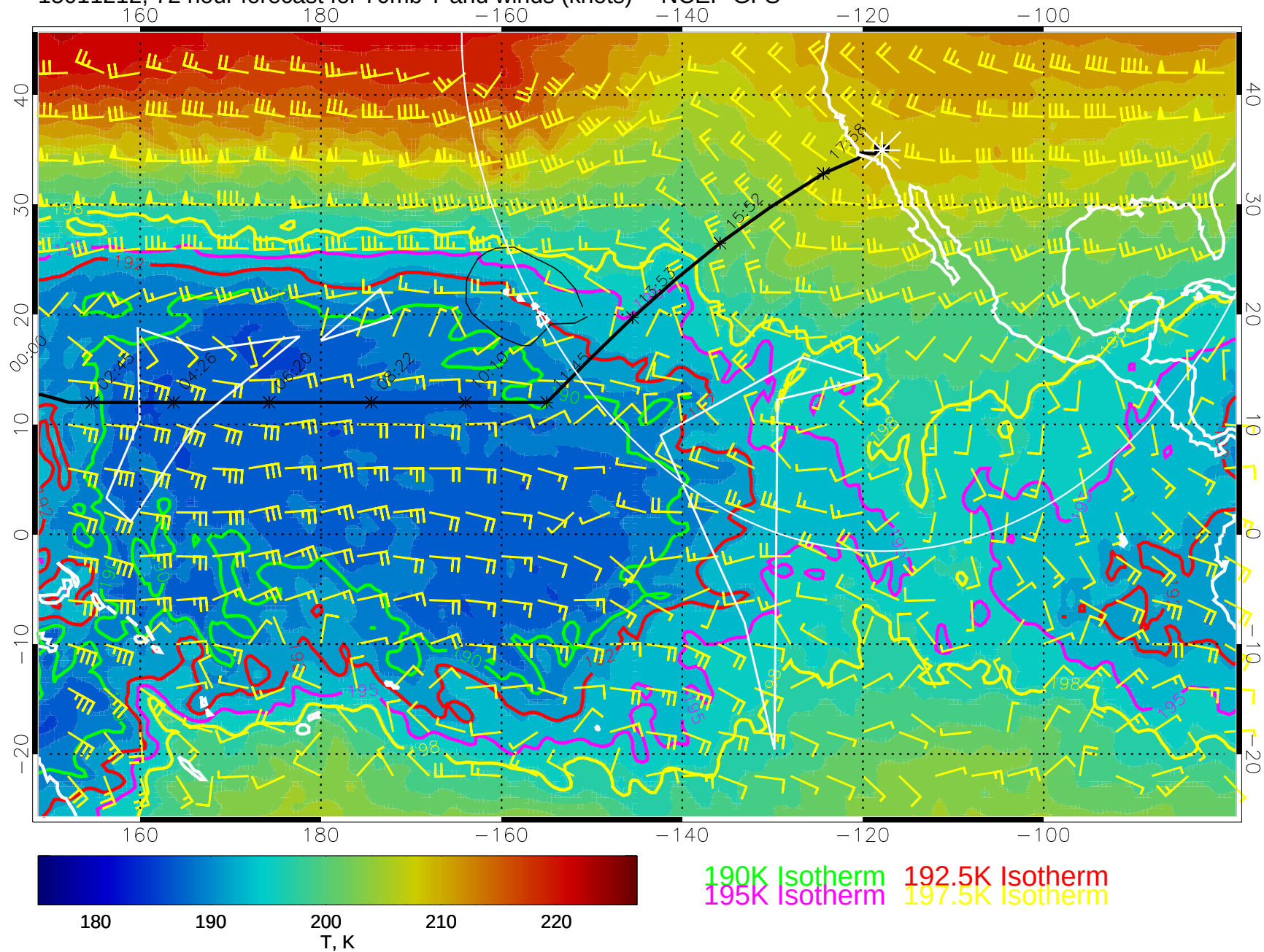
15011212, 72 hour forecast for 70mb T and winds (knots) -- NCEP GFS
