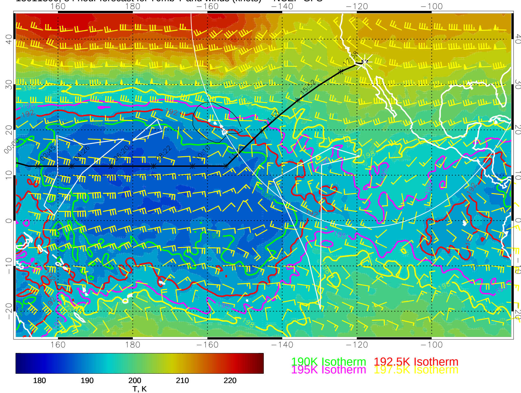
15011300, 84 hour forecast for 70mb T and winds (knots) -- NCEP GFS
