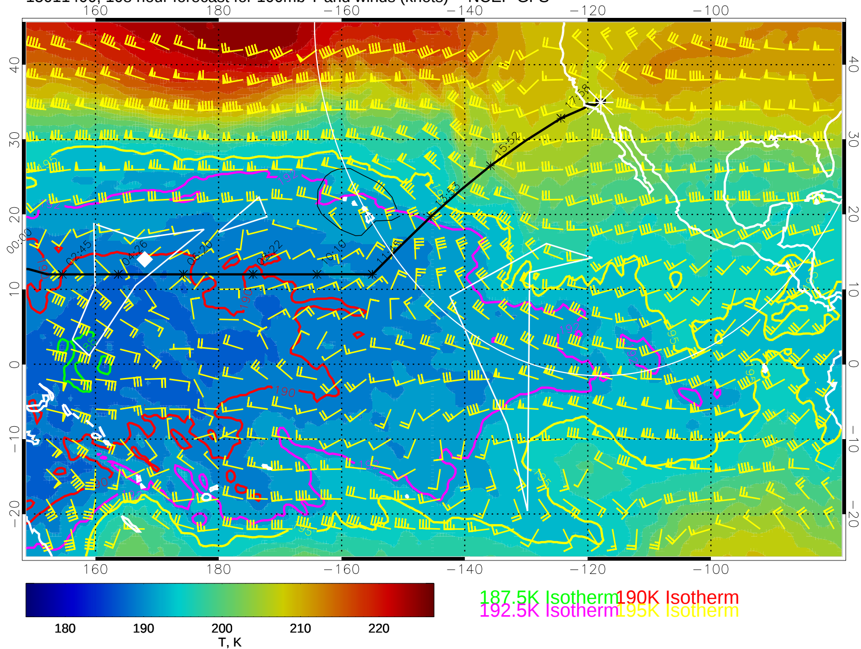
15011400, 108 hour forecast for 100mb T and winds (knots) -- NCEP GFS
