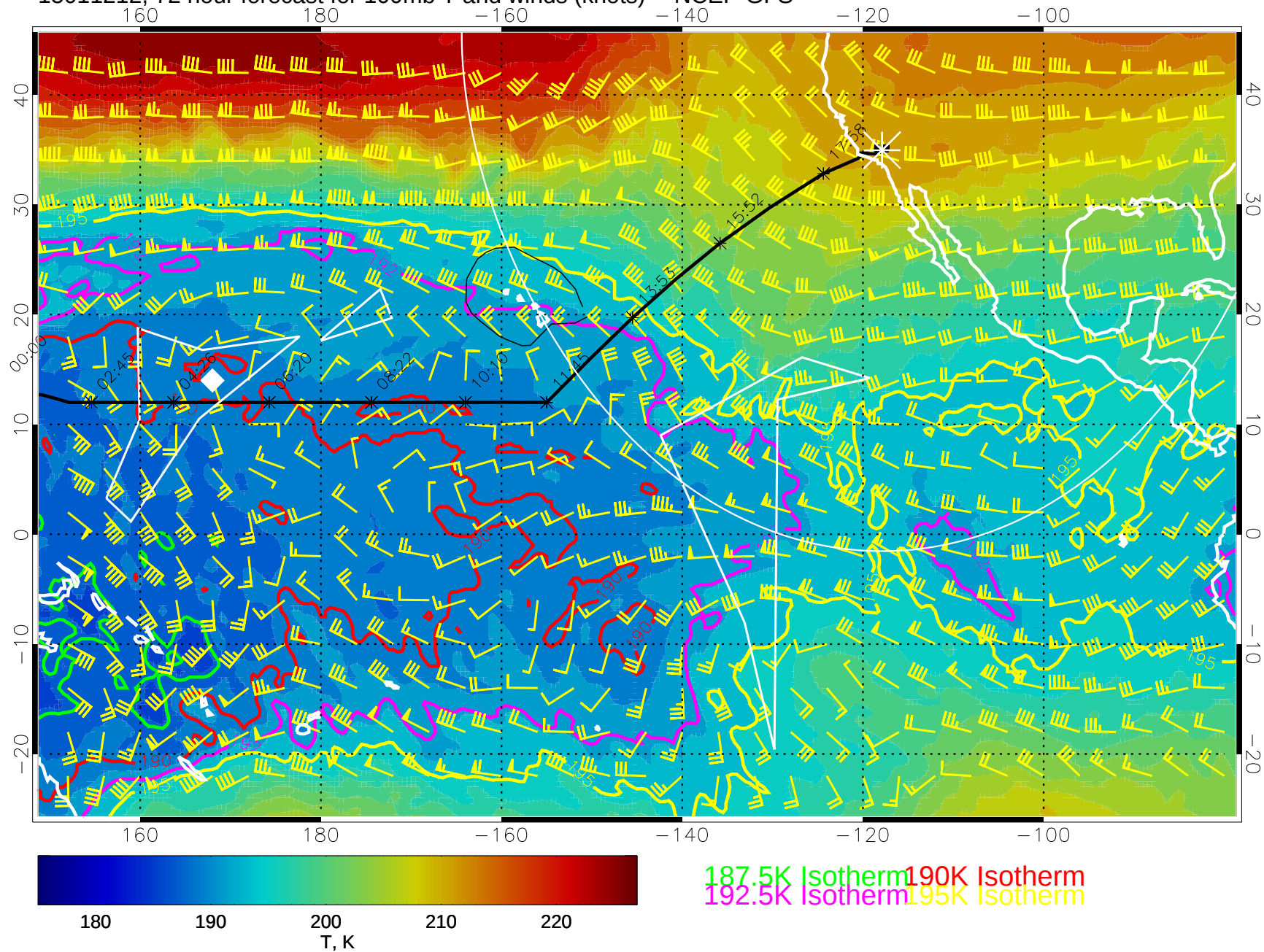
15011212, 72 hour forecast for 100mb T and winds (knots) -- NCEP GFS
