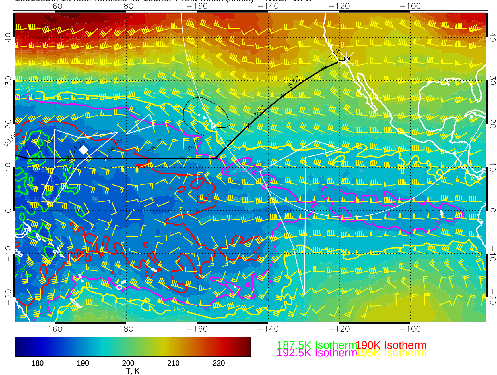
15011006, 18 hour forecast for 100mb T and winds (knots) -- NCEP GFS
