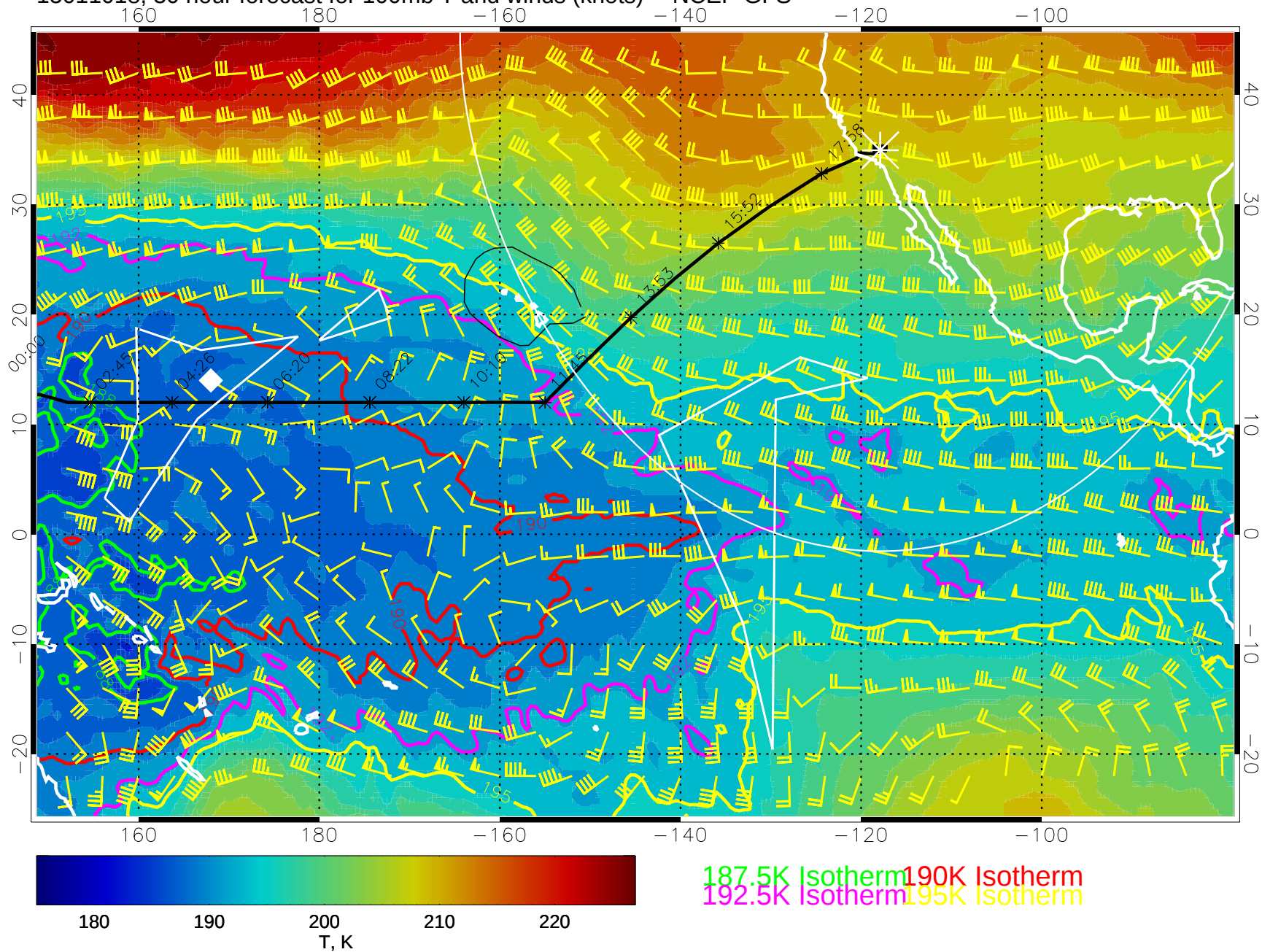
15011018, 30 hour forecast for 100mb T and winds (knots) -- NCEP GFS
