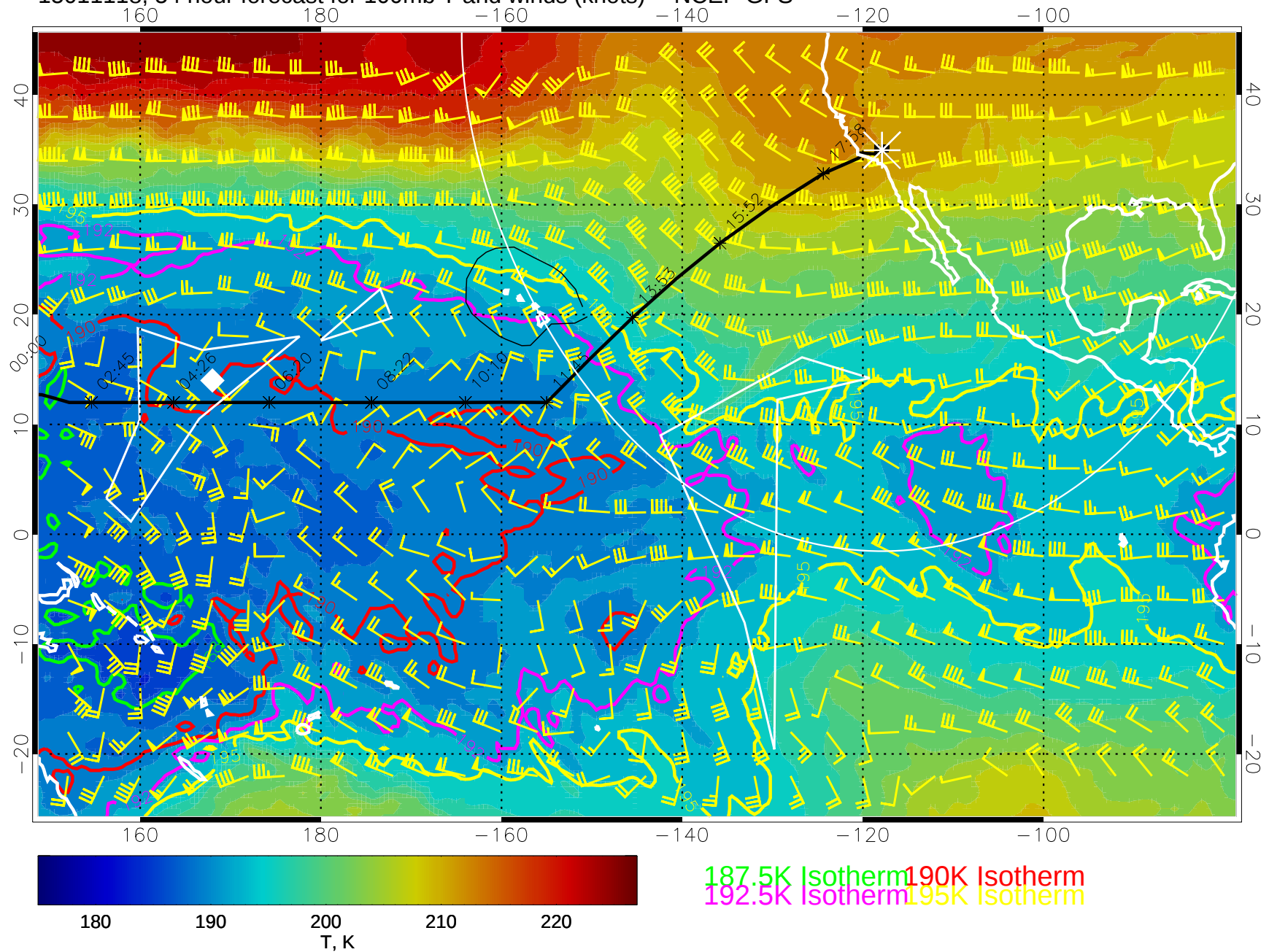
15011118, 54 hour forecast for 100mb T and winds (knots) -- NCEP GFS
