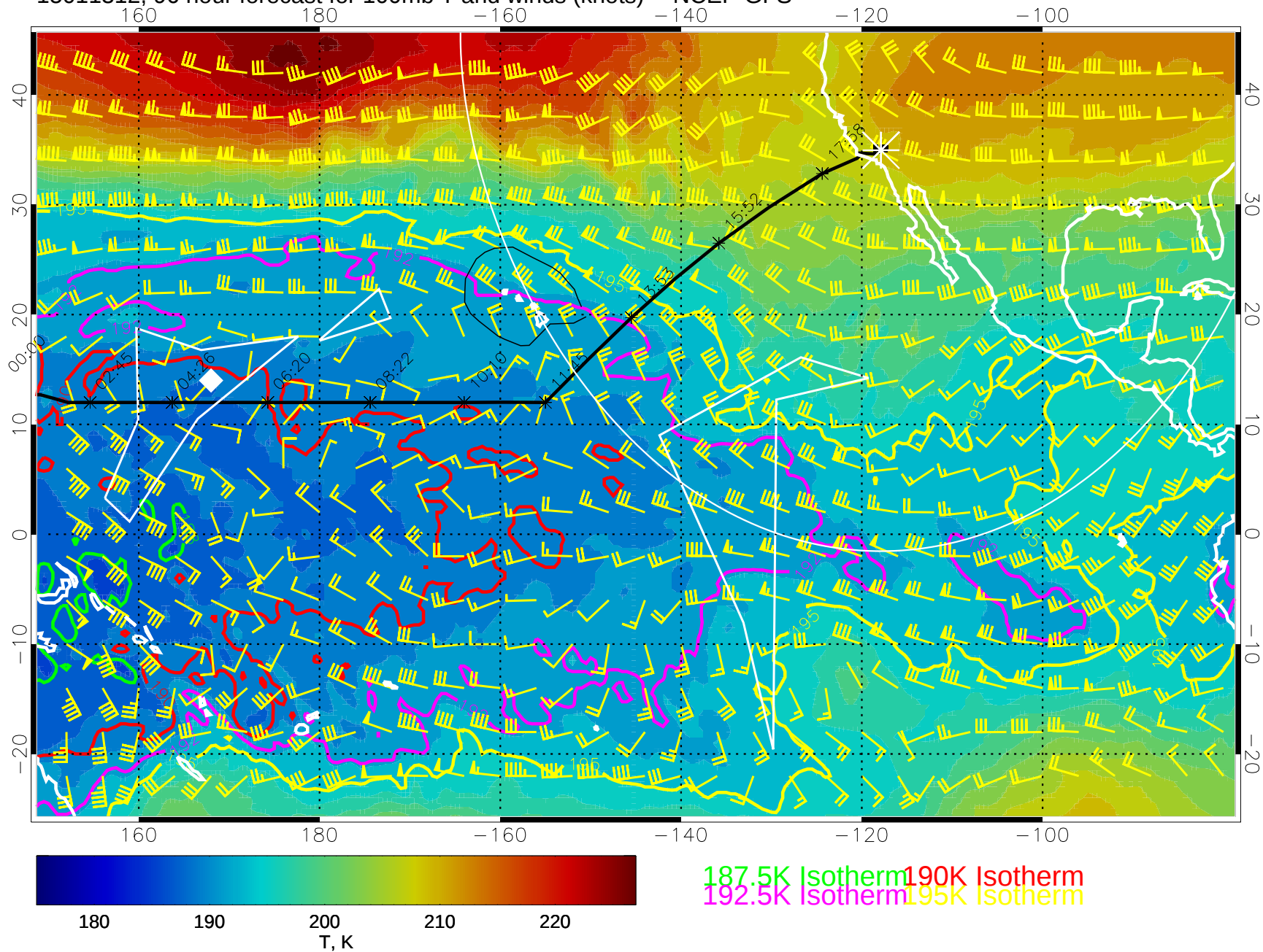
15011312, 96 hour forecast for 100mb T and winds (knots) -- NCEP GFS
