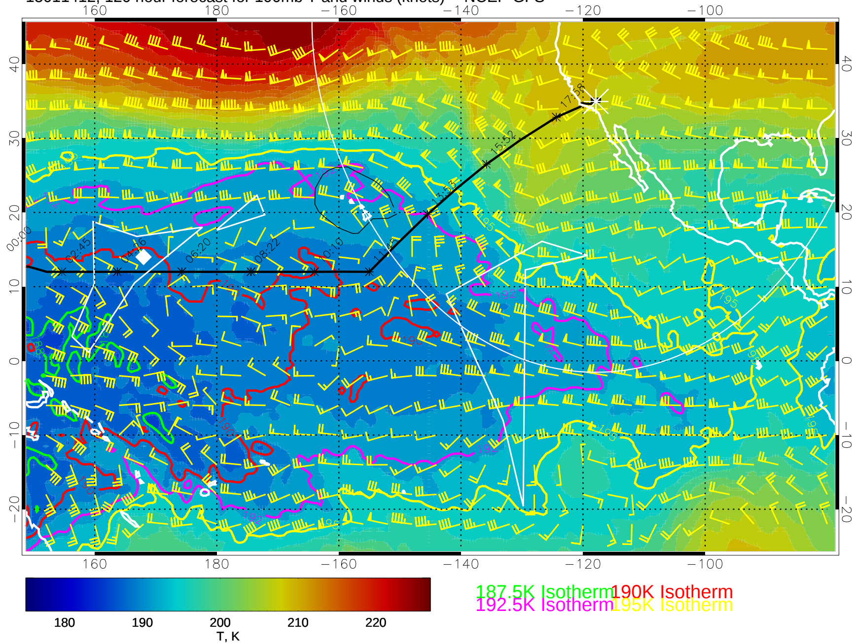
15011412, 120 hour forecast for 100mb T and winds (knots) -- NCEP GFS
