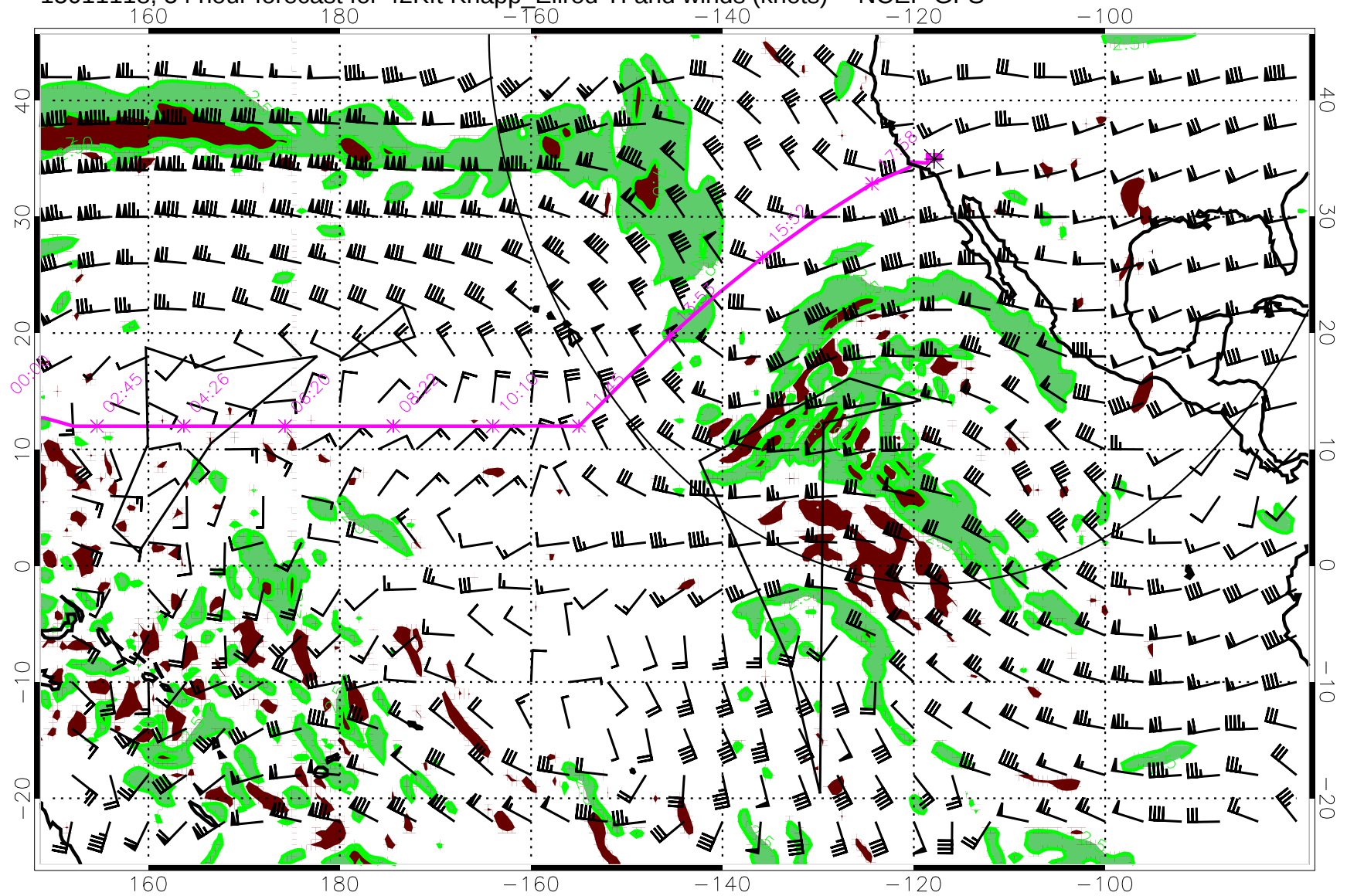
15011118, 54 hour forecast for 42Kft Knapp_Ellrod TI and winds (knots) -- NCEP GFS
