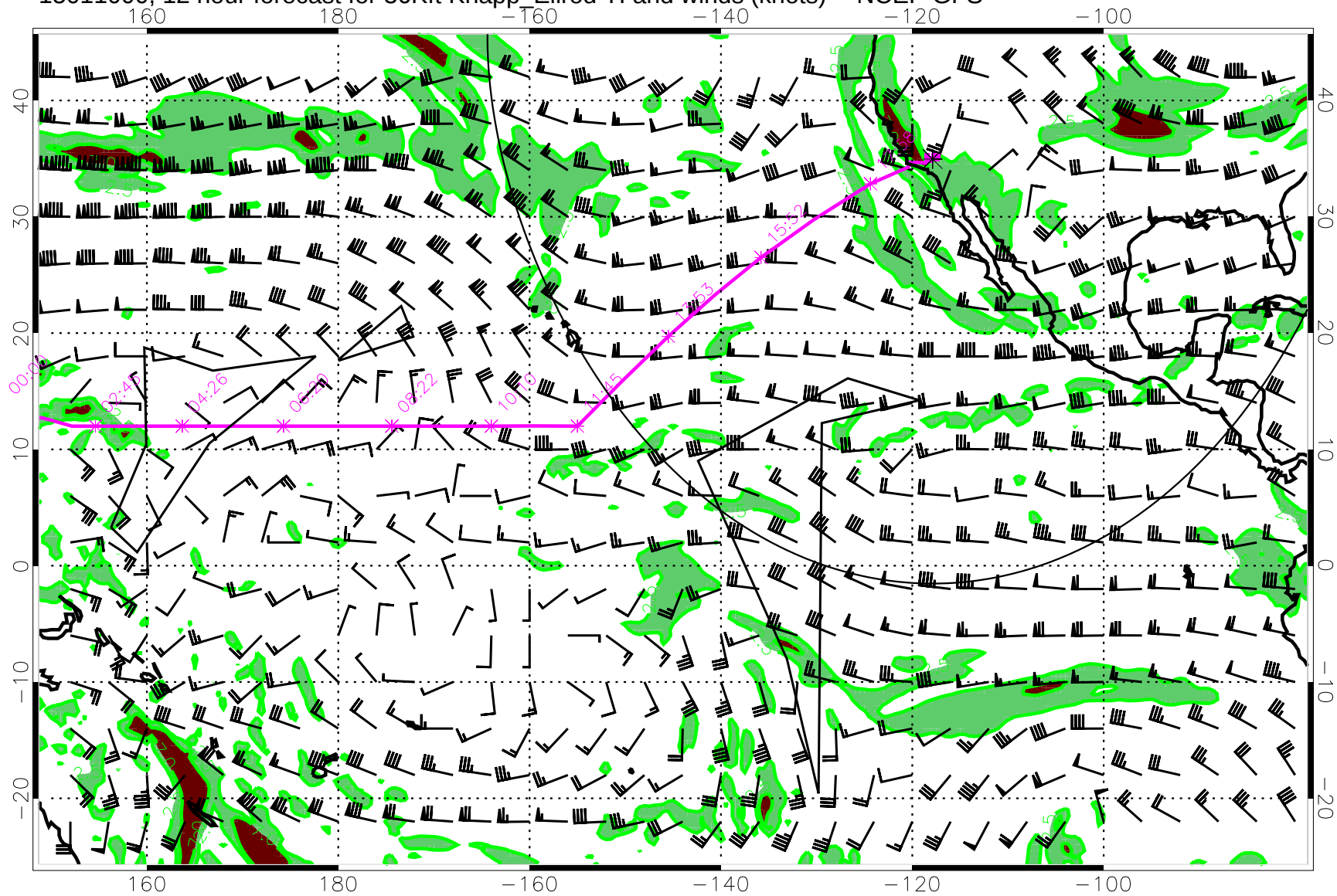
15011000, 12 hour forecast for 36Kft Knapp_Ellrod TI and winds (knots) -- NCEP GFS
