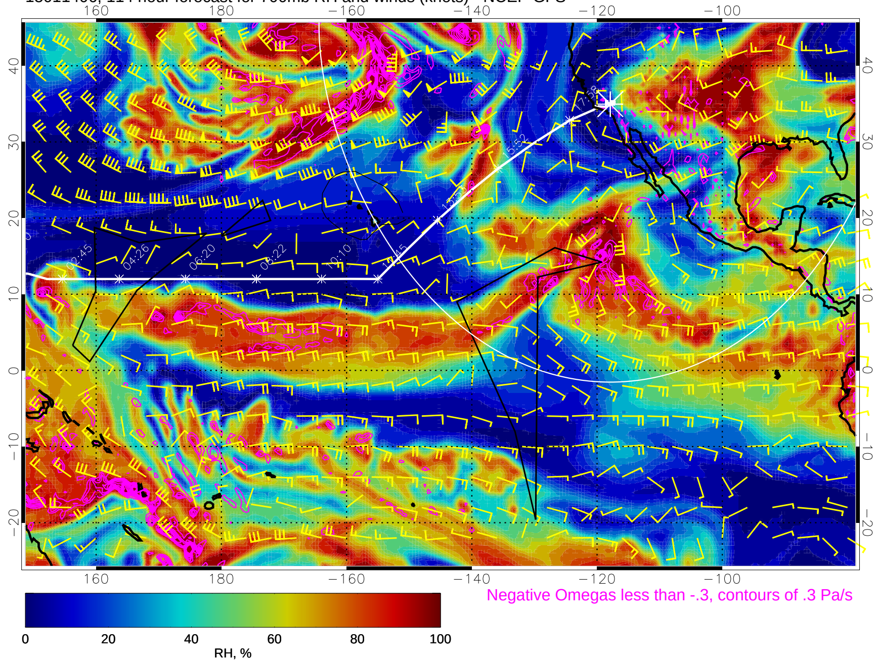
15011406, 114 hour forecast for 700mb RH and winds (knots) - NCEP GFS
