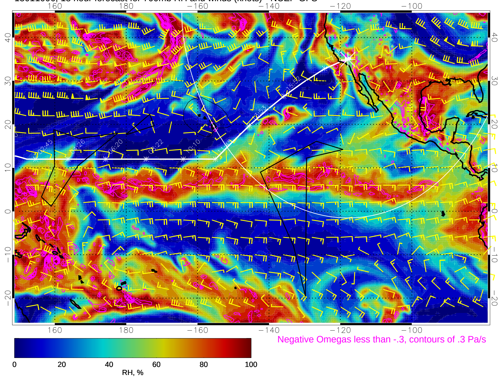
15011006, 18 hour forecast for 700mb RH and winds (knots) - NCEP GFS
