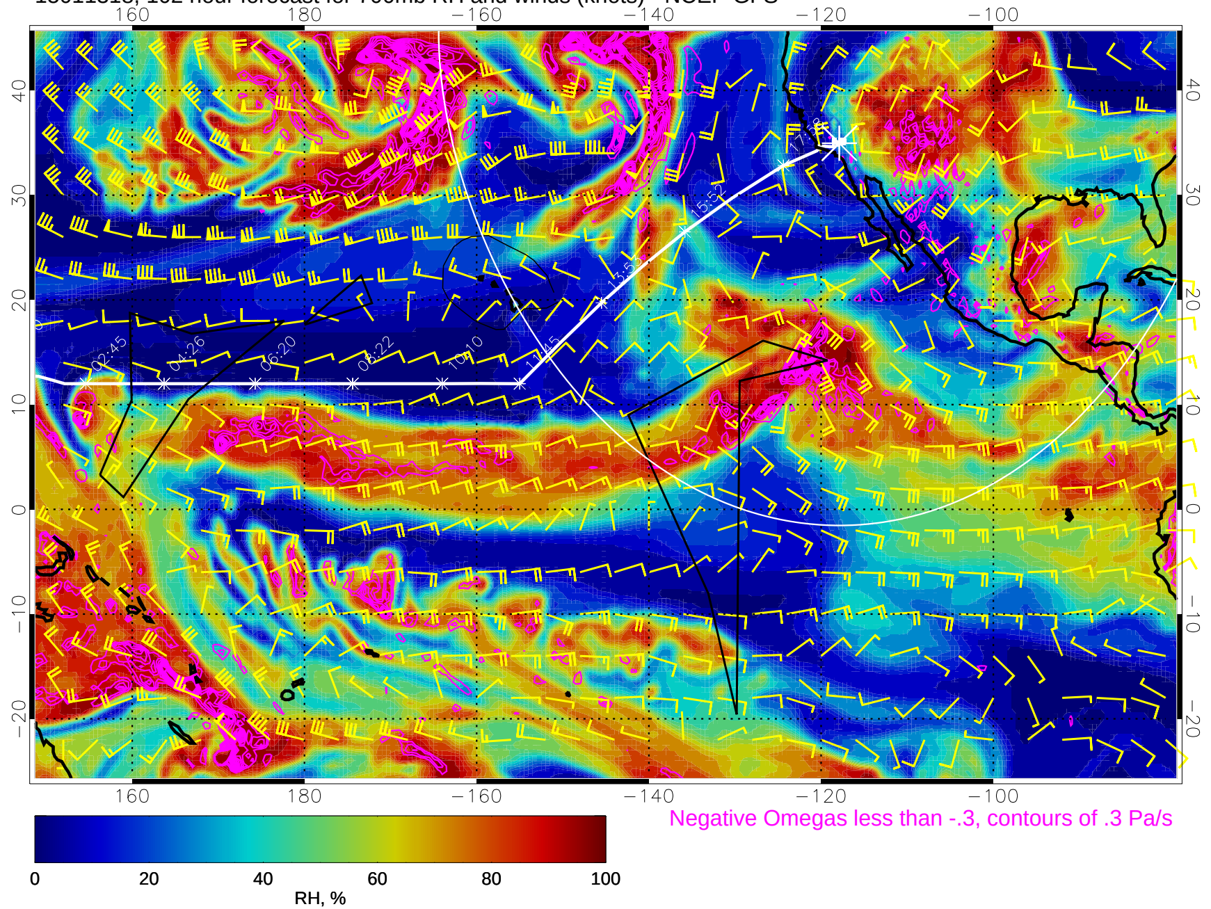
15011318, 102 hour forecast for 700mb RH and winds (knots) - NCEP GFS
