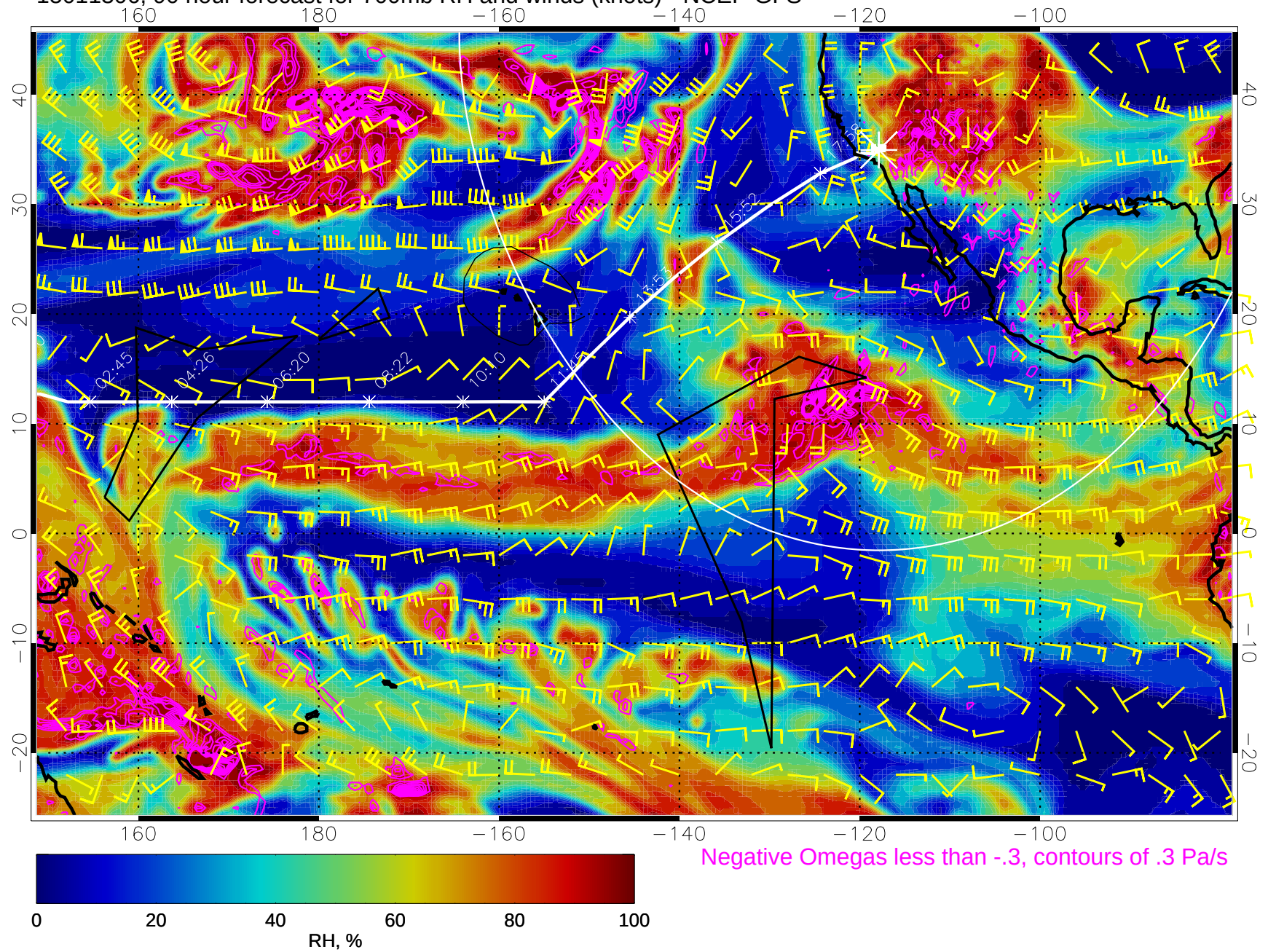
15011306, 90 hour forecast for 700mb RH and winds (knots) - NCEP GFS
