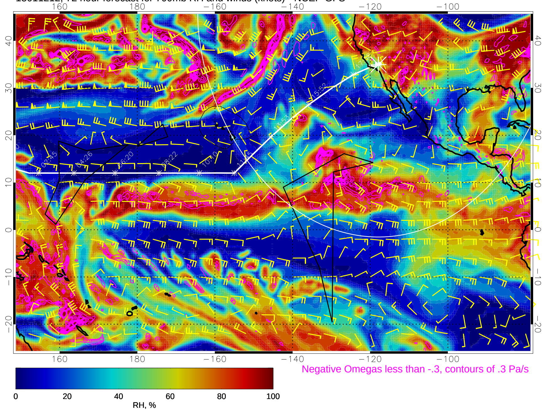
15011212, 72 hour forecast for 700mb RH and winds (knots) - NCEP GFS
