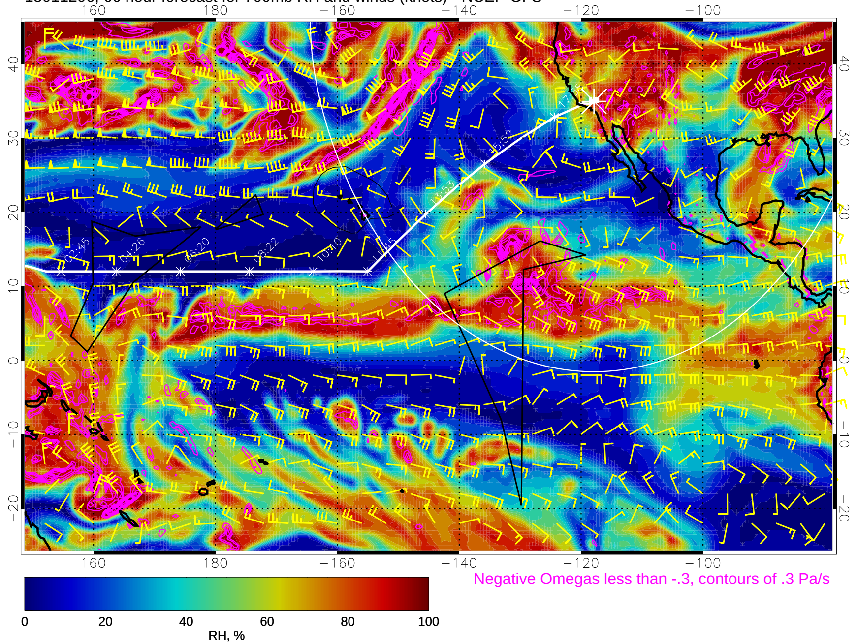
15011206, 66 hour forecast for 700mb RH and winds (knots) - NCEP GFS
