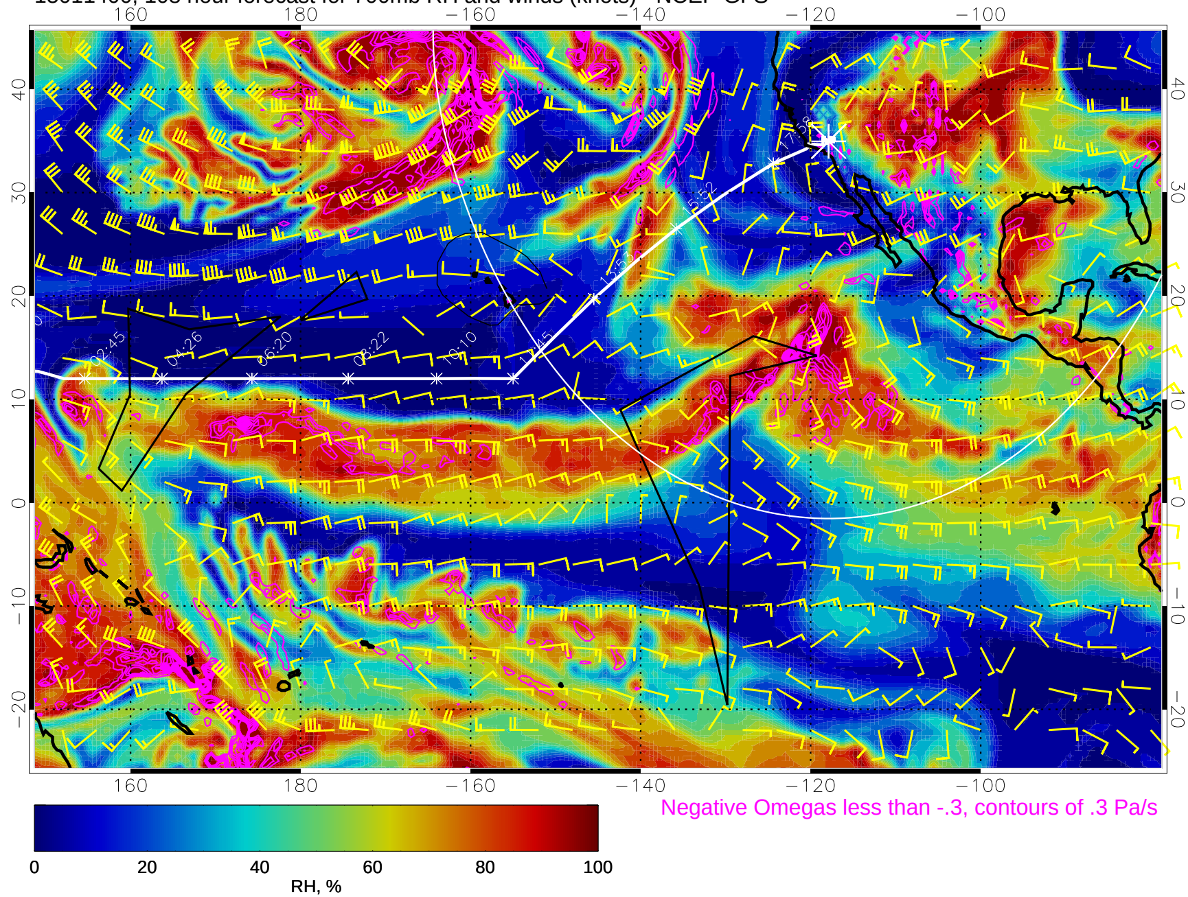
15011400, 108 hour forecast for 700mb RH and winds (knots) - NCEP GFS
