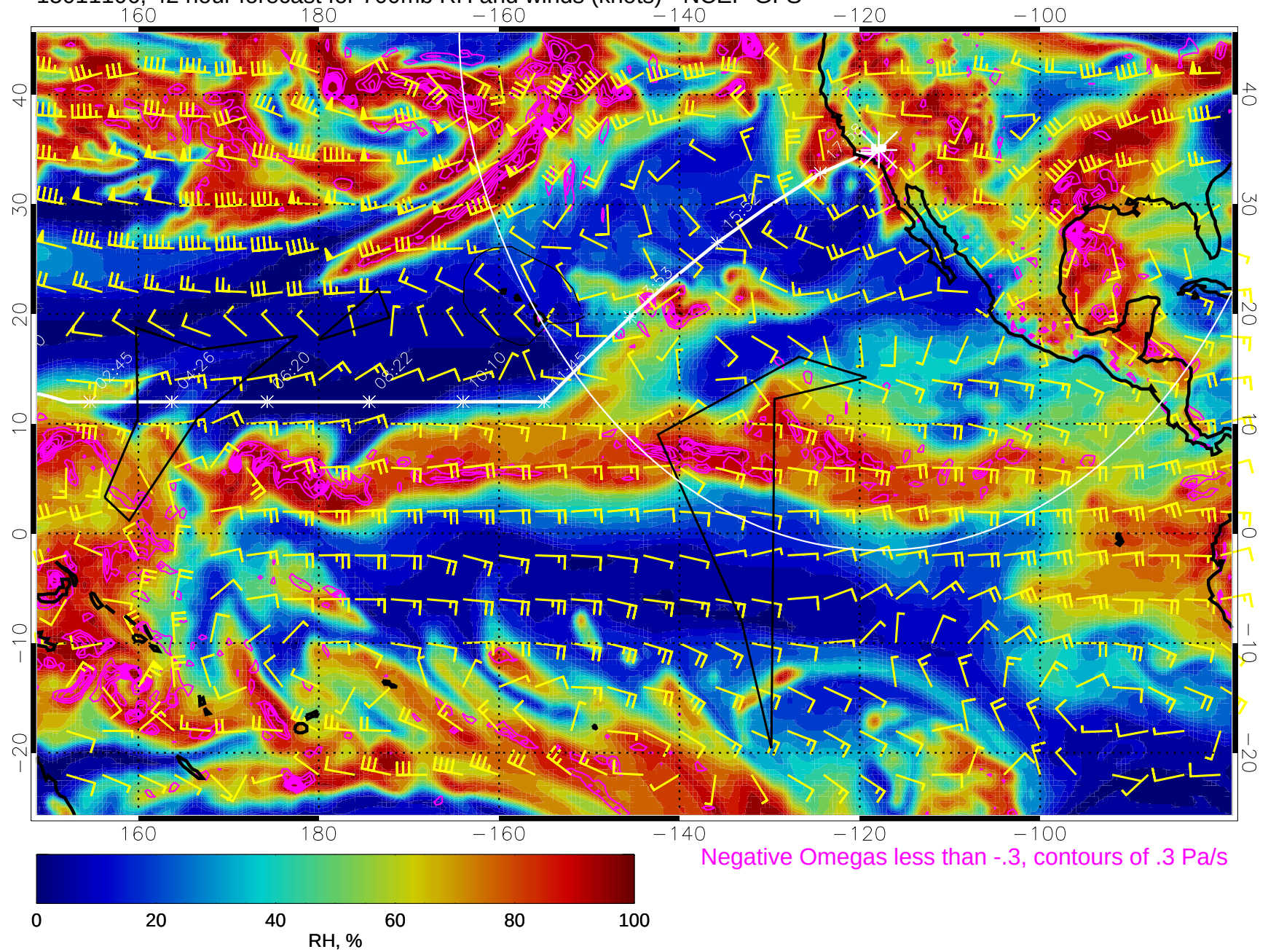
15011106, 42 hour forecast for 700mb RH and winds (knots) - NCEP GFS
