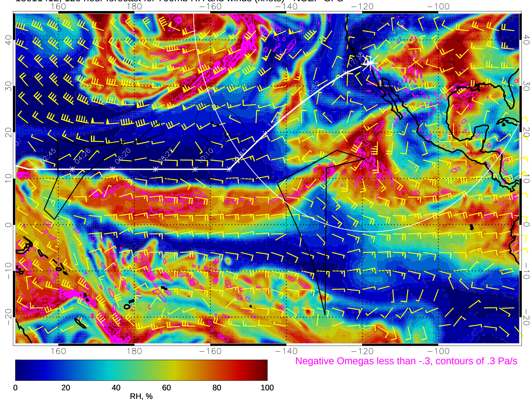
15011412, 120 hour forecast for 700mb RH and winds (knots) - NCEP GFS
