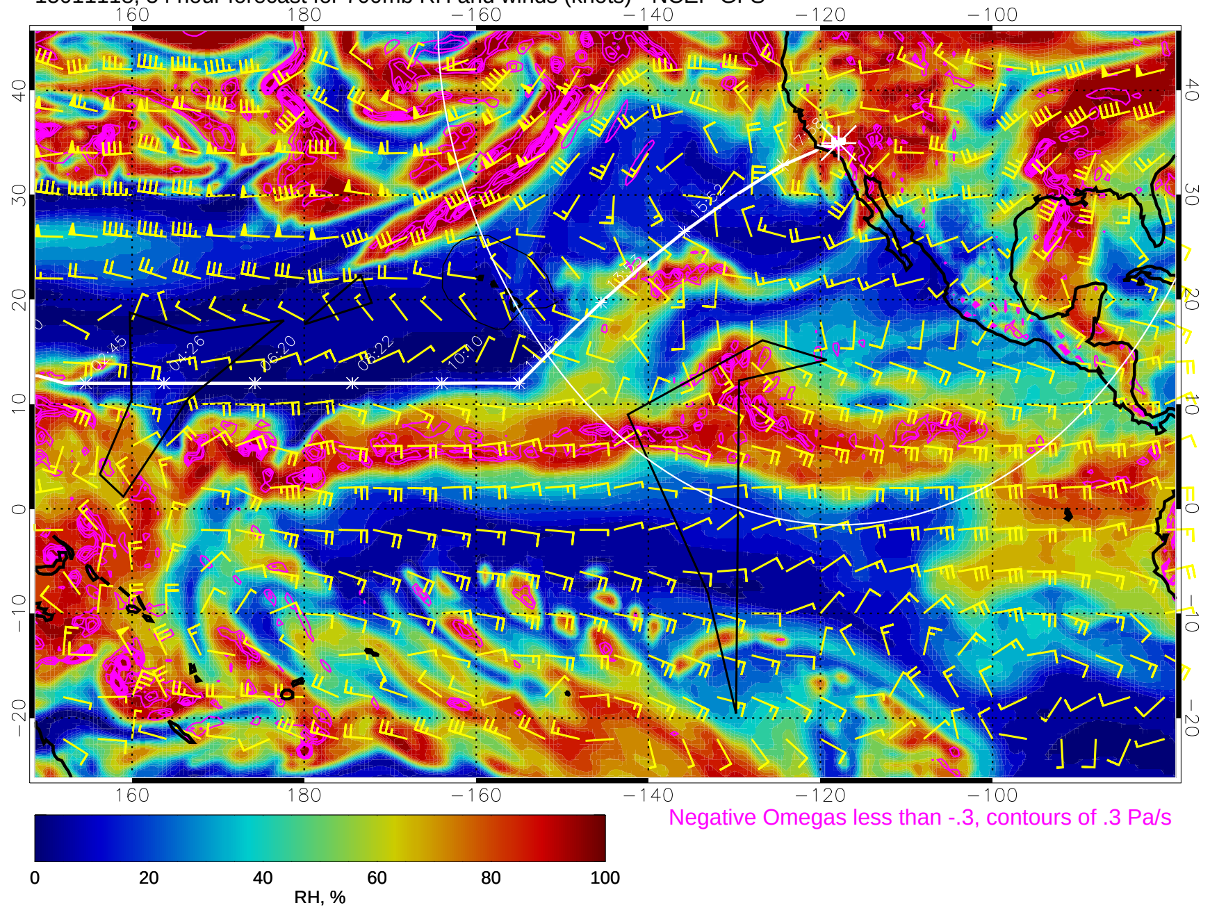
15011118, 54 hour forecast for 700mb RH and winds (knots) - NCEP GFS
