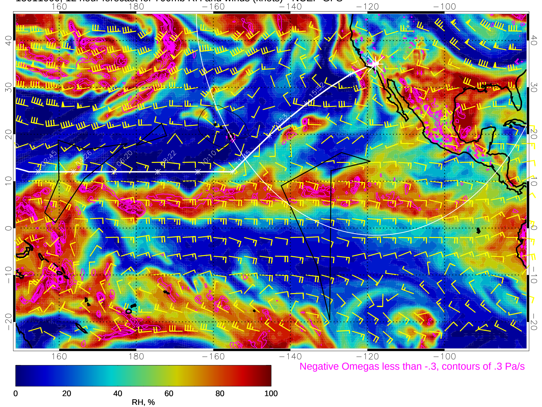
15011000, 12 hour forecast for 700mb RH and winds (knots) - NCEP GFS
