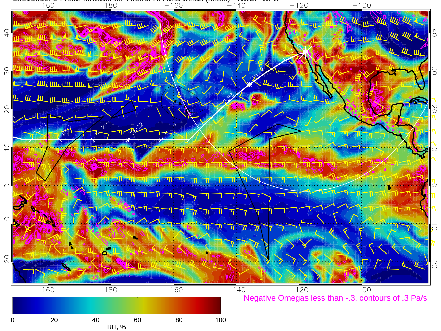
15011012, 24 hour forecast for 700mb RH and winds (knots) - NCEP GFS
