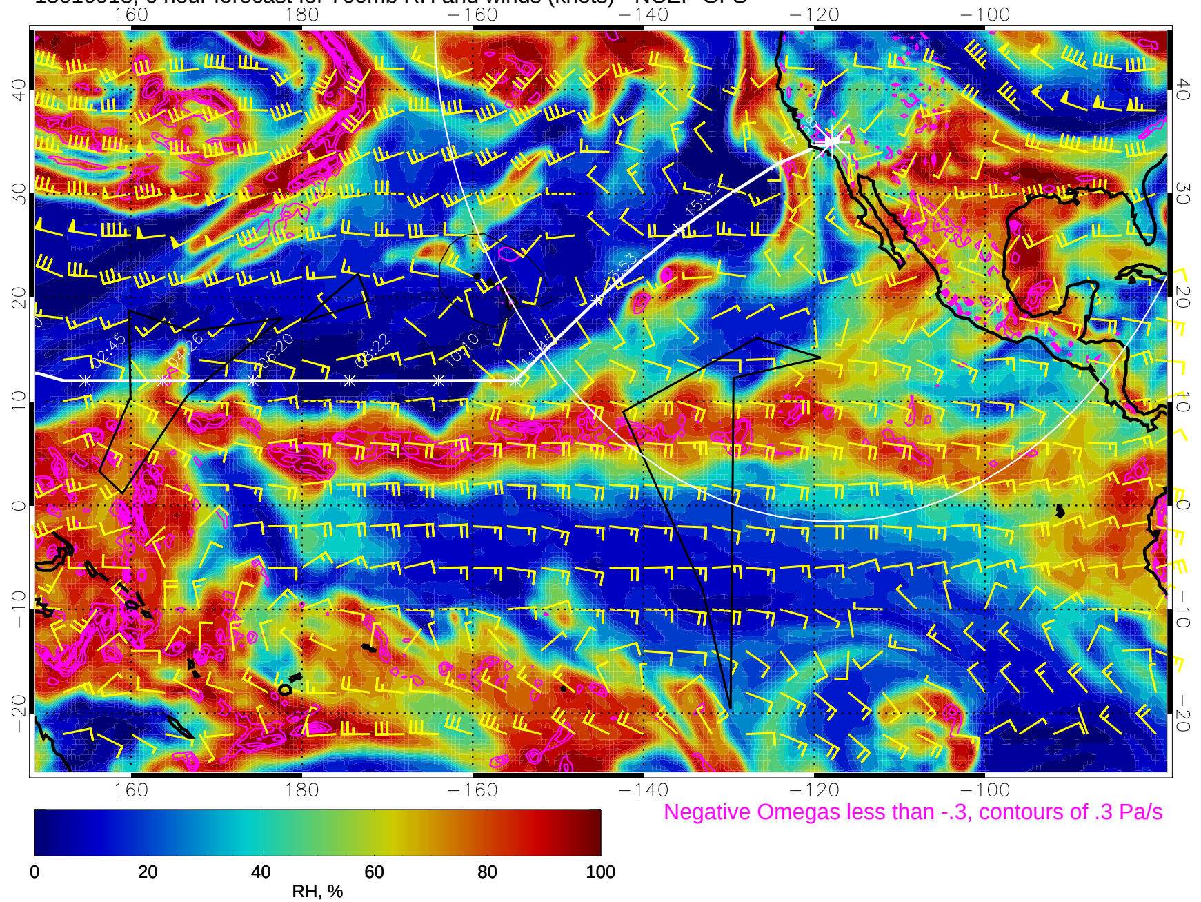
15010918, 6 hour forecast for 700mb RH and winds (knots) - NCEP GFS
