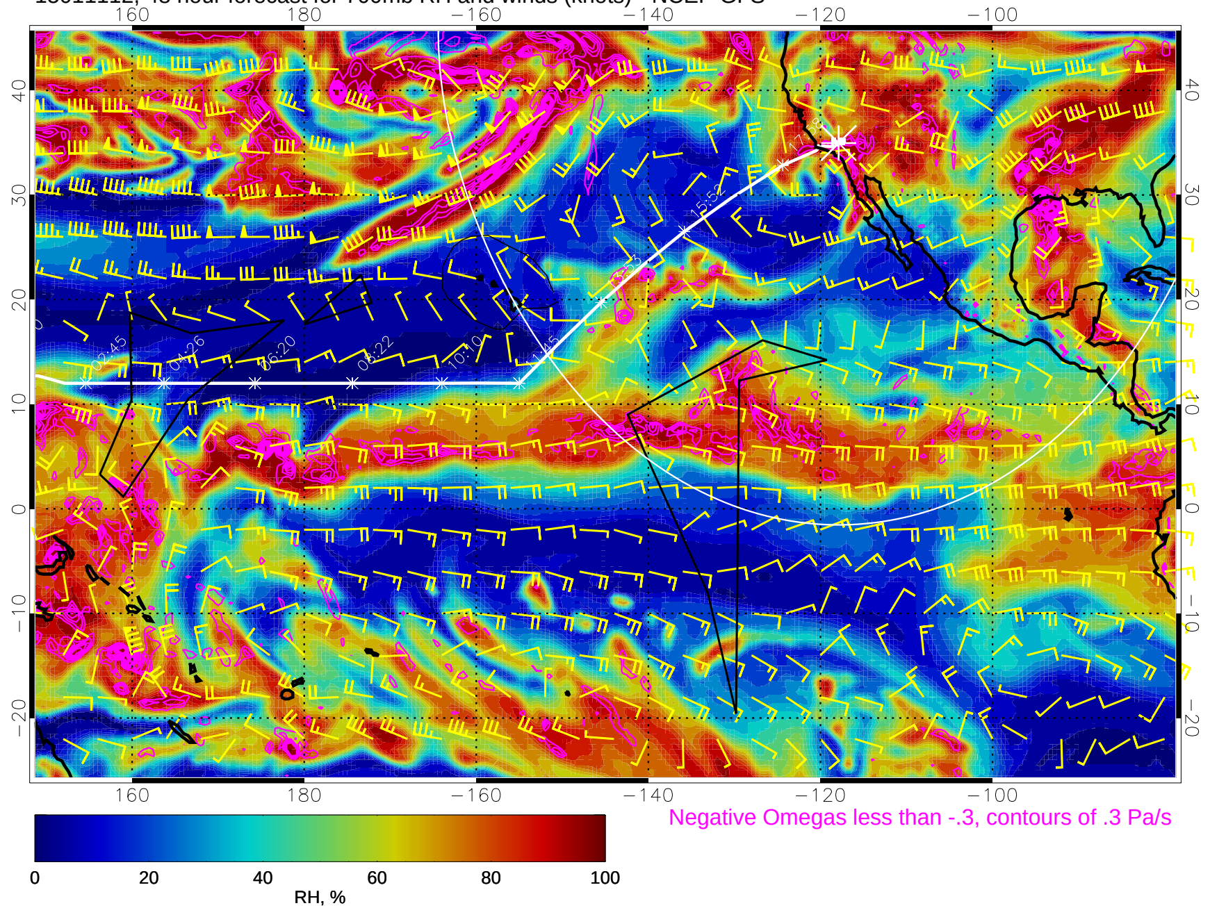
15011112, 48 hour forecast for 700mb RH and winds (knots) - NCEP GFS
