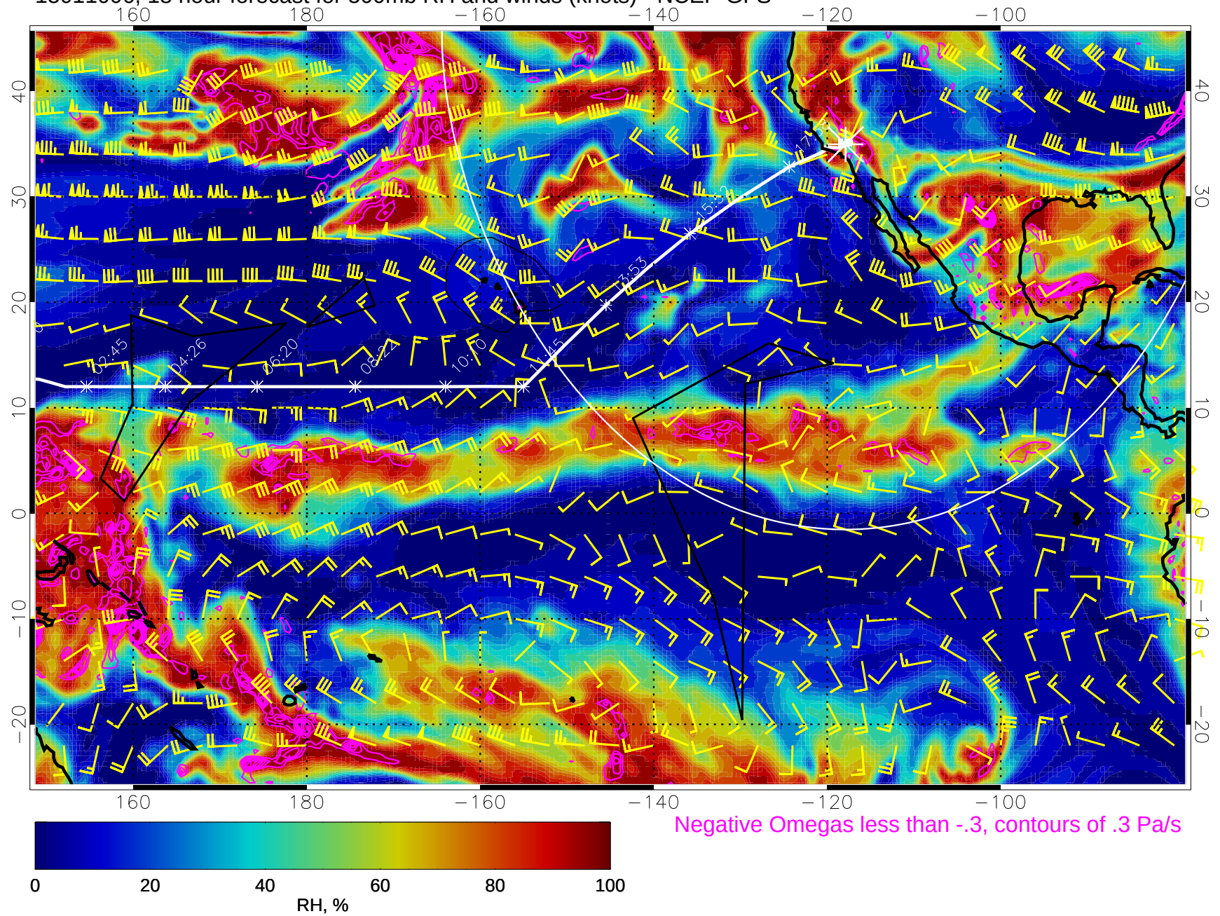
15011006, 18 hour forecast for 500mb RH and winds (knots) - NCEP GFS
