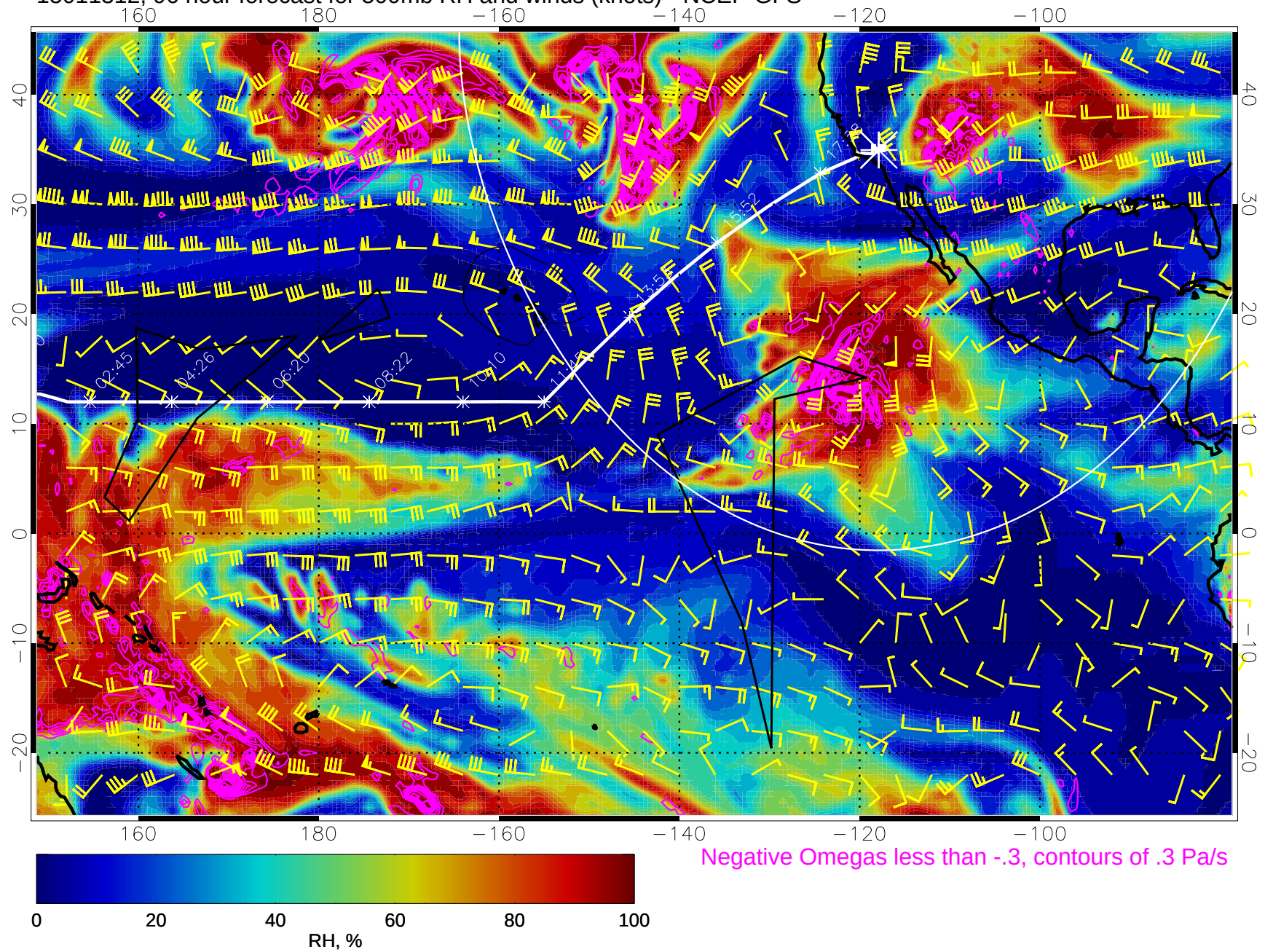
15011312, 96 hour forecast for 500mb RH and winds (knots) - NCEP GFS
