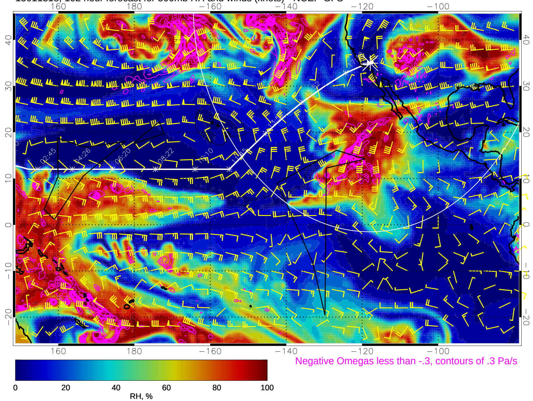
15011318, 102 hour forecast for 500mb RH and winds (knots) - NCEP GFS
