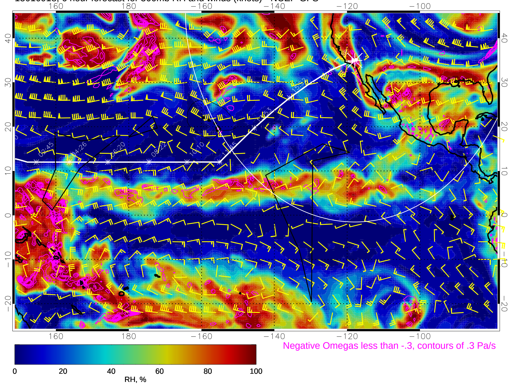
15010918, 6 hour forecast for 500mb RH and winds (knots) - NCEP GFS
