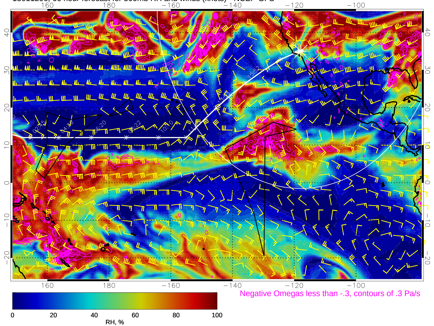
15011206, 66 hour forecast for 500mb RH and winds (knots) - NCEP GFS
