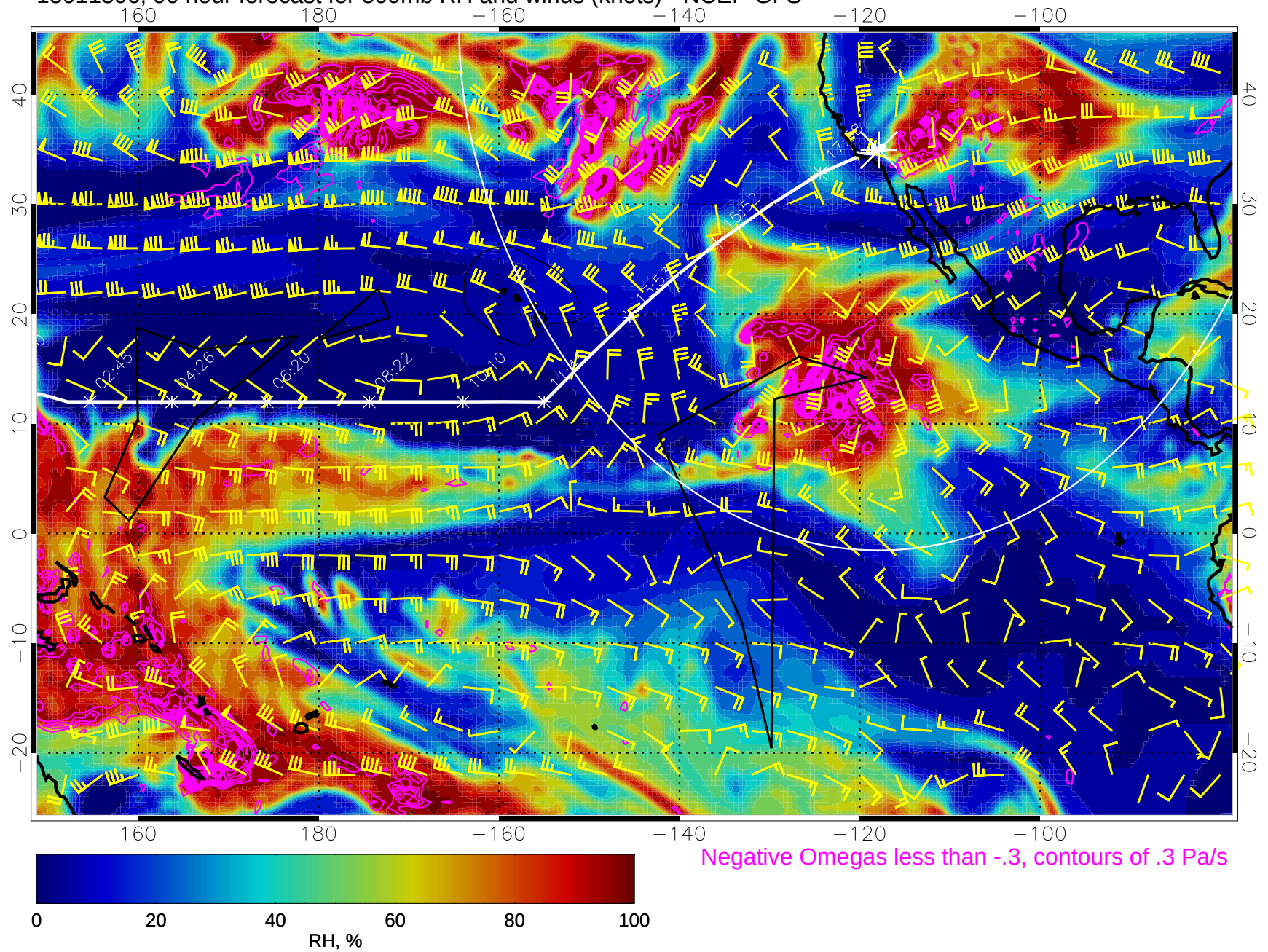
15011306, 90 hour forecast for 500mb RH and winds (knots) - NCEP GFS
