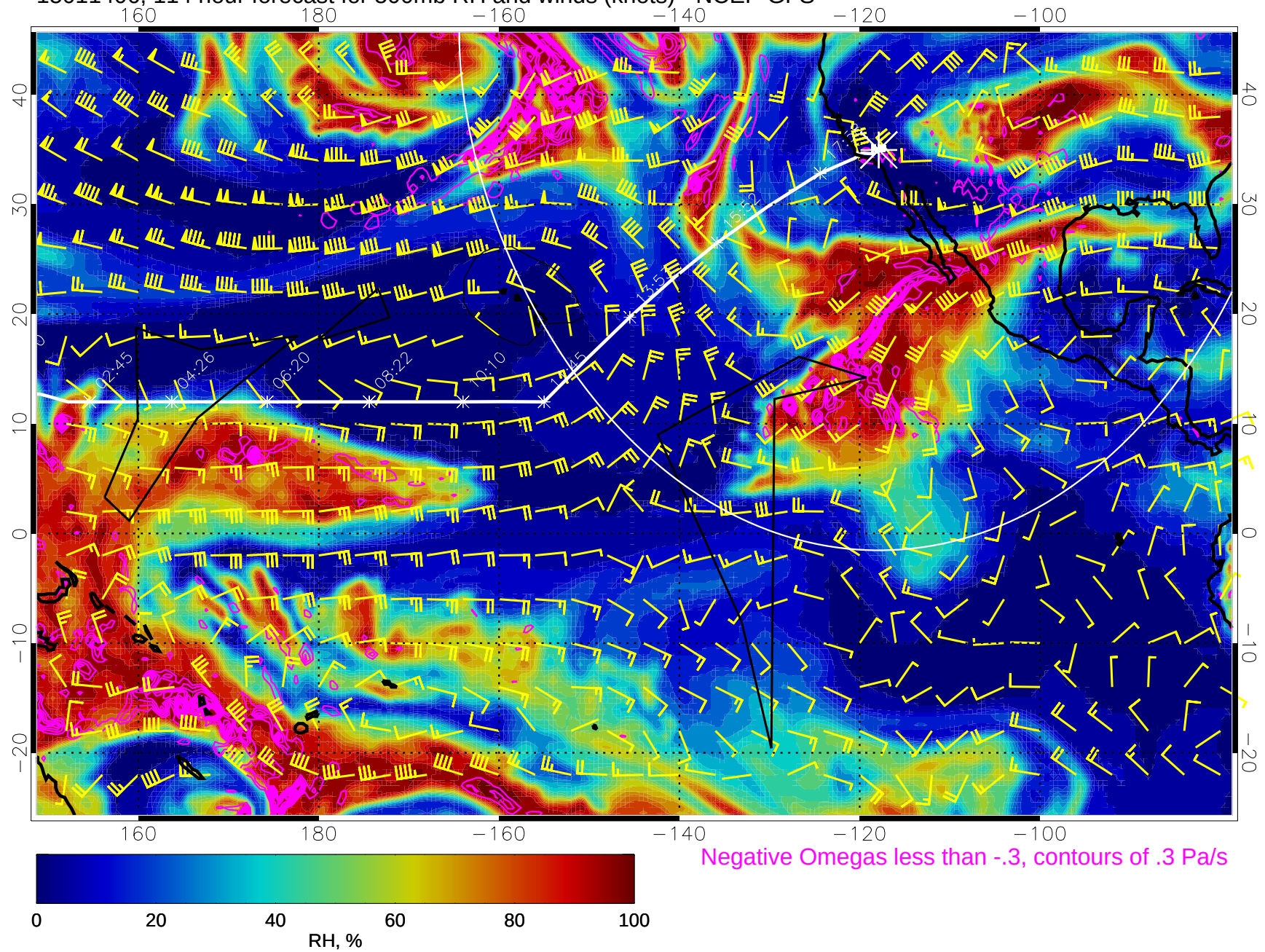
15011406, 114 hour forecast for 500mb RH and winds (knots) - NCEP GFS
