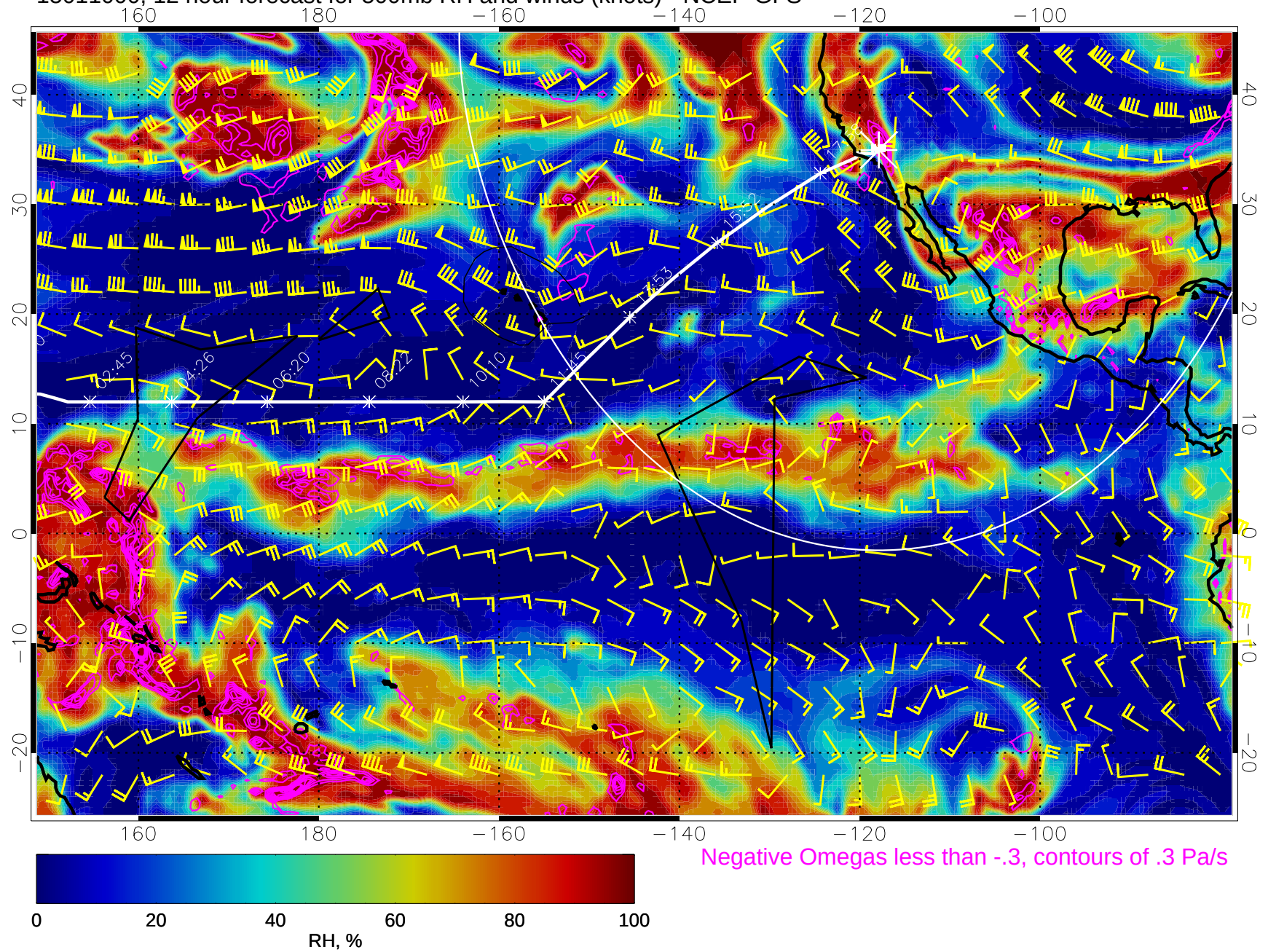
15011000, 12 hour forecast for 500mb RH and winds (knots) - NCEP GFS
