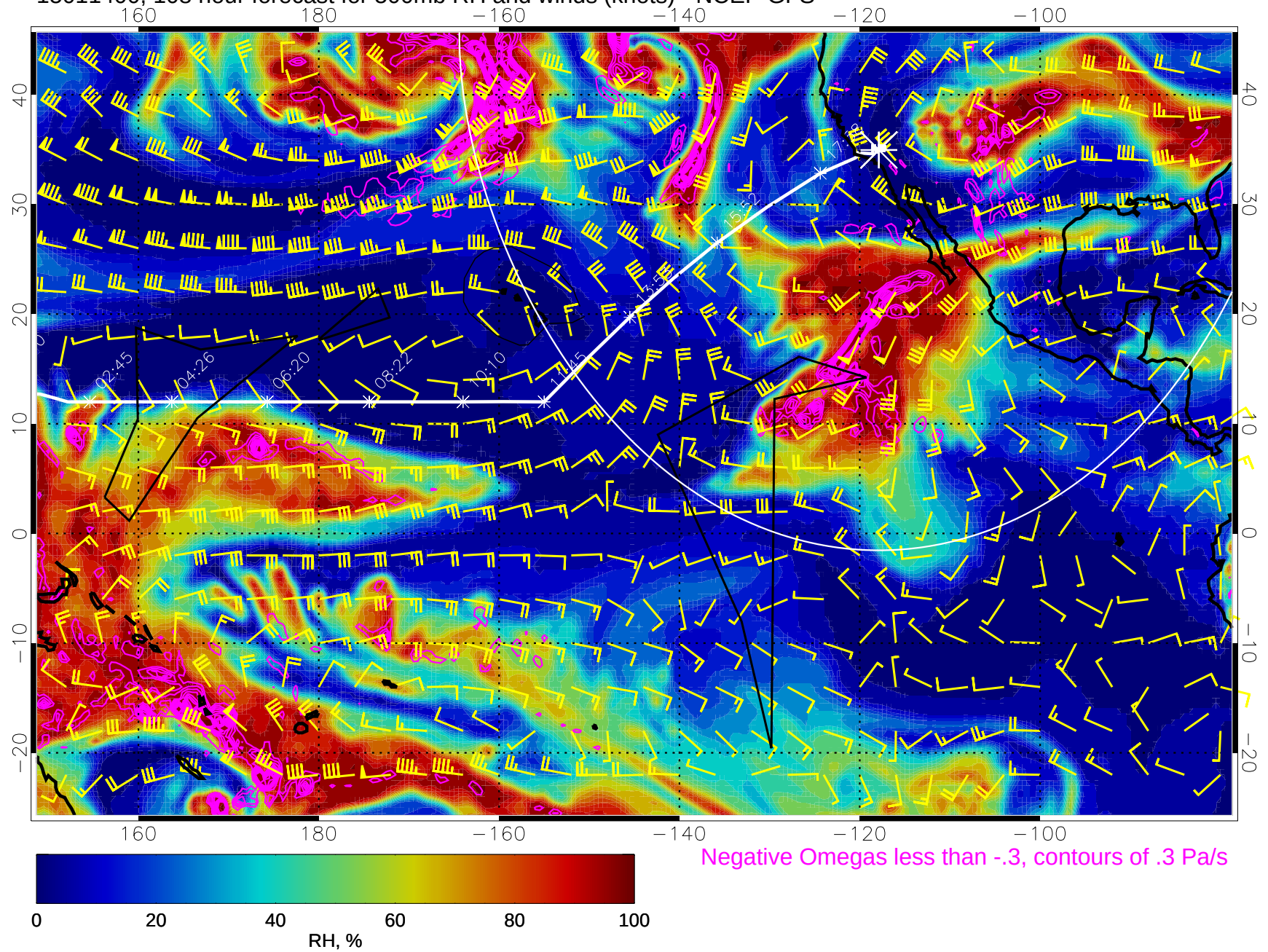
15011400, 108 hour forecast for 500mb RH and winds (knots) - NCEP GFS
