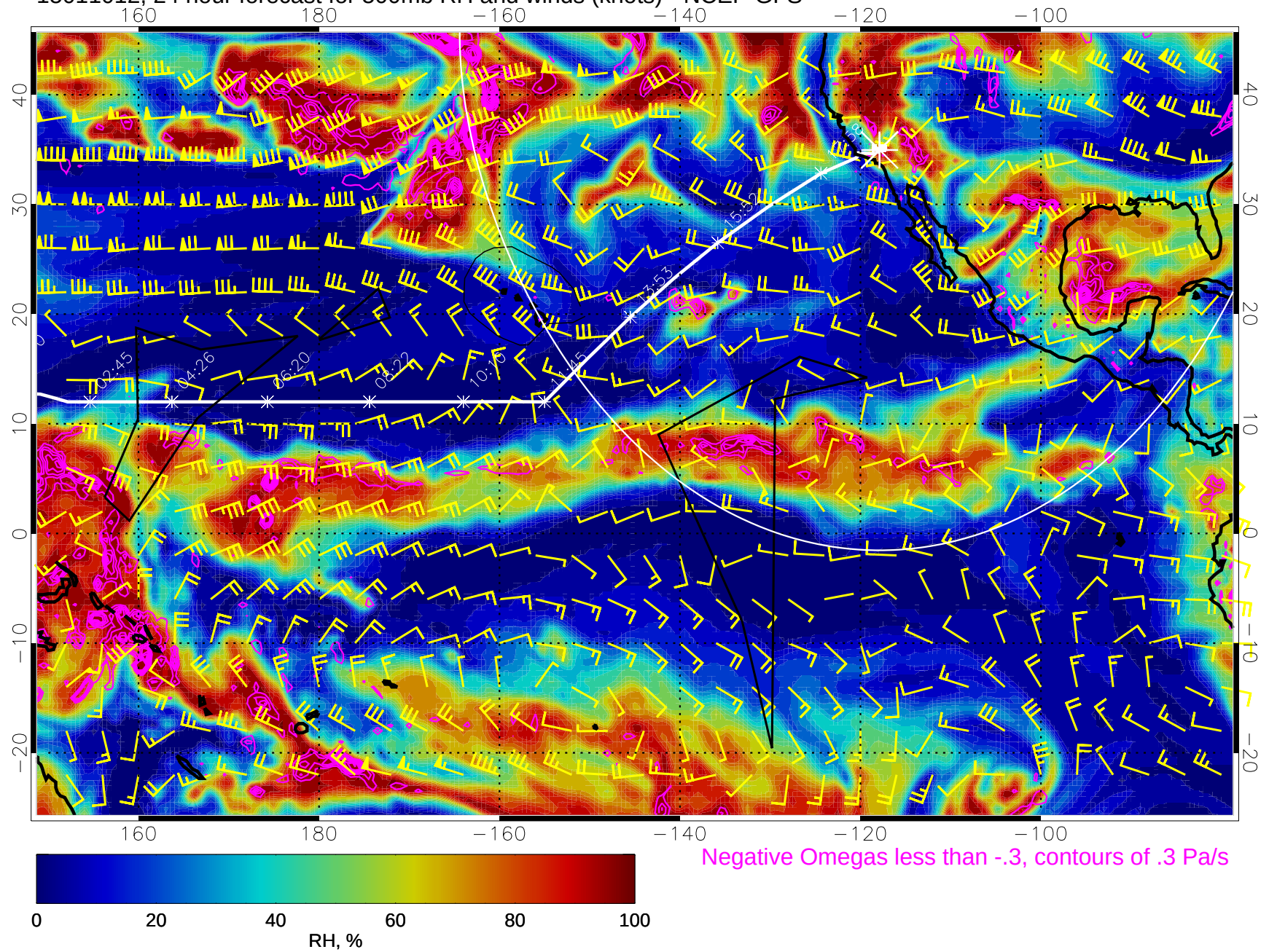
15011012, 24 hour forecast for 500mb RH and winds (knots) - NCEP GFS
