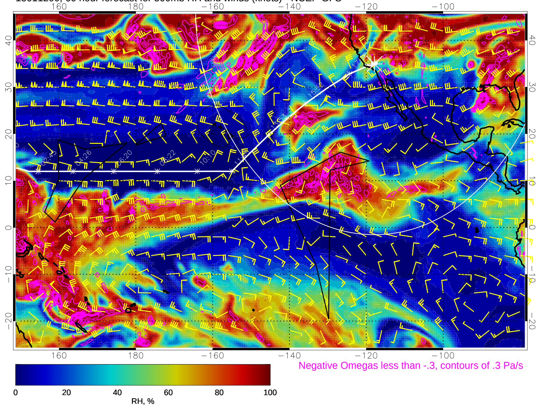
15011200, 60 hour forecast for 500mb RH and winds (knots) - NCEP GFS
