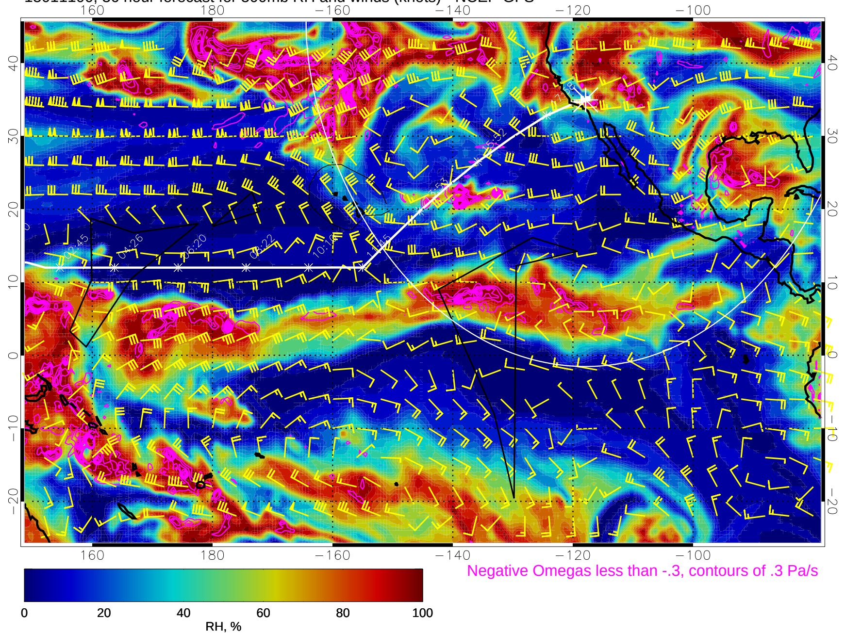
15011100, 36 hour forecast for 500mb RH and winds (knots) - NCEP GFS
