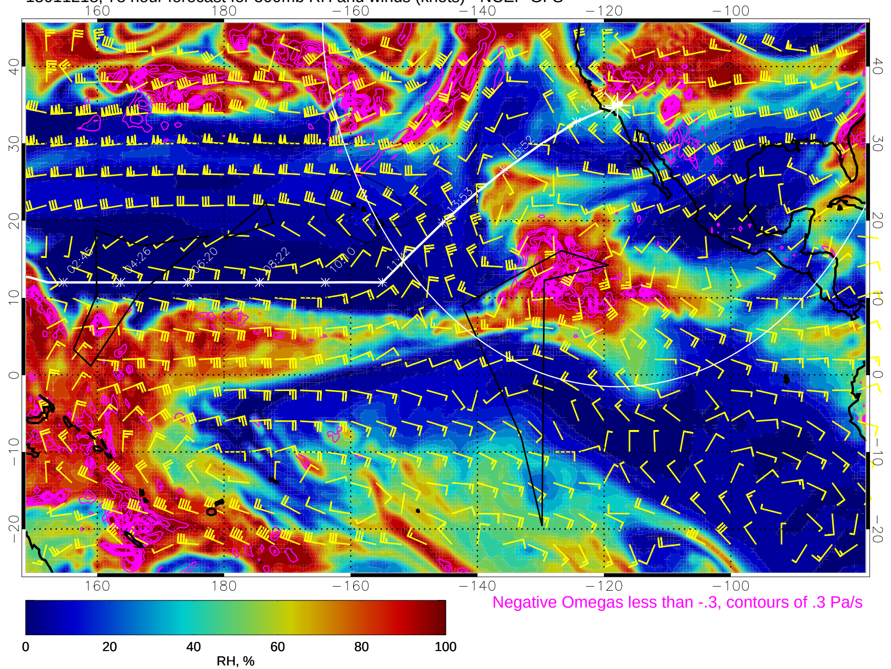
15011218, 78 hour forecast for 500mb RH and winds (knots) - NCEP GFS
