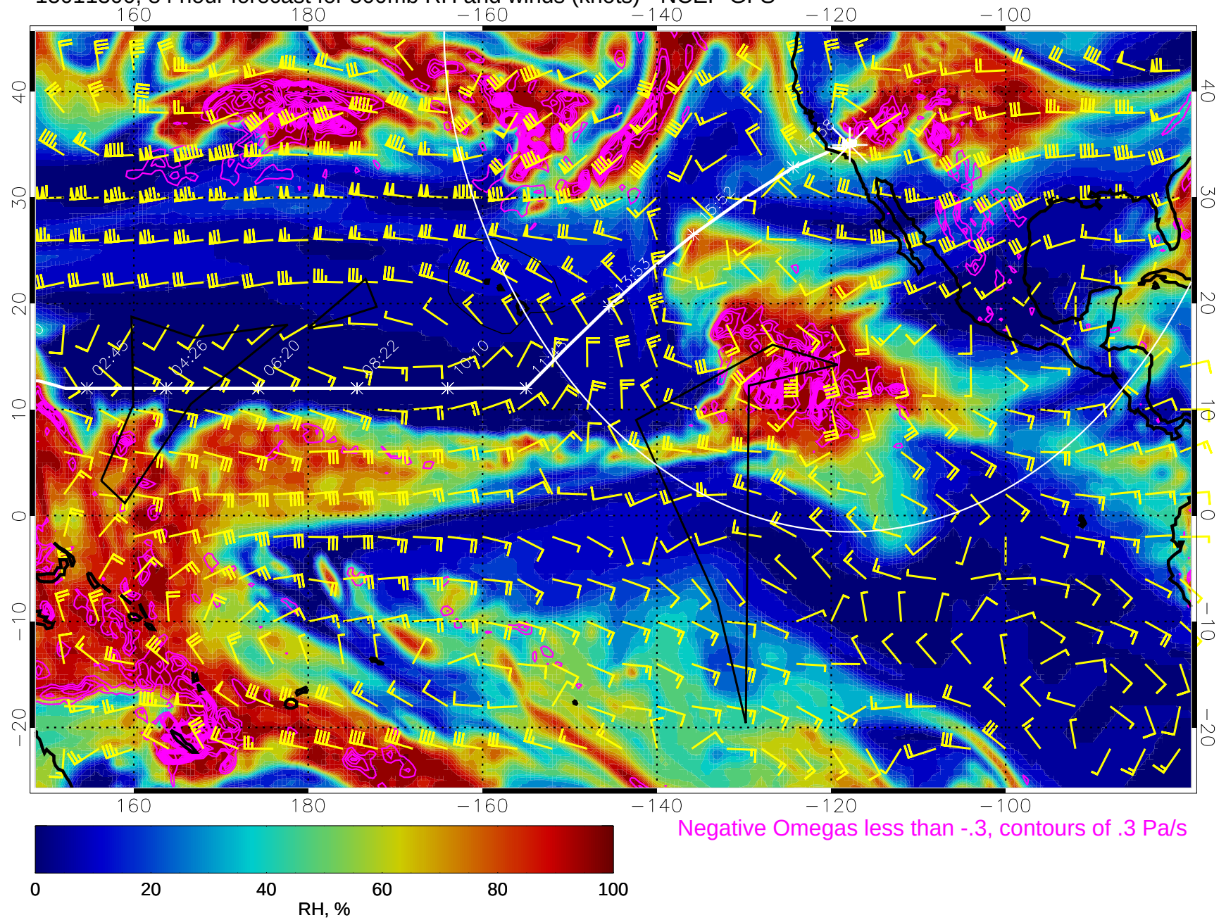
15011300, 84 hour forecast for 500mb RH and winds (knots) - NCEP GFS
