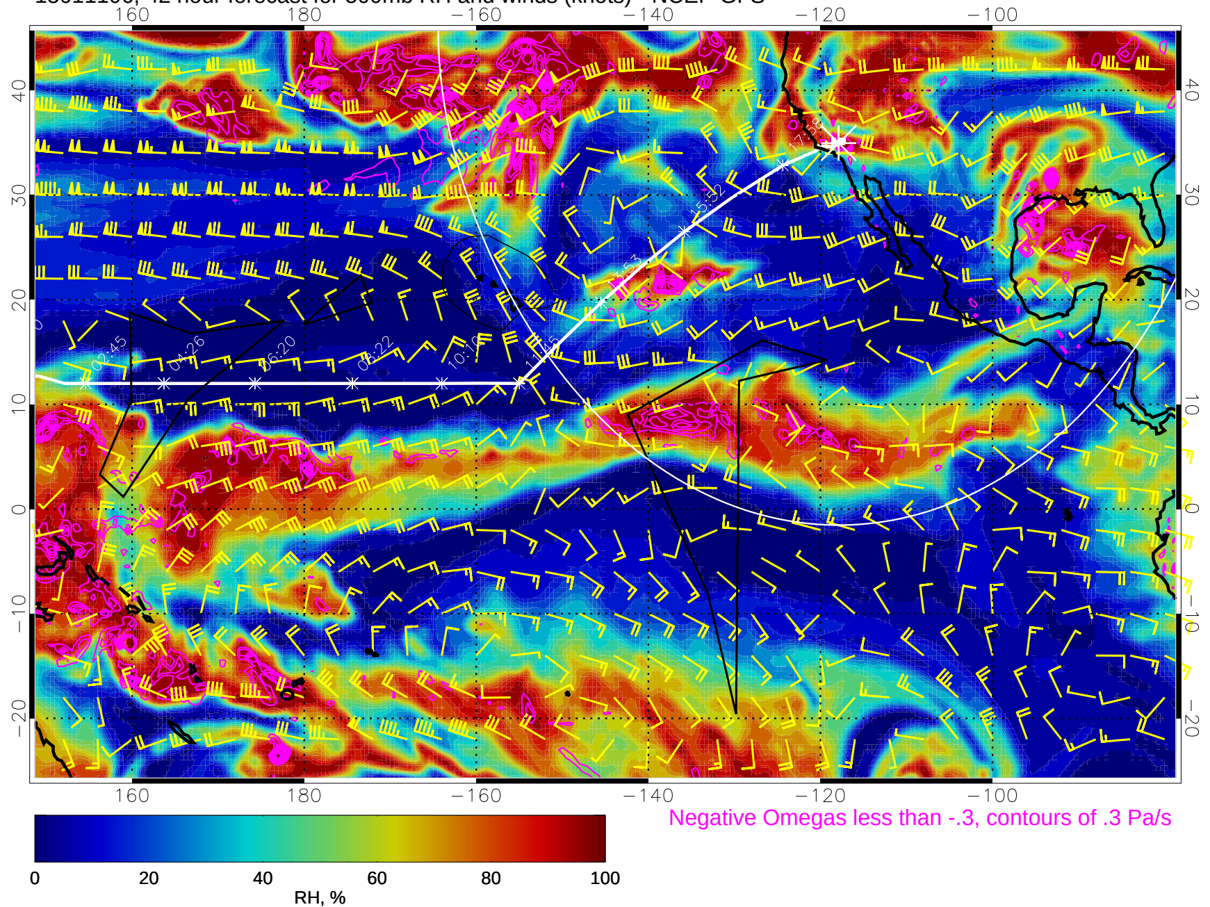
15011106, 42 hour forecast for 500mb RH and winds (knots) - NCEP GFS
