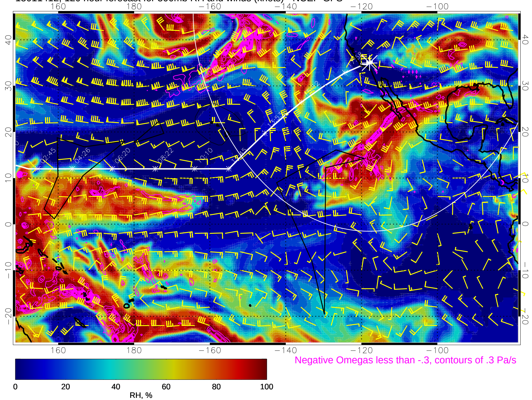
15011412, 120 hour forecast for 500mb RH and winds (knots) - NCEP GFS
