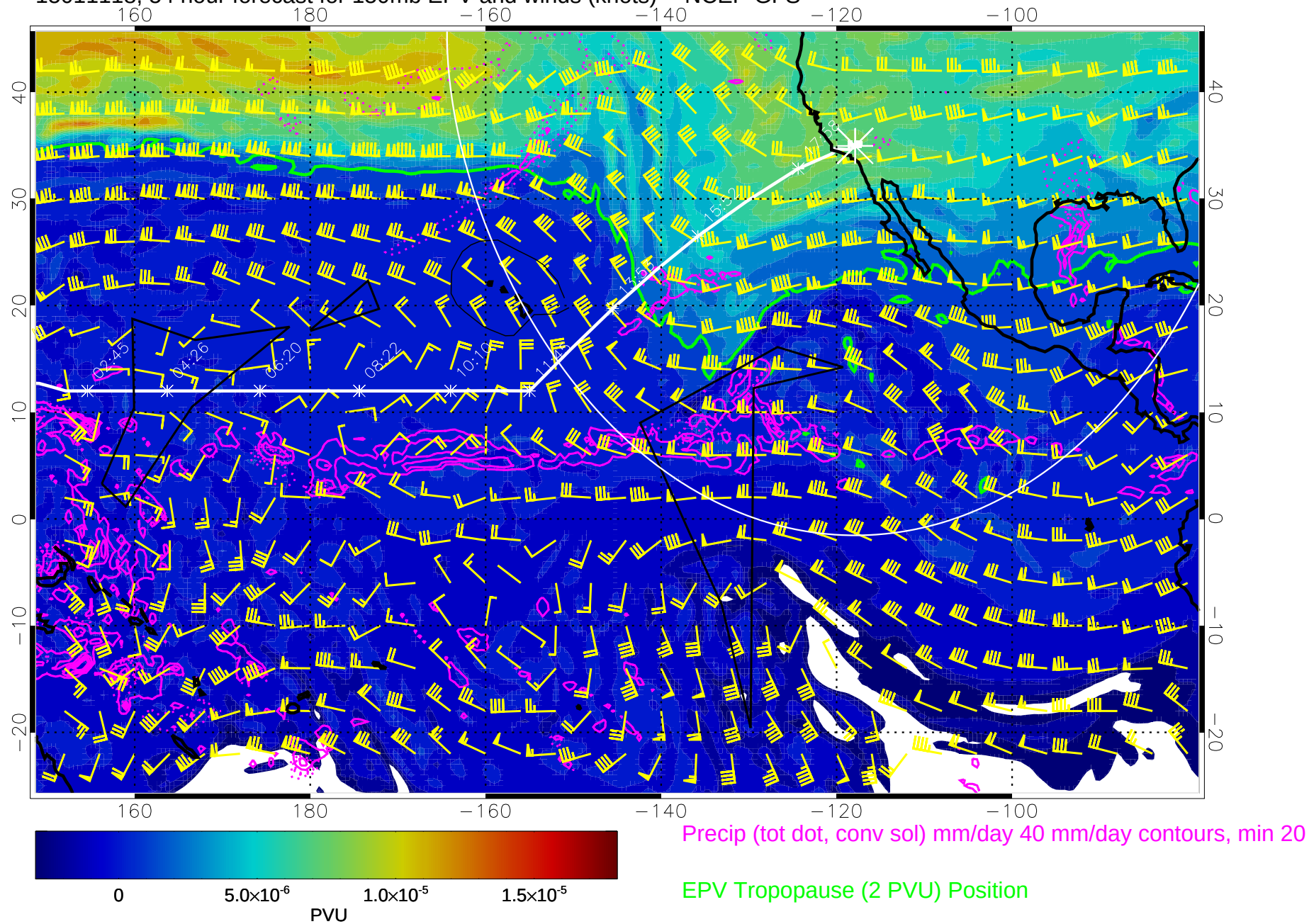
15011118, 54 hour forecast for 150mb EPV and winds (knots) -- NCEP GFS
