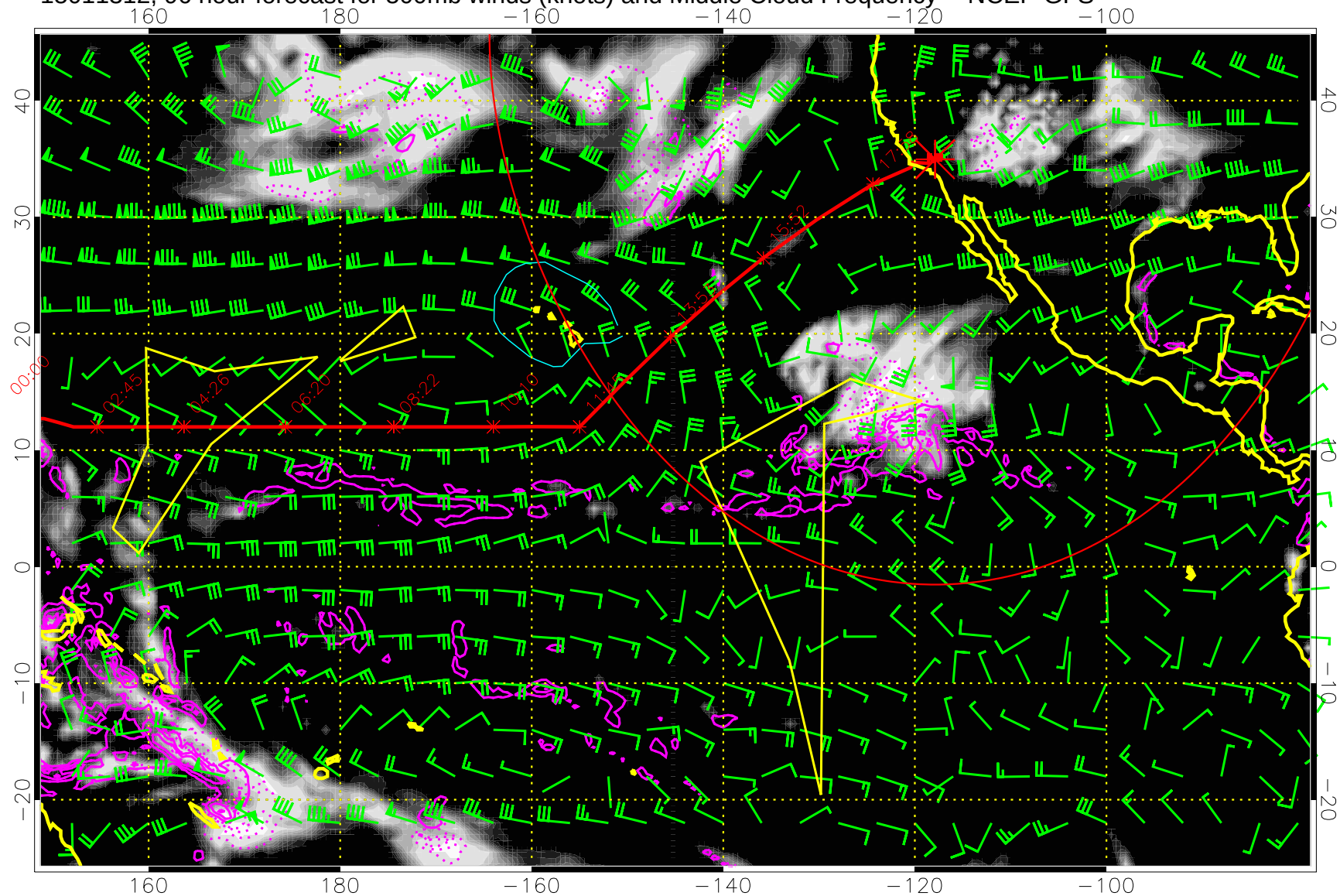
15011312, 96 hour forecast for 500mb winds (knots) and Middle Cloud Frequency -- NCEP GFS
