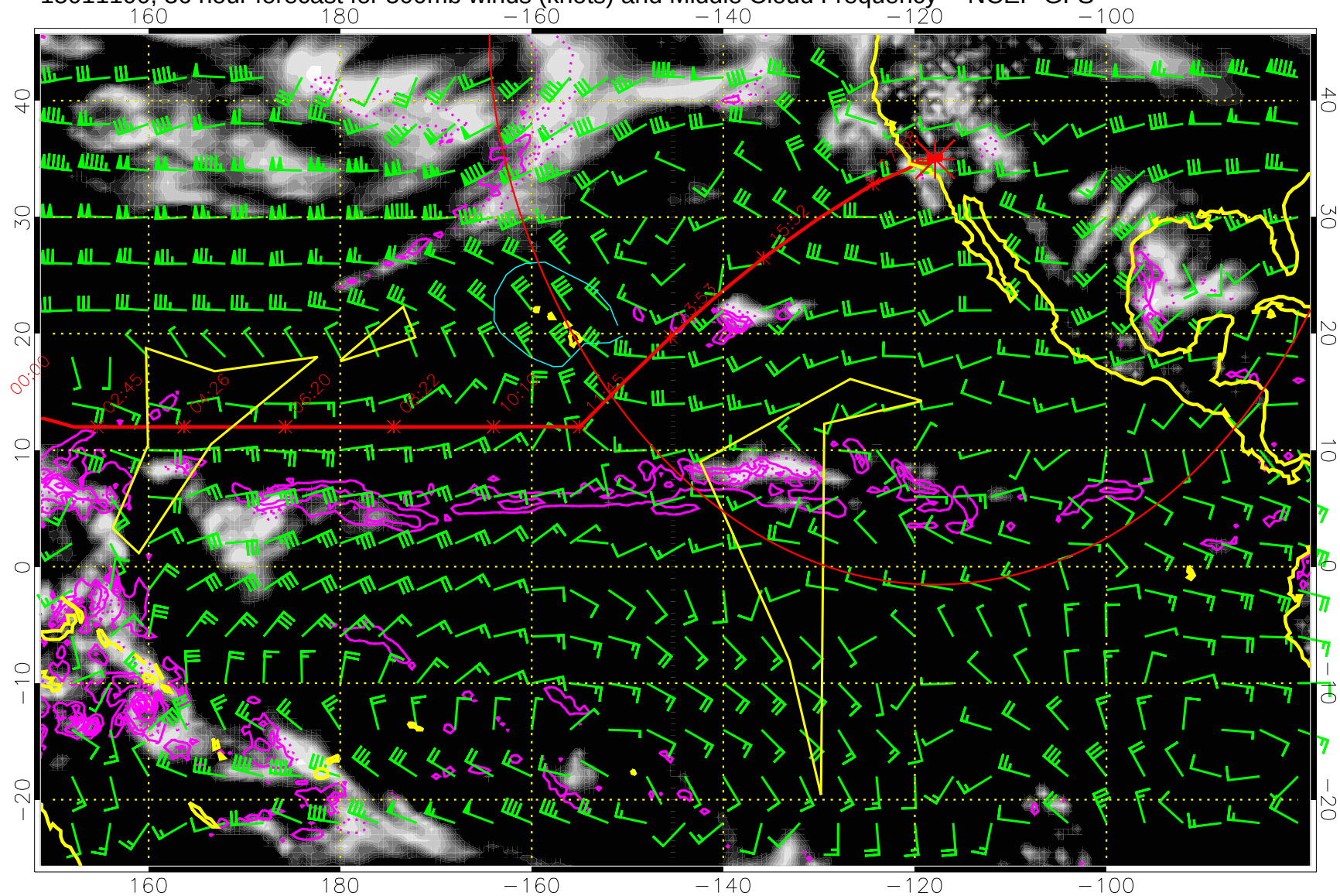
15011100, 36 hour forecast for 500mb winds (knots) and Middle Cloud Frequency -- NCEP GFS
