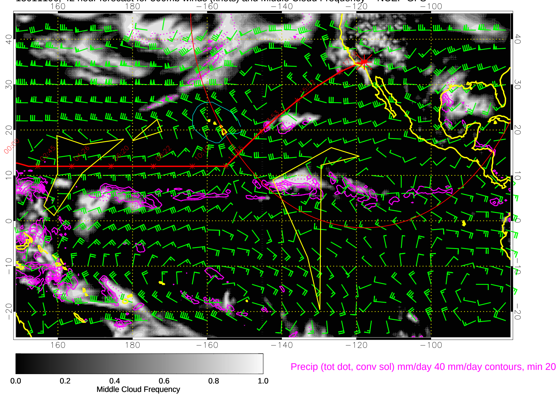
15011106, 42 hour forecast for 500mb winds (knots) and Middle Cloud Frequency -- NCEP GFS
