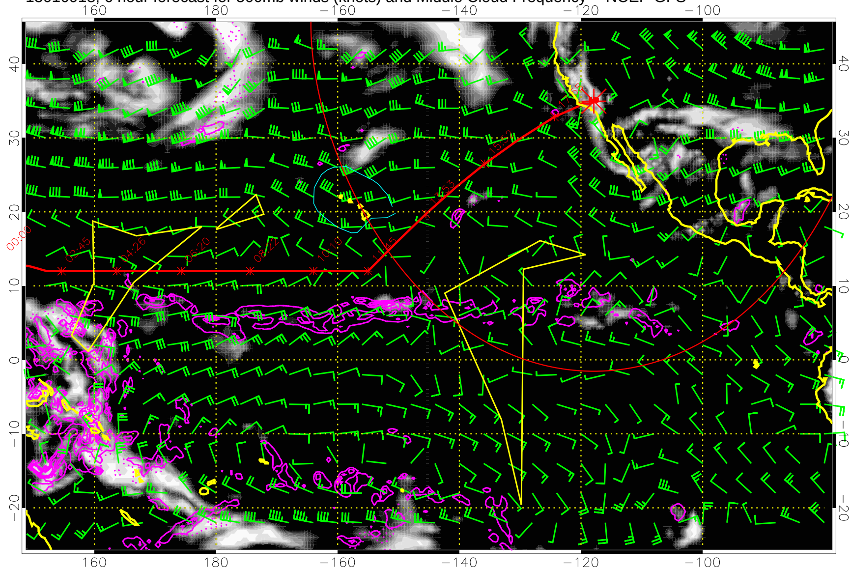
15010918, 6 hour forecast for 500mb winds (knots) and Middle Cloud Frequency -- NCEP GFS
