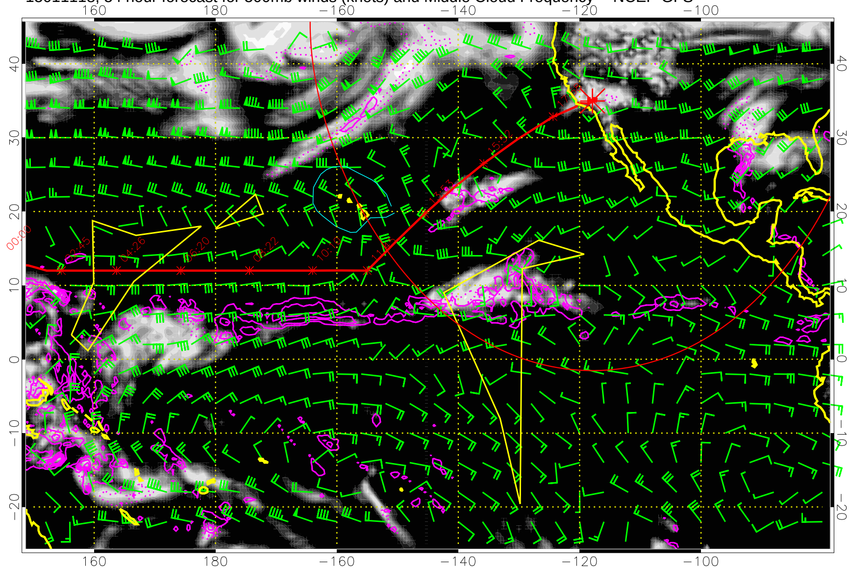
15011118, 54 hour forecast for 500mb winds (knots) and Middle Cloud Frequency -- NCEP GFS
