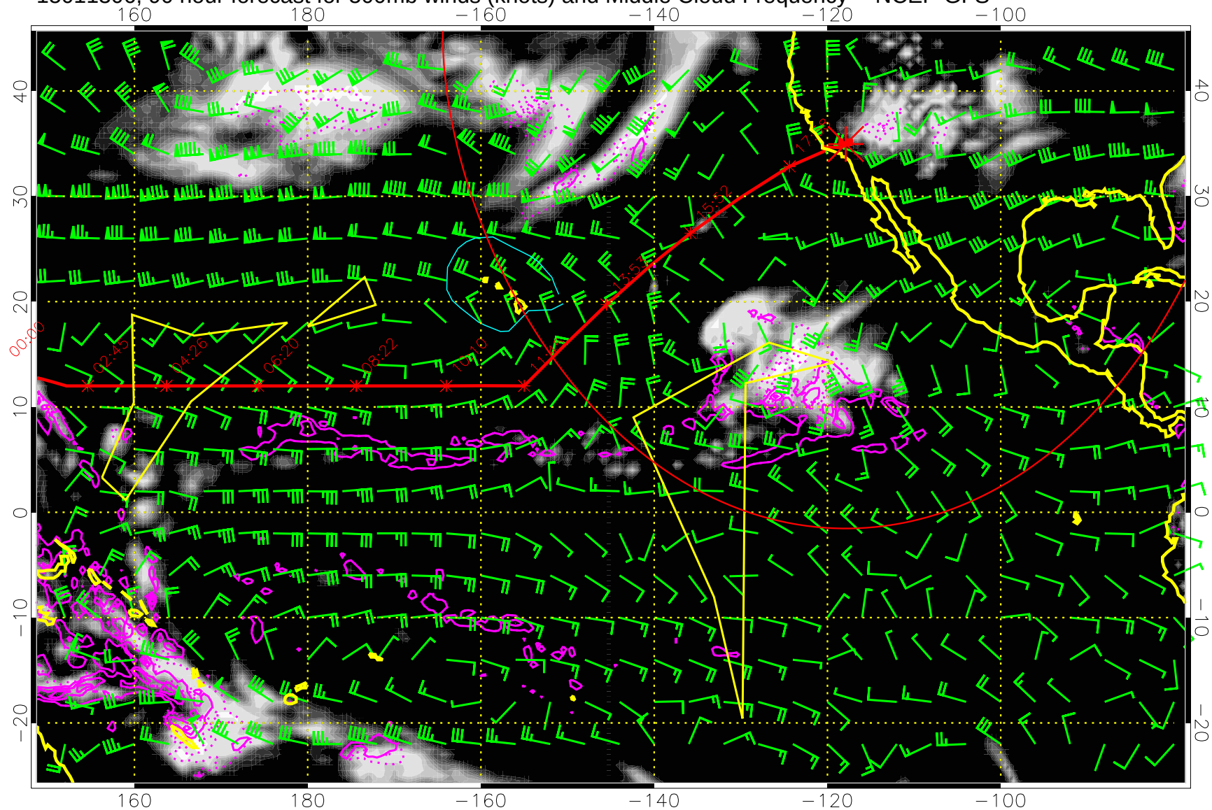
15011306, 90 hour forecast for 500mb winds (knots) and Middle Cloud Frequency -- NCEP GFS
