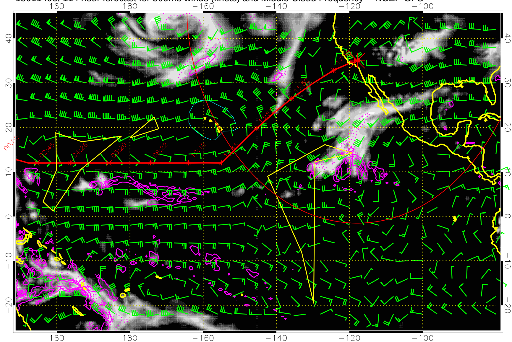
15011406, 114 hour forecast for 500mb winds (knots) and Middle Cloud Frequency -- NCEP GFS
