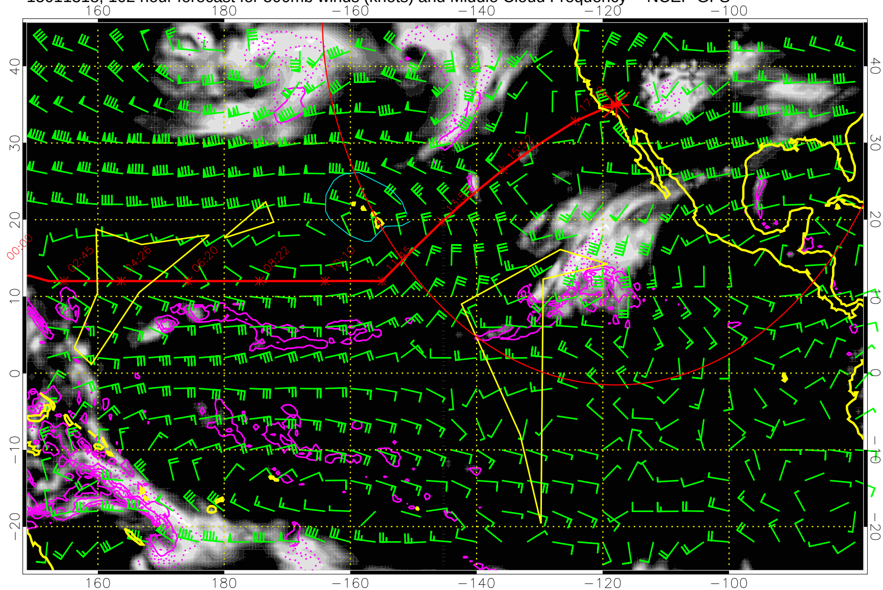
15011318, 102 hour forecast for 500mb winds (knots) and Middle Cloud Frequency -- NCEP GFS
