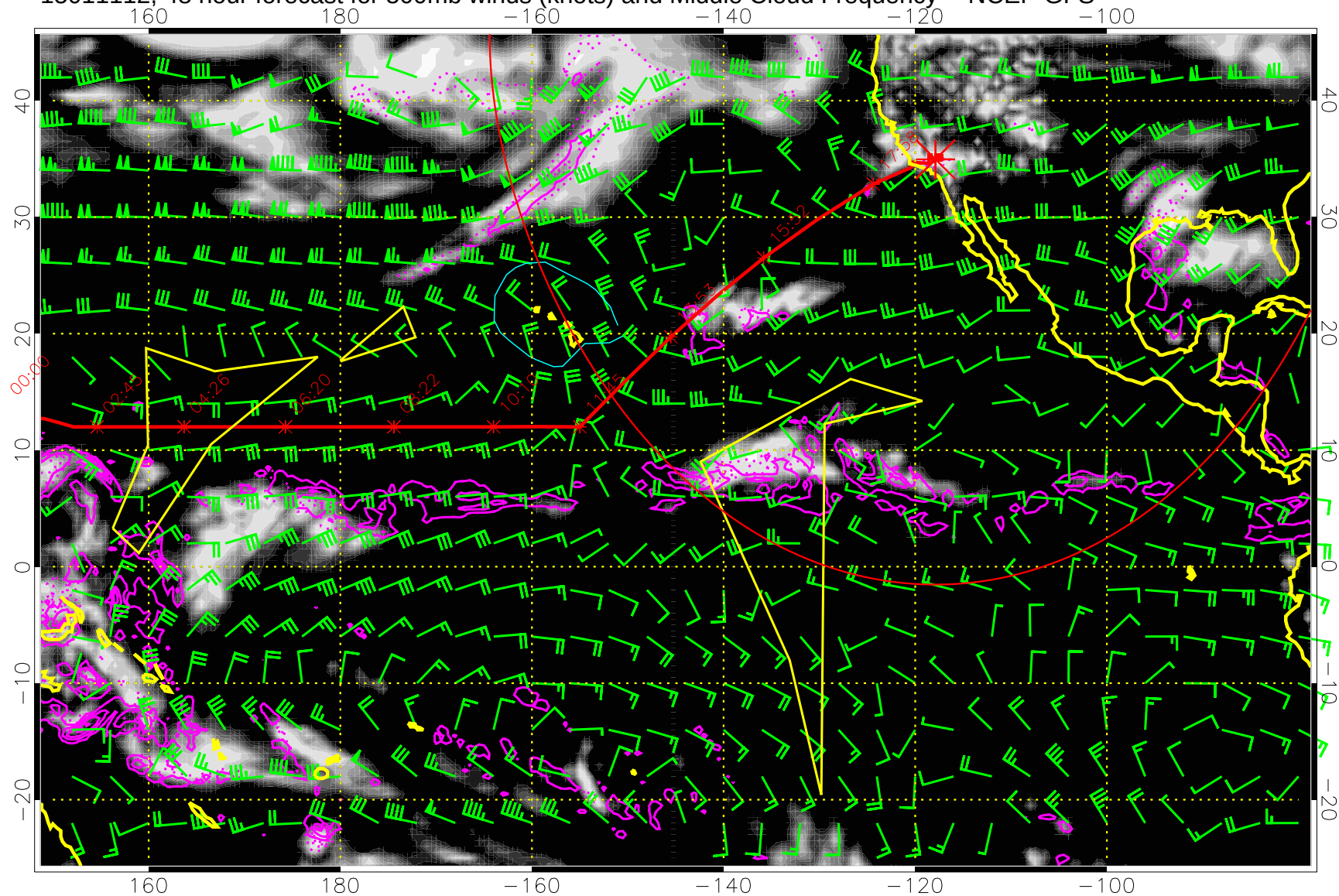
15011112, 48 hour forecast for 500mb winds (knots) and Middle Cloud Frequency -- NCEP GFS
