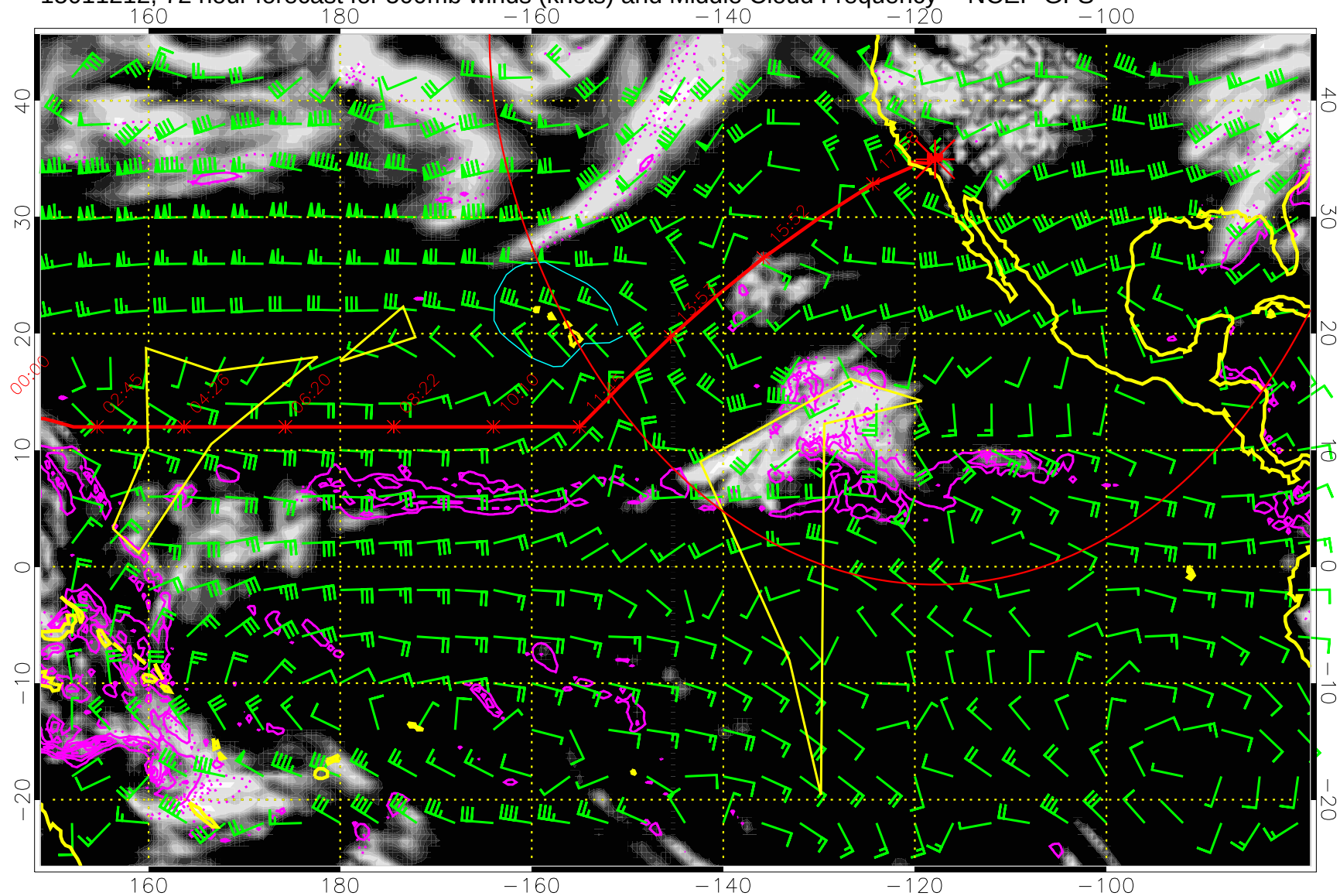
15011212, 72 hour forecast for 500mb winds (knots) and Middle Cloud Frequency -- NCEP GFS
