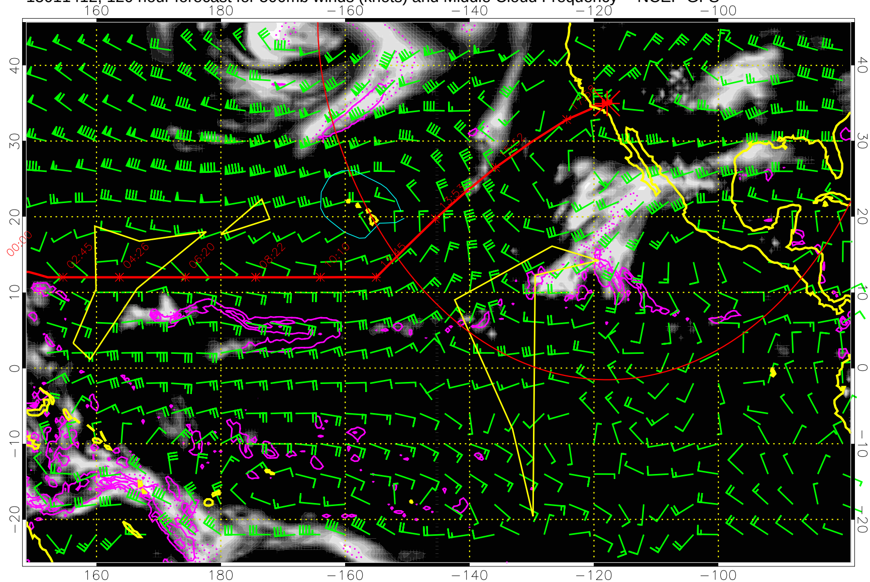
15011412, 120 hour forecast for 500mb winds (knots) and Middle Cloud Frequency -- NCEP GFS
