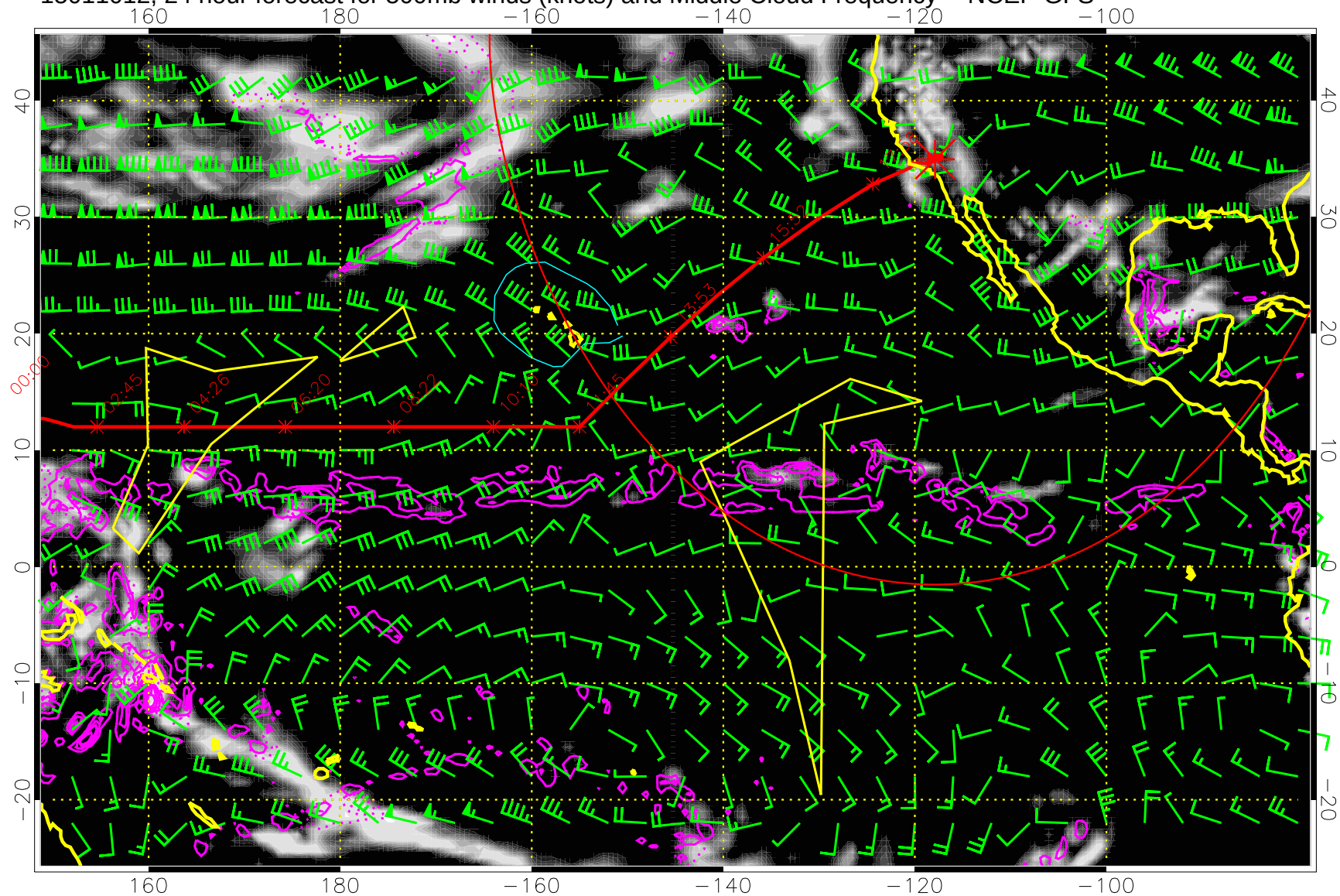
15011012, 24 hour forecast for 500mb winds (knots) and Middle Cloud Frequency -- NCEP GFS
