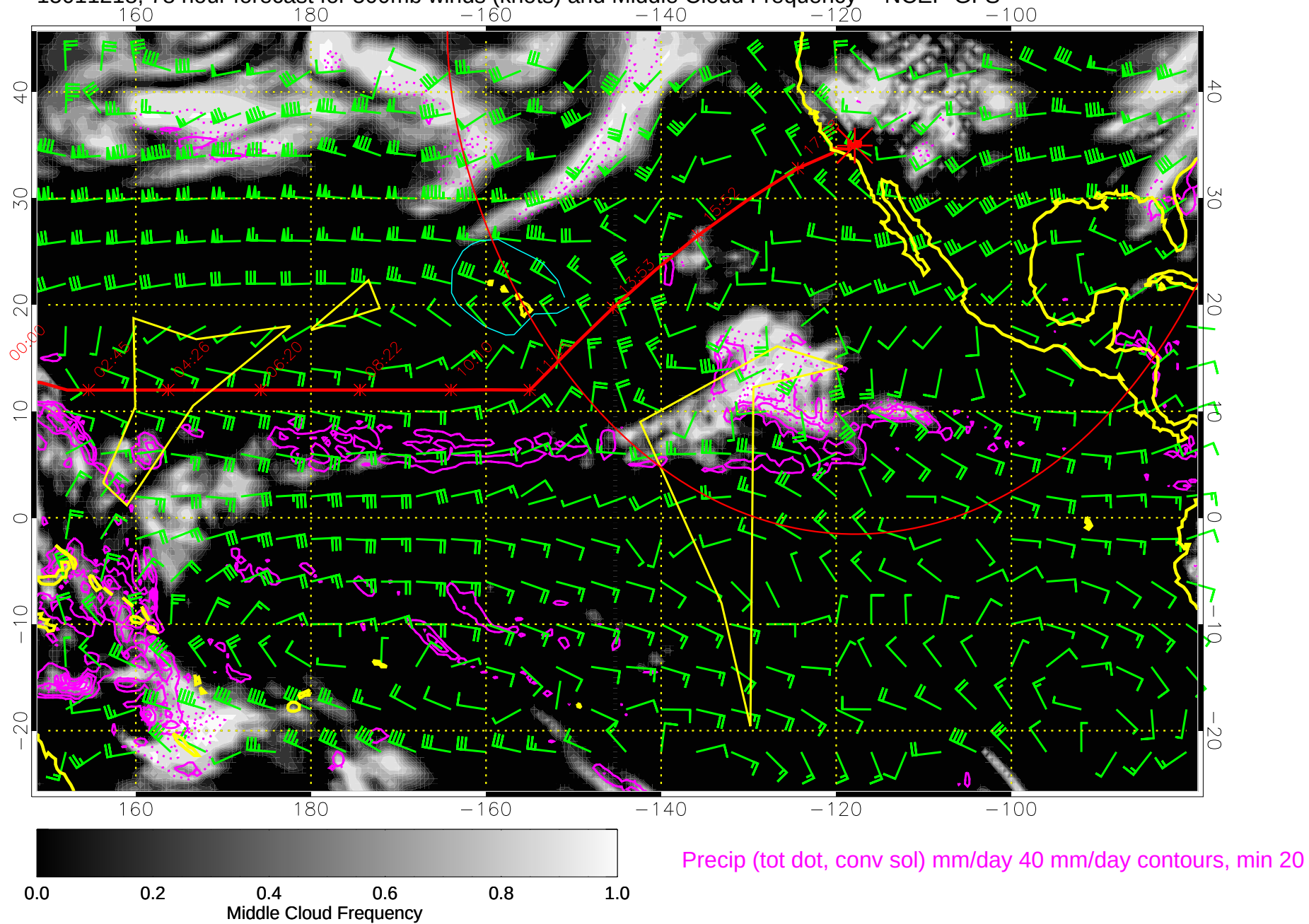
15011218, 78 hour forecast for 500mb winds (knots) and Middle Cloud Frequency -- NCEP GFS
