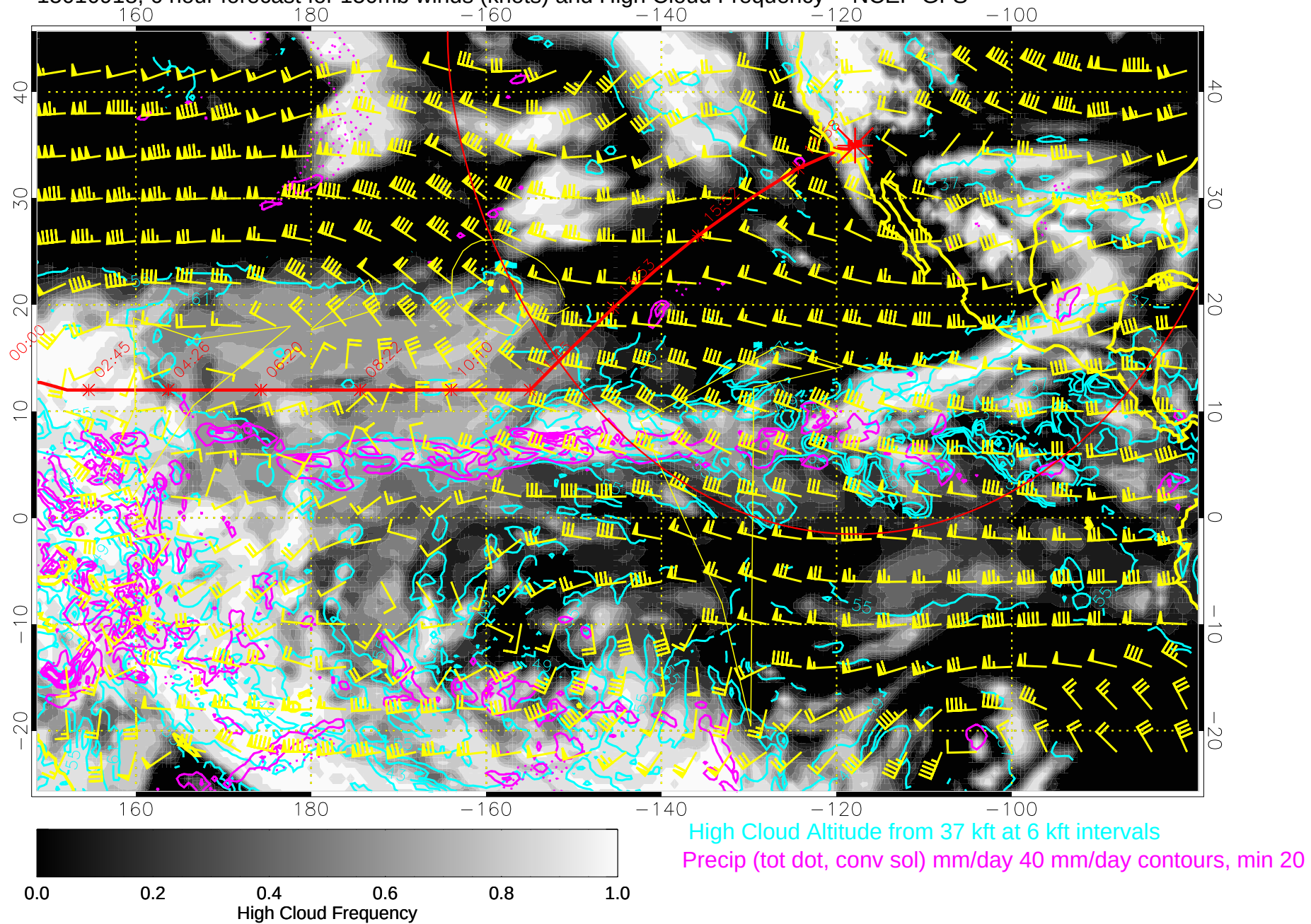
15010918, 6 hour forecast for 150mb winds (knots) and High Cloud Frequency -- NCEP GFS
