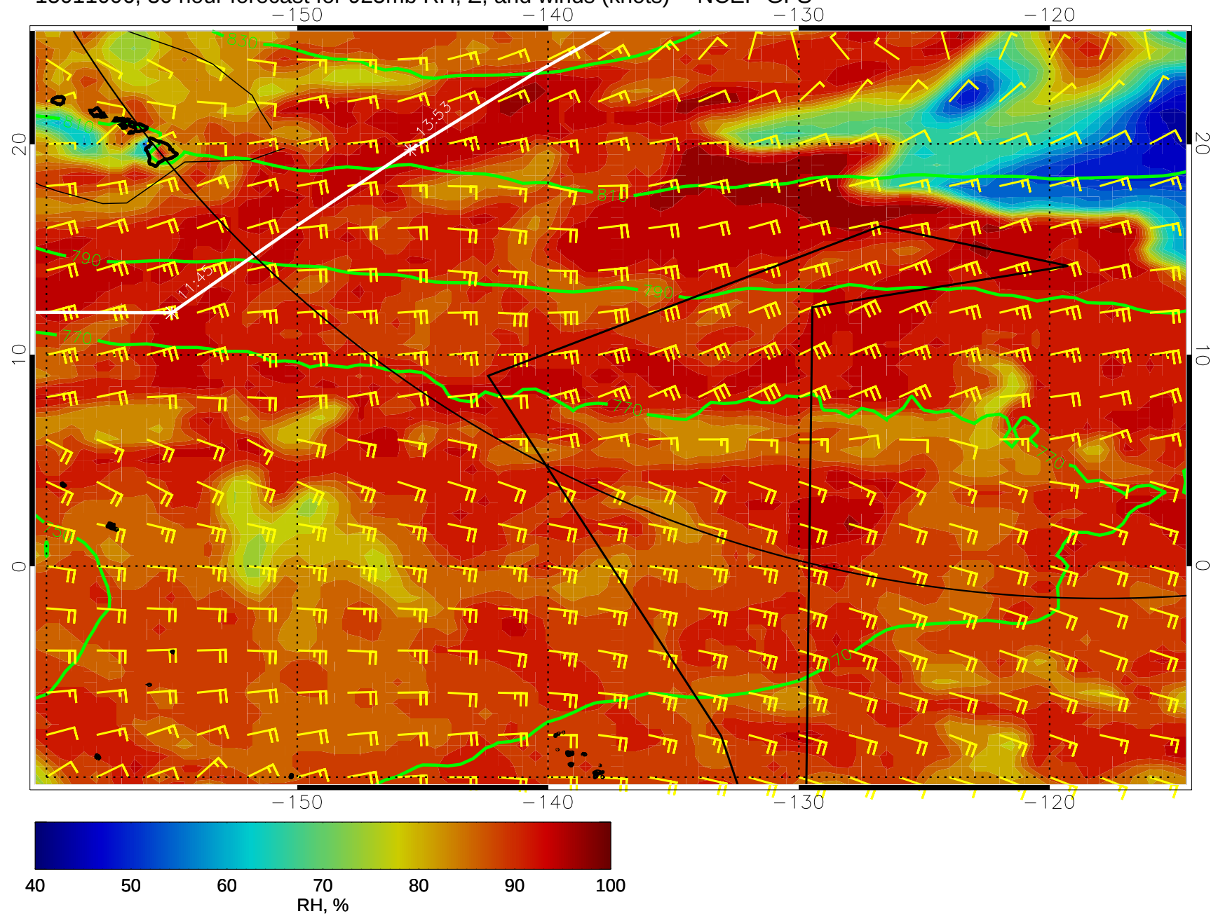
15011006, 30 hour forecast for 925mb RH, Z, and winds (knots) -- NCEP GFS
