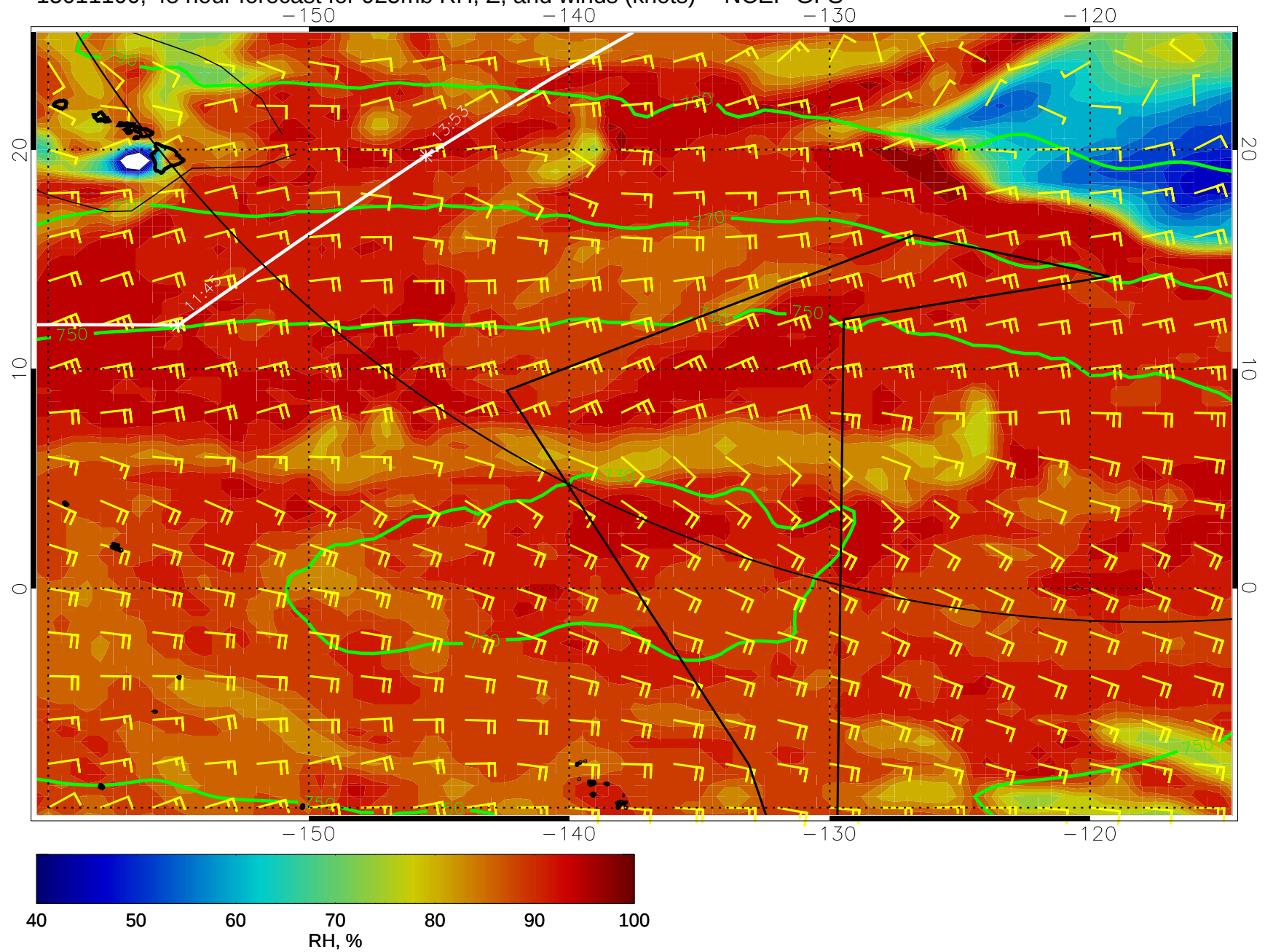
15011100, 48 hour forecast for 925mb RH, Z, and winds (knots) -- NCEP GFS
