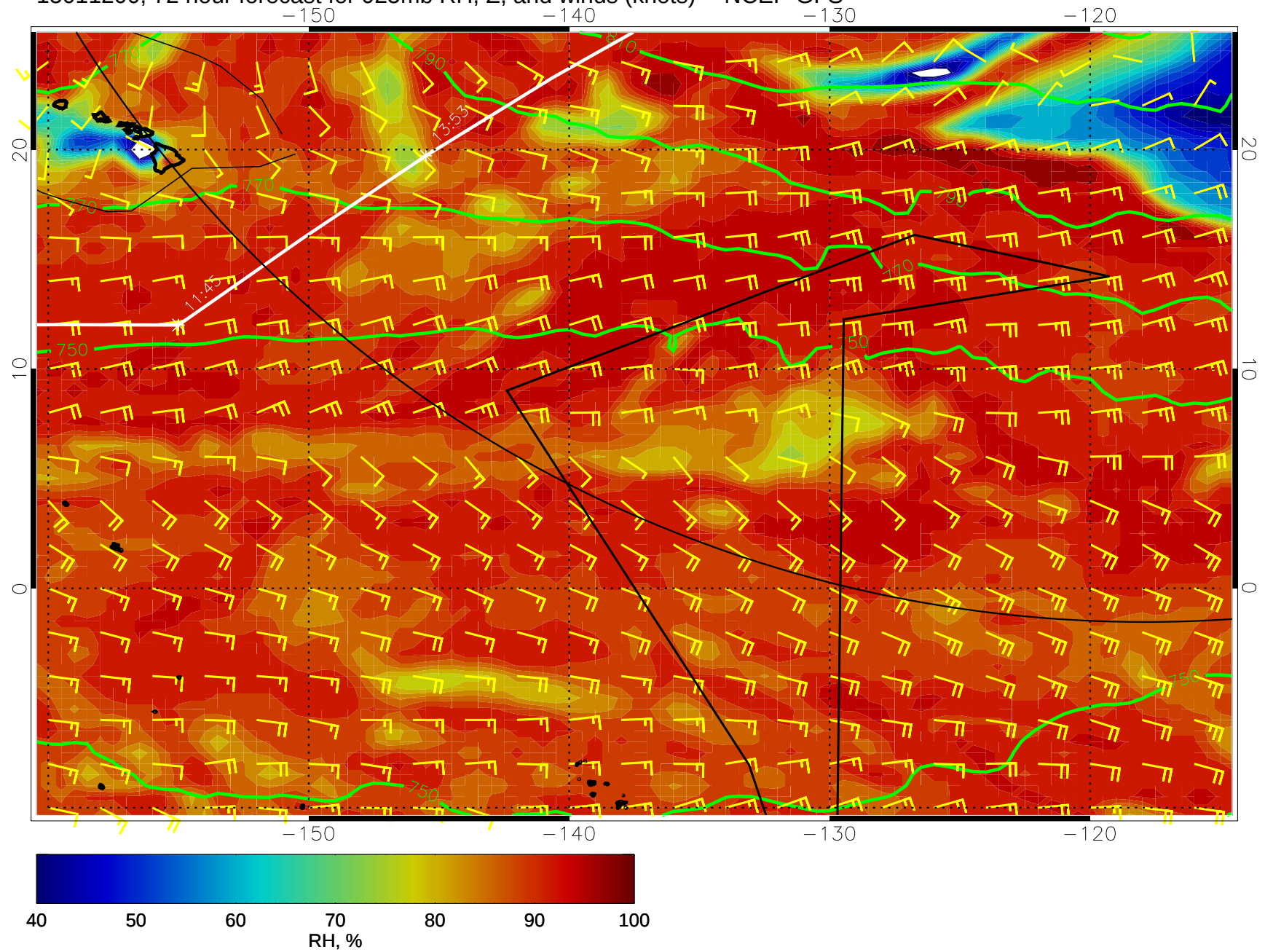
15011200, 72 hour forecast for 925mb RH, Z, and winds (knots) -- NCEP GFS
