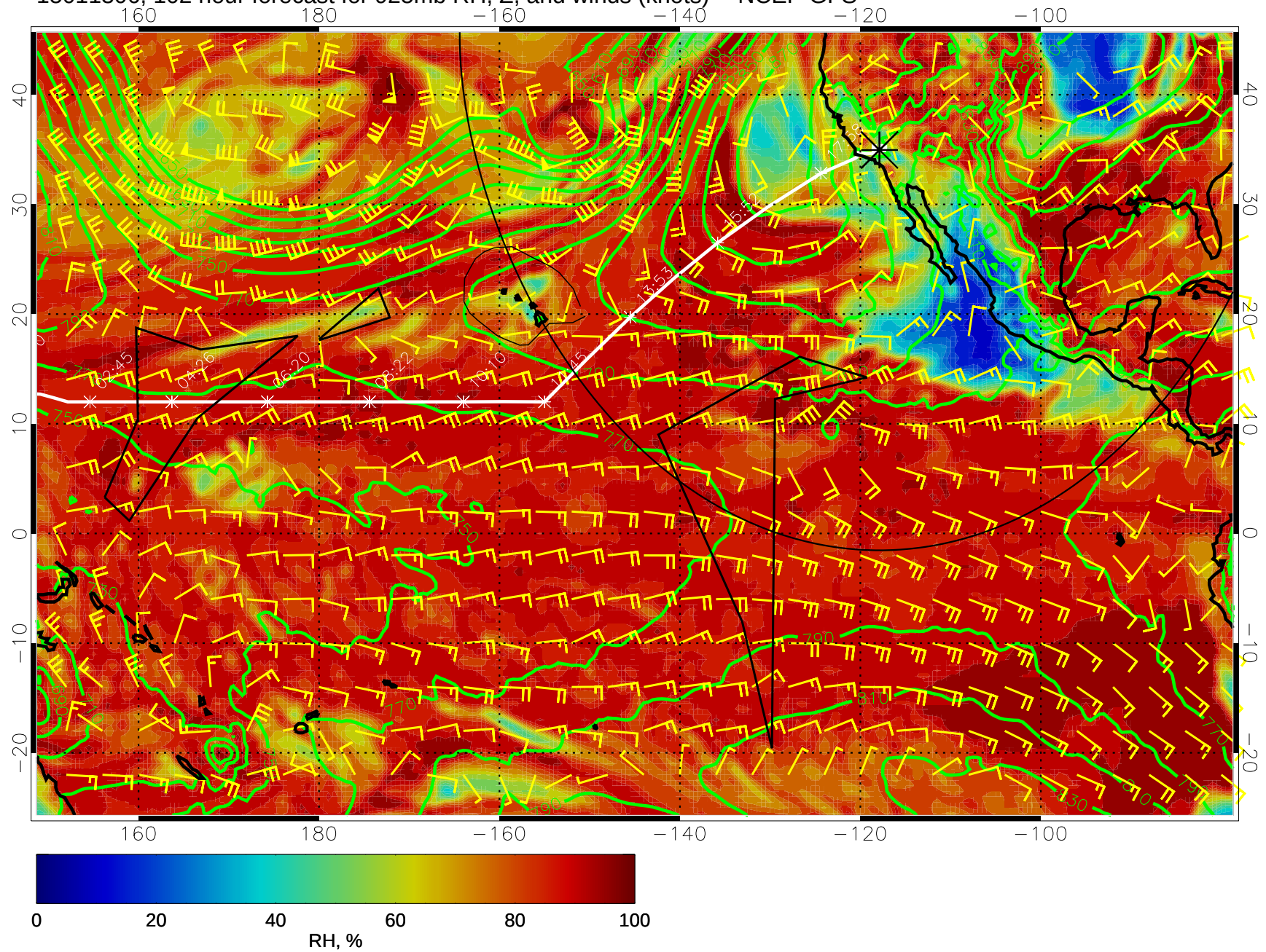
15011306, 102 hour forecast for 925mb RH, Z, and winds (knots) -- NCEP GFS
