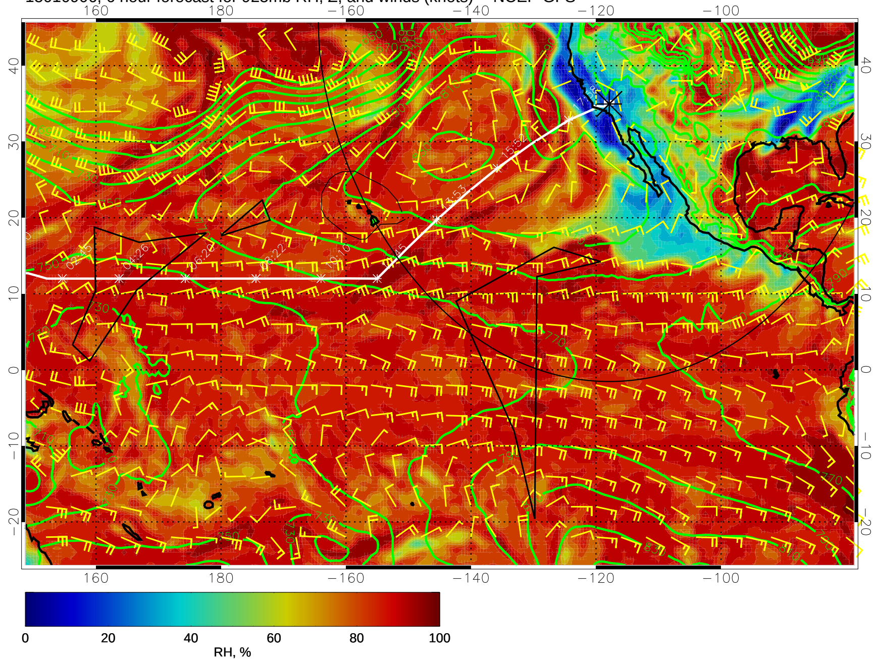
15010906, 6 hour forecast for 925mb RH, Z, and winds (knots) -- NCEP GFS
