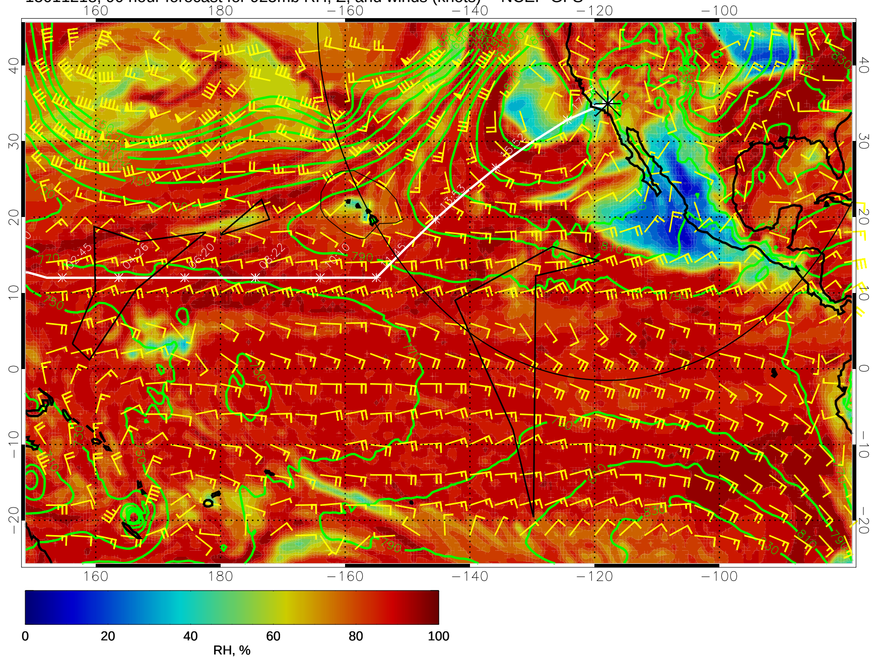
15011218, 90 hour forecast for 925mb RH, Z, and winds (knots) -- NCEP GFS
