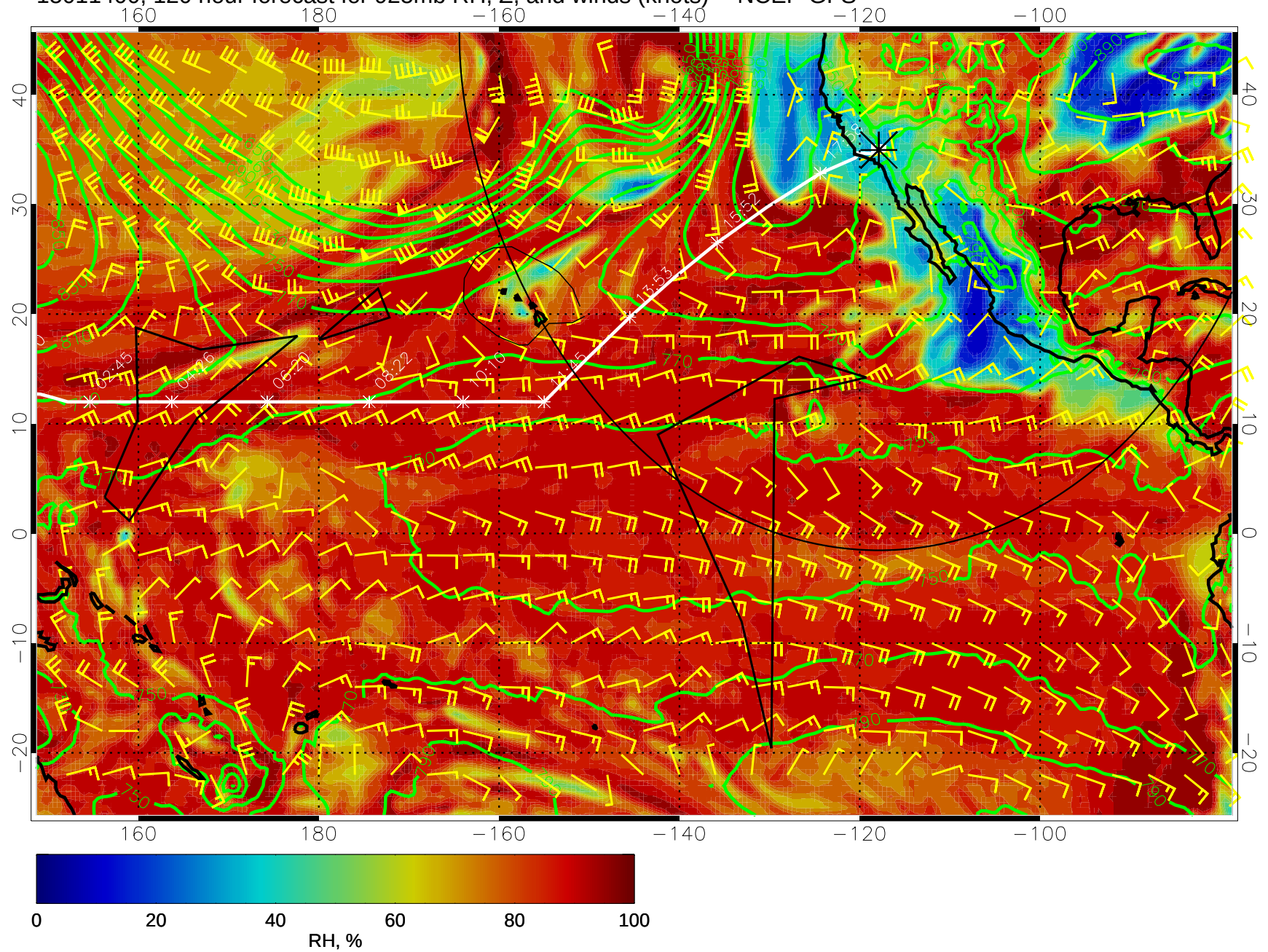
15011400, 120 hour forecast for 925mb RH, Z, and winds (knots) -- NCEP GFS
