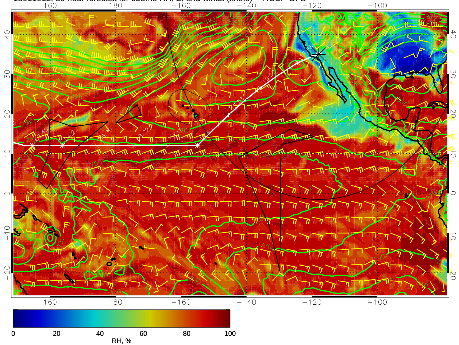
15011012, 36 hour forecast for 925mb RH, Z, and winds (knots) -- NCEP GFS
