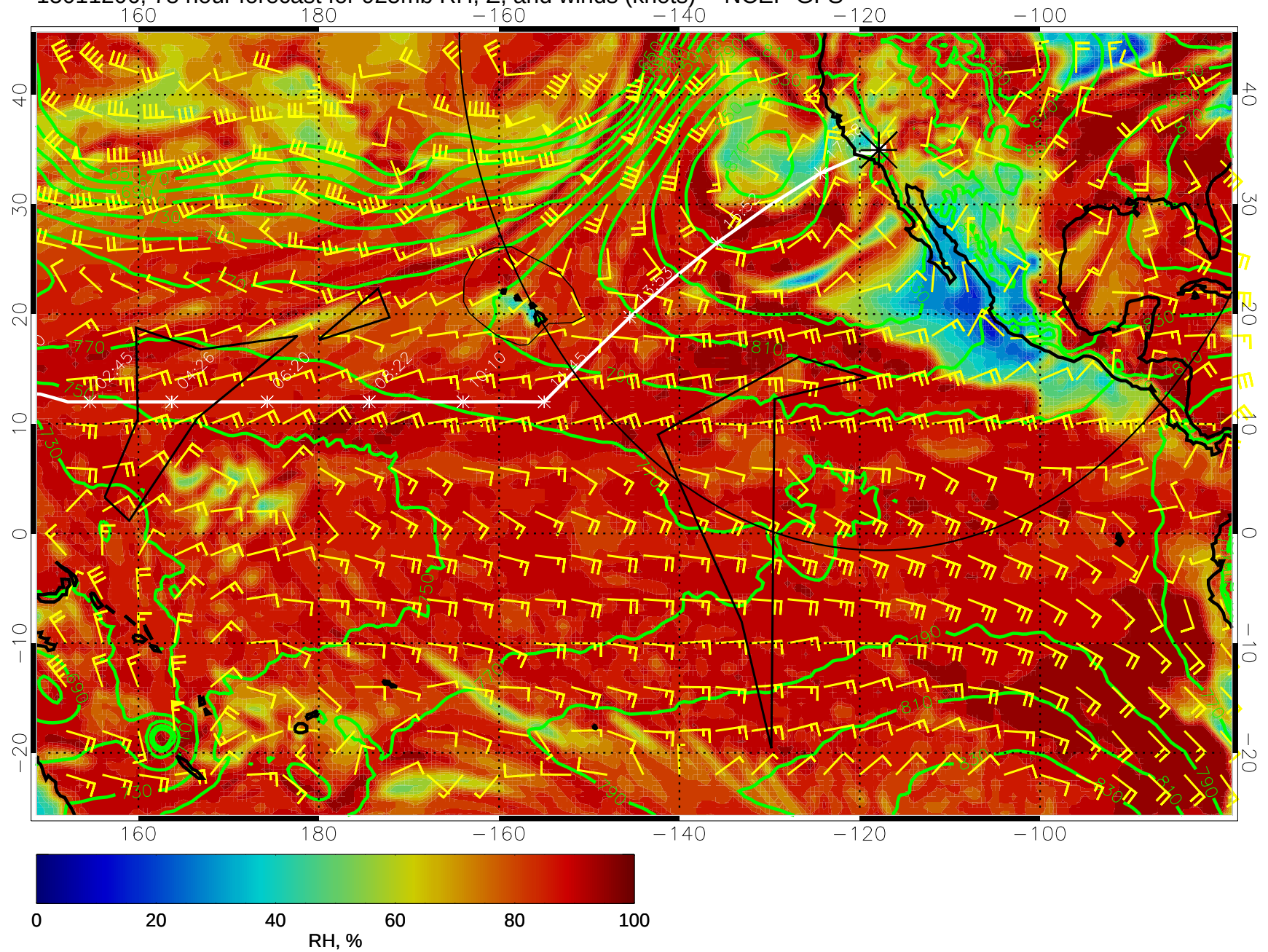
15011206, 78 hour forecast for 925mb RH, Z, and winds (knots) -- NCEP GFS
