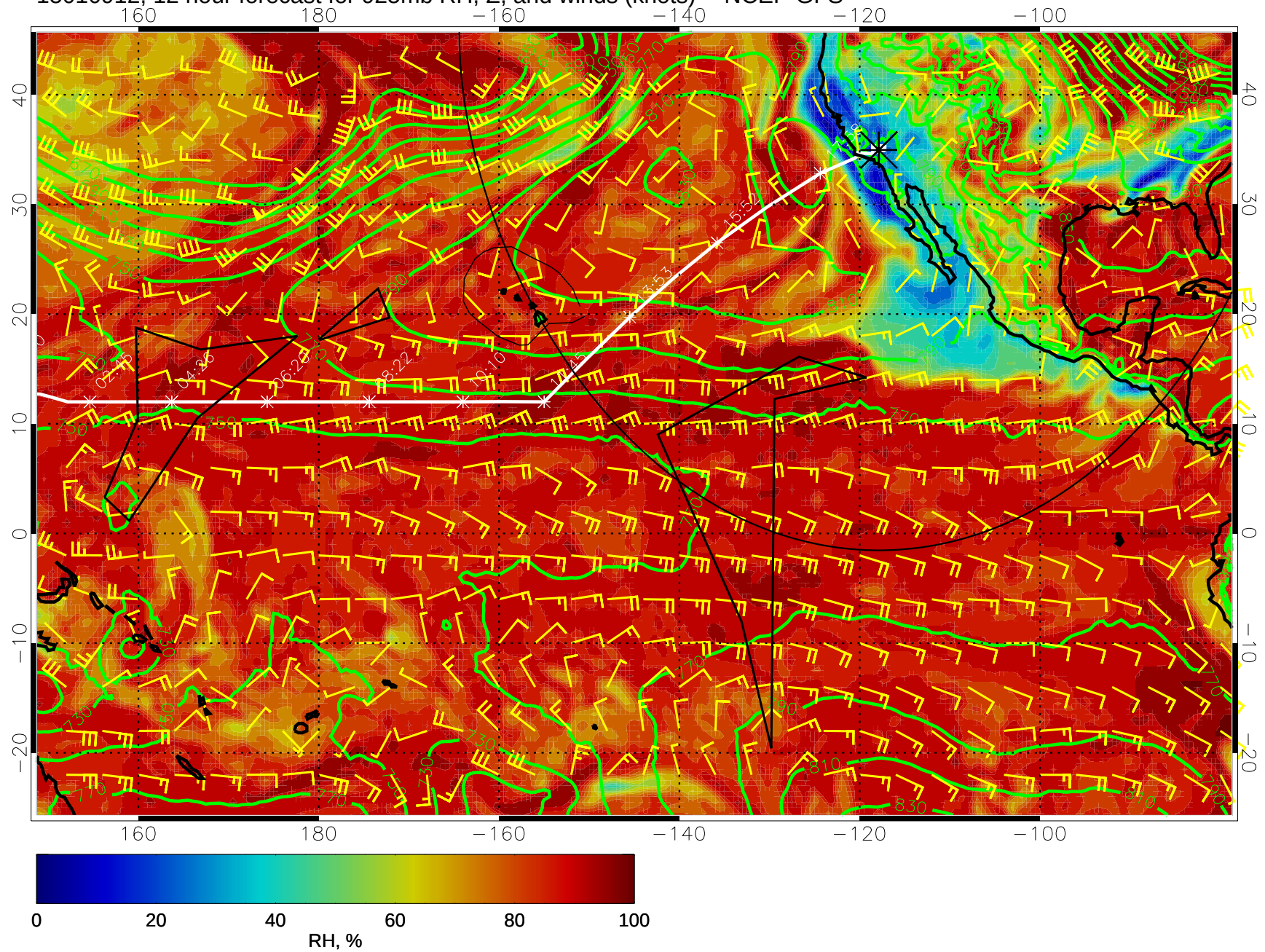
15010912, 12 hour forecast for 925mb RH, Z, and winds (knots) -- NCEP GFS
