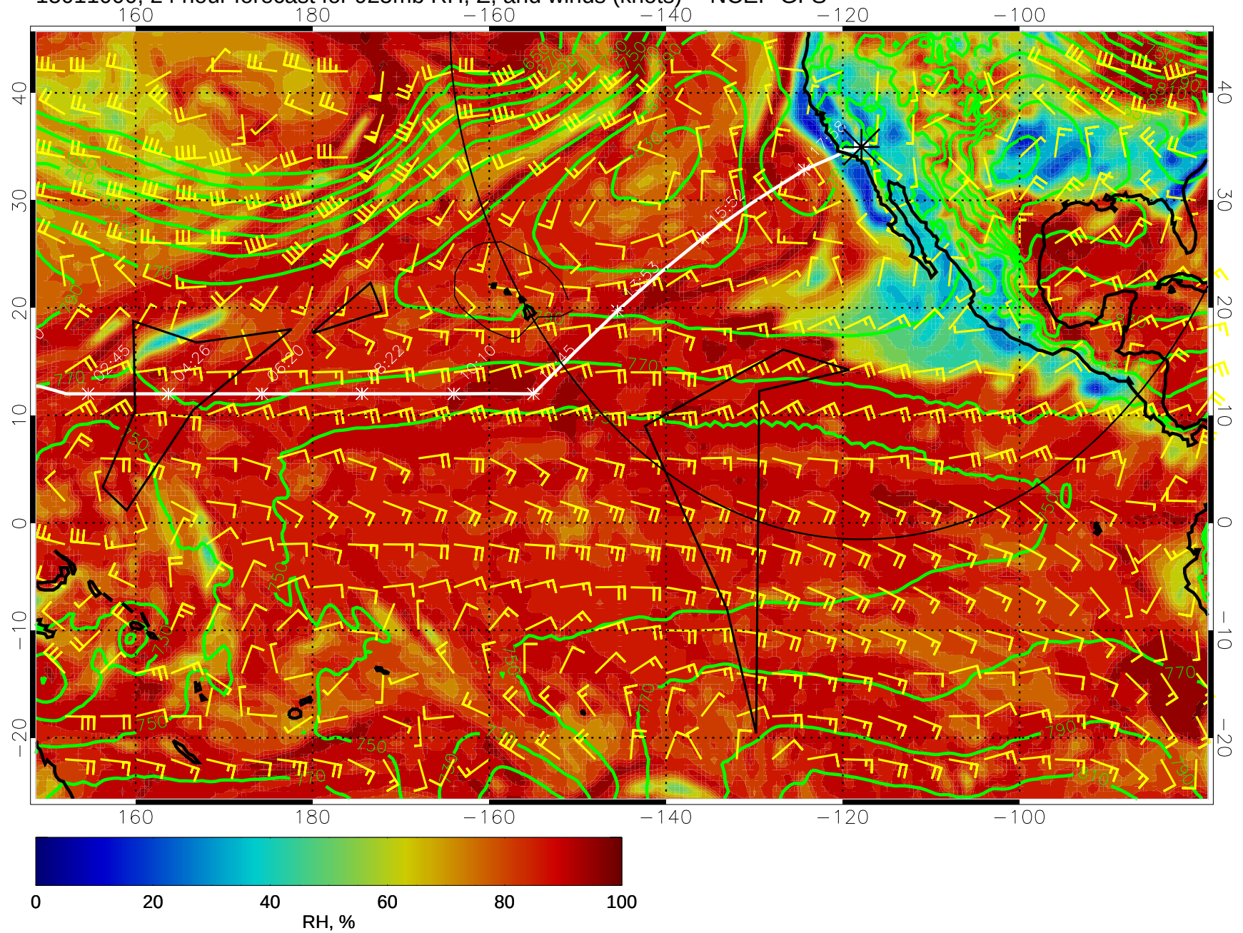
15011000, 24 hour forecast for 925mb RH, Z, and winds (knots) -- NCEP GFS
