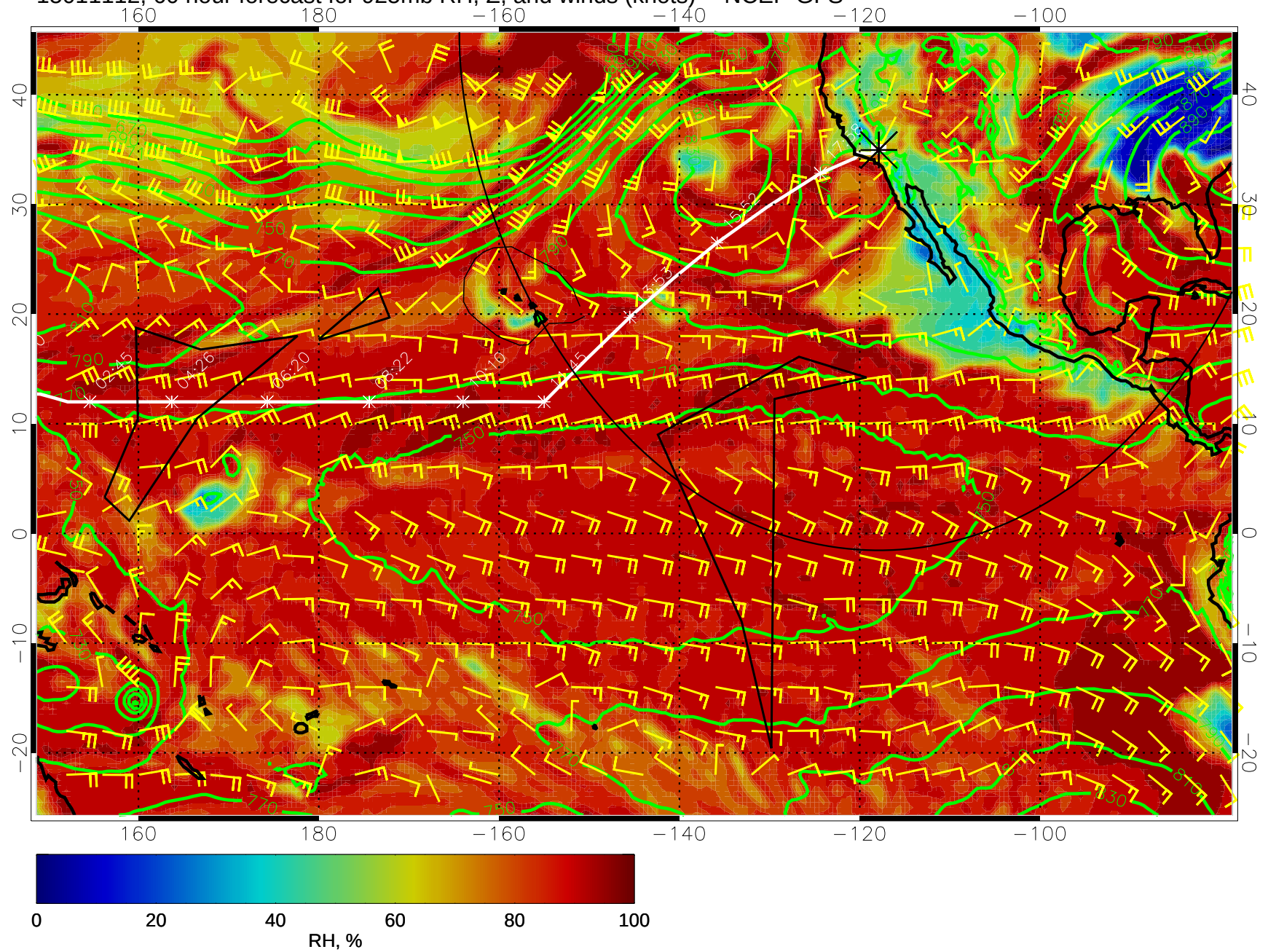
15011112, 60 hour forecast for 925mb RH, Z, and winds (knots) -- NCEP GFS
