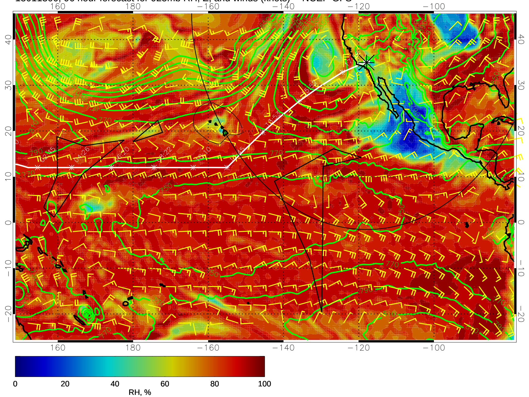
15011300, 96 hour forecast for 925mb RH, Z, and winds (knots) -- NCEP GFS
