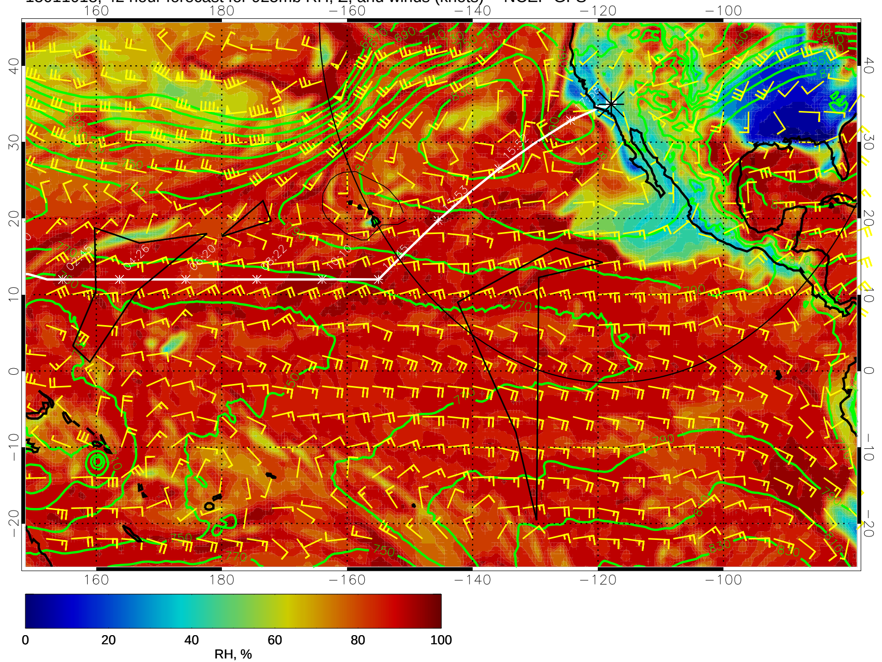
15011018, 42 hour forecast for 925mb RH, Z, and winds (knots) -- NCEP GFS
