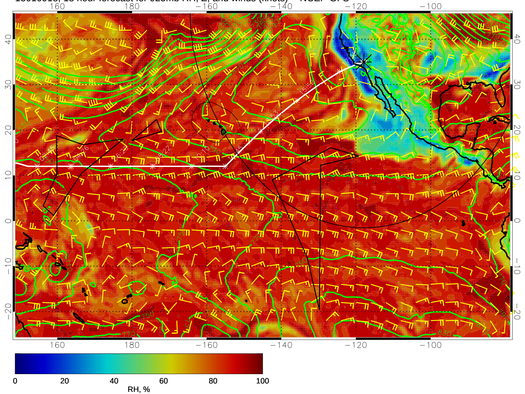
15010918, 18 hour forecast for 925mb RH, Z, and winds (knots) -- NCEP GFS
