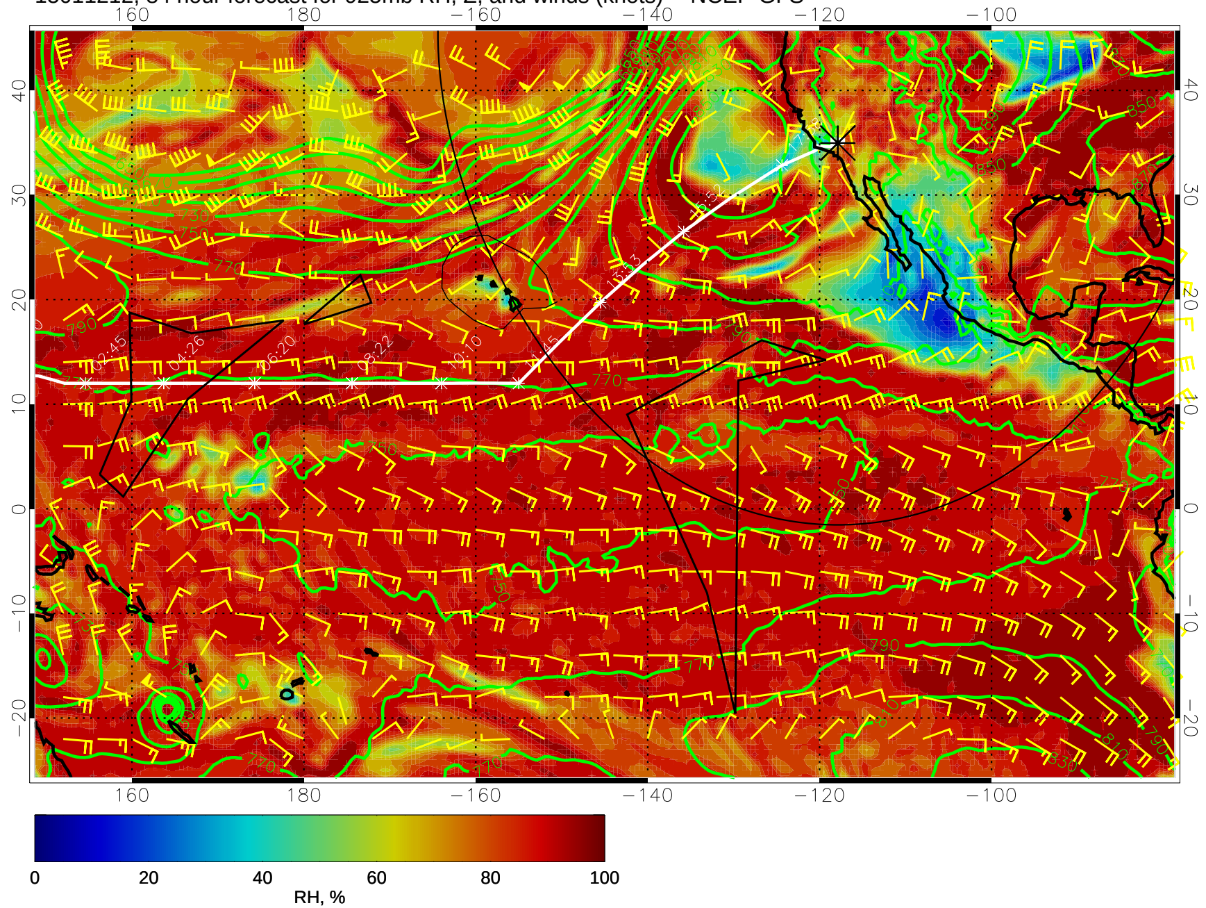
15011212, 84 hour forecast for 925mb RH, Z, and winds (knots) -- NCEP GFS
