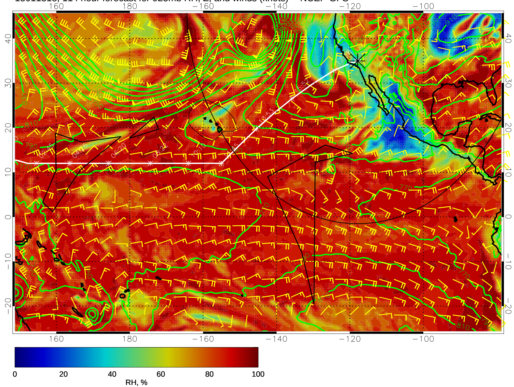
15011318, 114 hour forecast for 925mb RH, Z, and winds (knots) -- NCEP GFS
