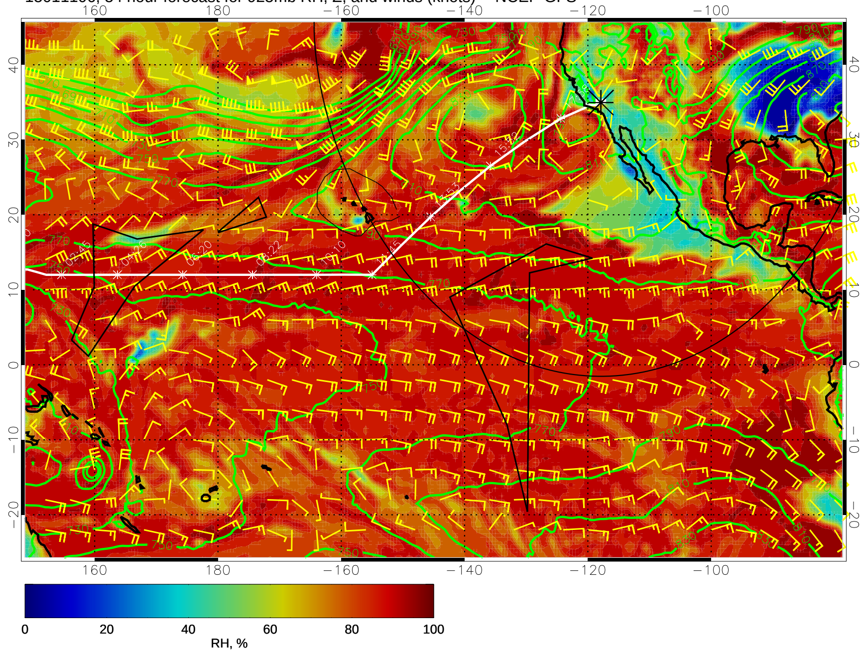
15011106, 54 hour forecast for 925mb RH, Z, and winds (knots) -- NCEP GFS
