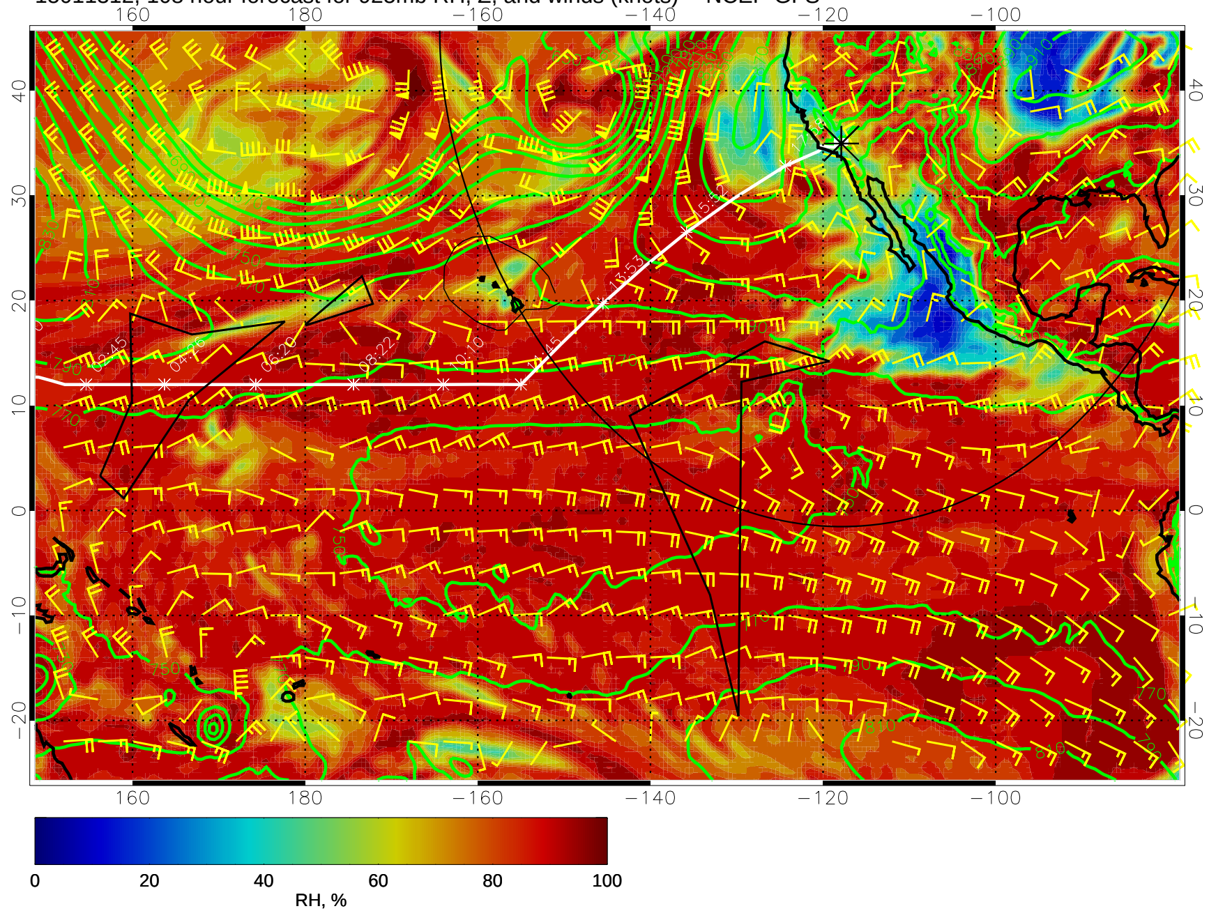
15011312, 108 hour forecast for 925mb RH, Z, and winds (knots) -- NCEP GFS
