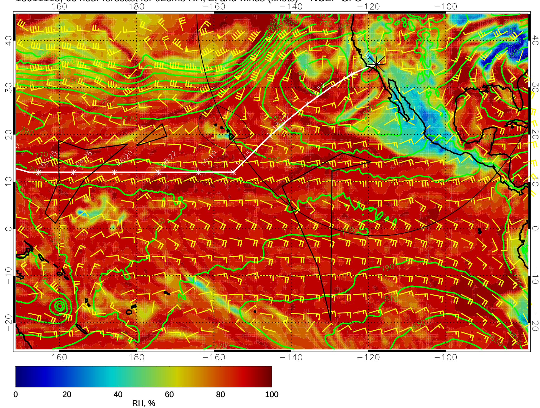
15011118, 66 hour forecast for 925mb RH, Z, and winds (knots) -- NCEP GFS
