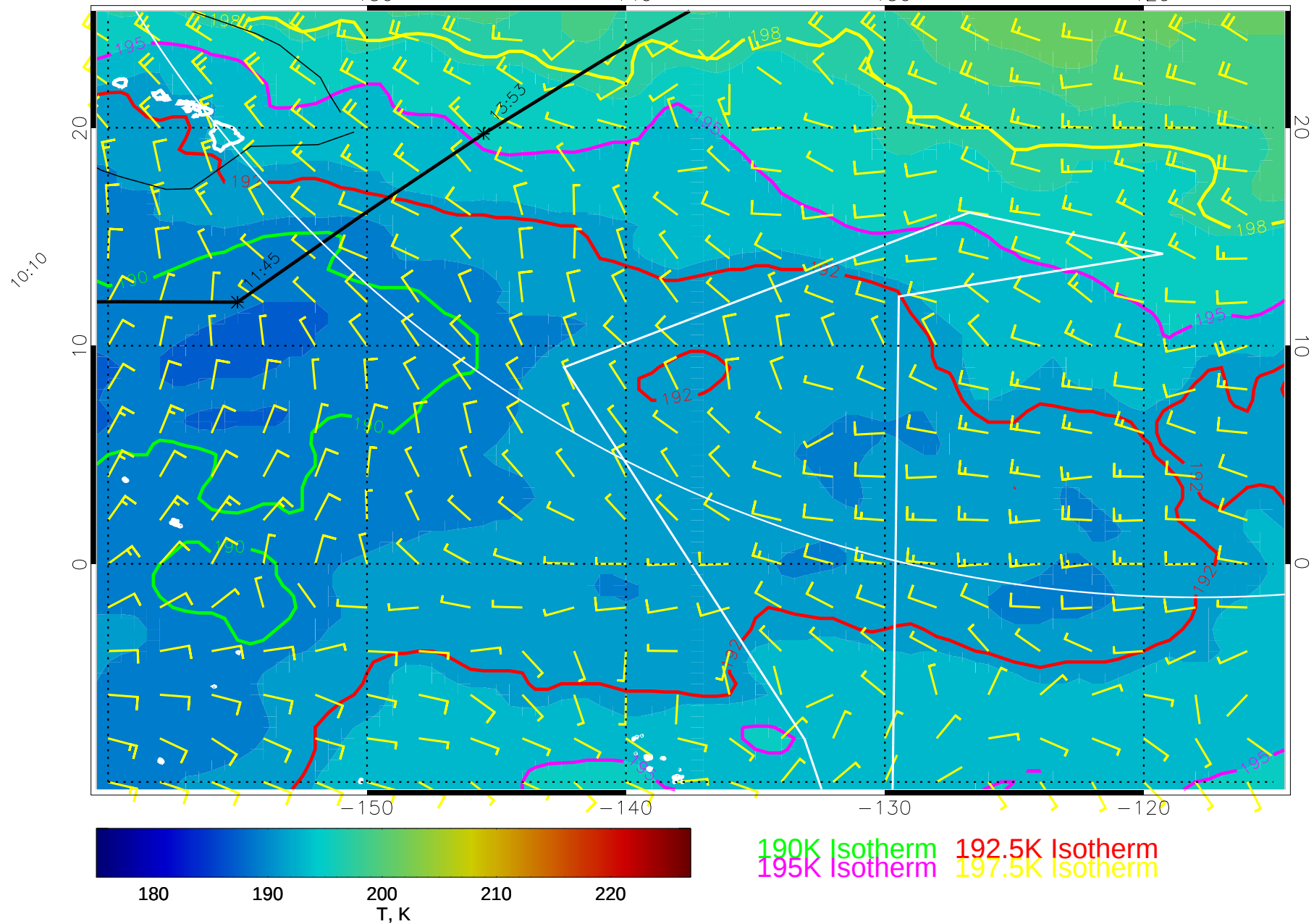
15010912, 12 hour forecast for 70mb T and winds (knots) -- NCEP GFS
