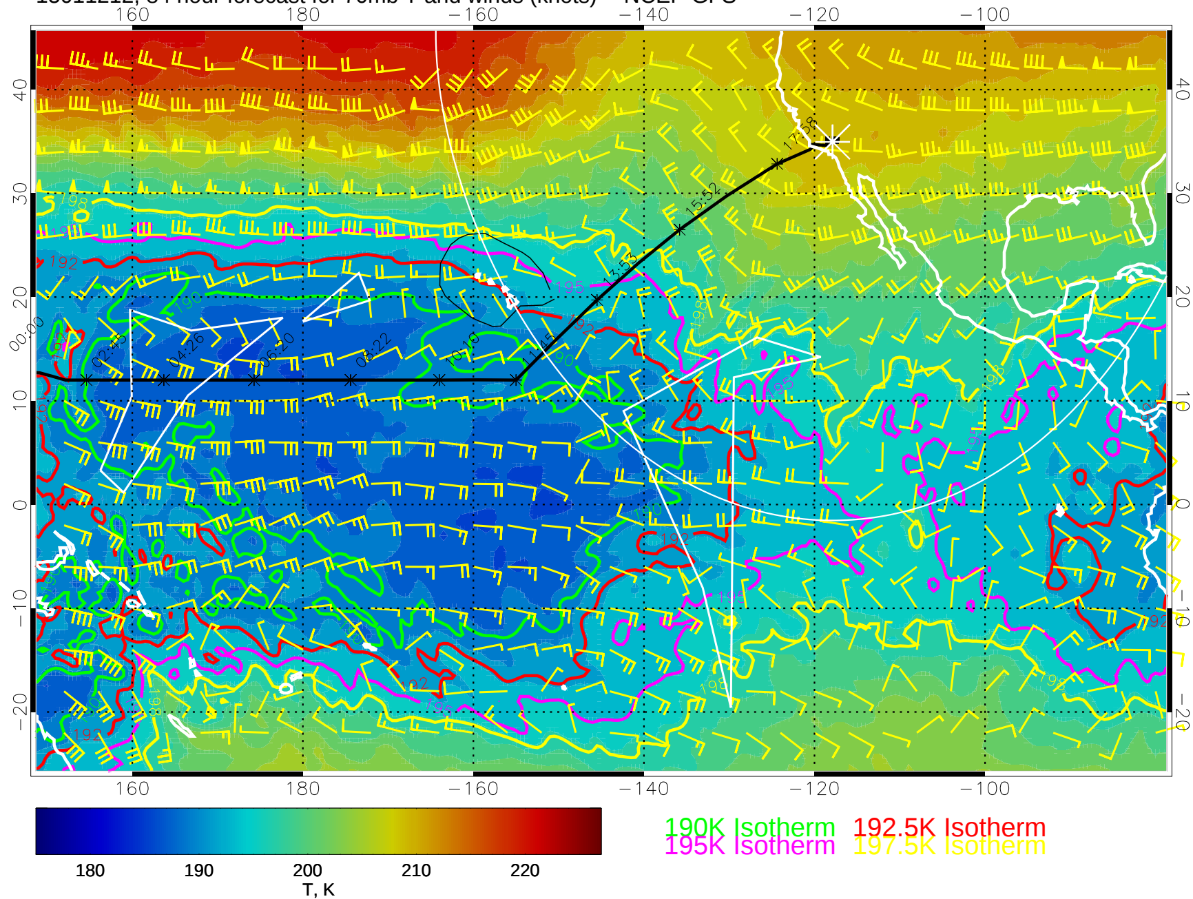
15011212, 84 hour forecast for 70mb T and winds (knots) -- NCEP GFS
