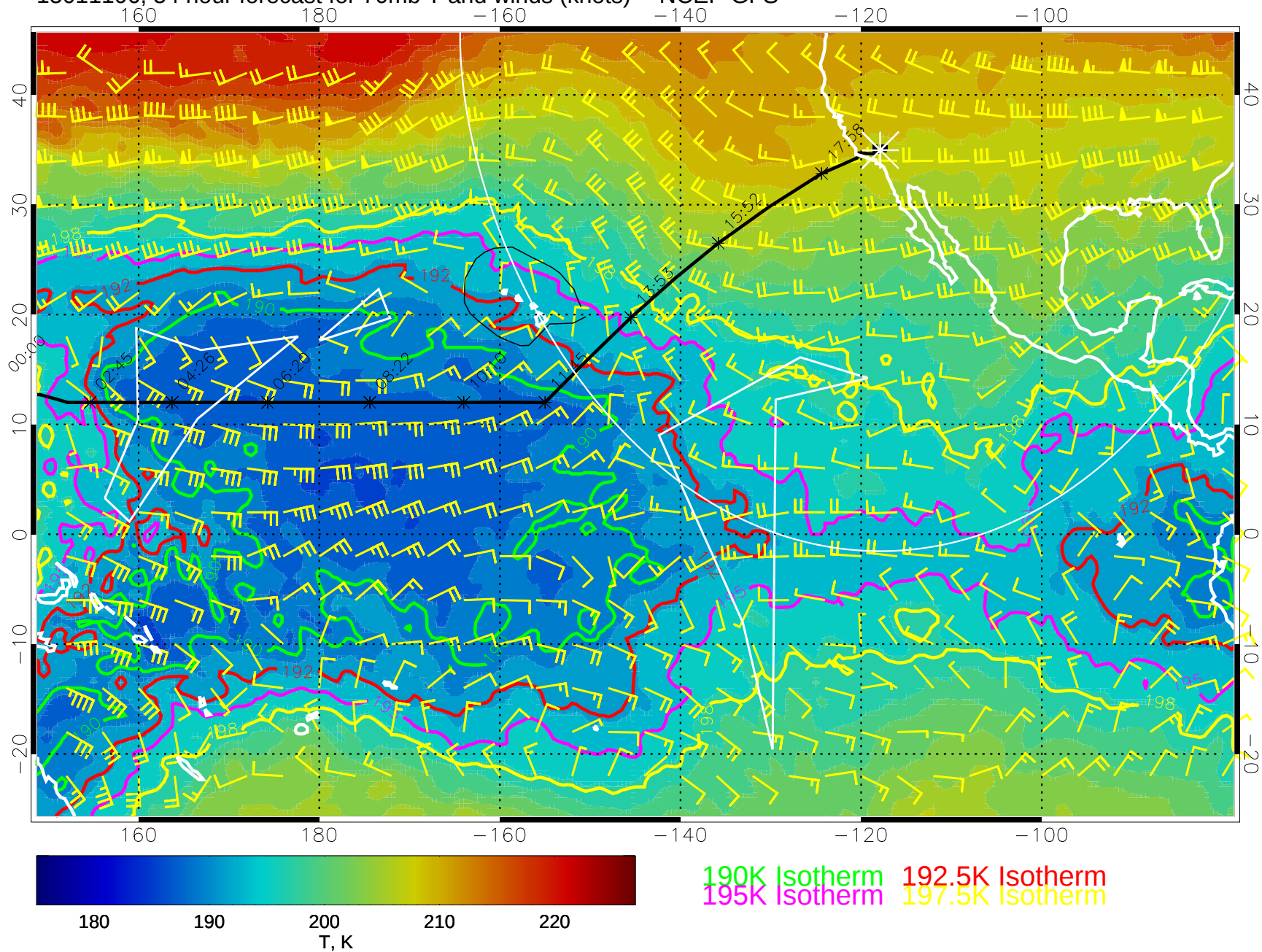
15011106, 54 hour forecast for 70mb T and winds (knots) -- NCEP GFS
