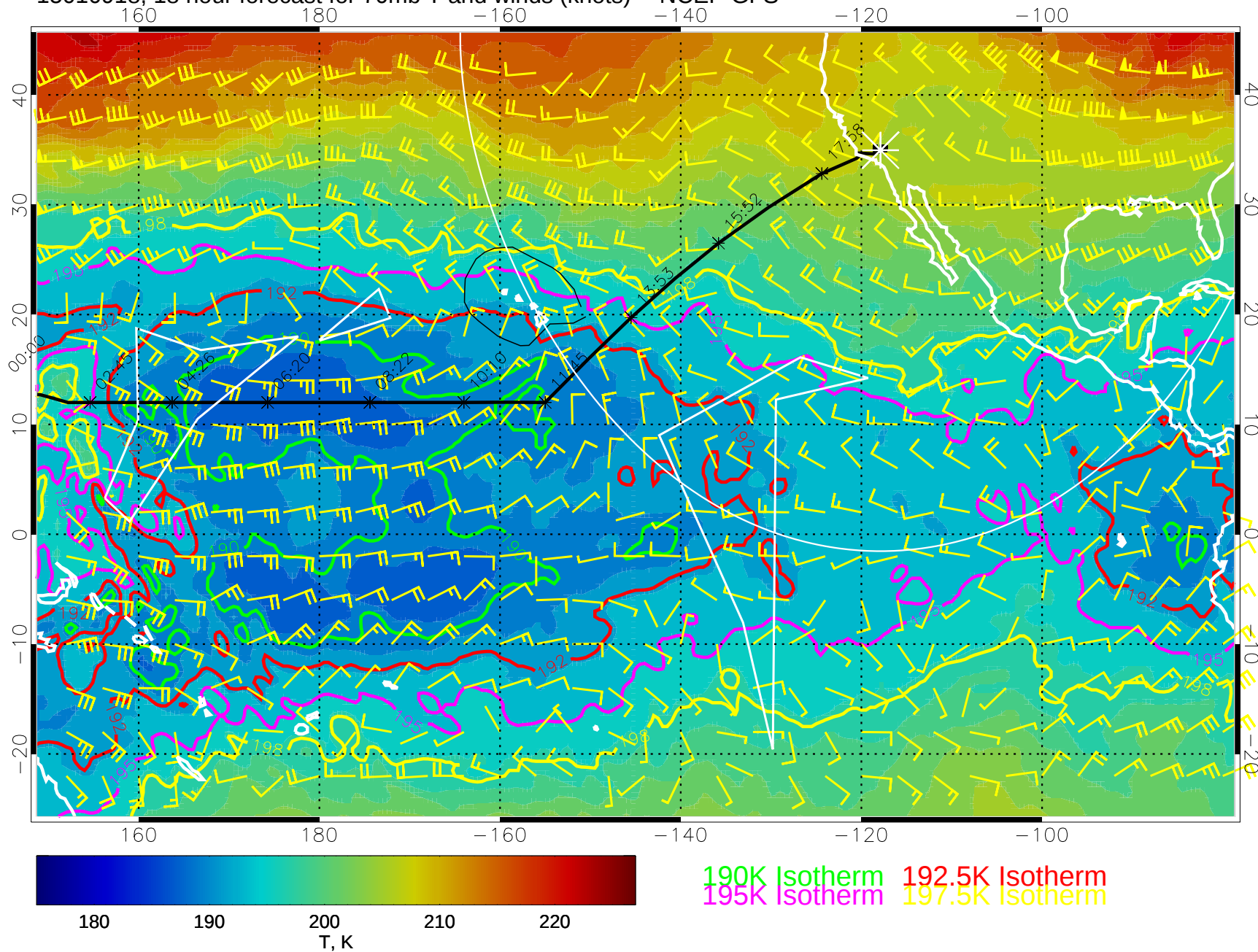
15010918, 18 hour forecast for 70mb T and winds (knots) -- NCEP GFS
