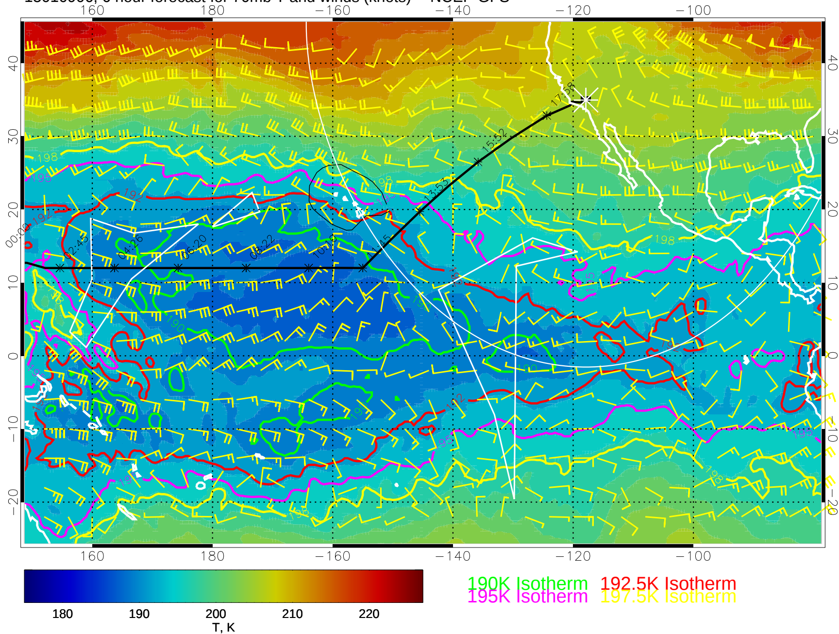
15010906, 6 hour forecast for 70mb T and winds (knots) -- NCEP GFS
