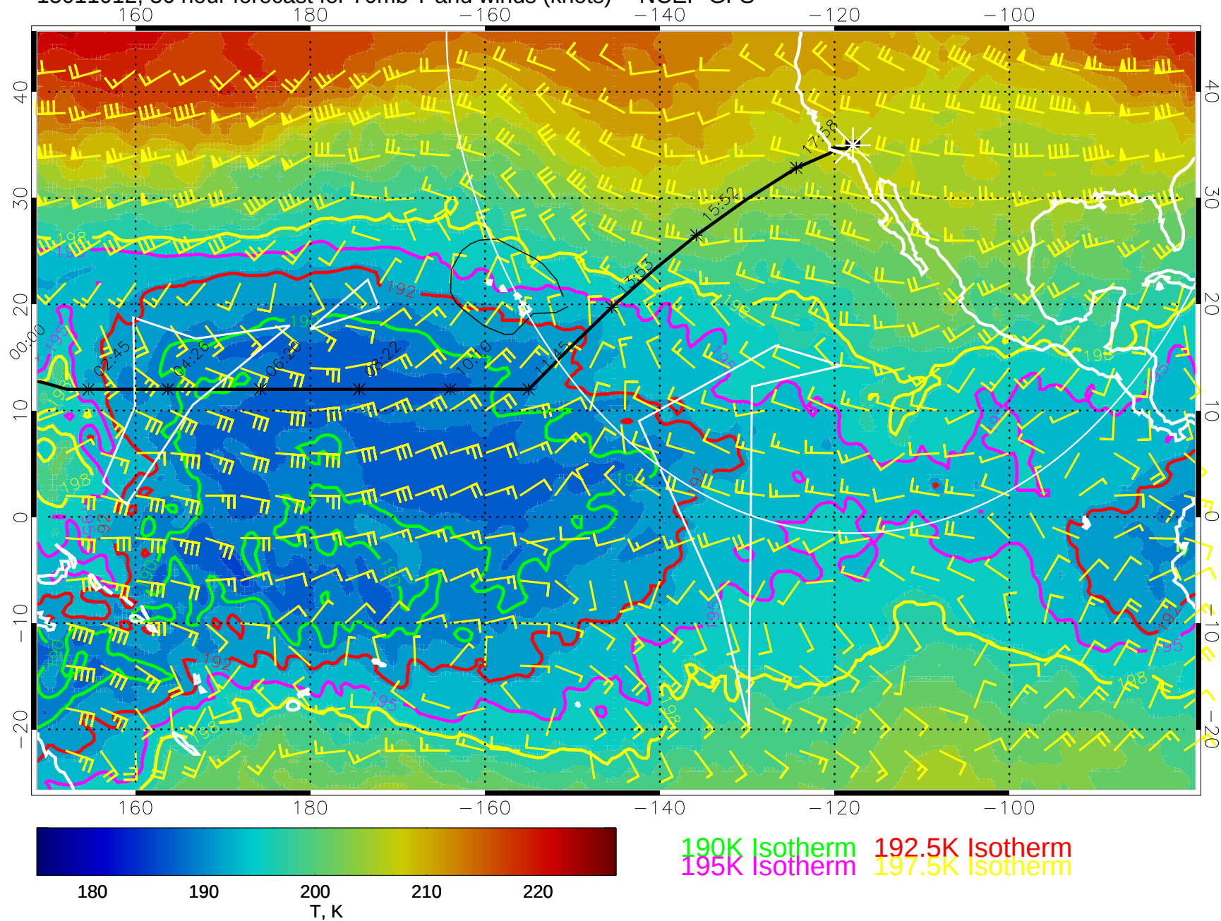
15011012, 36 hour forecast for 70mb T and winds (knots) -- NCEP GFS
