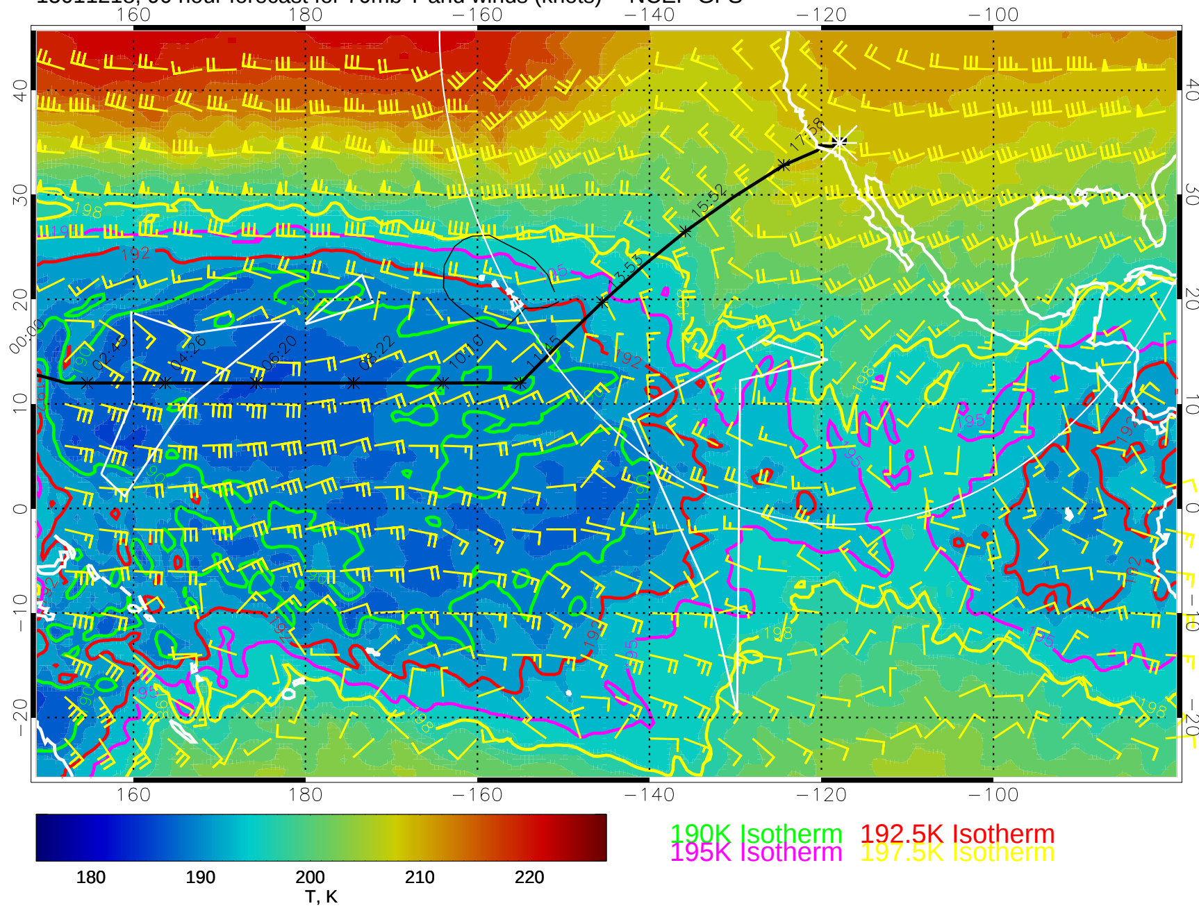
15011218, 90 hour forecast for 70mb T and winds (knots) -- NCEP GFS
