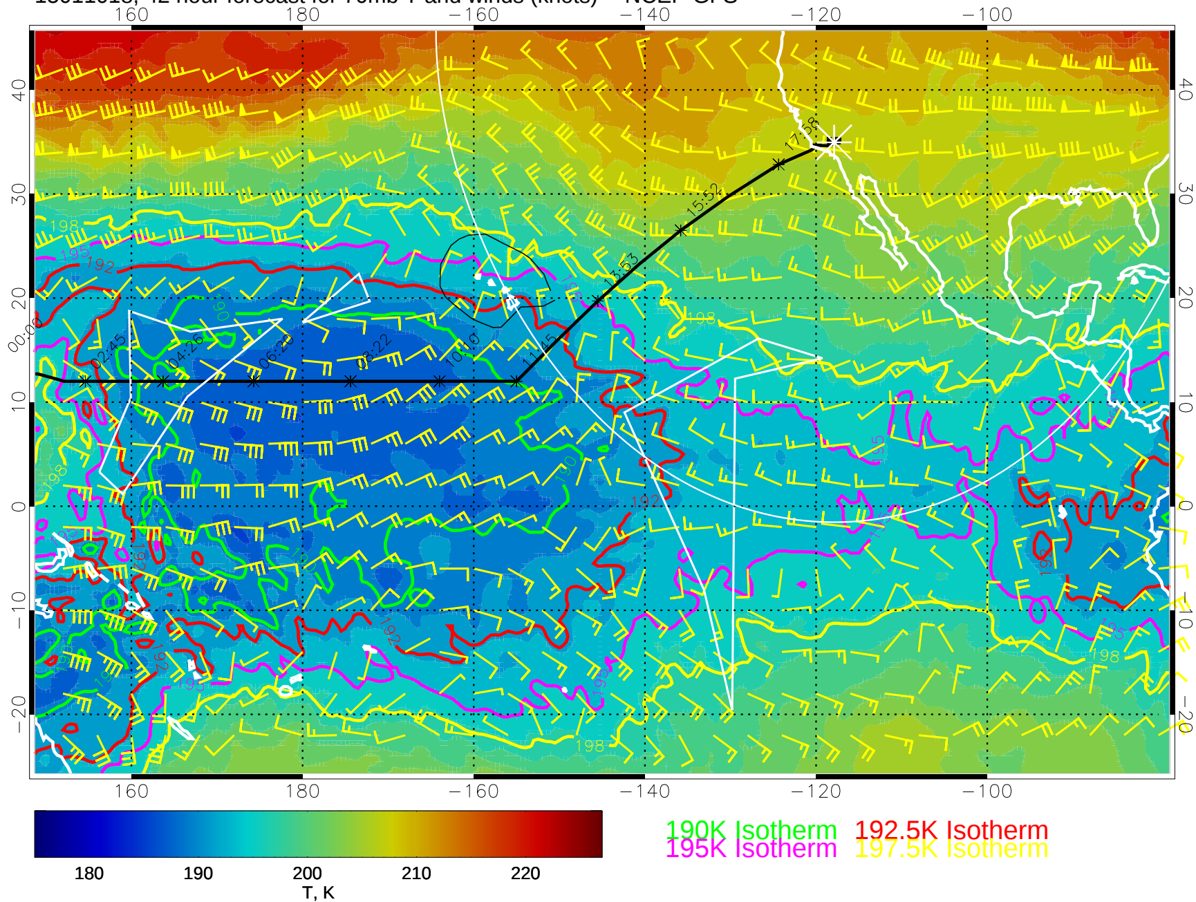
15011018, 42 hour forecast for 70mb T and winds (knots) -- NCEP GFS
