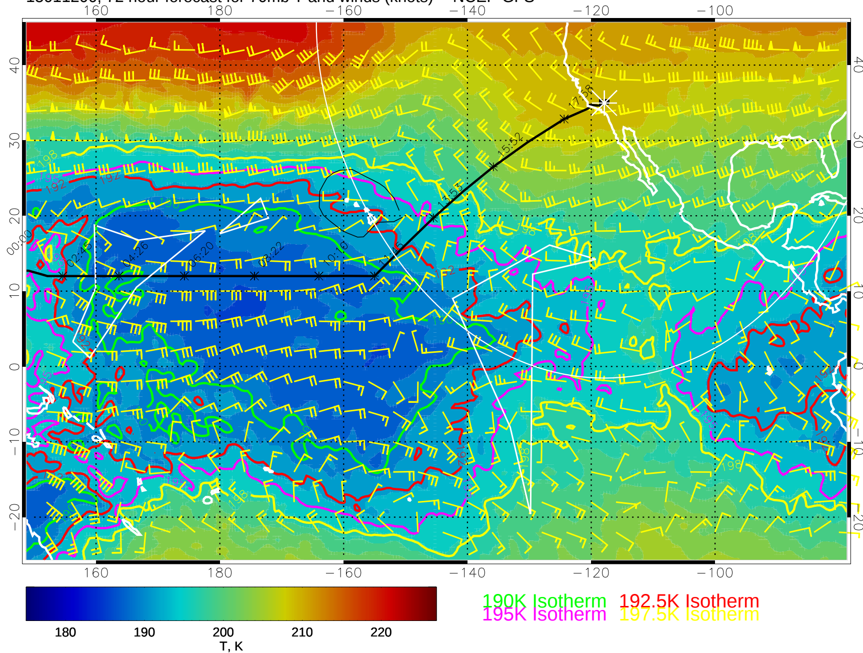
15011200, 72 hour forecast for 70mb T and winds (knots) -- NCEP GFS
