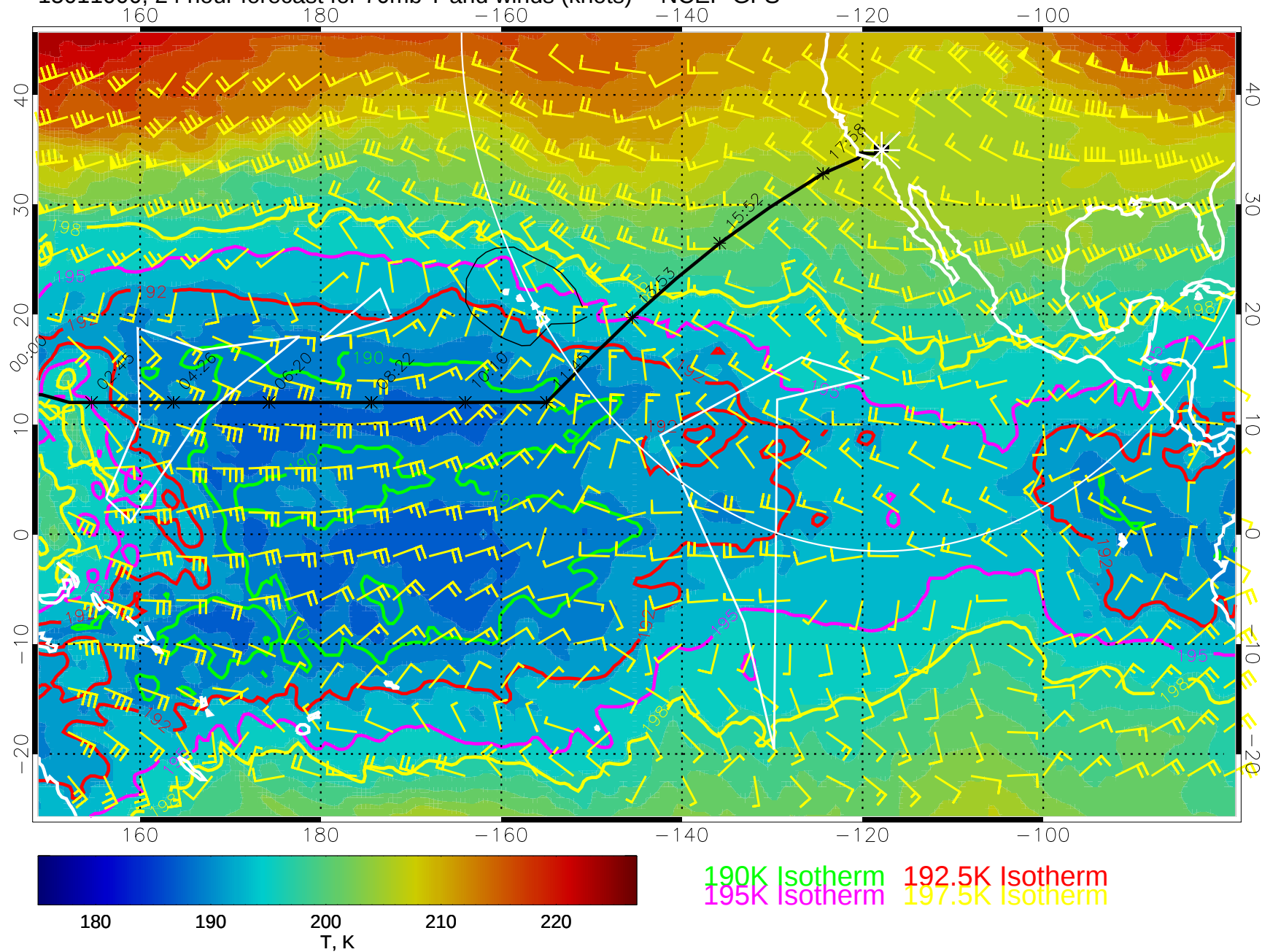
15011000, 24 hour forecast for 70mb T and winds (knots) -- NCEP GFS
