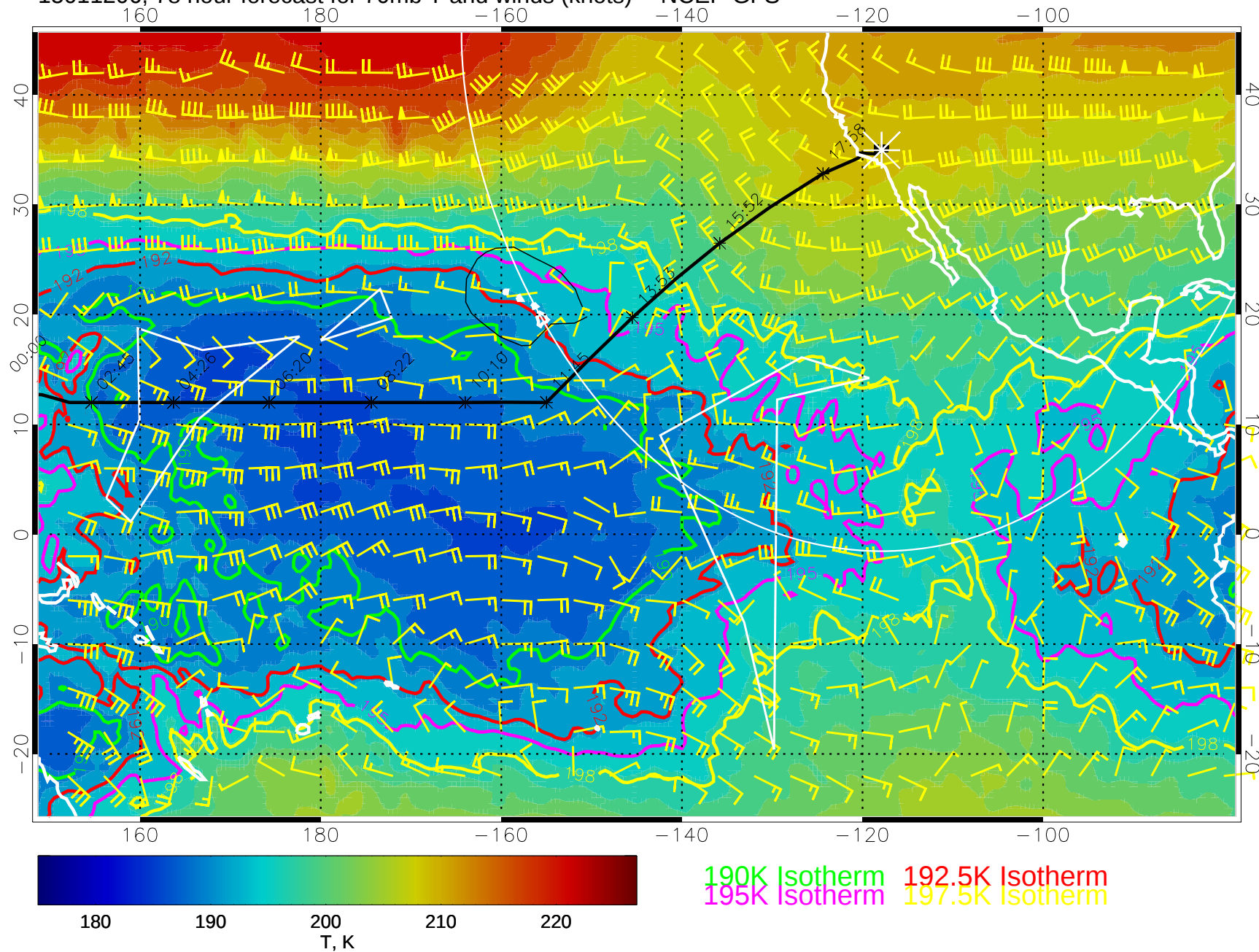
15011206, 78 hour forecast for 70mb T and winds (knots) -- NCEP GFS
