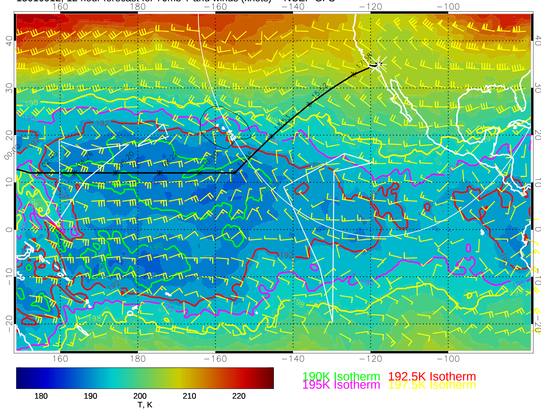
15010912, 12 hour forecast for 70mb T and winds (knots) -- NCEP GFS
