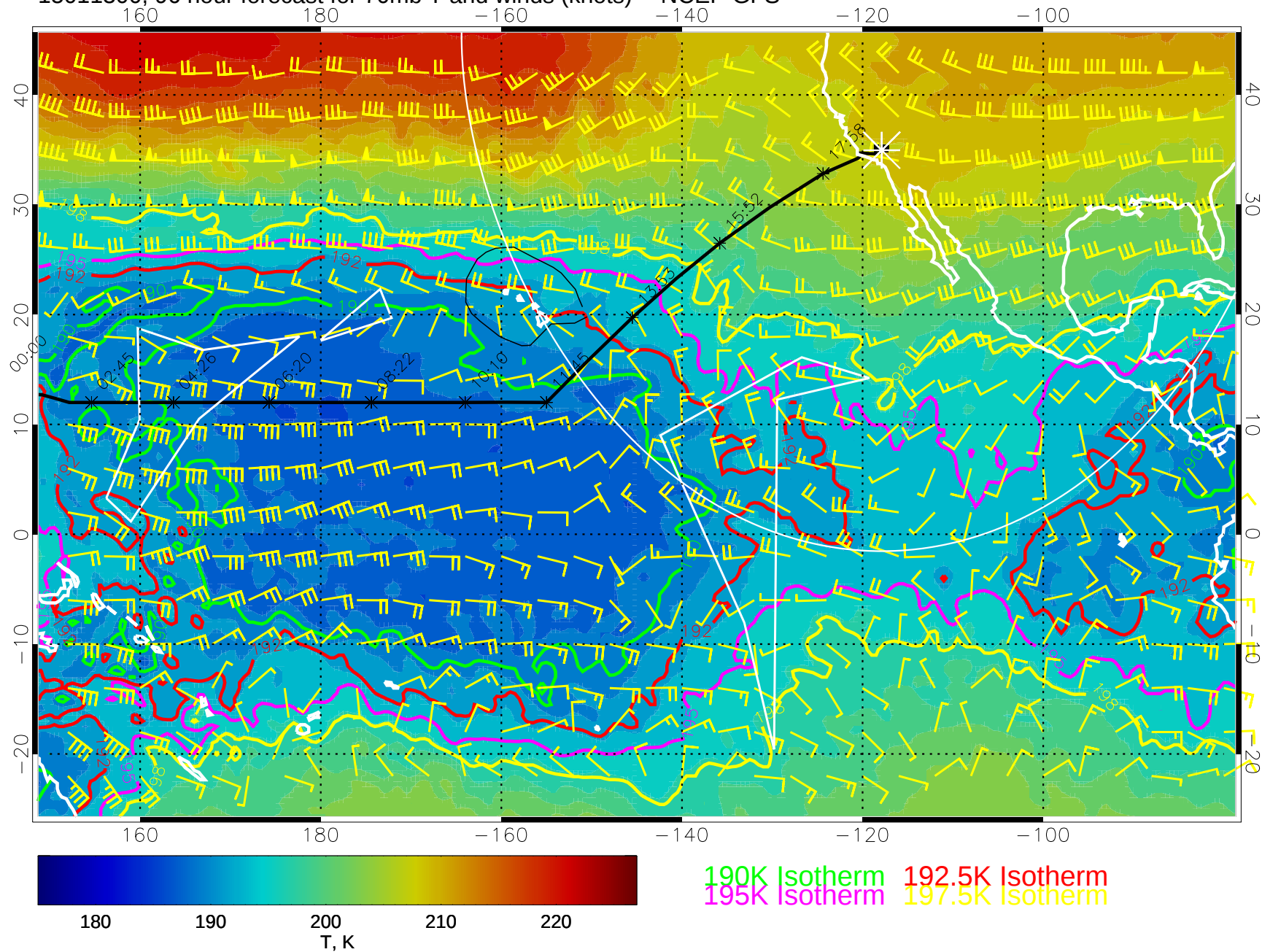
15011300, 96 hour forecast for 70mb T and winds (knots) -- NCEP GFS
