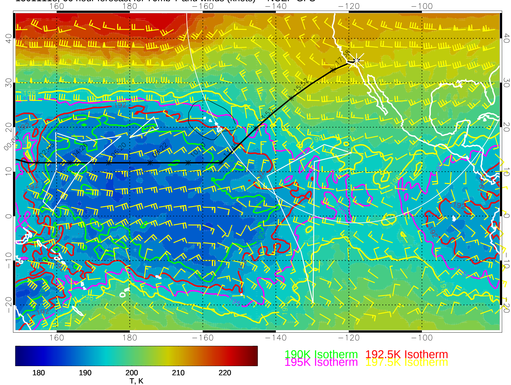
15011118, 66 hour forecast for 70mb T and winds (knots) -- NCEP GFS
