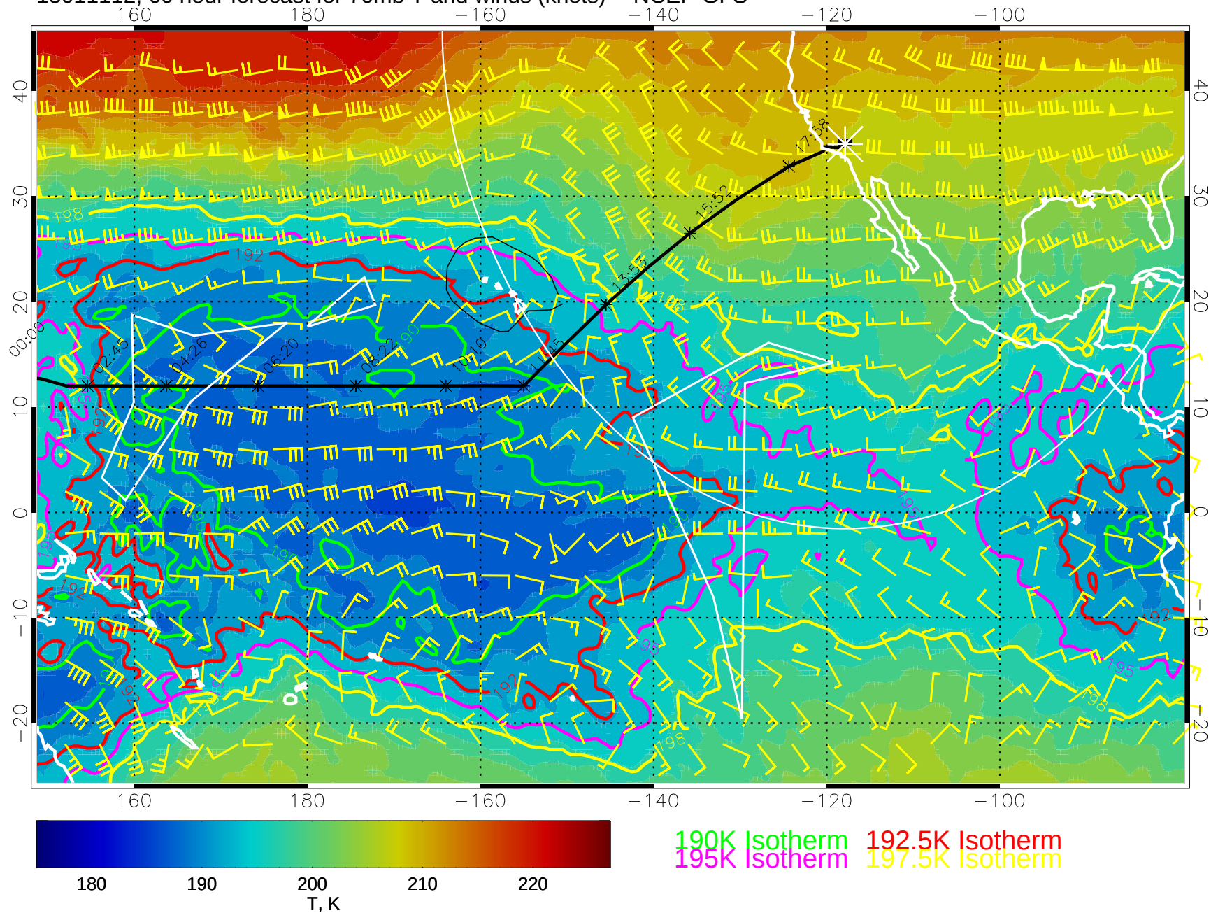
15011112, 60 hour forecast for 70mb T and winds (knots) -- NCEP GFS
