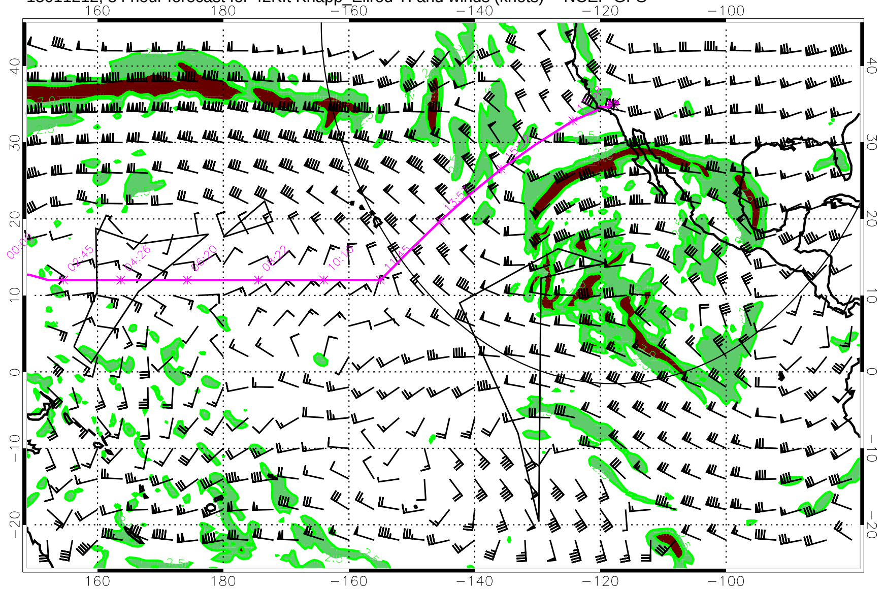
15011212, 84 hour forecast for 42Kft Knapp_Ellrod TI and winds (knots) -- NCEP GFS
