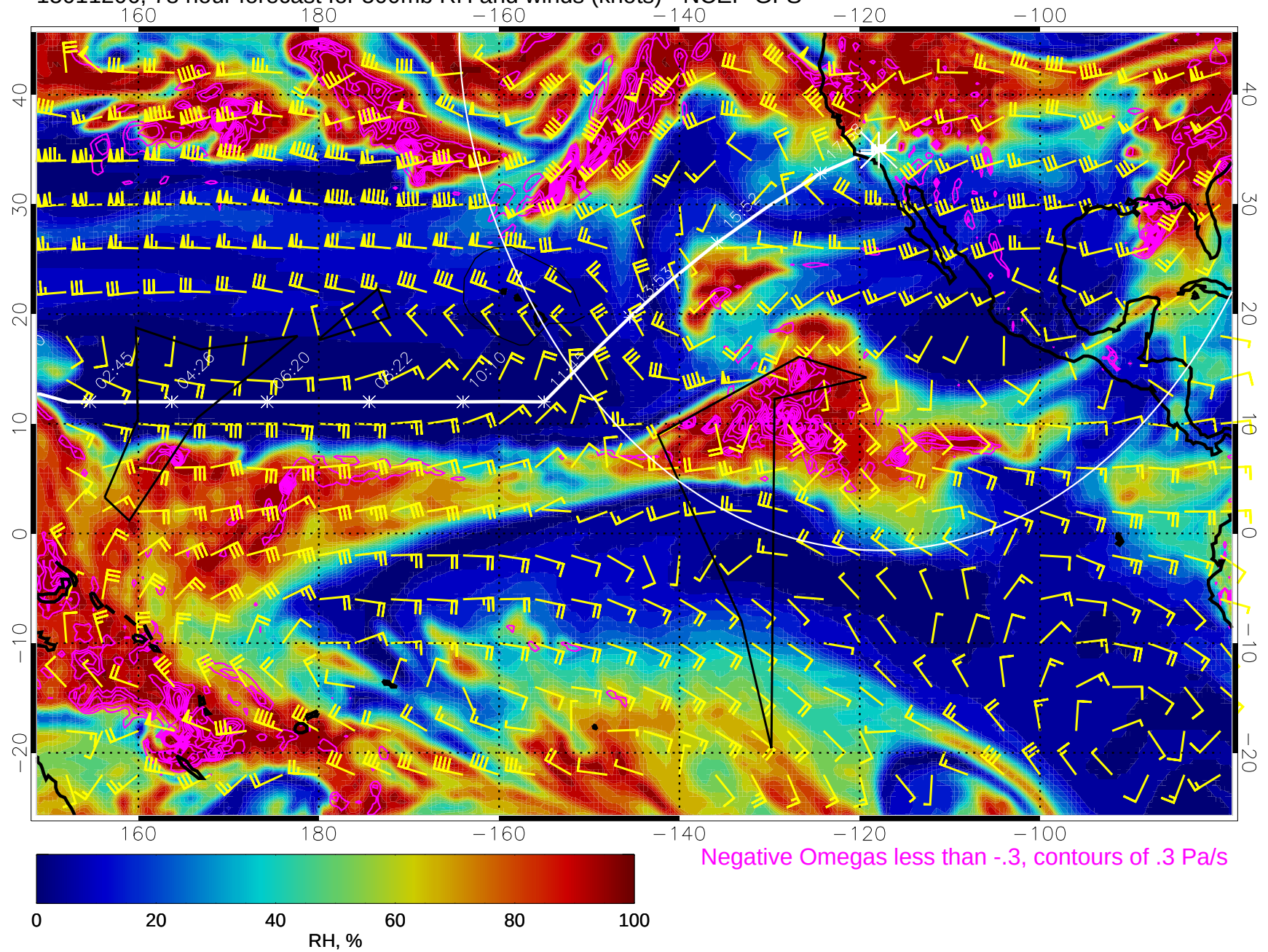
15011206, 78 hour forecast for 500mb RH and winds (knots) - NCEP GFS
