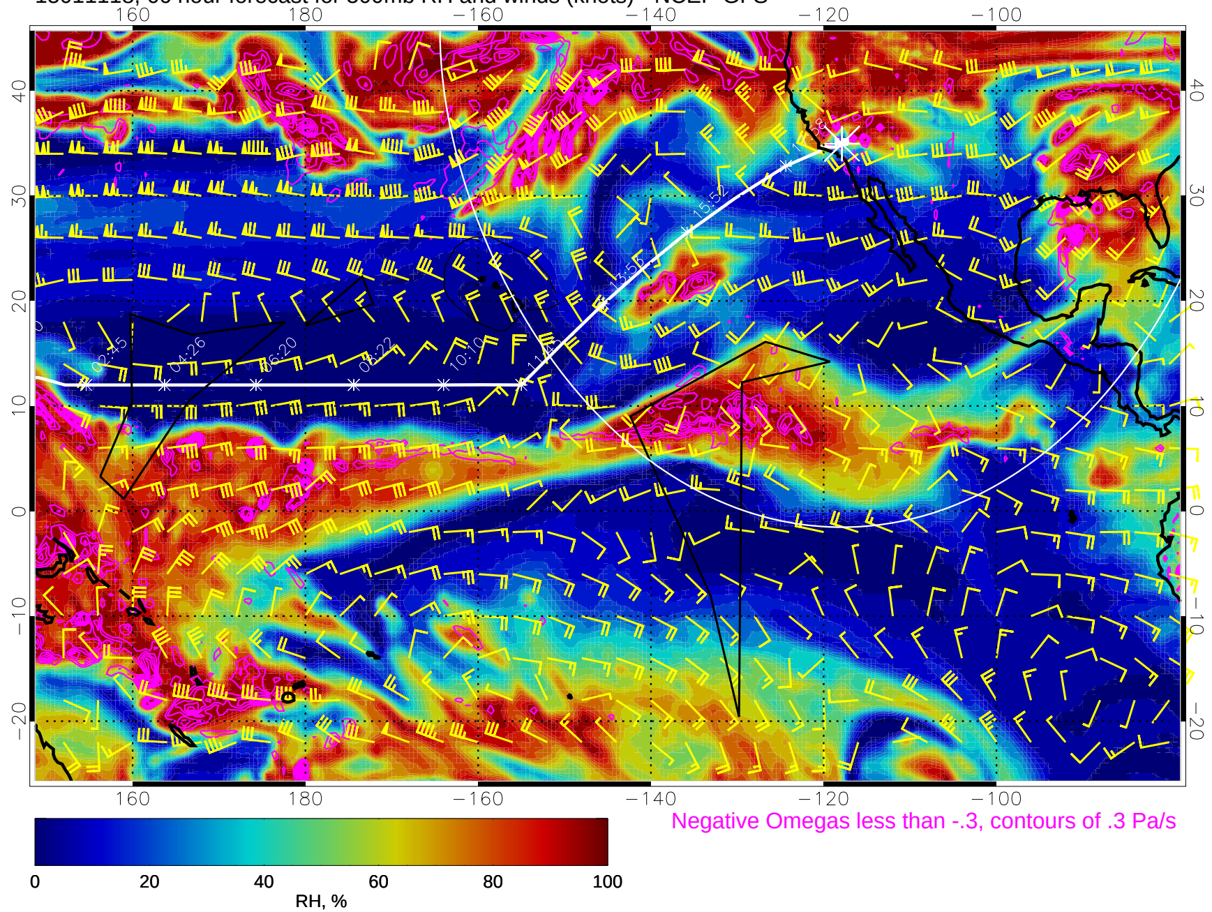
15011118, 66 hour forecast for 500mb RH and winds (knots) - NCEP GFS
