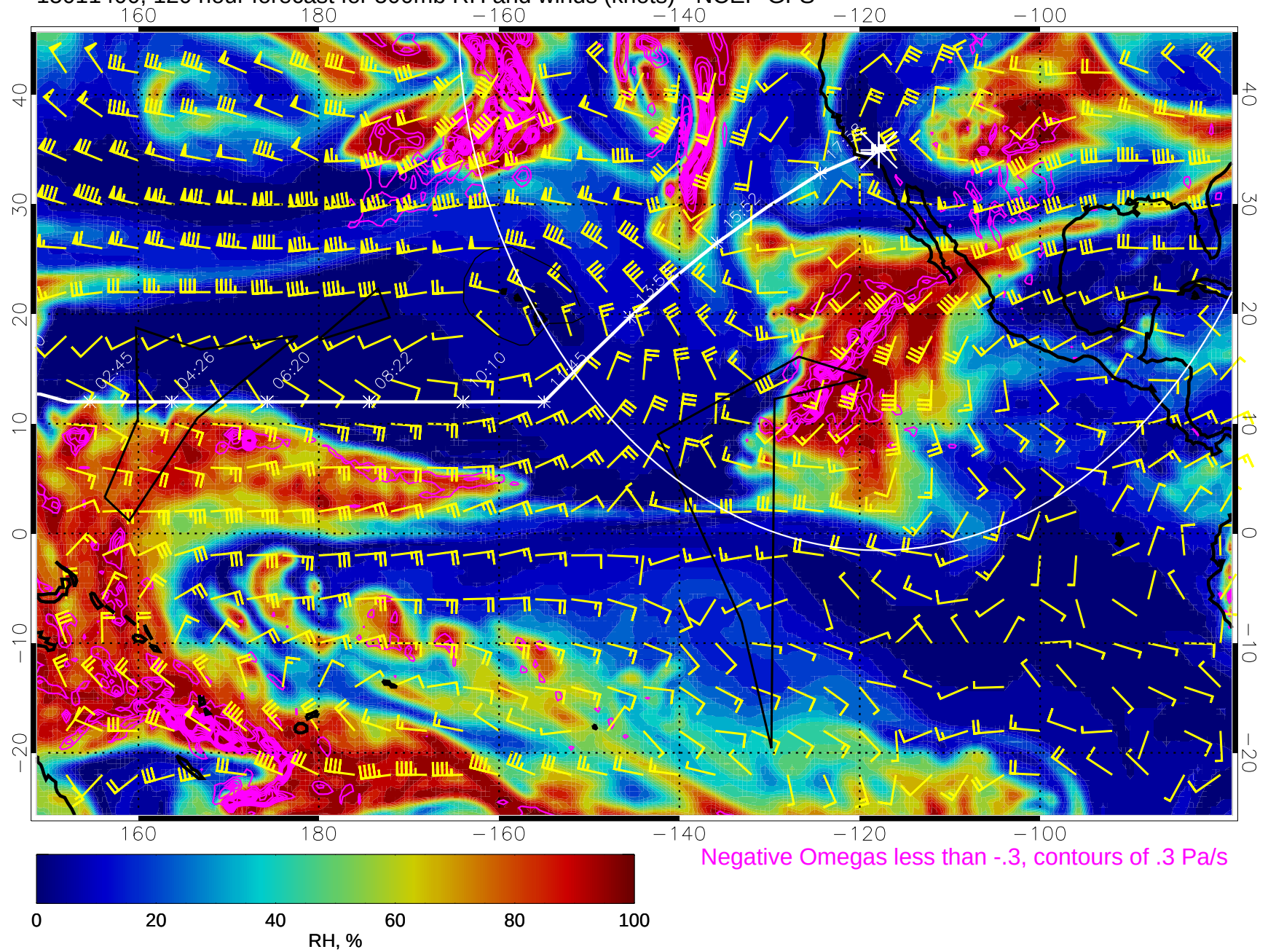
15011400, 120 hour forecast for 500mb RH and winds (knots) - NCEP GFS
