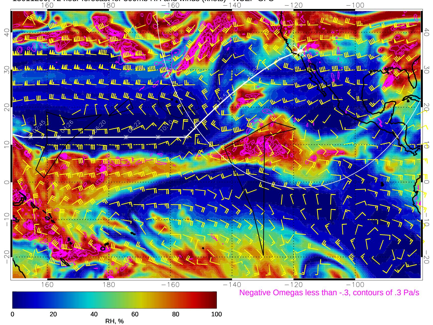
15011200, 72 hour forecast for 500mb RH and winds (knots) - NCEP GFS
