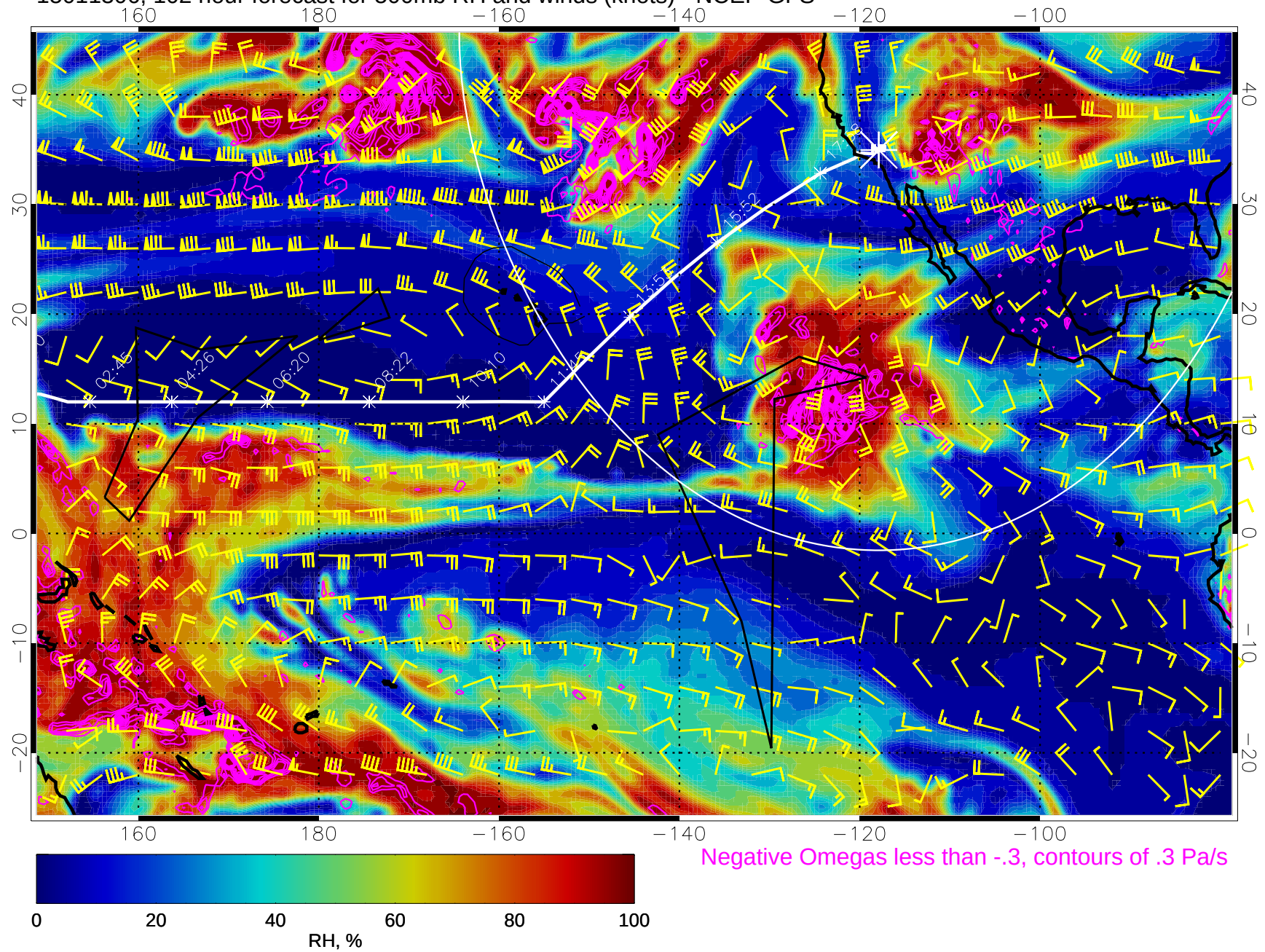
15011306, 102 hour forecast for 500mb RH and winds (knots) - NCEP GFS
