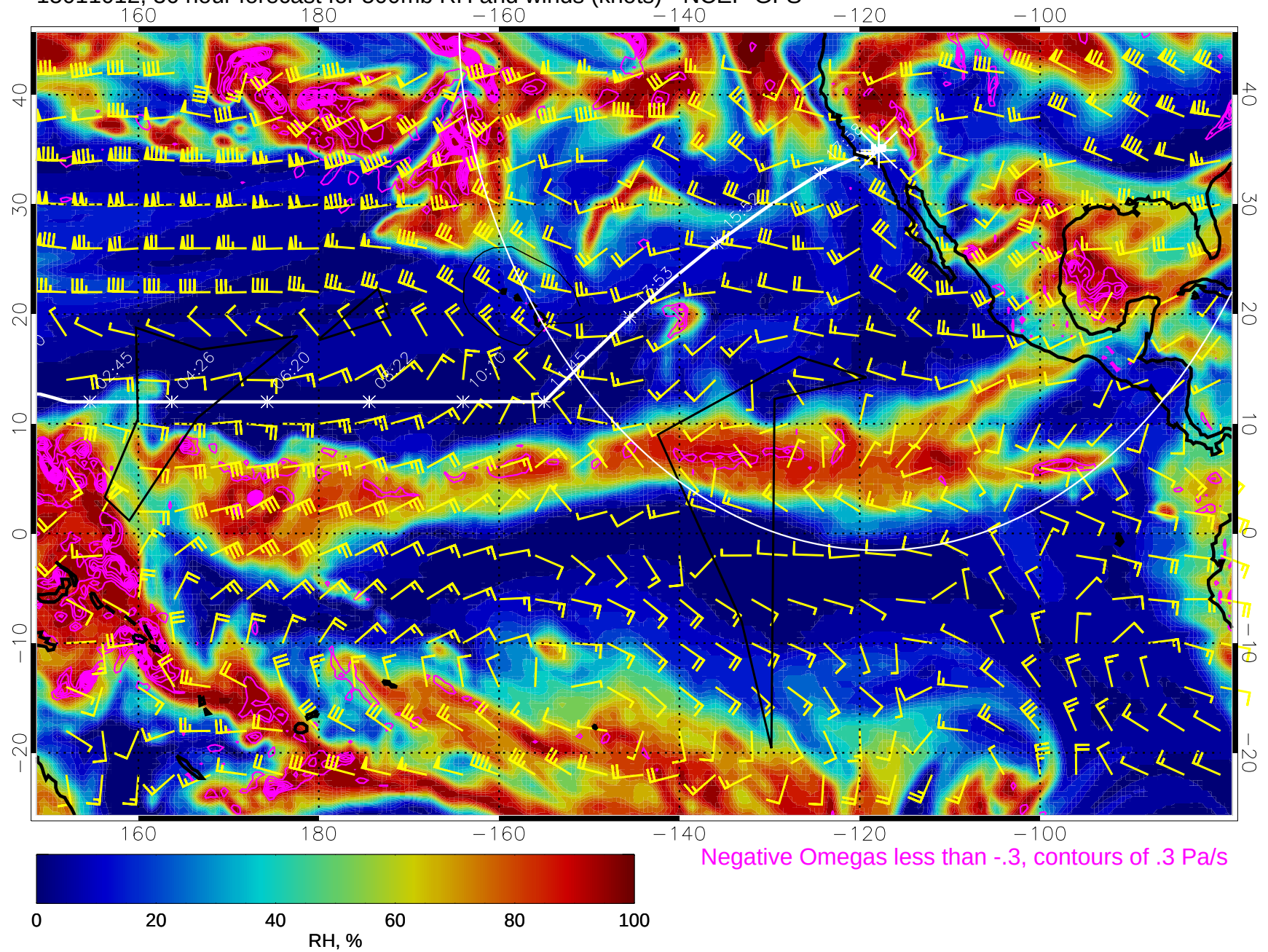
15011012, 36 hour forecast for 500mb RH and winds (knots) - NCEP GFS
