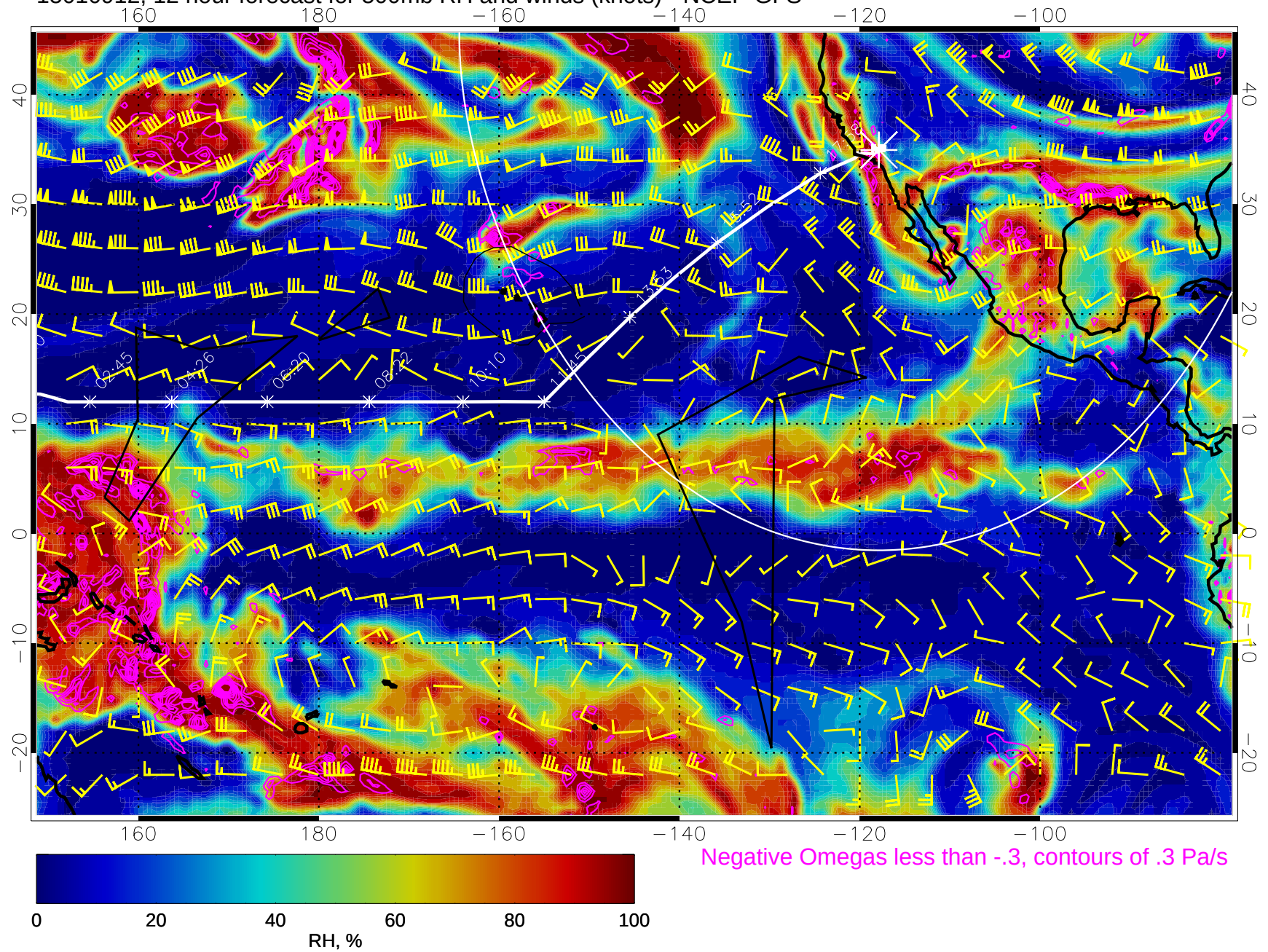
15010912, 12 hour forecast for 500mb RH and winds (knots) - NCEP GFS
