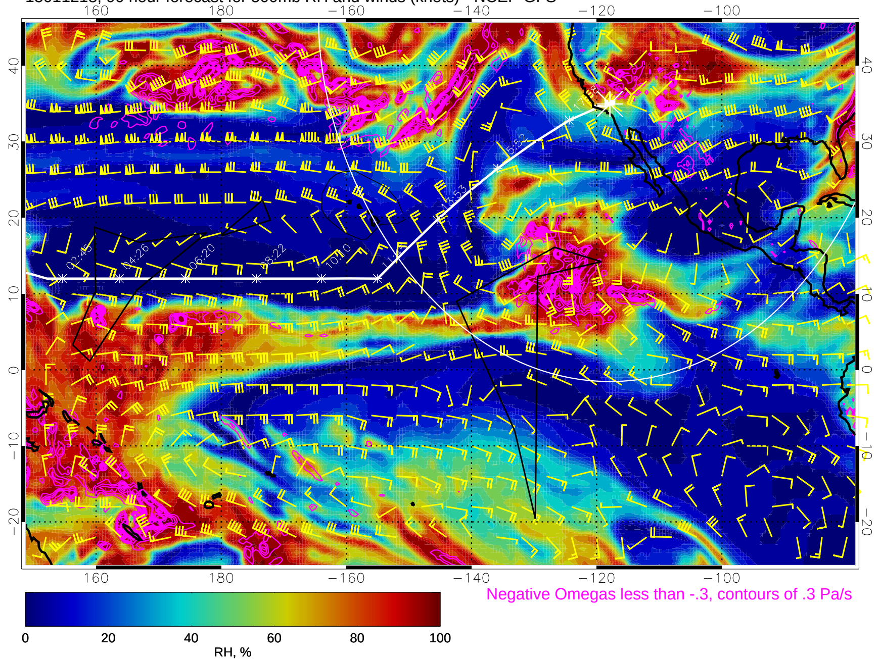
15011218, 90 hour forecast for 500mb RH and winds (knots) - NCEP GFS
