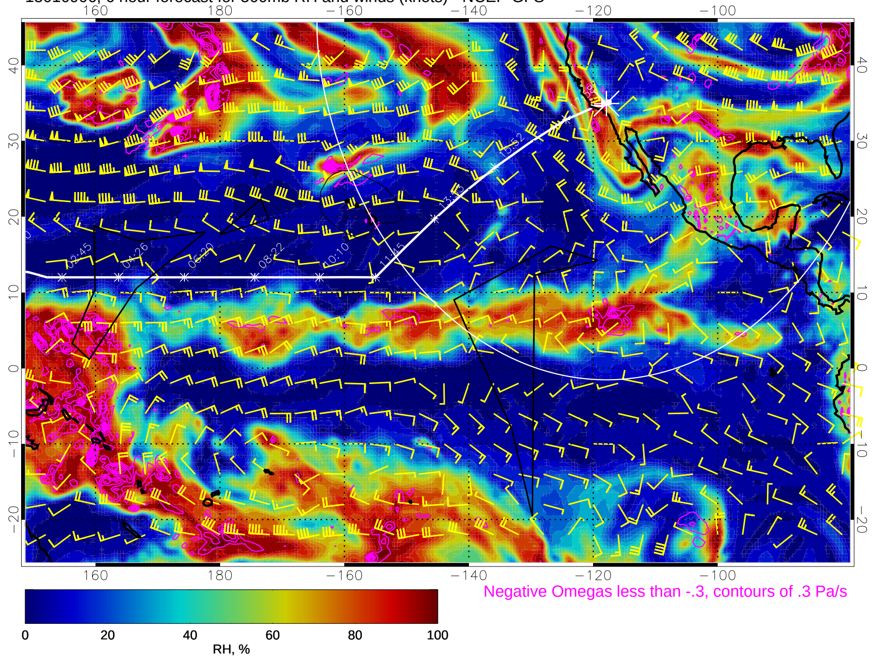
15010906, 6 hour forecast for 500mb RH and winds (knots) - NCEP GFS
