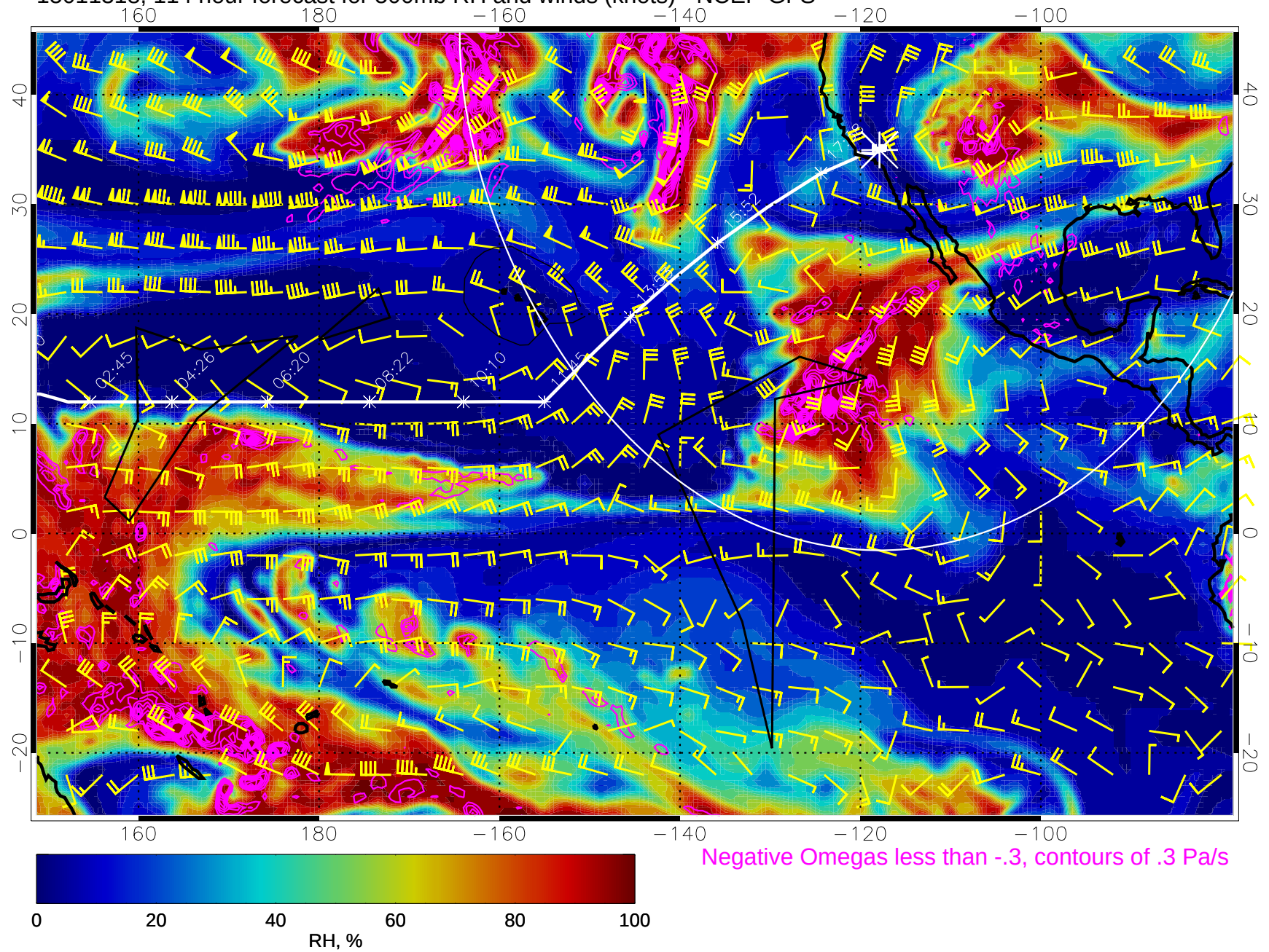
15011318, 114 hour forecast for 500mb RH and winds (knots) - NCEP GFS
