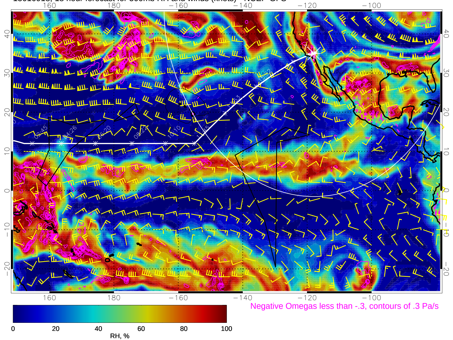
15010918, 18 hour forecast for 500mb RH and winds (knots) - NCEP GFS
