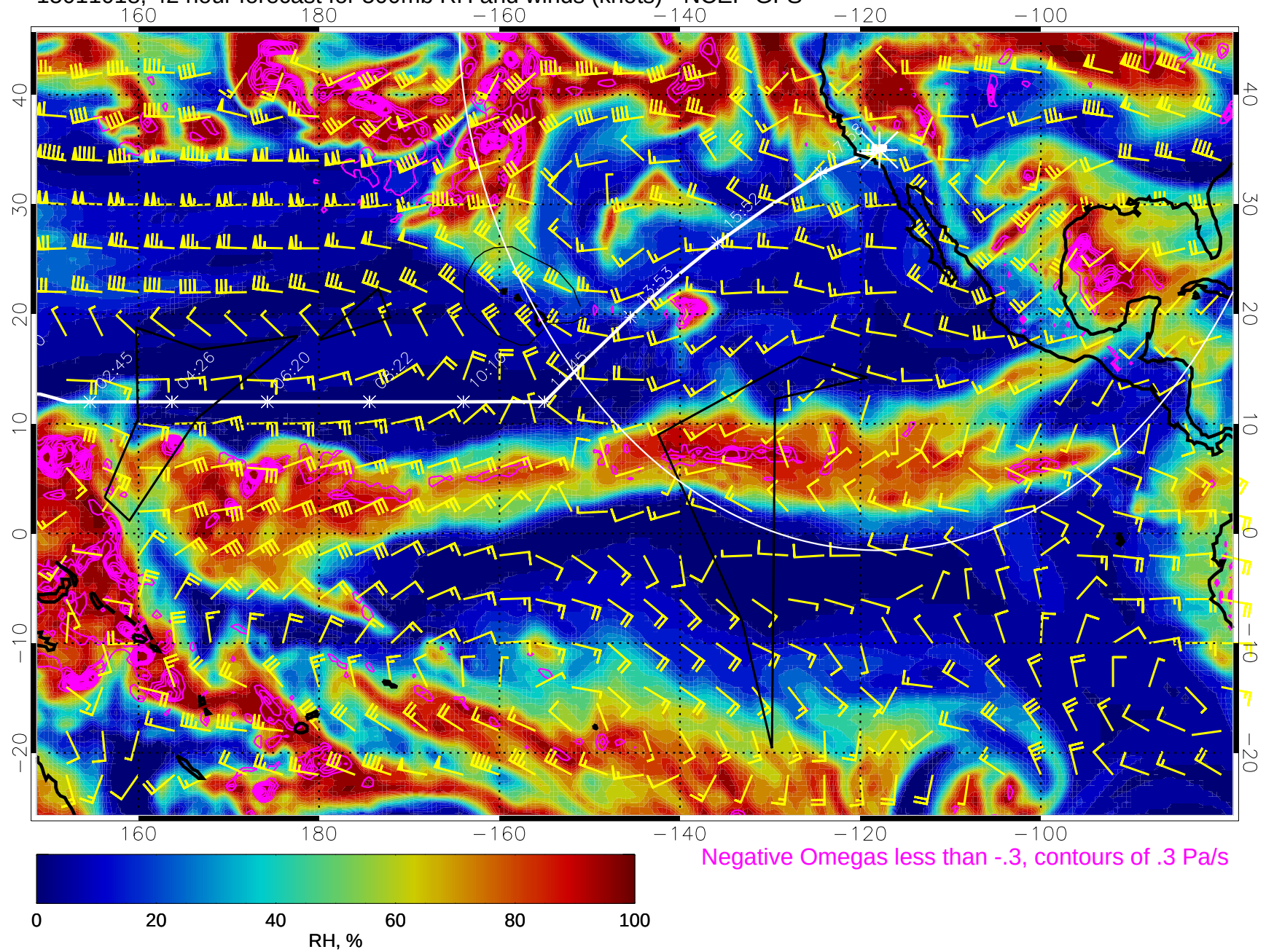
15011018, 42 hour forecast for 500mb RH and winds (knots) - NCEP GFS
