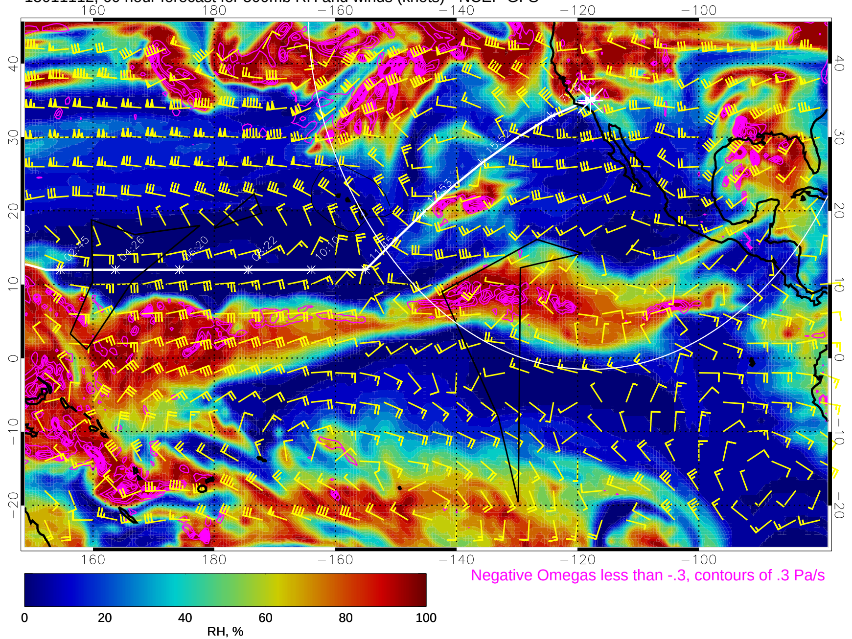
15011112, 60 hour forecast for 500mb RH and winds (knots) - NCEP GFS
