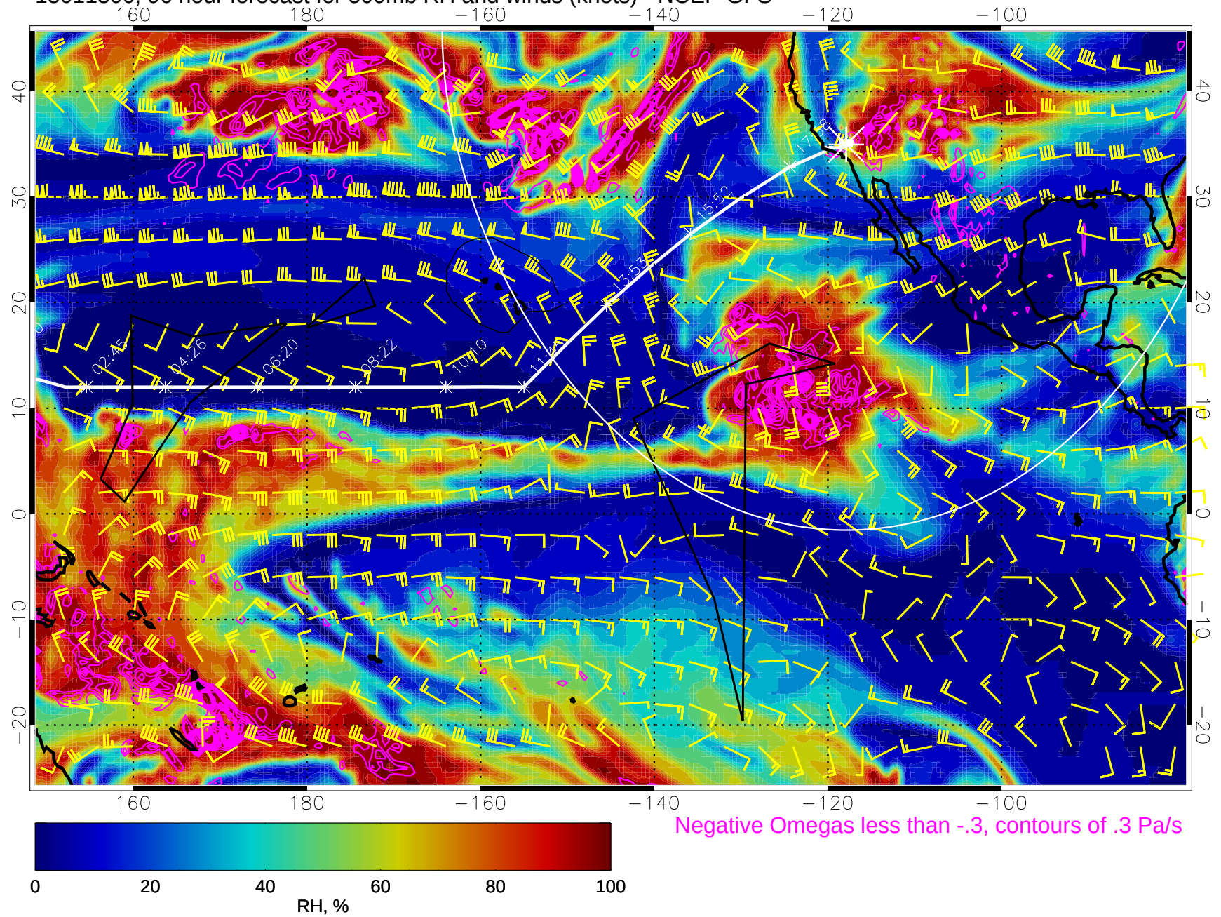
15011300, 96 hour forecast for 500mb RH and winds (knots) - NCEP GFS
