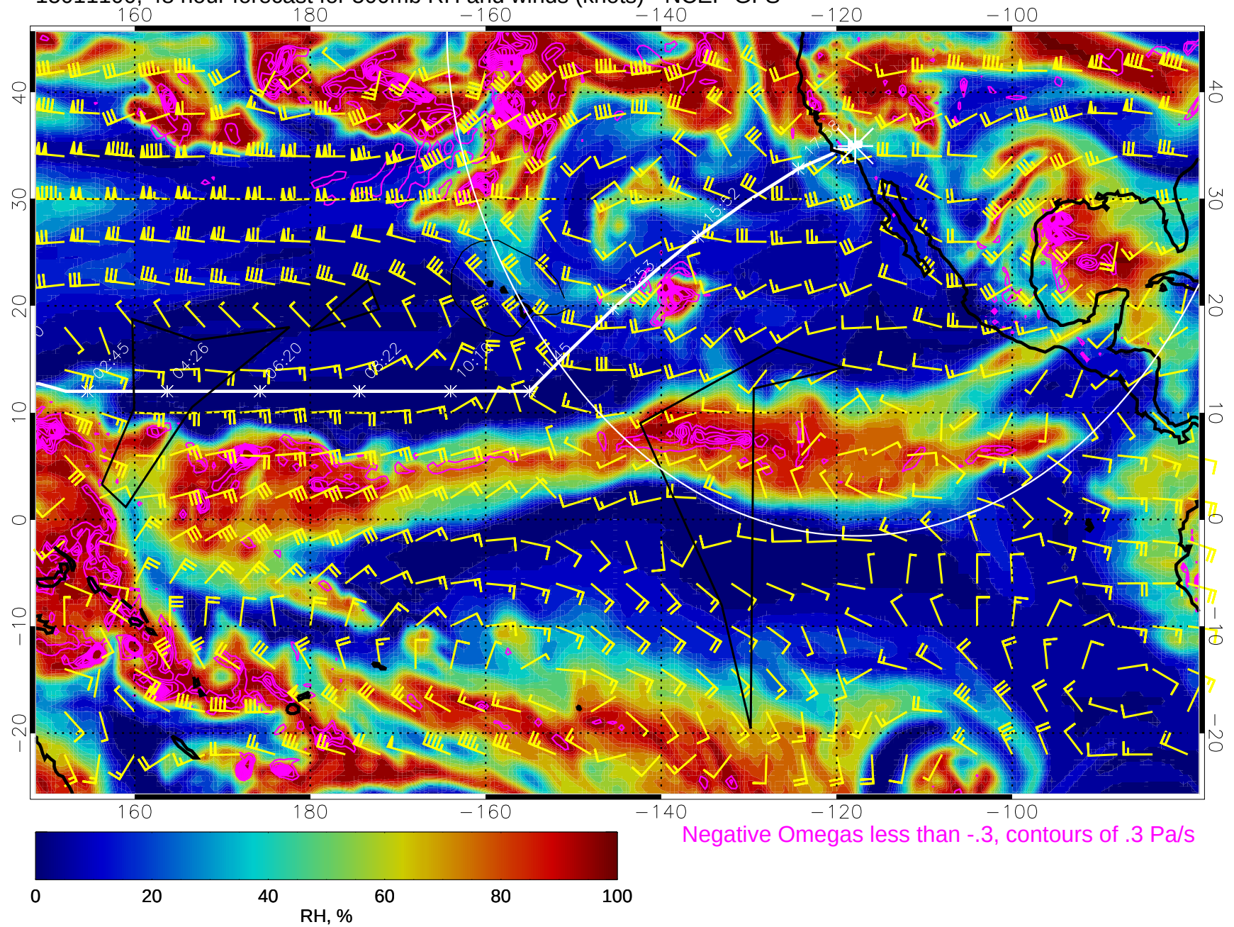
15011100, 48 hour forecast for 500mb RH and winds (knots) - NCEP GFS
