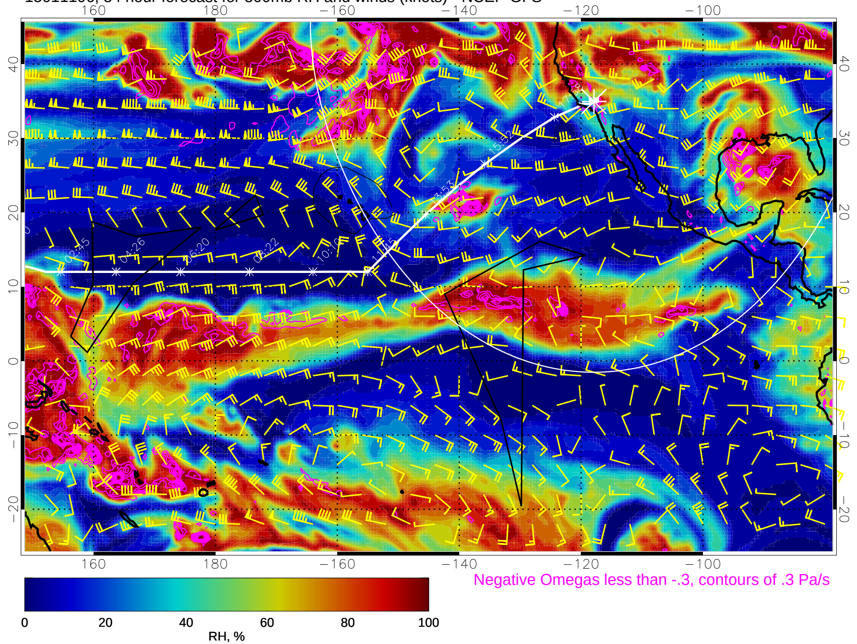
15011106, 54 hour forecast for 500mb RH and winds (knots) - NCEP GFS
