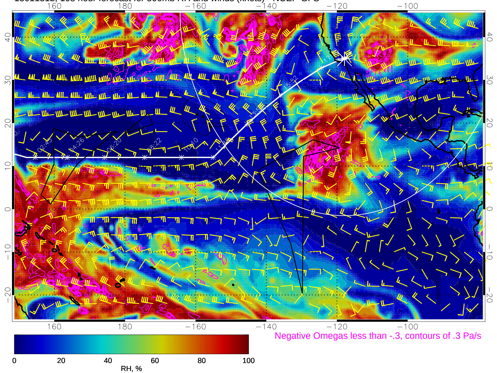
15011312, 108 hour forecast for 500mb RH and winds (knots) - NCEP GFS
