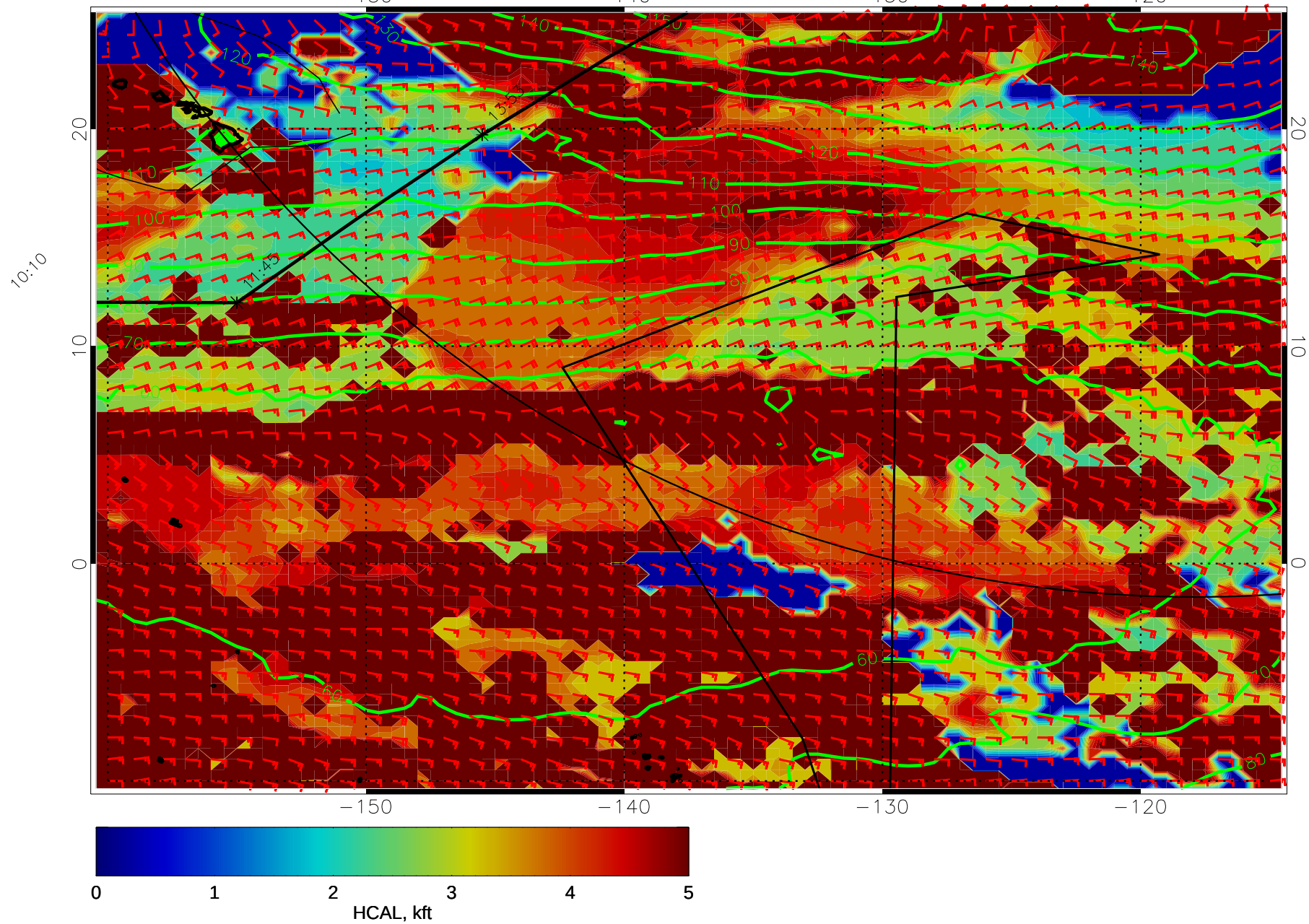
15011112, 60 hour forecast for HCAL, 1000mb Z, and winds (knots) -- NCEP GFS
