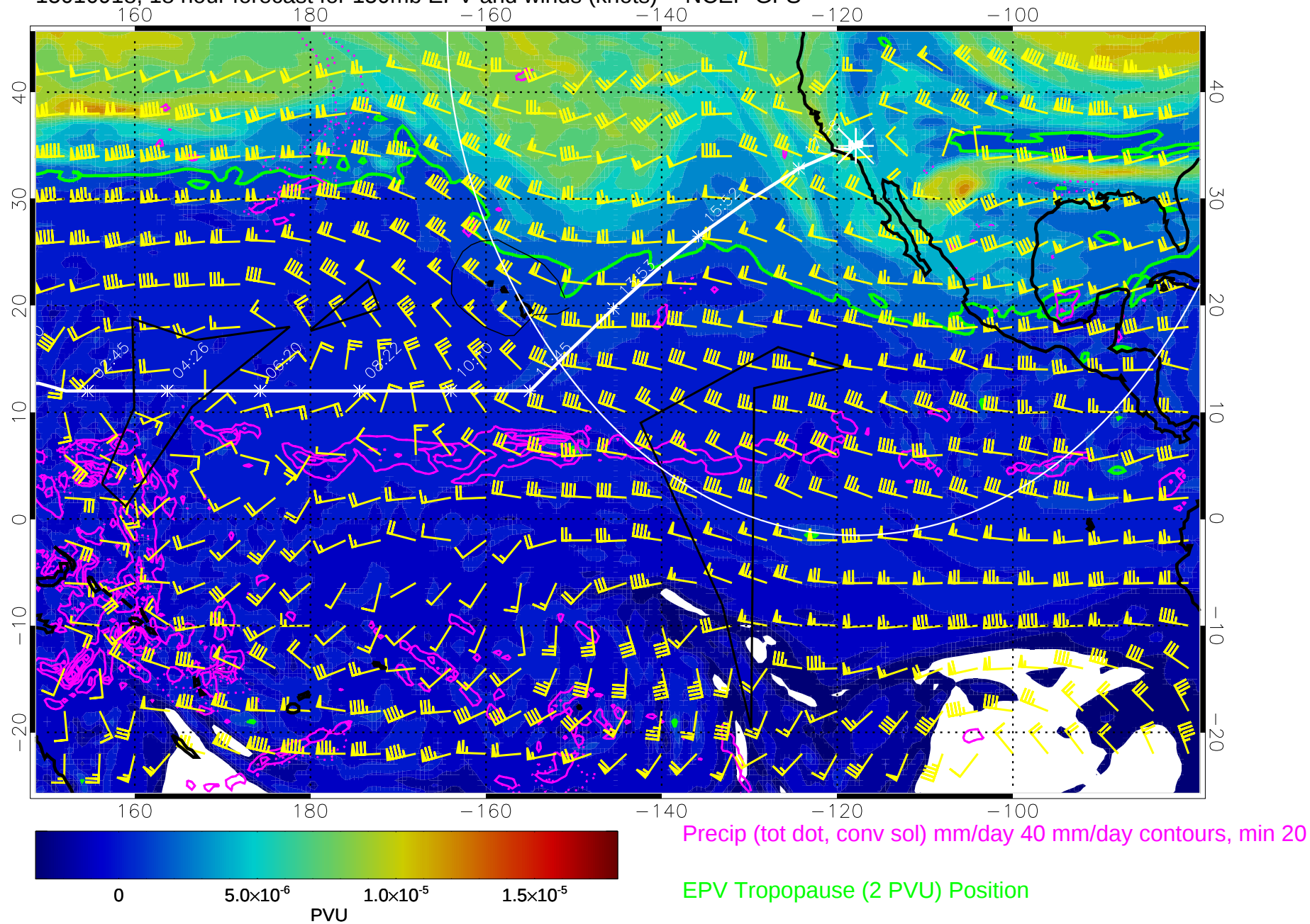
15010918, 18 hour forecast for 150mb EPV and winds (knots) -- NCEP GFS
