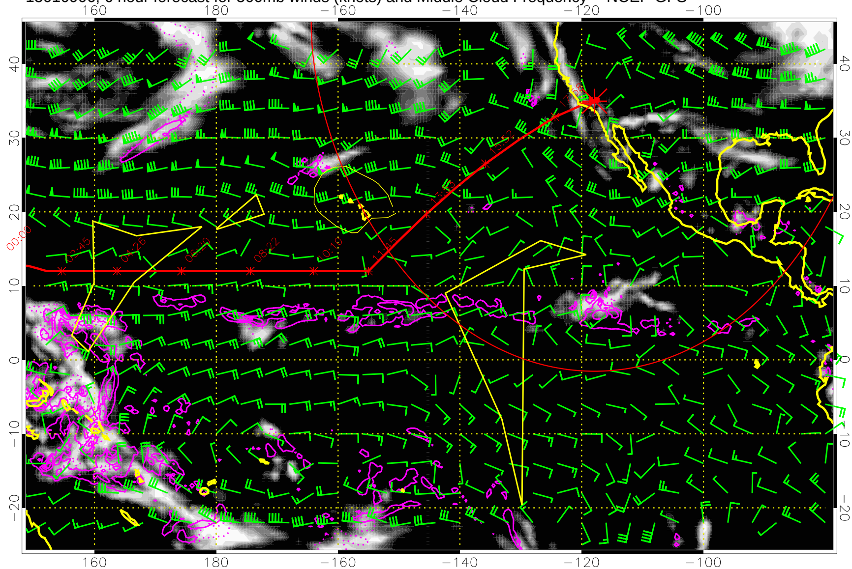
15010906, 6 hour forecast for 500mb winds (knots) and Middle Cloud Frequency -- NCEP GFS
