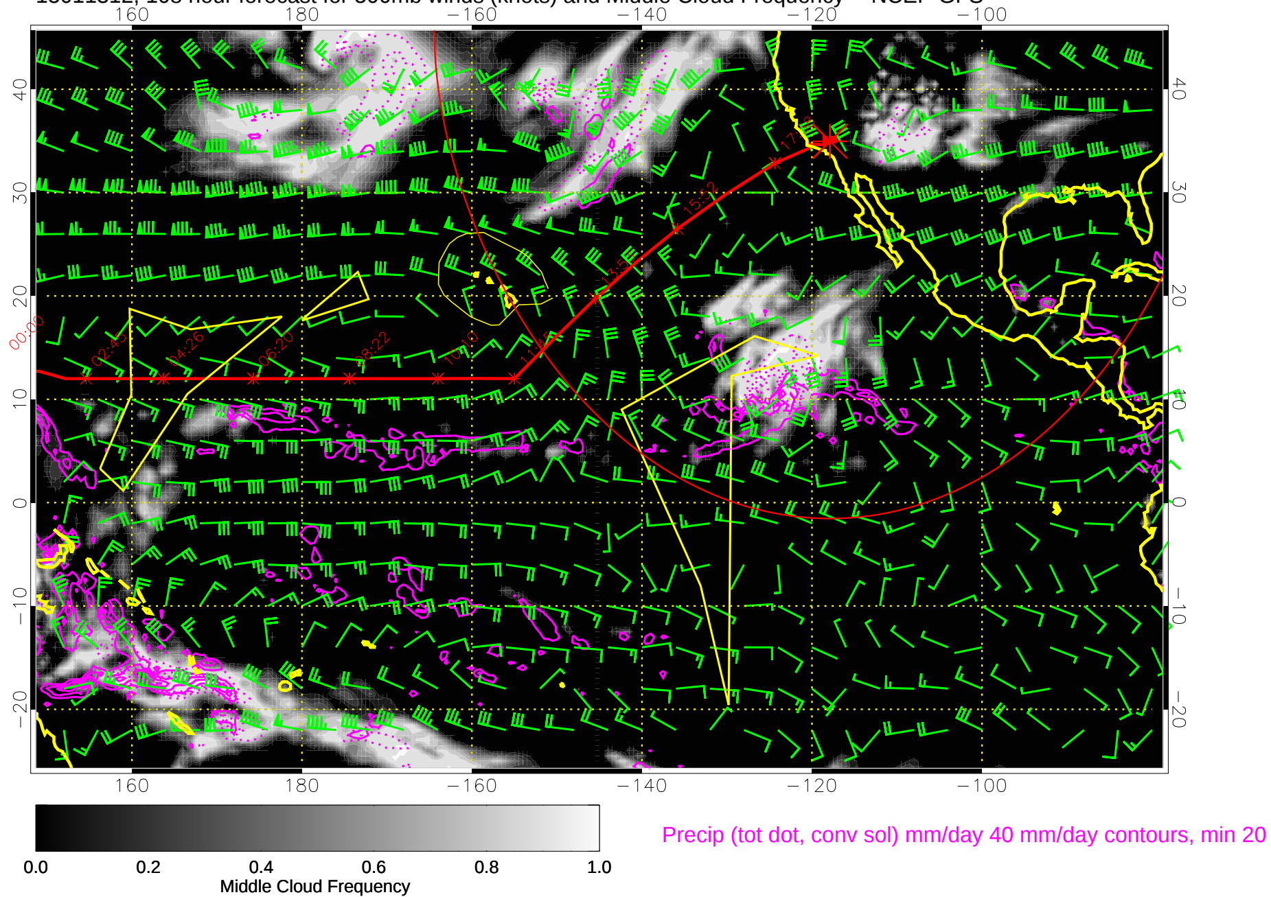
15011312, 108 hour forecast for 500mb winds (knots) and Middle Cloud Frequency -- NCEP GFS
