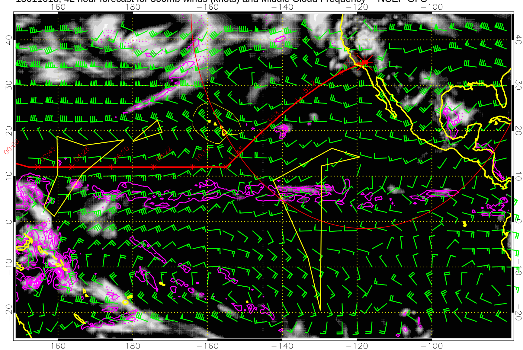
15011018, 42 hour forecast for 500mb winds (knots) and Middle Cloud Frequency -- NCEP GFS
