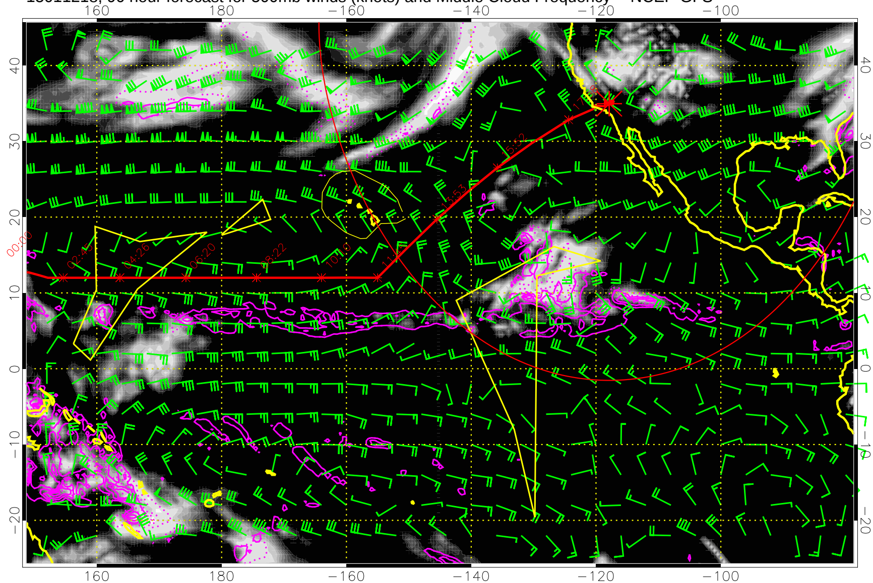
15011218, 90 hour forecast for 500mb winds (knots) and Middle Cloud Frequency -- NCEP GFS
