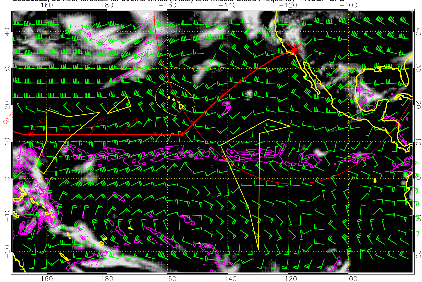
15011012, 36 hour forecast for 500mb winds (knots) and Middle Cloud Frequency -- NCEP GFS
