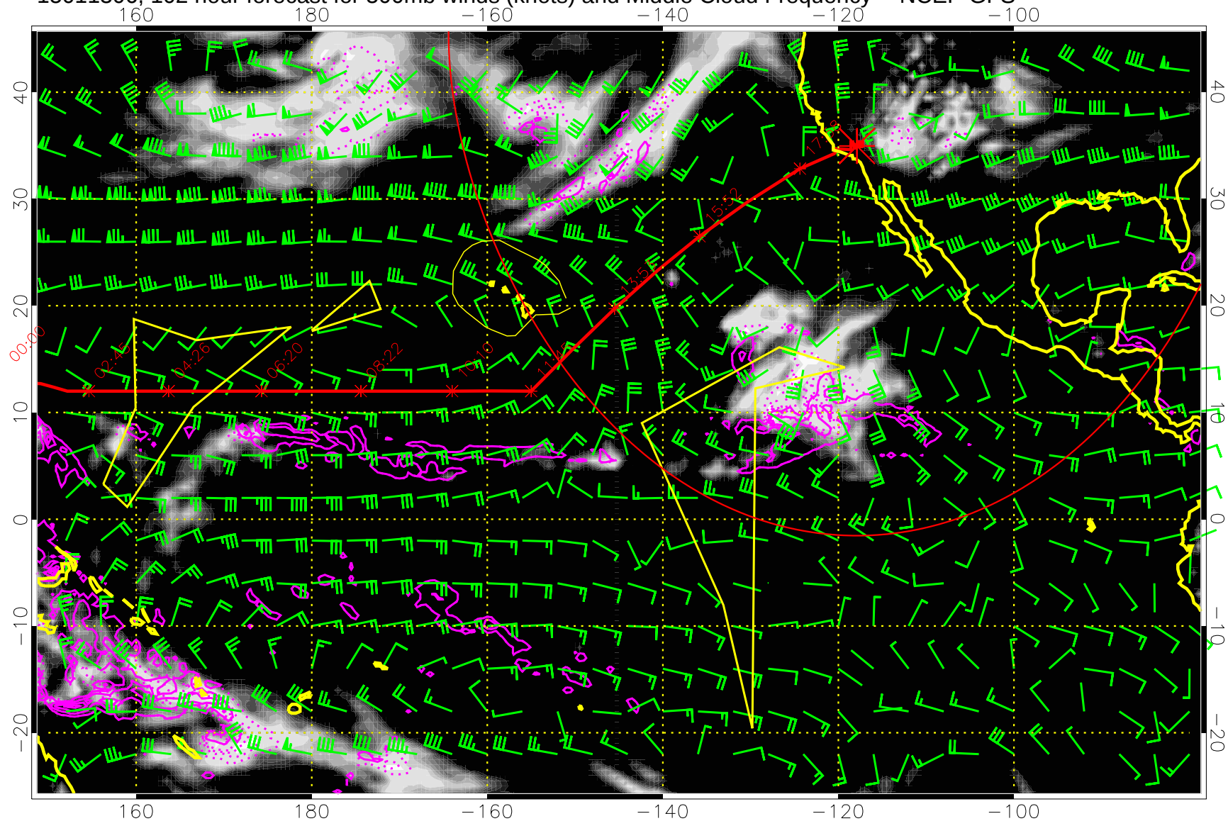
15011306, 102 hour forecast for 500mb winds (knots) and Middle Cloud Frequency -- NCEP GFS
