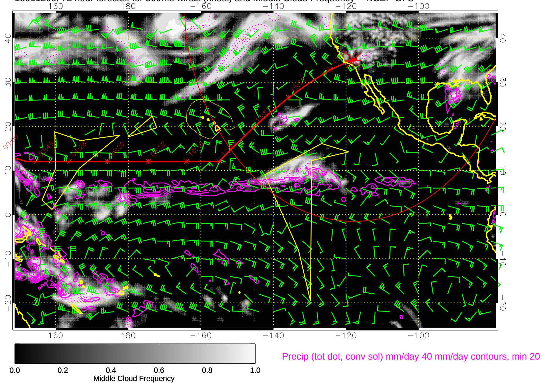
15011200, 72 hour forecast for 500mb winds (knots) and Middle Cloud Frequency -- NCEP GFS
