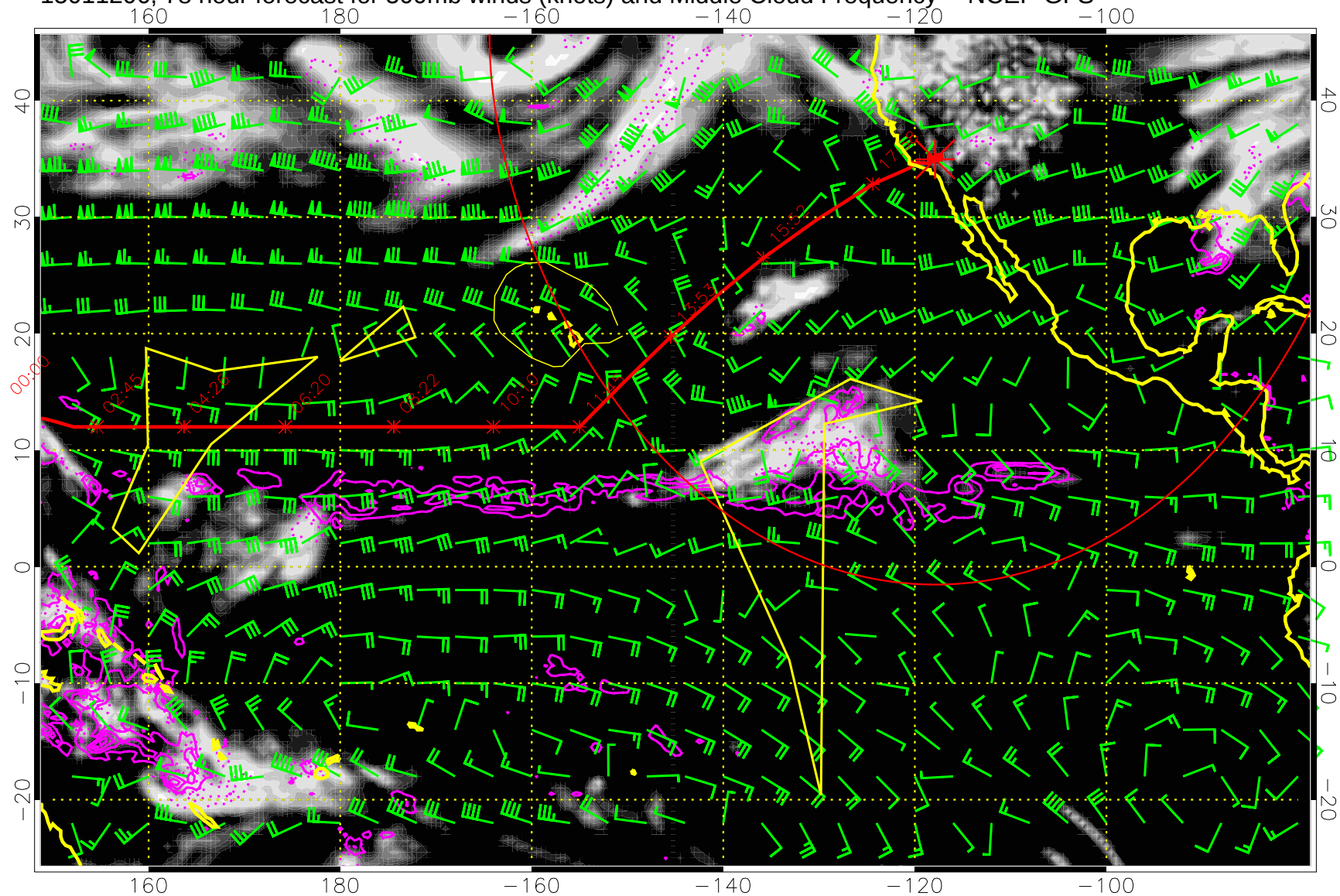
15011206, 78 hour forecast for 500mb winds (knots) and Middle Cloud Frequency -- NCEP GFS
