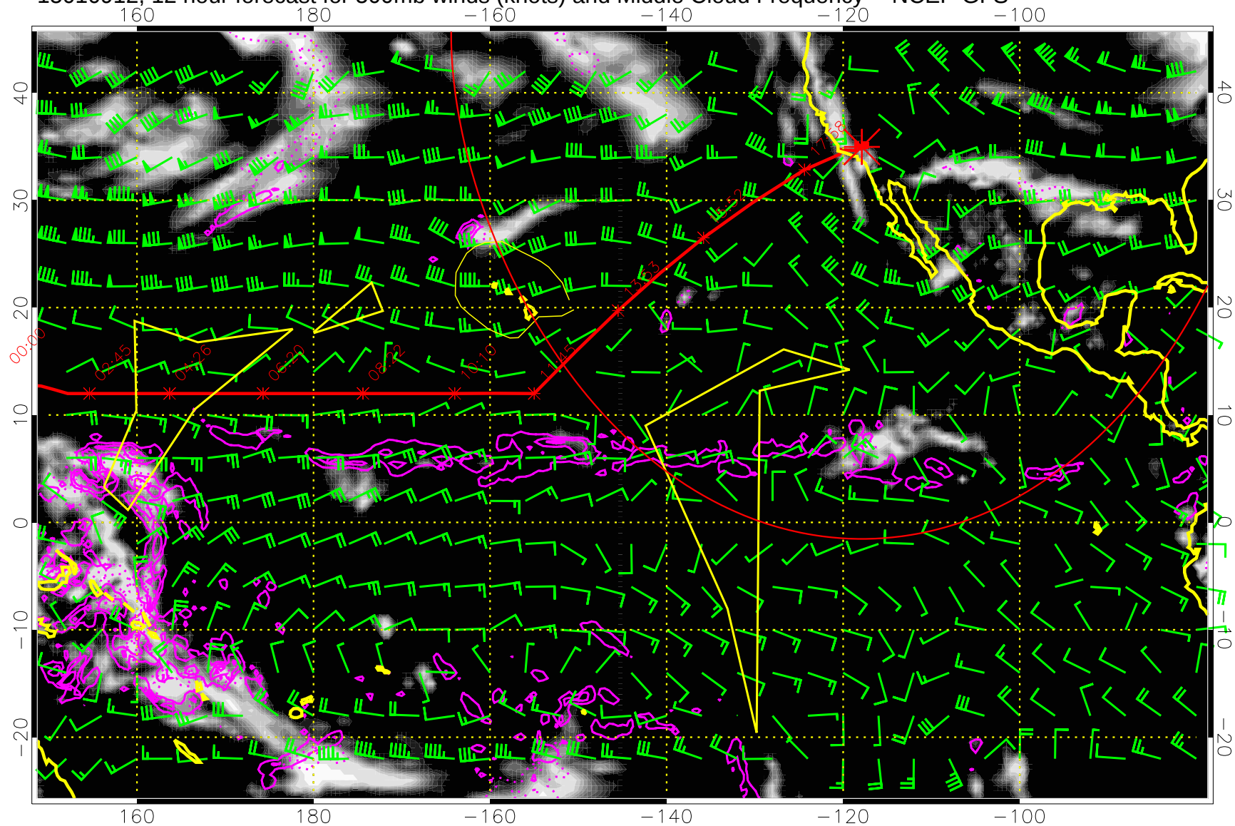
15010912, 12 hour forecast for 500mb winds (knots) and Middle Cloud Frequency -- NCEP GFS
