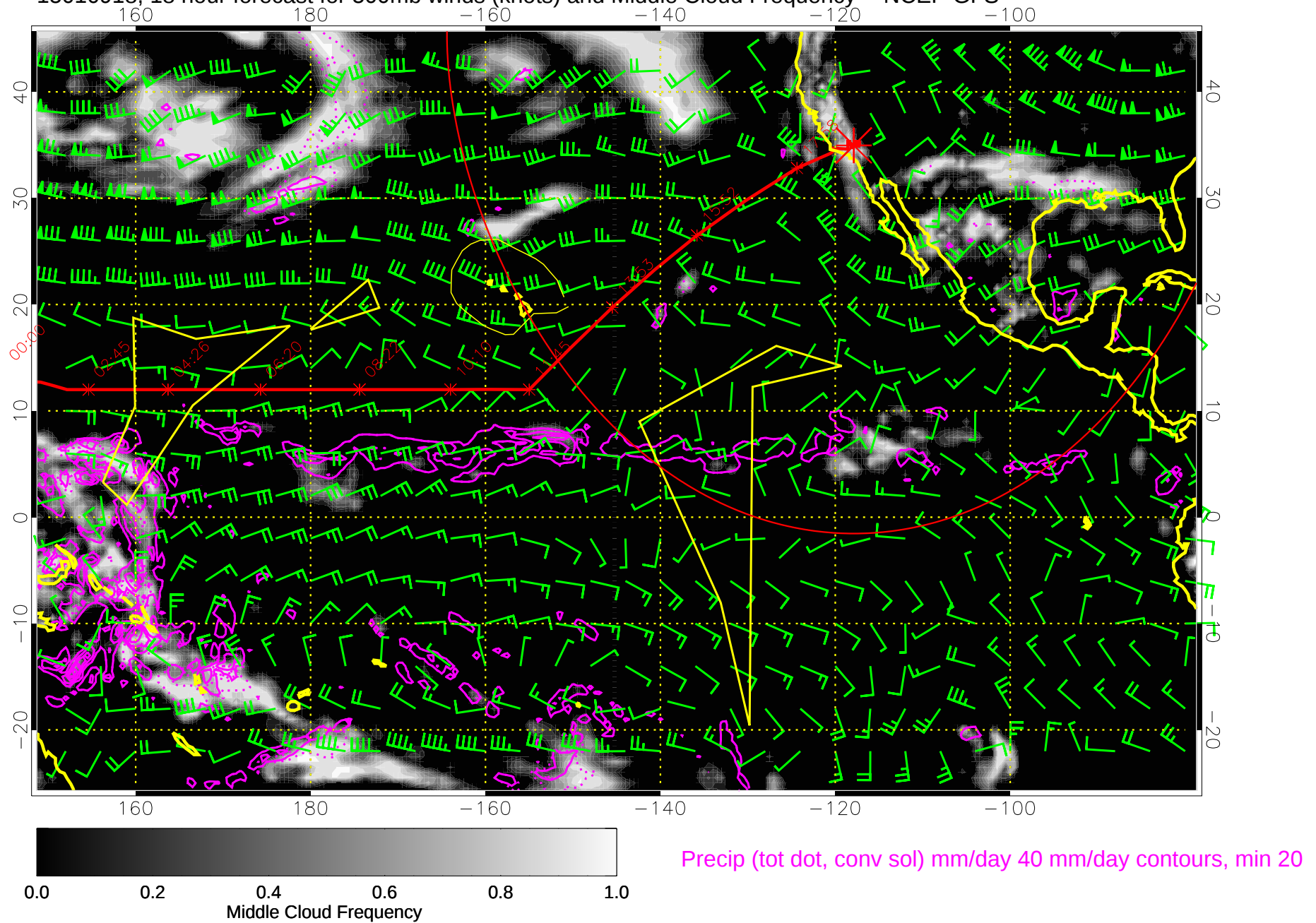
15010918, 18 hour forecast for 500mb winds (knots) and Middle Cloud Frequency -- NCEP GFS
