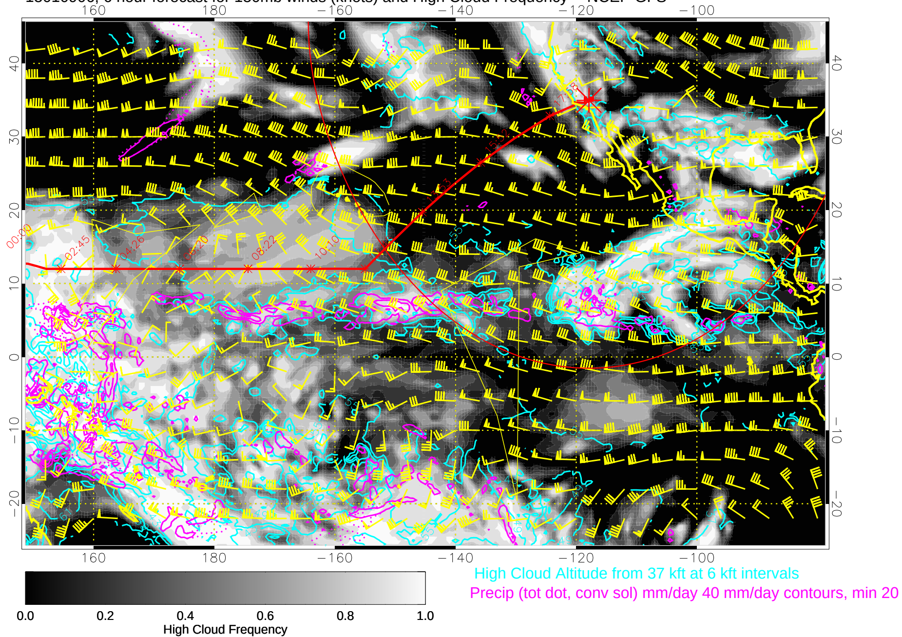
15010906, 6 hour forecast for 150mb winds (knots) and High Cloud Frequency -- NCEP GFS
