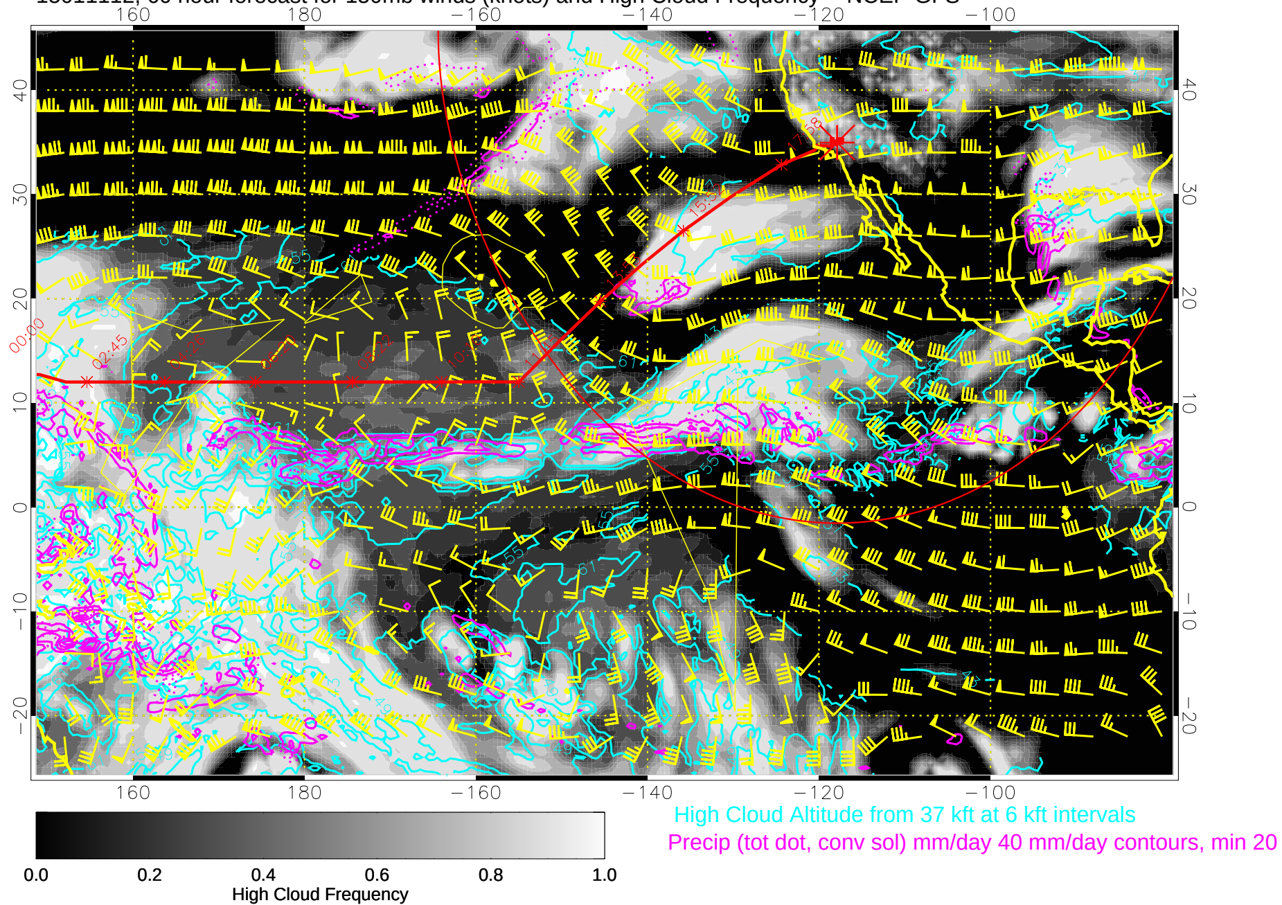
15011112, 60 hour forecast for 150mb winds (knots) and High Cloud Frequency -- NCEP GFS
