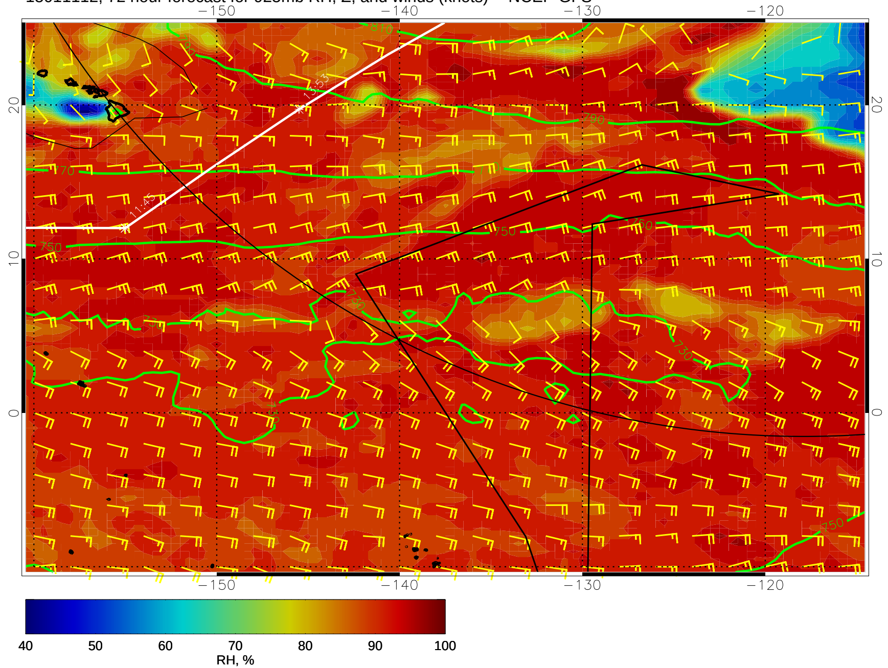
15011112, 72 hour forecast for 925mb RH, Z, and winds (knots) -- NCEP GFS
