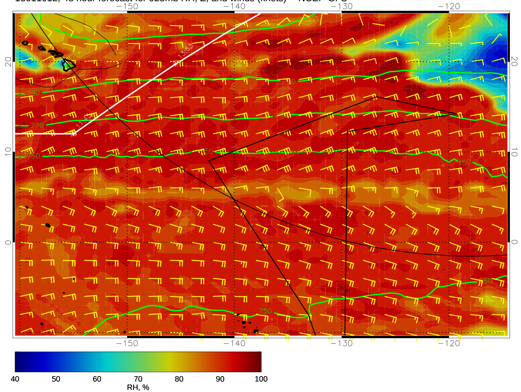
15011012, 48 hour forecast for 925mb RH, Z, and winds (knots) -- NCEP GFS
