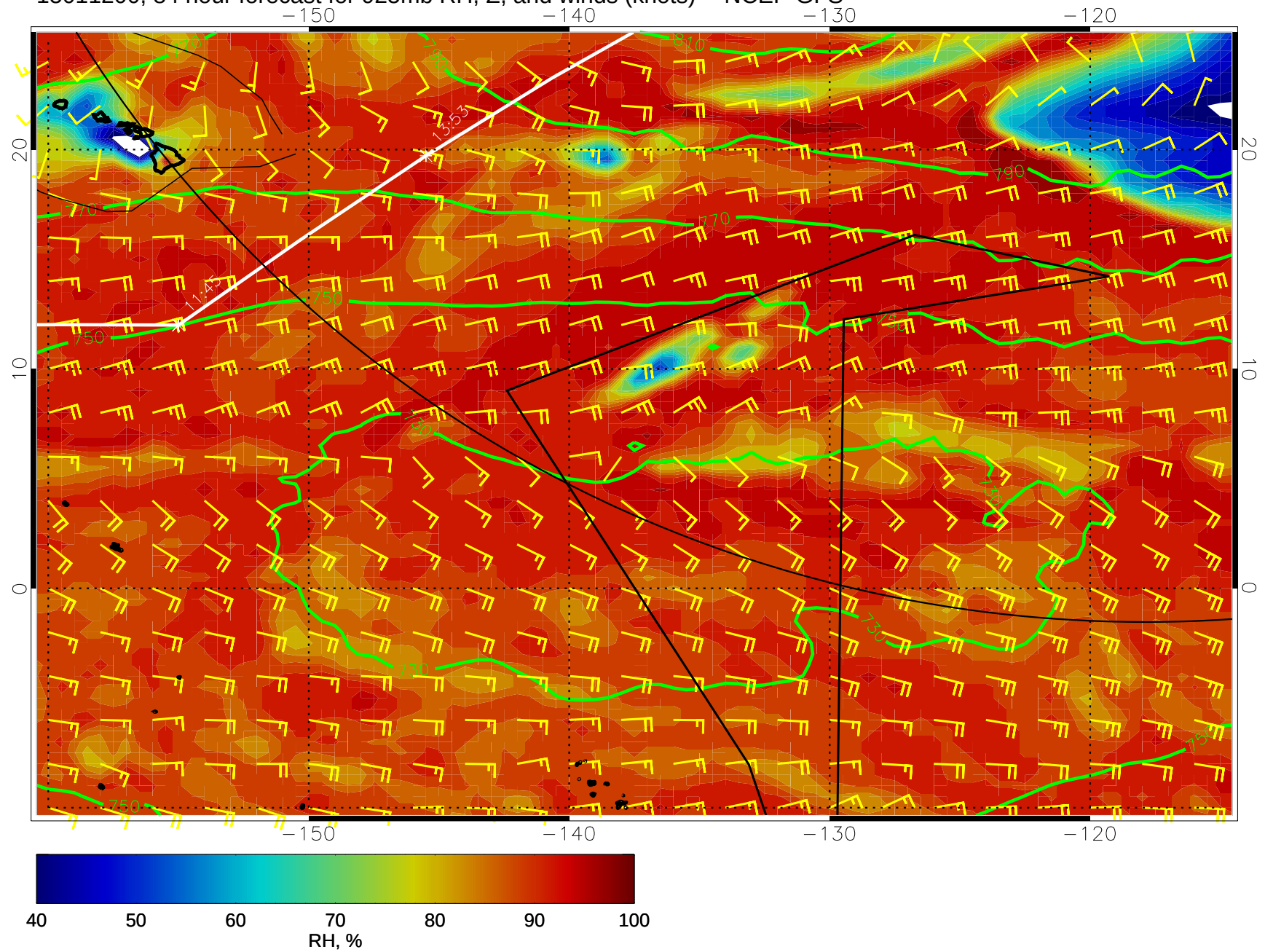
15011200, 84 hour forecast for 925mb RH, Z, and winds (knots) -- NCEP GFS
