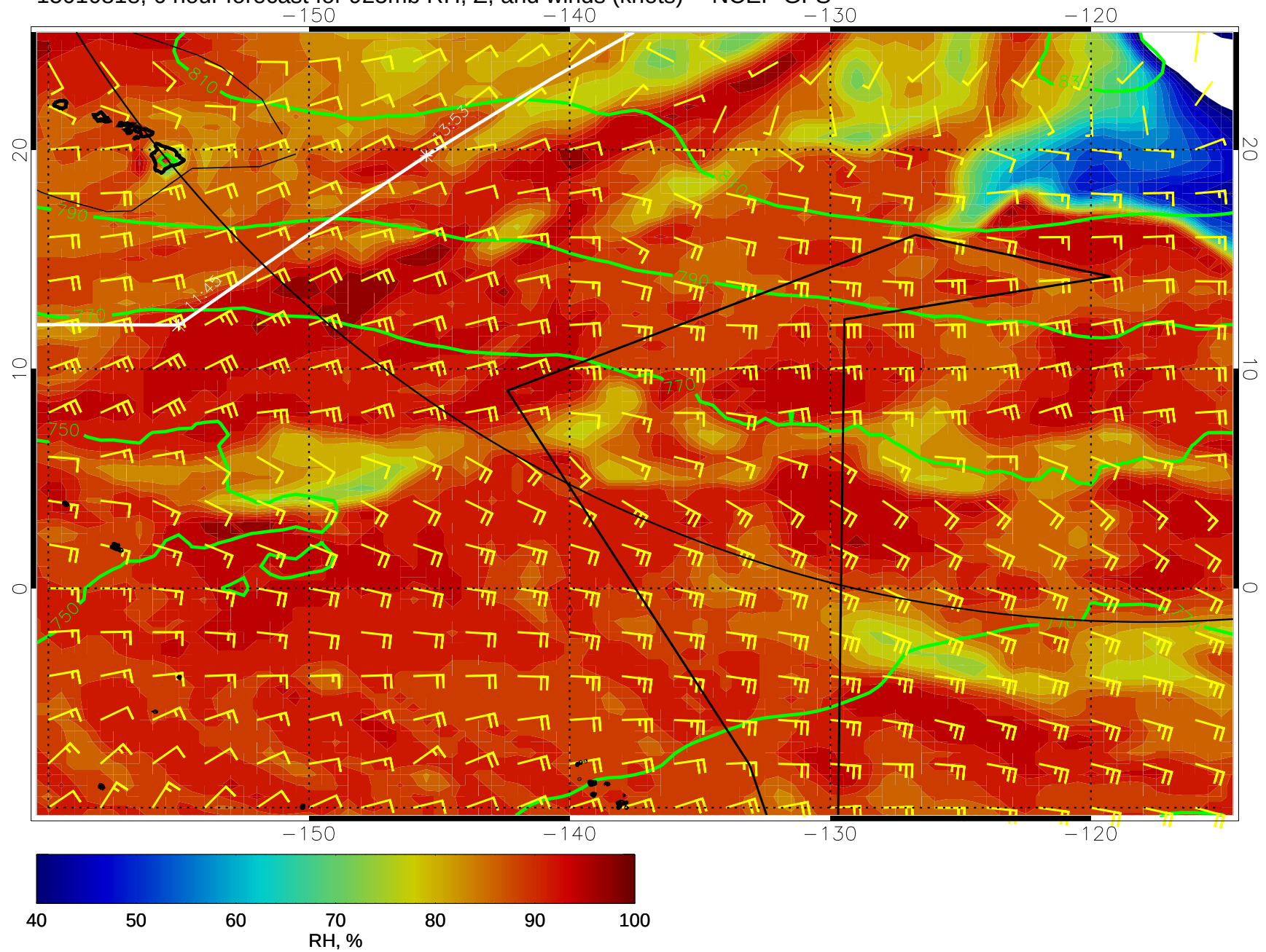
15010818, 6 hour forecast for 925mb RH, Z, and winds (knots) -- NCEP GFS
