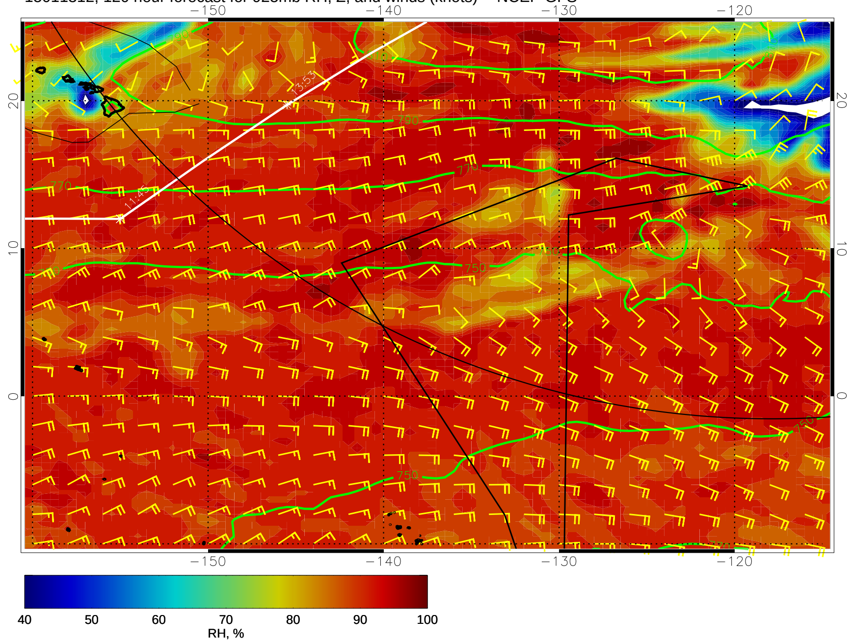
15011312, 120 hour forecast for 925mb RH, Z, and winds (knots) -- NCEP GFS
