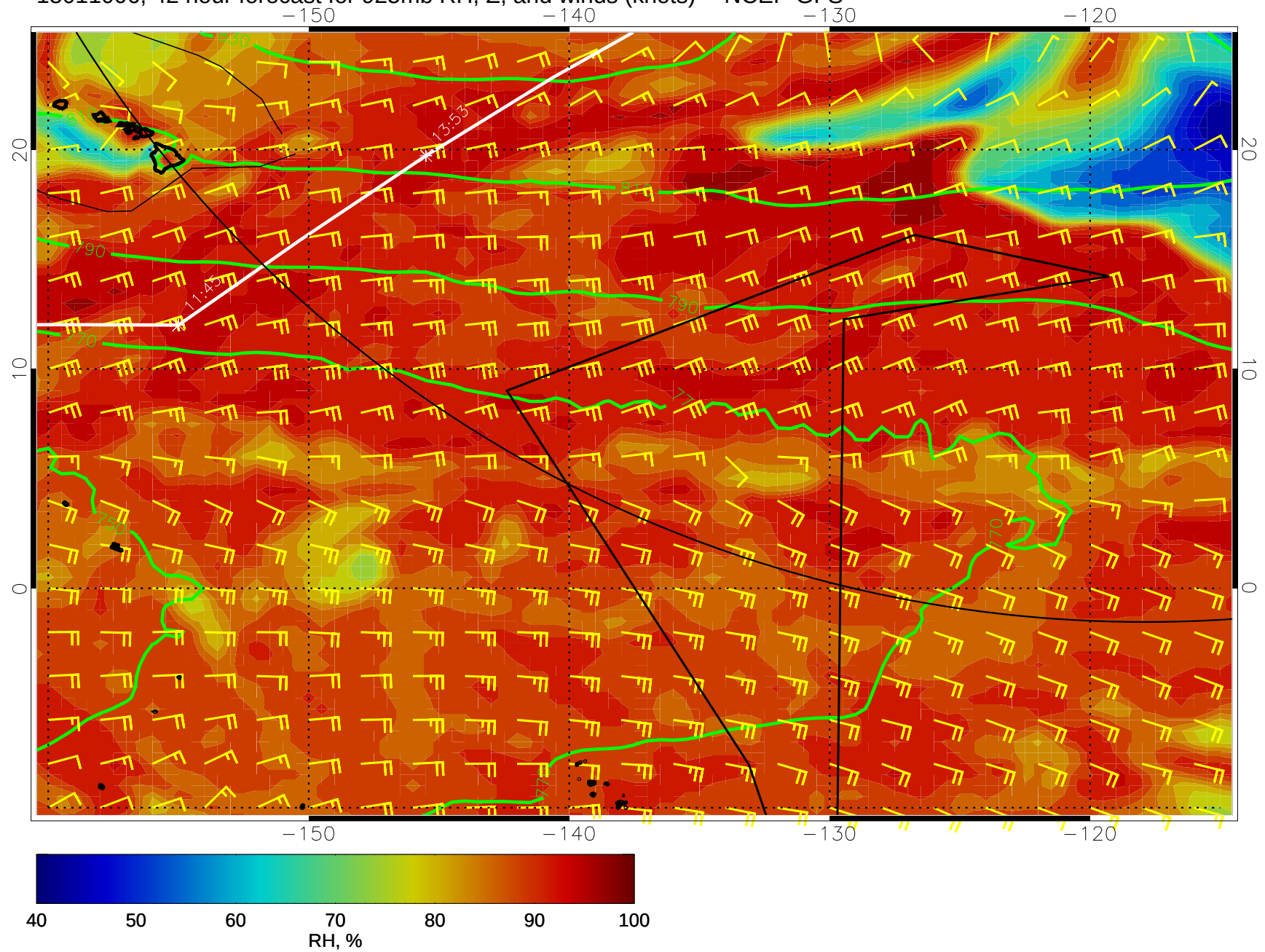
15011006, 42 hour forecast for 925mb RH, Z, and winds (knots) -- NCEP GFS
