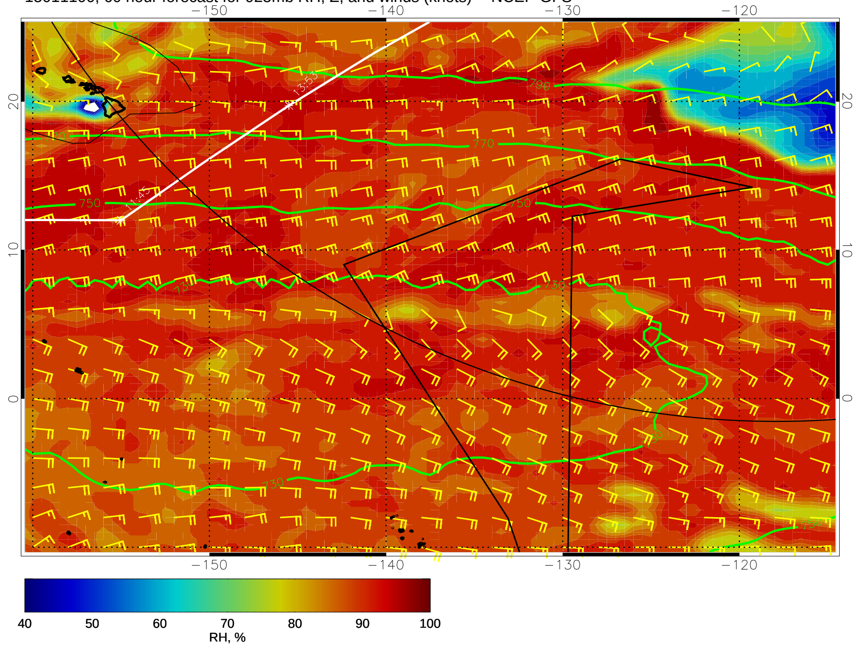
15011100, 60 hour forecast for 925mb RH, Z, and winds (knots) -- NCEP GFS
