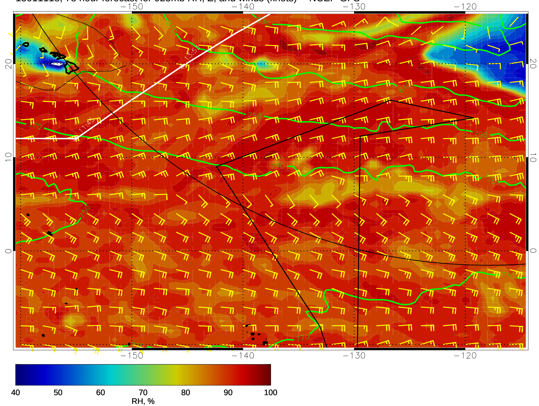
15011118, 78 hour forecast for 925mb RH, Z, and winds (knots) -- NCEP GFS
