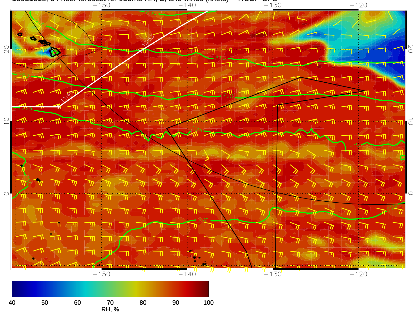
15011018, 54 hour forecast for 925mb RH, Z, and winds (knots) -- NCEP GFS
