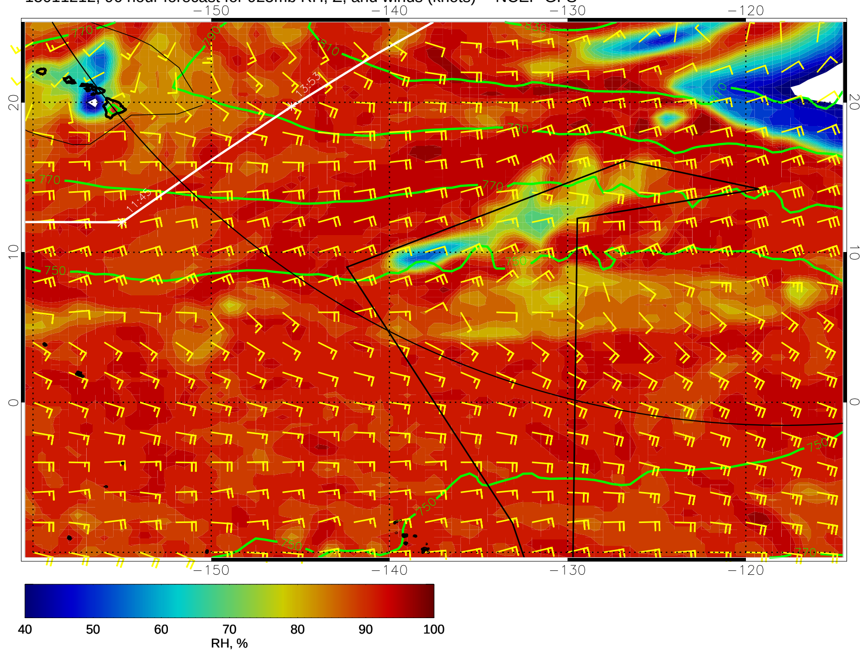
15011212, 96 hour forecast for 925mb RH, Z, and winds (knots) -- NCEP GFS
