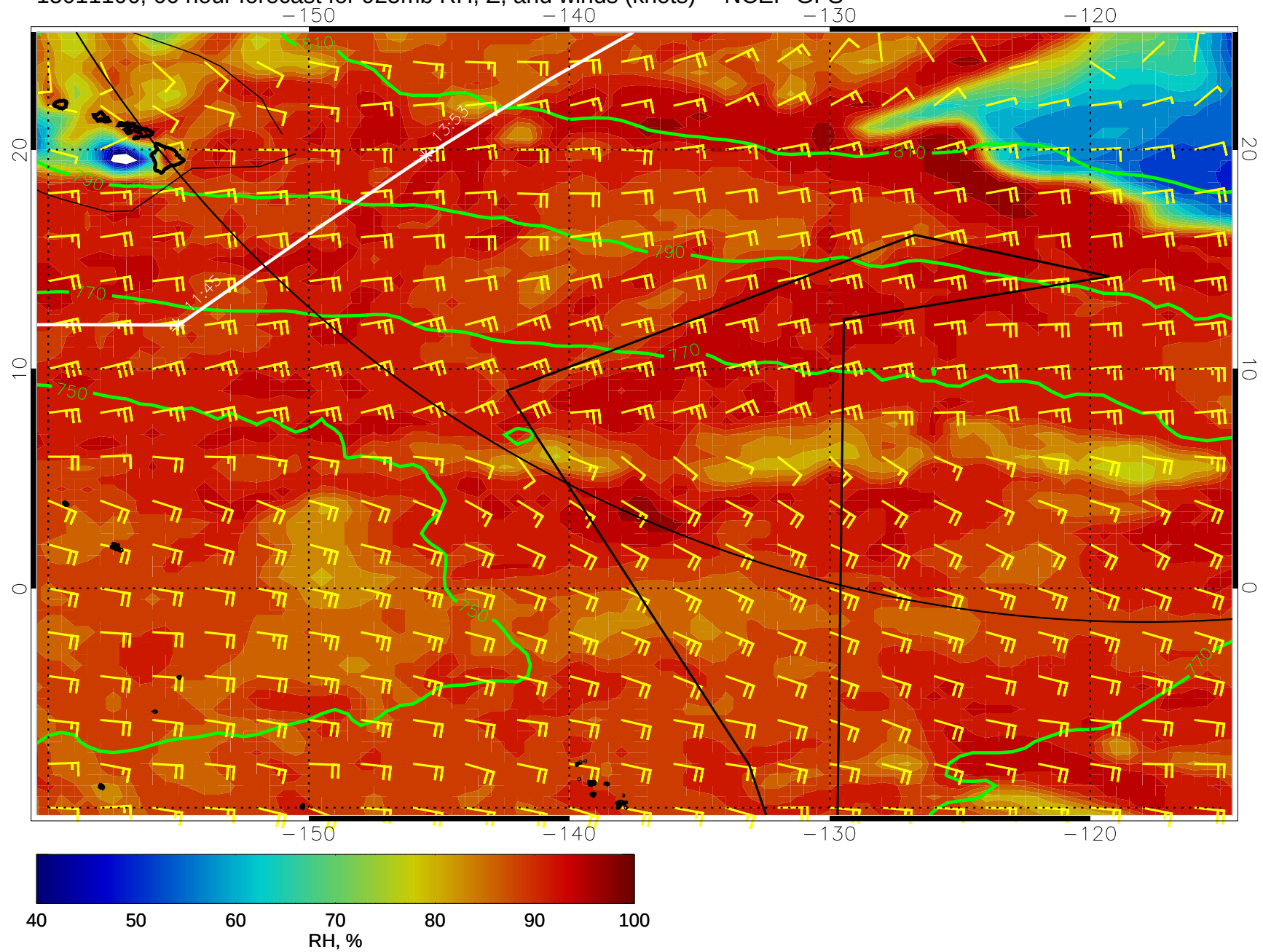
15011106, 66 hour forecast for 925mb RH, Z, and winds (knots) -- NCEP GFS
