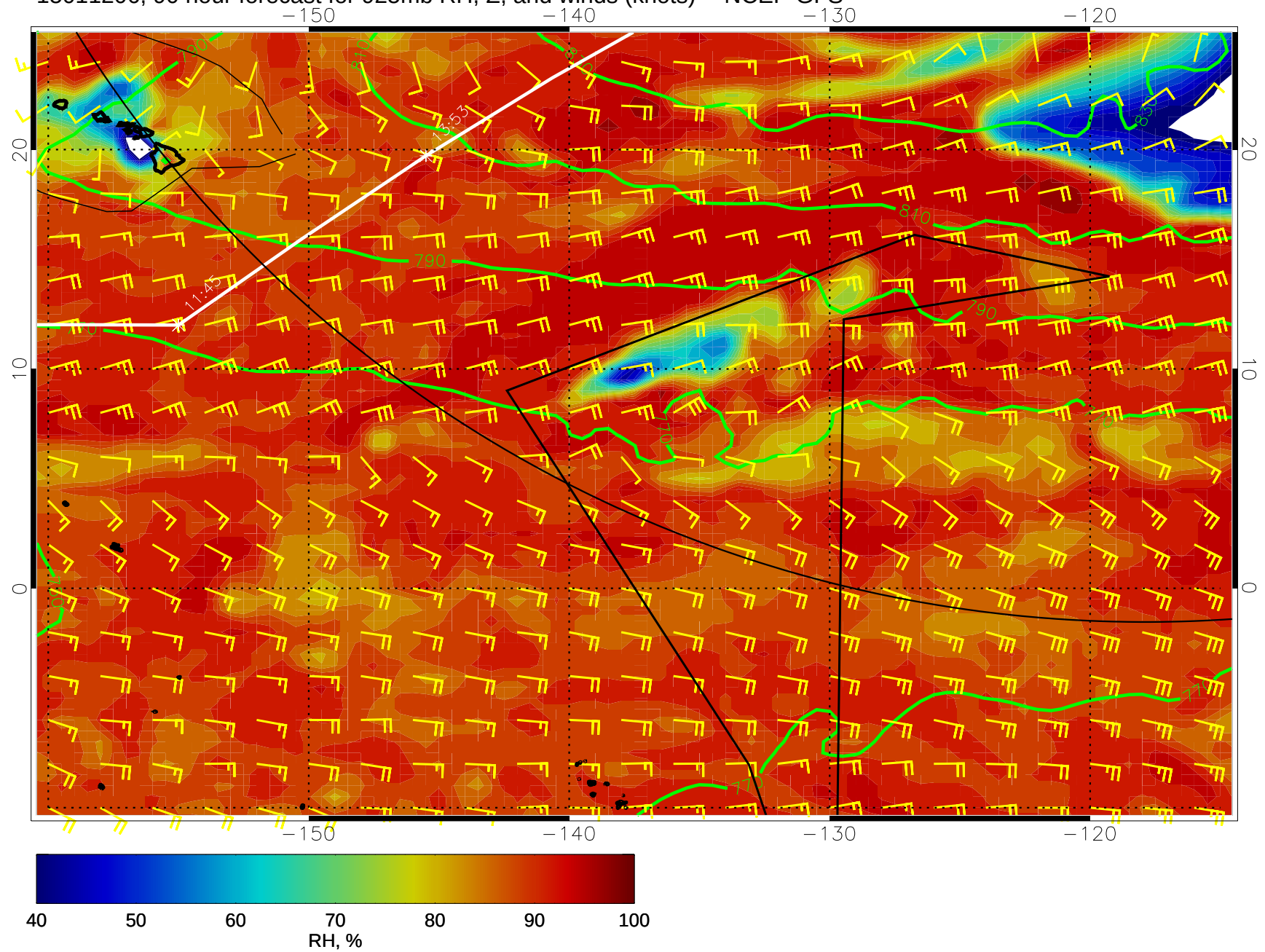
15011206, 90 hour forecast for 925mb RH, Z, and winds (knots) -- NCEP GFS
