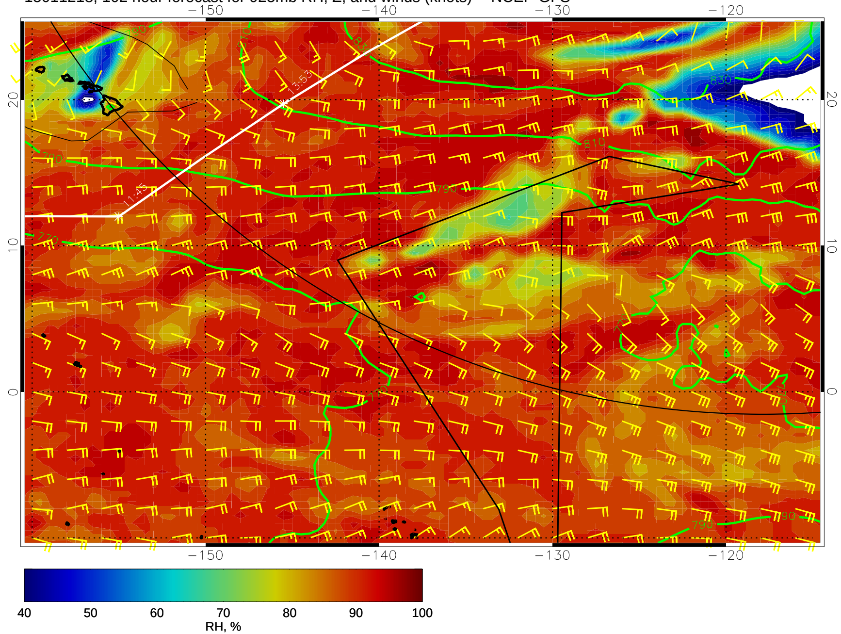
15011218, 102 hour forecast for 925mb RH, Z, and winds (knots) -- NCEP GFS
