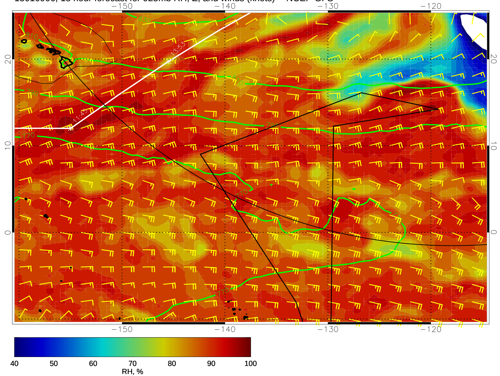
15010906, 18 hour forecast for 925mb RH, Z, and winds (knots) -- NCEP GFS
