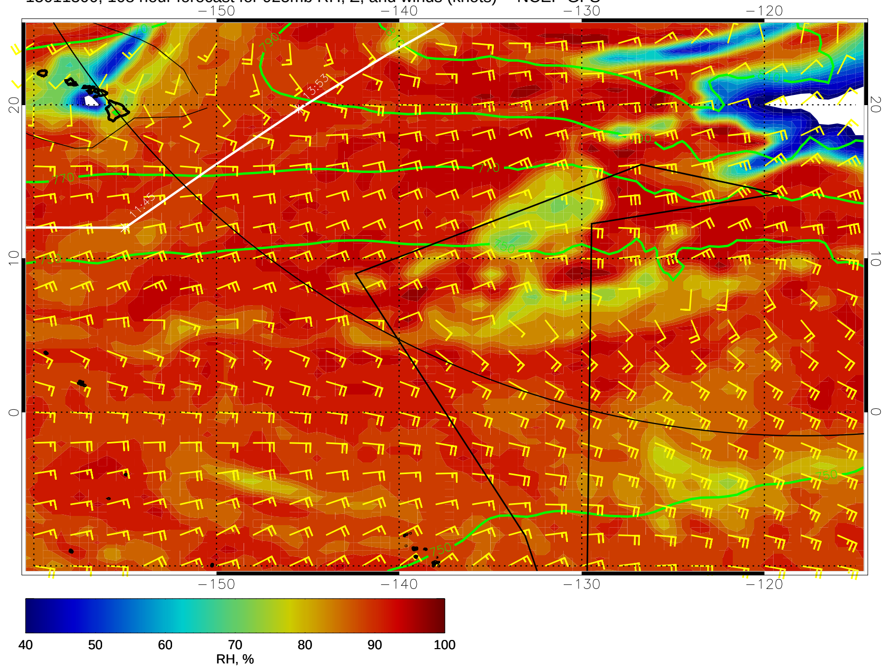
15011300, 108 hour forecast for 925mb RH, Z, and winds (knots) -- NCEP GFS
