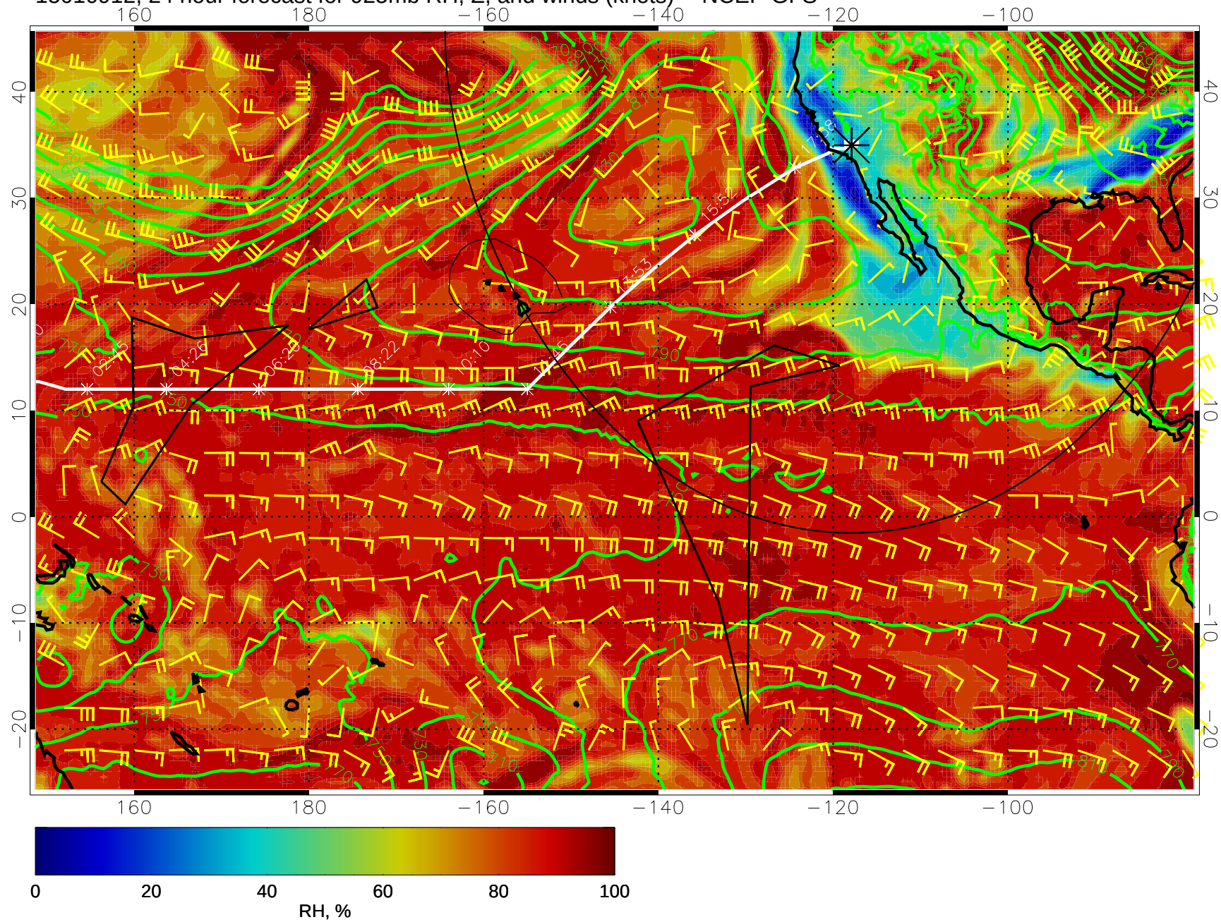
15010912, 24 hour forecast for 925mb RH, Z, and winds (knots) -- NCEP GFS
