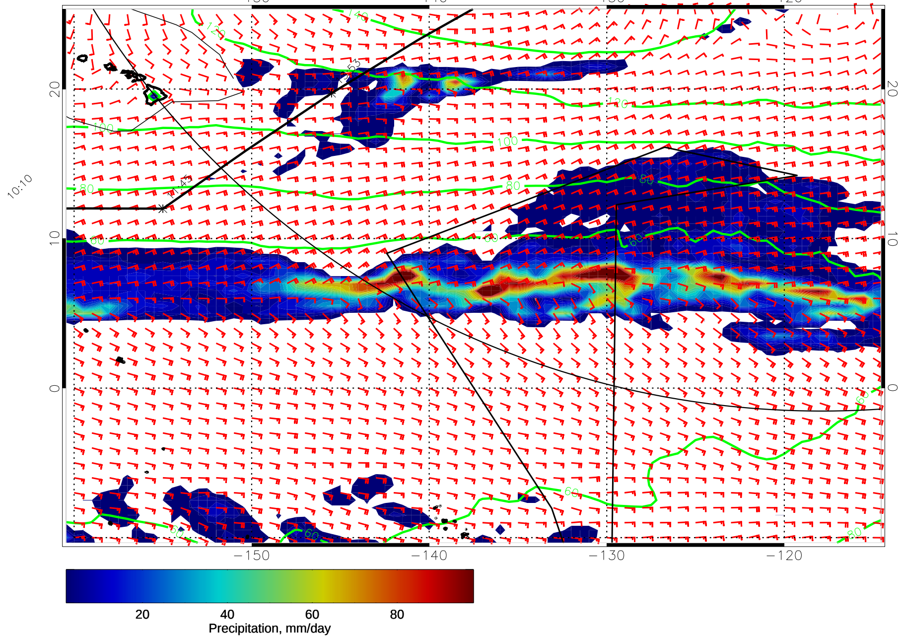
15011112, 72 hour forecast for precip, 1000mb Z, and winds (knots) -- NCEP GFS
