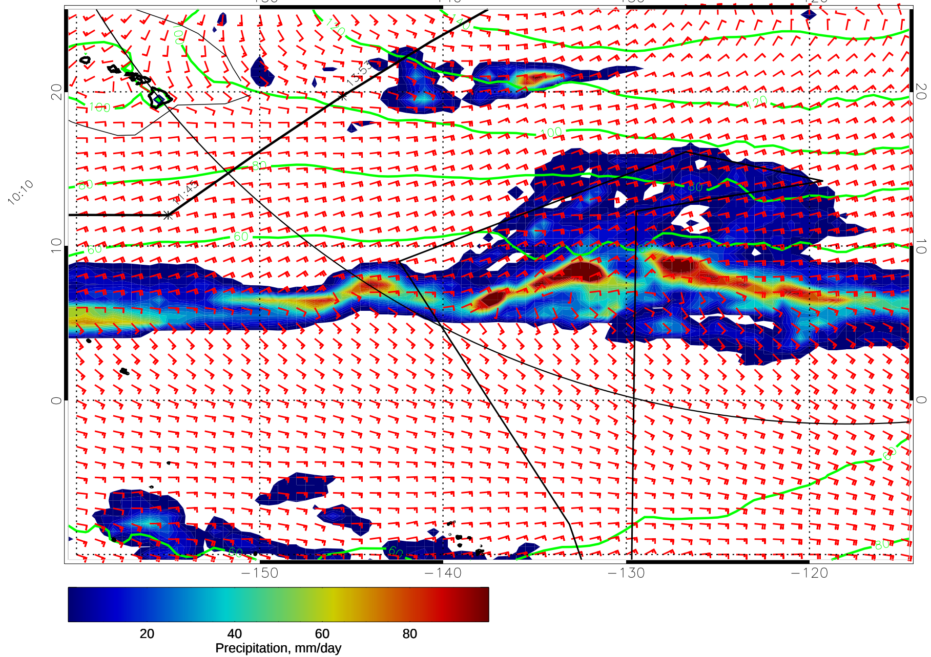
15011200, 84 hour forecast for precip, 1000mb Z, and winds (knots) -- NCEP GFS
