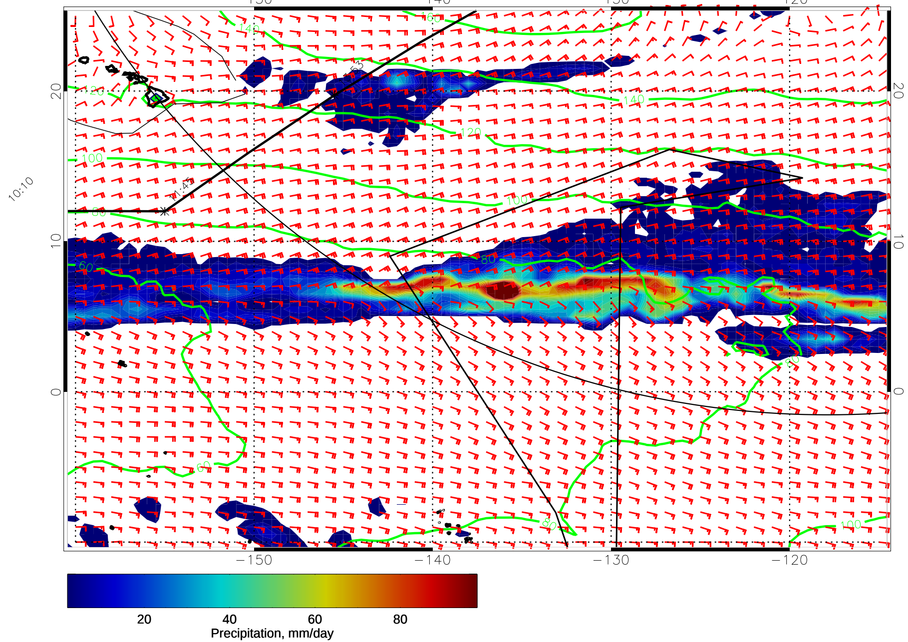
15011106, 66 hour forecast for precip, 1000mb Z, and winds (knots) -- NCEP GFS
