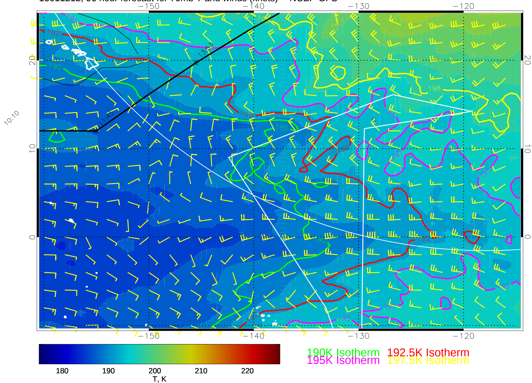
15011212, 96 hour forecast for 70mb T and winds (knots) -- NCEP GFS
