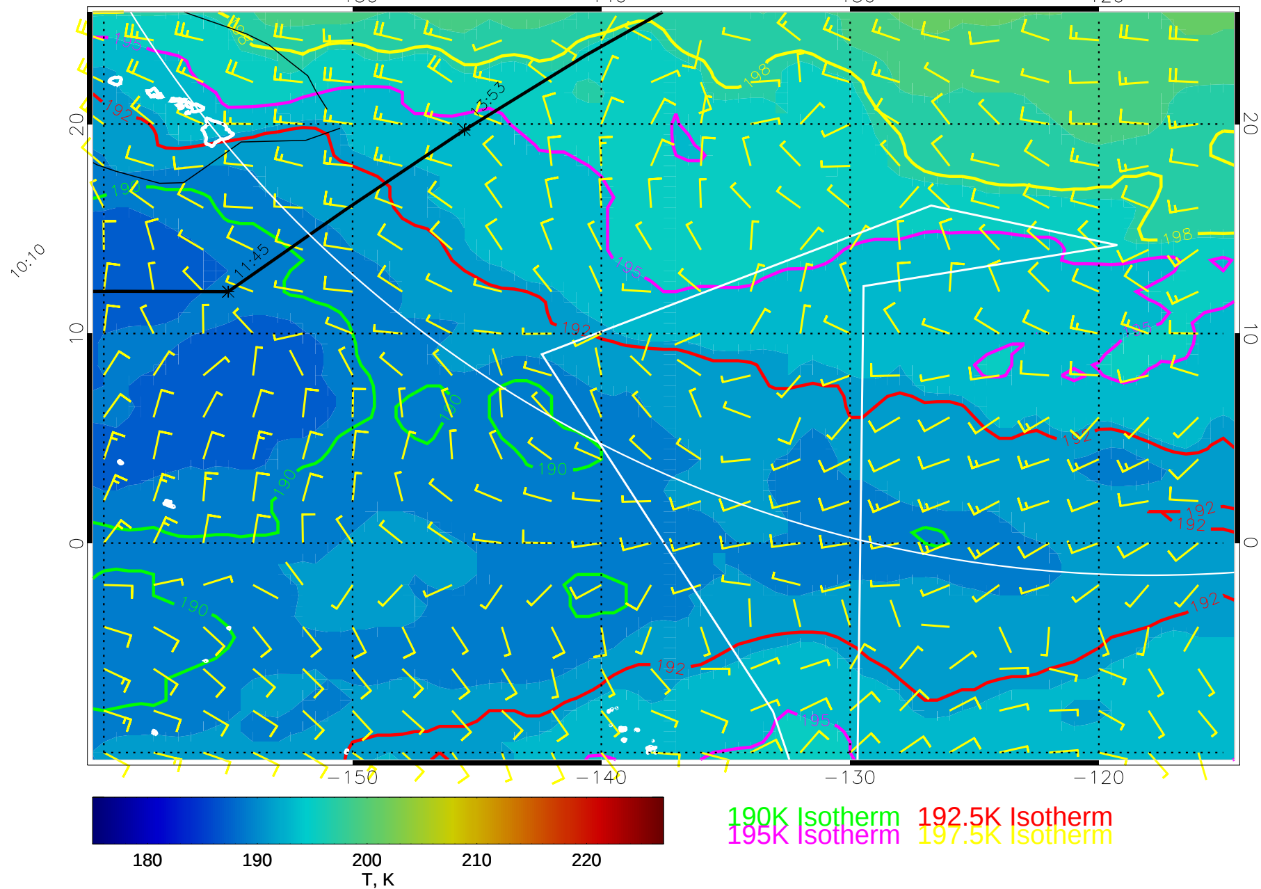
15010906, 18 hour forecast for 70mb T and winds (knots) -- NCEP GFS
