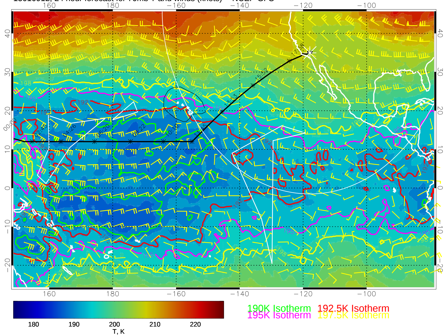
15010912, 24 hour forecast for 70mb T and winds (knots) -- NCEP GFS
