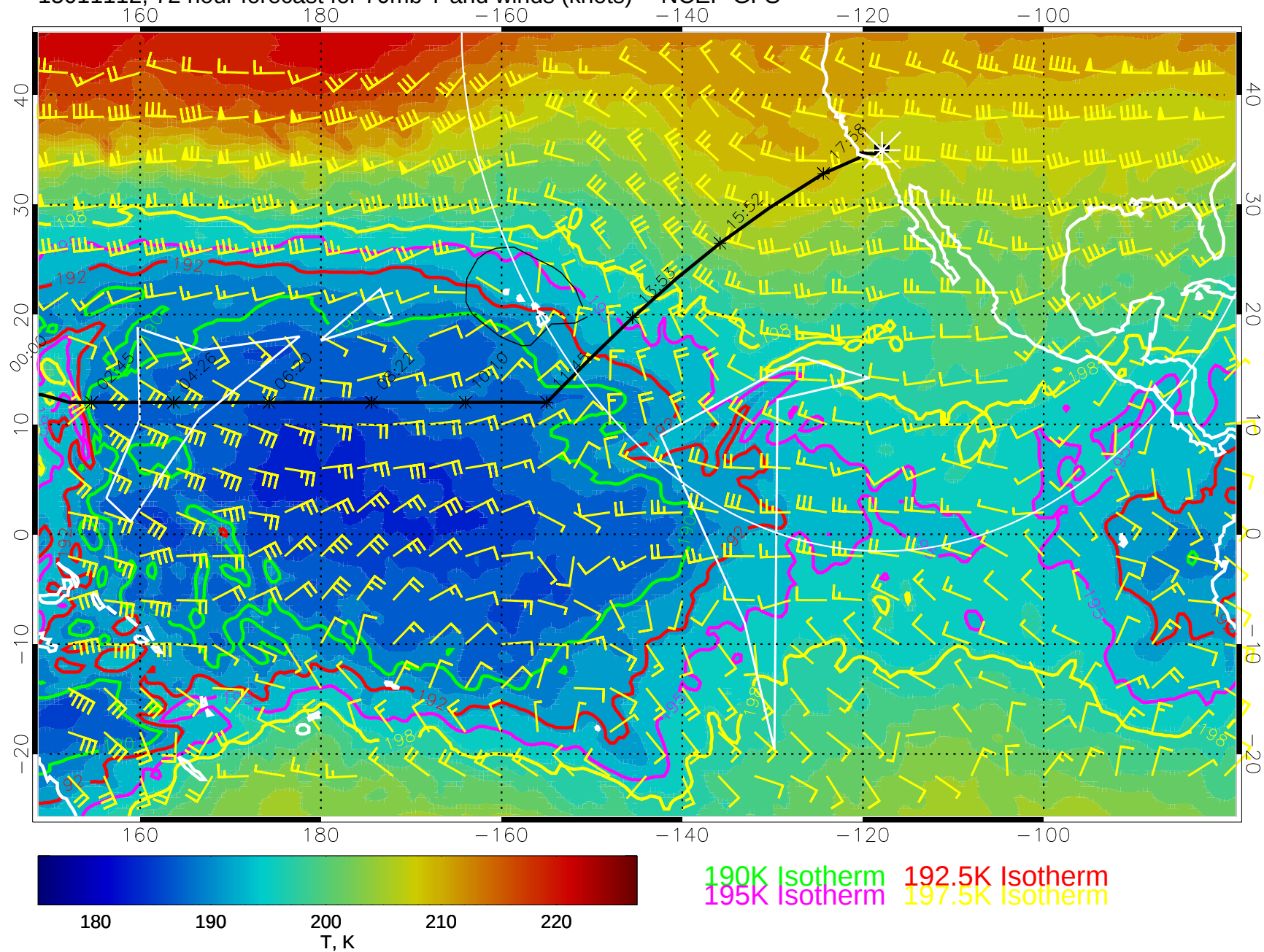
15011112, 72 hour forecast for 70mb T and winds (knots) -- NCEP GFS
