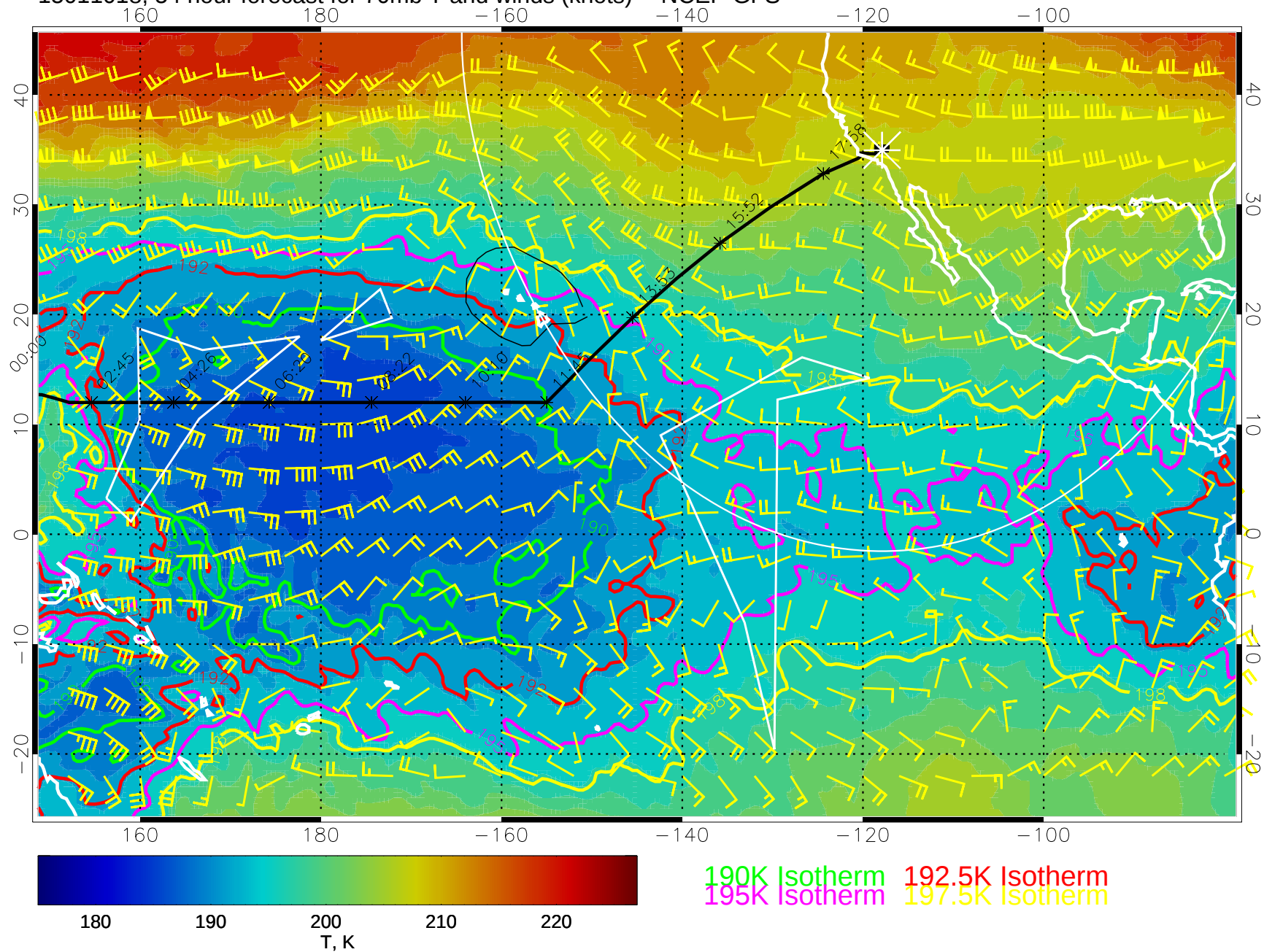
15011018, 54 hour forecast for 70mb T and winds (knots) -- NCEP GFS
