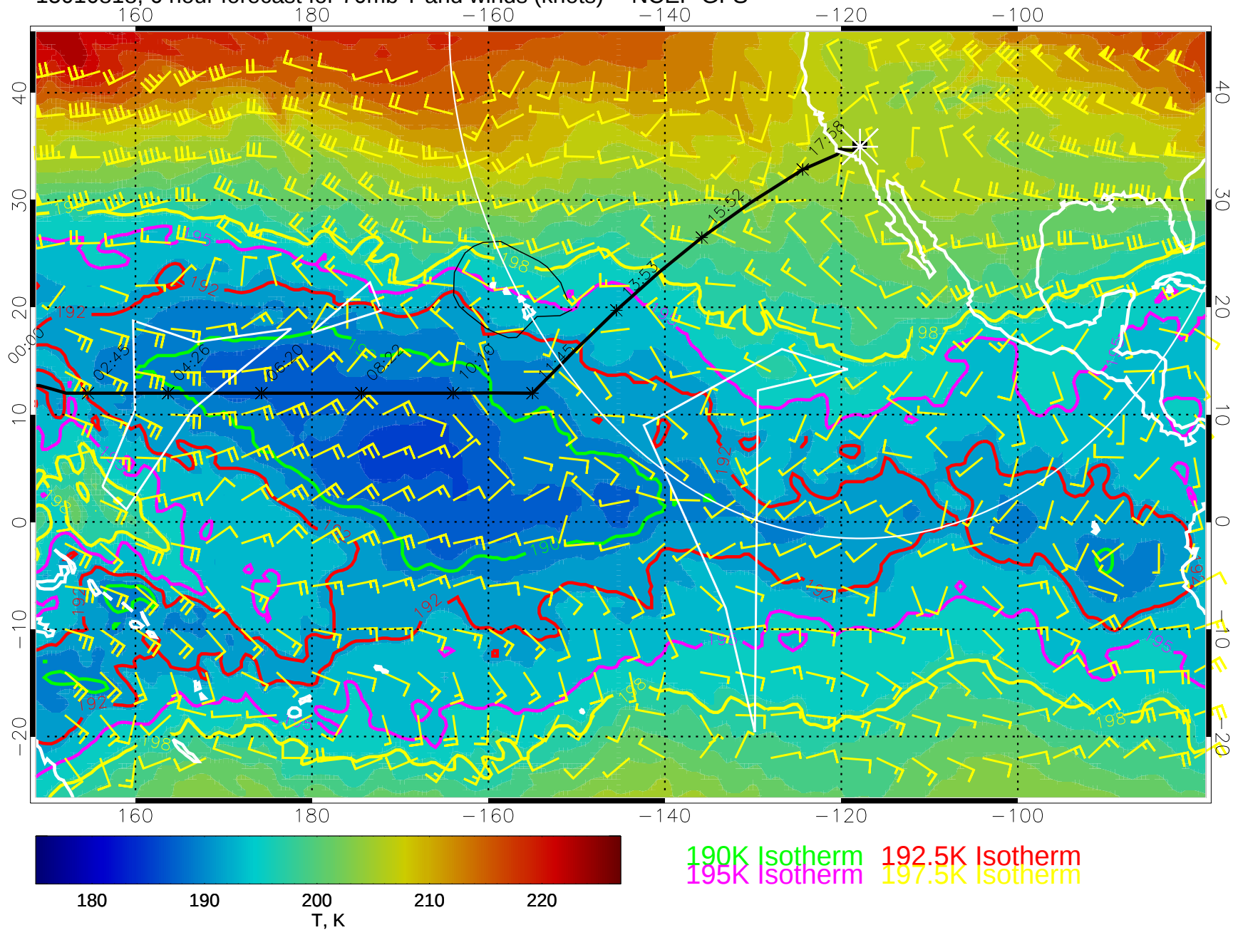
15010818, 6 hour forecast for 70mb T and winds (knots) -- NCEP GFS
