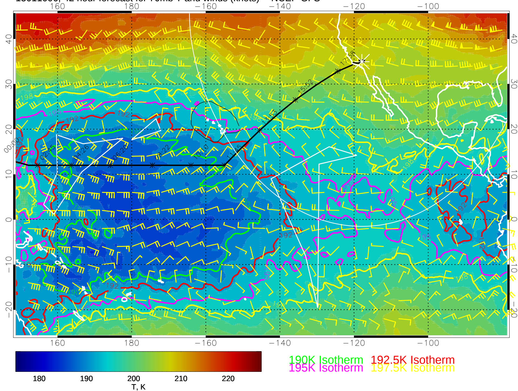
15011006, 42 hour forecast for 70mb T and winds (knots) -- NCEP GFS
