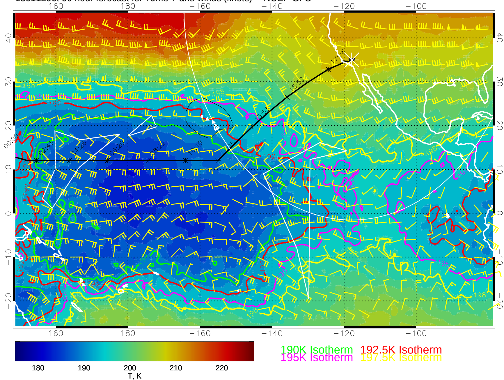
15011206, 90 hour forecast for 70mb T and winds (knots) -- NCEP GFS
