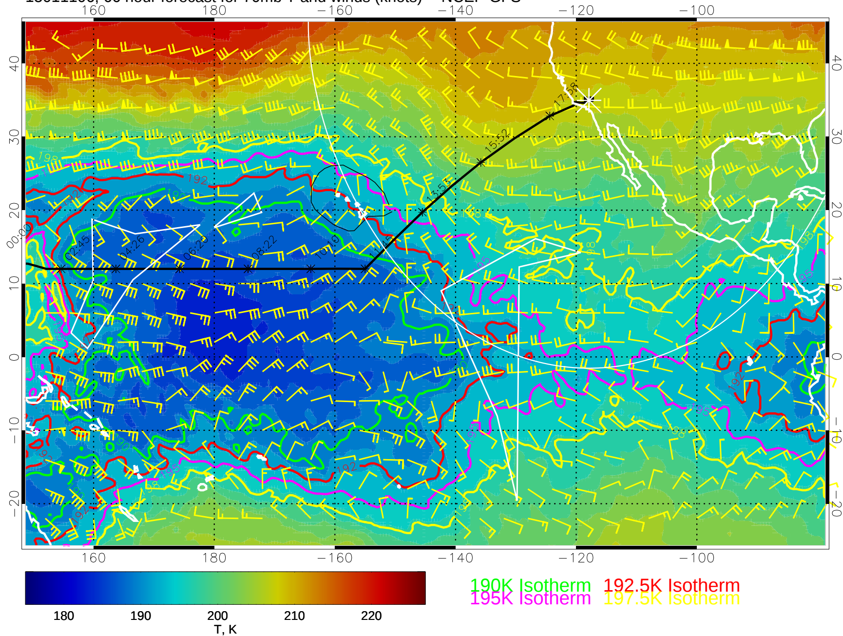
15011106, 66 hour forecast for 70mb T and winds (knots) -- NCEP GFS
