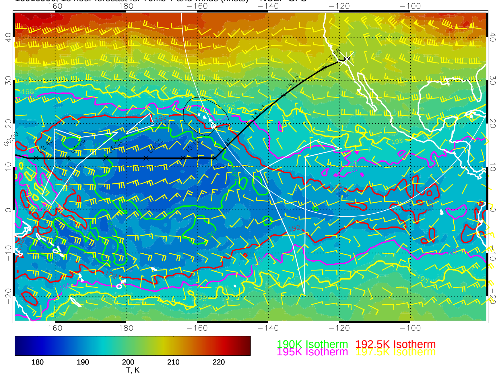
15010906, 18 hour forecast for 70mb T and winds (knots) -- NCEP GFS
