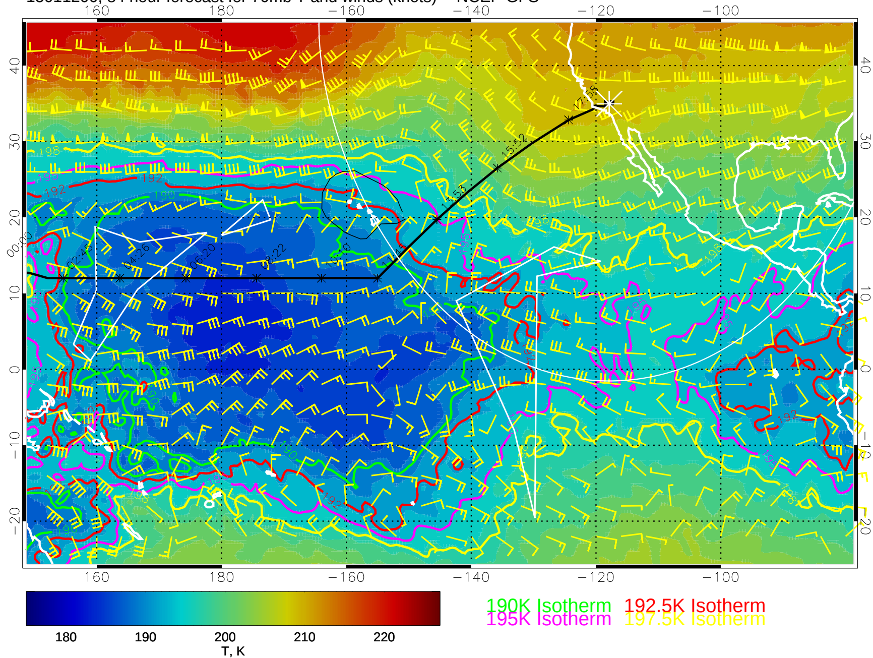
15011200, 84 hour forecast for 70mb T and winds (knots) -- NCEP GFS
