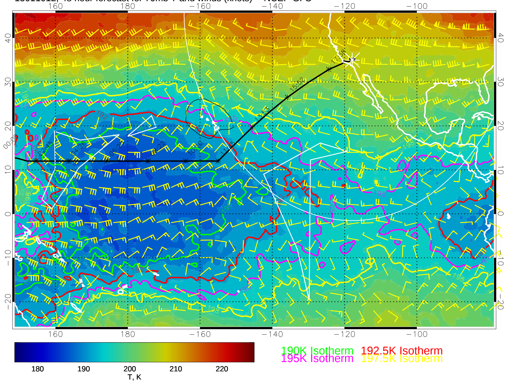
15011012, 48 hour forecast for 70mb T and winds (knots) -- NCEP GFS
