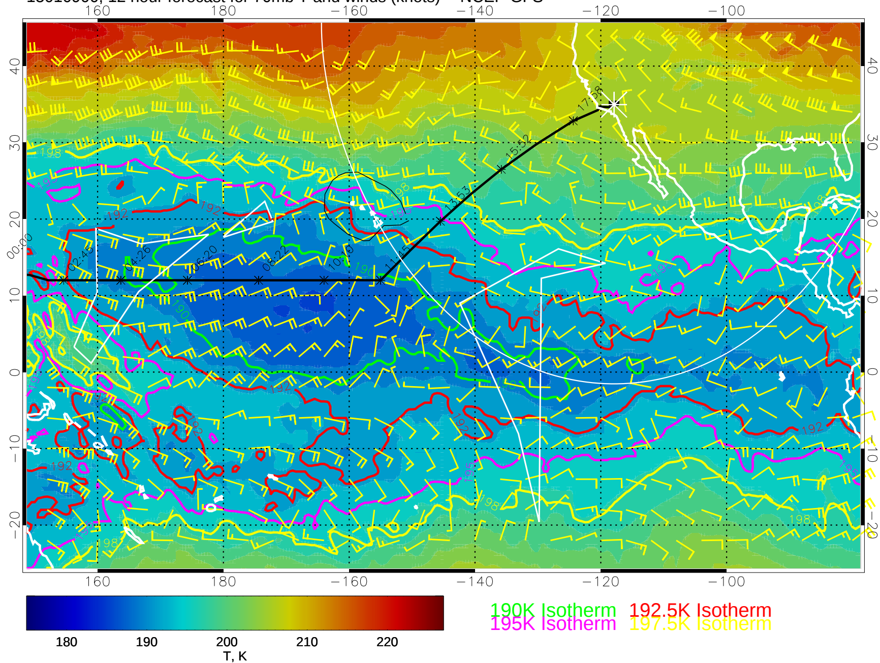
15010900, 12 hour forecast for 70mb T and winds (knots) -- NCEP GFS
