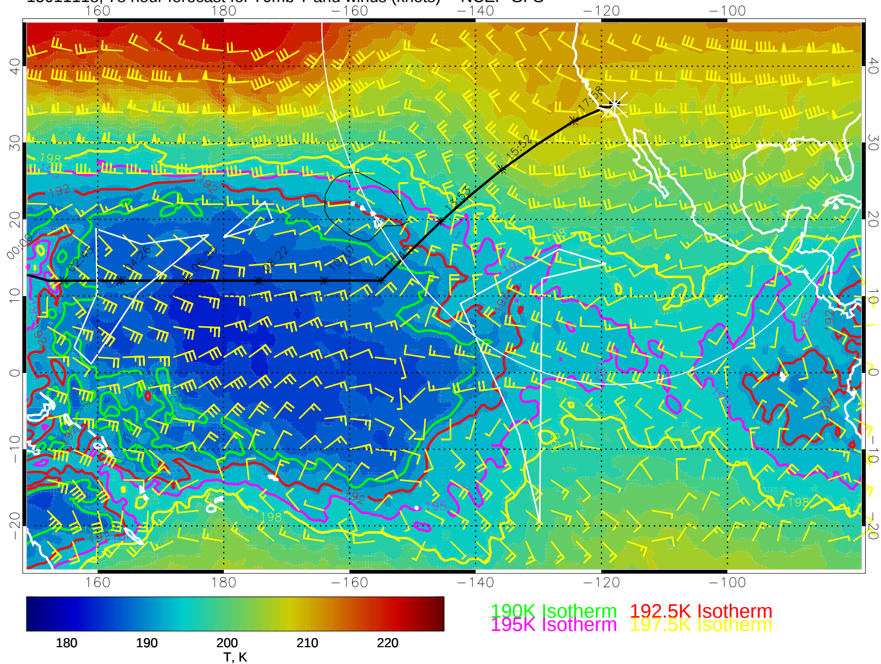
15011118, 78 hour forecast for 70mb T and winds (knots) -- NCEP GFS
