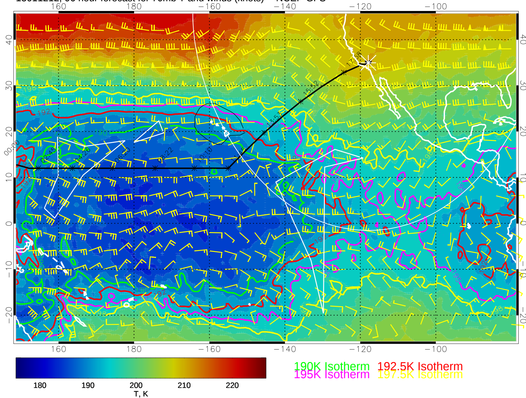
15011212, 96 hour forecast for 70mb T and winds (knots) -- NCEP GFS
