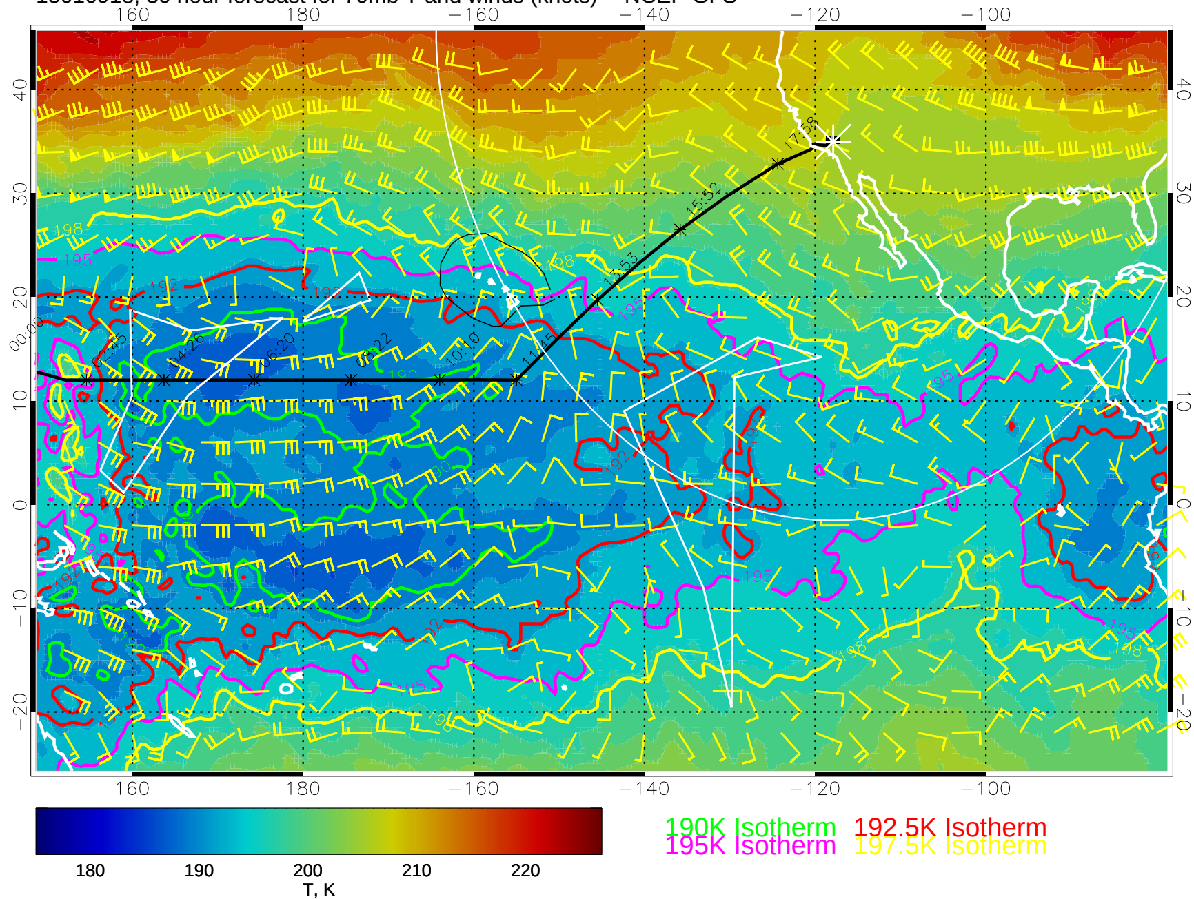
15010918, 30 hour forecast for 70mb T and winds (knots) -- NCEP GFS
