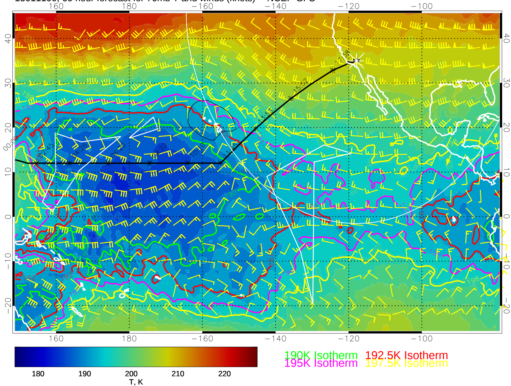
15011100, 60 hour forecast for 70mb T and winds (knots) -- NCEP GFS
