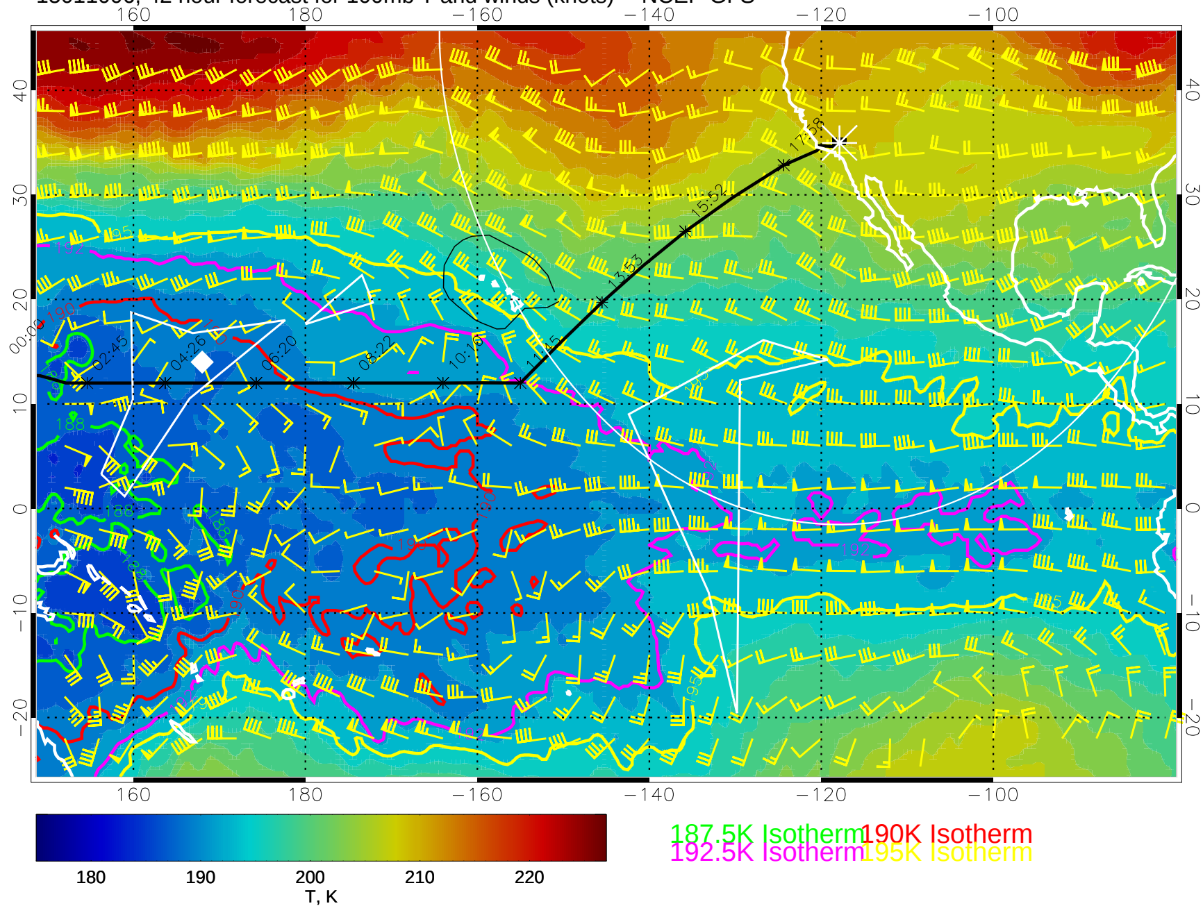
15011006, 42 hour forecast for 100mb T and winds (knots) -- NCEP GFS
