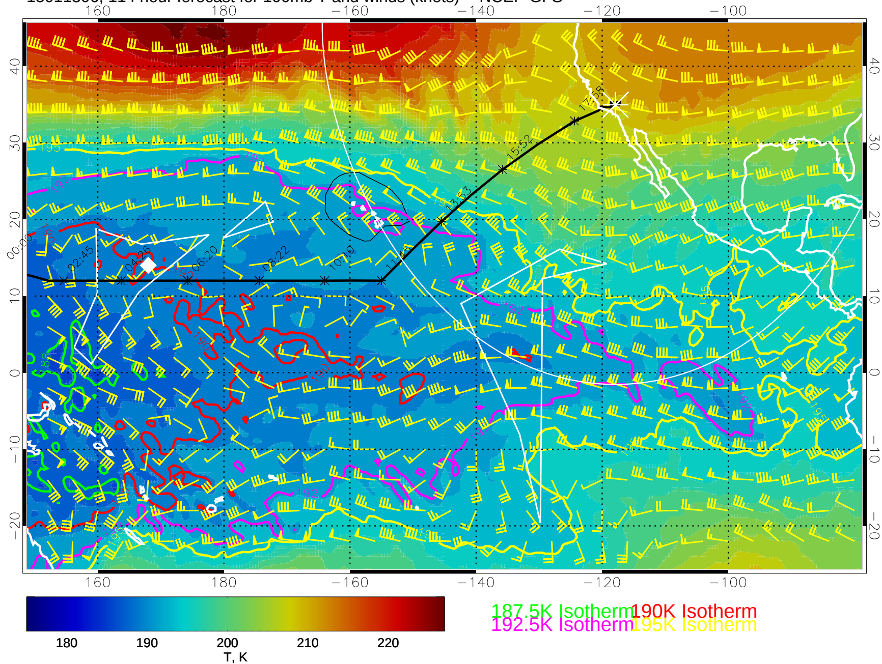
15011306, 114 hour forecast for 100mb T and winds (knots) -- NCEP GFS
