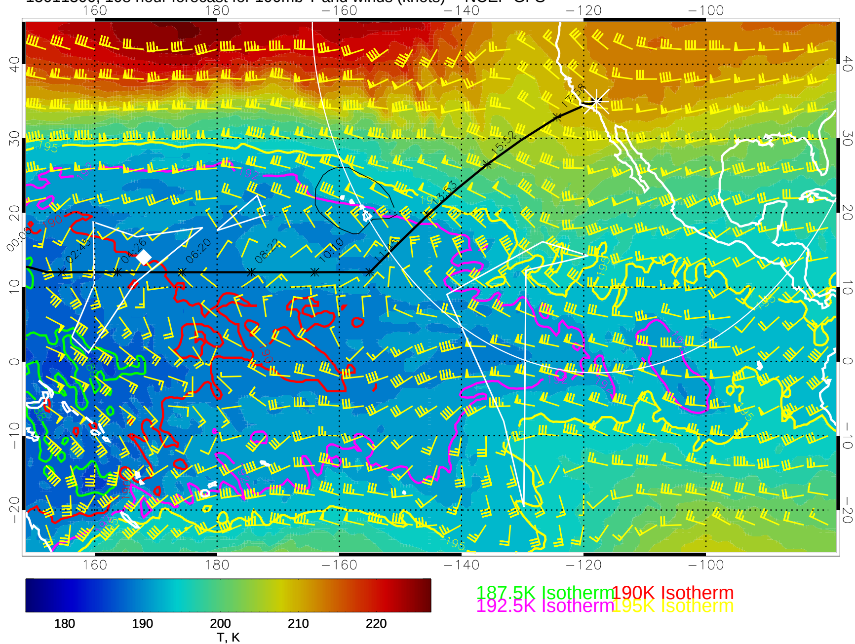
15011300, 108 hour forecast for 100mb T and winds (knots) -- NCEP GFS
