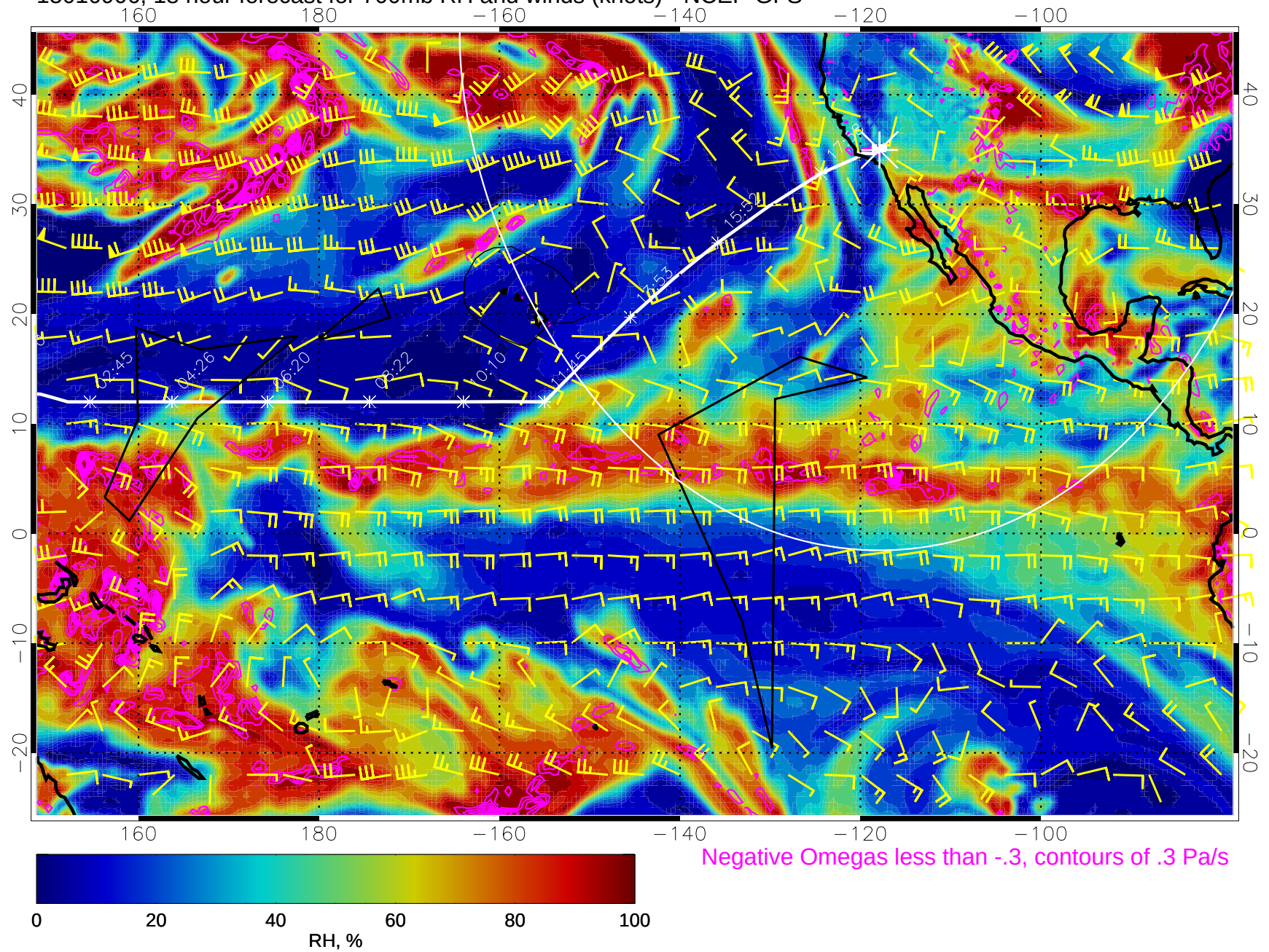
15010906, 18 hour forecast for 700mb RH and winds (knots) - NCEP GFS
