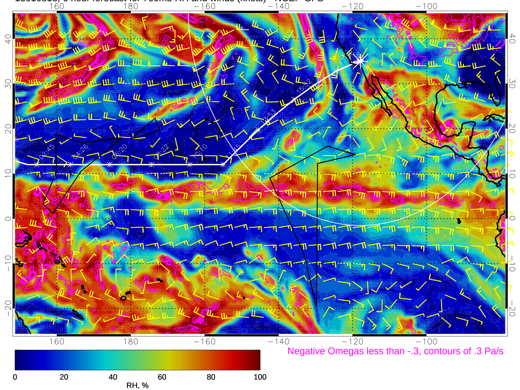
15010818, 6 hour forecast for 700mb RH and winds (knots) - NCEP GFS
