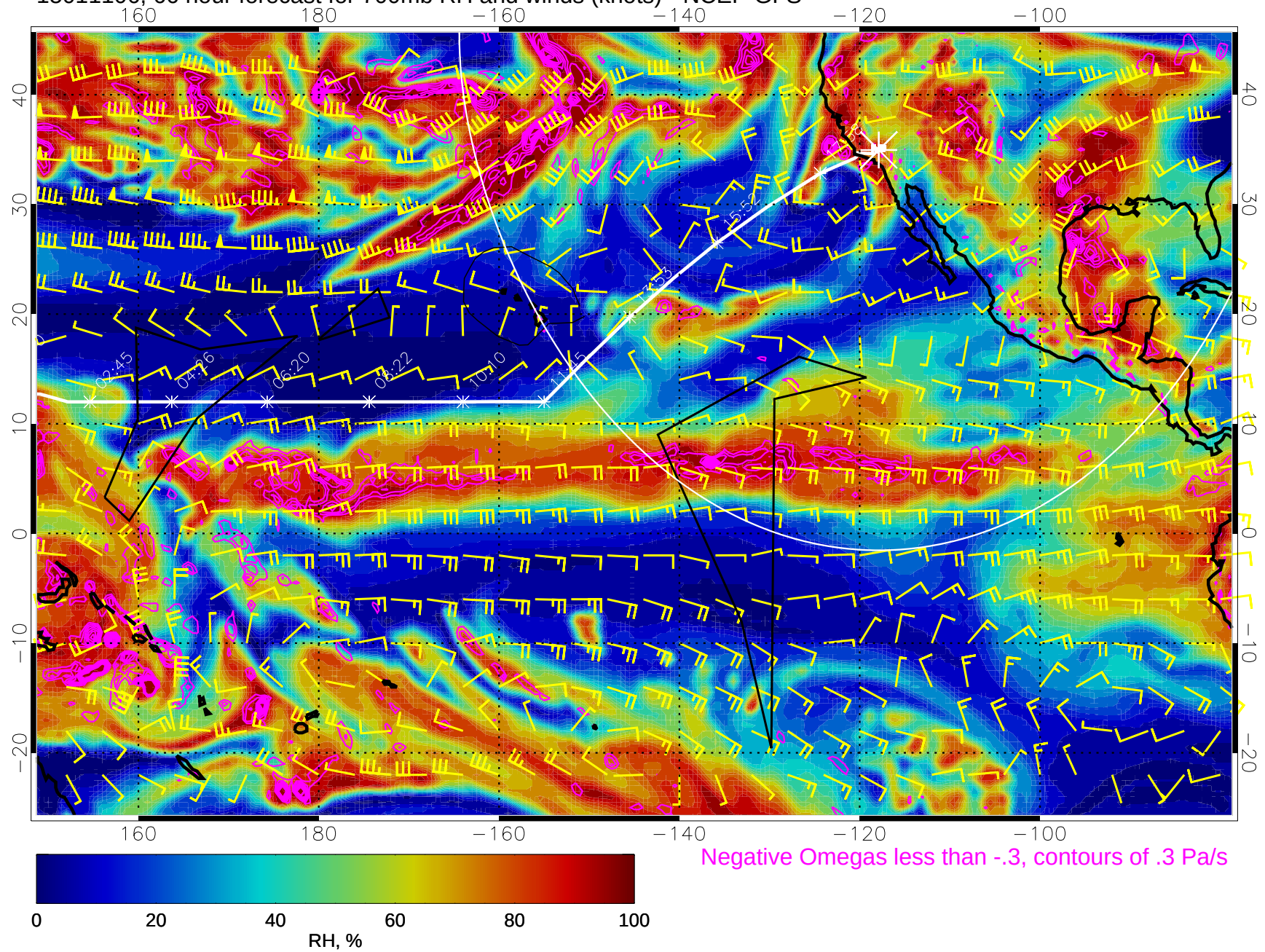
15011106, 66 hour forecast for 700mb RH and winds (knots) - NCEP GFS
