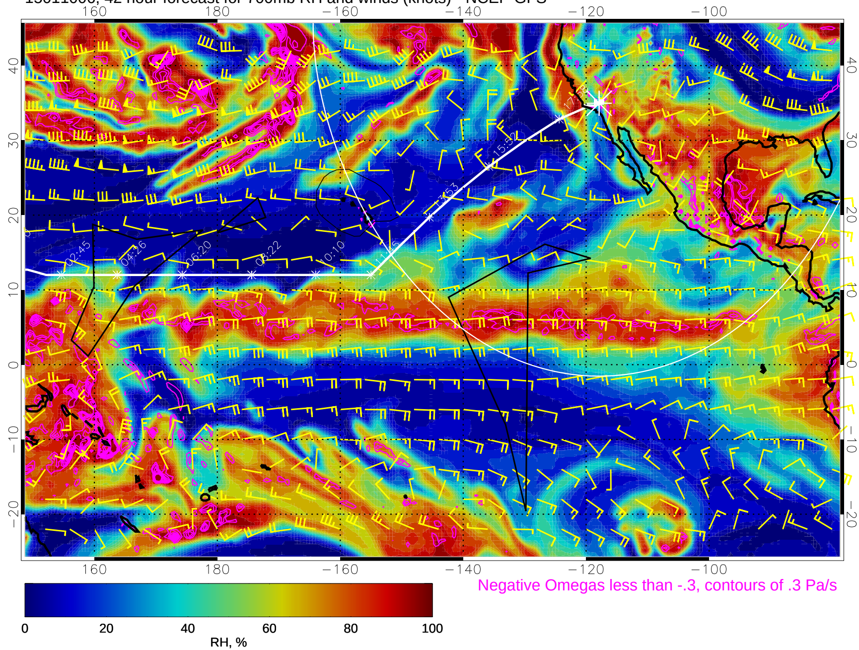
15011006, 42 hour forecast for 700mb RH and winds (knots) - NCEP GFS
