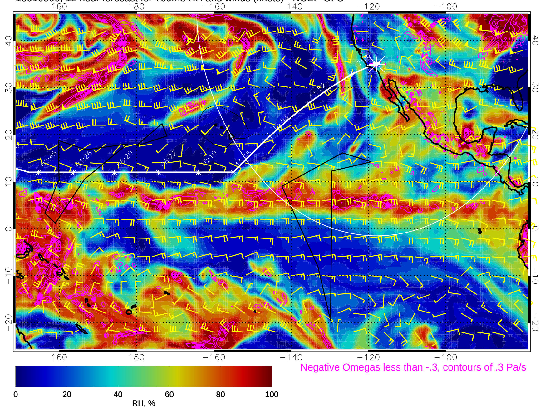
15010900, 12 hour forecast for 700mb RH and winds (knots) - NCEP GFS
