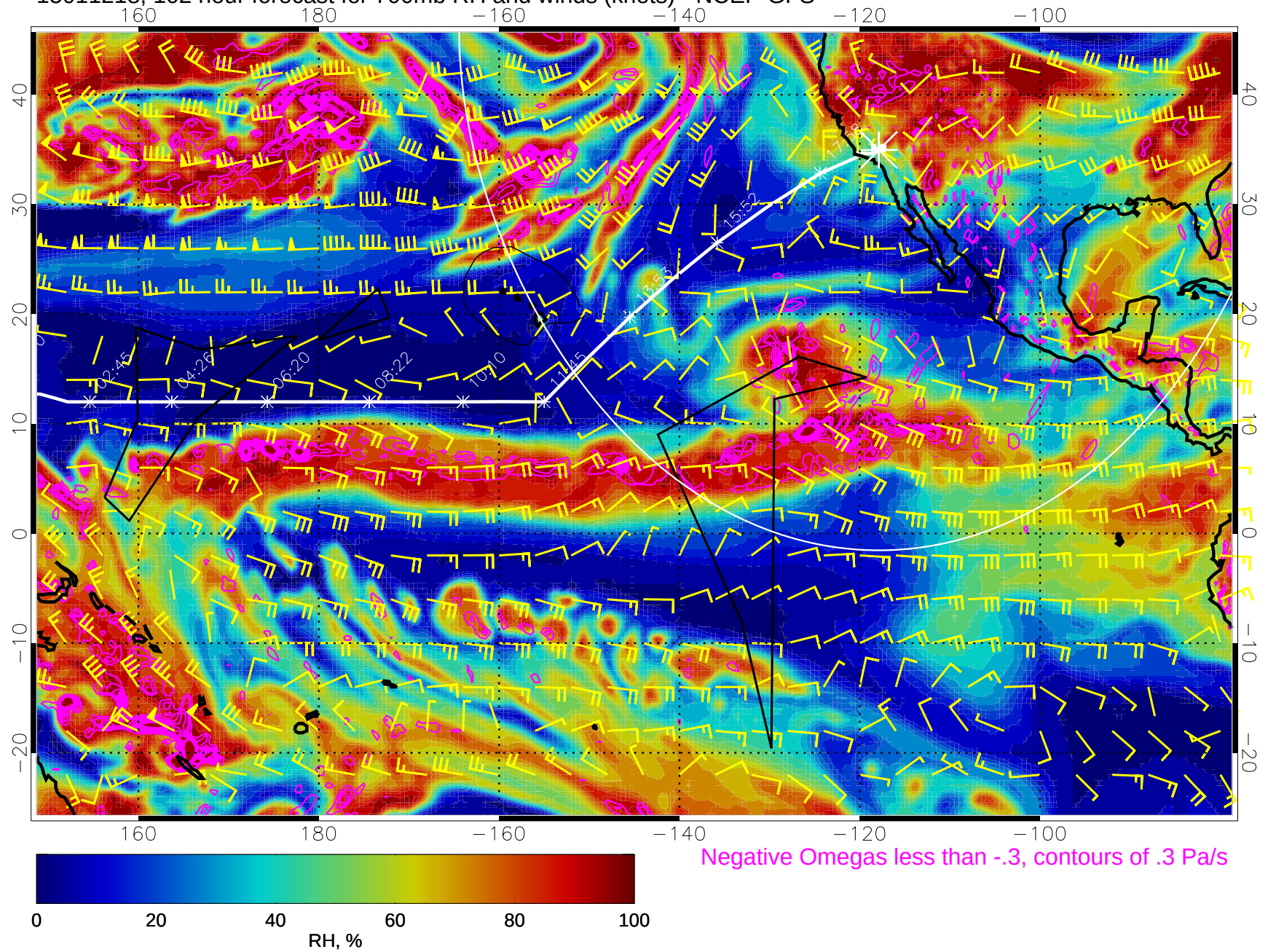
15011218, 102 hour forecast for 700mb RH and winds (knots) - NCEP GFS
