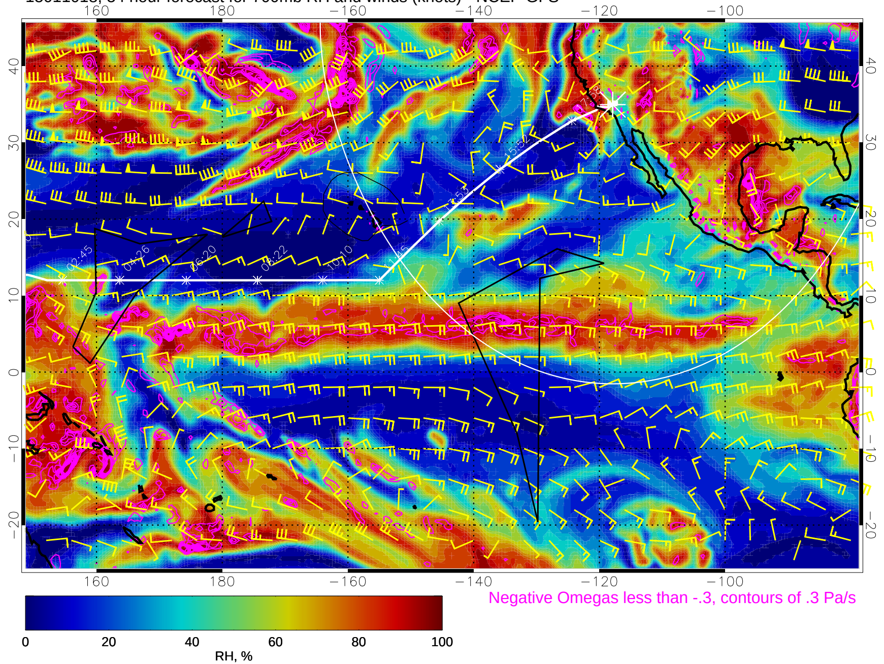
15011018, 54 hour forecast for 700mb RH and winds (knots) - NCEP GFS
