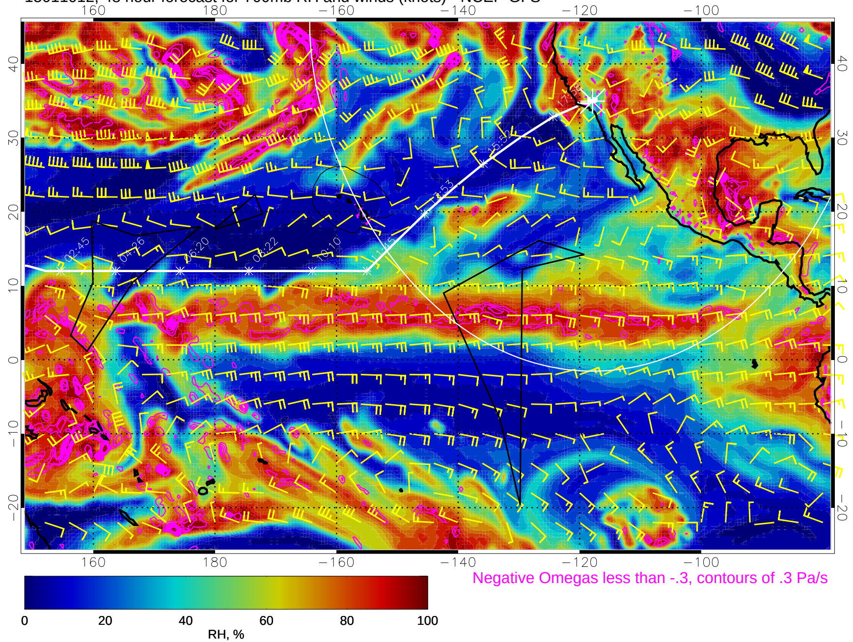
15011012, 48 hour forecast for 700mb RH and winds (knots) - NCEP GFS
