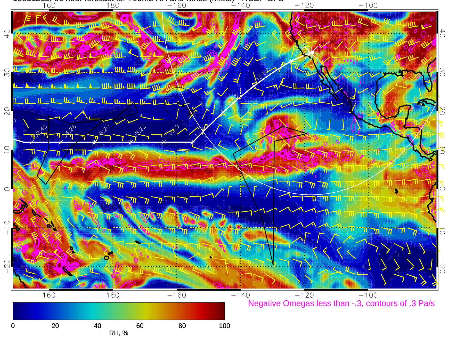
15011212, 96 hour forecast for 700mb RH and winds (knots) - NCEP GFS
