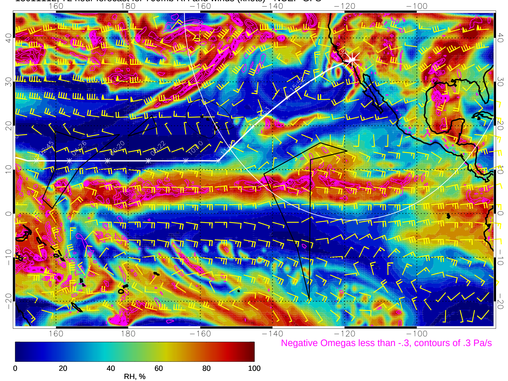
15011112, 72 hour forecast for 700mb RH and winds (knots) - NCEP GFS
