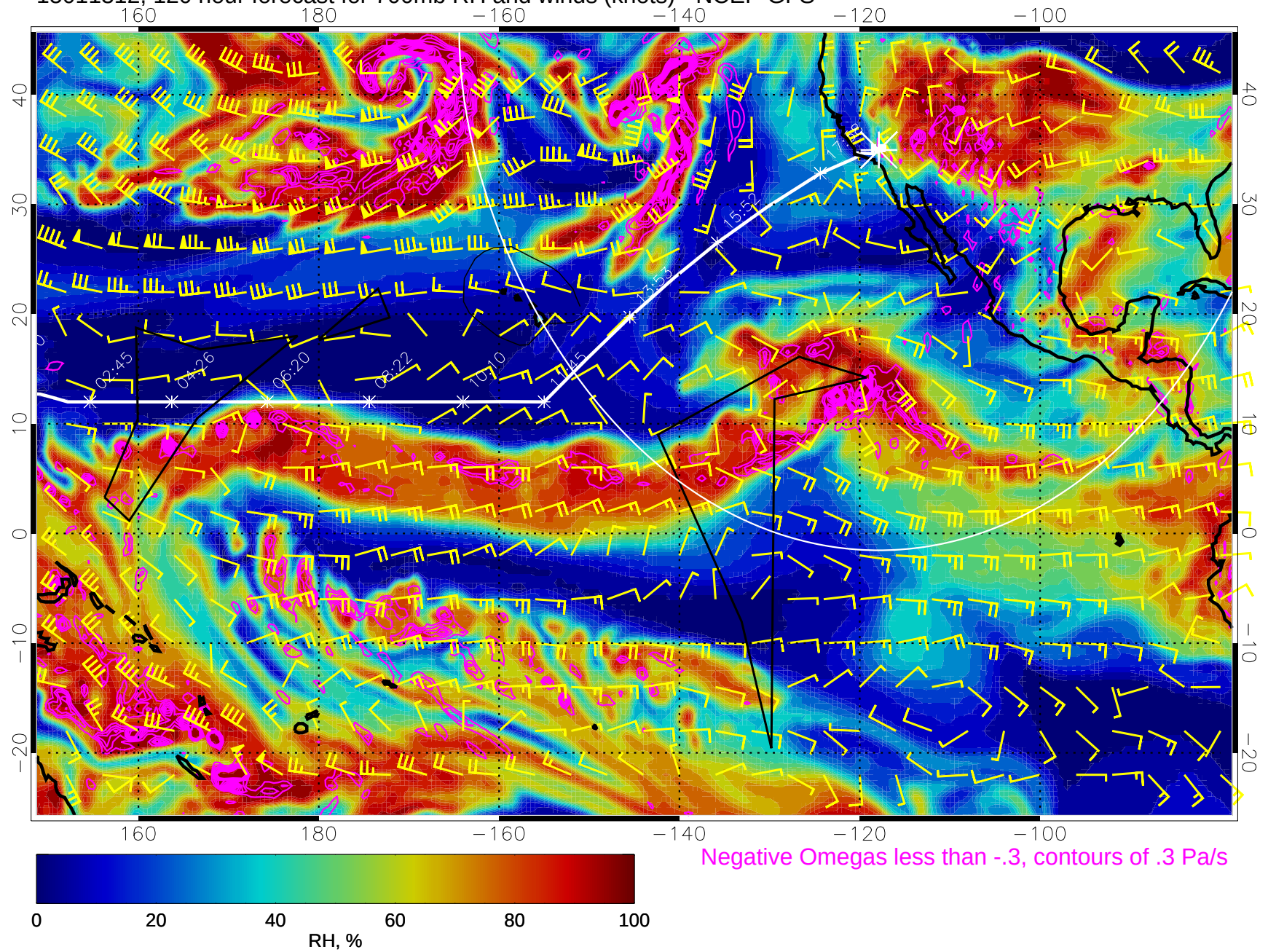
15011312, 120 hour forecast for 700mb RH and winds (knots) - NCEP GFS
