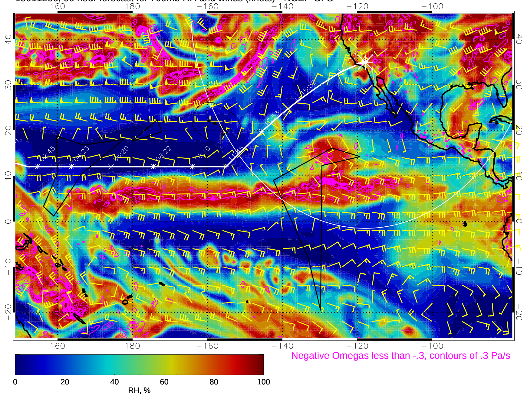
15011206, 90 hour forecast for 700mb RH and winds (knots) - NCEP GFS
