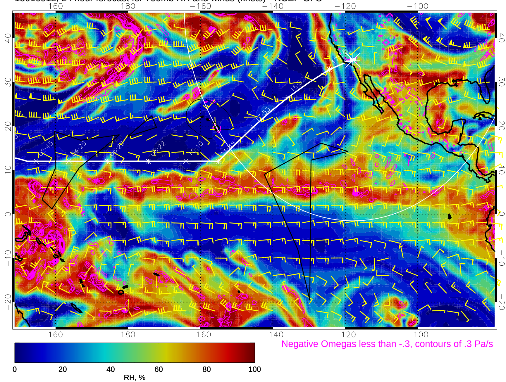
15010912, 24 hour forecast for 700mb RH and winds (knots) - NCEP GFS
