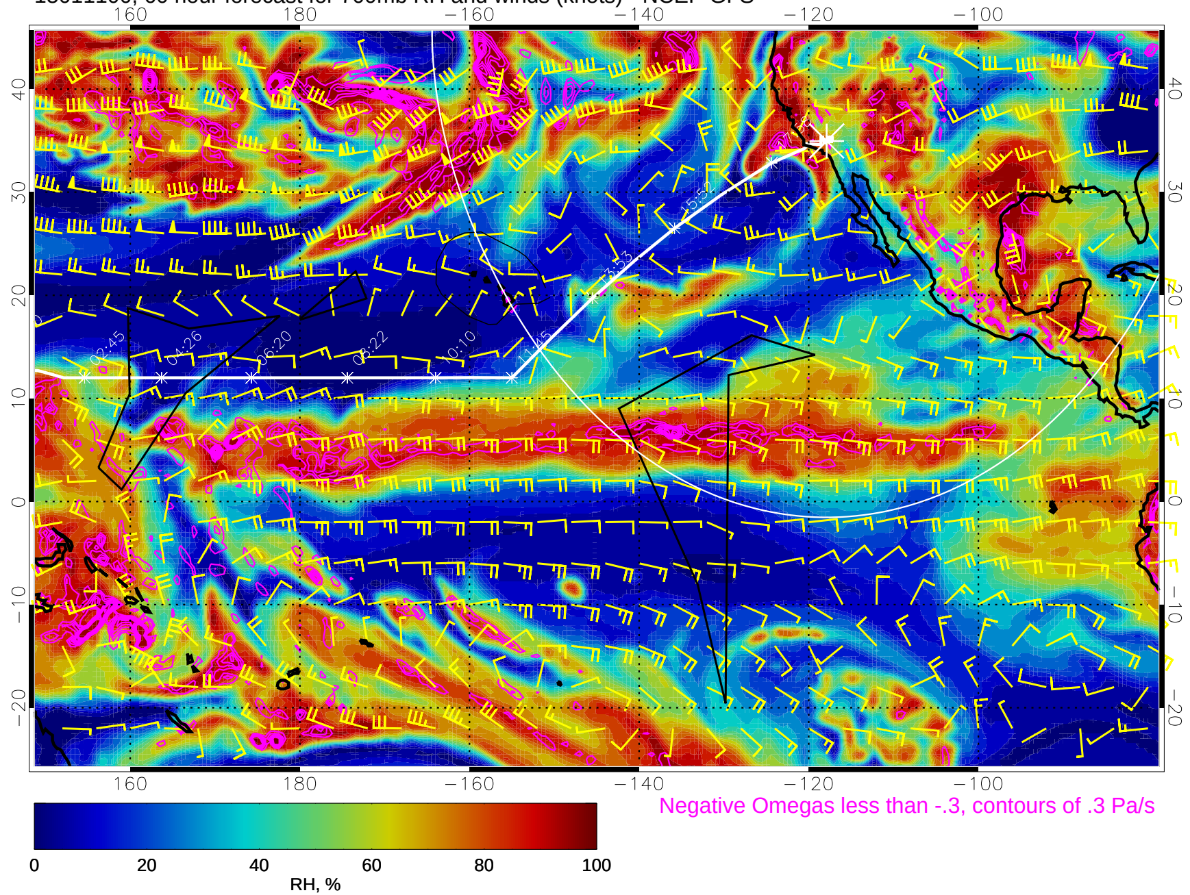
15011100, 60 hour forecast for 700mb RH and winds (knots) - NCEP GFS
