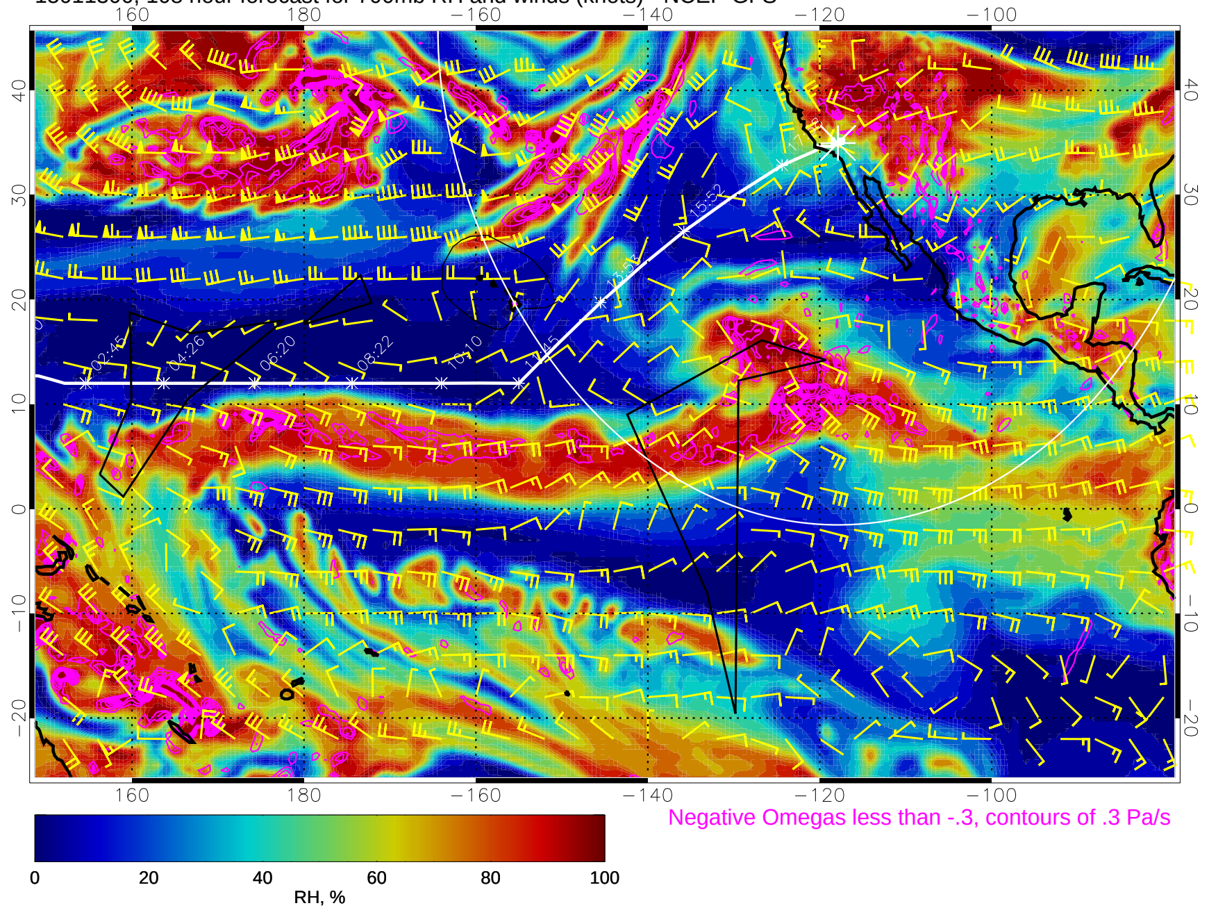
15011300, 108 hour forecast for 700mb RH and winds (knots) - NCEP GFS
