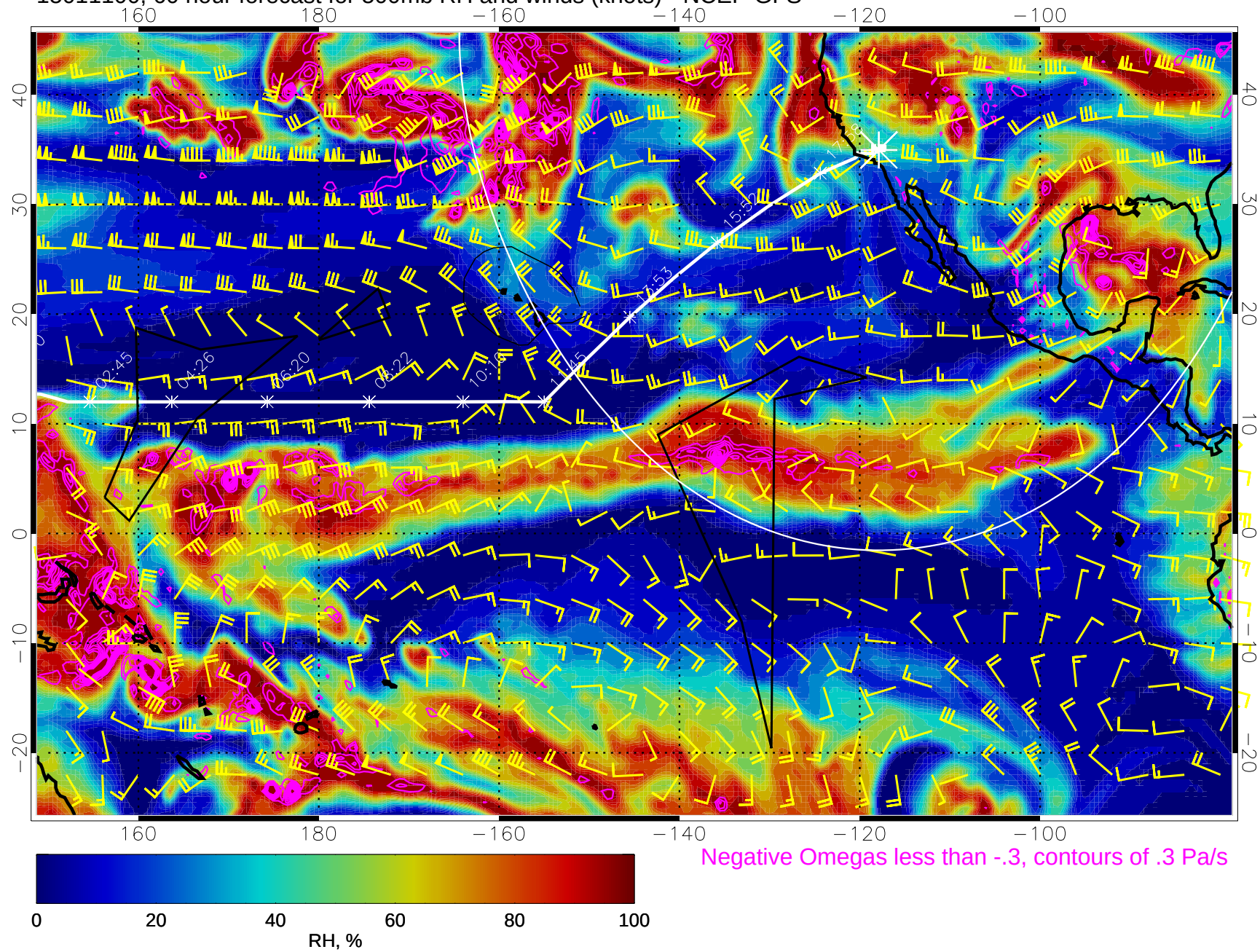
15011100, 60 hour forecast for 500mb RH and winds (knots) - NCEP GFS
