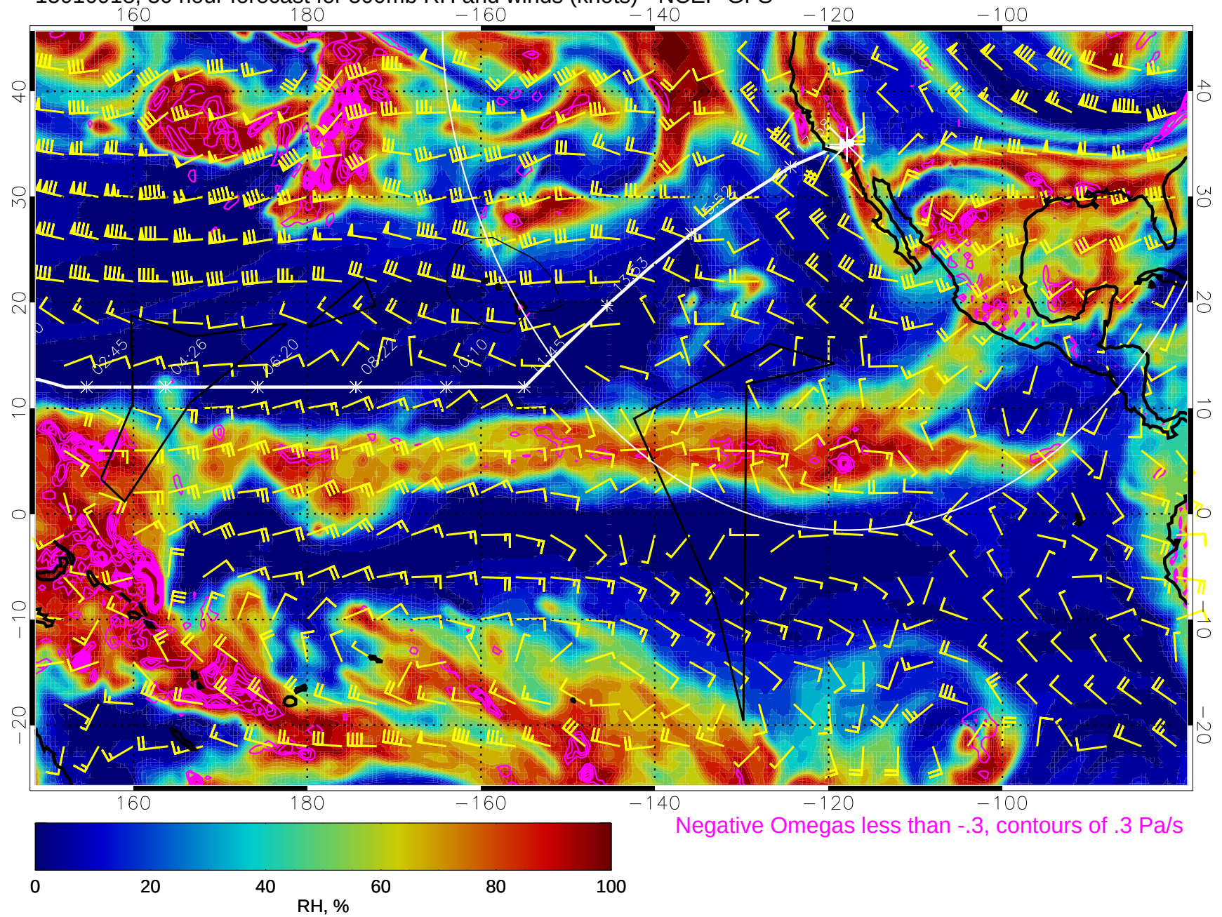
15010918, 30 hour forecast for 500mb RH and winds (knots) - NCEP GFS
