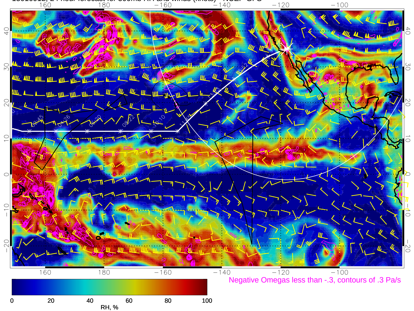
15010912, 24 hour forecast for 500mb RH and winds (knots) - NCEP GFS
