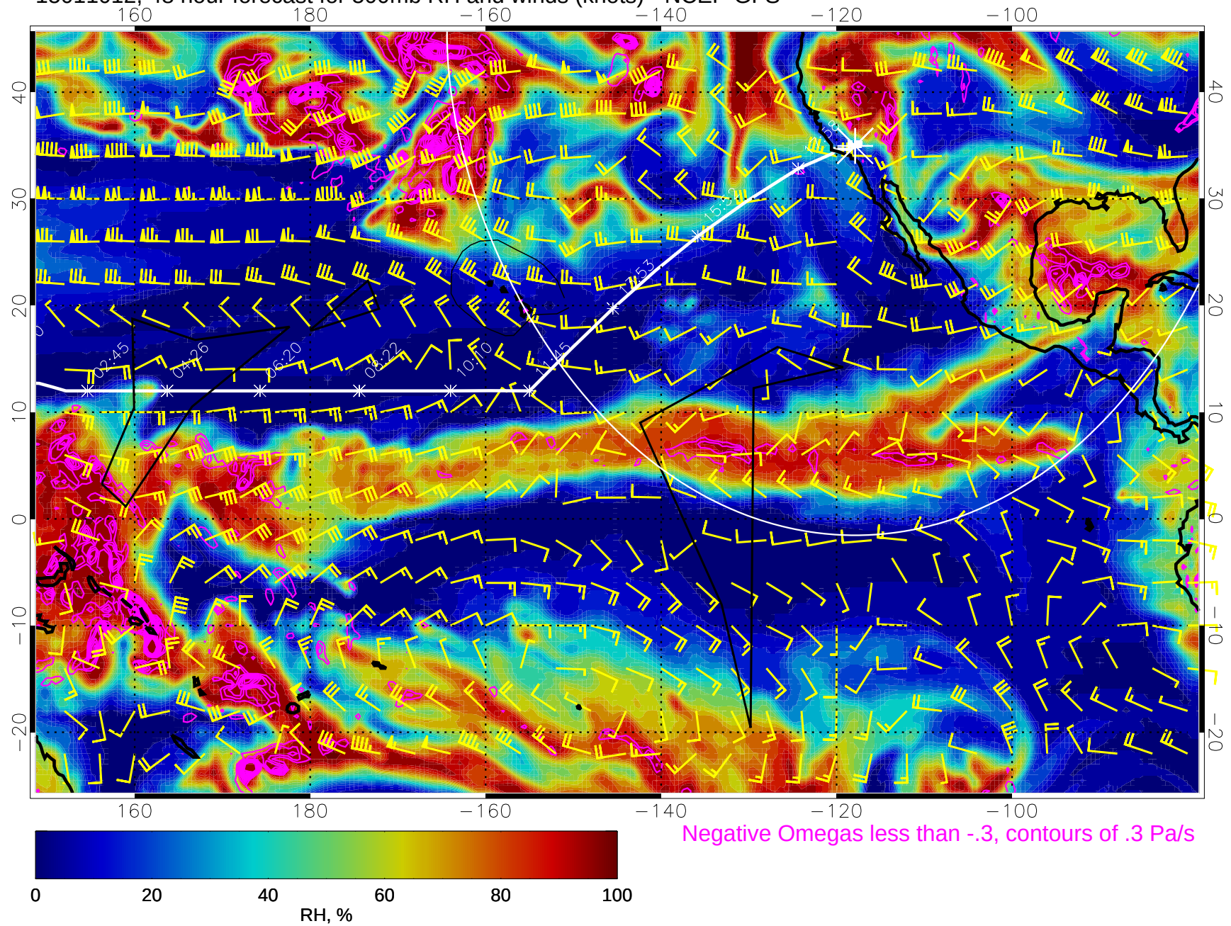
15011012, 48 hour forecast for 500mb RH and winds (knots) - NCEP GFS
