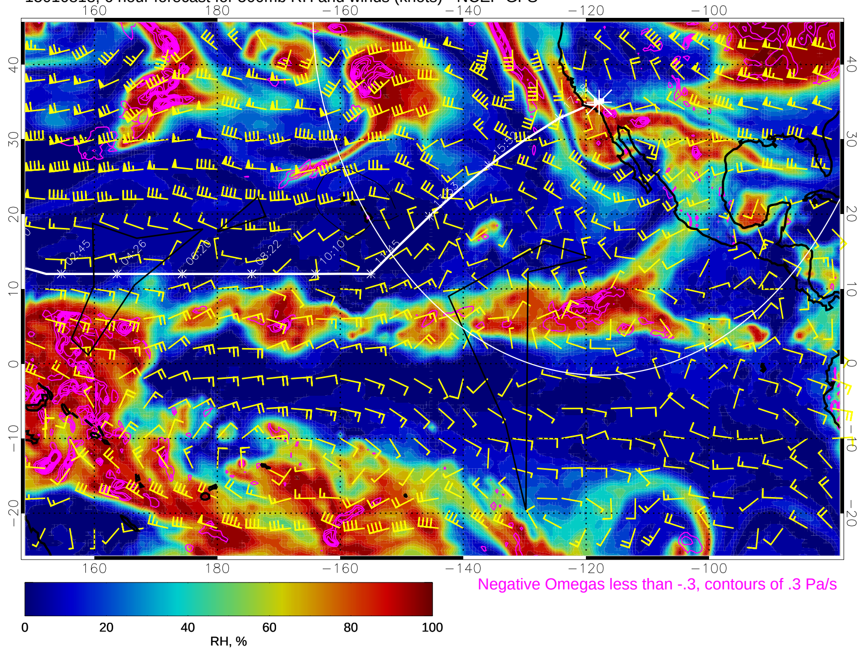
15010818, 6 hour forecast for 500mb RH and winds (knots) - NCEP GFS
