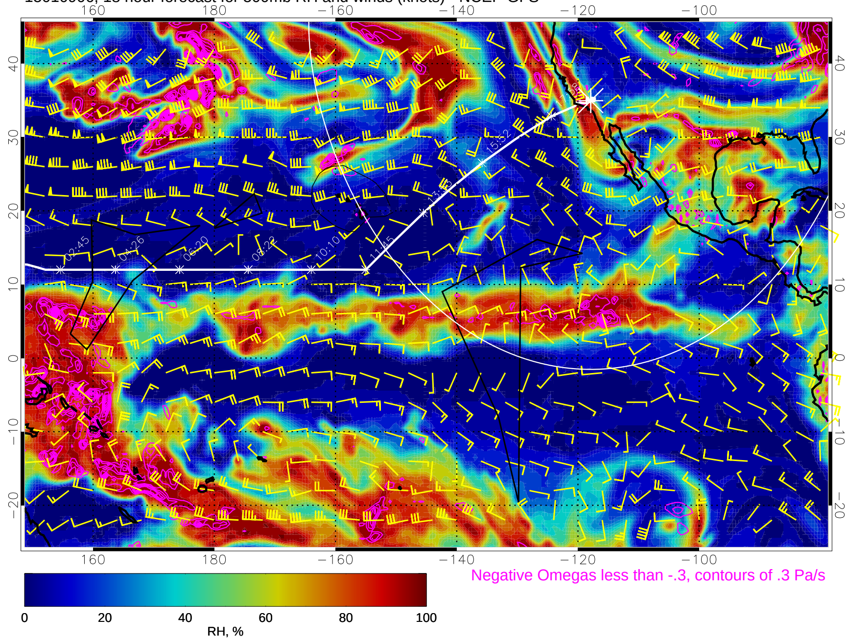
15010906, 18 hour forecast for 500mb RH and winds (knots) - NCEP GFS
