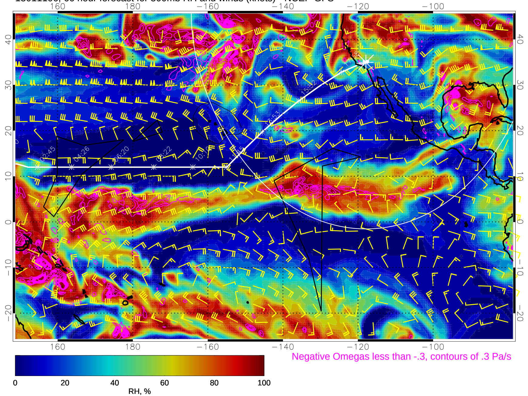
15011106, 66 hour forecast for 500mb RH and winds (knots) - NCEP GFS
