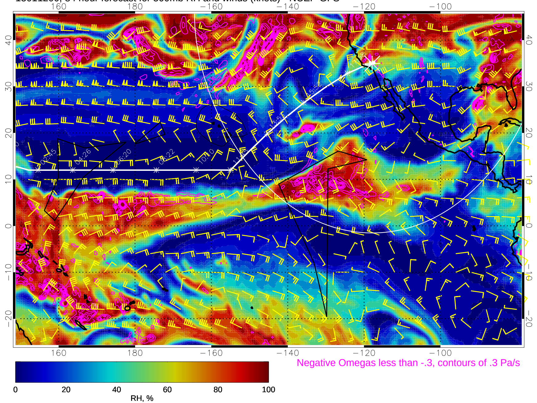
15011200, 84 hour forecast for 500mb RH and winds (knots) - NCEP GFS
