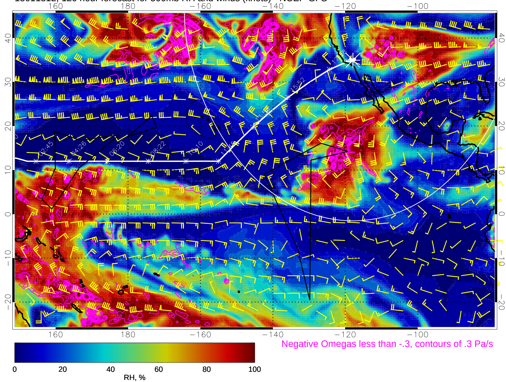
15011312, 120 hour forecast for 500mb RH and winds (knots) - NCEP GFS
