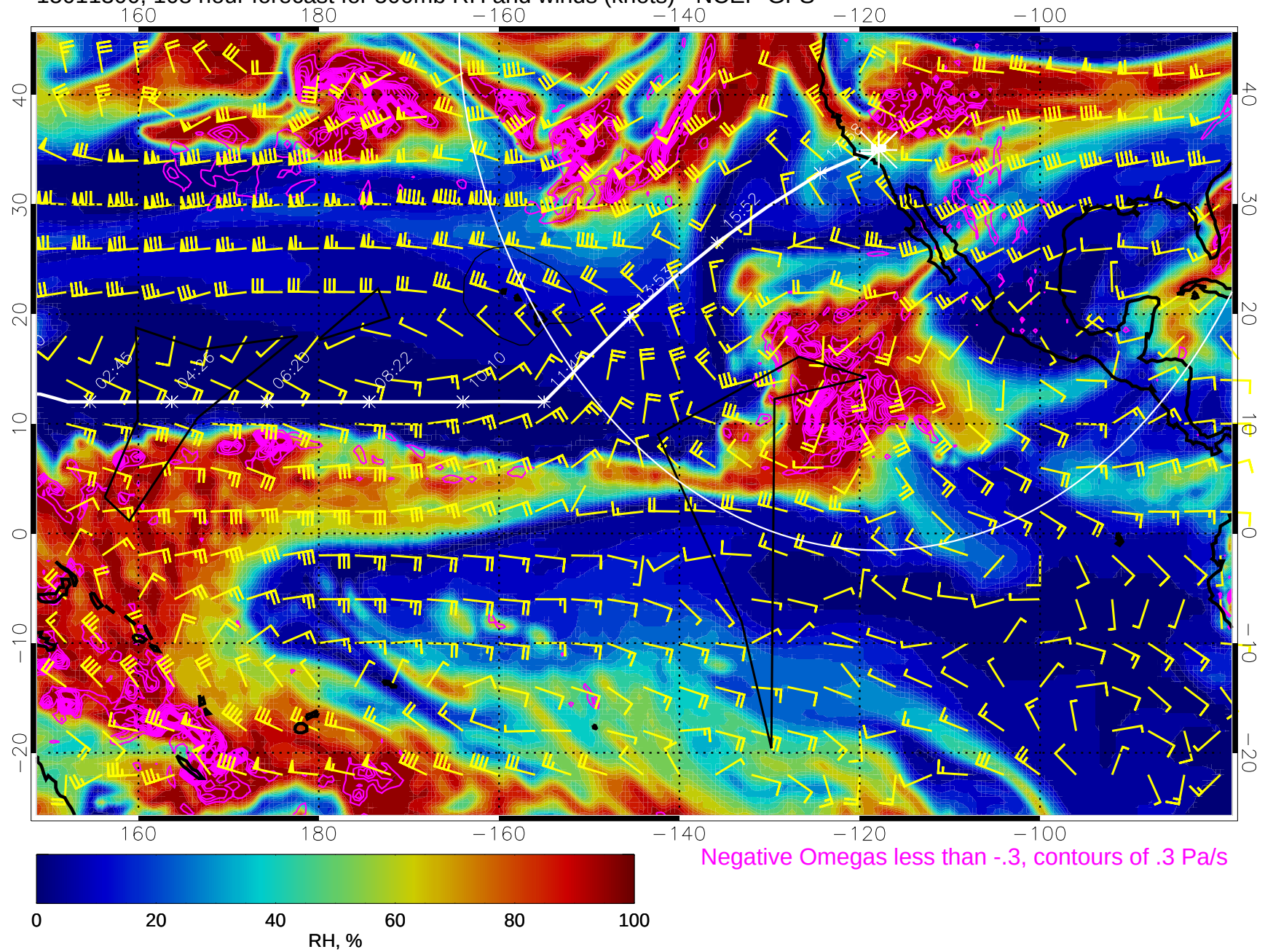
15011300, 108 hour forecast for 500mb RH and winds (knots) - NCEP GFS
