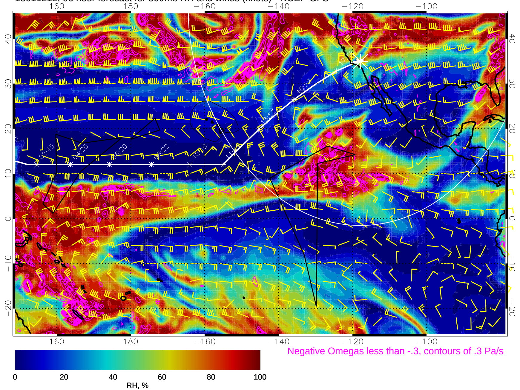
15011212, 96 hour forecast for 500mb RH and winds (knots) - NCEP GFS
