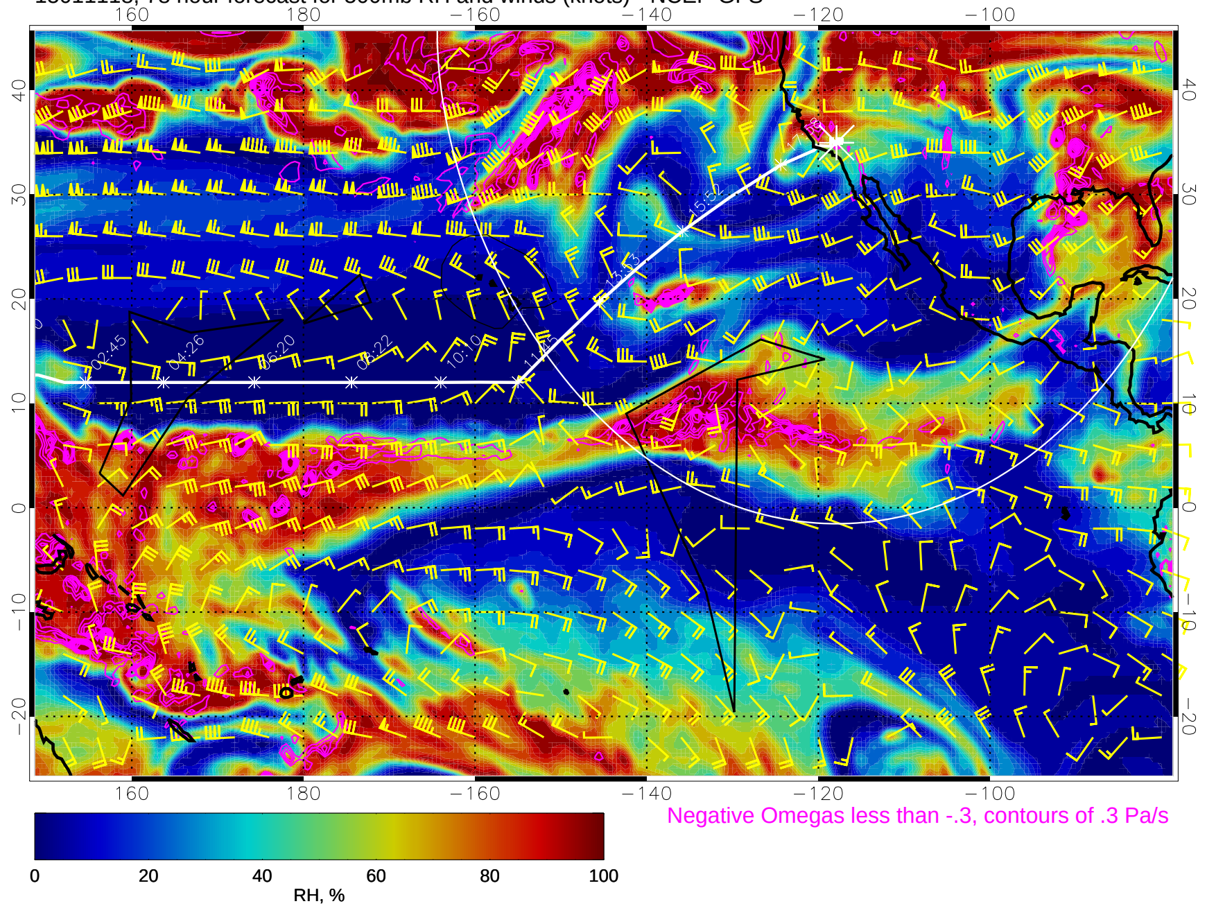
15011118, 78 hour forecast for 500mb RH and winds (knots) - NCEP GFS
