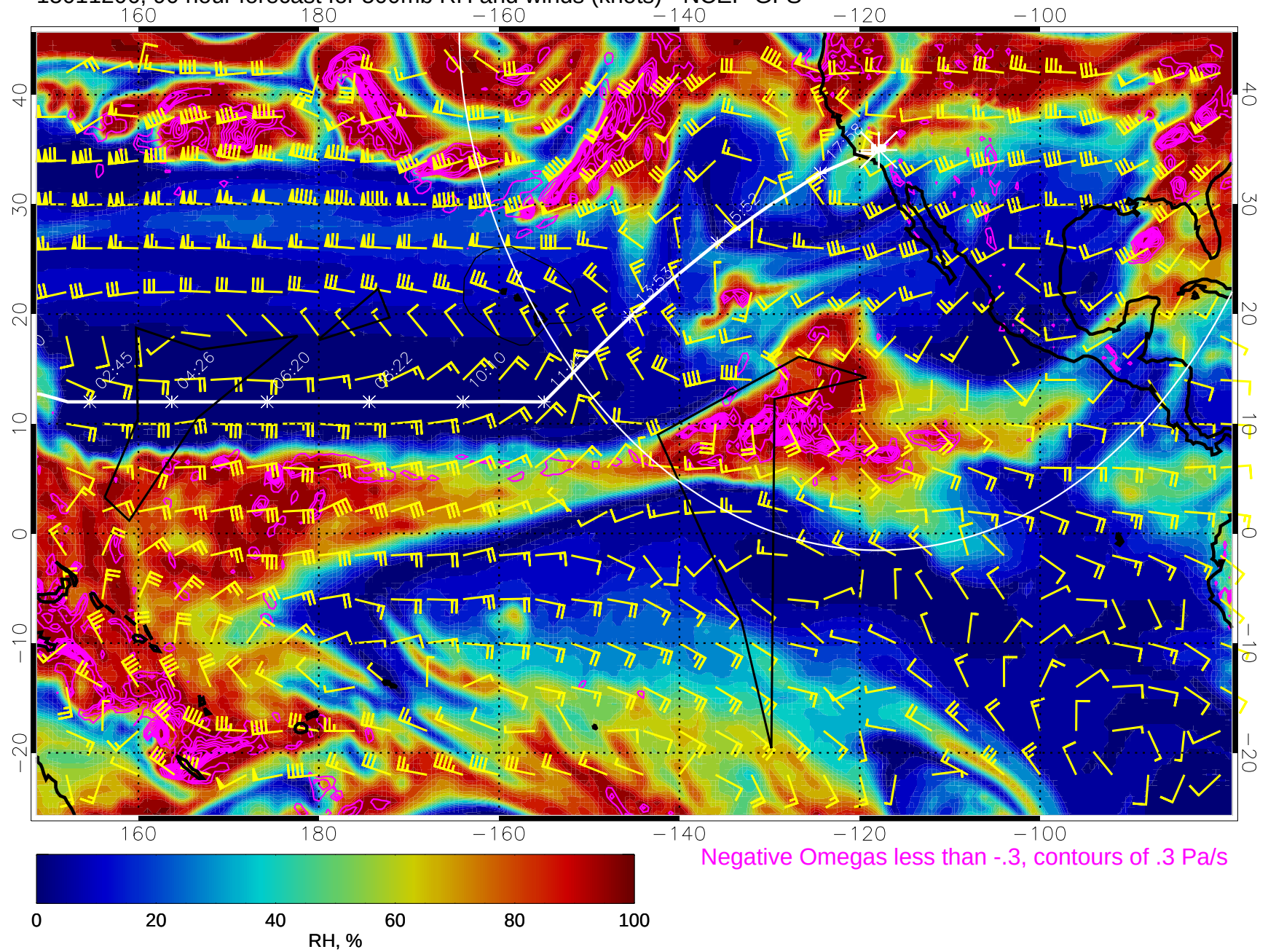
15011206, 90 hour forecast for 500mb RH and winds (knots) - NCEP GFS
