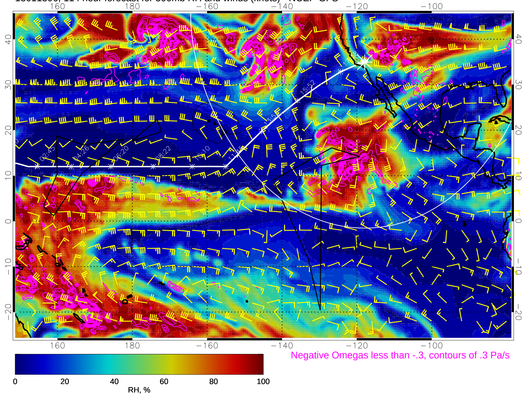
15011306, 114 hour forecast for 500mb RH and winds (knots) - NCEP GFS
