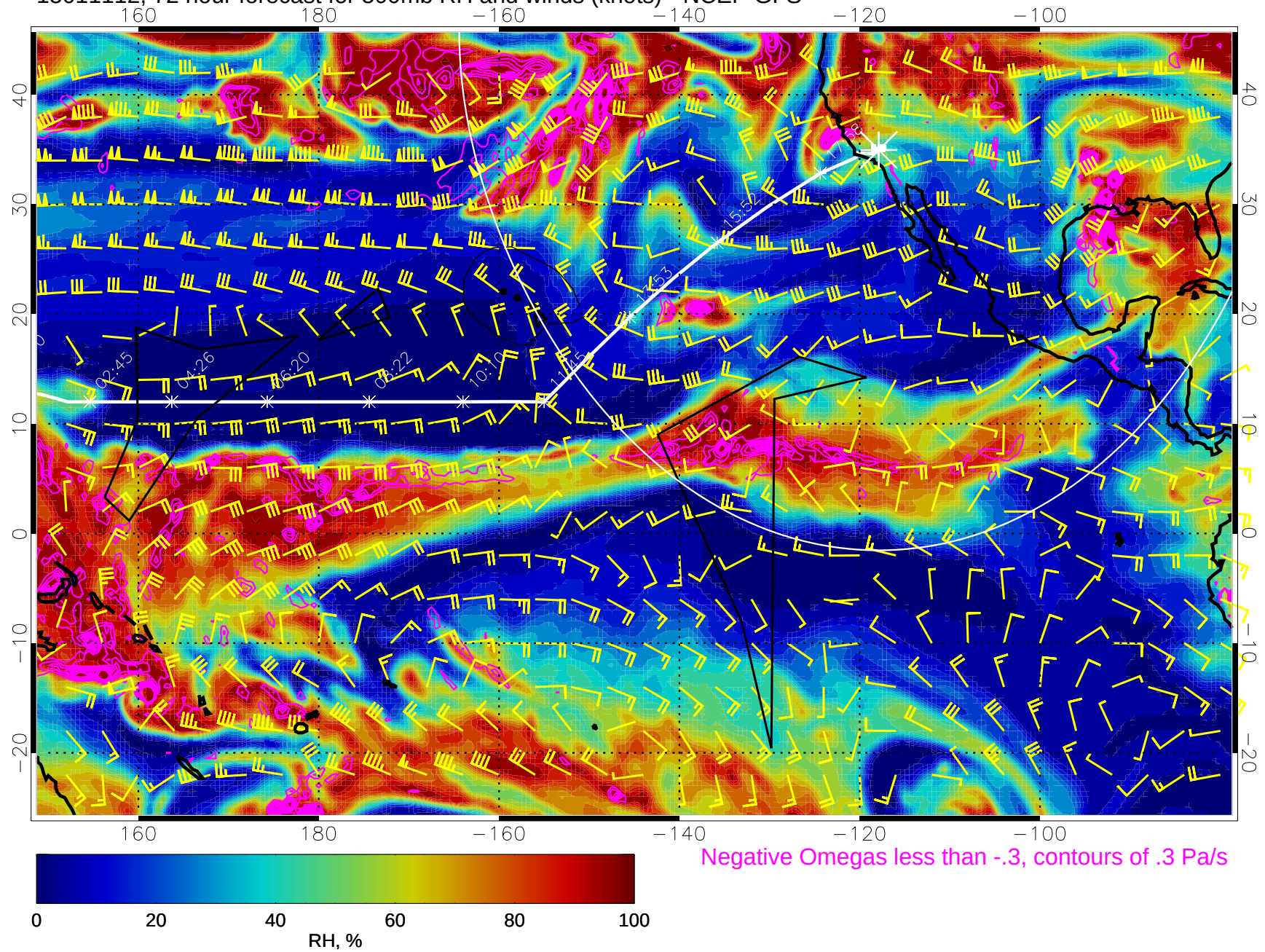
15011112, 72 hour forecast for 500mb RH and winds (knots) - NCEP GFS
