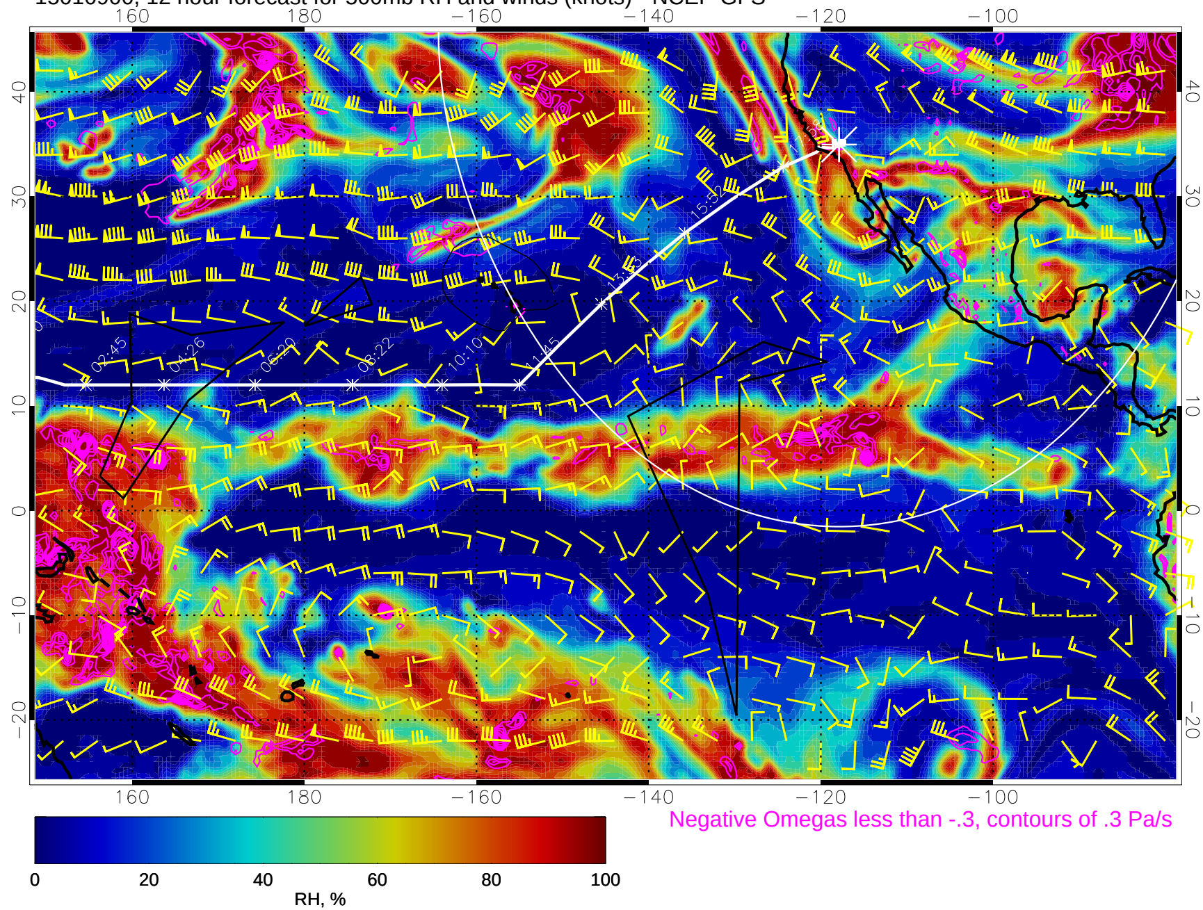
15010900, 12 hour forecast for 500mb RH and winds (knots) - NCEP GFS
