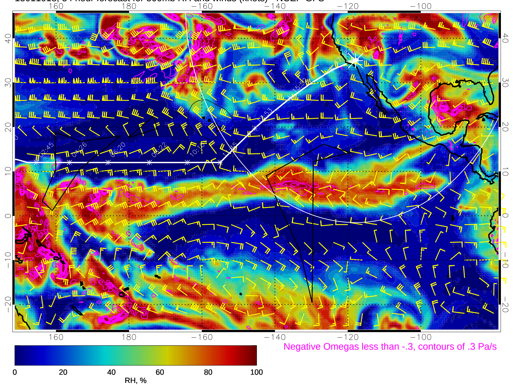
15011018, 54 hour forecast for 500mb RH and winds (knots) - NCEP GFS
