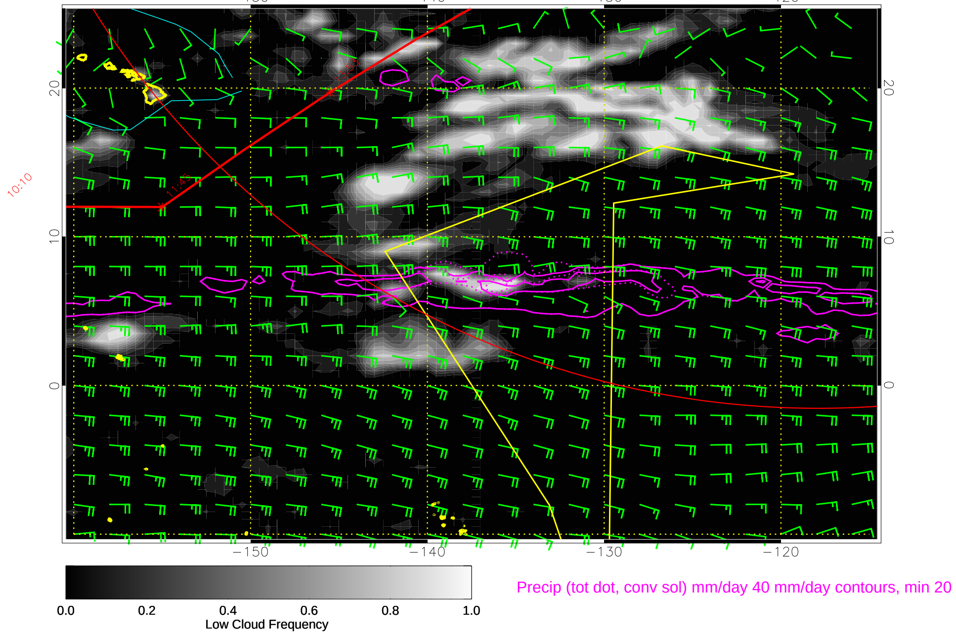
15011106, 66 hour forecast for 850mb winds (knots) and Low Cloud Frequency -- NCEP GFS
