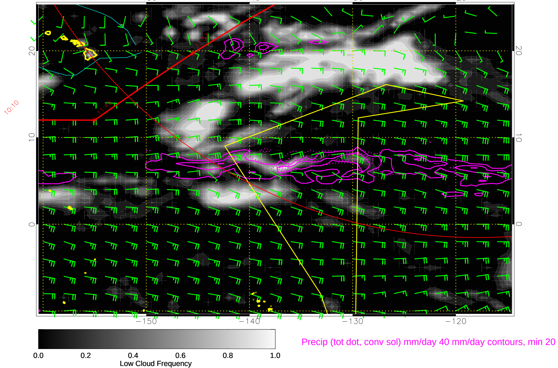
15011112, 72 hour forecast for 850mb winds (knots) and Low Cloud Frequency -- NCEP GFS
