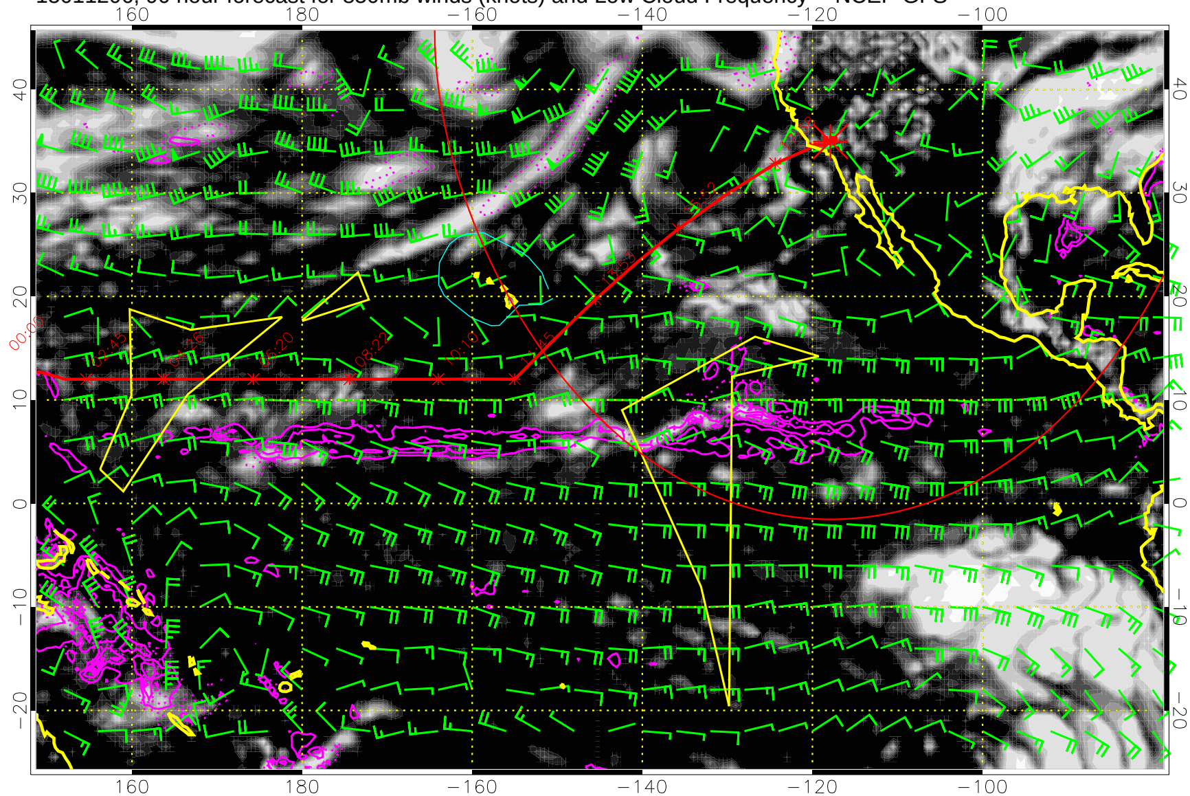
15011206, 90 hour forecast for 850mb winds (knots) and Low Cloud Frequency -- NCEP GFS
