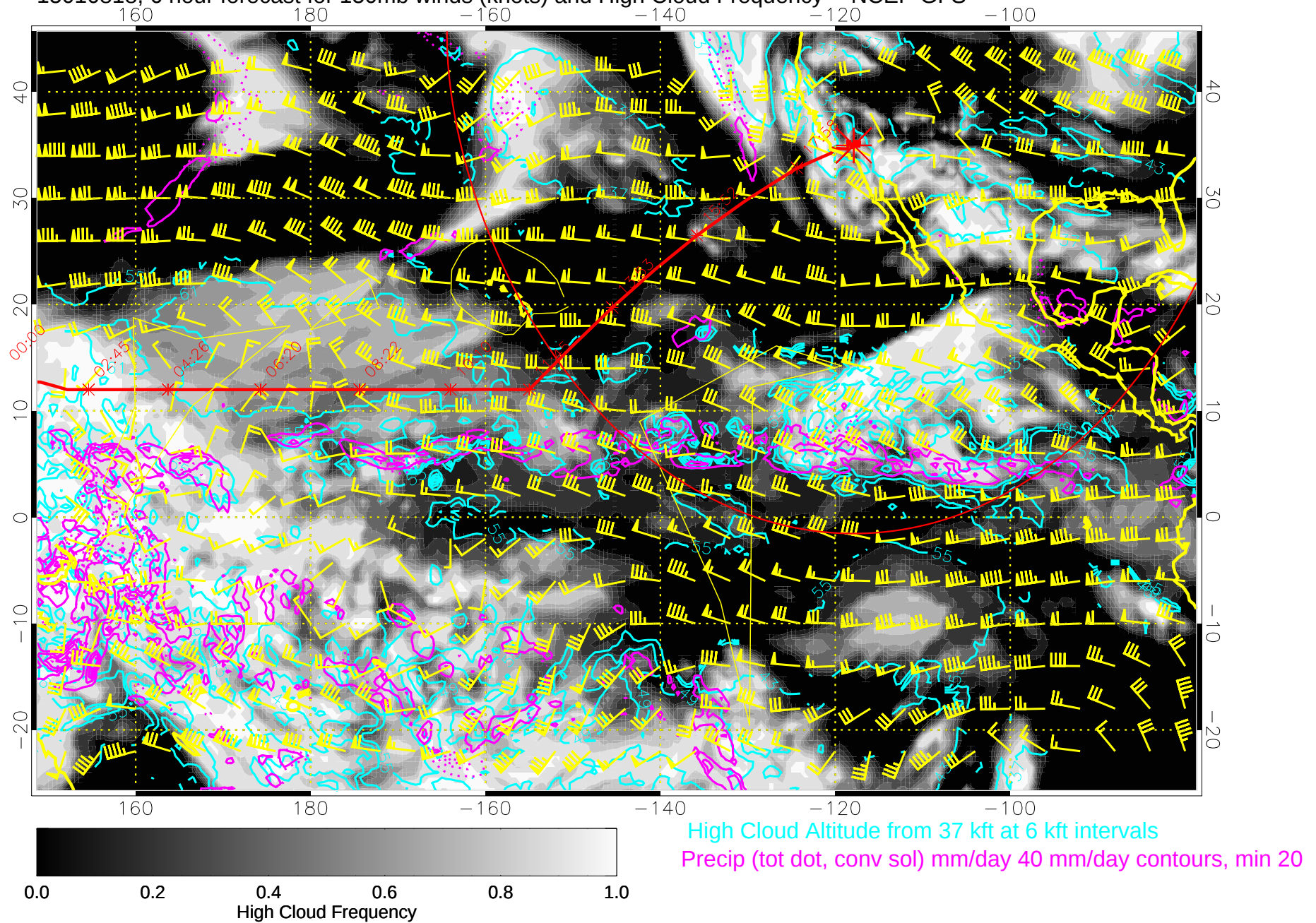
15010818, 6 hour forecast for 150mb winds (knots) and High Cloud Frequency -- NCEP GFS
