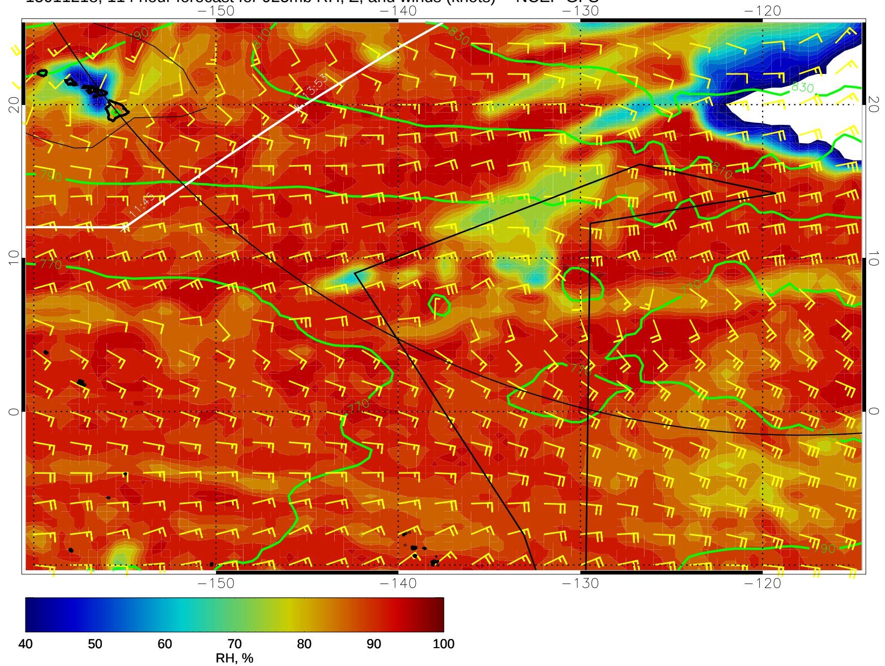
15011218, 114 hour forecast for 925mb RH, Z, and winds (knots) -- NCEP GFS
