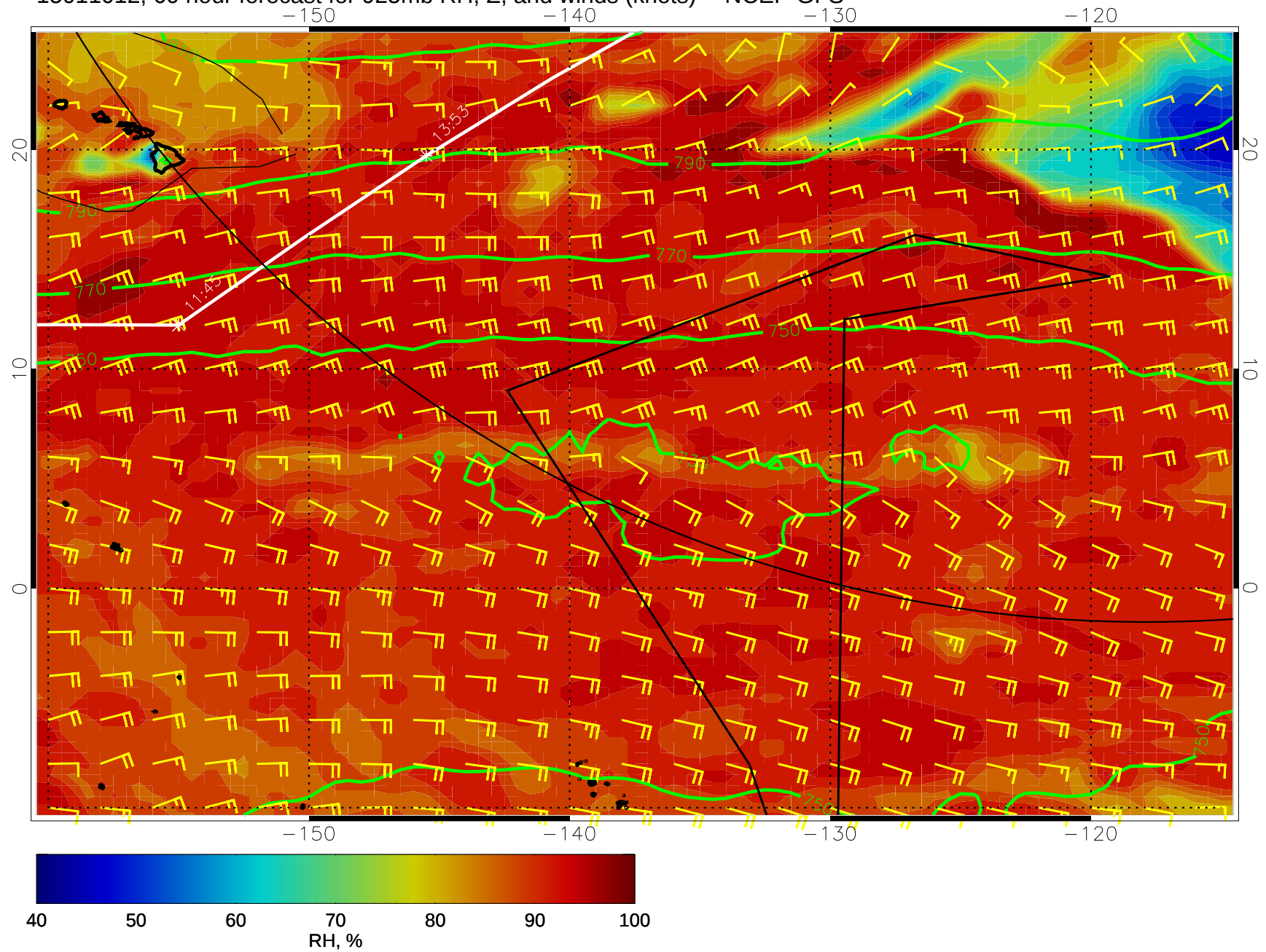
15011012, 60 hour forecast for 925mb RH, Z, and winds (knots) -- NCEP GFS
