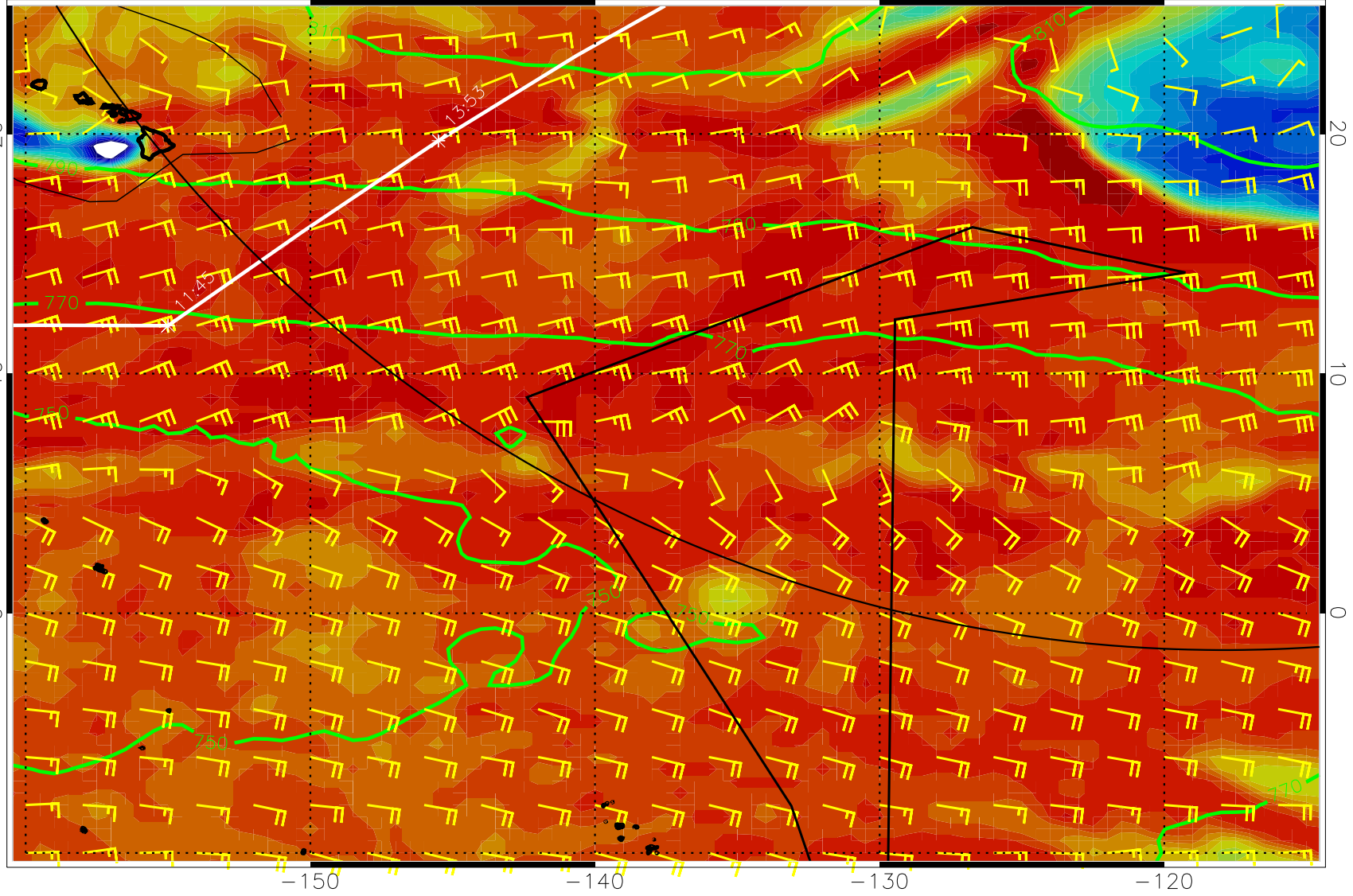
East for elements A, B, and C (km/s) \sim 150 \sim 140 \sim 130 \sim 120
