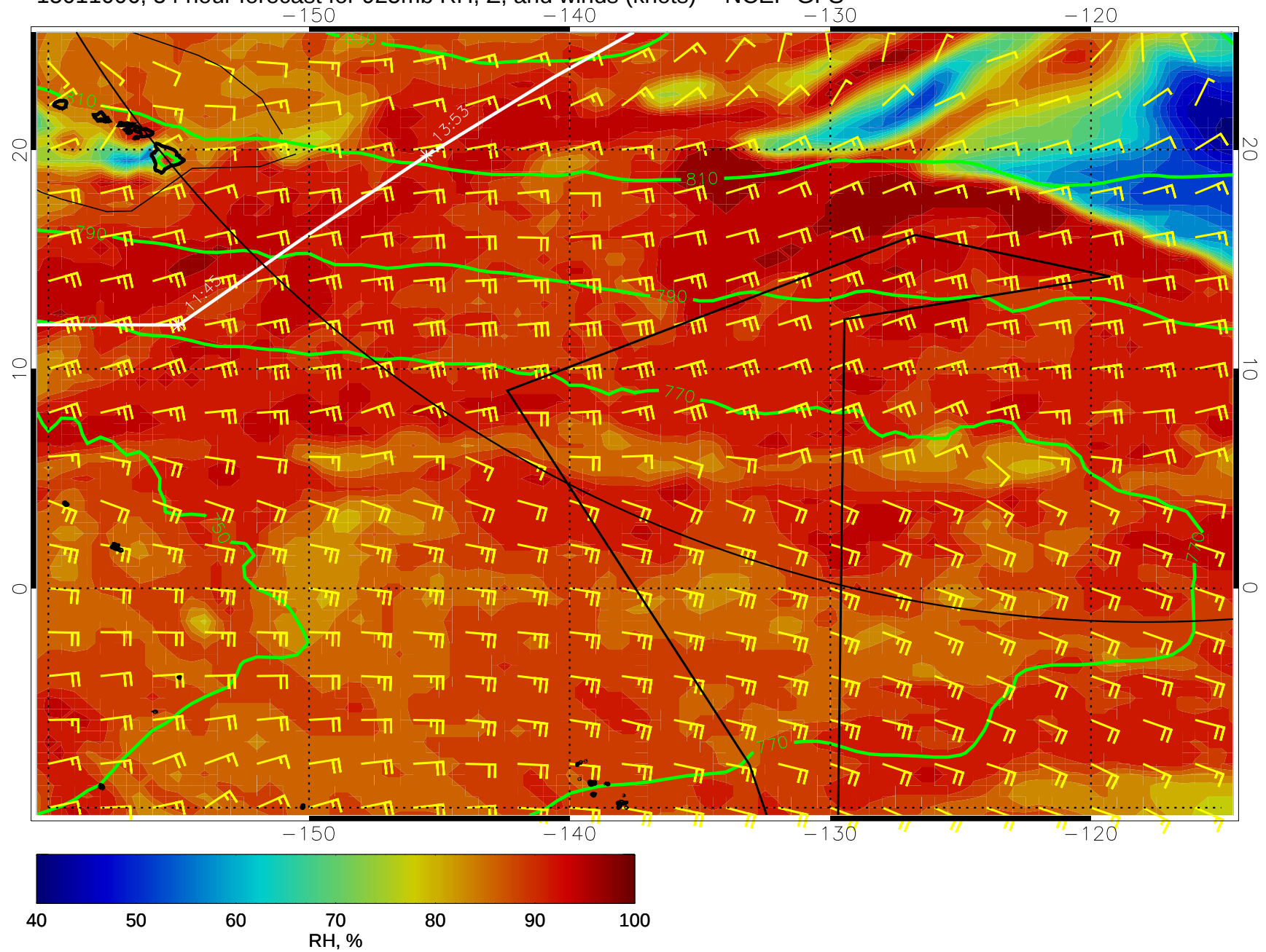
15011006, 54 hour forecast for 925mb RH, Z, and winds (knots) -- NCEP GFS
