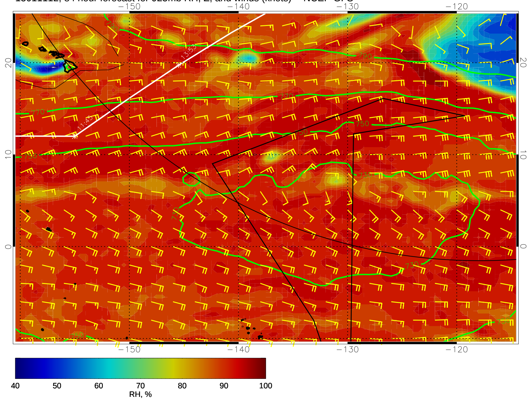
15011112, 84 hour forecast for 925mb RH, Z, and winds (knots) -- NCEP GFS
