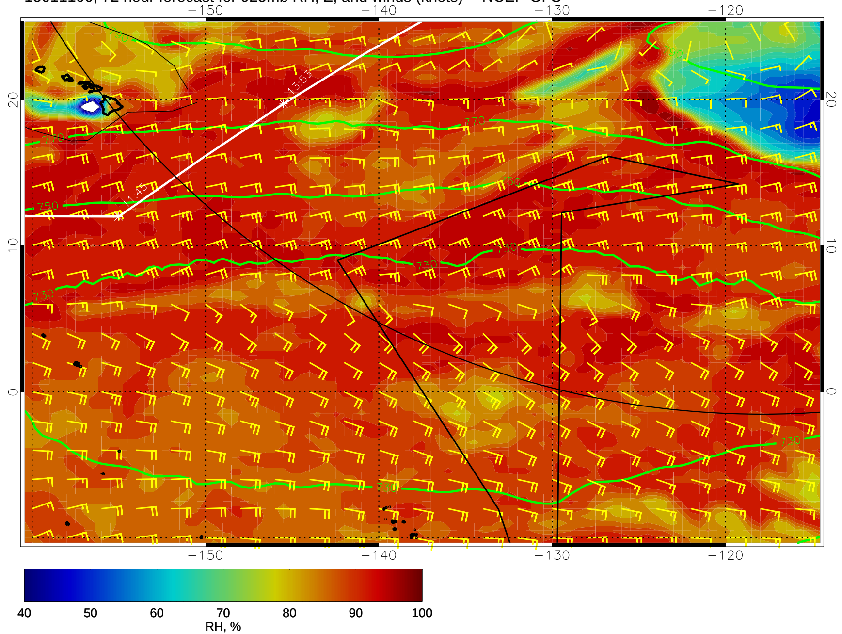
15011100, 72 hour forecast for 925mb RH, Z, and winds (knots) -- NCEP GFS
