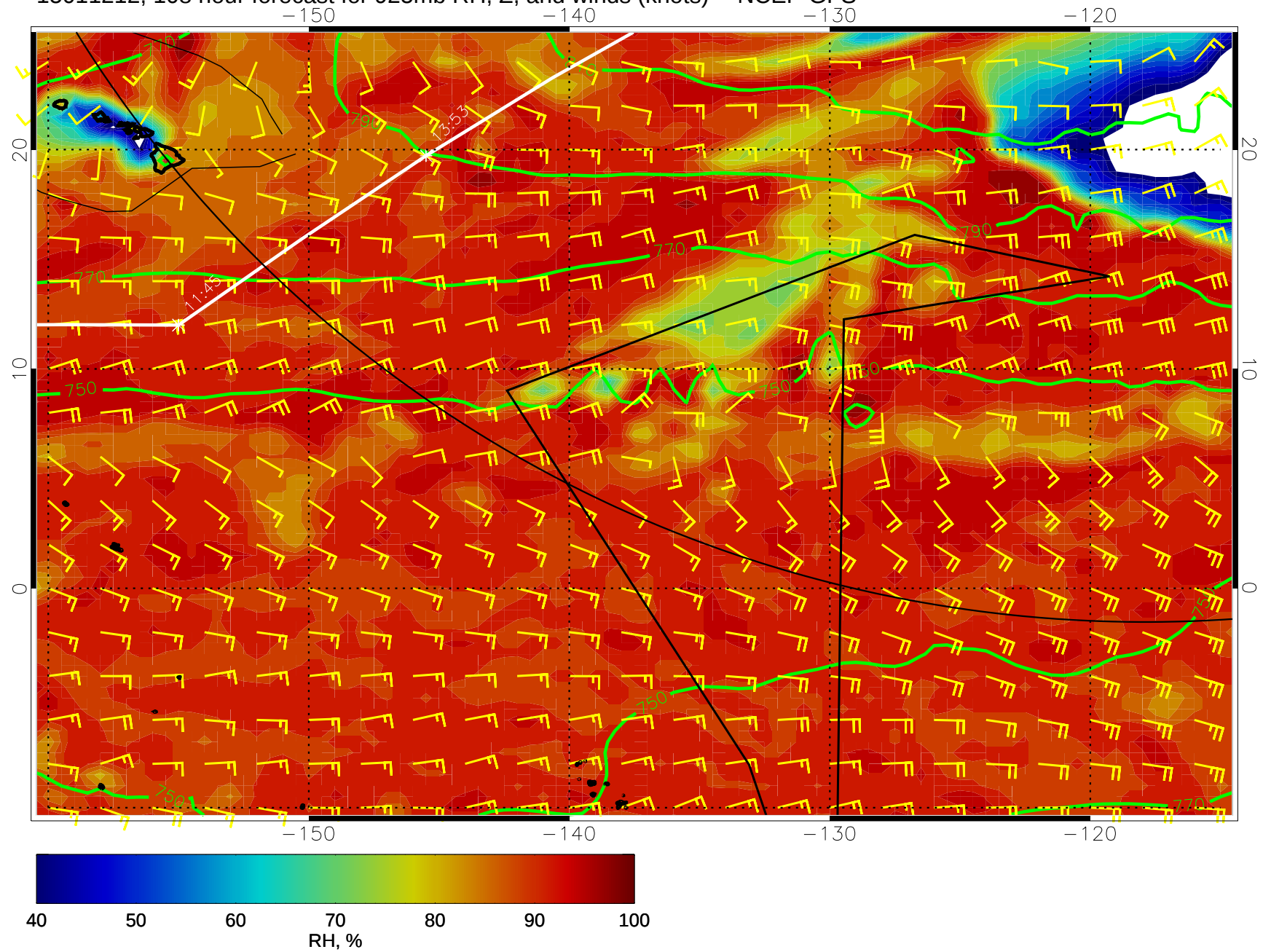
15011212, 108 hour forecast for 925mb RH, Z, and winds (knots) -- NCEP GFS
