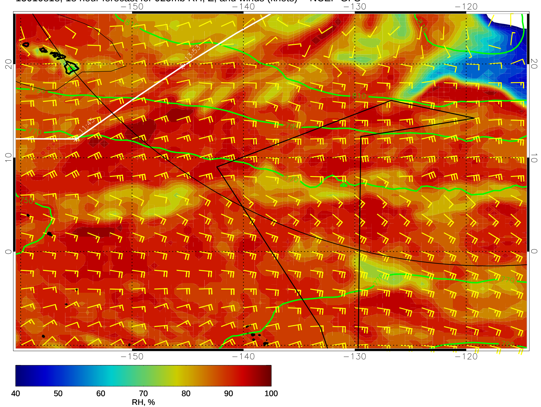
15010818, 18 hour forecast for 925mb RH, Z, and winds (knots) -- NCEP GFS
