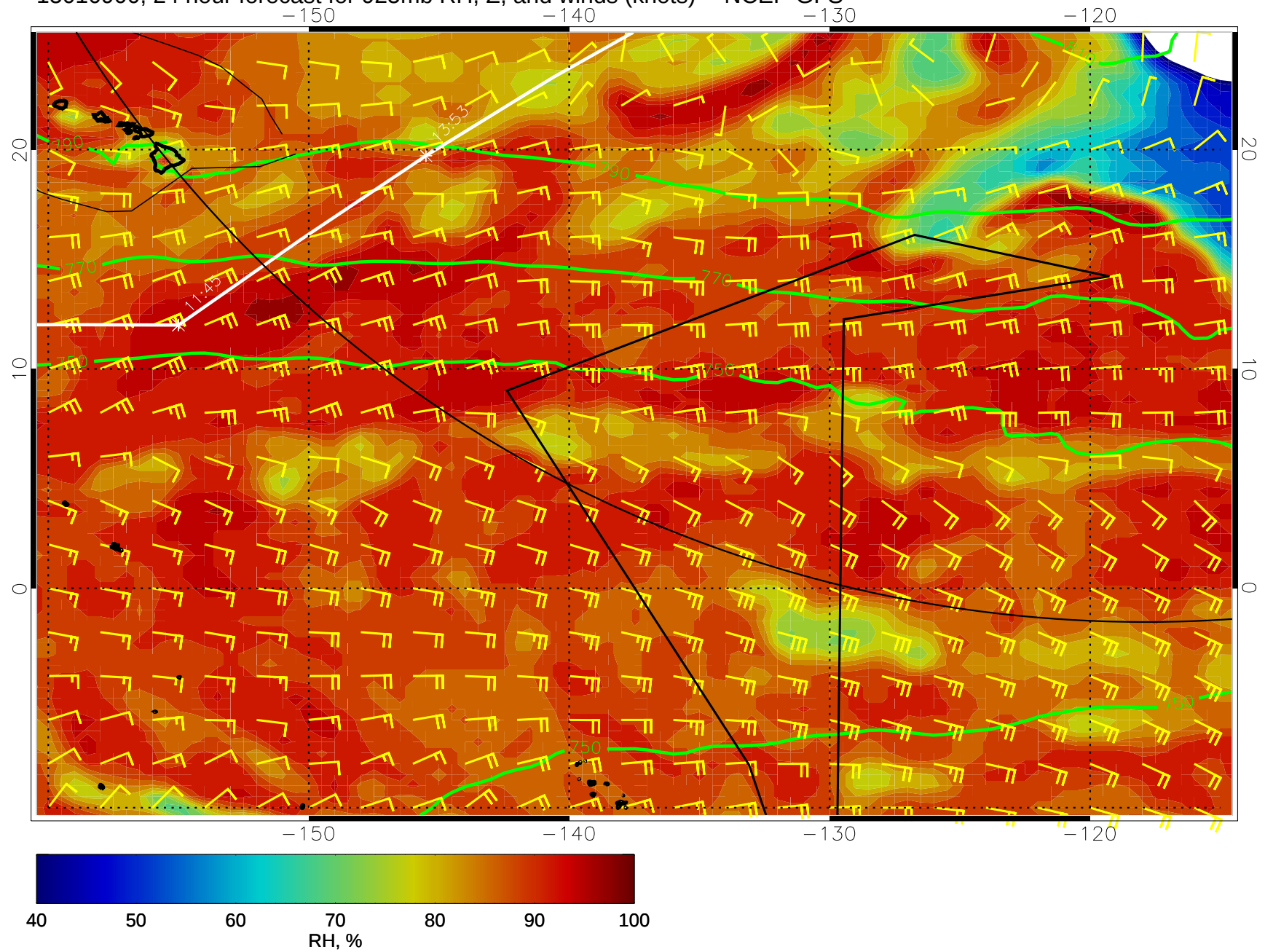
15010900, 24 hour forecast for 925mb RH, Z, and winds (knots) -- NCEP GFS
