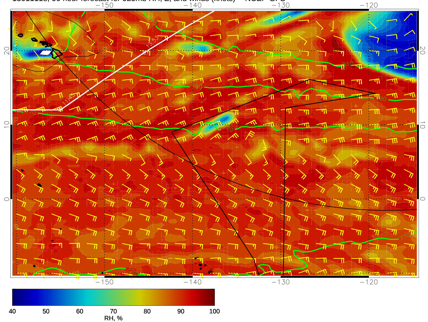
15011118, 90 hour forecast for 925mb RH, Z, and winds (knots) -- NCEP GFS
