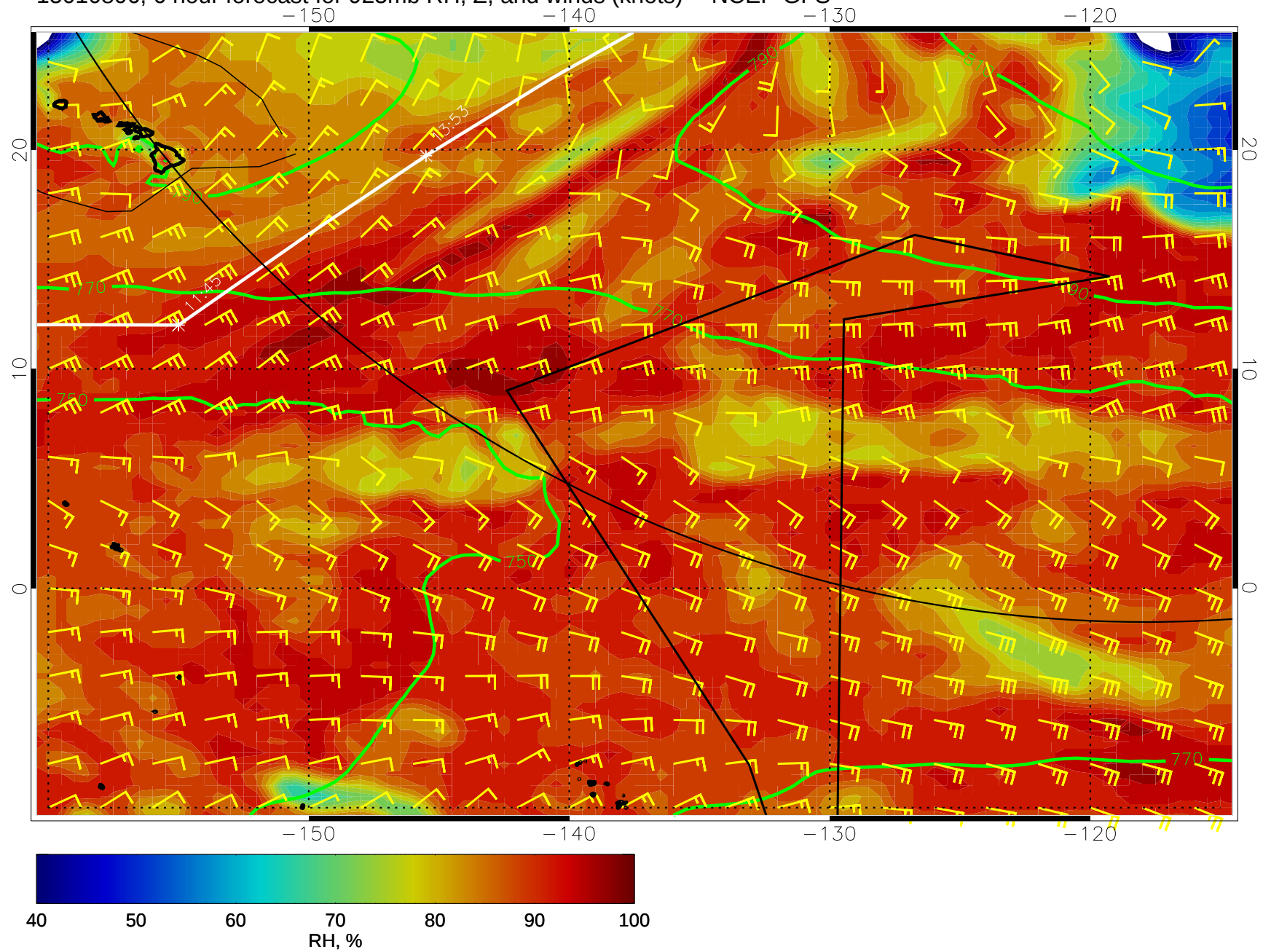
15010806, 6 hour forecast for 925mb RH, Z, and winds (knots) -- NCEP GFS
