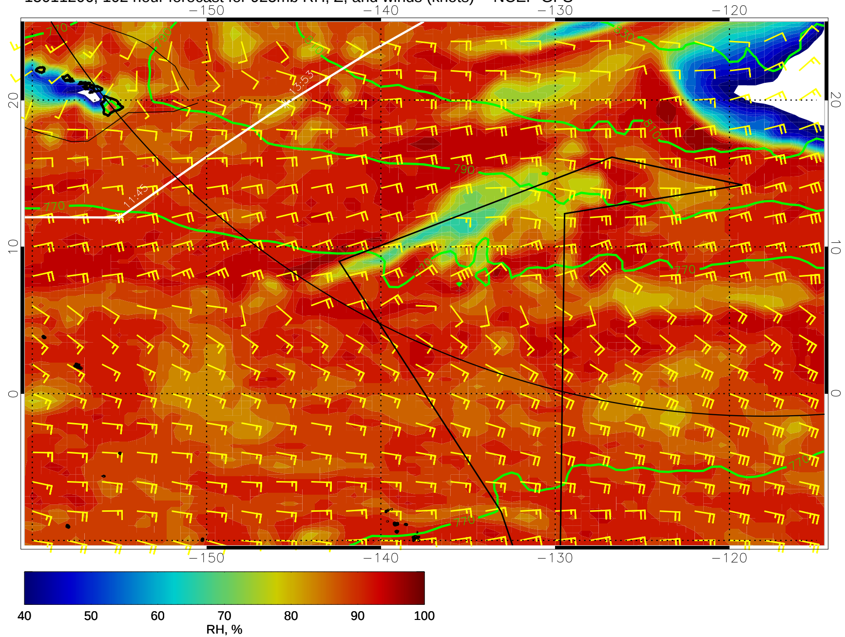
15011206, 102 hour forecast for 925mb RH, Z, and winds (knots) -- NCEP GFS
