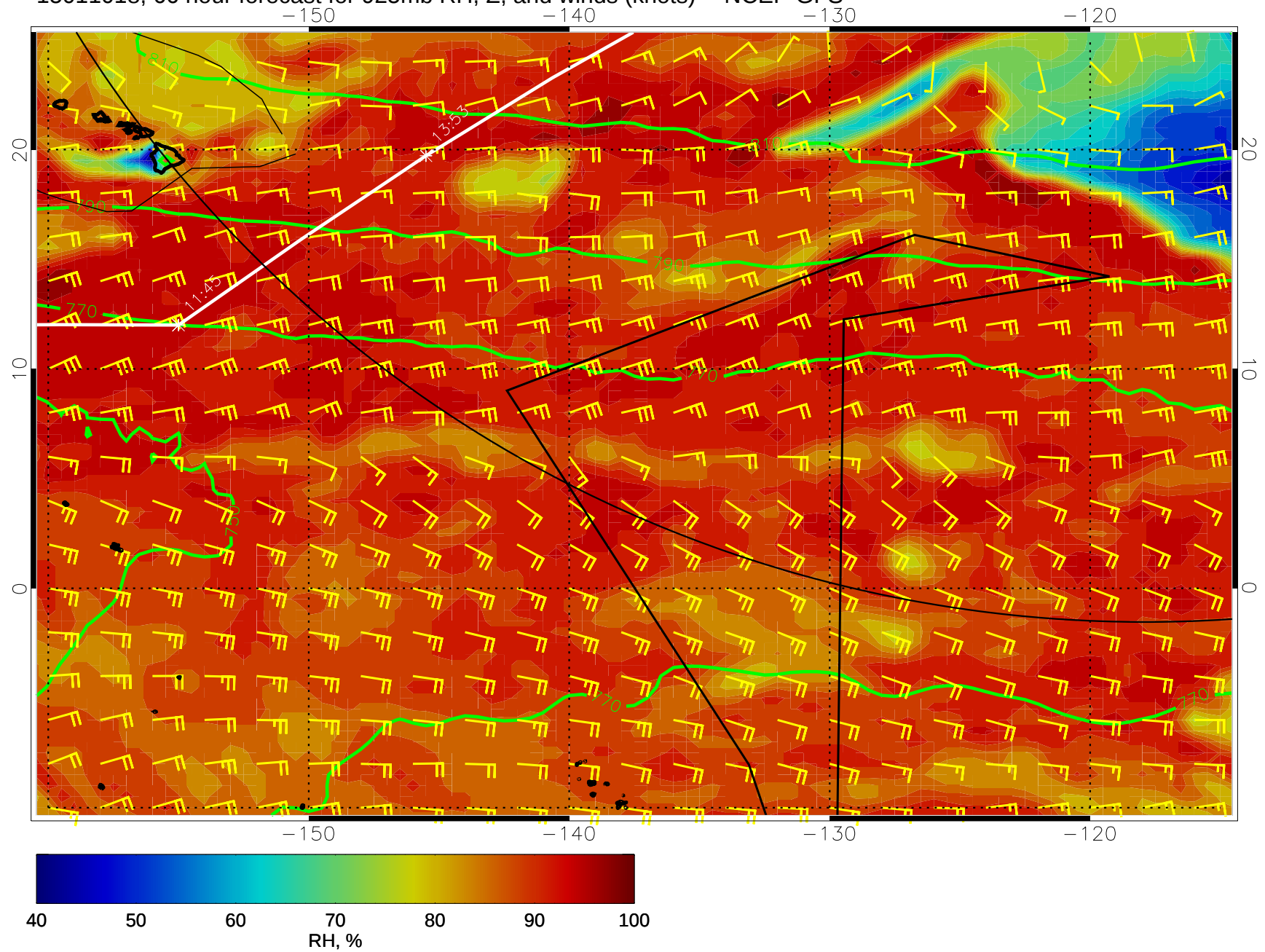
15011018, 66 hour forecast for 925mb RH, Z, and winds (knots) -- NCEP GFS
