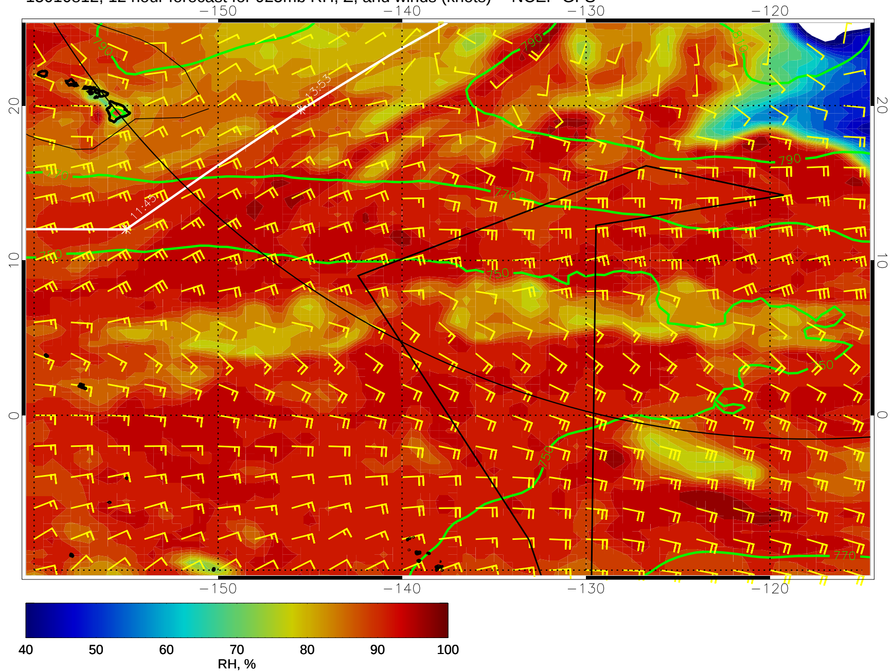
15010812, 12 hour forecast for 925mb RH, Z, and winds (knots) -- NCEP GFS
