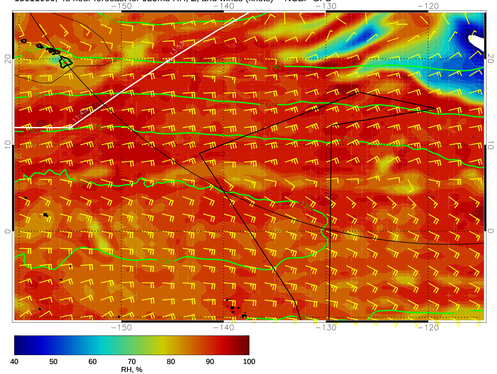
15011000, 48 hour forecast for 925mb RH, Z, and winds (knots) -- NCEP GFS
