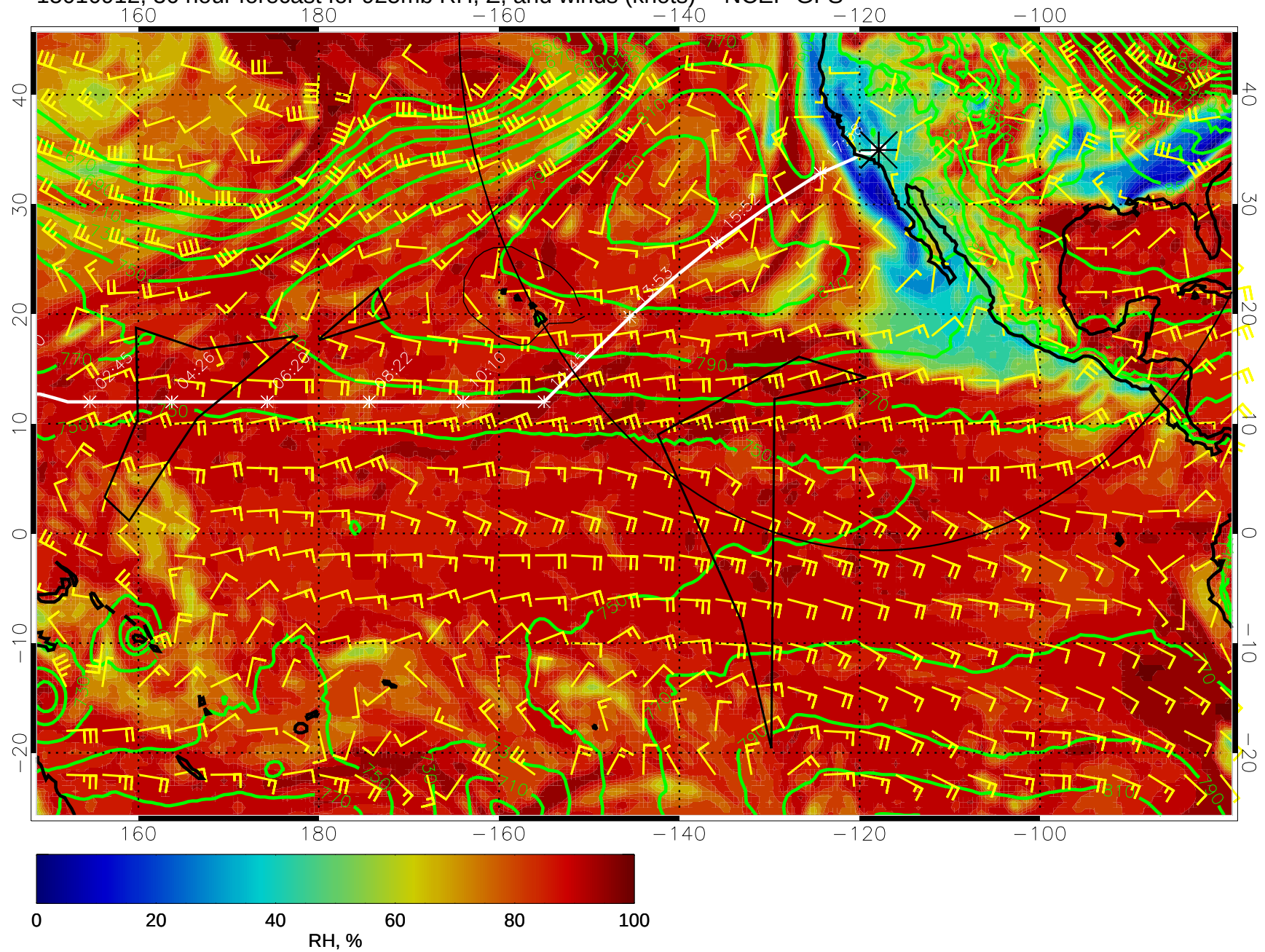
15010912, 36 hour forecast for 925mb RH, Z, and winds (knots) -- NCEP GFS
