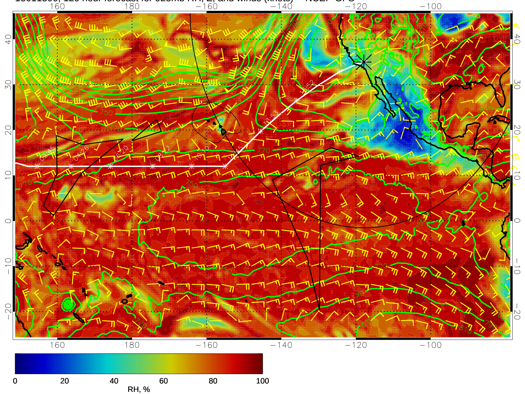
15011300, 120 hour forecast for 925mb RH, Z, and winds (knots) -- NCEP GFS
