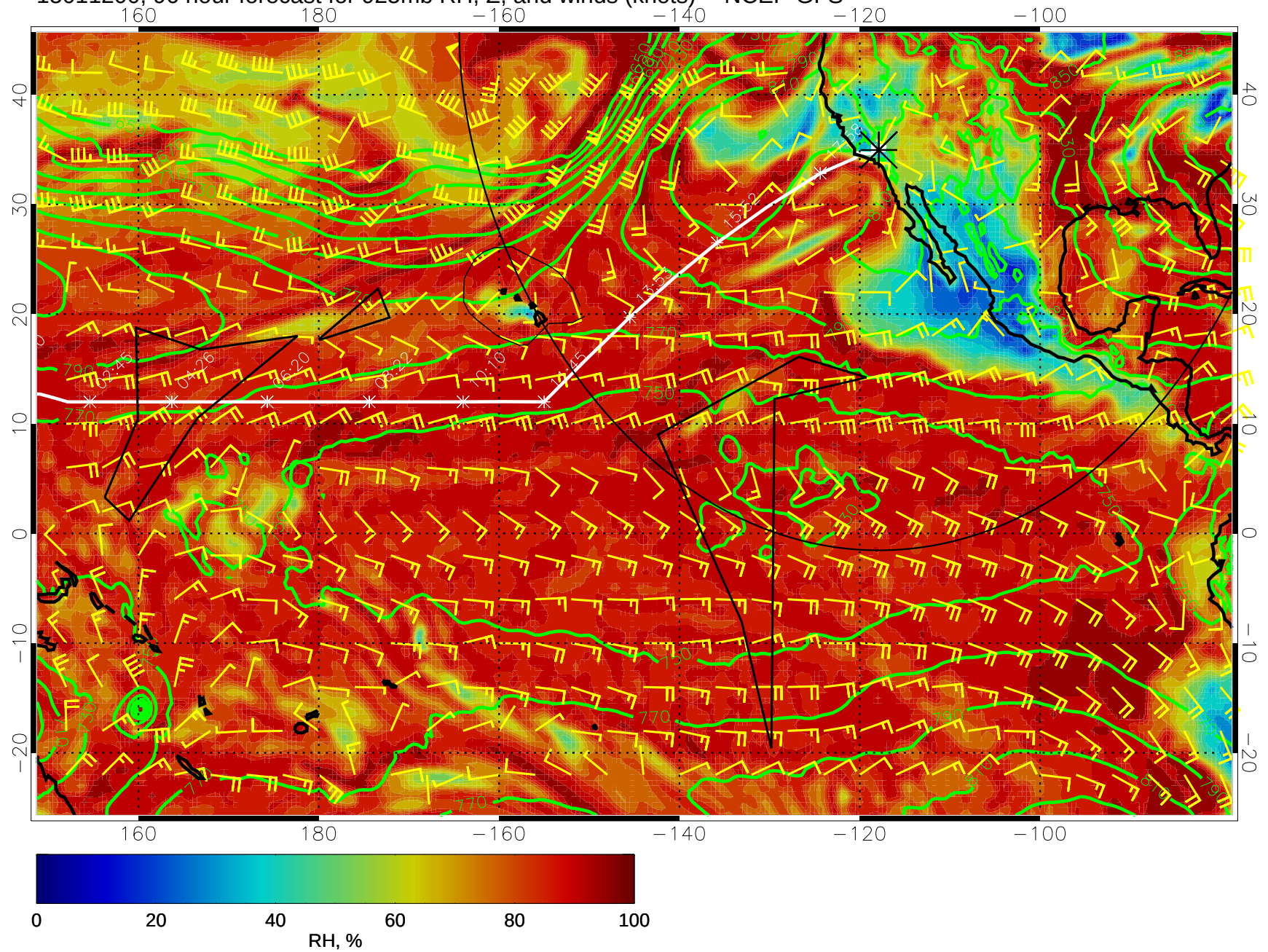
15011200, 96 hour forecast for 925mb RH, Z, and winds (knots) -- NCEP GFS
