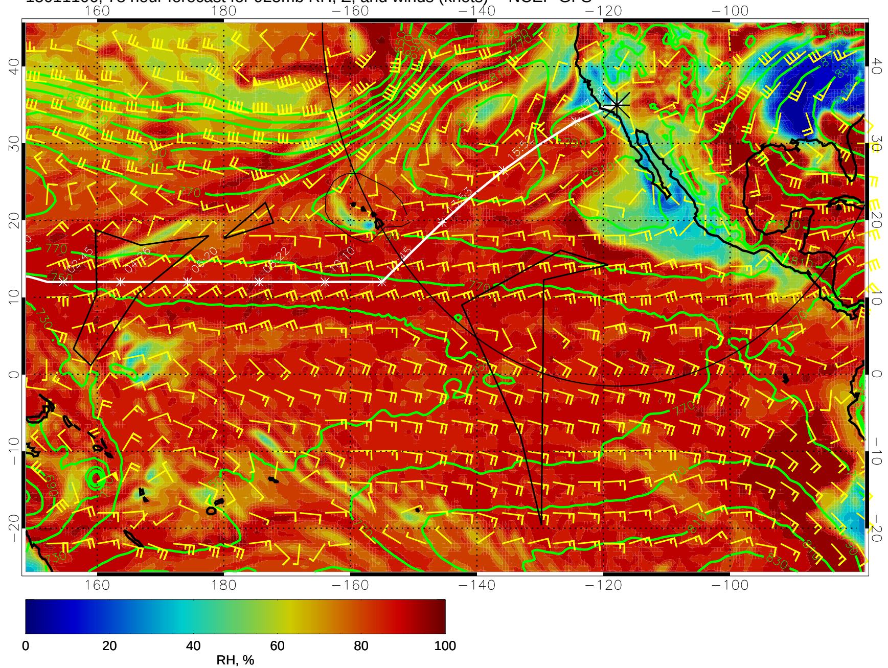
15011106, 78 hour forecast for 925mb RH, Z, and winds (knots) -- NCEP GFS
