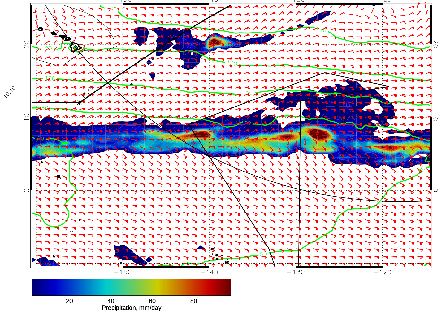
15011106, 78 hour forecast for precip, 1000mb Z, and winds (knots) -- NCEP GFS
