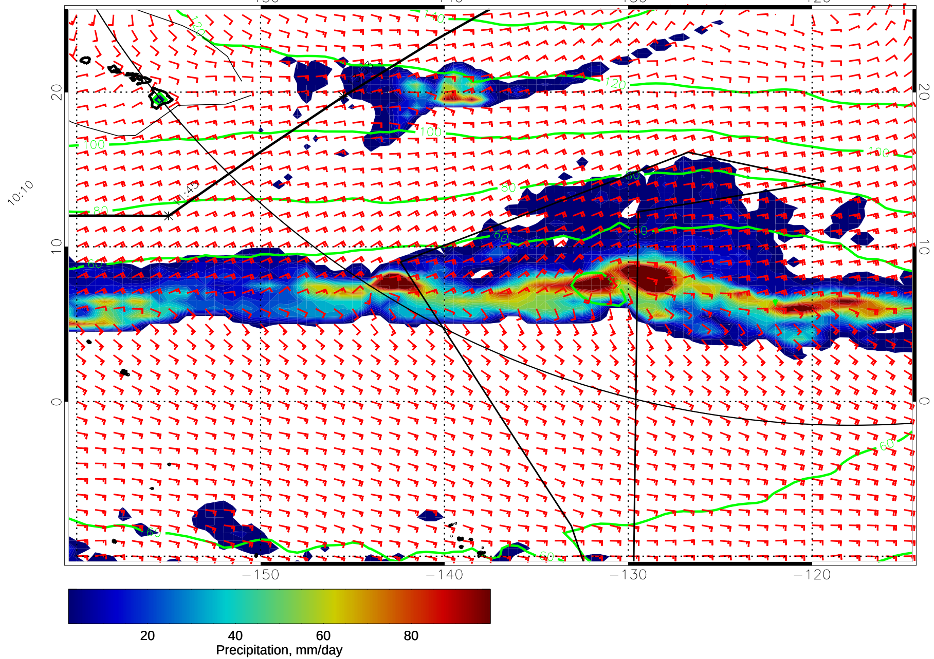
15011112, 84 hour forecast for precip, 1000mb Z, and winds (knots) -- NCEP GFS
