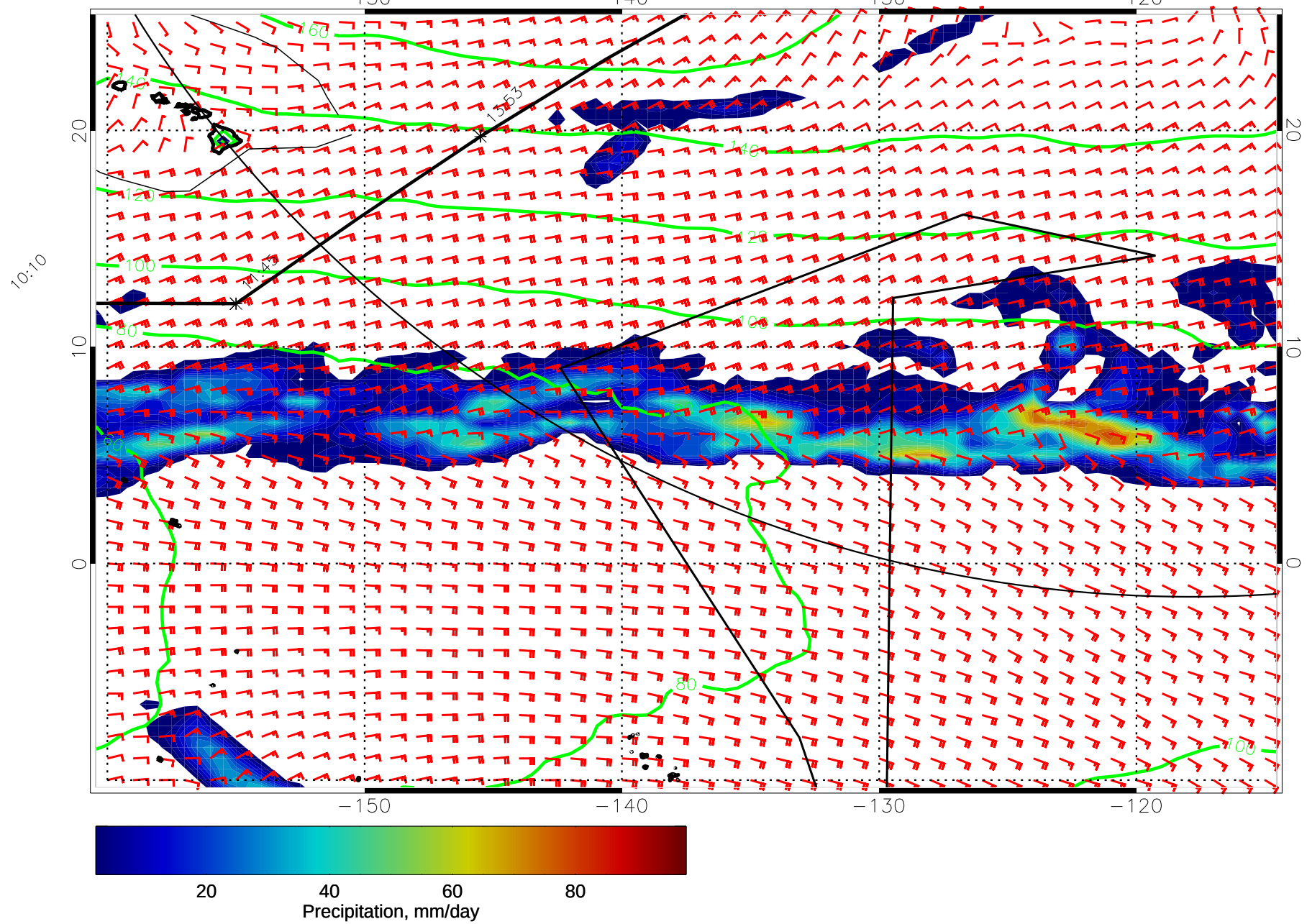
15011006, 54 hour forecast for precip, 1000mb Z, and winds (knots) -- NCEP GFS
