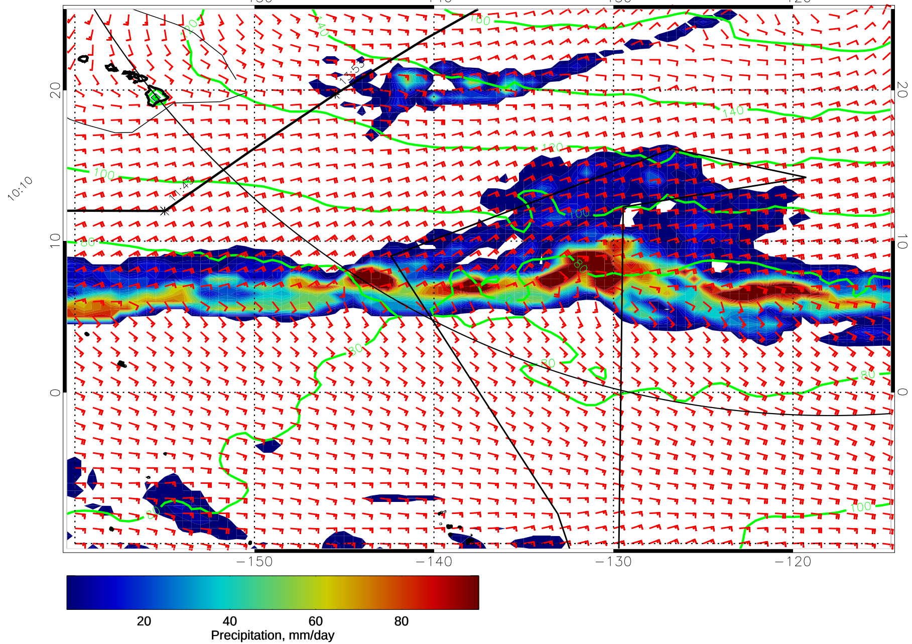
15011118, 90 hour forecast for precip, 1000mb Z, and winds (knots) -- NCEP GFS
