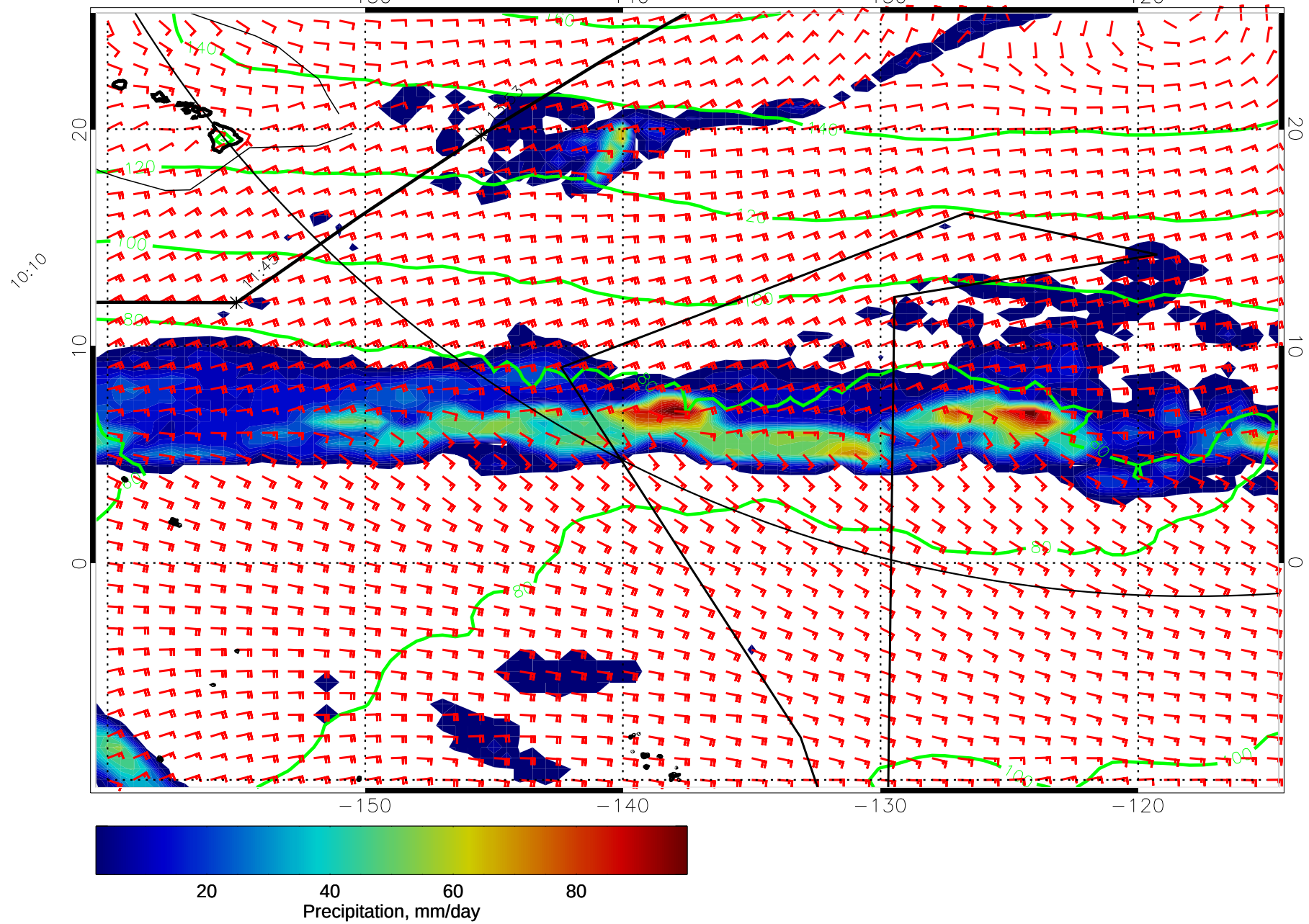
15011018, 66 hour forecast for precip, 1000mb Z, and winds (knots) -- NCEP GFS
