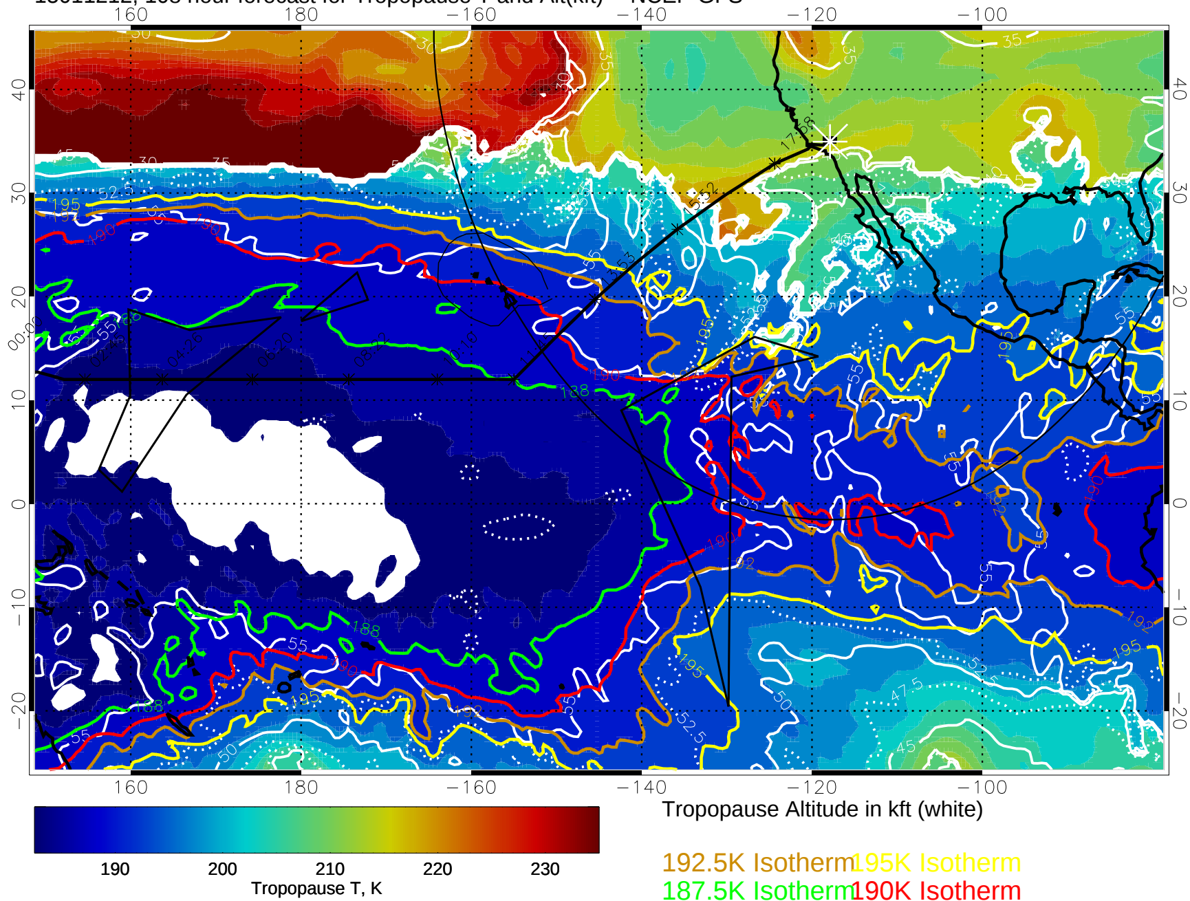
15011212, 108 hour forecast for Tropopause T and Alt(kft) -- NCEP GFS
