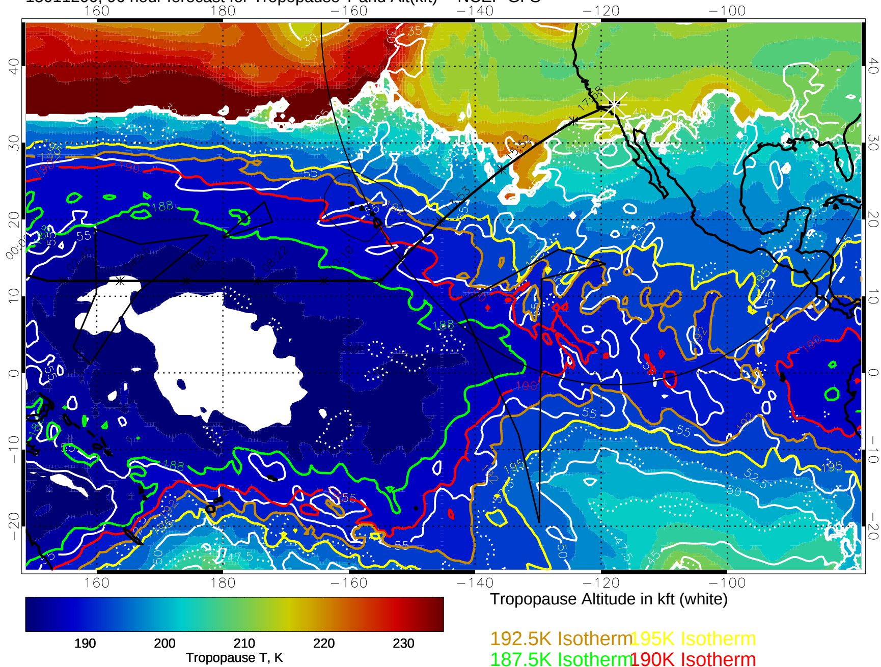
15011200, 96 hour forecast for Tropopause T and Alt(kft) -- NCEP GFS
