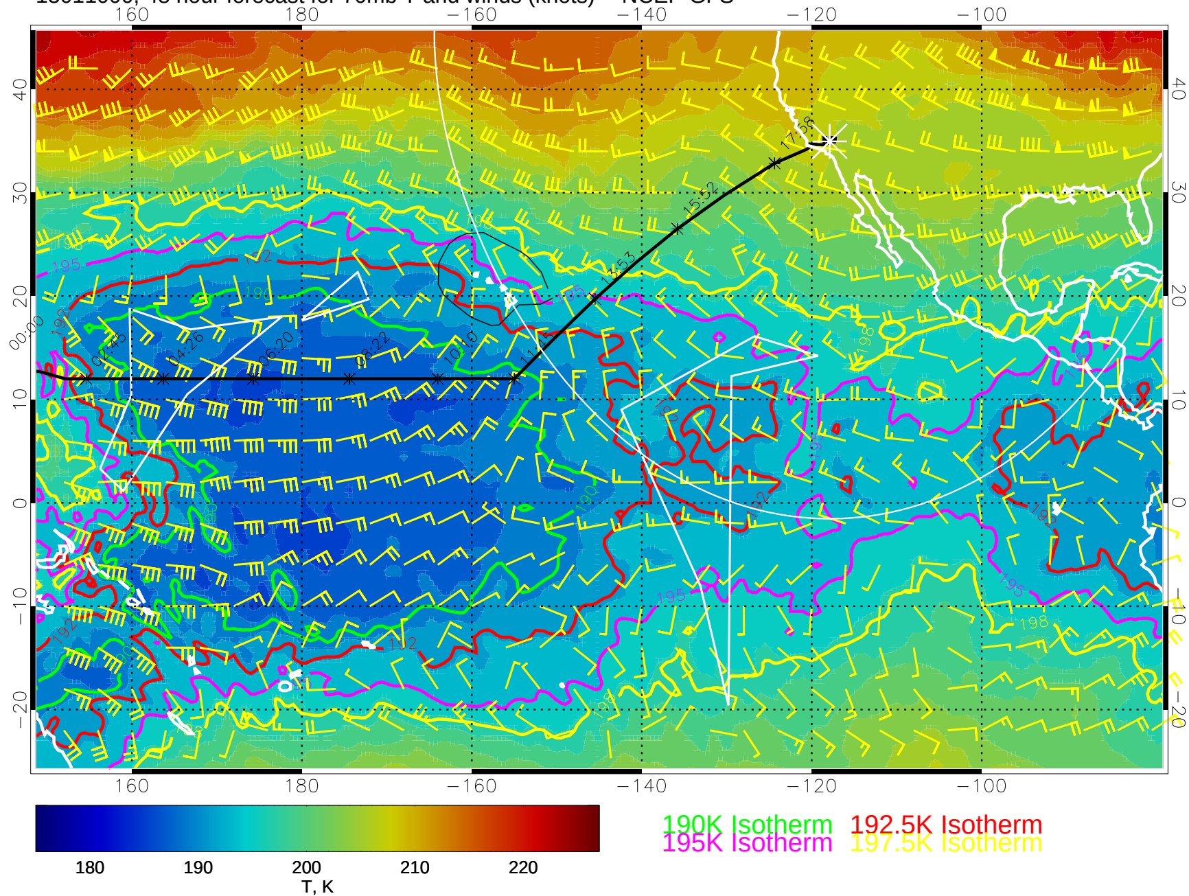
15011000, 48 hour forecast for 70mb T and winds (knots) -- NCEP GFS
