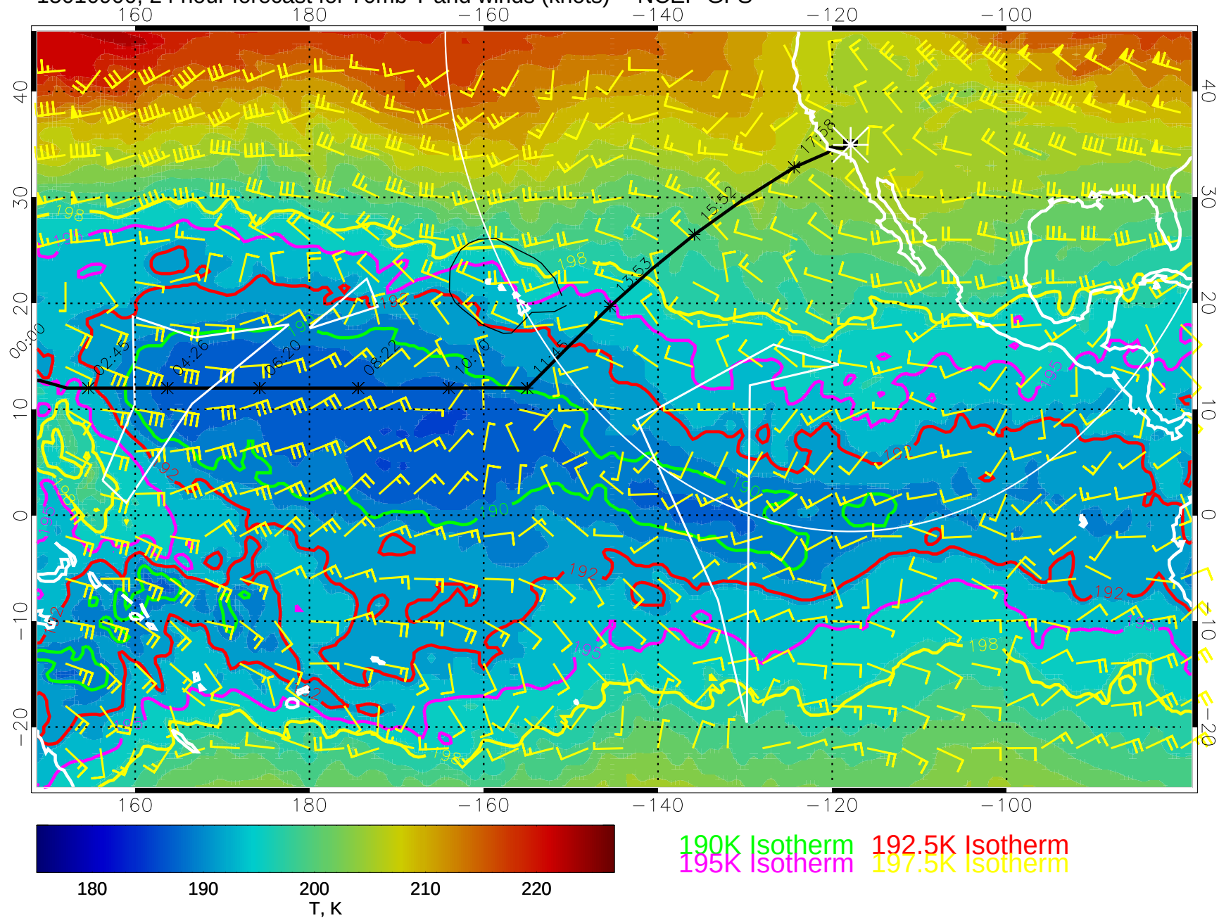
15010900, 24 hour forecast for 70mb T and winds (knots) -- NCEP GFS
