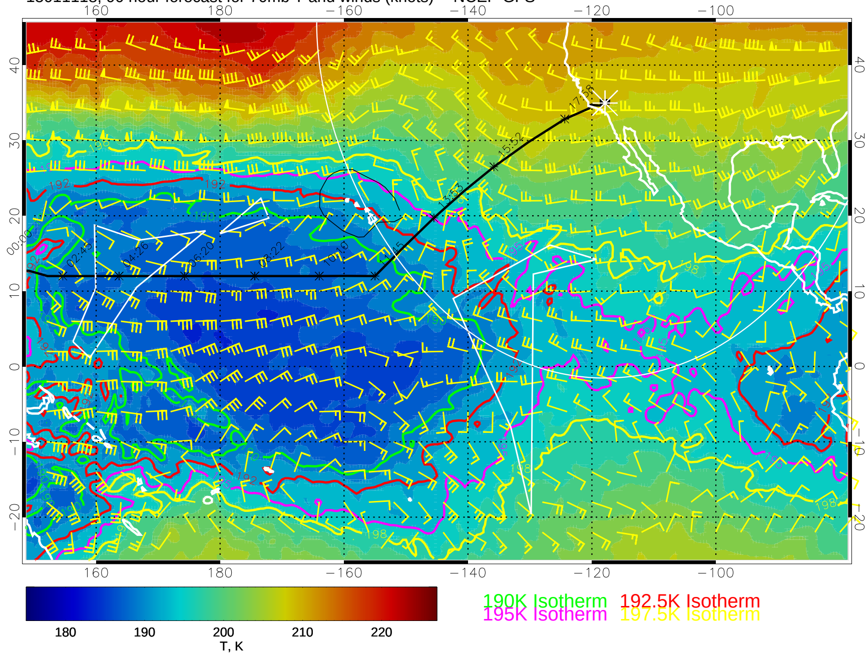
15011118, 90 hour forecast for 70mb T and winds (knots) -- NCEP GFS
