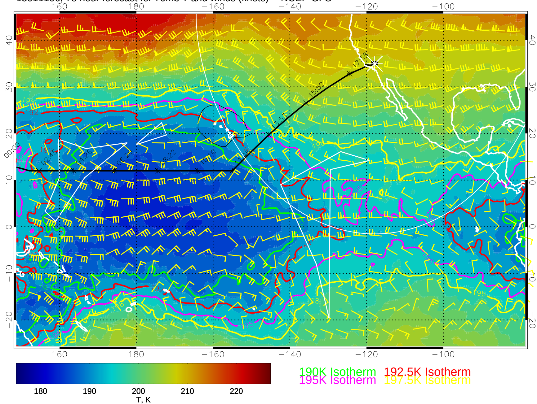
15011106, 78 hour forecast for 70mb T and winds (knots) -- NCEP GFS
