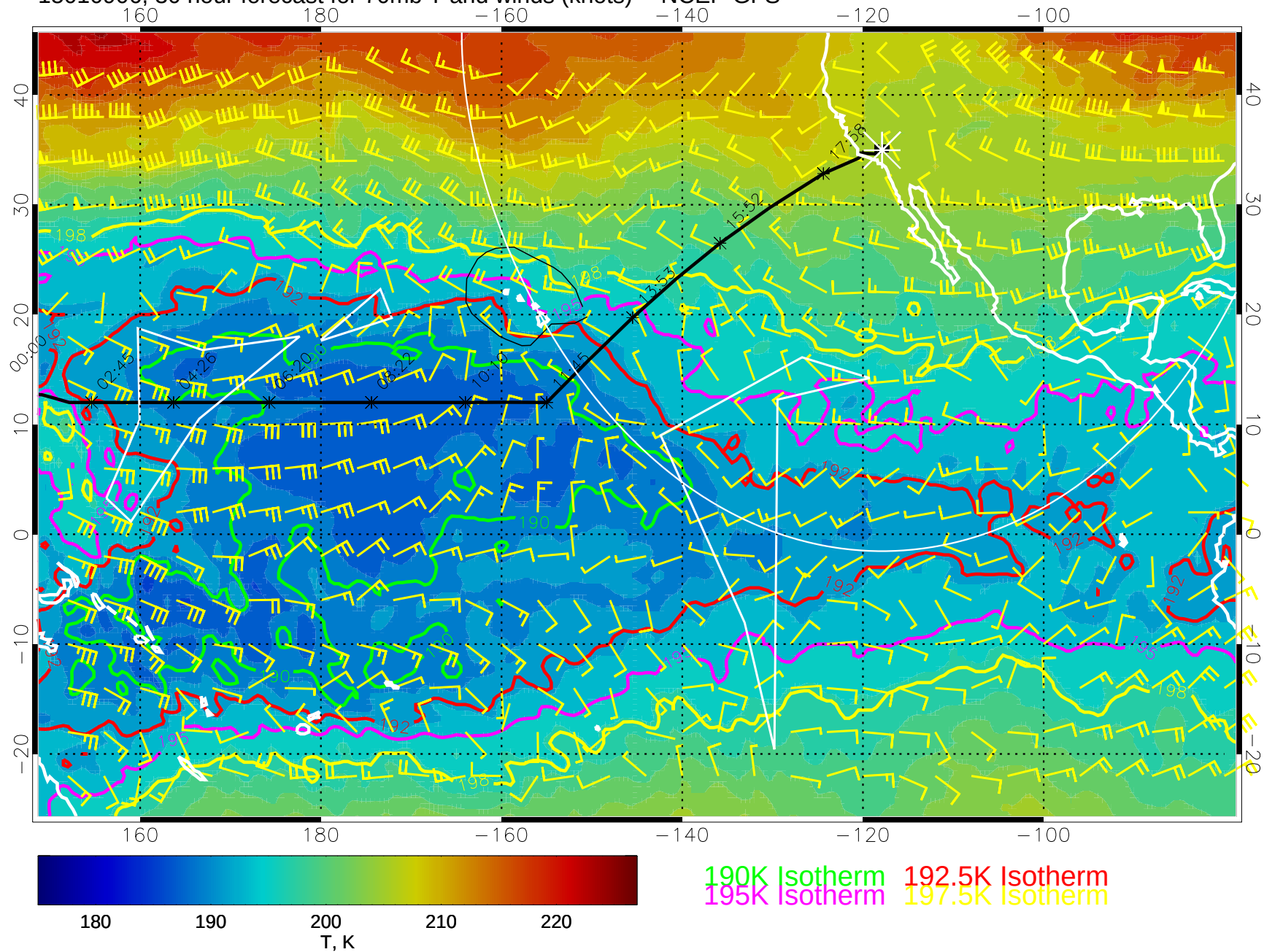
15010906, 30 hour forecast for 70mb T and winds (knots) -- NCEP GFS
