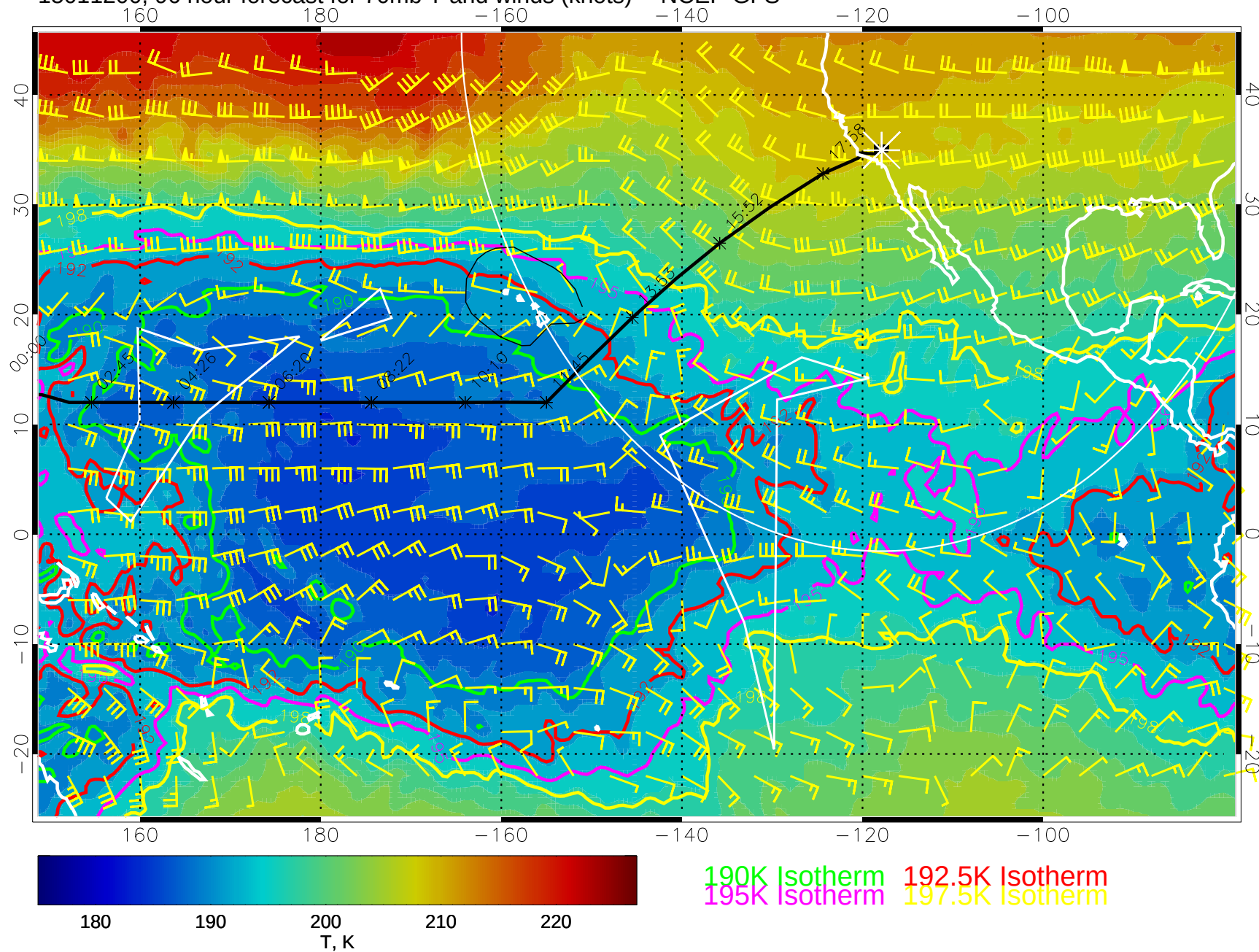
15011200, 96 hour forecast for 70mb T and winds (knots) -- NCEP GFS
