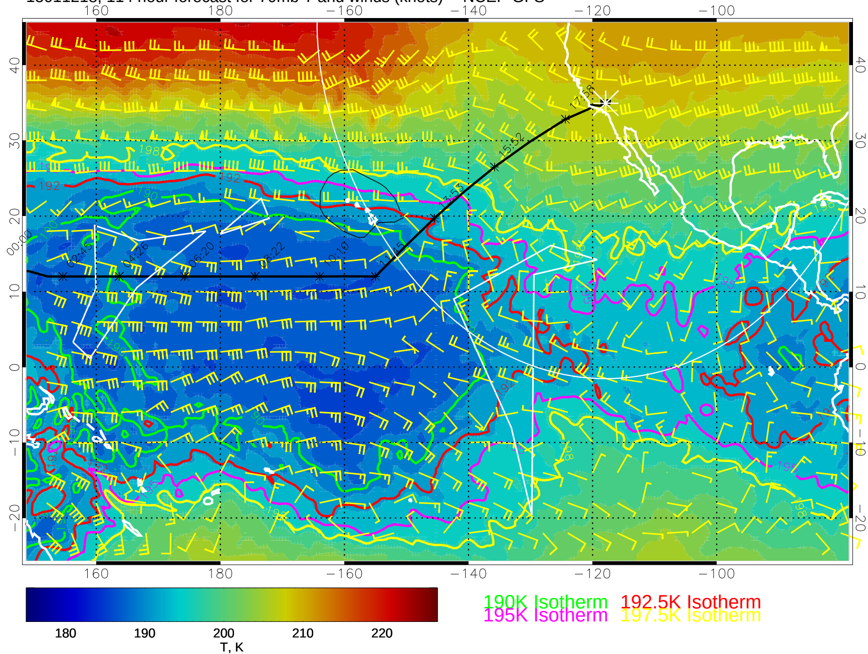
15011218, 114 hour forecast for 70mb T and winds (knots) -- NCEP GFS
