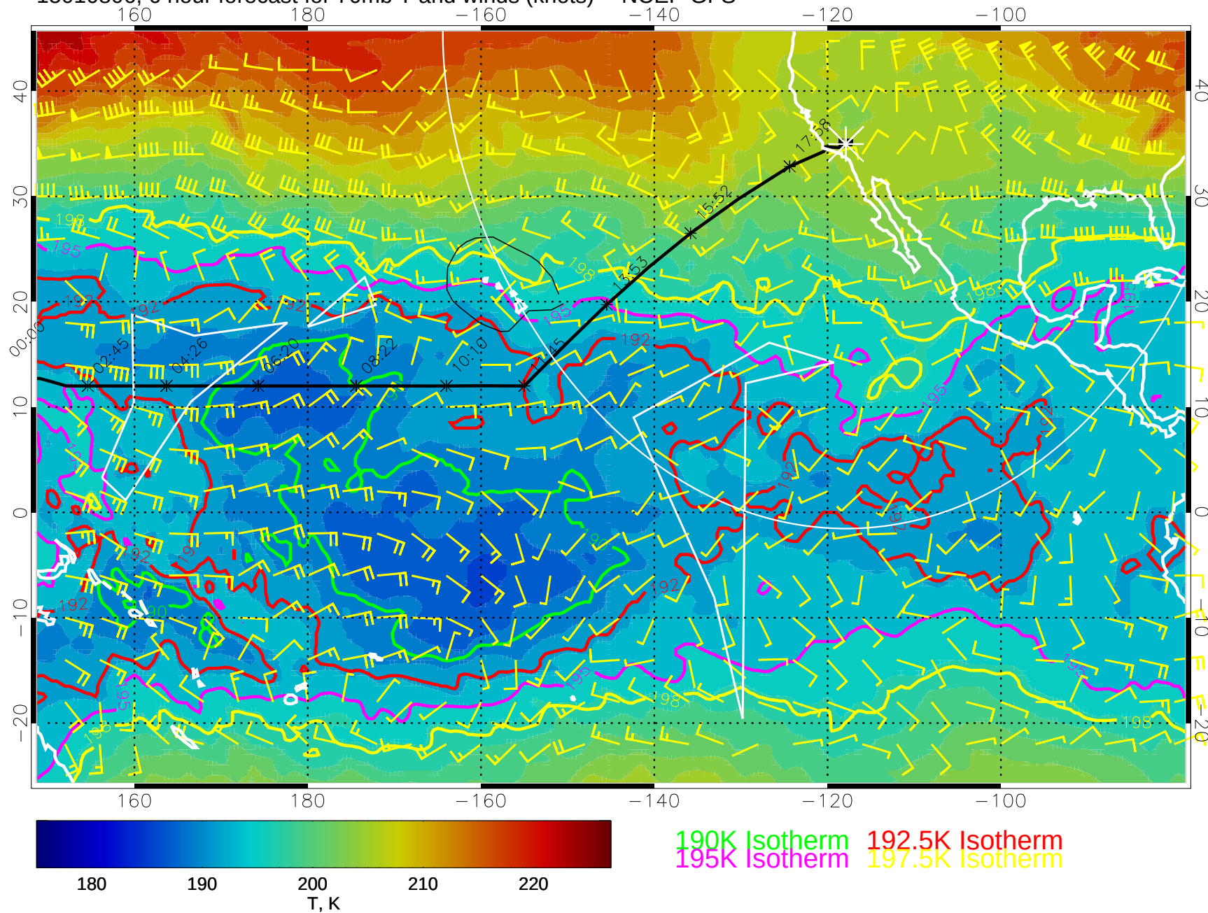
15010806, 6 hour forecast for 70mb T and winds (knots) -- NCEP GFS
