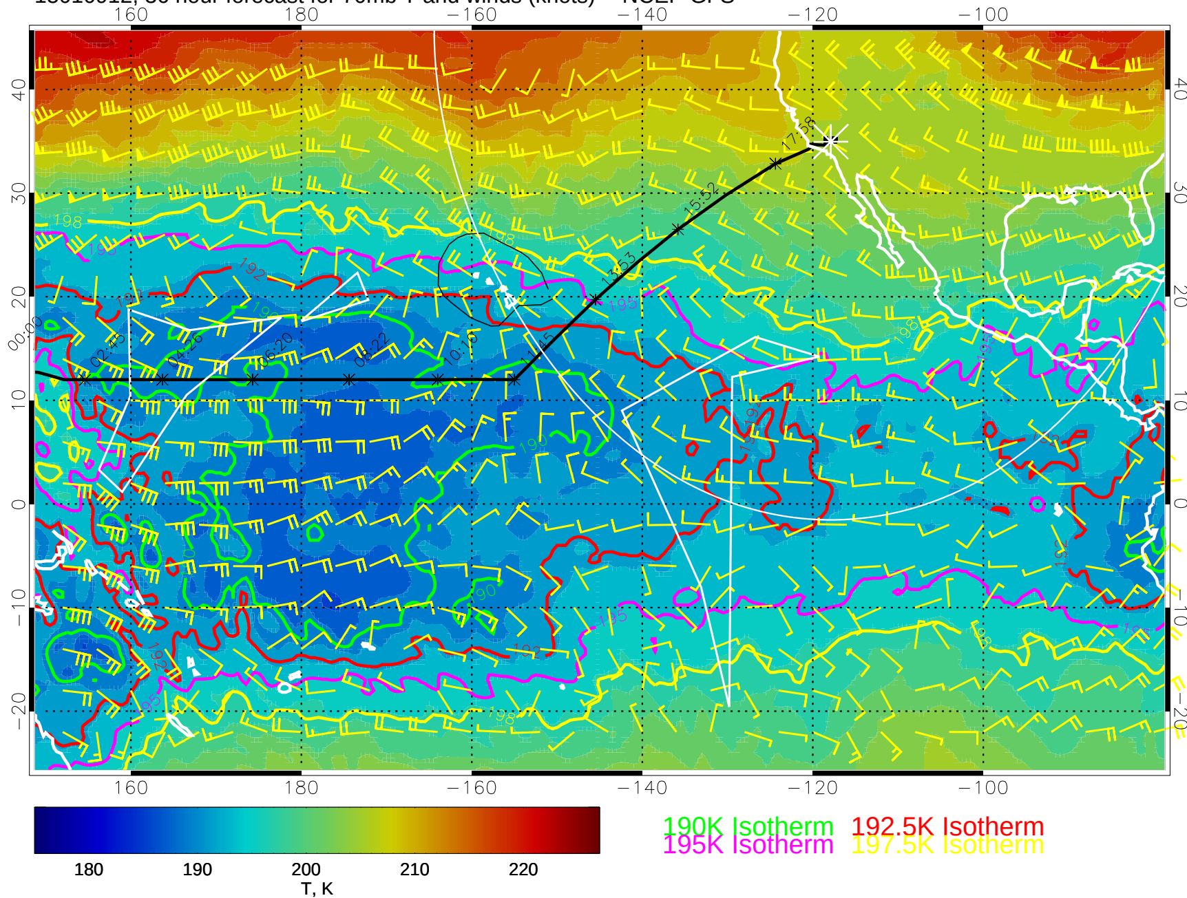
15010912, 36 hour forecast for 70mb T and winds (knots) -- NCEP GFS
