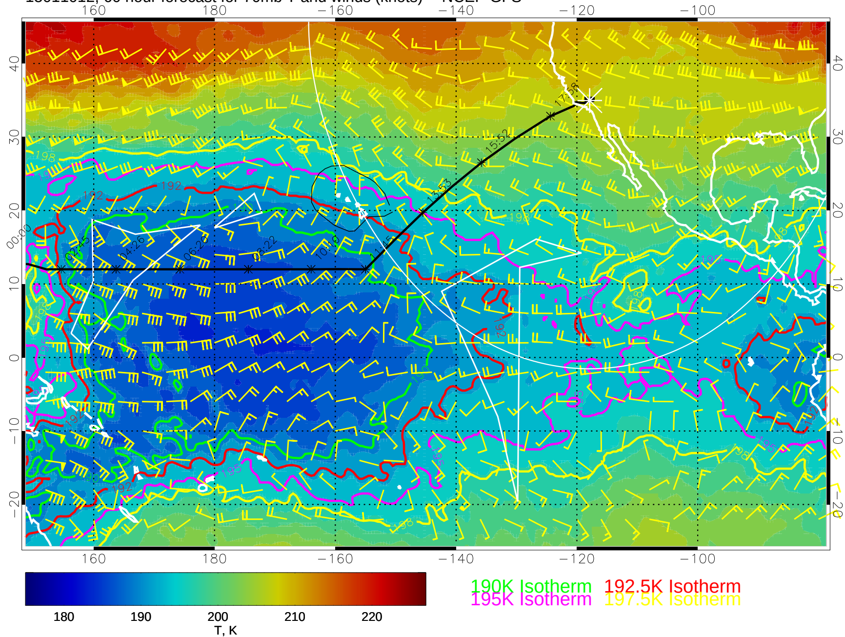
15011012, 60 hour forecast for 70mb T and winds (knots) -- NCEP GFS
