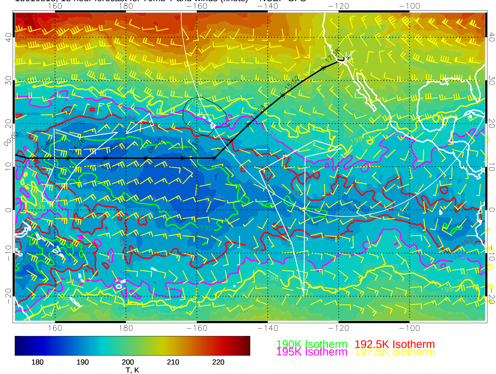
15010818, 18 hour forecast for 70mb T and winds (knots) -- NCEP GFS
