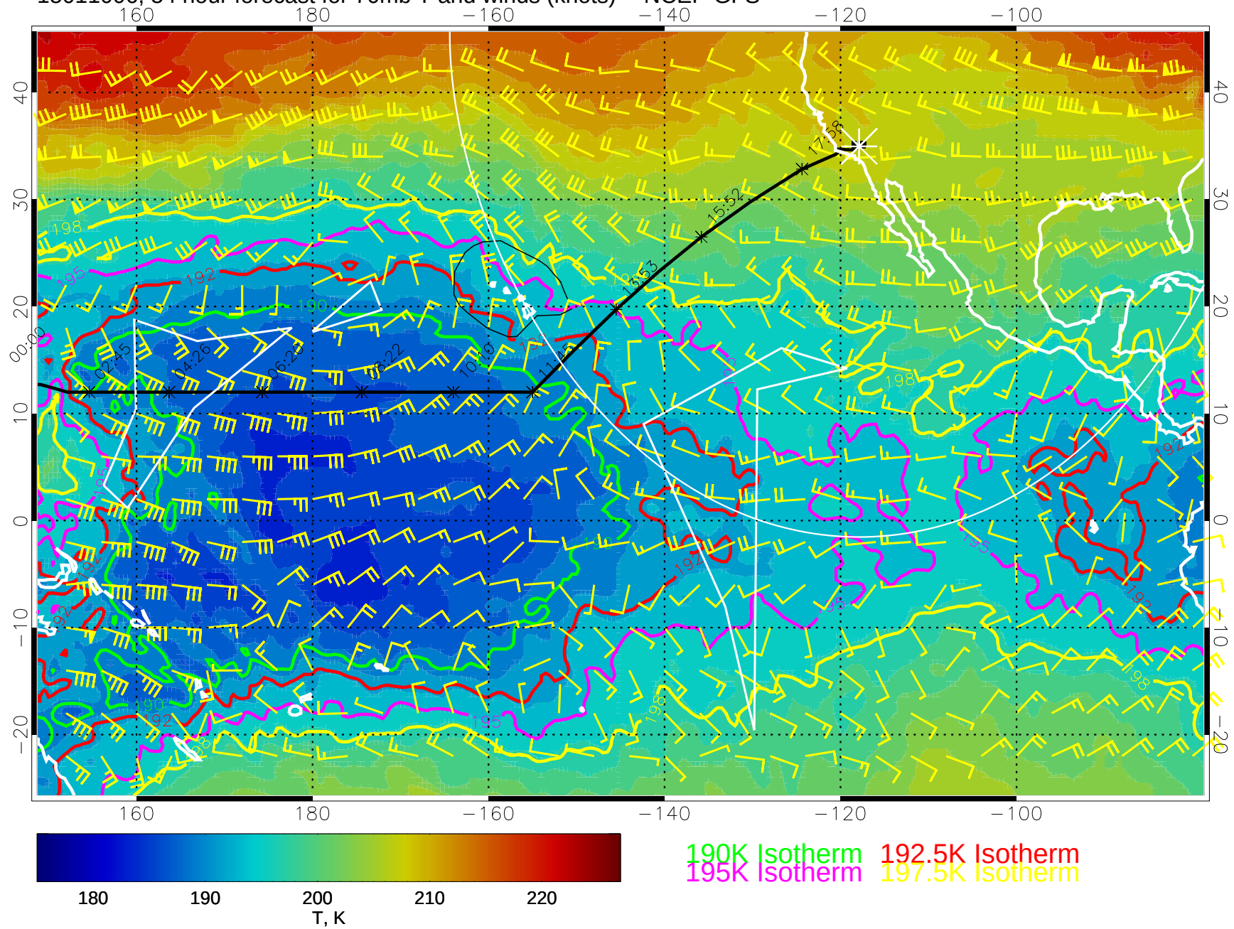
15011006, 54 hour forecast for 70mb T and winds (knots) -- NCEP GFS
