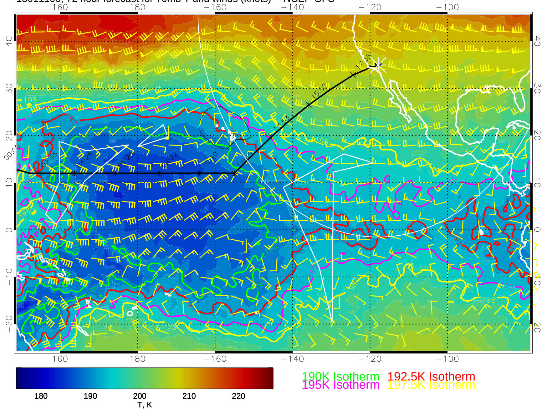
15011100, 72 hour forecast for 70mb T and winds (knots) -- NCEP GFS
