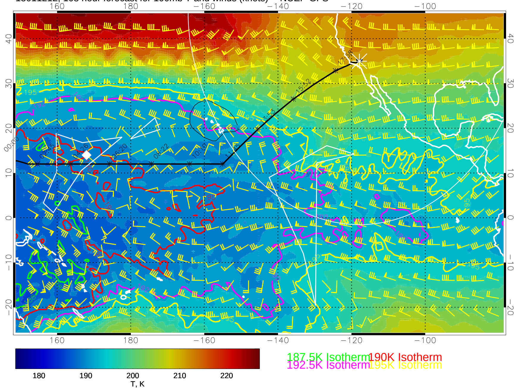
15011212, 108 hour forecast for 100mb T and winds (knots) -- NCEP GFS
