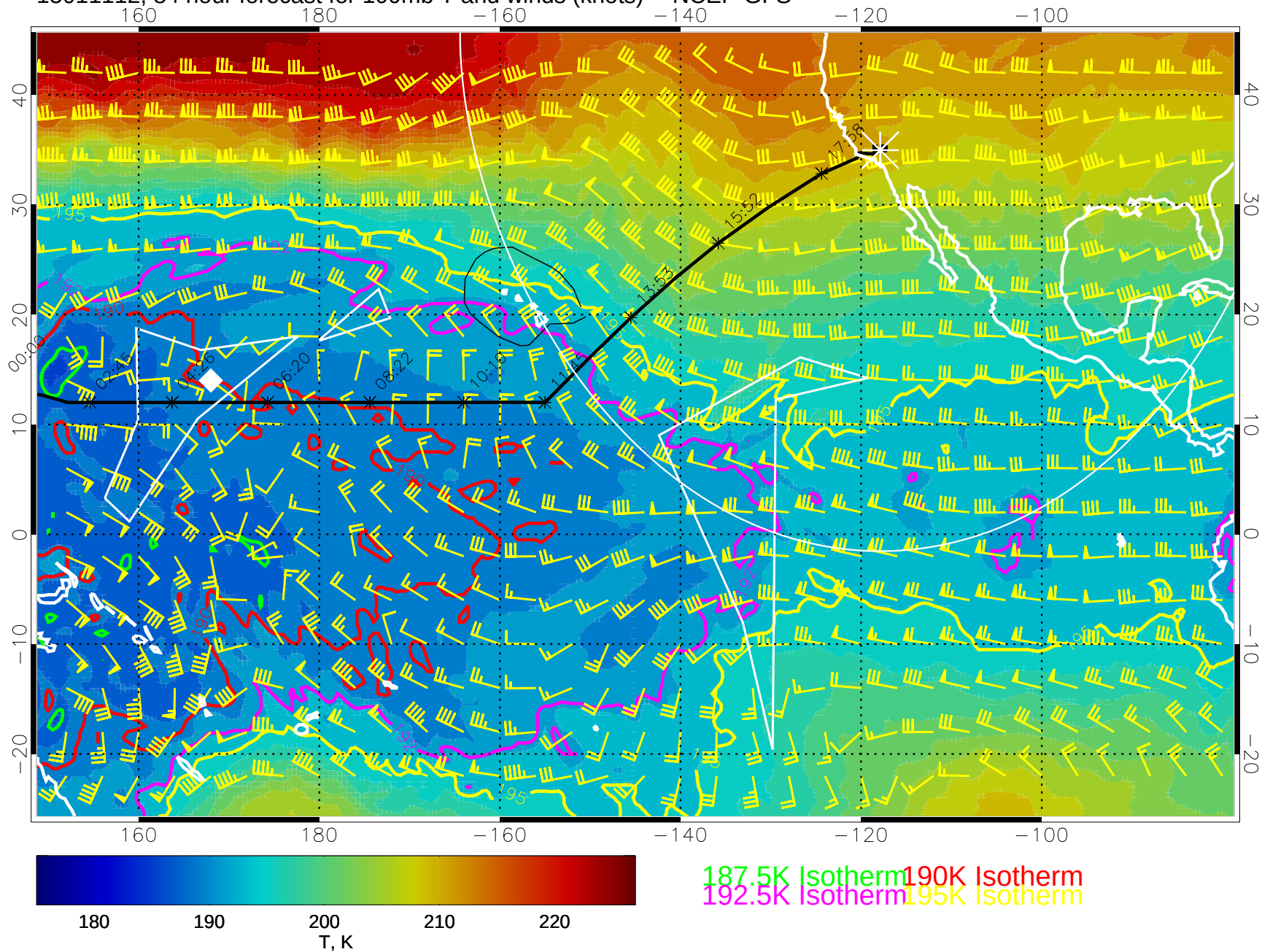
15011112, 84 hour forecast for 100mb T and winds (knots) -- NCEP GFS
