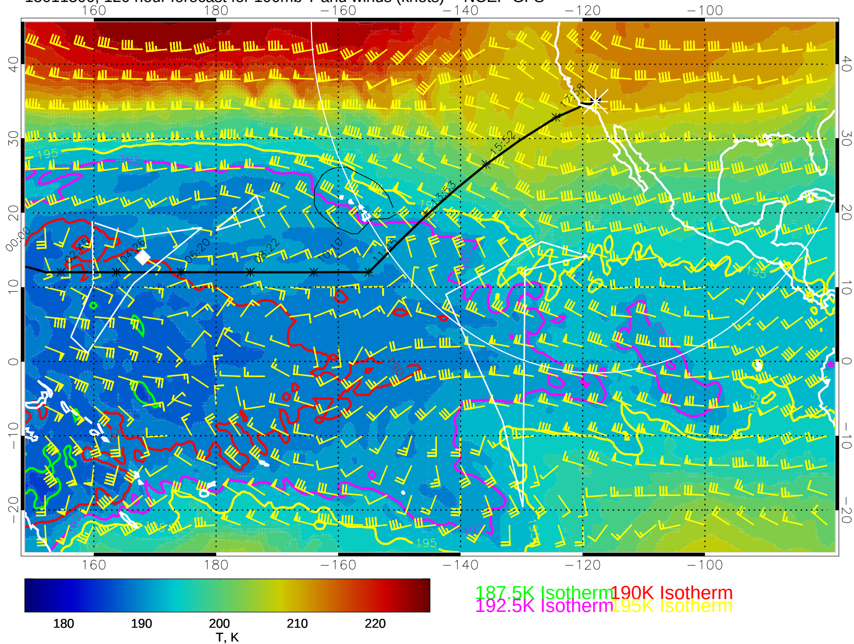
15011300, 120 hour forecast for 100mb T and winds (knots) -- NCEP GFS
