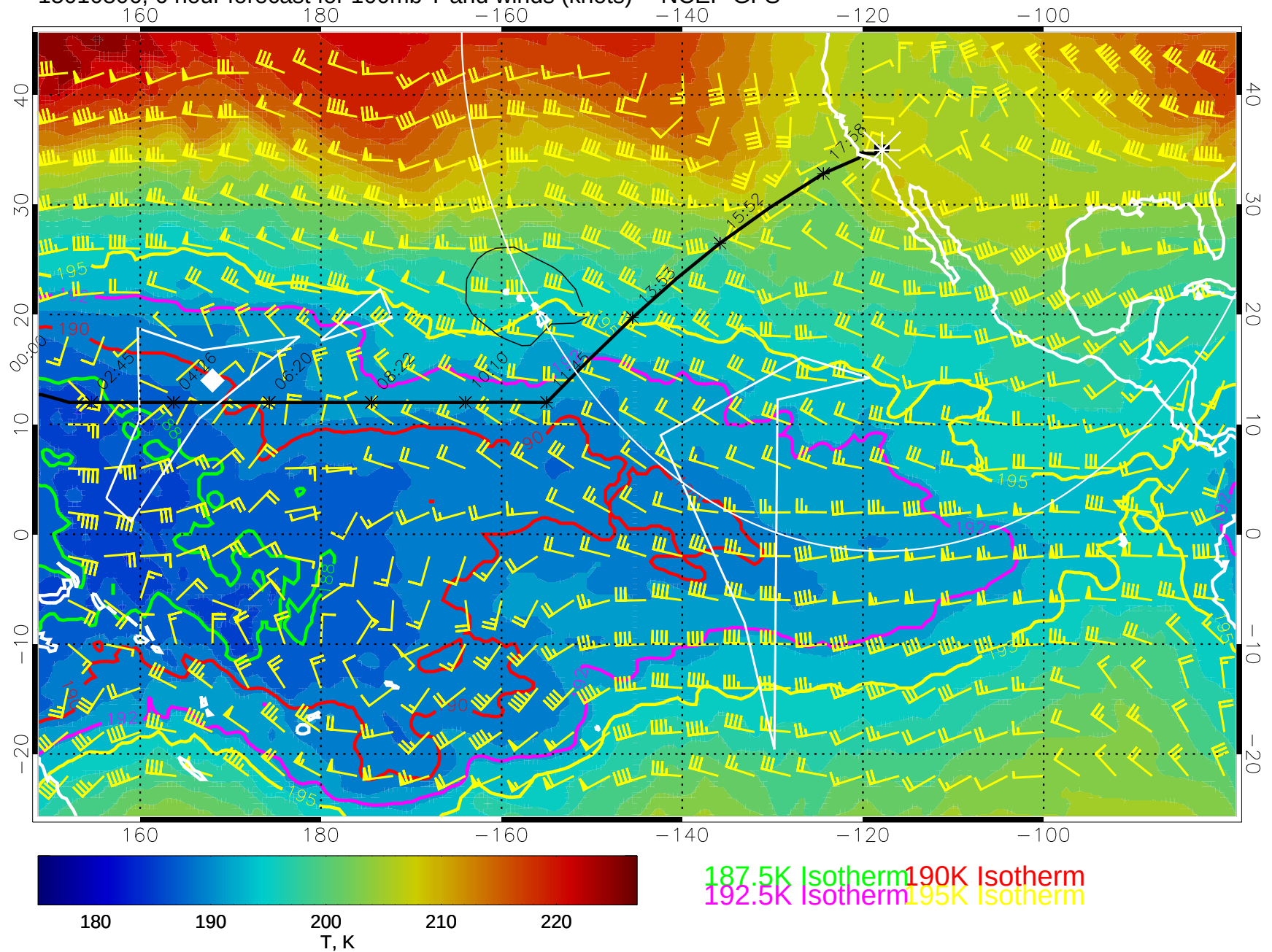
15010806, 6 hour forecast for 100mb T and winds (knots) -- NCEP GFS
