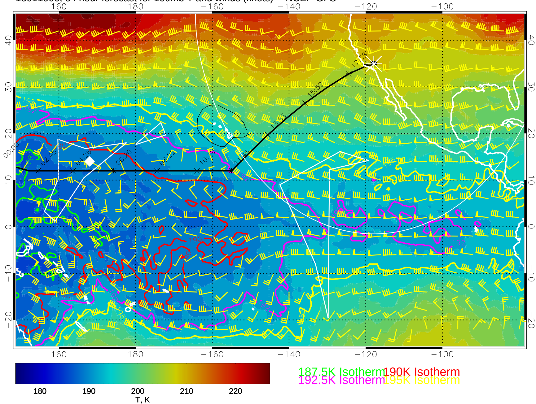
15011006, 54 hour forecast for 100mb T and winds (knots) -- NCEP GFS
