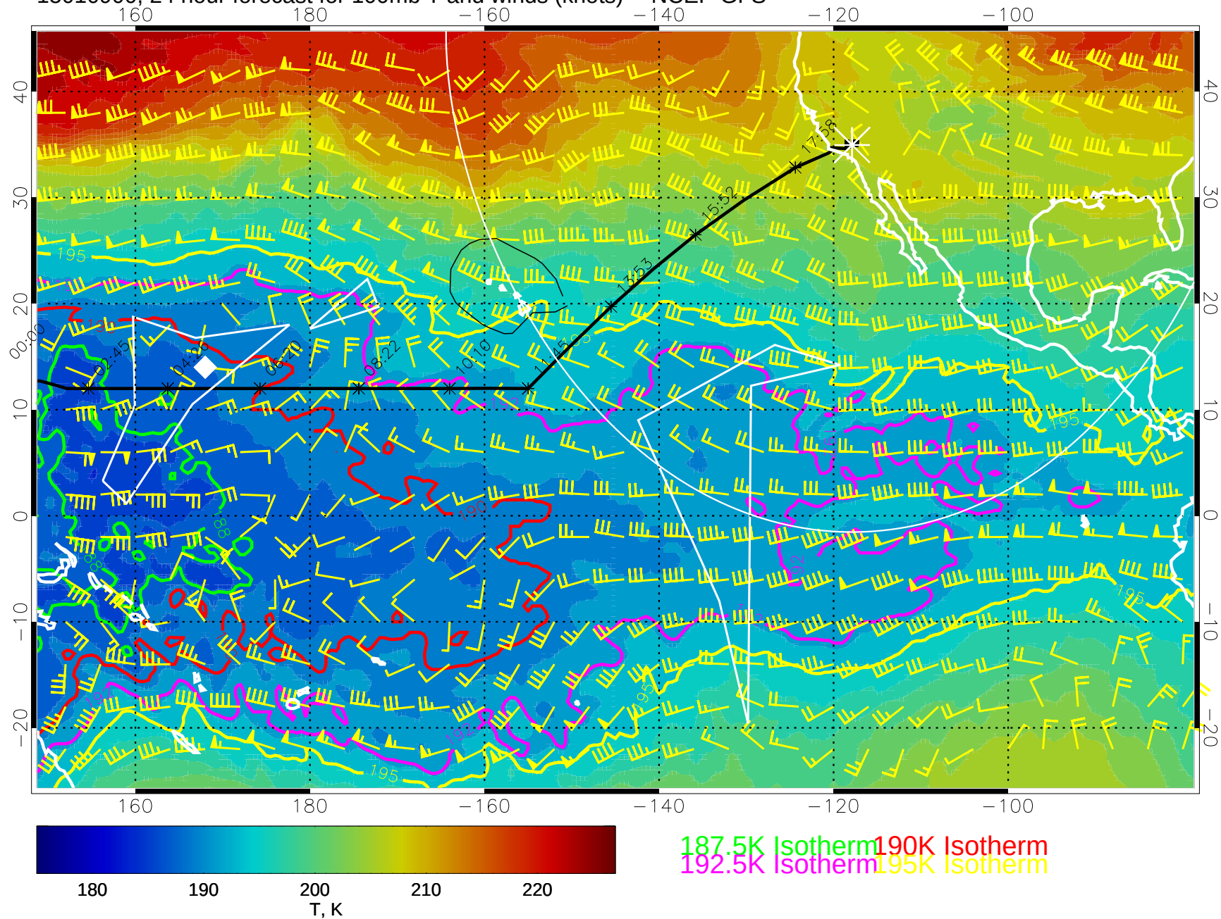
15010900, 24 hour forecast for 100mb T and winds (knots) -- NCEP GFS
