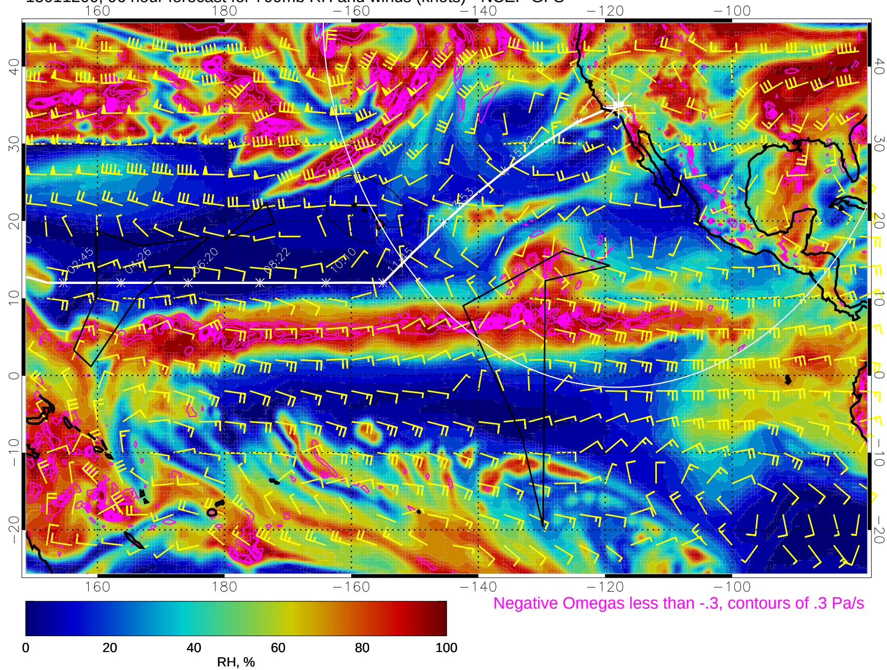
15011200, 96 hour forecast for 700mb RH and winds (knots) - NCEP GFS
