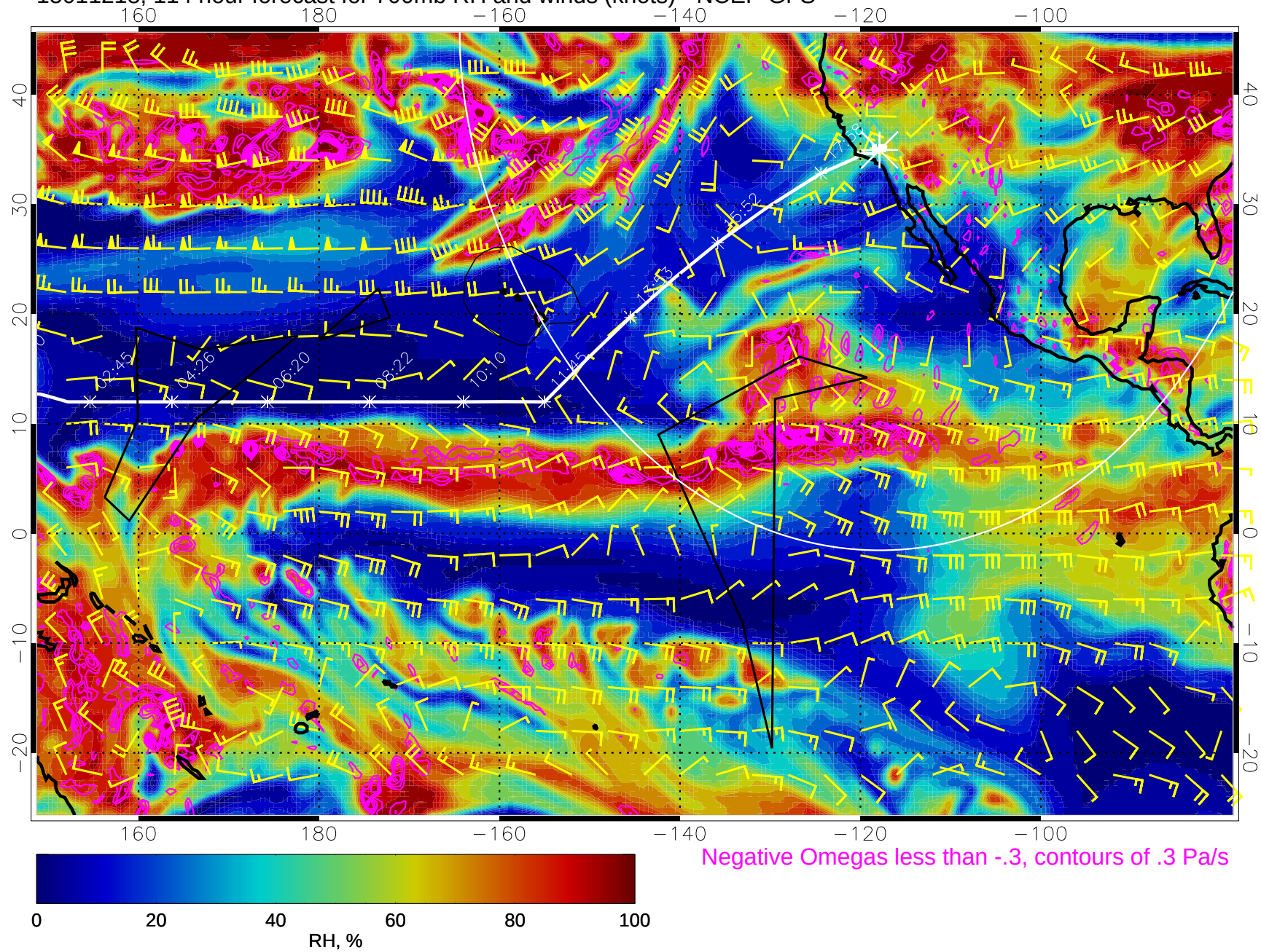
15011218, 114 hour forecast for 700mb RH and winds (knots) - NCEP GFS
