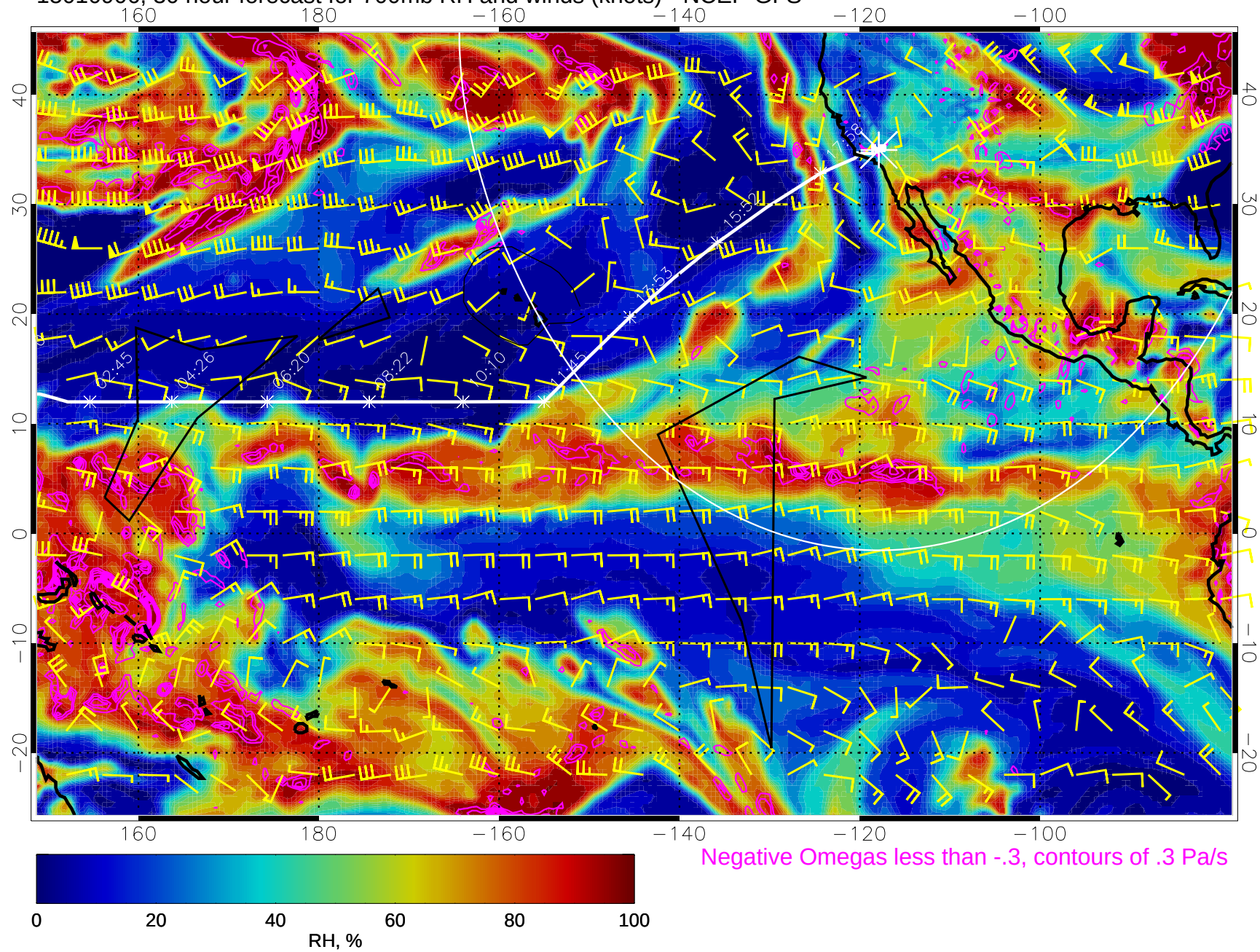
15010906, 30 hour forecast for 700mb RH and winds (knots) - NCEP GFS
