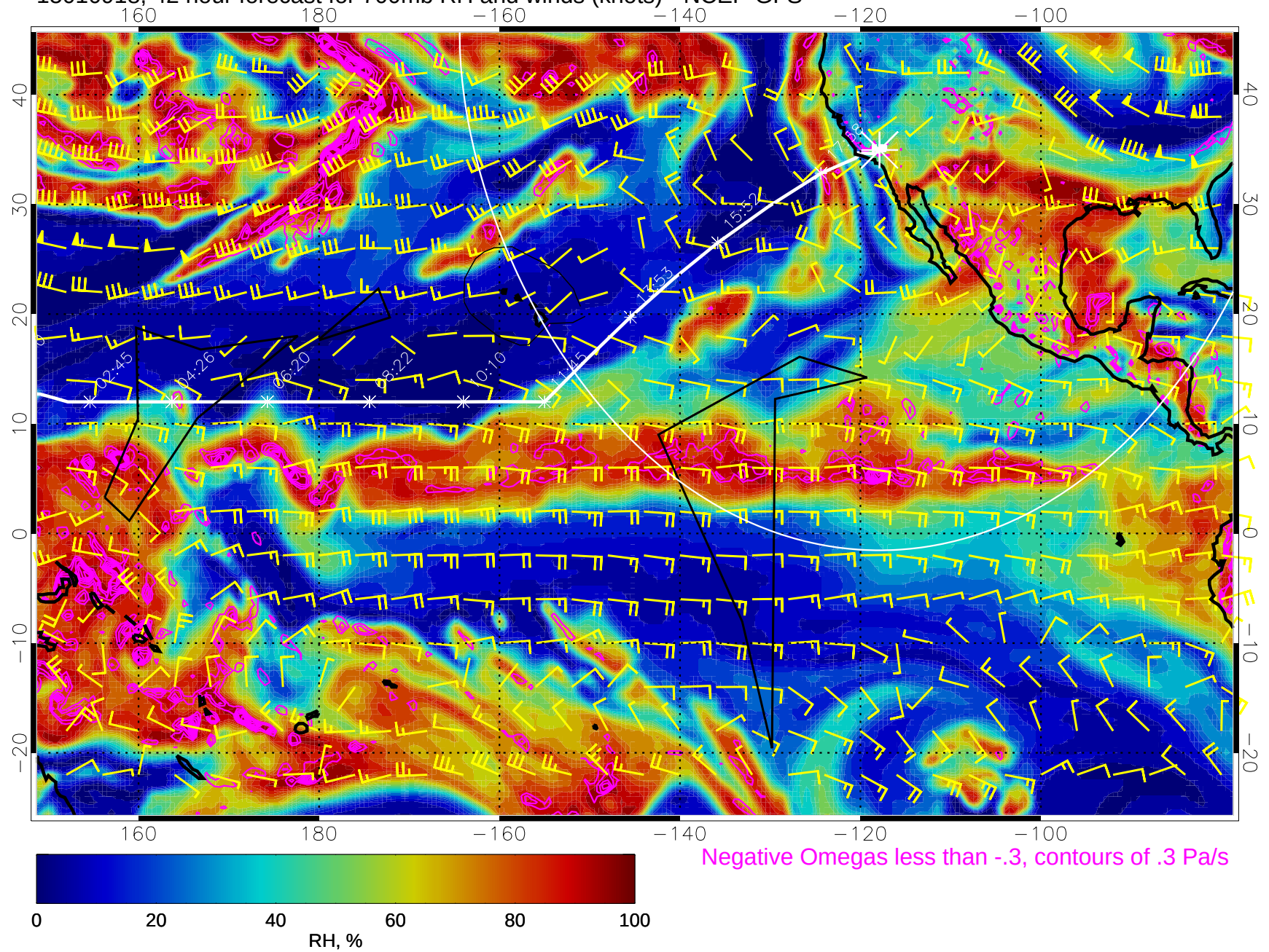
15010918, 42 hour forecast for 700mb RH and winds (knots) - NCEP GFS
