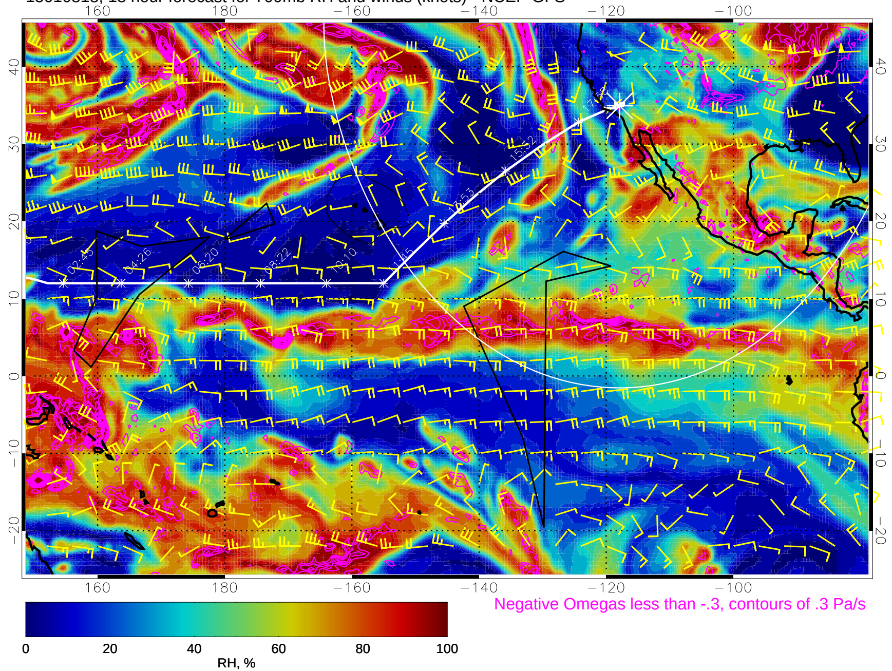
15010818, 18 hour forecast for 700mb RH and winds (knots) - NCEP GFS
