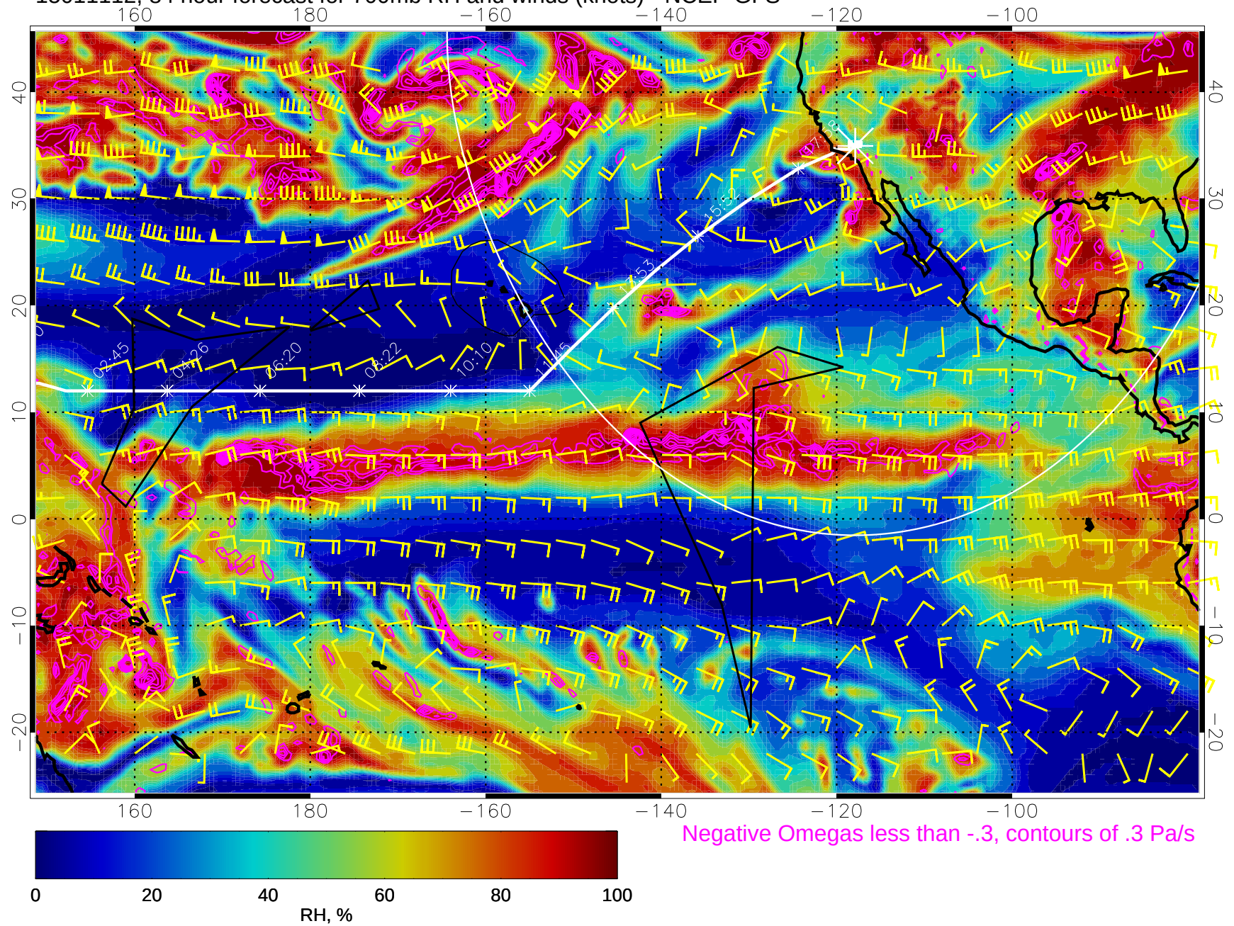
15011112, 84 hour forecast for 700mb RH and winds (knots) - NCEP GFS
