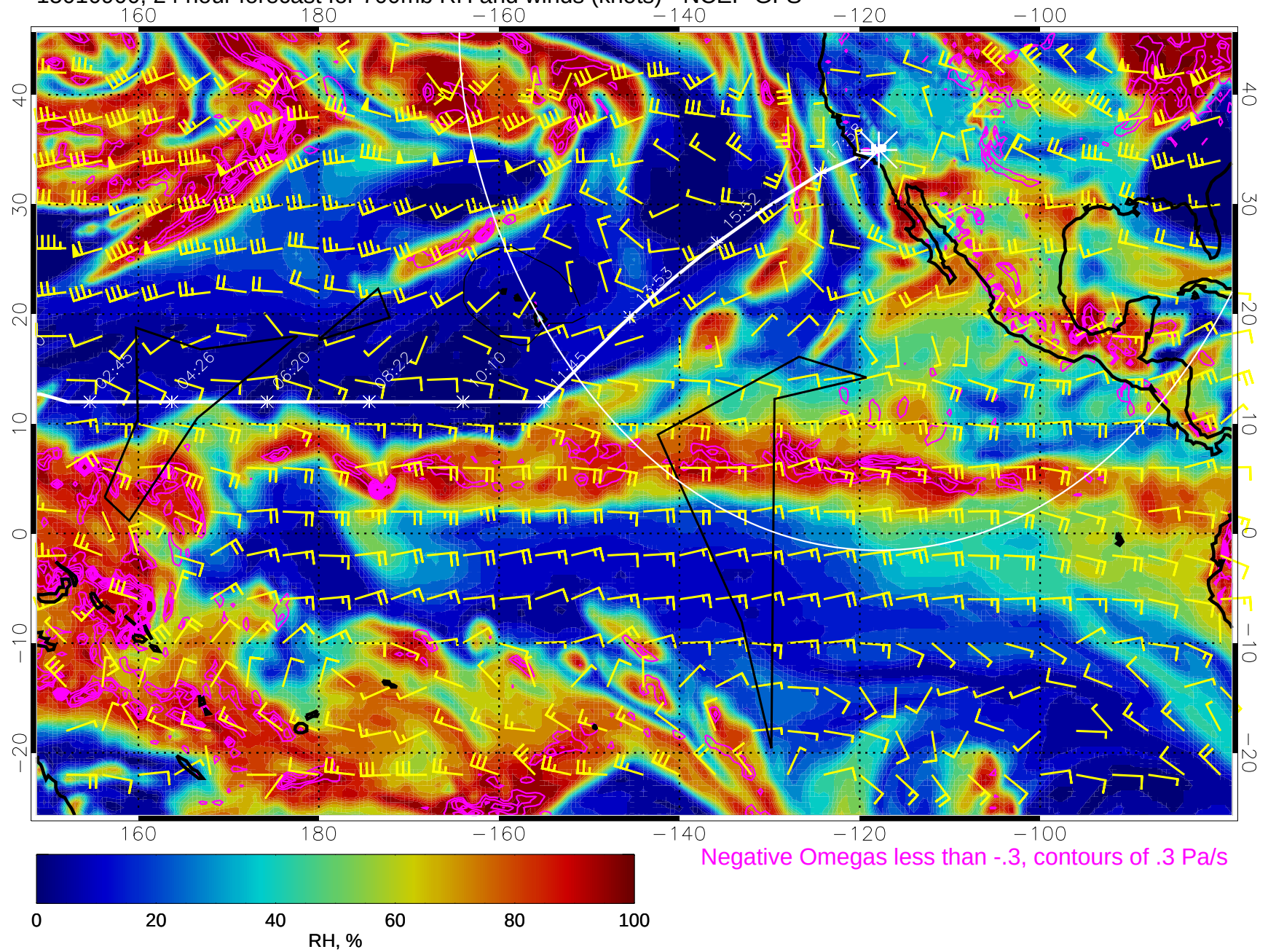
15010900, 24 hour forecast for 700mb RH and winds (knots) - NCEP GFS
