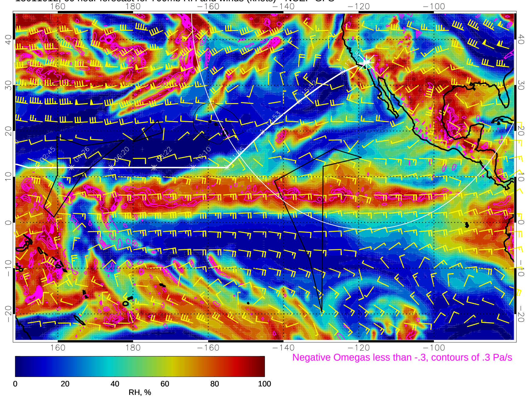
15011012, 60 hour forecast for 700mb RH and winds (knots) - NCEP GFS
