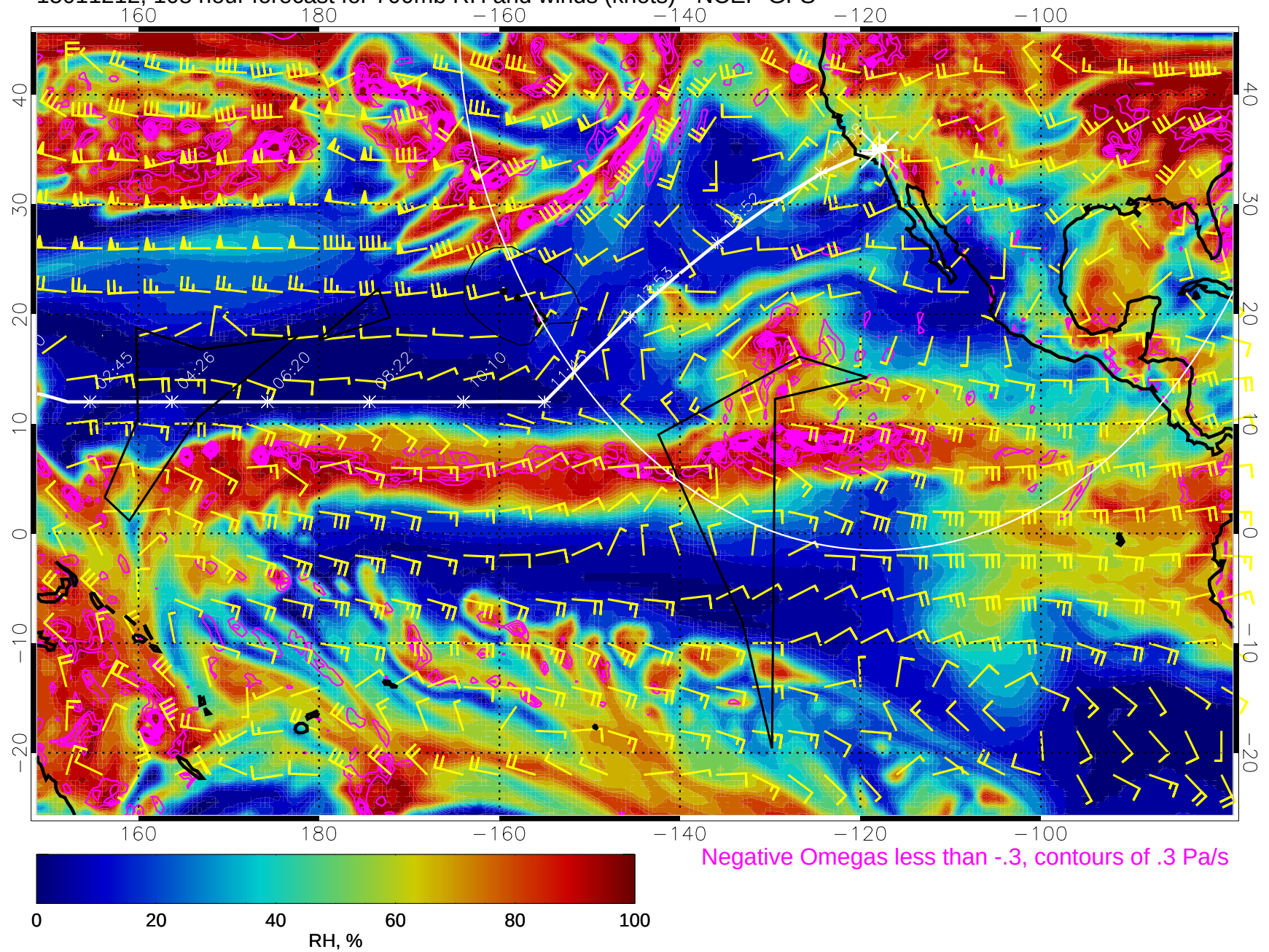
15011212, 108 hour forecast for 700mb RH and winds (knots) - NCEP GFS
