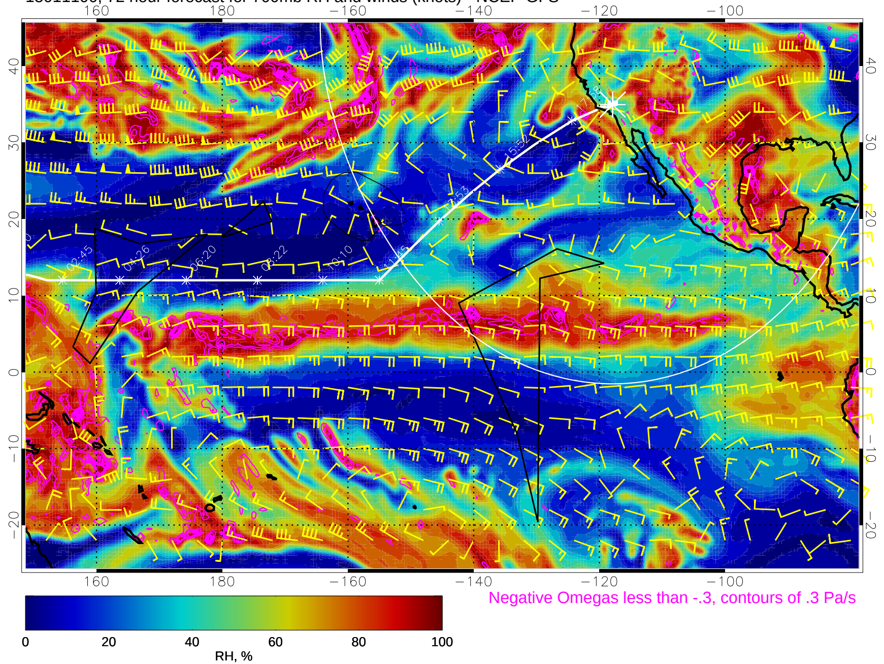
15011100, 72 hour forecast for 700mb RH and winds (knots) - NCEP GFS
