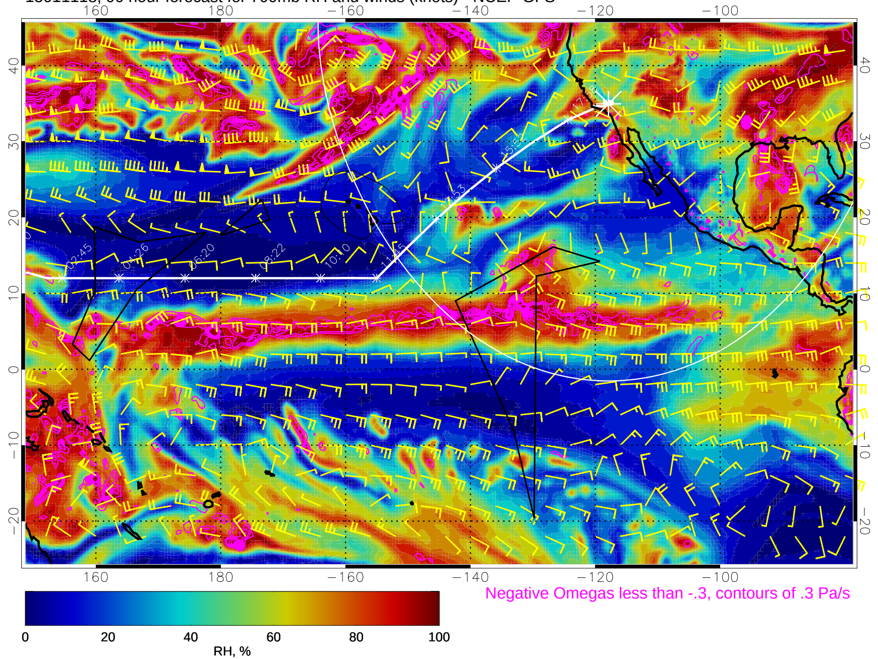
15011118, 90 hour forecast for 700mb RH and winds (knots) - NCEP GFS
