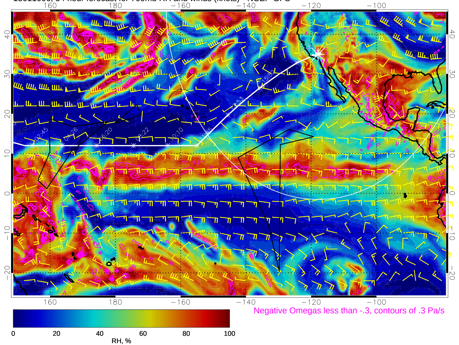
15011006, 54 hour forecast for 700mb RH and winds (knots) - NCEP GFS
