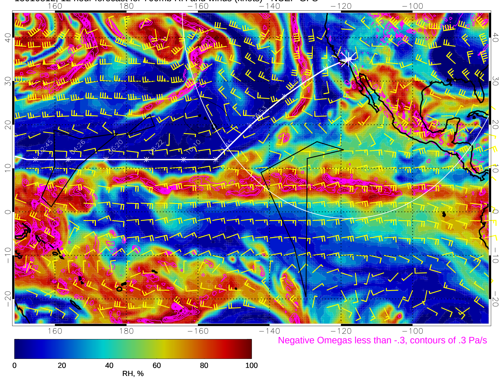
15010812, 12 hour forecast for 700mb RH and winds (knots) - NCEP GFS
