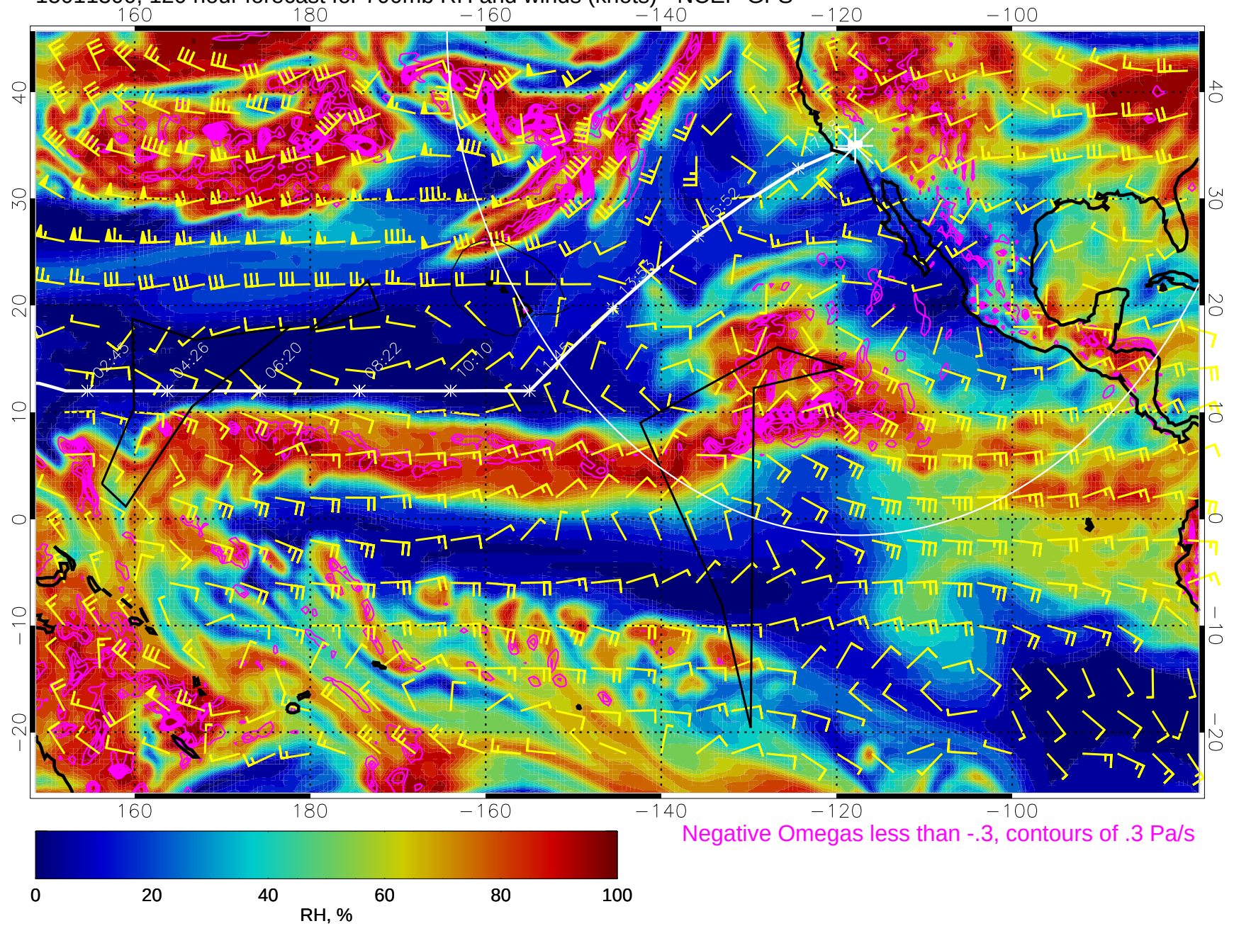
15011300, 120 hour forecast for 700mb RH and winds (knots) - NCEP GFS
