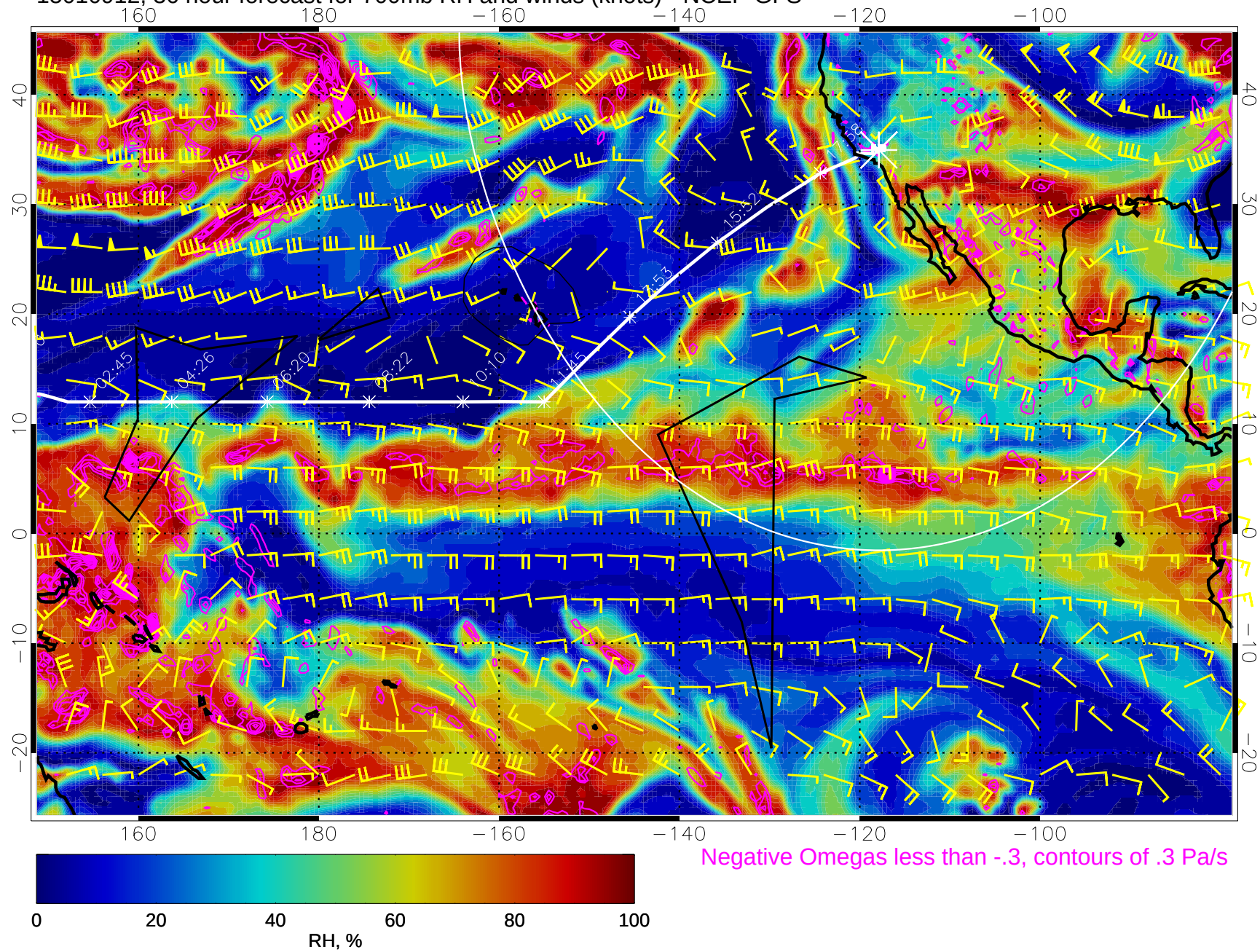
15010912, 36 hour forecast for 700mb RH and winds (knots) - NCEP GFS
